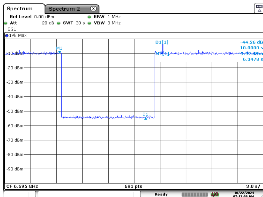
Plot 7-90. Contention Based Protocol Timing Plot (20MHz (UNII Band 7) – Ch. 149)
