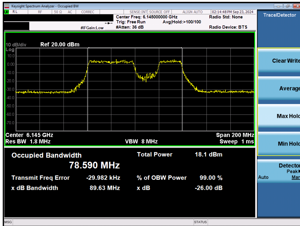
Plot 7-7. 26dB Bandwidth Plot MIMO ANT1 (80MHz 802.11be (484+242 Tones) (UNII Band 5) – Ch. 39) VLP
