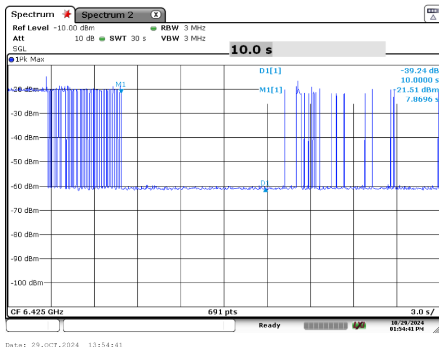
Plot 7-88. Contention Based Protocol Timing Plot (320MHz (UNII Band 5) – Ch. 47 Mid)
