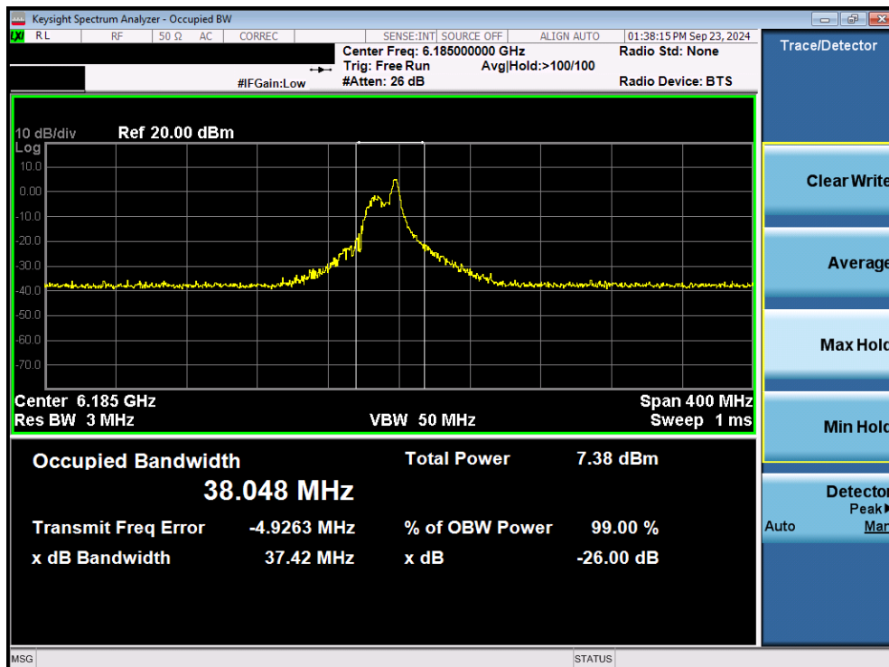
Plot 7-4. 26dB Bandwidth Plot MIMO ANT1 (160MHz 802.11ax/be (26 Tones) (UNII Band 5) – Ch. 47) - VLP
