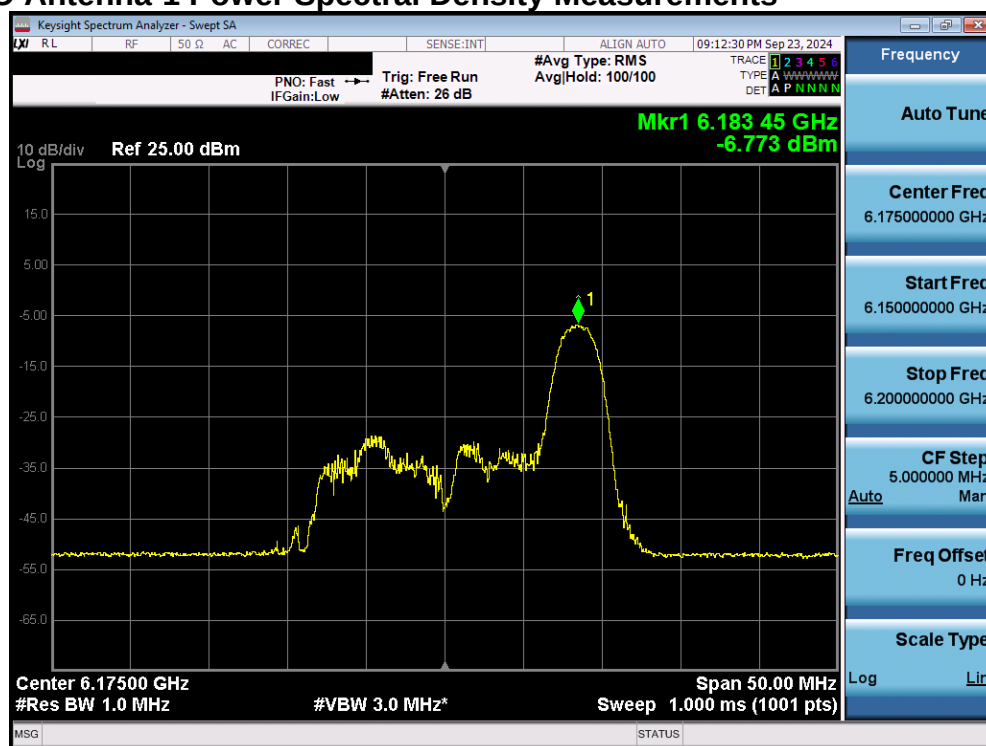
Plot 7-29. Power Spectral Density Plot MIMO ANT1 (20MHz 802.11ax/be (26 Tones) (UNII Band 5) – Ch. 45) - VLP
