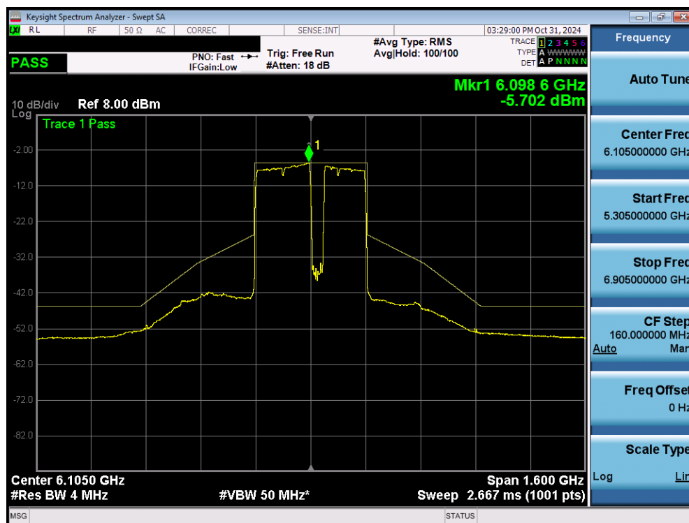
Plot 7-65. In Band Emissions Plot MIMO ANT1 (320MHz 802.11be (3*996+484 Tones) (UNII Band 5) – Ch. 31) VLP
