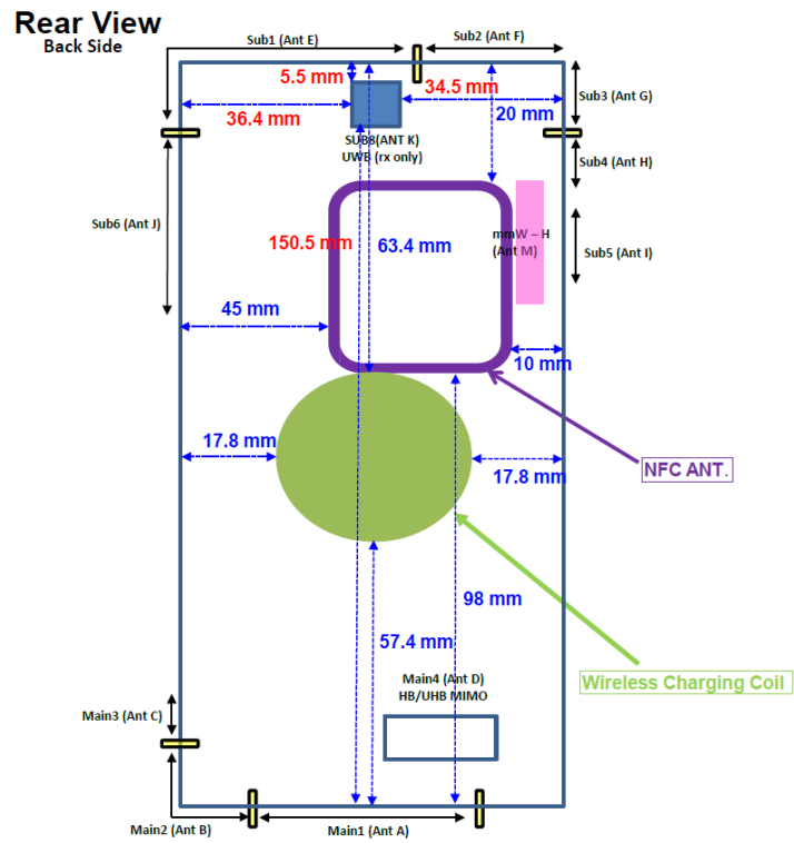
Figure J-2 NFC Antenna Locations
