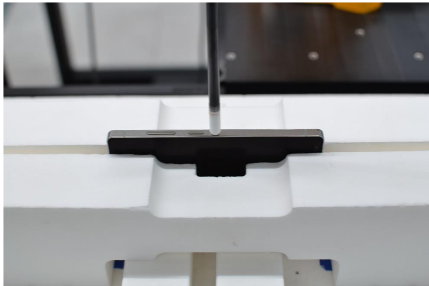
SAR Test Setup Photo 24 – PD, Right Edge at 2mm
