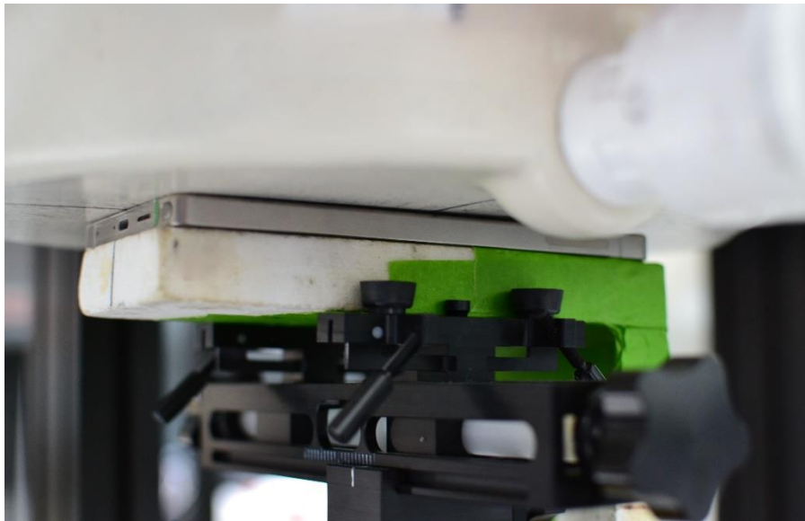
SAR Test Setup Photo 6 – Phablet, Back Side at 0mm
