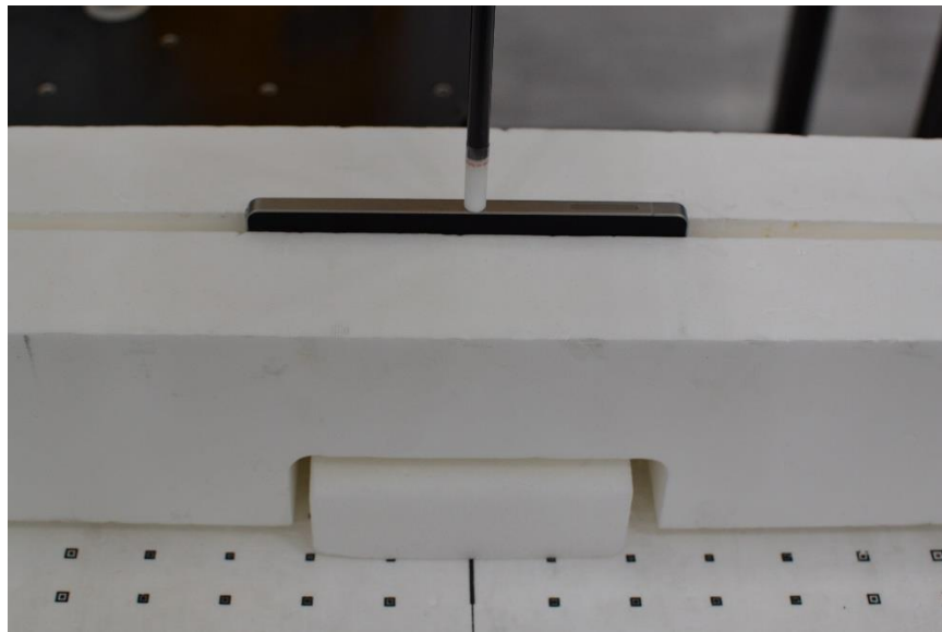
SAR Test Setup Photo 22 – PD, Left Edge at 2mm
