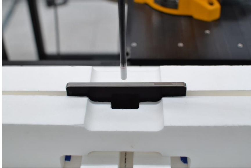
SAR Test Setup Photo 23 – PD, Left Edge at 8.58mm
