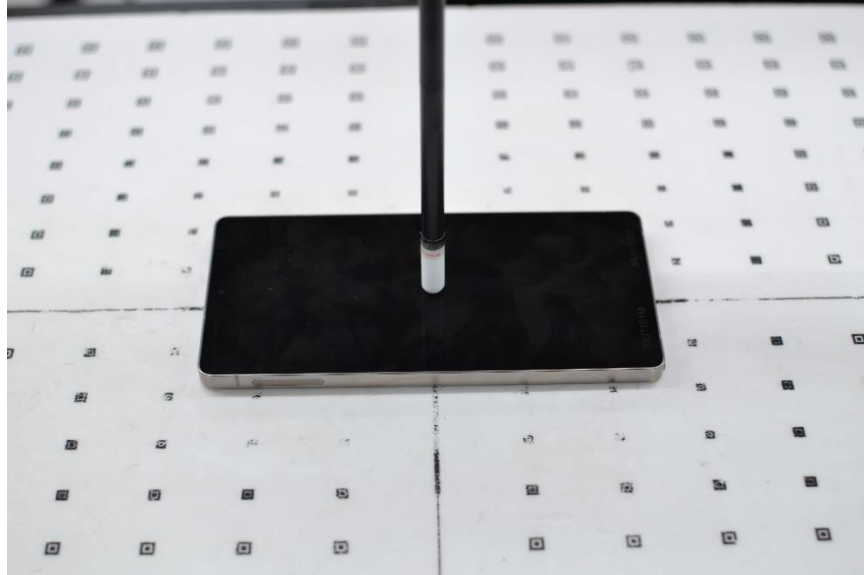
SAR Test Setup Photo 19 – PD, Front Side at 2mm
