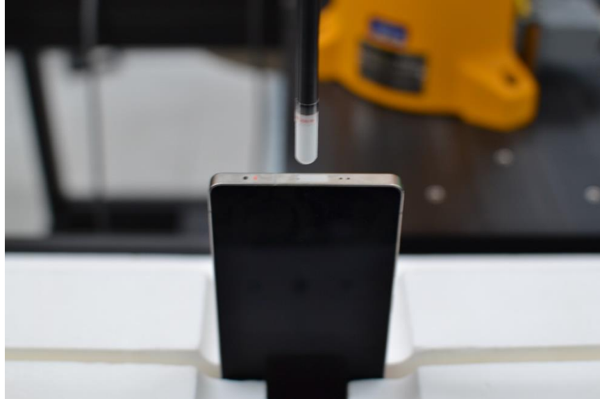
SAR Test Setup Photo 21 – PD, Top Edge at 9.24mm
