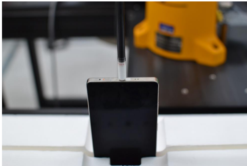
SAR Test Setup Photo 20 – PD, Top Edge at 2mm
