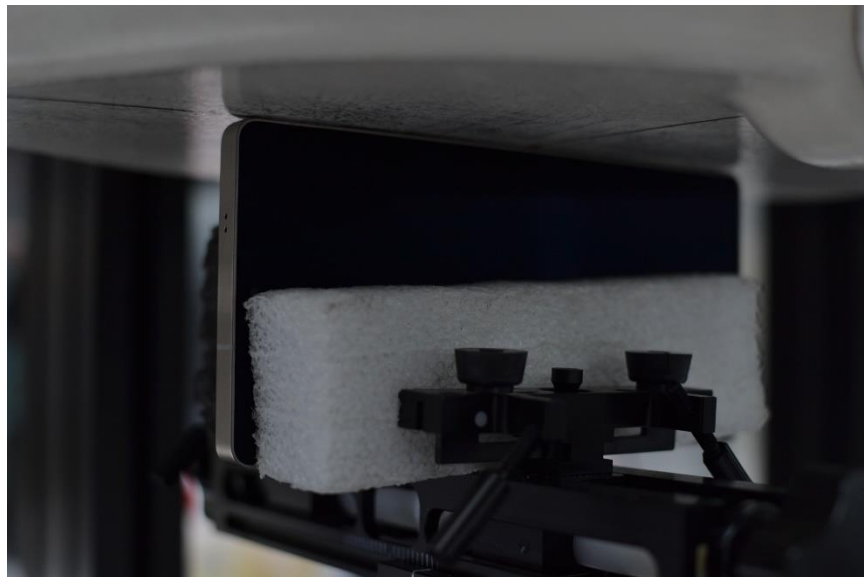
SAR Test Setup Photo 14 – Phablet, Right Edge at 0mm
