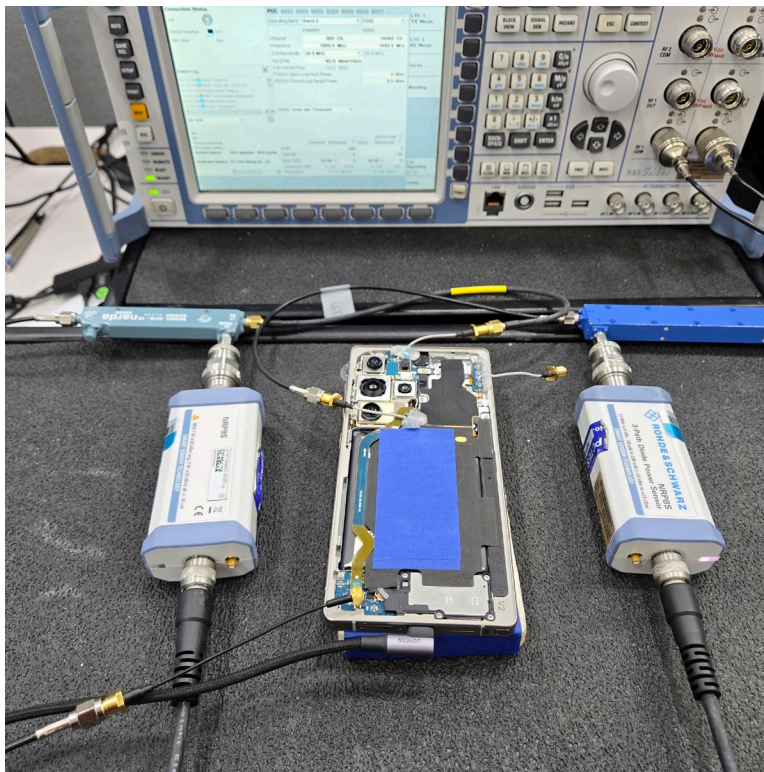
Test Setup Photo 10 – Conducted Test Setup (Figure 6-1e)
