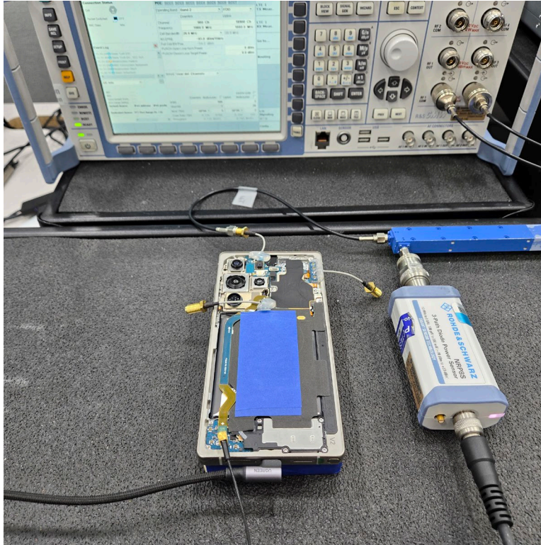
Test Setup Photo 9 – Conducted Test Setup (Figure 6-1d)
