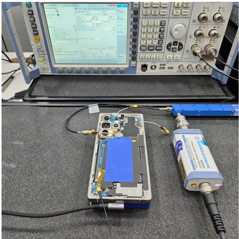
Test Setup Photo 8 – Conducted Test Setup (Figure 6-1d)
