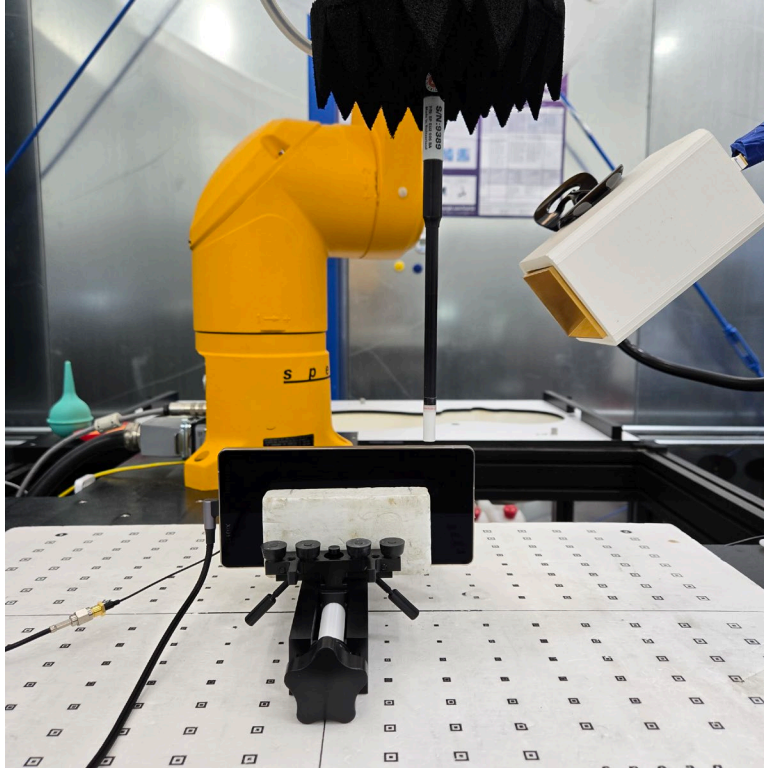
Test Setup Photo 13 – Conducted Test Setup (Figure 7-2)
