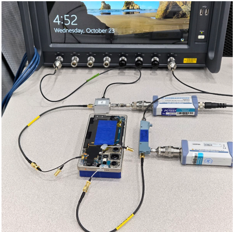
Test Setup Photo 7 – Conducted Test Setup (Figure 6-1c)
