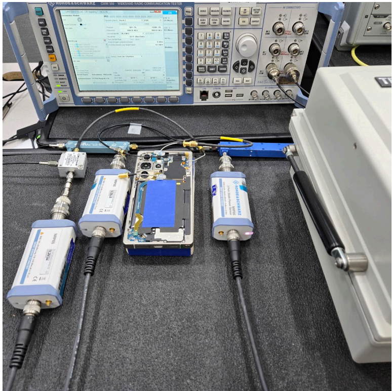
Test Setup Photo 11 – Conducted Test Setup (Figure 6-1f)
