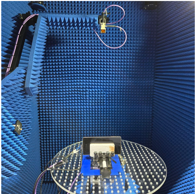
Test Setup Photo 12 – Conducted Test Setup (Figure 7-1)
