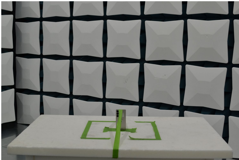
Figure 10. Test Setup – Z Position – 30MHz-1GHz
