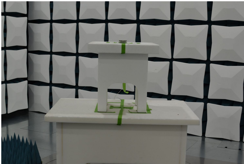
Figure 6. Test Setup – Wireless Charging Pad – 1GHz-40GHz
