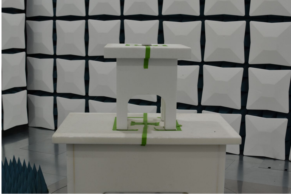
Figure 3. Test Setup – X Position – 1GHz-40GHz
