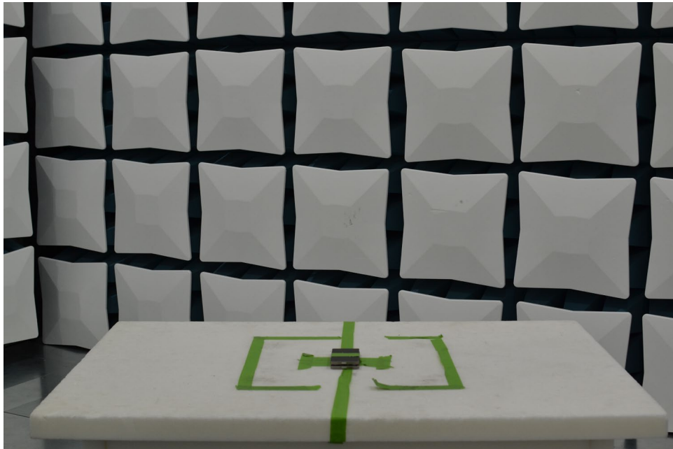
Figure 13. Test Setup – Wireless Power Transfer – 30MHz-1GHz – Z
