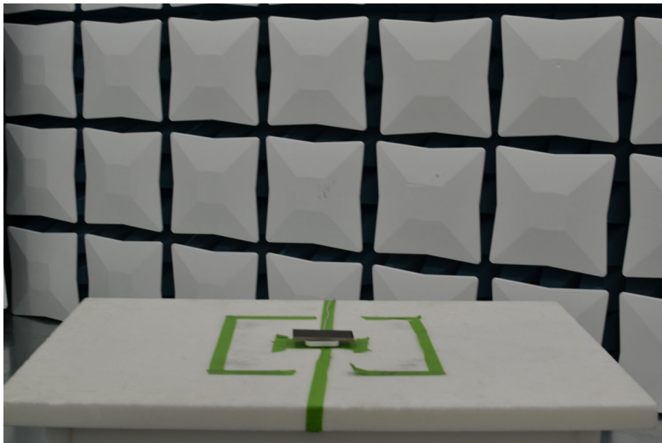
Figure 12. Test Setup – Wireless Charging Pad – 30MHz-1GHz
