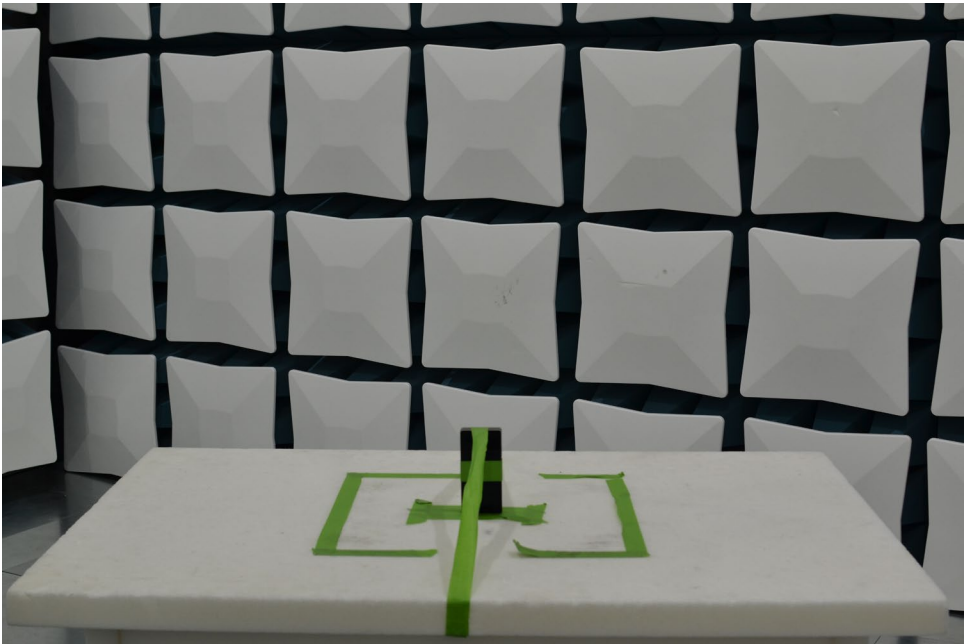
Figure 15. Test Setup –Wireless Power Transfer – 30MHz-1GHz – Z
