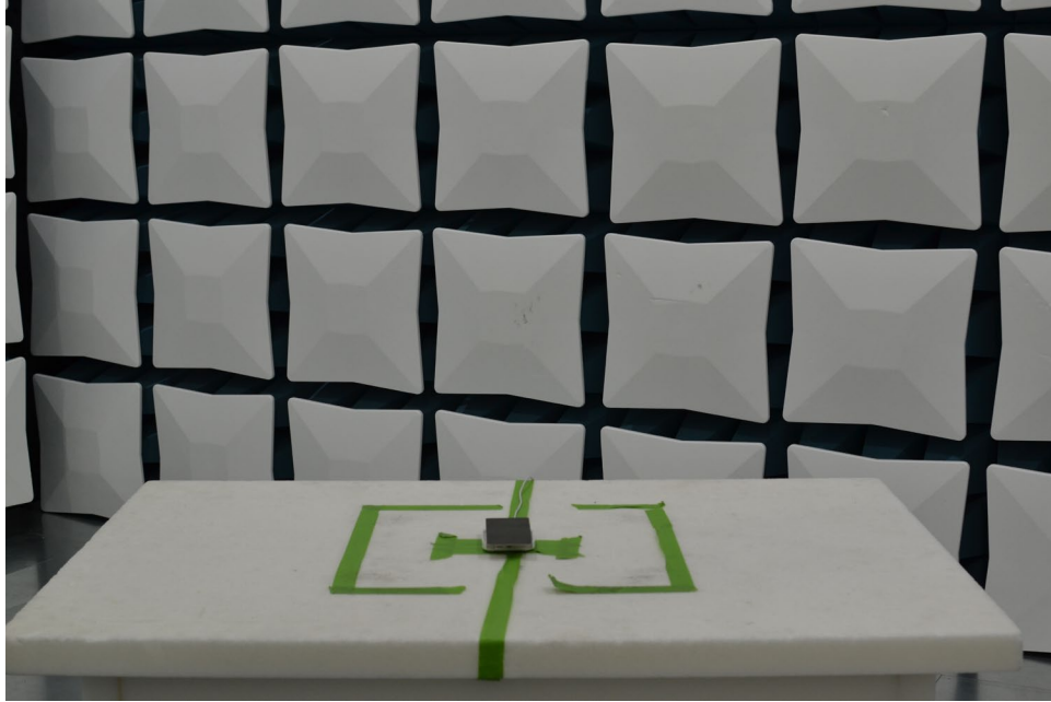
Figure 11. Test Setup – Wireless Charging Pad – 30MHz-1GHz
