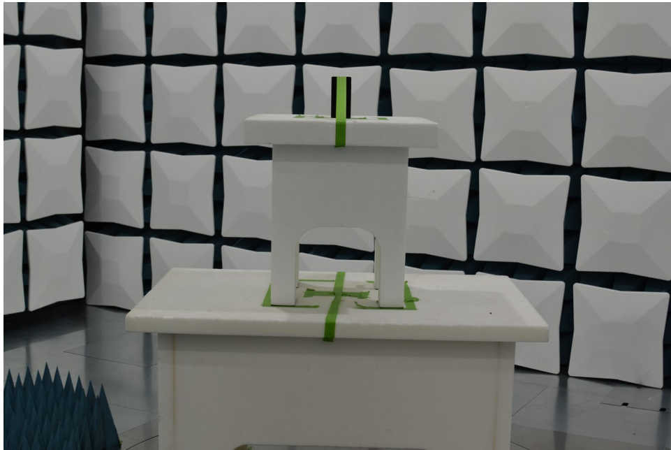
Figure 5. Test Setup – Z Position – 1GHz-40GHz
