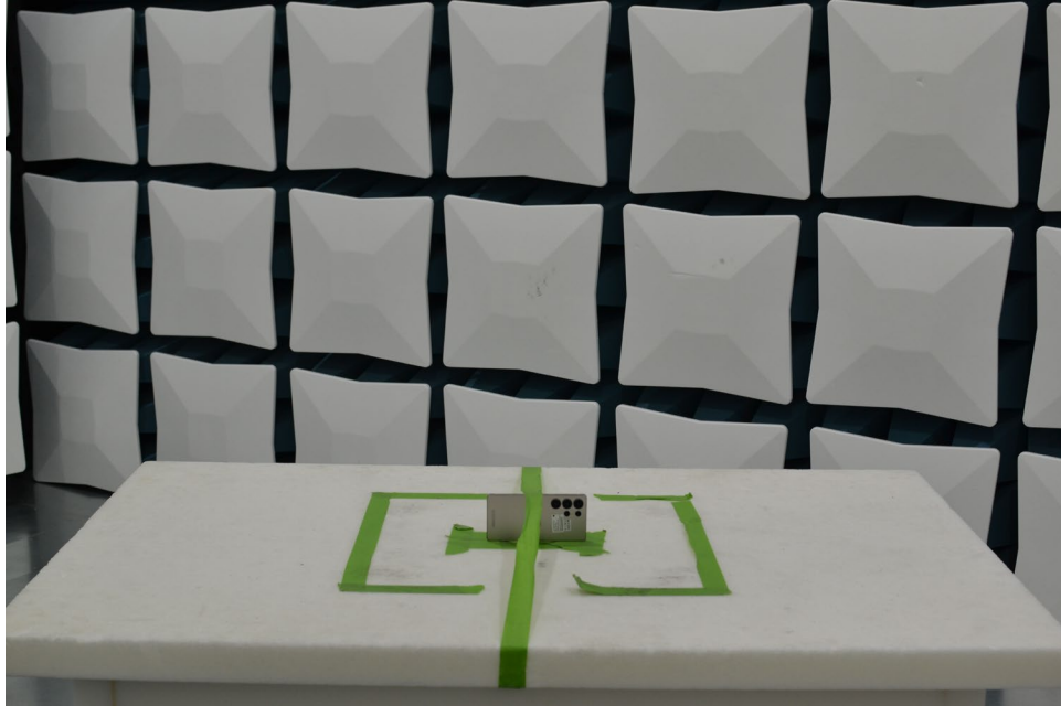
Figure 9. Test Setup – Y Position – 30MHz-1GHz
