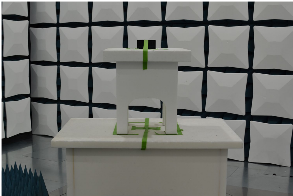
Figure 4. Test Setup – Y Position – 1GHz-40GHz
