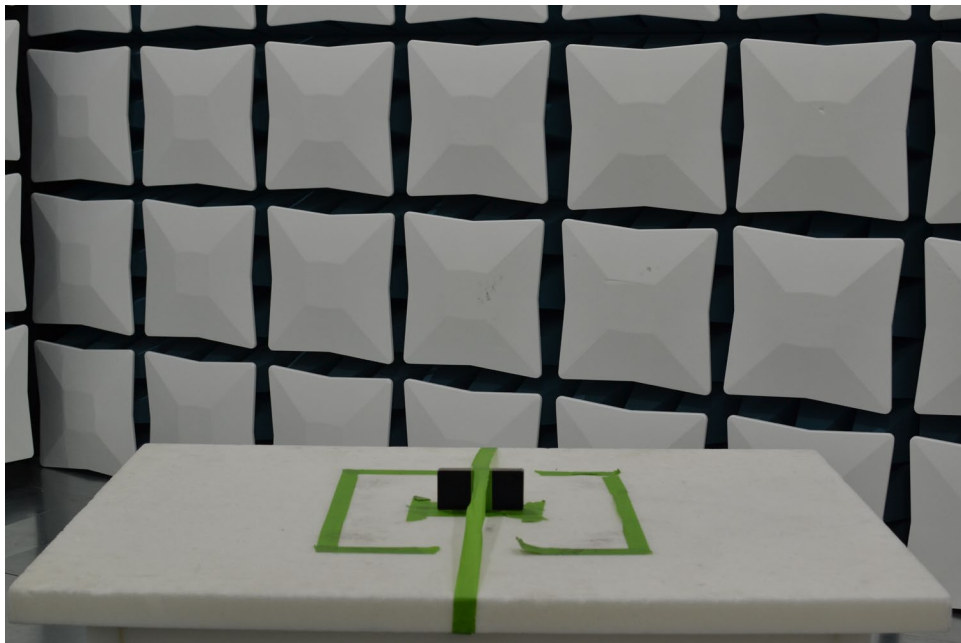
Figure 14. Test Setup – Wireless Power Transfer – 30MHz-1GHz – Y
