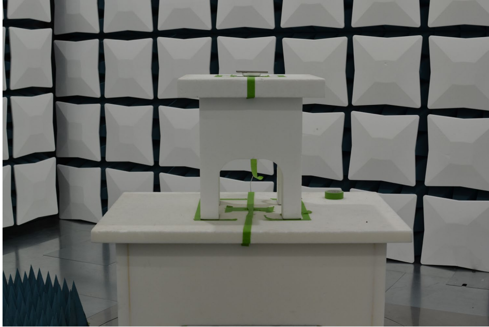
Figure 7. Test Setup – Wireless Charging Pad – 1GHz-40GHz
