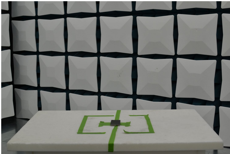
Figure 8. Test Setup – X Position – 30MHz-1GHz
