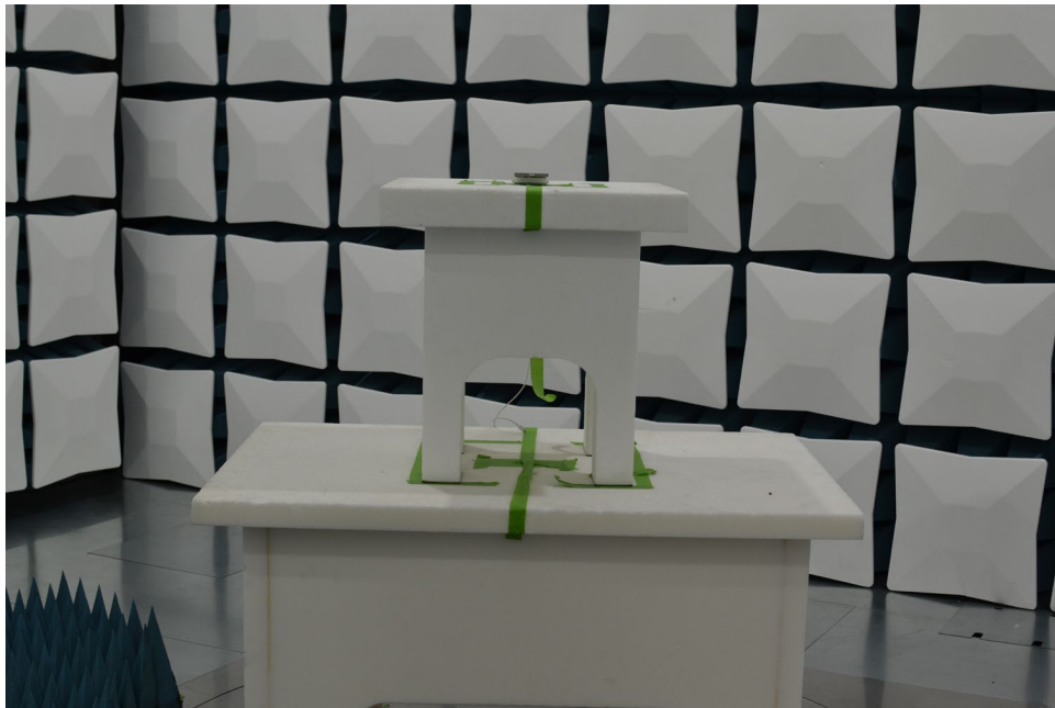
Figure 8. Test Setup – Wireless Charging Pad – 1GHz-40GHz
