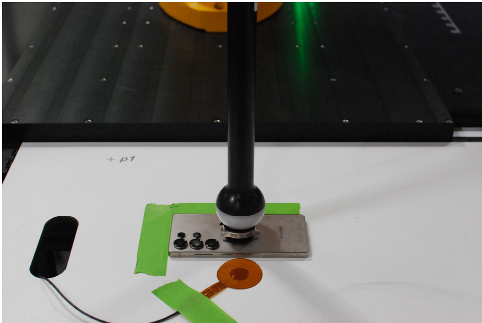
Test Setup Photo 10 Device to Watch, Back side, 0mm
