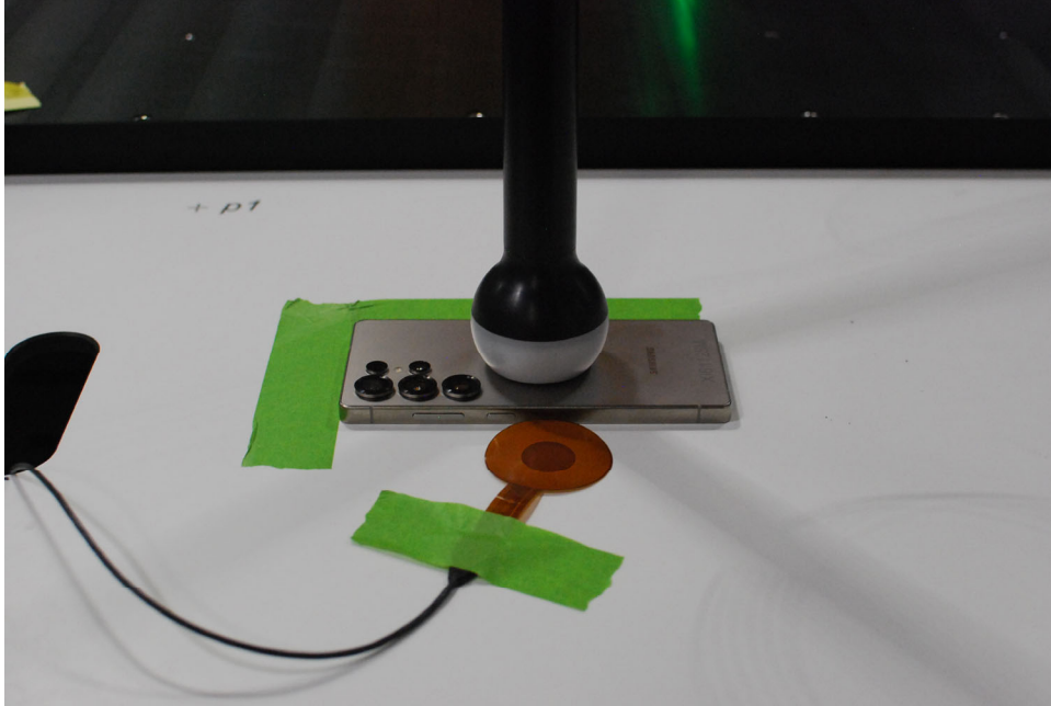
Test Setup Photo 11 Digitizer, Back side, 0mm
