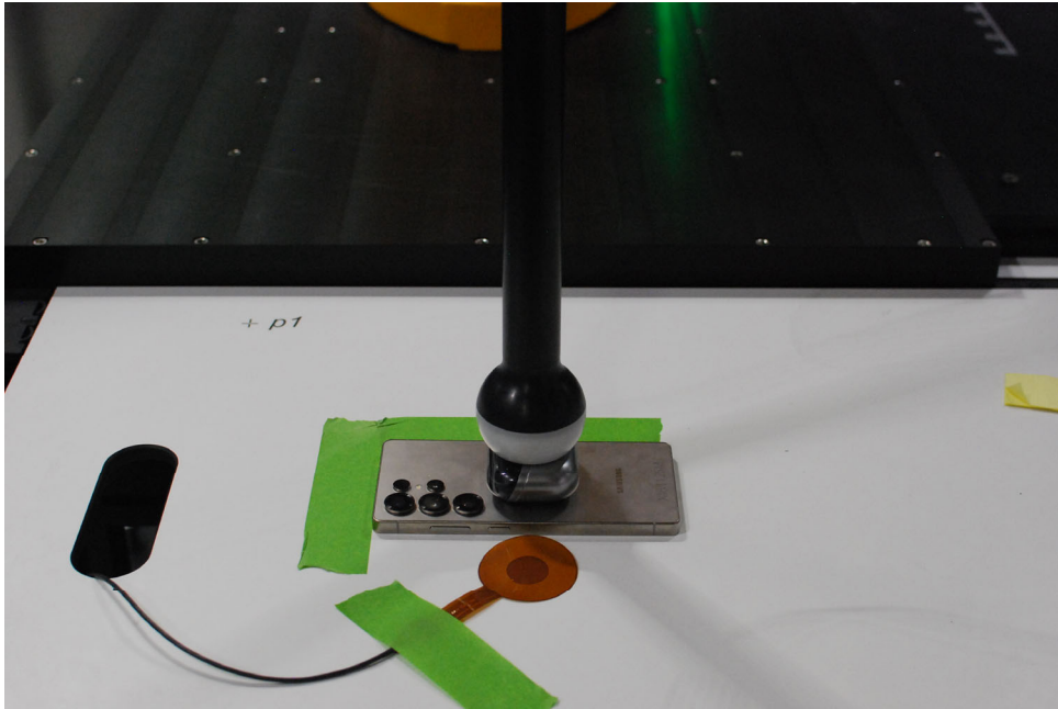
Test Setup Photo 9 Device to Earbuds, Back side, 0mm
