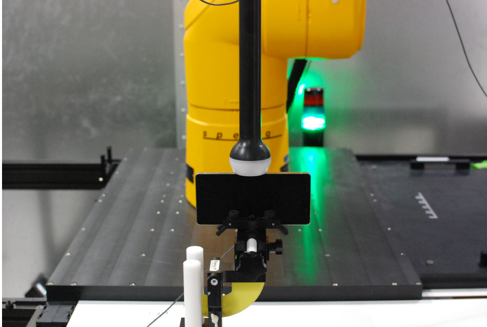
Test Setup Photo 5 Ping Signal, Right Side, 0mm
