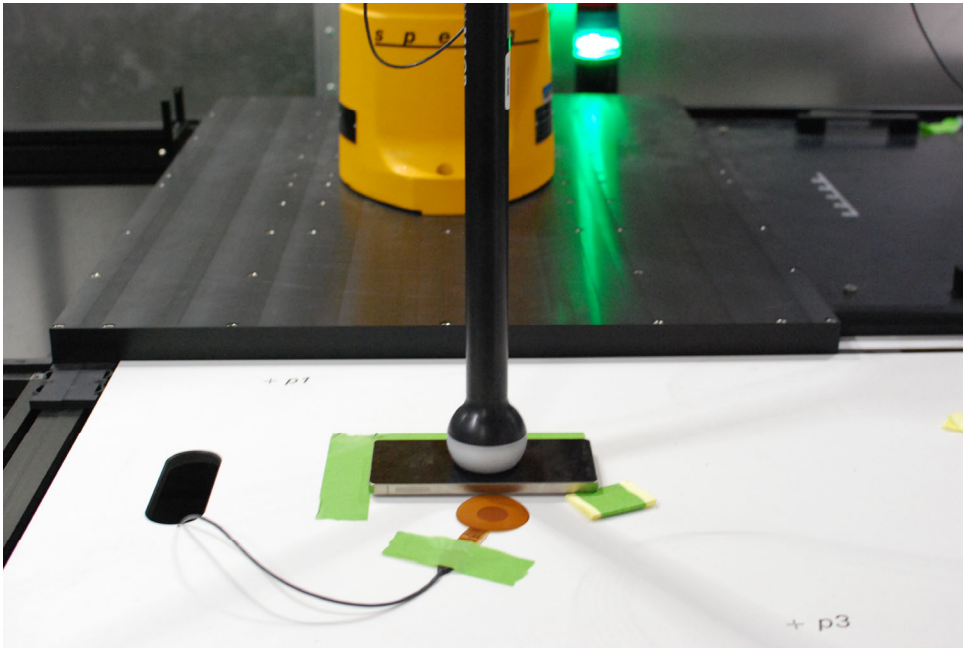
Test Setup Photo 2 Ping Signal, Front side, 0mm
