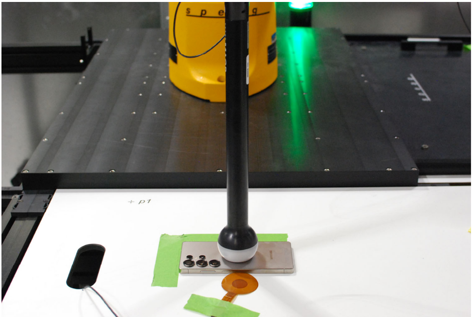
Test Setup Photo 1 Ping Signal, Back side, 0mm
