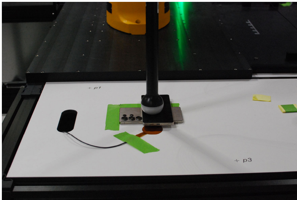
Test Setup Photo 8 Device to Device (Offset), Back side, 0mm
