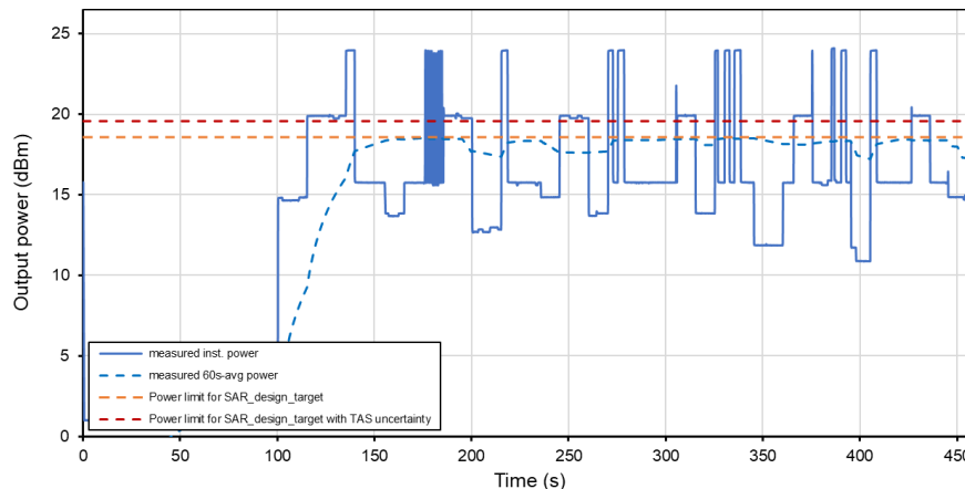
Time-Averaged Conducted Power Test Sequence B Tech: LTE, Band 13
