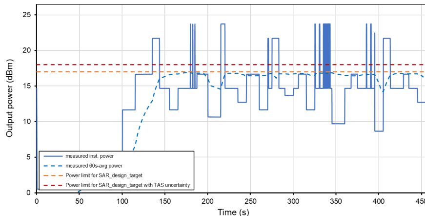
Time-Averaged Conducted Power Test Sequence B Tech: WCDMA, Band 2
