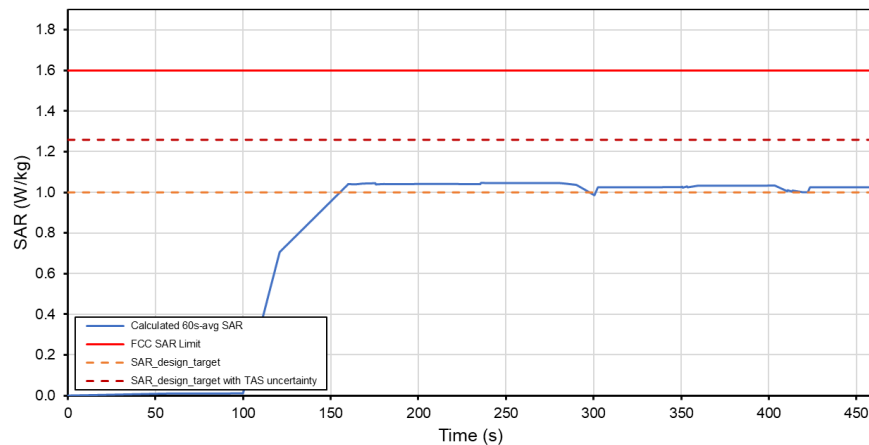
Total Time-Averaged SAR Test Sequence A Tech: NR, Band 26
