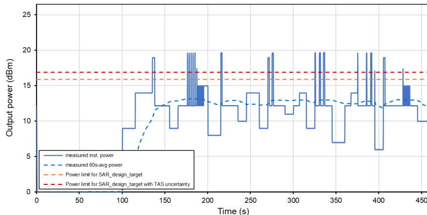
Time-Averaged Conducted Power Test Sequence B Tech: LTE, Band 41 PC3
