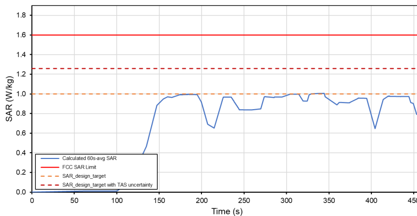
Total Time-Averaged SAR Test Sequence B Tech: NR, Band 26
