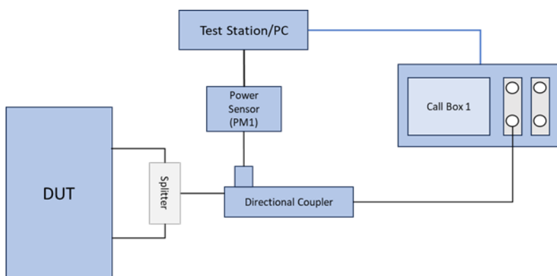
(b) Appendix A – Test Setup Photo 4
