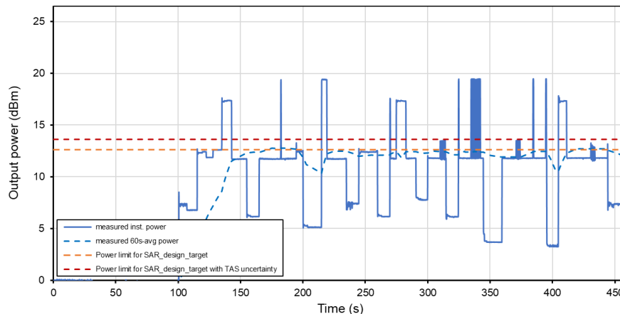
Time-Averaged Conducted Power Test Sequence B Tech: NR, Band n77 PC2
