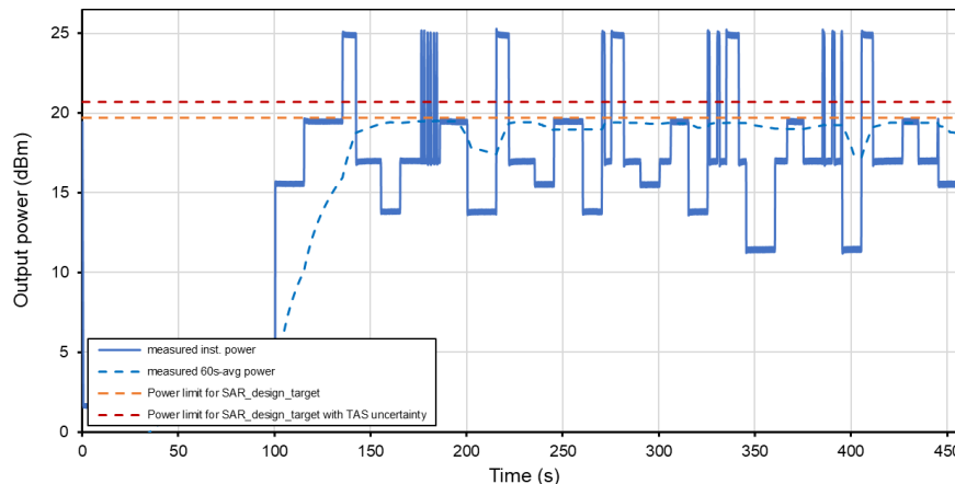
Time-Averaged Conducted Power Test Sequence B Tech: GSM, Band GSM850
