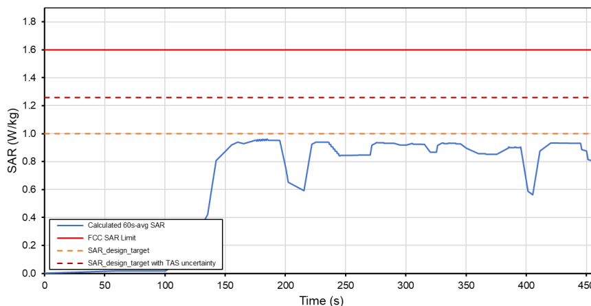
Total Time-Averaged SAR Test Sequence B Tech: GSM, Band GSM850
