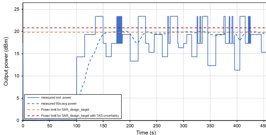
Time-Averaged Conducted Power Test Sequence B Tech: WCDMA, Band 5
