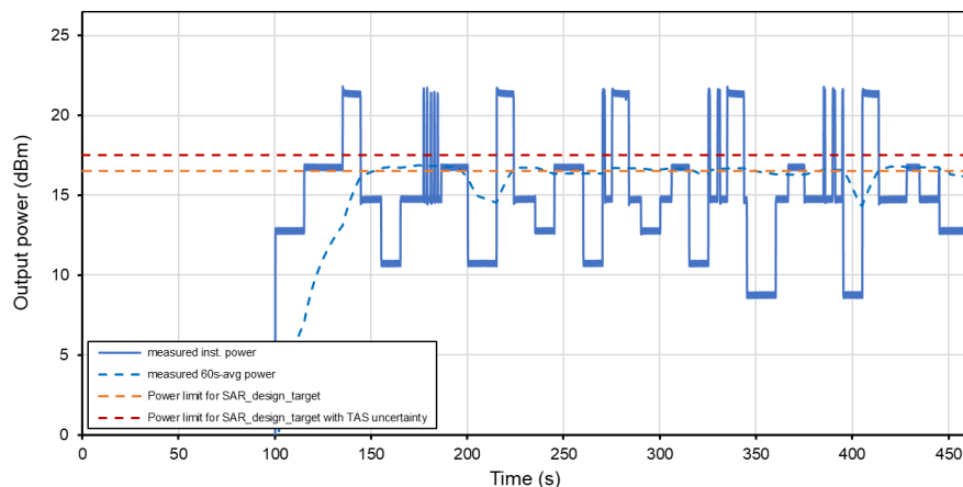
Time-Averaged Conducted Power Test Sequence B Tech: GSM, Band 1900
