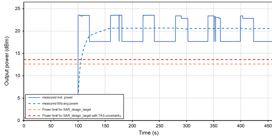
Time-Averaged Conducted Power Test Sequence A Tech: NR, Band 26
