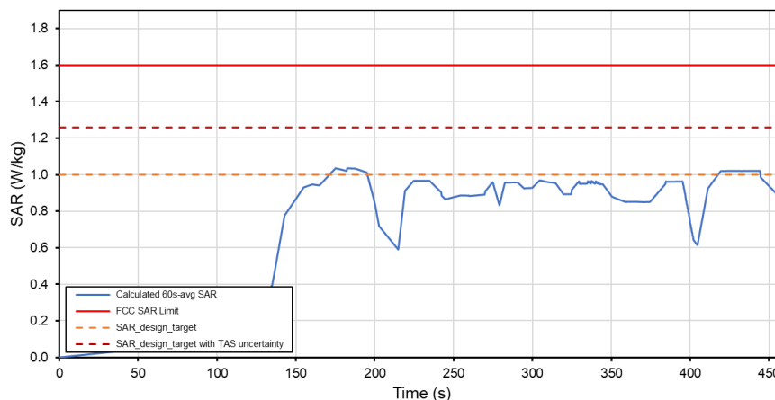
Total Time-Averaged SAR Test Sequence B Tech: NR, Band n77 PC2
