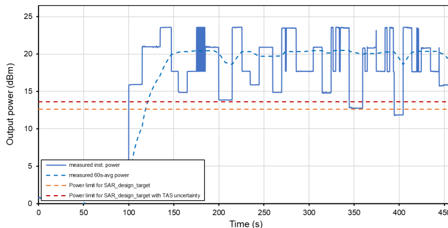
Time-Averaged Conducted Power Test Sequence B Tech: NR, Band 26
