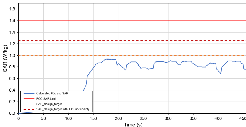
Total Time-Averaged SAR Test Sequence B Tech: LTE, Band 41 PC3
