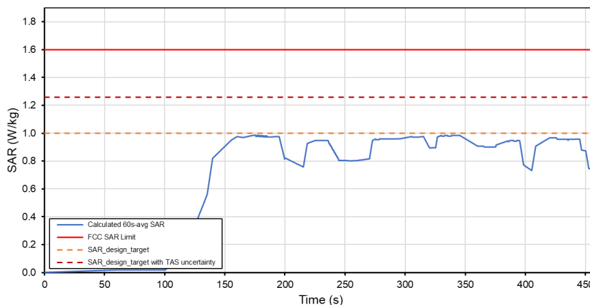
Total Time-Averaged SAR Test Sequence B Tech: LTE, Band 13
