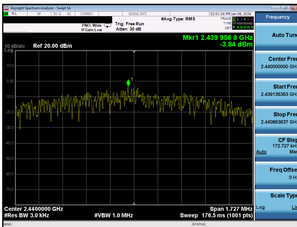
Plot 7-89. Power Spectral Density Plot (Bluetooth (LE), 2Mbps – Ch. 17) – Dual Ant 2
