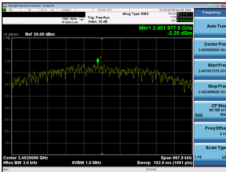
Plot 7-85. Power Spectral Density Plot (Bluetooth (LE), 1Mbps – Ch. 37) – Dual Ant 2
