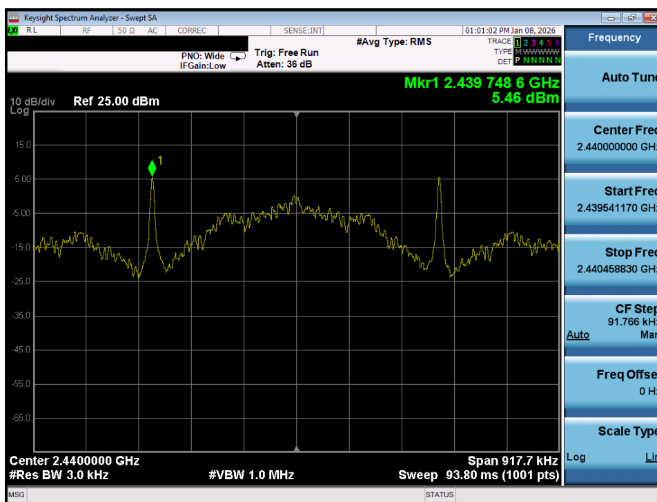
Plot 7-62. Power Spectral Density Plot (Bluetooth (LE), 125kbps – Ch. 17) – Ant 1
