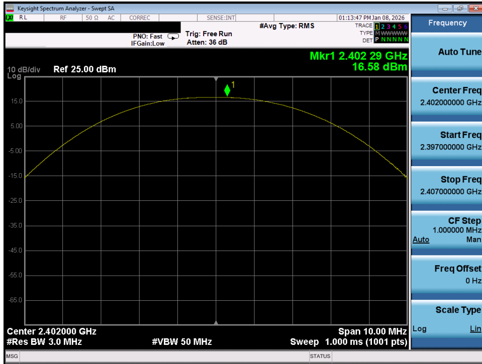
Plot 7-37. Peak Power Plot (Bluetooth (LE), 1Mbps – Ch. 37) – Ant 1
