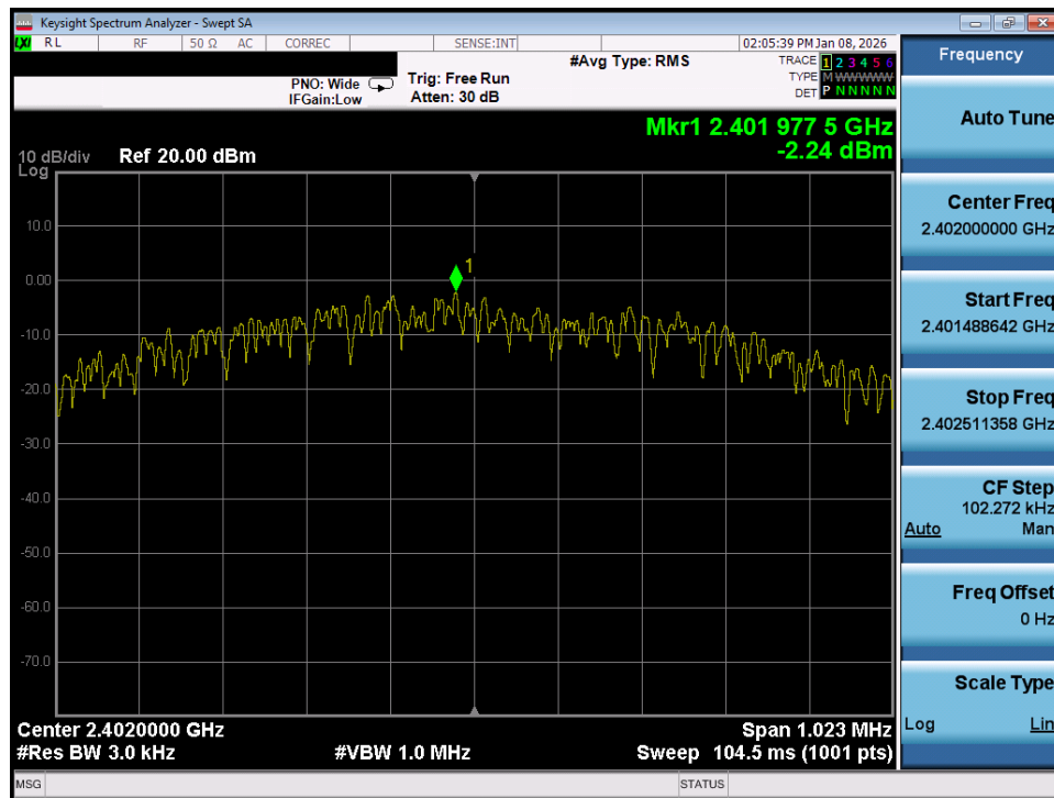
Plot 7-79. Power Spectral Density Plot (Bluetooth (LE), 1Mbps – Ch. 37) – Dual Ant 1
