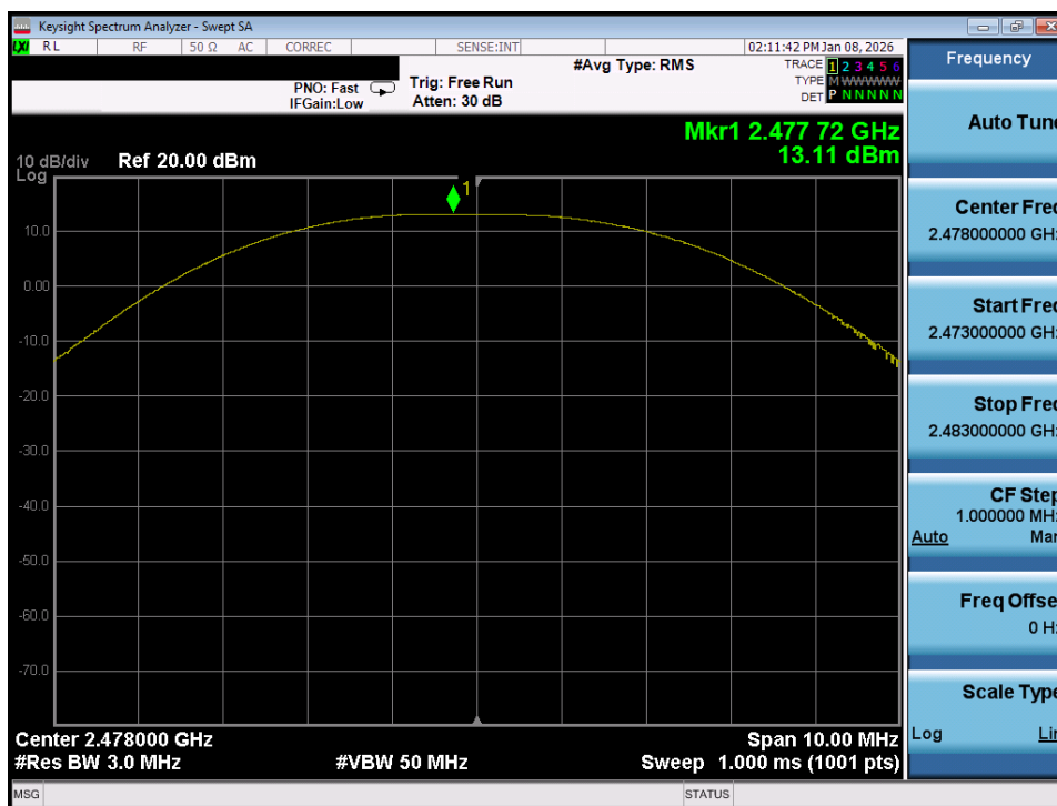
Plot 7-54. Peak Power Plot (Bluetooth (LE), 2Mbps – Ch. 36) – Dual Ant 1
