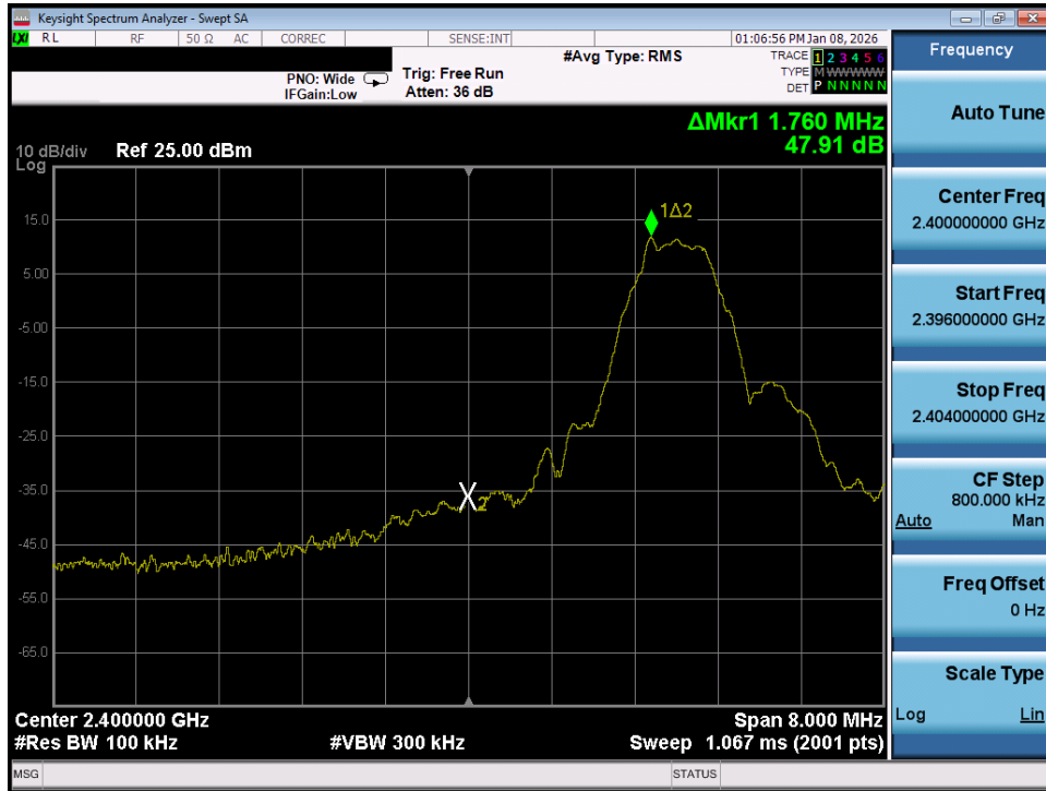
Plot 7-93. Band Edge Plot (Bluetooth (LE), 500kbps – Ch. 37) – Ant 1
