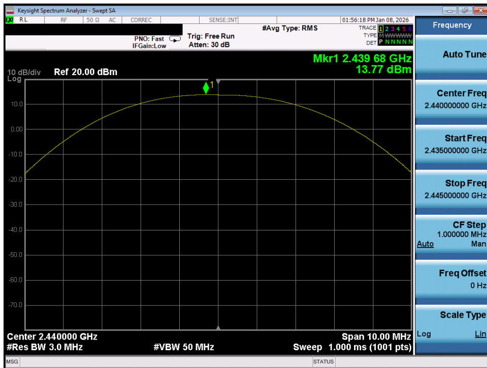
Plot 7-56. Peak Power Plot (Bluetooth (LE), 1Mbps – Ch. 17) – Dual Ant 2
