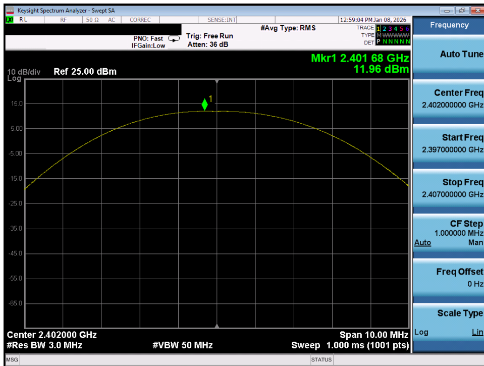
Plot 7-31. Peak Power Plot (Bluetooth (LE), 125kbps – Ch. 37) – Ant 1
