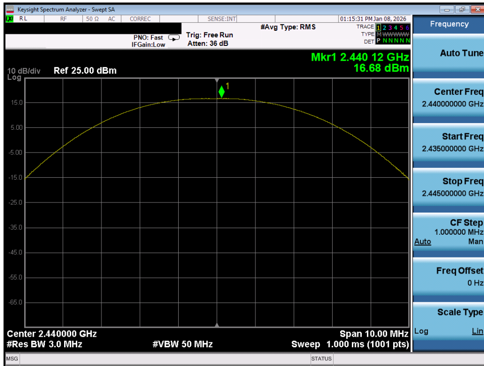
Plot 7-38. Peak Power Plot (Bluetooth (LE), 1Mbps – Ch. 17) – Ant 1
