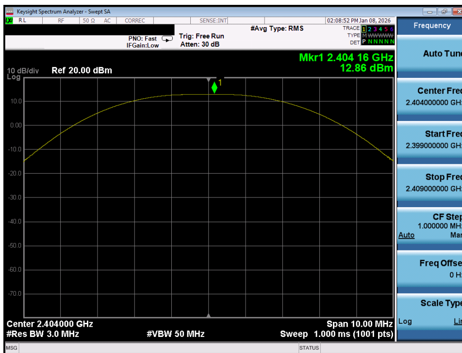
Plot 7-52. Peak Power Plot (Bluetooth (LE), 2Mbps – Ch. 0) – Dual Ant 1
