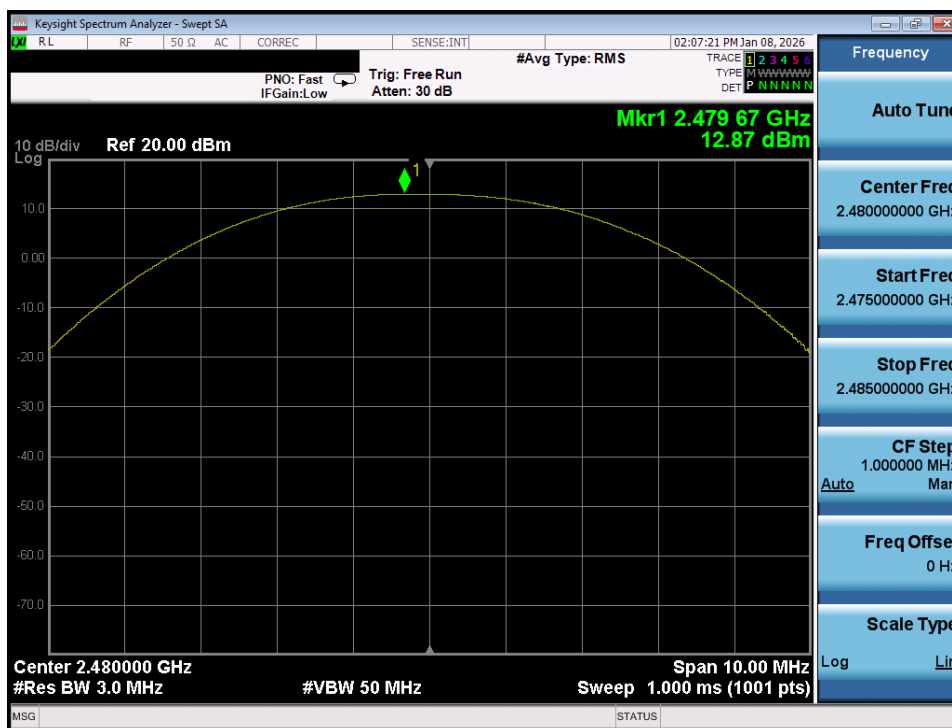
Plot 7-51. Peak Power Plot (Bluetooth (LE), 1Mbps – Ch. 39) – Dual Ant 1
