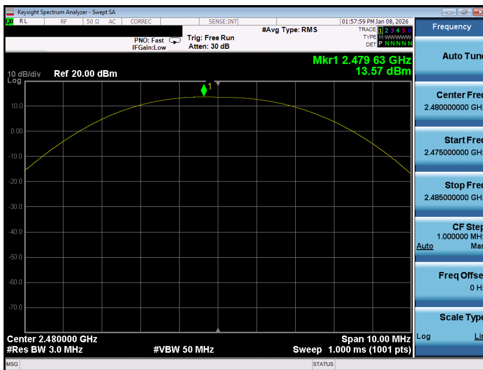
Plot 7-57. Peak Power Plot (Bluetooth (LE), 1Mbps – Ch. 39) – Dual Ant 2
