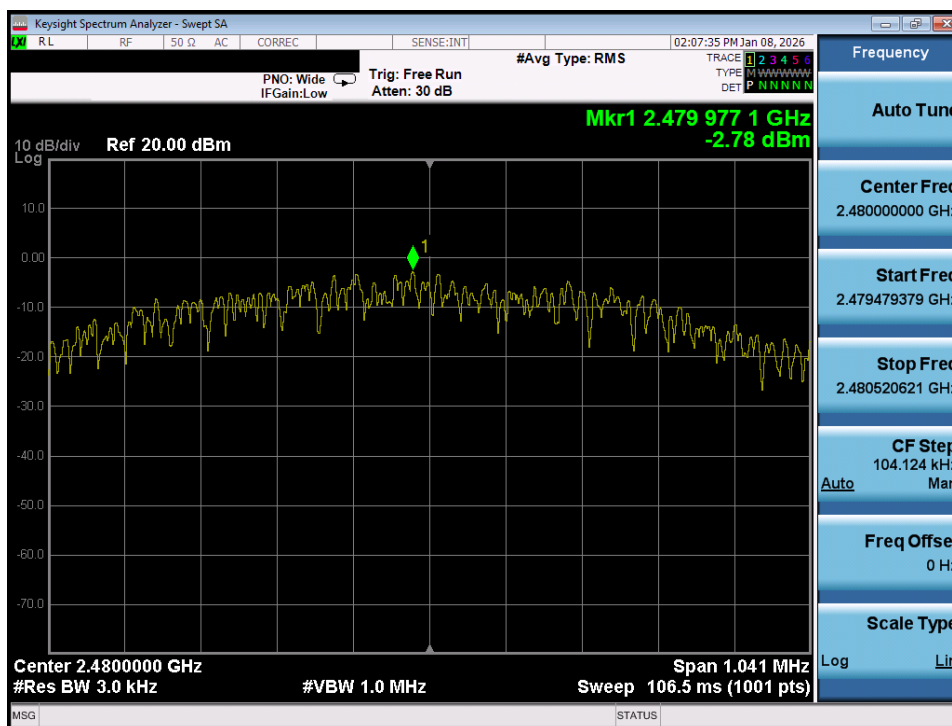
Plot 7-81. Power Spectral Density Plot (Bluetooth (LE), 1Mbps – Ch. 39) – Dual Ant 1
