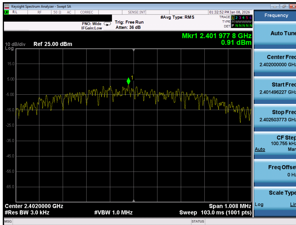
Plot 7-73. Power Spectral Density Plot (Bluetooth (LE), 1Mbps – Ch. 37) – Ant 2
