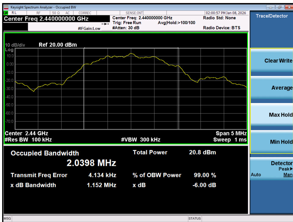
Plot 7-29. 6dB Bandwidth Plot (Bluetooth (LE), 2Mbps – Ch. 17) – Dual Ant 2
