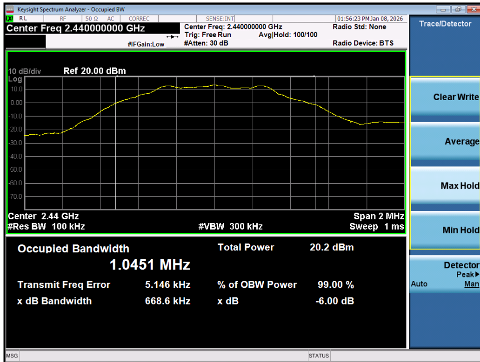
Plot 7-26. 6dB Bandwidth Plot (Bluetooth (LE), 1Mbps – Ch. 17) – Dual Ant 2
