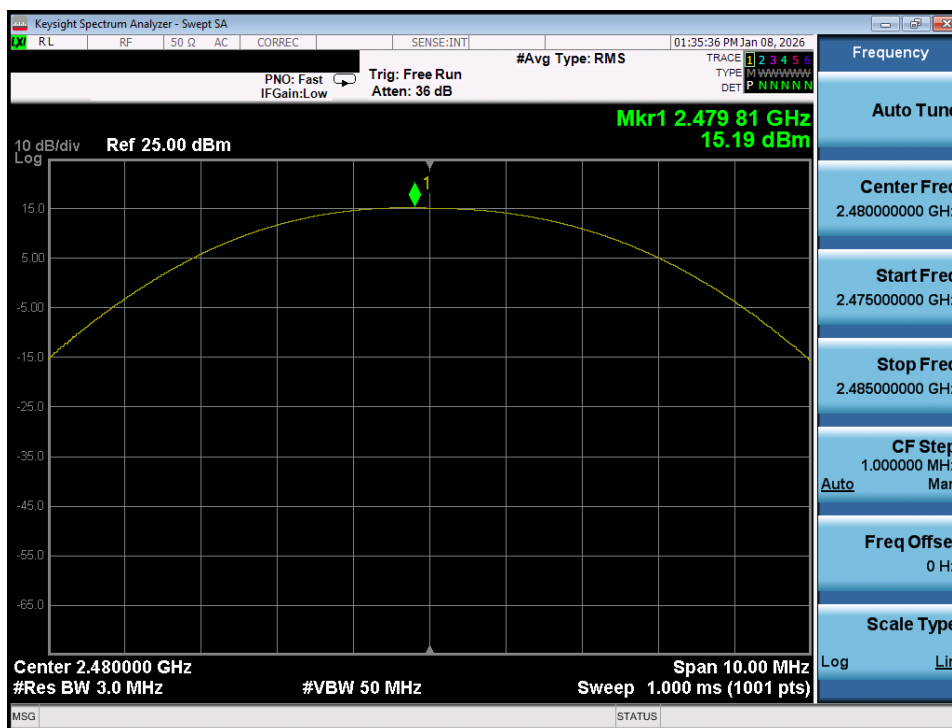
Plot 7-45. Peak Power Plot (Bluetooth (LE), 1Mbps – Ch. 39) – Ant 2
