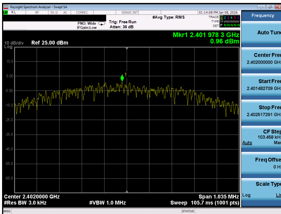
Plot 7-67. Power Spectral Density Plot (Bluetooth (LE), 1Mbps – Ch. 37) – Ant 1
