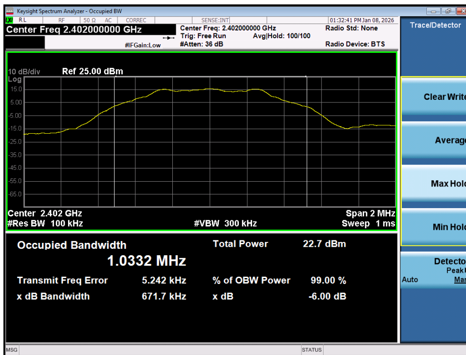
Plot 7-13. 6dB Bandwidth Plot (Bluetooth (LE), 1Mbps – Ch. 37) – Ant 2
