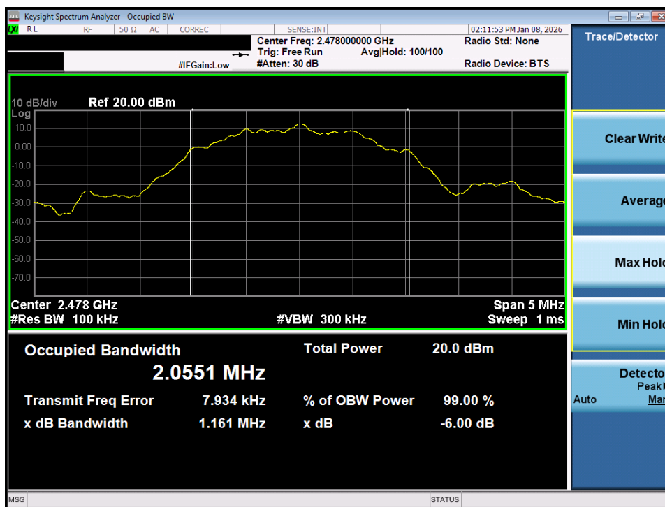
Plot 7-24. 6dB Bandwidth Plot (Bluetooth (LE), 2Mbps – Ch. 36) – Dual Ant 1
