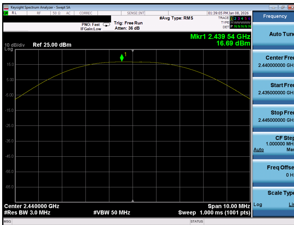
Plot 7-47. Peak Power Plot (Bluetooth (LE), 2Mbps – Ch. 17) – Ant 2
