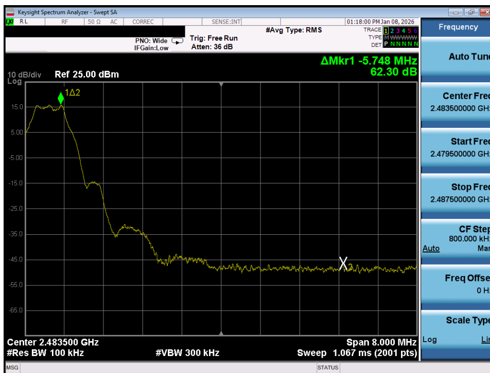
Plot 7-96. Band Edge Plot (Bluetooth (LE), 1Mbps – Ch. 39) – Ant 1
