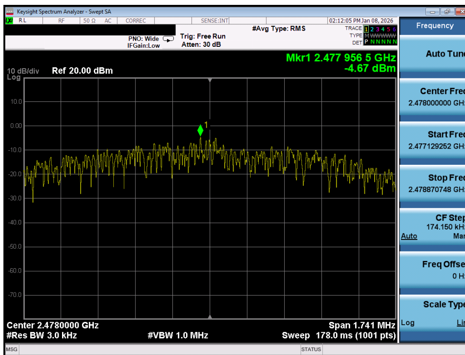
Plot 7-84. Power Spectral Density Plot (Bluetooth (LE), 2Mbps – Ch. 36) – Dual Ant 1
