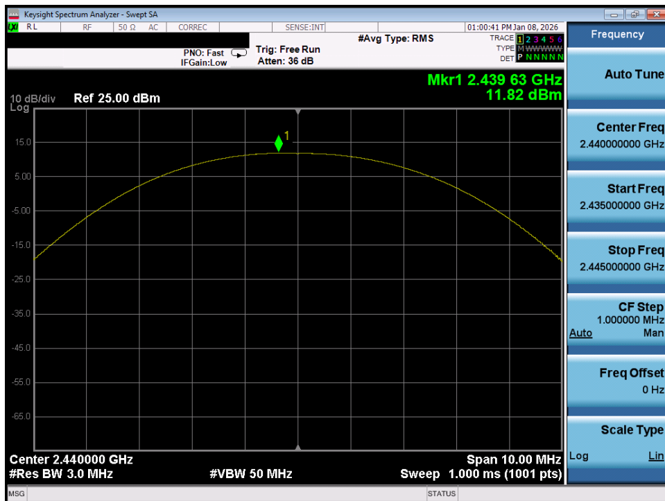
Plot 7-32. Peak Power Plot (Bluetooth (LE), 125kbps – Ch. 17) – Ant 1
