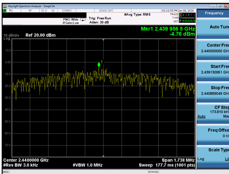
Plot 7-83. Power Spectral Density Plot (Bluetooth (LE), 2Mbps – Ch. 17) – Dual Ant 1
