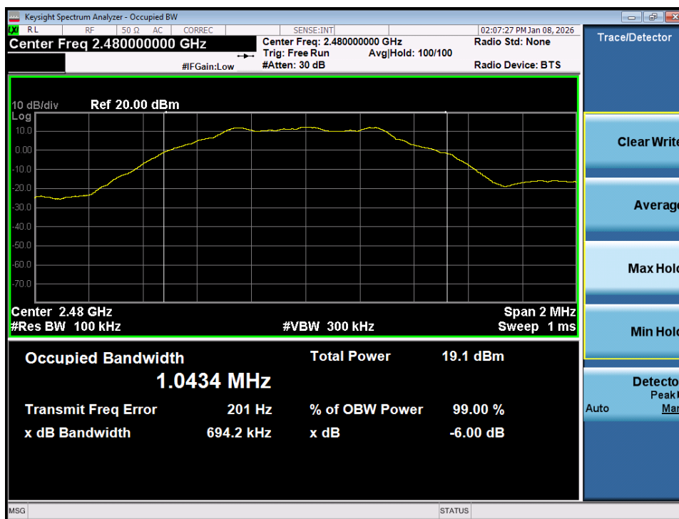
Plot 7-21. 6dB Bandwidth Plot (Bluetooth (LE), 1Mbps – Ch. 39) – Dual Ant 1
