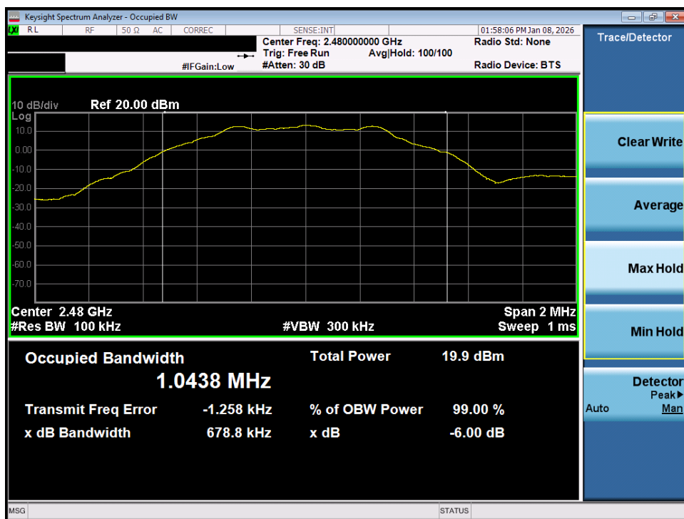
Plot 7-27. 6dB Bandwidth Plot (Bluetooth (LE), 1Mbps – Ch. 39) – Dual Ant 2
