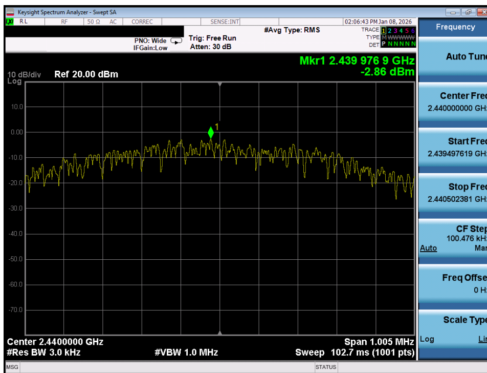
Plot 7-80. Power Spectral Density Plot (Bluetooth (LE), 1Mbps – Ch. 17) – Dual Ant 1
