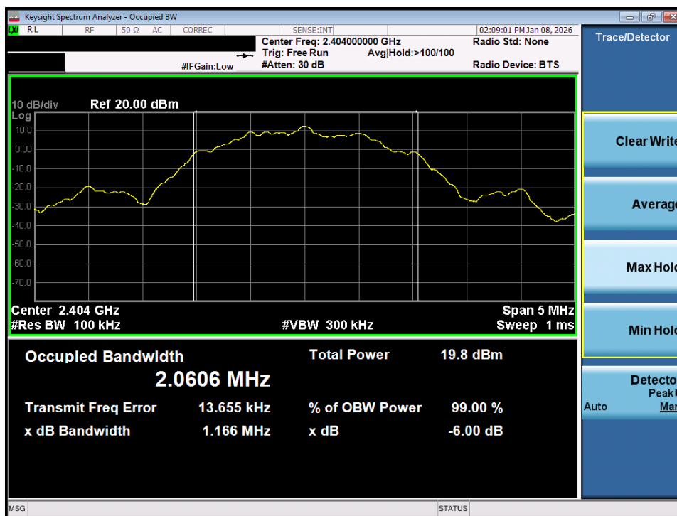
Plot 7-22. 6dB Bandwidth Plot (Bluetooth (LE), 2Mbps – Ch. 0) – Dual Ant 1
