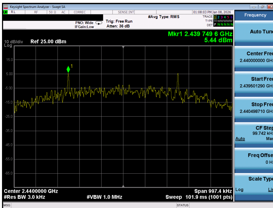
Plot 7-65. Power Spectral Density Plot (Bluetooth (LE), 500kbps – Ch. 17) – Ant 1
