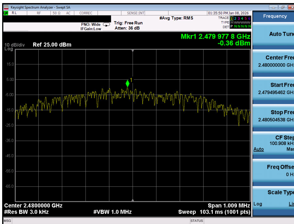
Plot 7-75. Power Spectral Density Plot (Bluetooth (LE), 1Mbps – Ch. 39) – Ant 2
