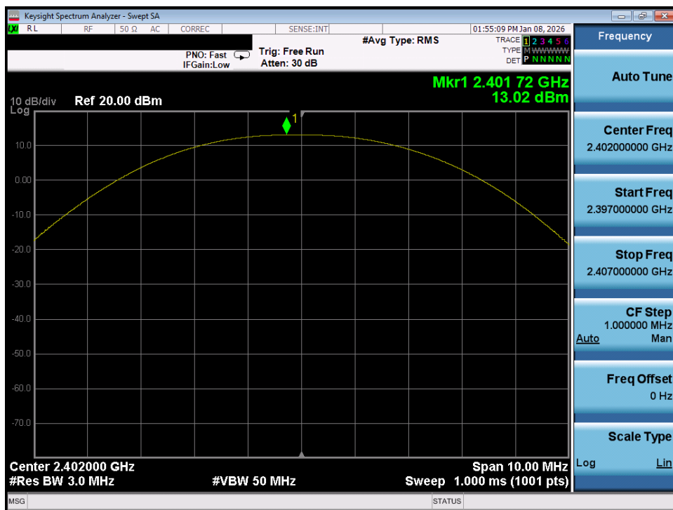
Plot 7-55. Peak Power Plot (Bluetooth (LE), 1Mbps – Ch. 37) – Dual Ant 2
