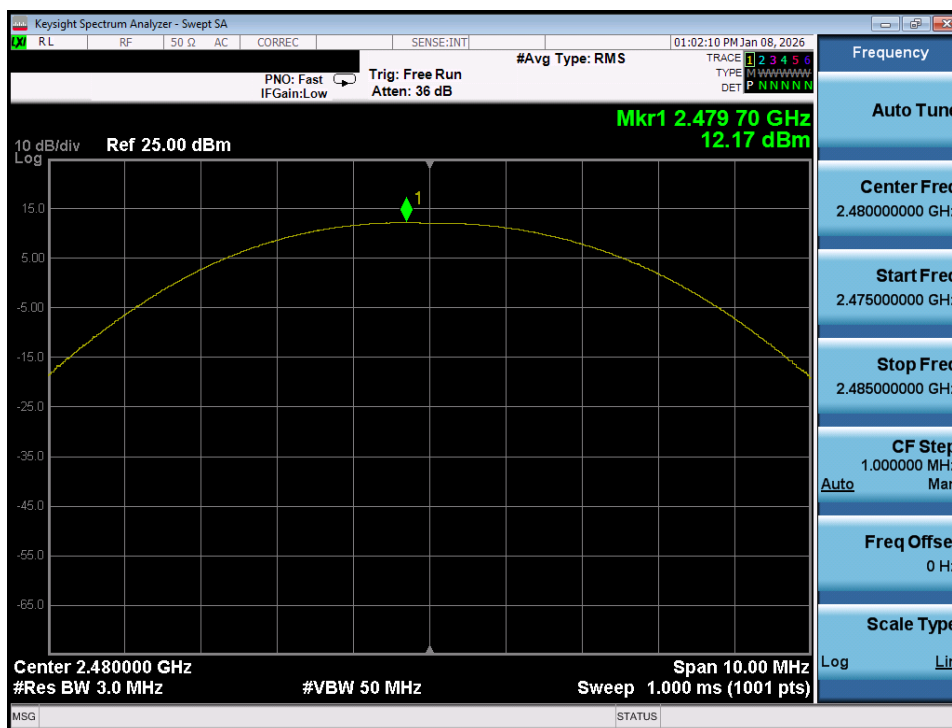
Plot 7-33. Peak Power Plot (Bluetooth (LE), 125kbps – Ch. 39) – Ant 1
