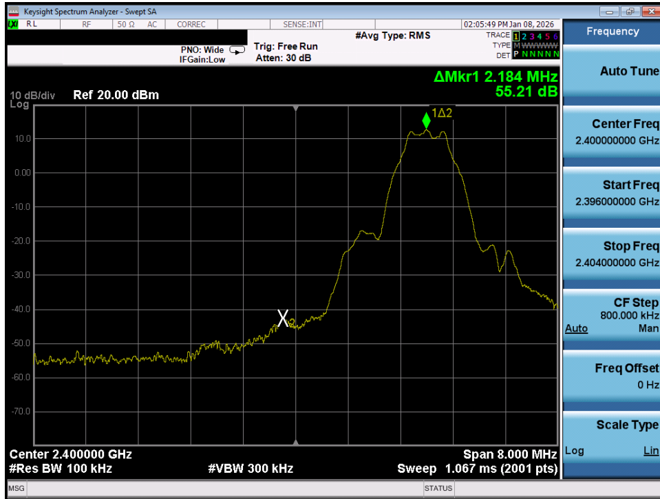
Plot 7-103. Band Edge Plot (Bluetooth (LE), 1Mbps – Ch. 37) – Dual Ant 1
