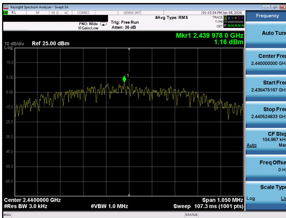
Plot 7-68. Power Spectral Density Plot (Bluetooth (LE), 1Mbps – Ch. 17) – Ant 1
