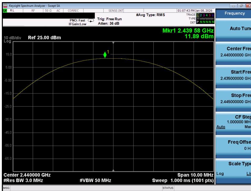
Plot 7-35. Peak Power Plot (Bluetooth (LE), 500kbps – Ch. 17) – Ant 1
