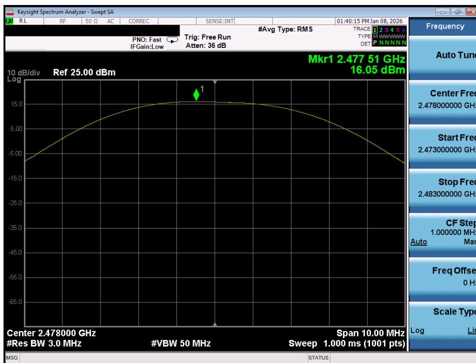
Plot 7-48. Peak Power Plot (Bluetooth (LE), 2Mbps – Ch. 36) – Ant 2
