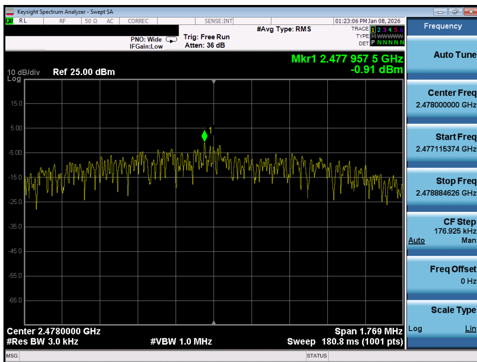
Plot 7-72. Power Spectral Density Plot (Bluetooth (LE), 2Mbps – Ch. 36) – Ant 1
