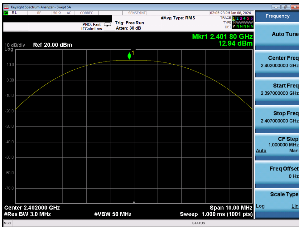
Plot 7-49. Peak Power Plot (Bluetooth (LE), 1Mbps – Ch. 37) – Dual Ant 1
