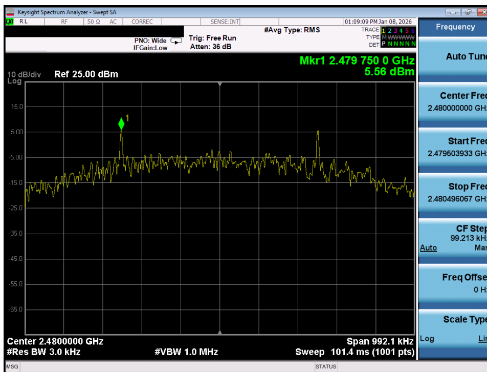
Plot 7-66. Power Spectral Density Plot (Bluetooth (LE), 500kbps – Ch. 39) – Ant 1
