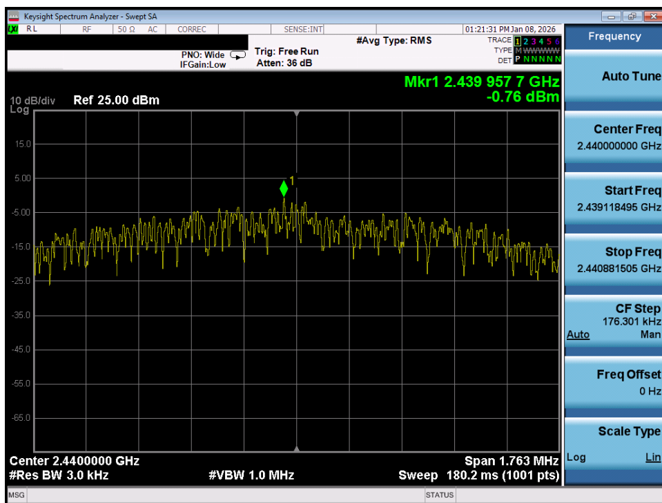
Plot 7-71. Power Spectral Density Plot (Bluetooth (LE), 2Mbps – Ch. 17) – Ant 1
