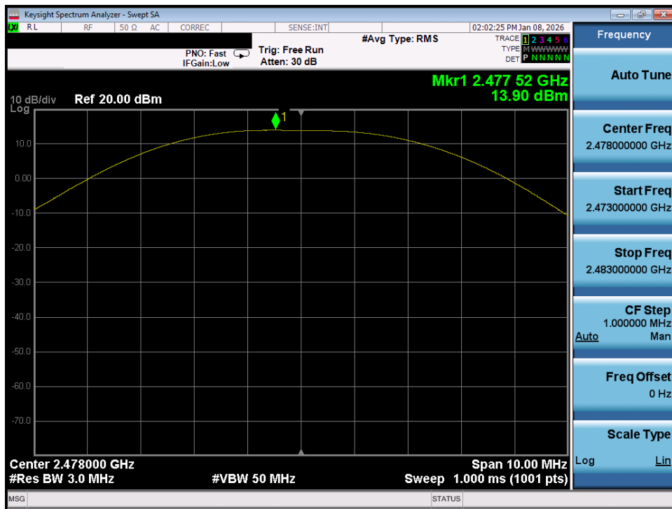
Plot 7-60. Peak Power Plot (Bluetooth (LE), 2Mbps – Ch. 36) – Dual Ant 2
