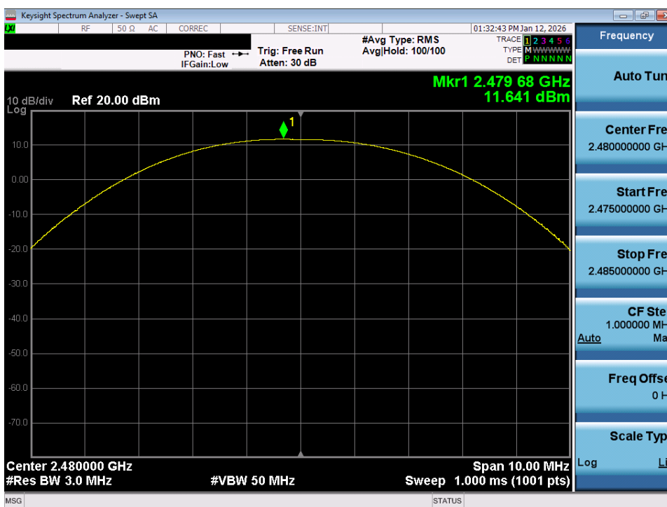
Plot 7-36. Peak Power Plot (Bluetooth (LE), 500kbps – Ch. 39) – Ant 1
