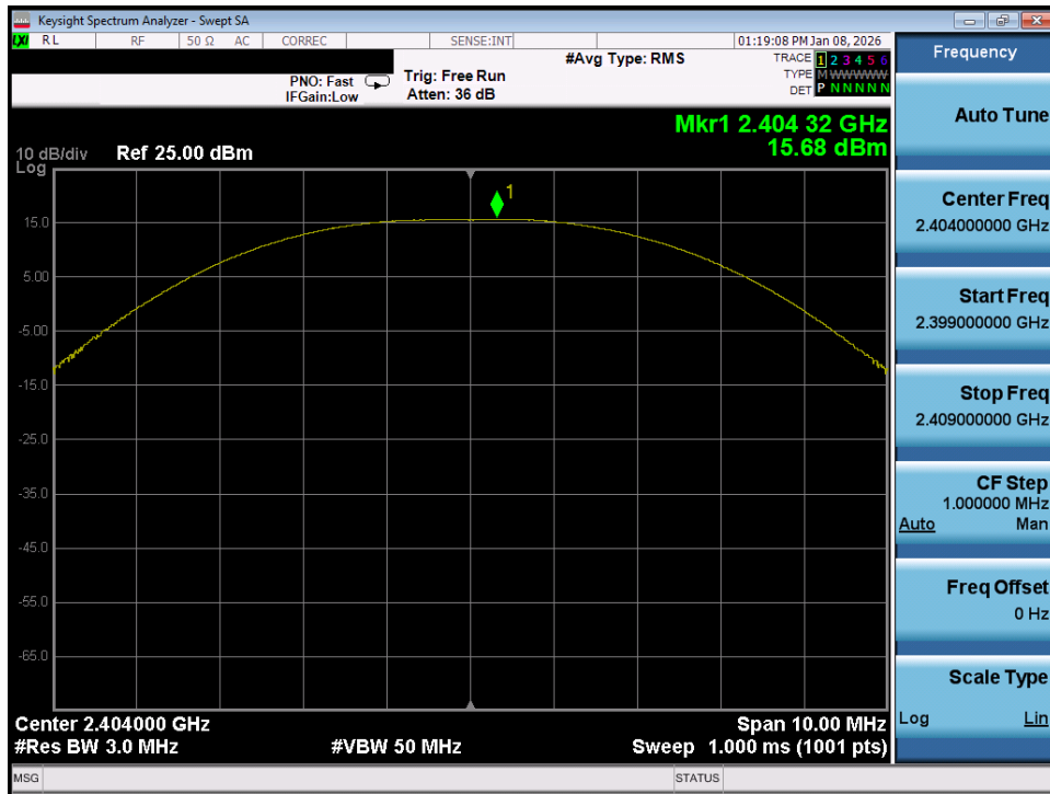
Plot 7-40. Peak Power Plot (Bluetooth (LE), 2Mbps – Ch. 0) – Ant 1
