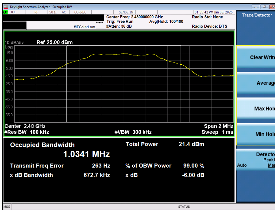
Plot 7-15. 6dB Bandwidth Plot (Bluetooth (LE), 1Mbps – Ch. 39) – Ant 2
