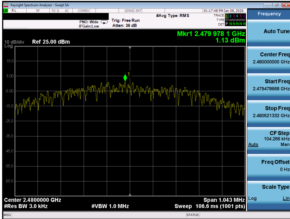
Plot 7-69. Power Spectral Density Plot (Bluetooth (LE), 1Mbps – Ch. 39) – Ant 1
