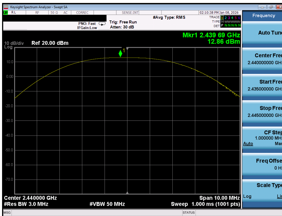
Plot 7-53. Peak Power Plot (Bluetooth (LE), 2Mbps – Ch. 17) – Dual Ant 1
