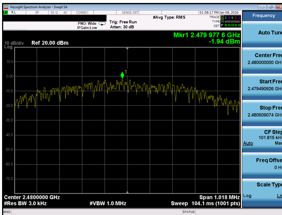
Plot 7-87. Power Spectral Density Plot (Bluetooth (LE), 1Mbps – Ch. 39) – Dual Ant 2
