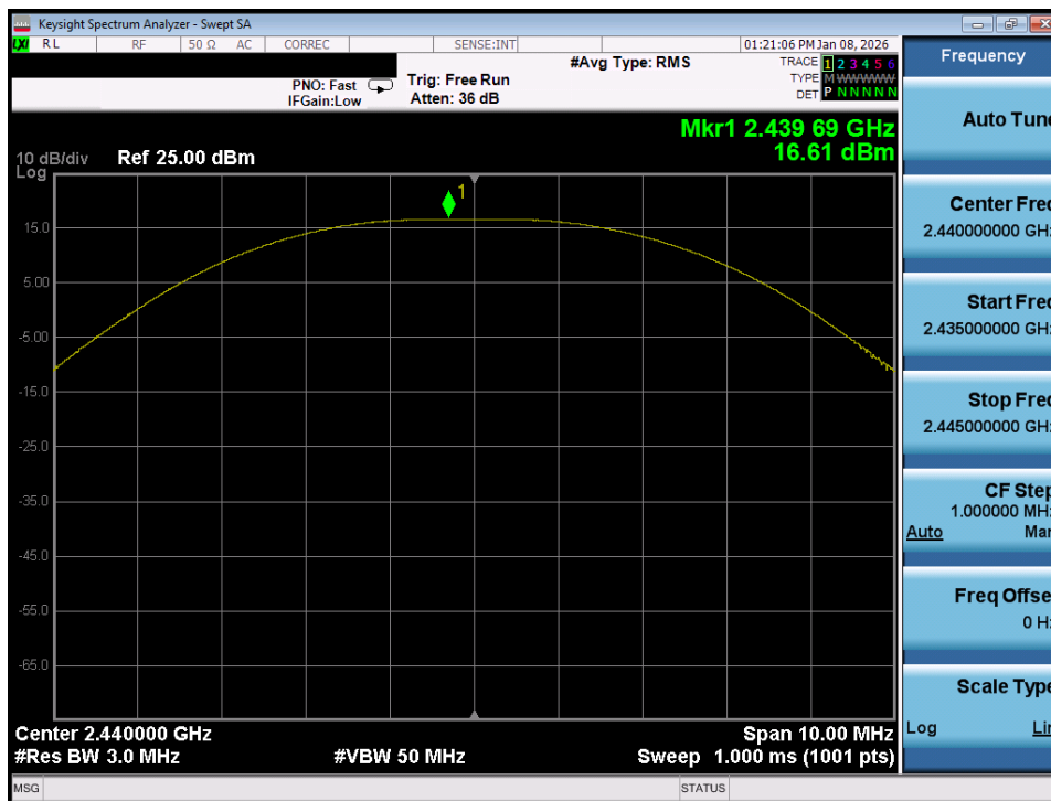
Plot 7-41. Peak Power Plot (Bluetooth (LE), 2Mbps – Ch. 17) – Ant 1
