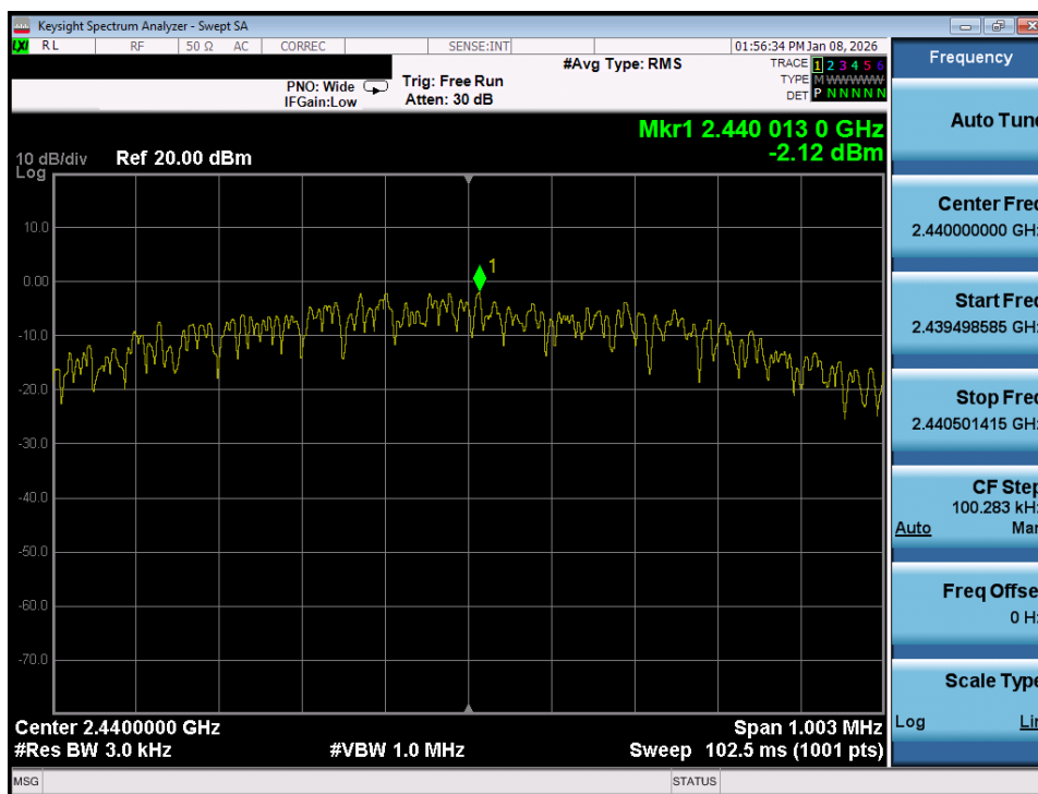
Plot 7-86. Power Spectral Density Plot (Bluetooth (LE), 1Mbps – Ch. 17) – Dual Ant 2
