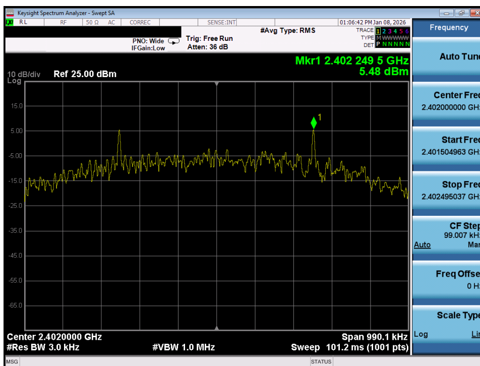
Plot 7-64. Power Spectral Density Plot (Bluetooth (LE), 500kbps – Ch. 37) – Ant 1
