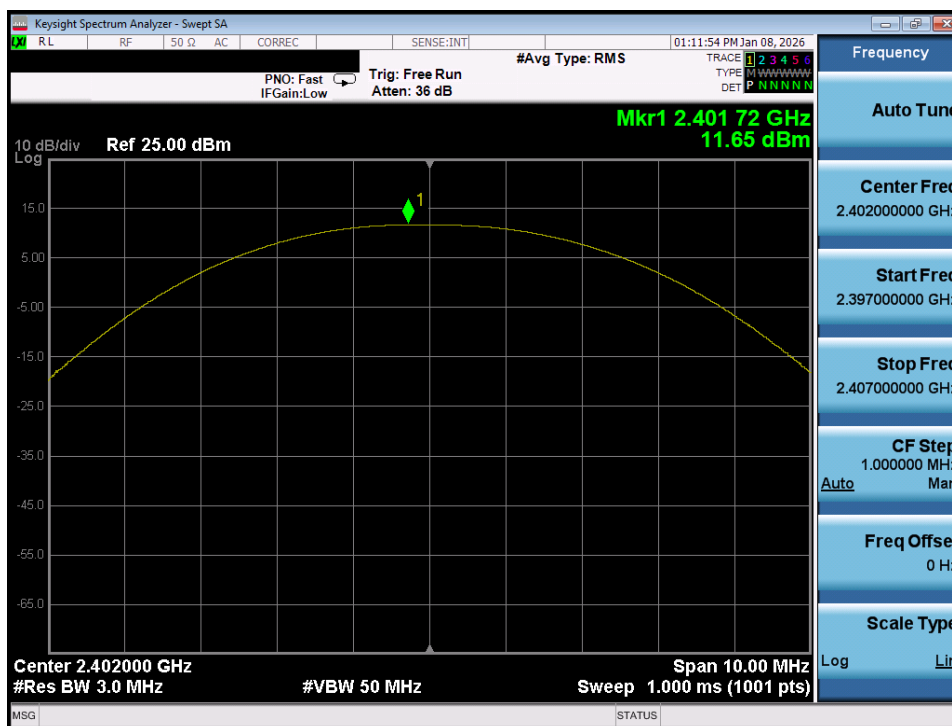
Plot 7-34. Peak Power Plot (Bluetooth (LE), 500kbps – Ch. 37) – Ant 1
