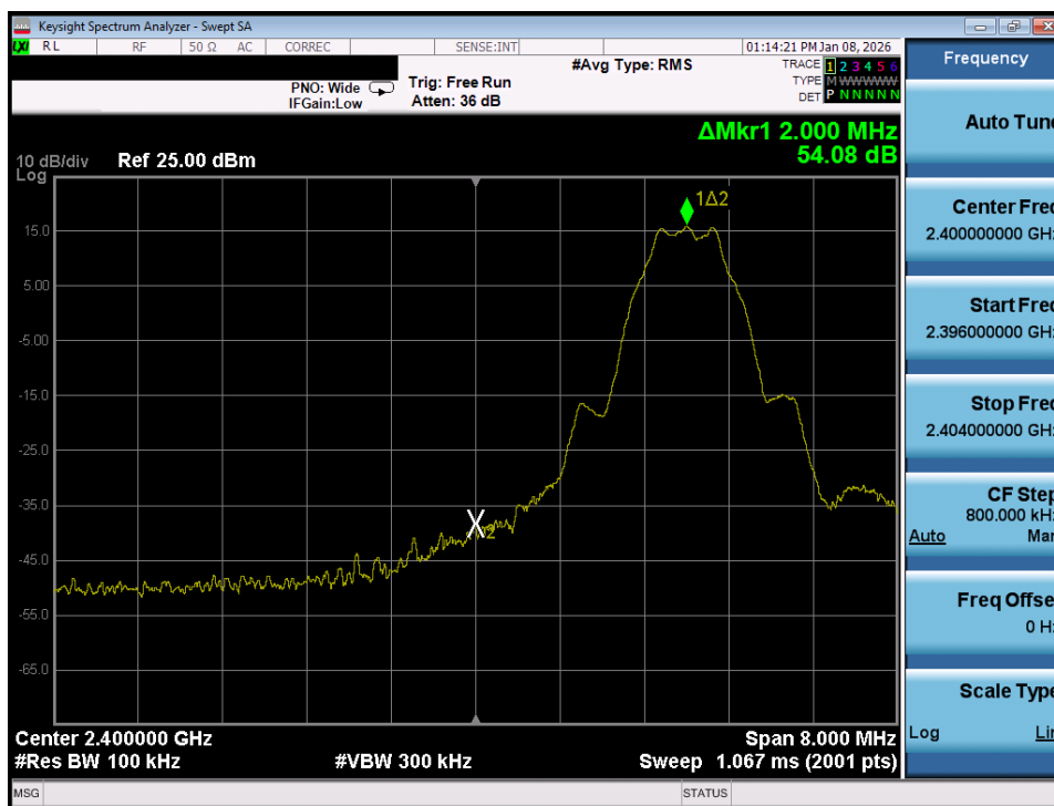
Plot 7-95. Band Edge Plot (Bluetooth (LE), 1Mbps – Ch. 37) – Ant 1
