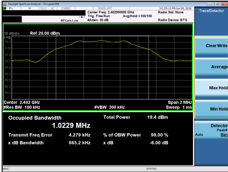
Plot 7-25. 6dB Bandwidth Plot (Bluetooth (LE), 1Mbps – Ch. 37) – Dual Ant 2
