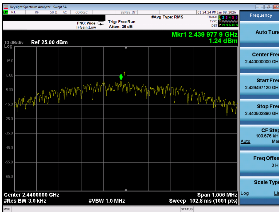
Plot 7-74. Power Spectral Density Plot (Bluetooth (LE), 1Mbps – Ch. 17) – Ant 2
