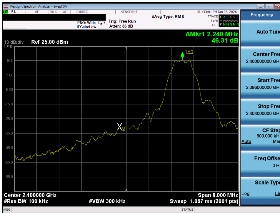
Plot 7-99. Band Edge Plot (Bluetooth (LE), 1Mbps – Ch. 37) – Ant 2
