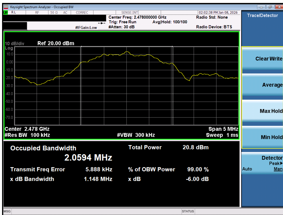
Plot 7-30. 6dB Bandwidth Plot (Bluetooth (LE), 2Mbps – Ch. 36) – Dual Ant 2
