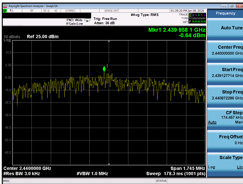
Plot 7-77. Power Spectral Density Plot (Bluetooth (LE), 2Mbps – Ch. 17) – Ant 2
