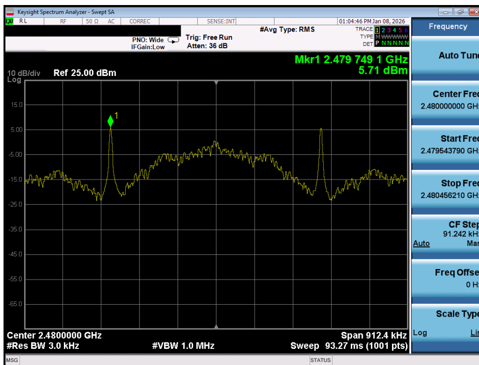
Plot 7-63. Power Spectral Density Plot (Bluetooth (LE), 125kbps – Ch. 39) – Ant 1
