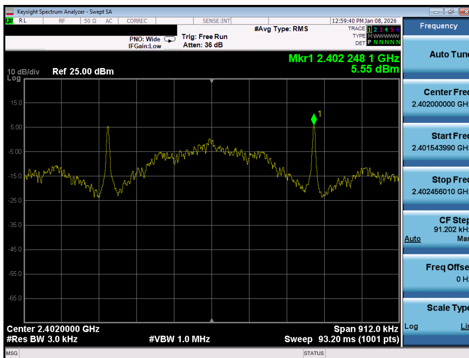
Plot 7-61. Power Spectral Density Plot (Bluetooth (LE), 125kbps – Ch. 37) – Ant 1
