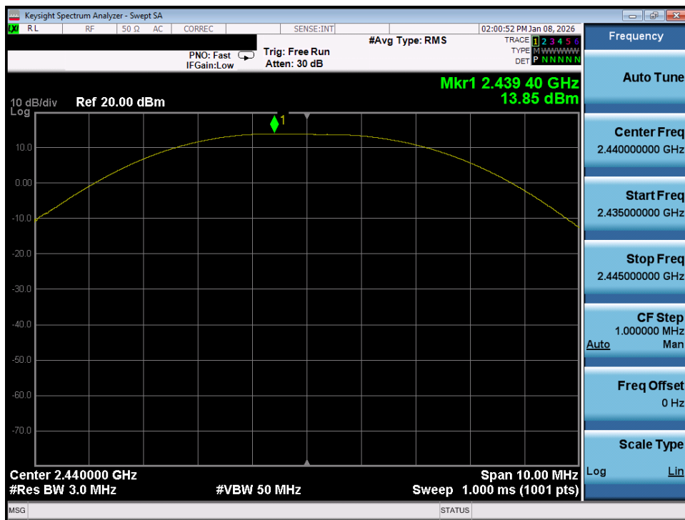
Plot 7-59. Peak Power Plot (Bluetooth (LE), 2Mbps – Ch. 17) – Dual Ant 2
