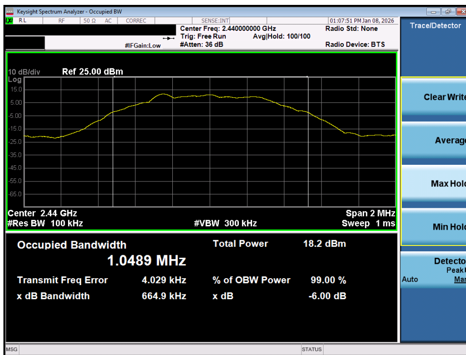
Plot 7-5. 6dB Bandwidth Plot (Bluetooth (LE), 500kbps – Ch. 17) – Ant 1
