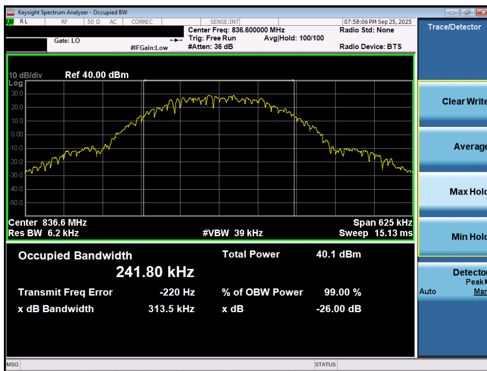
Plot 7-23. Occupied Bandwidth Plot (GPRS, Ch. 190 – Ant1)
