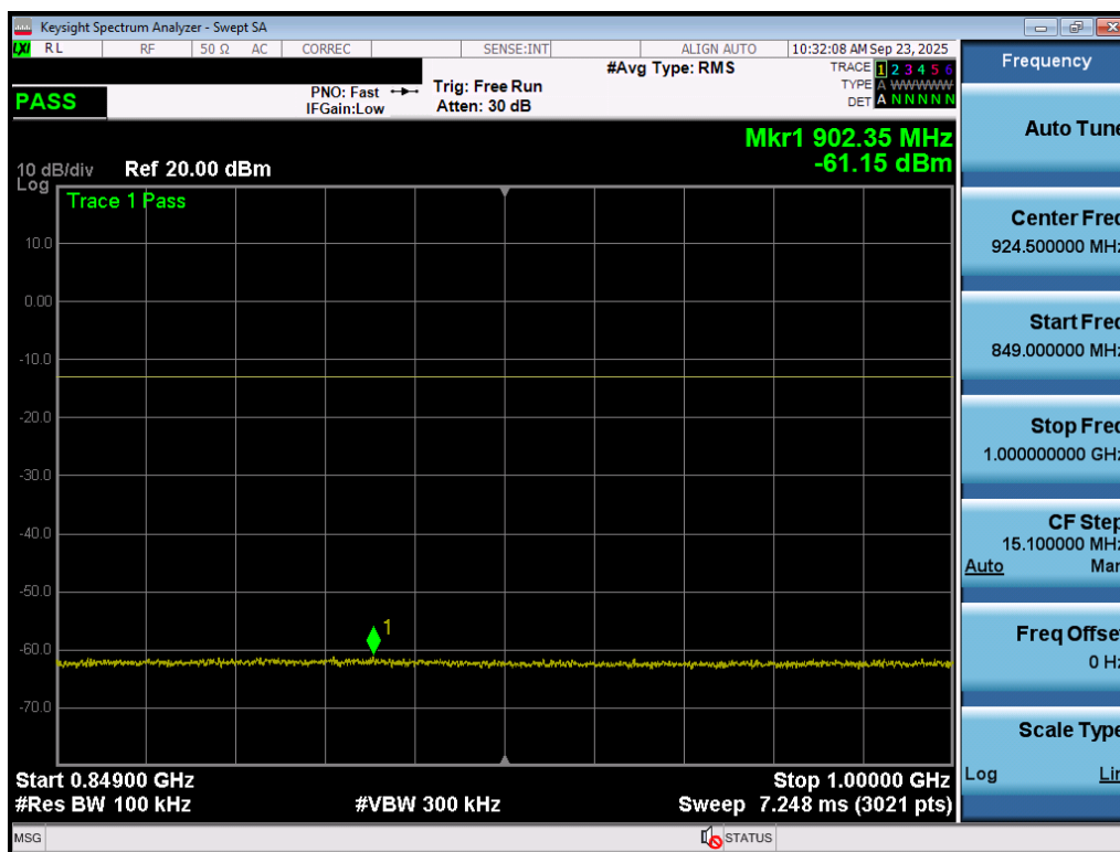
Plot 7-55. Conducted Spurious Plot (LTE Band 26/5 - 15MHz QPSK - 1 RB - Mid Channel – Ant1)
