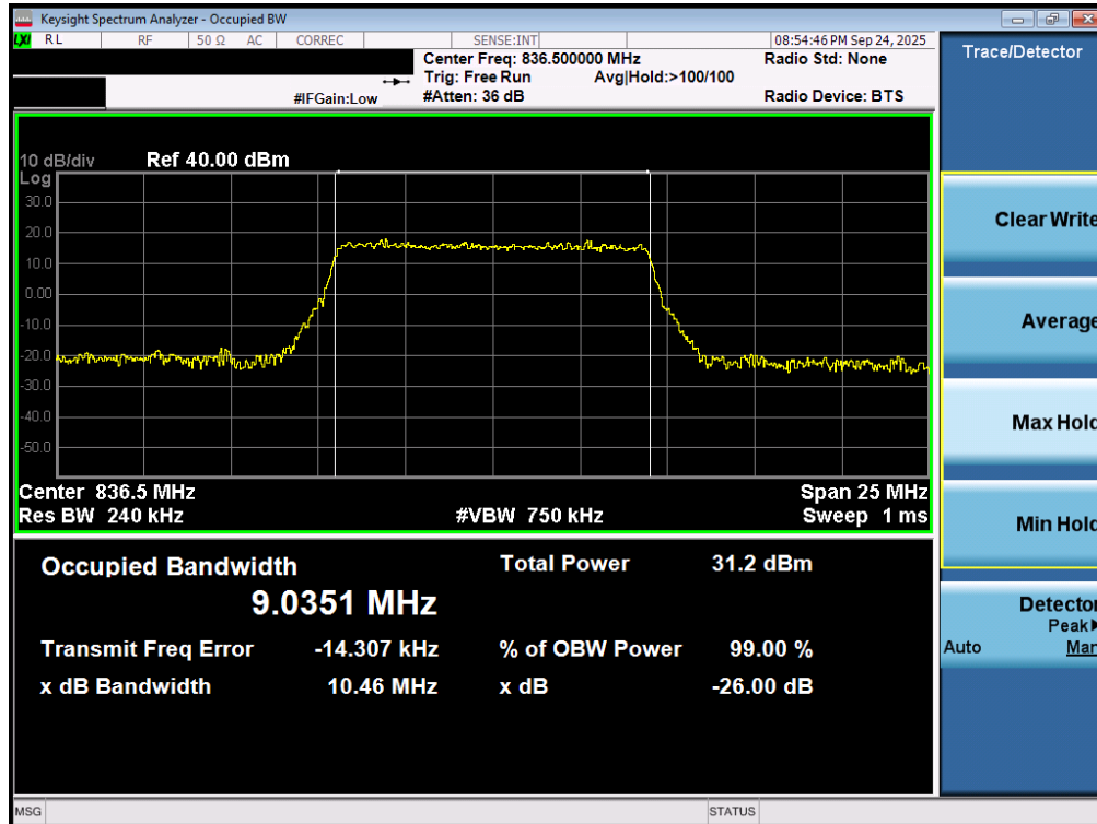
Plot 7-29. Occupied Bandwidth Plot (LTE Band 26/5 - 10MHz 16-QAM - Full RB - Ant2)
