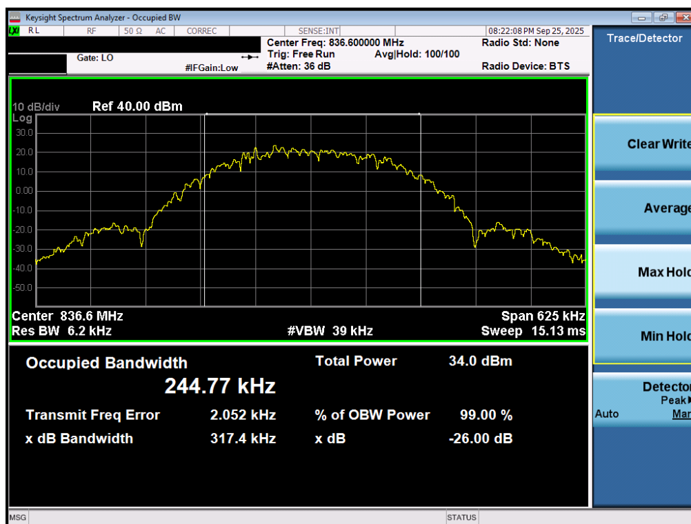
Plot 7-49. Occupied Bandwidth Plot (EDGE, Ch. 190 – Ant2)
