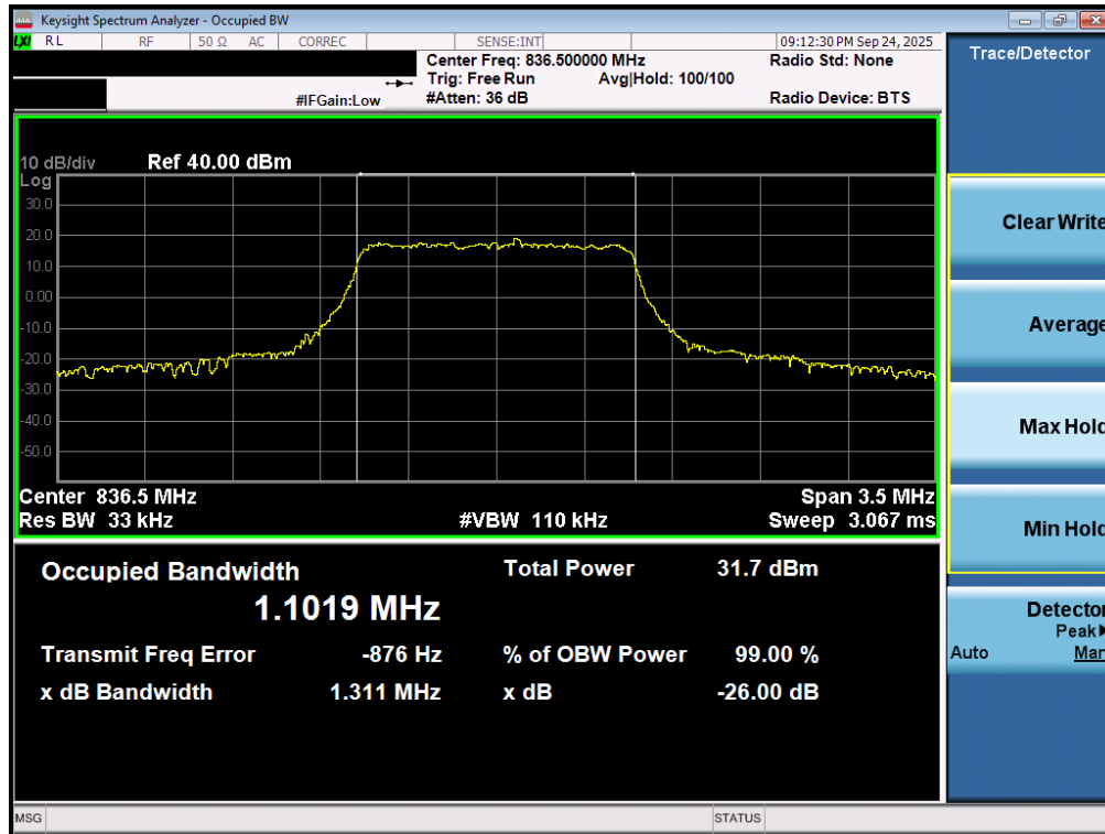
Plot 7-34. Occupied Bandwidth Plot (LTE Band 26/5 - 1.4MHz QPSK - Full RB - Ant2)
