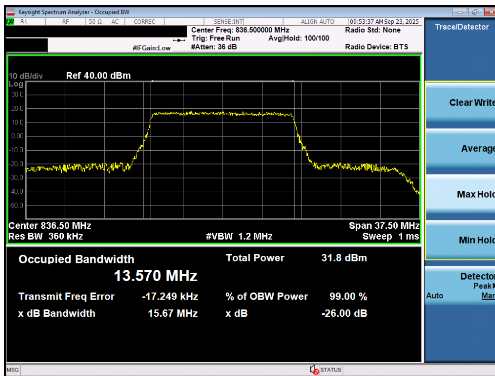
Plot 7-1. Occupied Bandwidth Plot (LTE Band 26 - 15MHz QPSK - Full RB - Ant1)
