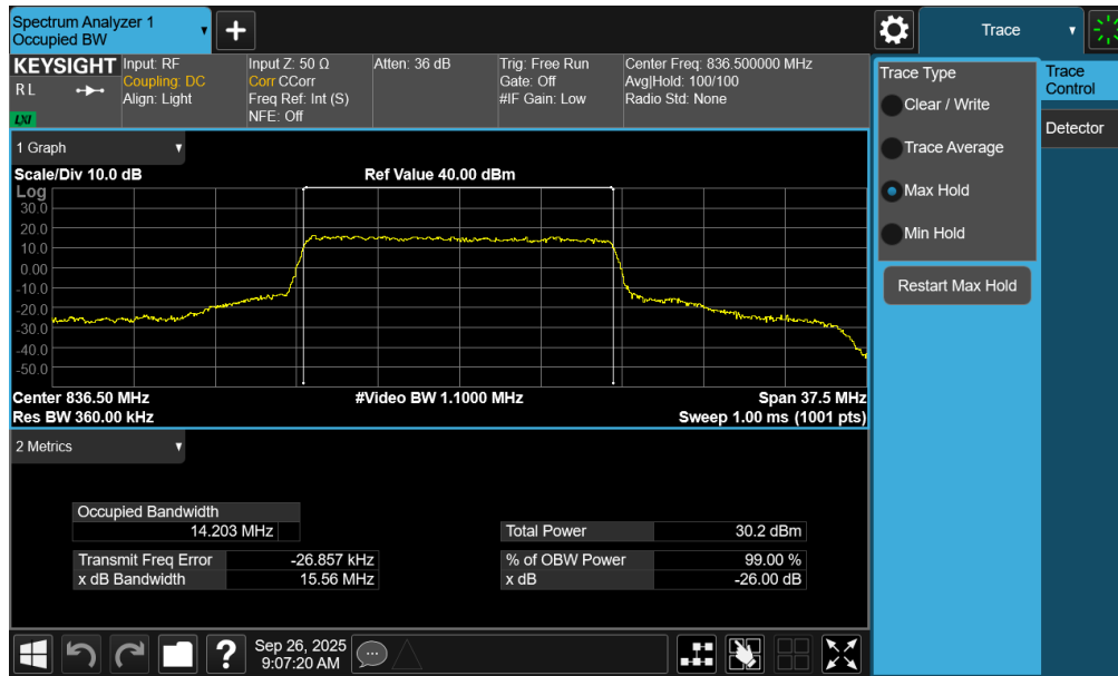
Plot 7-40. Occupied Bandwidth Plot (NR Band n26/5 - 15MHz QPSK - Full RB - Ant2)
