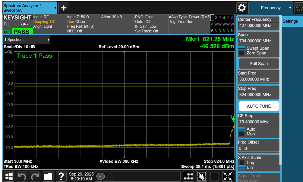
Plot 7-60. Conducted Spurious Plot (NR Band n26/5 - 20.0MHz - 1 RB - Low Channel - Ant1)
