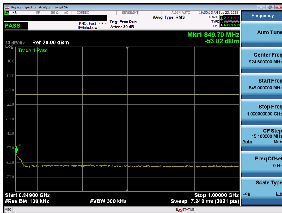
Plot 7-52. Conducted Spurious Plot (LTE Band 26/5 - 15MHz QPSK - 1 RB - Low Channel – Ant1)
