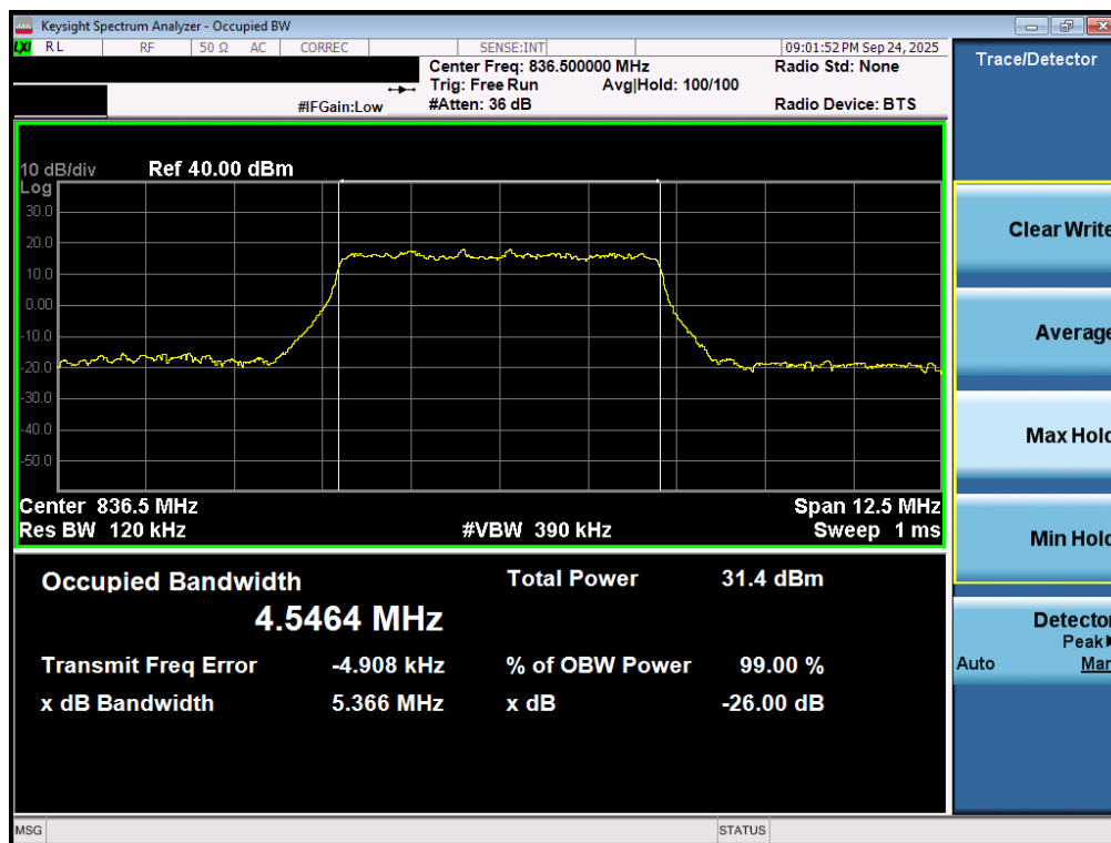
Plot 7-31. Occupied Bandwidth Plot (LTE Band 26/5 - 5MHz 16-QAM - Full RB - Ant2)
