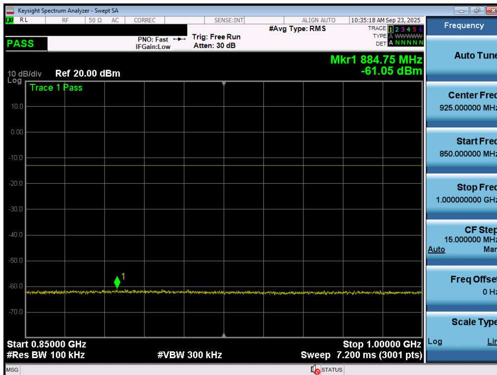
Plot 7-58. Conducted Spurious Plot (LTE Band 26/5 - 15MHz QPSK - 1 RB - High Channel – Ant1)
