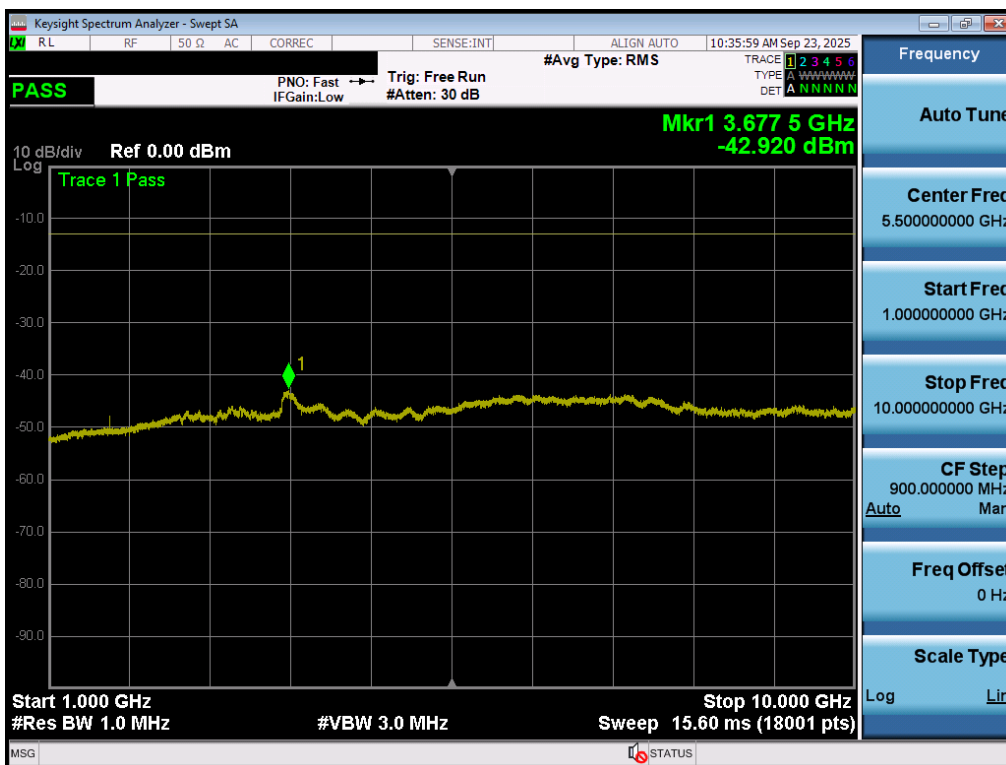
Plot 7-59. Conducted Spurious Plot (LTE Band 26/5 - 15MHz QPSK - 1 RB - High Channel – Ant1)
