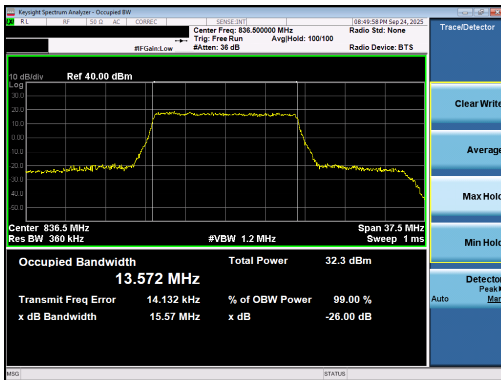
Plot 7-26. Occupied Bandwidth Plot (LTE Band 26 - 15MHz QPSK - Full RB - Ant2)
