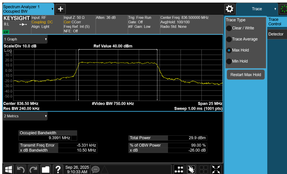
Plot 7-43. Occupied Bandwidth Plot (NR Band n26/5 - 10MHz QPSK - Full RB - Ant2)
