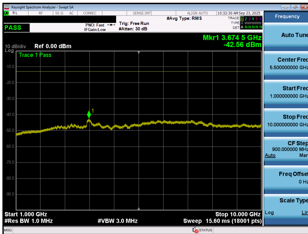
Plot 7-56. Conducted Spurious Plot (LTE Band 26/5 - 15MHz QPSK - 1 RB - Mid Channel – Ant1)
