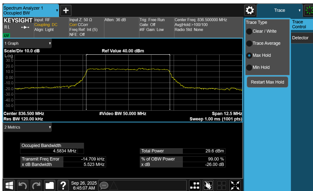
Plot 7-22. Occupied Bandwidth Plot (NR Band n26/5 - 5MHz 16-QAM - Full RB - Ant1)
