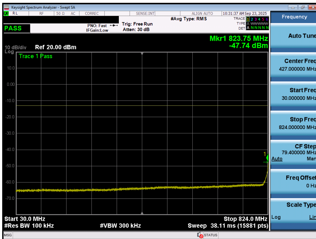
Plot 7-54. Conducted Spurious Plot (LTE Band 26/5 - 15MHz QPSK - 1 RB - Mid Channel – Ant1)
