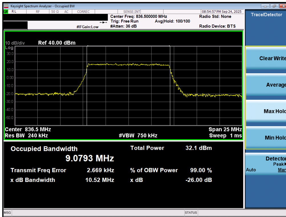
Plot 7-28. Occupied Bandwidth Plot (LTE Band 26/5 - 10MHz QPSK - Full RB - Ant2)
