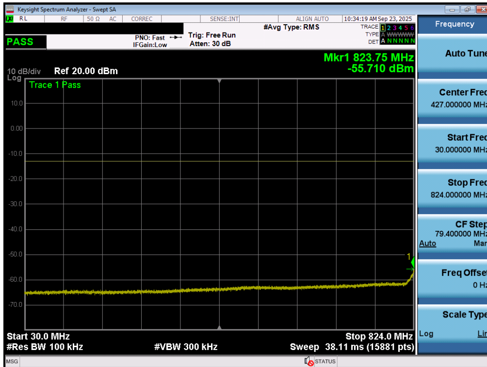
Plot 7-57. Conducted Spurious Plot (LTE Band 26/5 - 15MHz QPSK - 1 RB - High Channel – Ant1)
