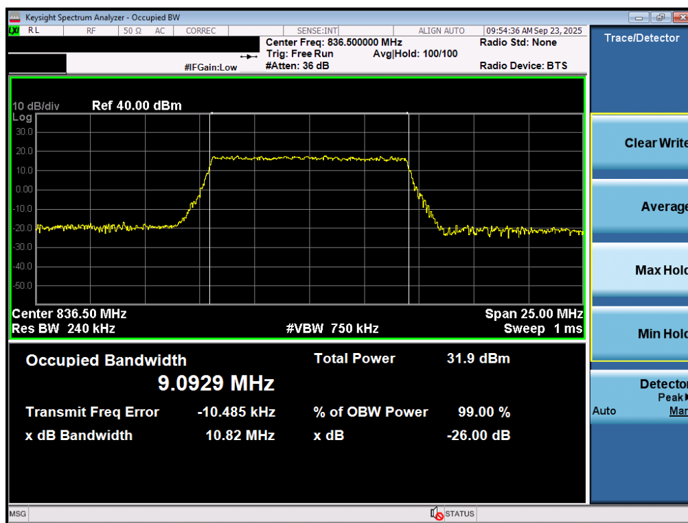
Plot 7-3. Occupied Bandwidth Plot (LTE Band 26/5 - 10MHz QPSK - Full RB - Ant1)
