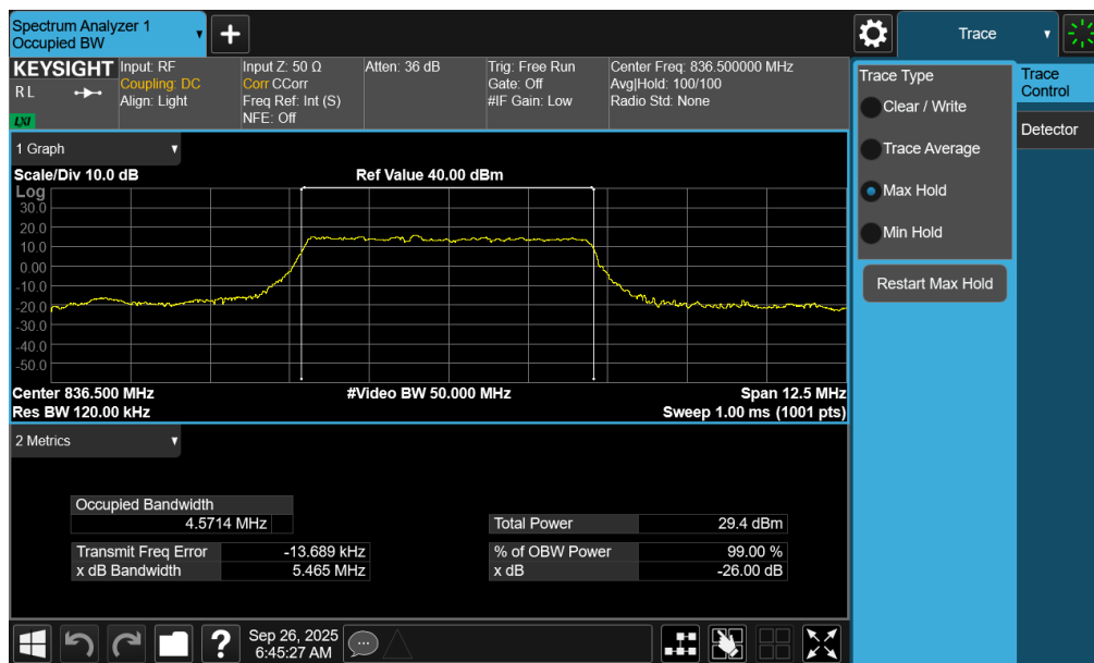
Plot 7-21. Occupied Bandwidth Plot (NR Band n26/5 - 5MHz QPSK - Full RB - Ant1)
