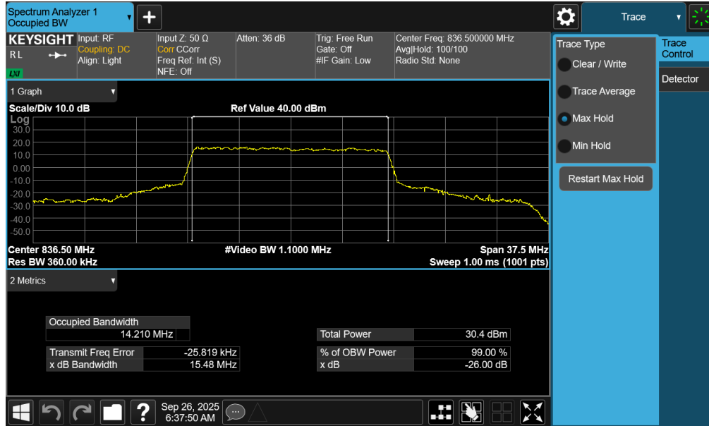
Plot 7-15. Occupied Bandwidth Plot (NR Band n26/5 - 15MHz QPSK - Full RB - Ant1)
