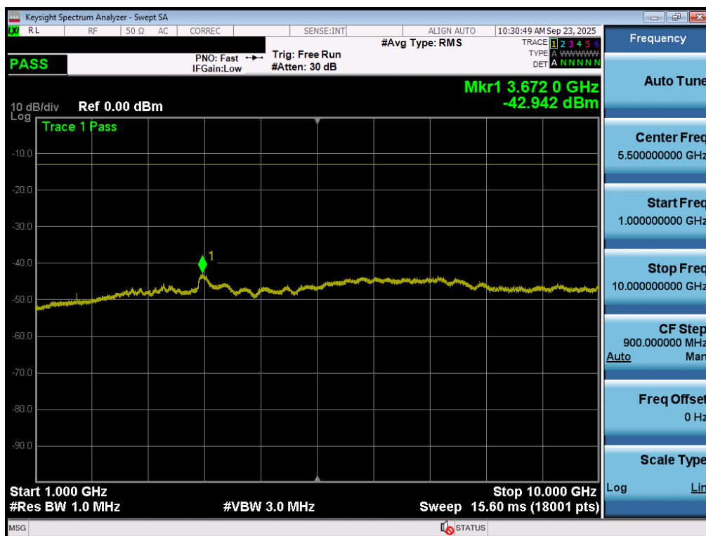
Plot 7-53. Conducted Spurious Plot (LTE Band 26/5 - 15MHz QPSK - 1 RB - Low Channel – Ant1)
