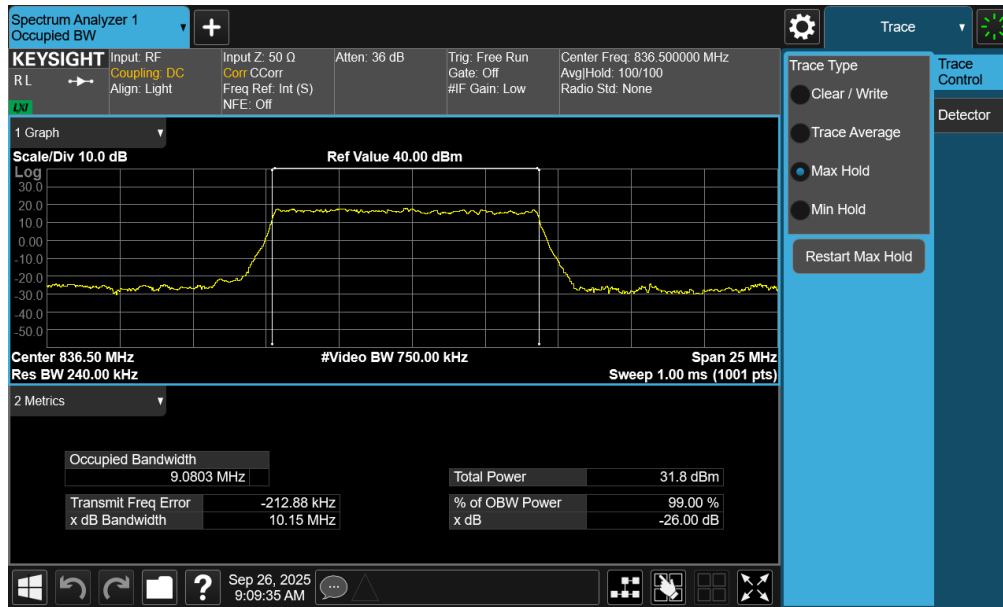
Plot 7-42. Occupied Bandwidth Plot (NR Band n26/5 - 10MHz \pi/2 BPSK - Full RB - Ant2)
