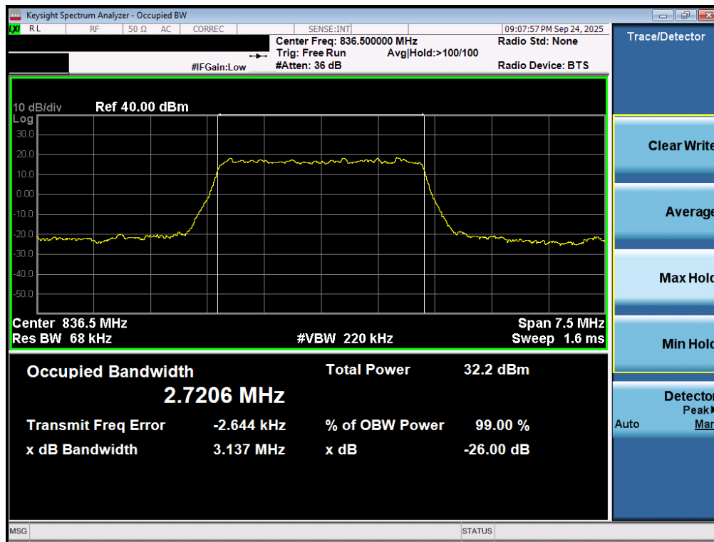
Plot 7-32. Occupied Bandwidth Plot (LTE Band 26/5 - 3MHz QPSK - Full RB - Ant2)
