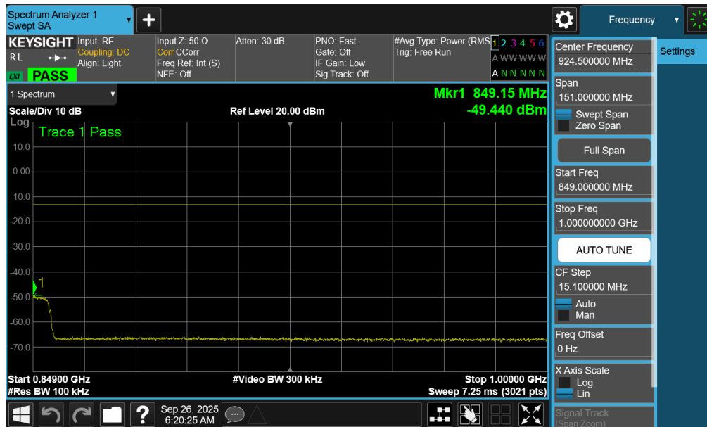
Plot 7-61. Conducted Spurious Plot (NR Band n26/5 - 20.0MHz - 1 RB - Low Channel - Ant1)
