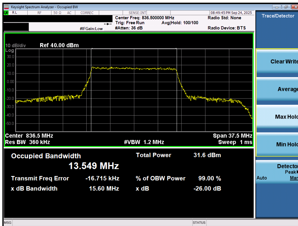
Plot 7-27. Occupied Bandwidth Plot (LTE Band 26 - 15MHz 16-QAM - Full RB - Ant2)
