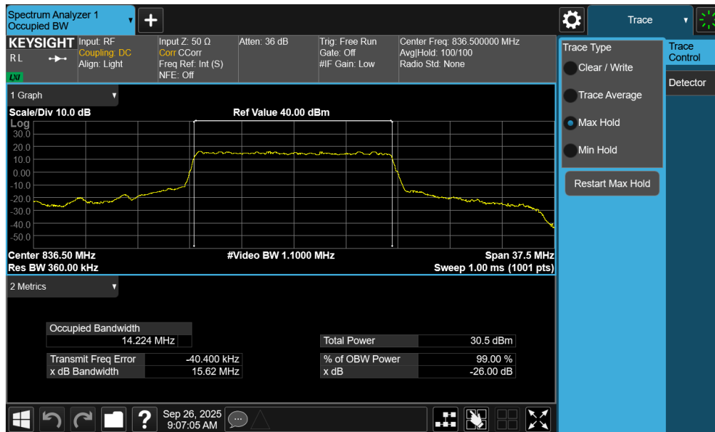
Plot 7-41. Occupied Bandwidth Plot (NR Band n26/5 - 15MHz 16-QAM - Full RB - Ant2)
