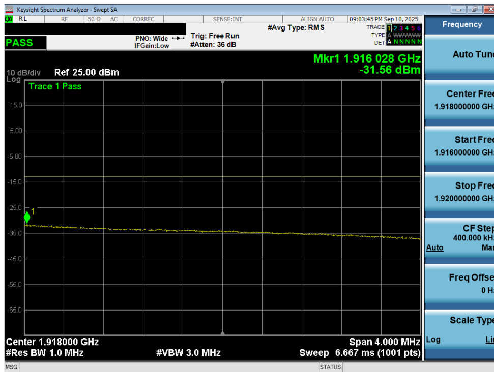
Plot 7-213. Extended Upper Band Edge Plot (LTE Band 25 - 20MHz QPSK – Full RB - Ant2)
