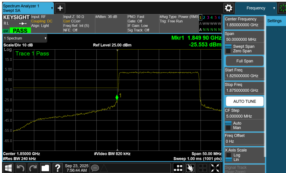
Plot 7-178. Lower Band Edge Plot (NR Band n25/2 - 20MHz QPSK – Full RB - Ant1)
