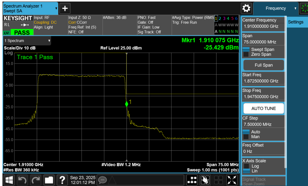
Plot 7-252. Upper Band Edge Plot (NR Band n2 - 30MHz QPSK – Full RB - Ant2)
