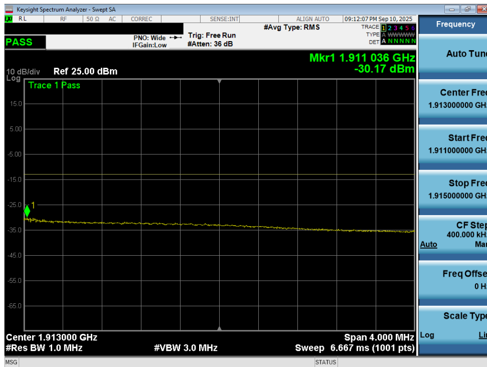
Plot 7-217. Extended Upper Band Edge Plot (LTE Band 2 - 15MHz QPSK – Full RB - Ant2)
