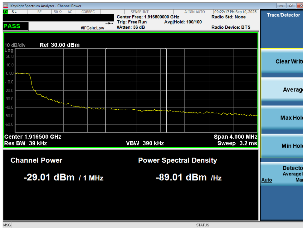
Plot 7-231. Extended Upper Band Edge Plot (LTE Band 25 - 5MHz QPSK – Full RB - Ant2)
