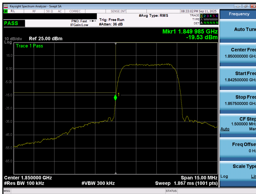
Plot 7-204. Lower Band Edge Plot (WCDMA PCS – Ch. 9262 - Ant1)
