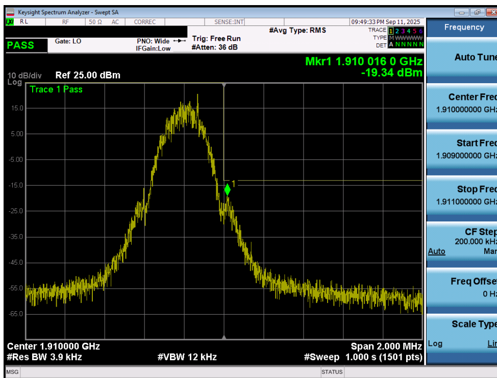
Plot 7-203. Upper Band Edge Plot (GPRS PCS – Ch. 810 - Ant1)
