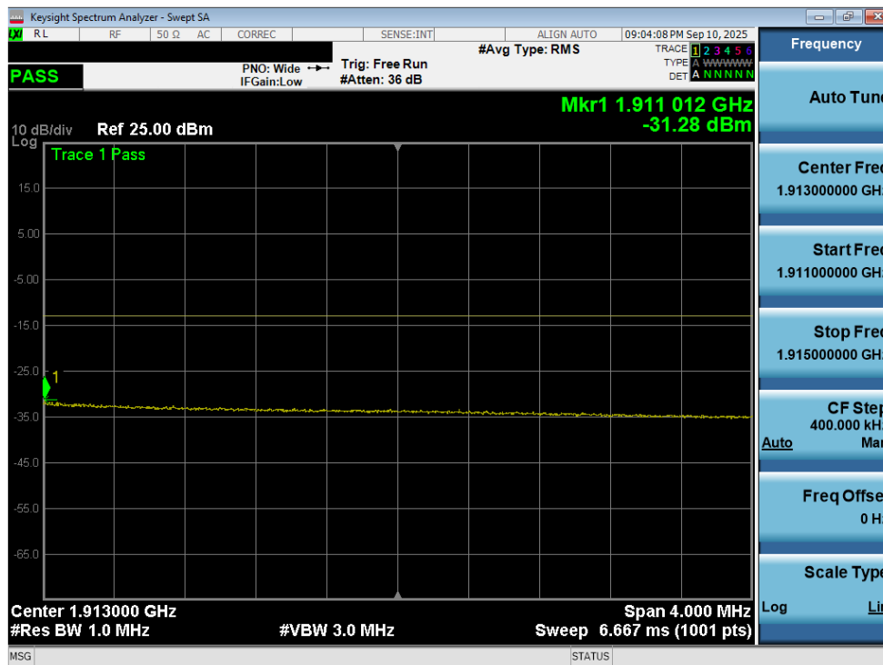
Plot 7-211. Extended Upper Band Edge Plot (LTE Band 2 - 20MHz QPSK – Full RB - Ant2)
