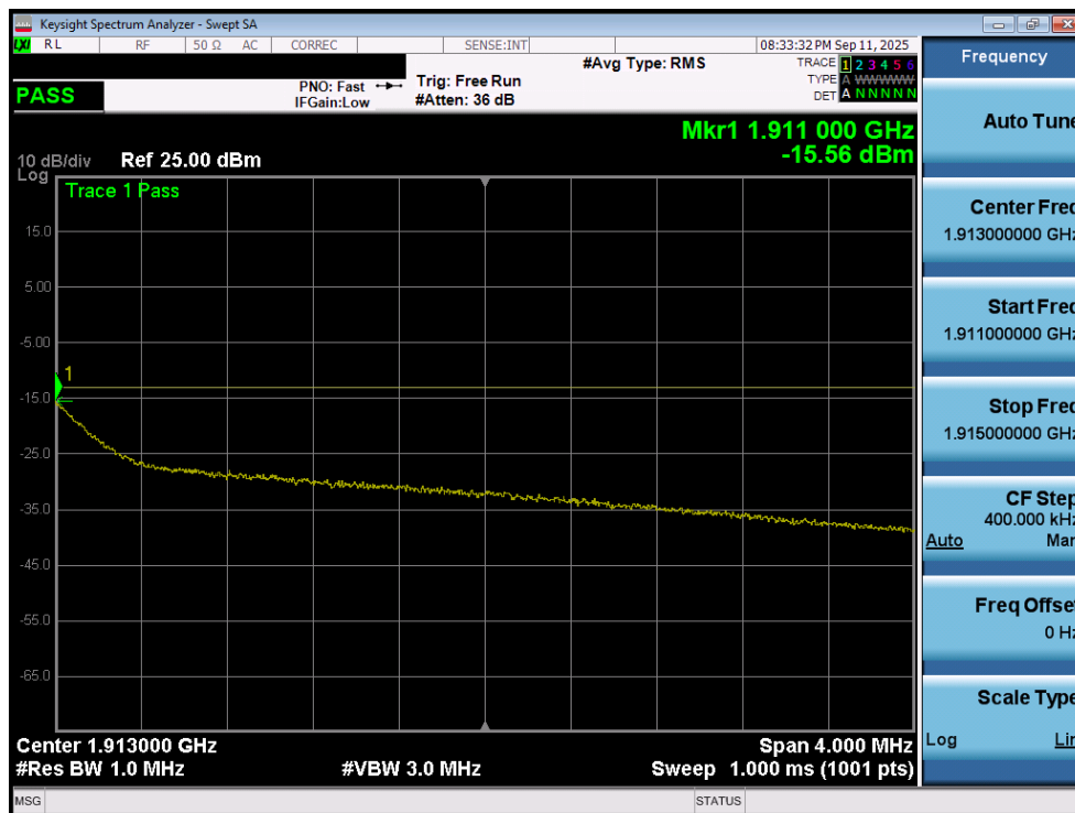
Plot 7-207. Extended Upper Band Edge Plot (WCDMA PCS – Ch. 9538 - Ant1)
