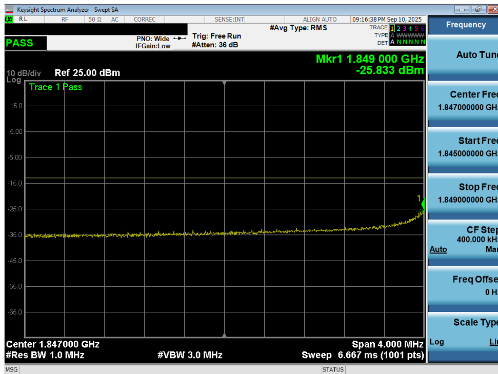
Plot 7-221. Extended Lower Band Edge Plot (LTE Band 25/2 - 10MHz QPSK – Full RB - Ant2)
