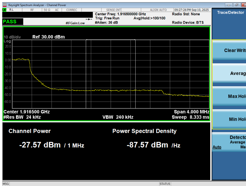
Plot 7-237. Extended Upper Band Edge Plot (LTE Band 25 - 3MHz QPSK – Full RB - Ant2)
