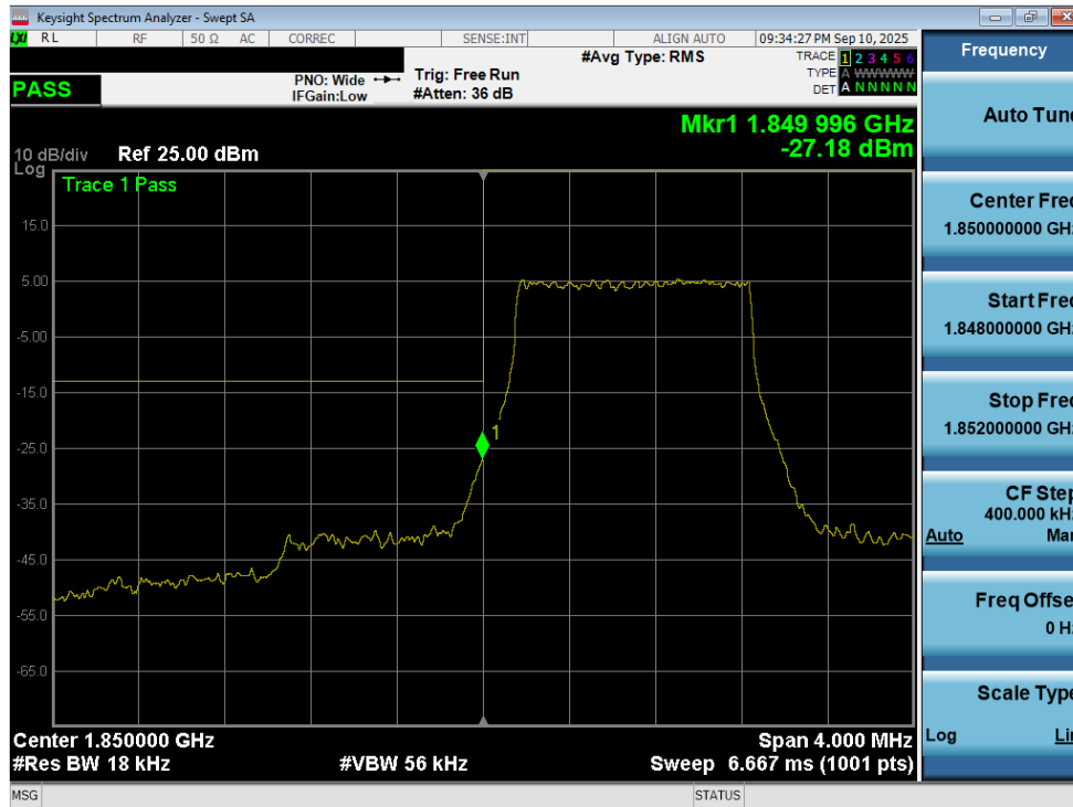
Plot 7-238. Lower Band Edge Plot (LTE Band 25/2 – 1.4MHz QPSK – Full RB - Ant2)
