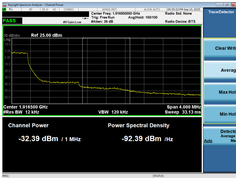
Plot 7-243. Extended Upper Band Edge Plot (LTE Band 25 – 1.4MHz QPSK – Full RB - Ant2)
