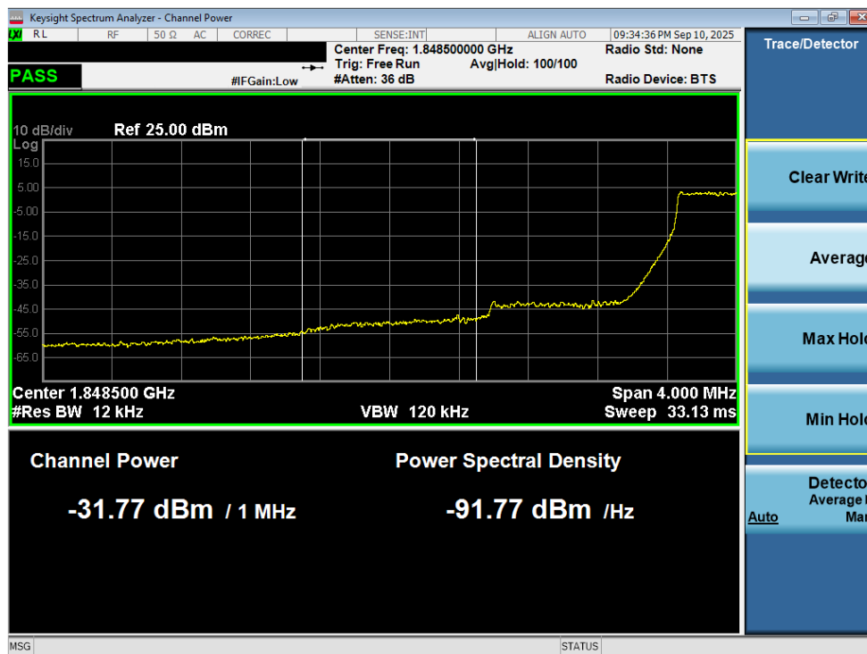
Plot 7-239. Extended Lower Band Edge Plot (LTE Band 25/2 – 1.4MHz QPSK – Full RB - Ant2)
