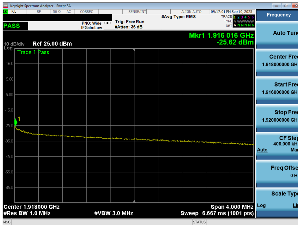
Plot 7-225. Extended Upper Band Edge Plot (LTE Band 25 - 10MHz QPSK – Full RB - Ant2)
