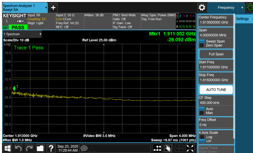
Plot 7-247. Extended Upper Band Edge Plot (NR Band n2 - 40MHz QPSK – Full RB - Ant2)
