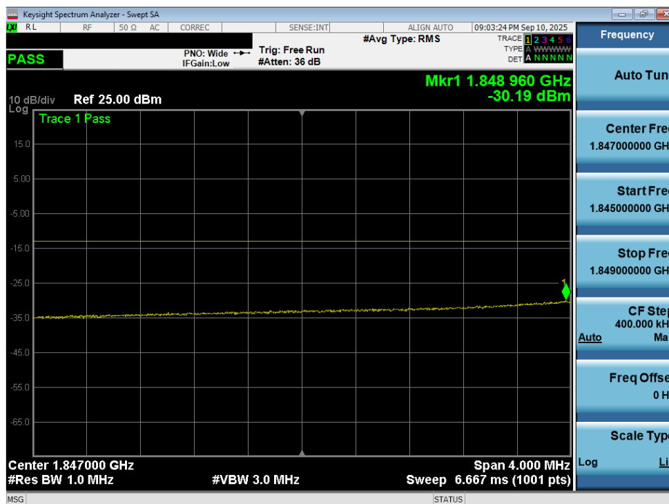
Plot 7-209. Extended Lower Band Edge Plot (LTE Band 25/2 - 20MHz QPSK – Full RB - Ant2)
