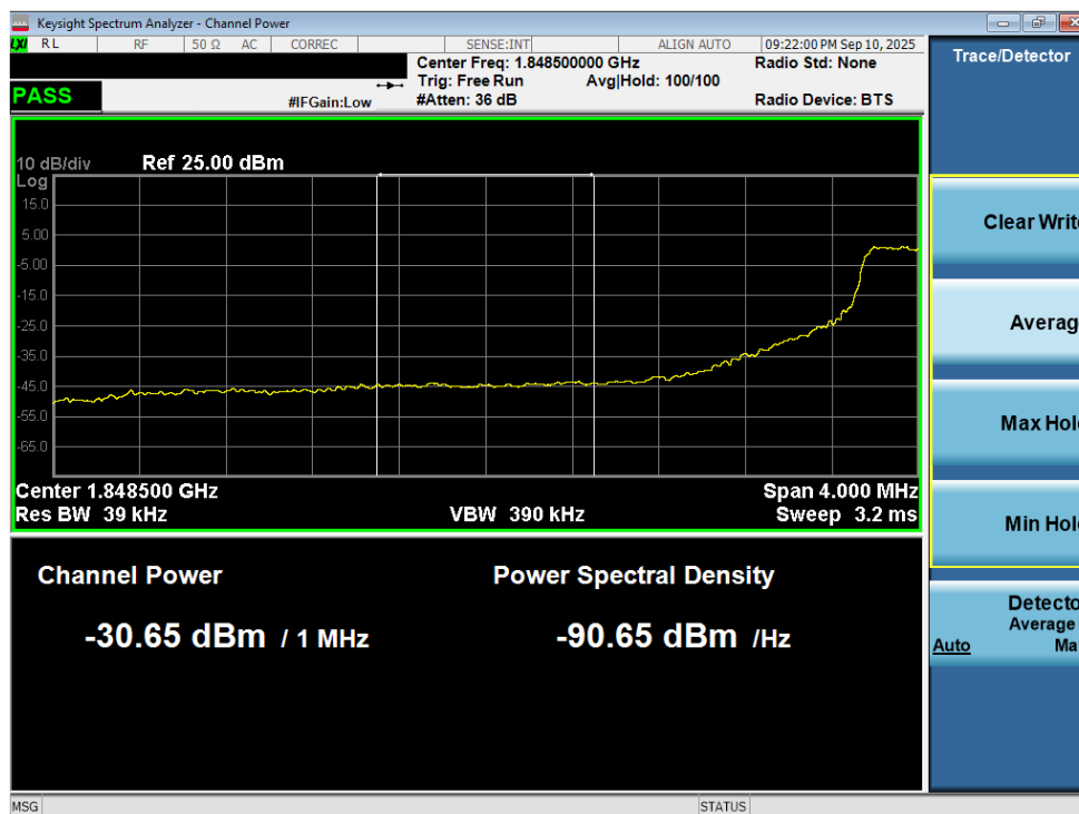
Plot 7-227. Extended Lower Band Edge Plot (LTE Band 25/2 - 5MHz QPSK – Full RB - Ant2)
