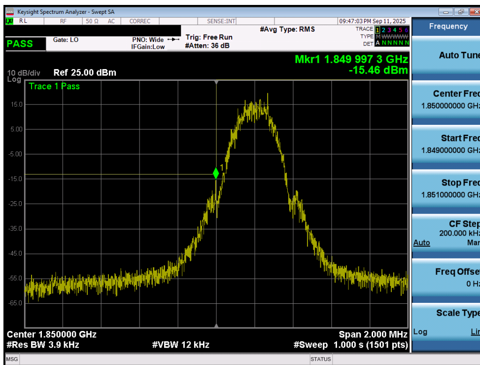
Plot 7-202. Lower Band Edge Plot (GPRS PCS – Ch. 512 - Ant1)
