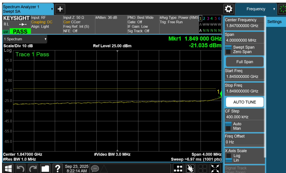
Plot 7-185. Extended Lower Band Edge Plot (NR Band n25/2 - 15MHz QPSK – Full RB - Ant1)
