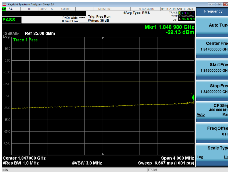
Plot 7-215. Extended Lower Band Edge Plot (LTE Band 25/2 - 15MHz QPSK – Full RB - Ant2)
