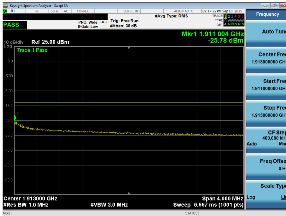
Plot 7-223. Extended Upper Band Edge Plot (LTE Band 2 - 10MHz QPSK – Full RB - Ant2)
