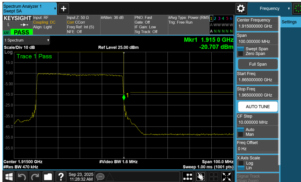
Plot 7-248. Upper Band Edge Plot (NR Band n25 - 40MHz QPSK – Full RB - Ant2)
