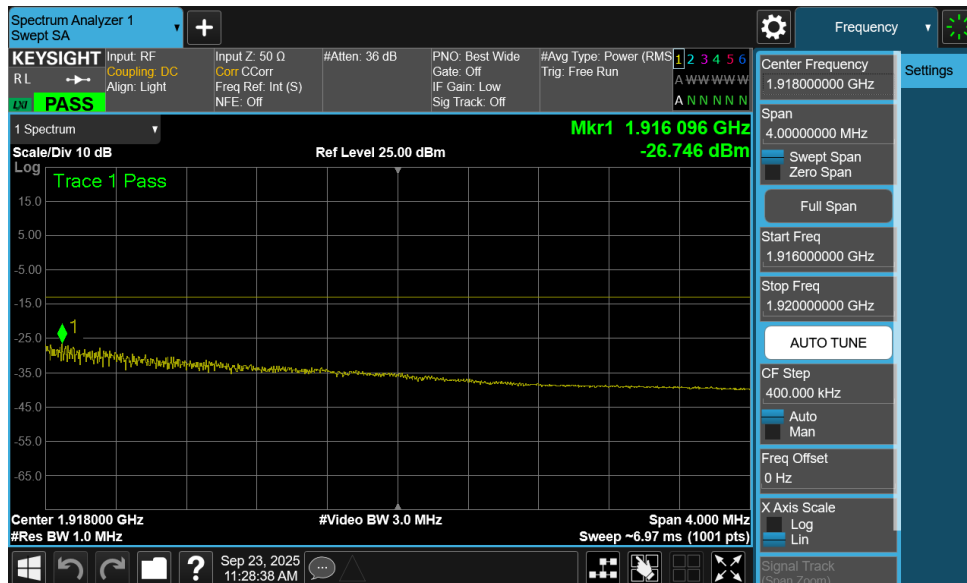
Plot 7-249. Extended Upper Band Edge Plot (NR Band n25 - 40MHz QPSK – Full RB - Ant2)
