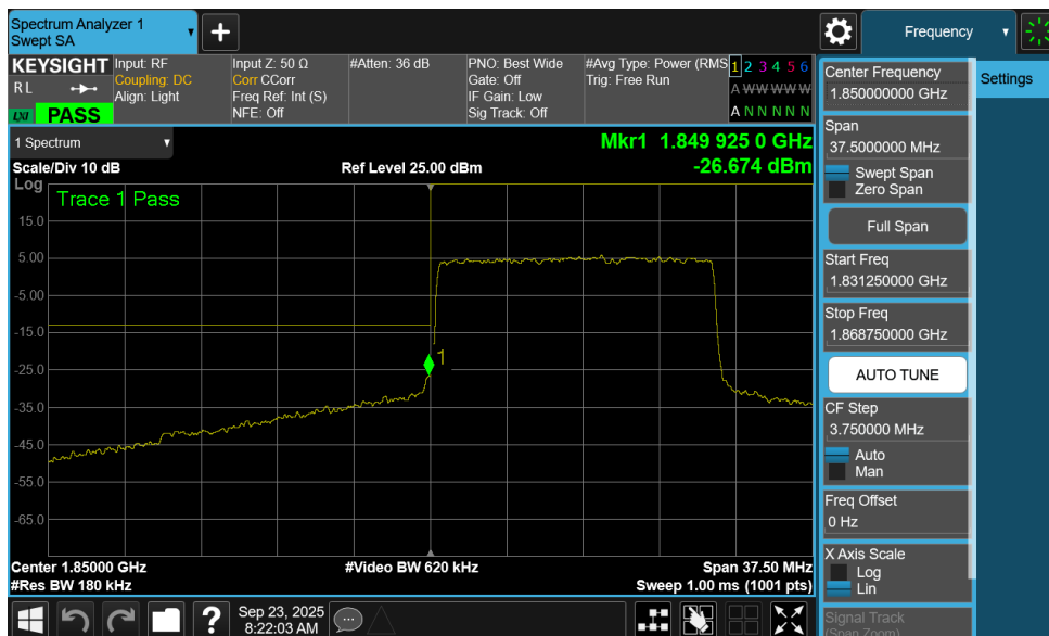
Plot 7-184. Lower Band Edge Plot (NR Band n25/2 - 15MHz QPSK – Full RB - Ant1)
