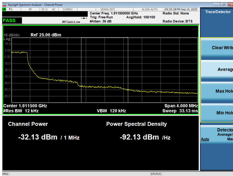
Plot 7-241. Extended Upper Band Edge Plot (LTE Band 2 – 1.4MHz QPSK – Full RB - Ant2)
