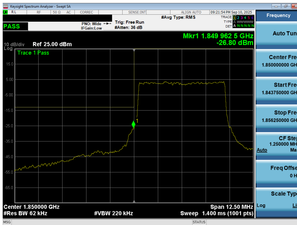
Plot 7-226. Lower Band Edge Plot (LTE Band 25/2 - 5MHz QPSK – Full RB - Ant2)
