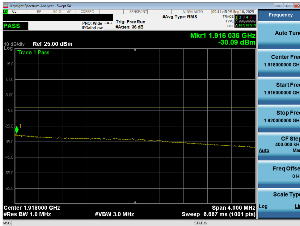
Plot 7-219. Extended Upper Band Edge Plot (LTE Band 25 - 15MHz QPSK – Full RB - Ant2)
