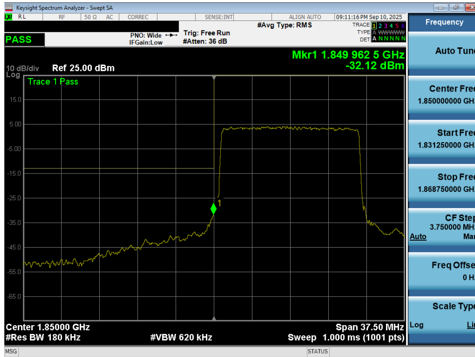
Plot 7-214. Lower Band Edge Plot (LTE Band 25/2 - 15MHz QPSK – Full RB - Ant2)
