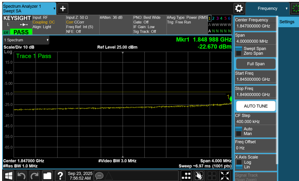
Plot 7-179. Extended Lower Band Edge Plot (NR Band n25/2 - 20MHz QPSK – Full RB - Ant1)
