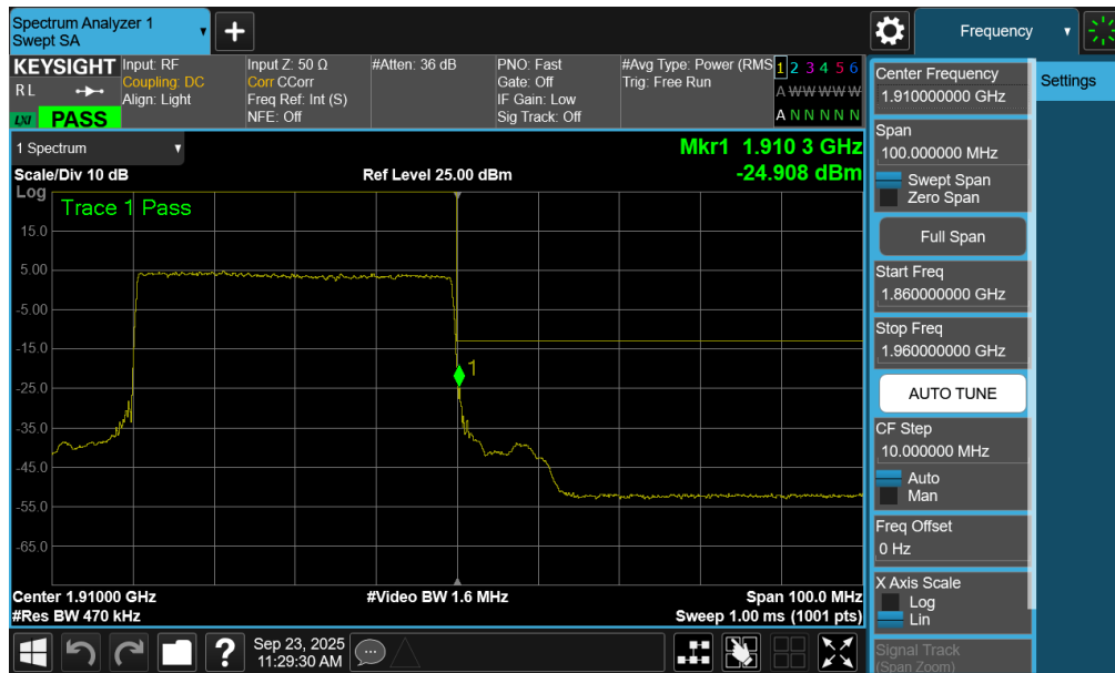
Plot 7-246. Upper Band Edge Plot (NR Band n2 - 40MHz QPSK – Full RB - Ant2)
