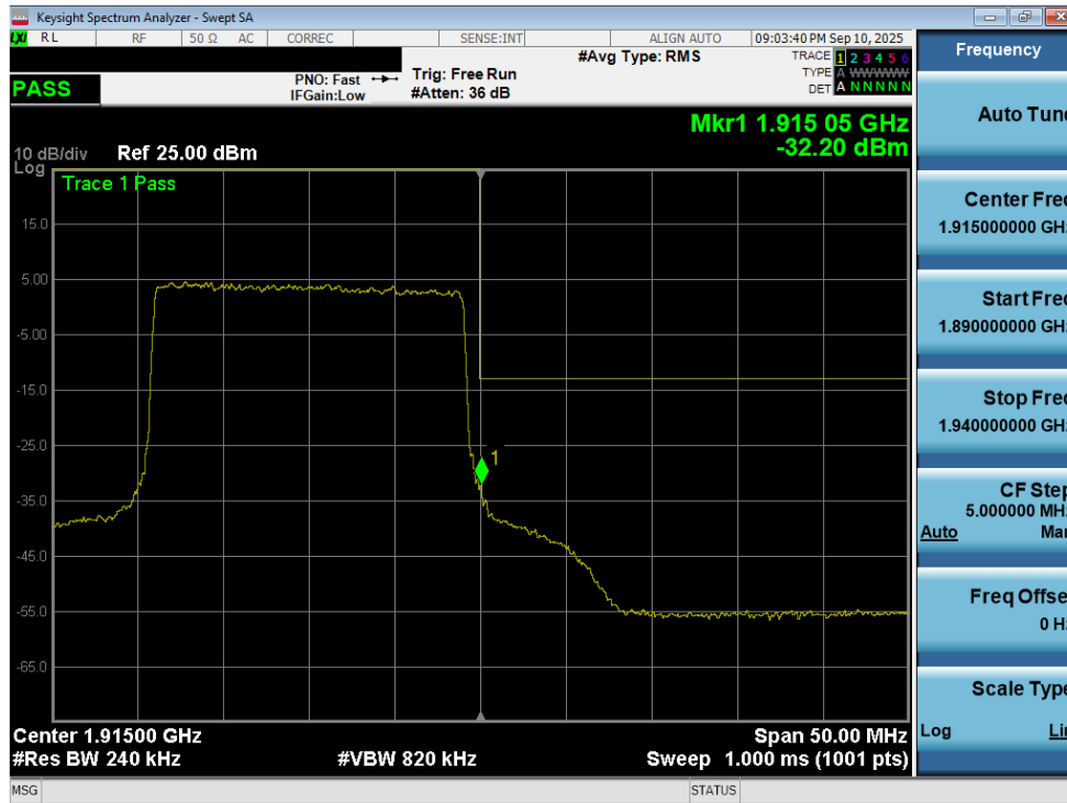
Plot 7-212. Upper Band Edge Plot (LTE Band 25 - 20MHz QPSK – Full RB - Ant2)
