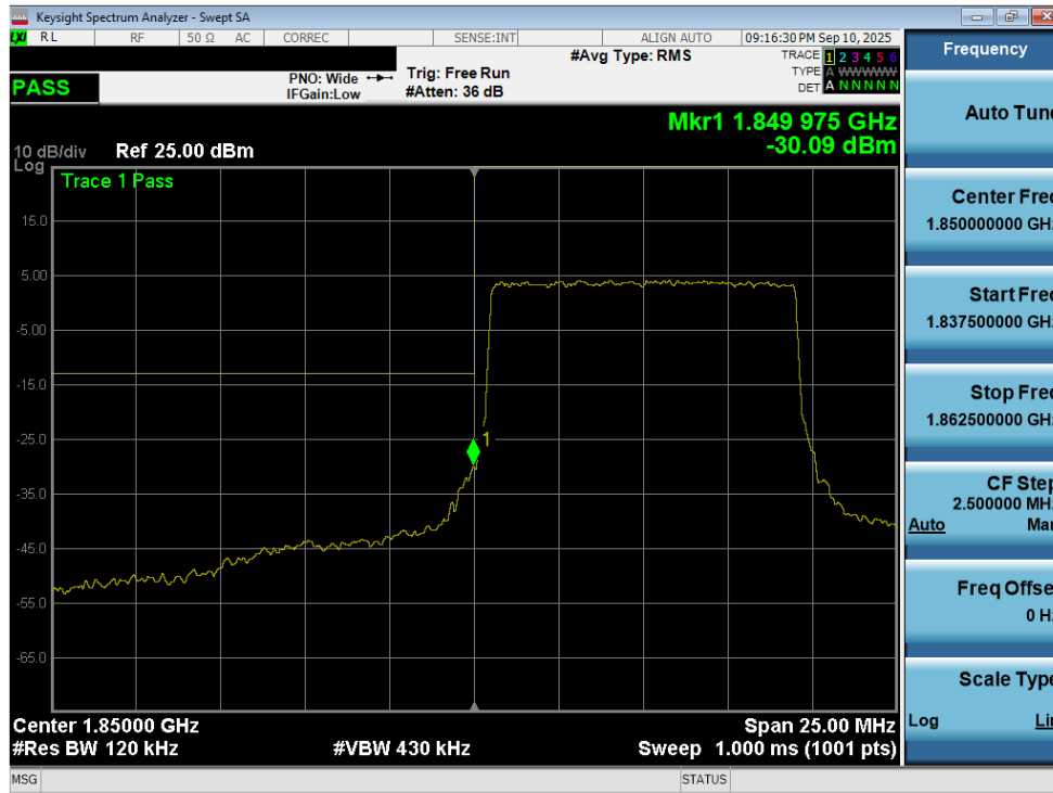
Plot 7-220. Lower Band Edge Plot (LTE Band 25/2 - 10MHz QPSK – Full RB - Ant2)
