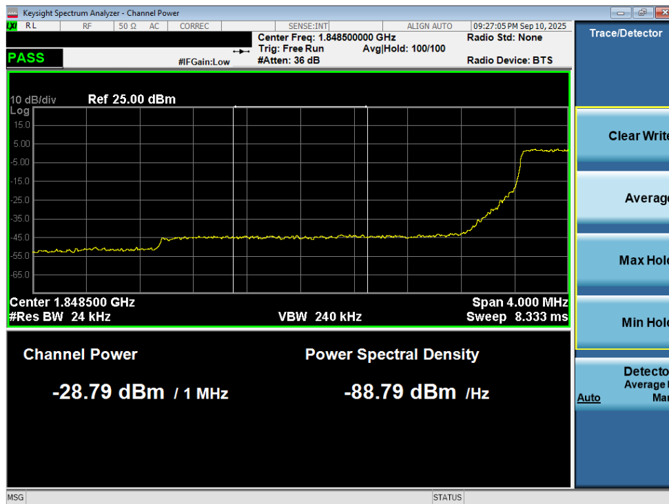
Plot 7-233. Extended Lower Band Edge Plot (LTE Band 25/2 - 3MHz QPSK – Full RB - Ant2)
