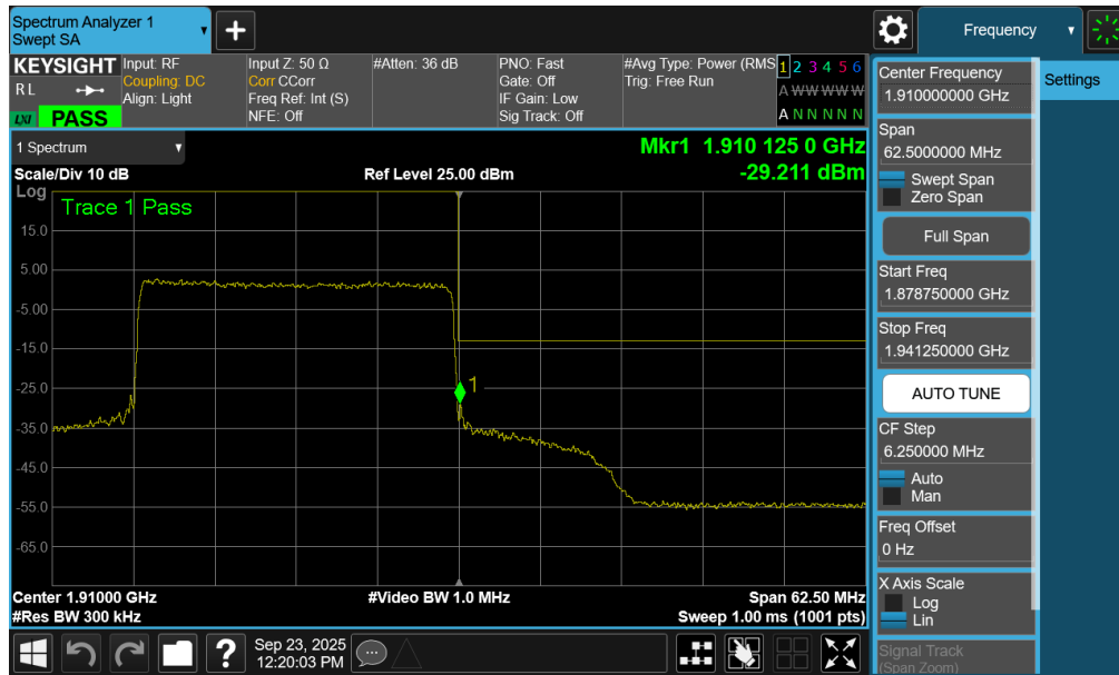
Plot 7-258. Upper Band Edge Plot (NR Band n2 - 25MHz QPSK – Full RB - Ant2)
