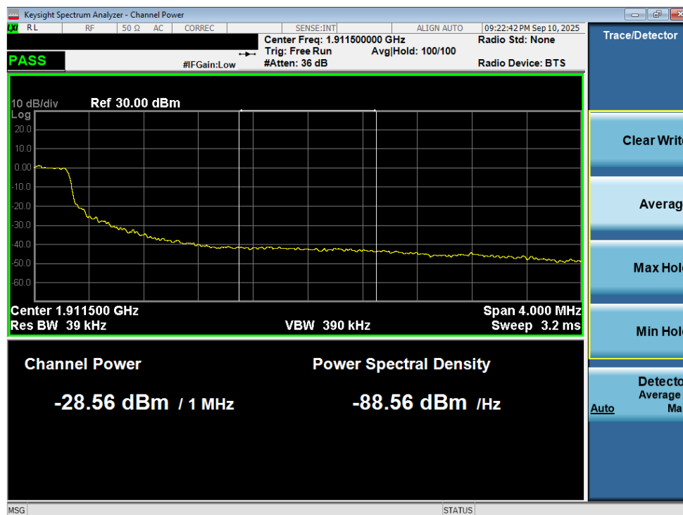
Plot 7-229. Extended Upper Band Edge Plot (LTE Band 2 - 5MHz QPSK – Full RB - Ant2)
