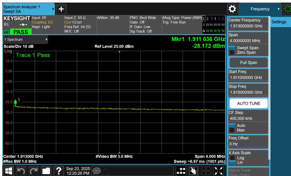
Plot 7-259. Extended Upper Band Edge Plot (NR Band n2 - 25MHz QPSK – Full RB - Ant2)
