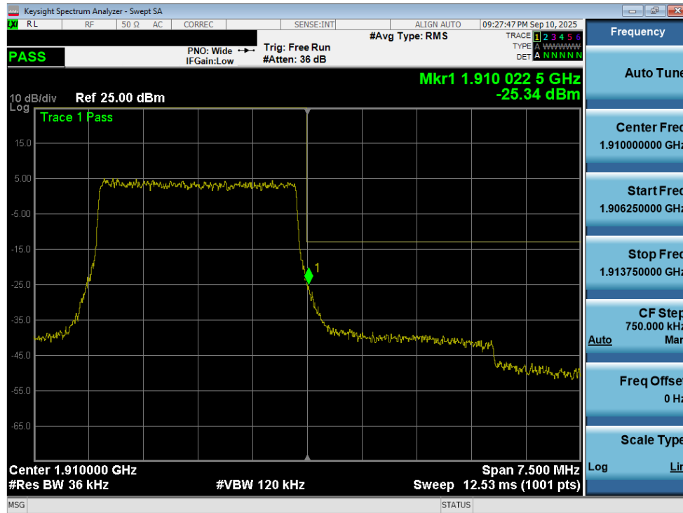
Plot 7-234. Upper Band Edge Plot (LTE Band 2 - 3MHz QPSK – Full RB - Ant2)
