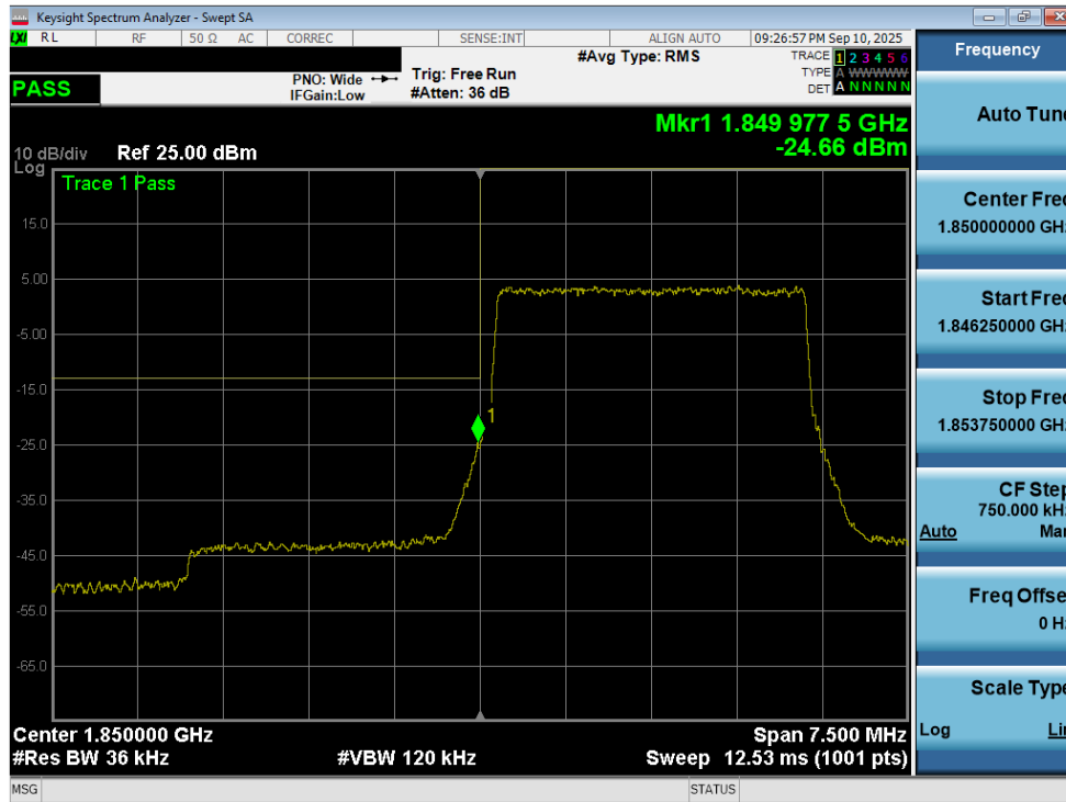
Plot 7-232. Lower Band Edge Plot (LTE Band 25/2 - 3MHz QPSK – Full RB - Ant2)
