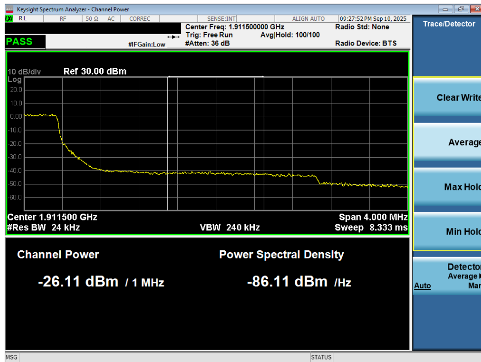
Plot 7-235. Extended Upper Band Edge Plot (LTE Band 2 - 3MHz QPSK – Full RB - Ant2)
