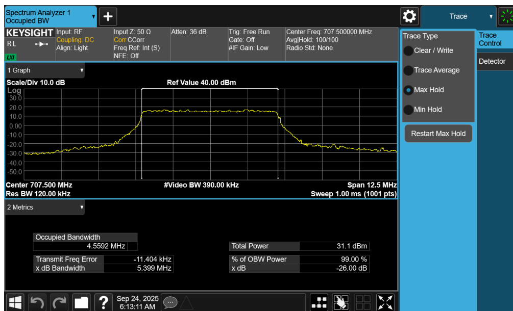
Plot 7-33. Occupied Bandwidth Plot (NR Band n12 - 5MHz CP-OFDM QPSK - Full RB – ANT1)
