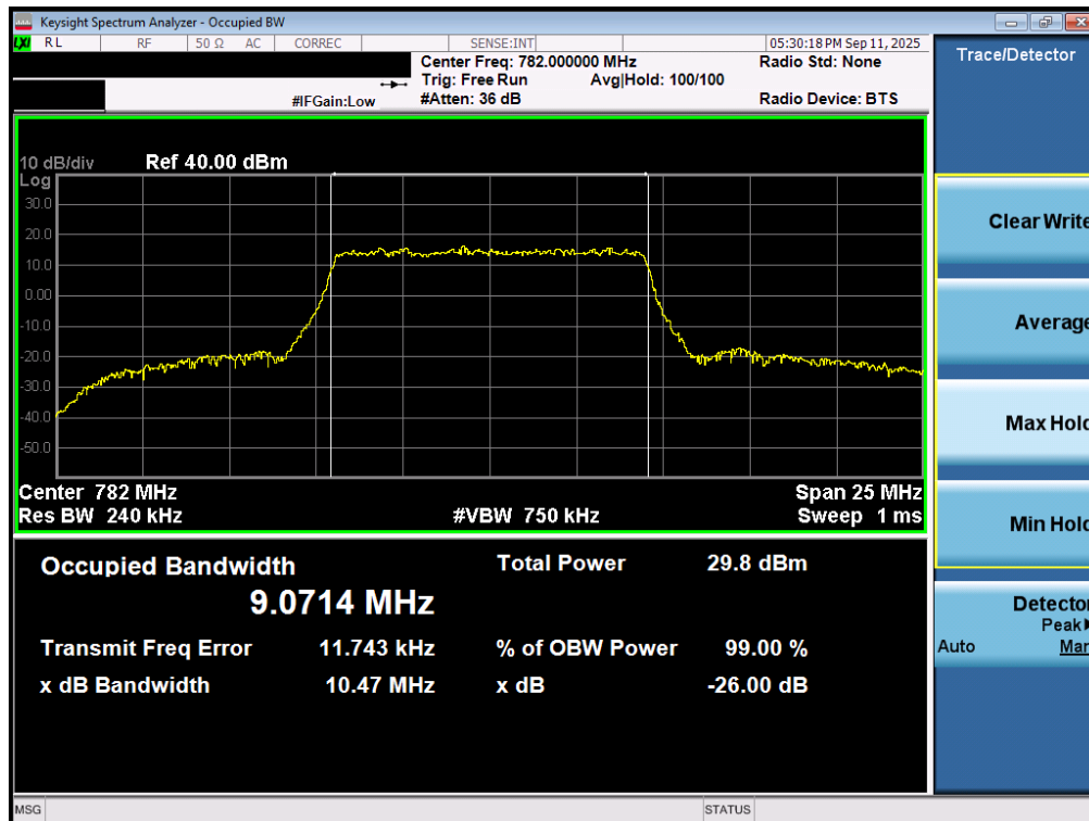
Plot 7-66. Occupied Bandwidth Plot (LTE Band 13 - 10MHz 16-QAM - Full RB – ANT2)
