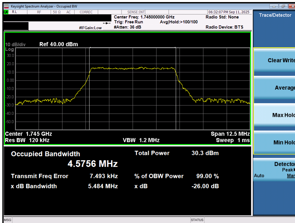
Plot 7-76. Occupied Bandwidth Plot (LTE Band 66/4 - 5MHz 16-QAM - Full RB - ANT2)
