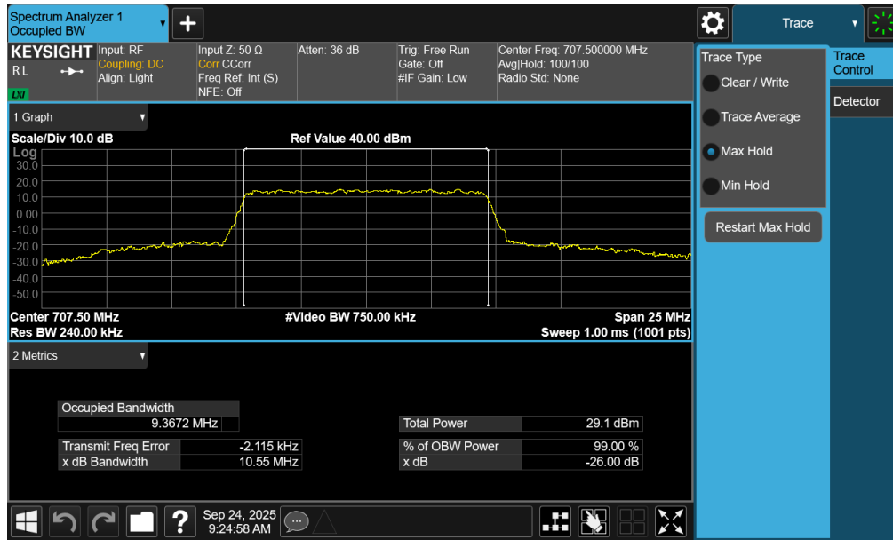
Plot 7-85. Occupied Bandwidth Plot (NR Band n12 - 10MHz CP-OFDM QPSK - Full RB – ANT2)
