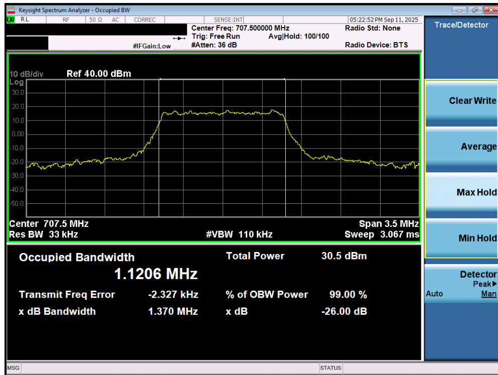
Plot 7-64. Occupied Bandwidth Plot (LTE Band 12 – 1.4MHz 16-QAM - Full RB – ANT2)
