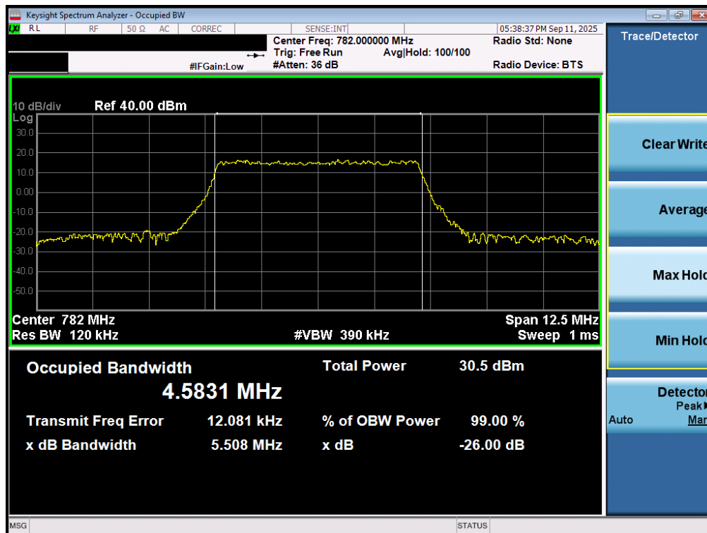
Plot 7-68. Occupied Bandwidth Plot (LTE Band 13 - 5MHz 16-QAM - Full RB – ANT2)
