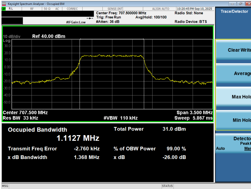
Plot 7-8. Occupied Bandwidth Plot (LTE Band 12 – 1.4MHz QPSK - Full RB – ANT1)
