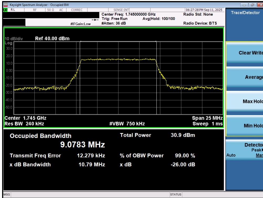
Plot 7-73. Occupied Bandwidth Plot (LTE Band 66/4 - 10MHz QPSK - Full RB - ANT2)
