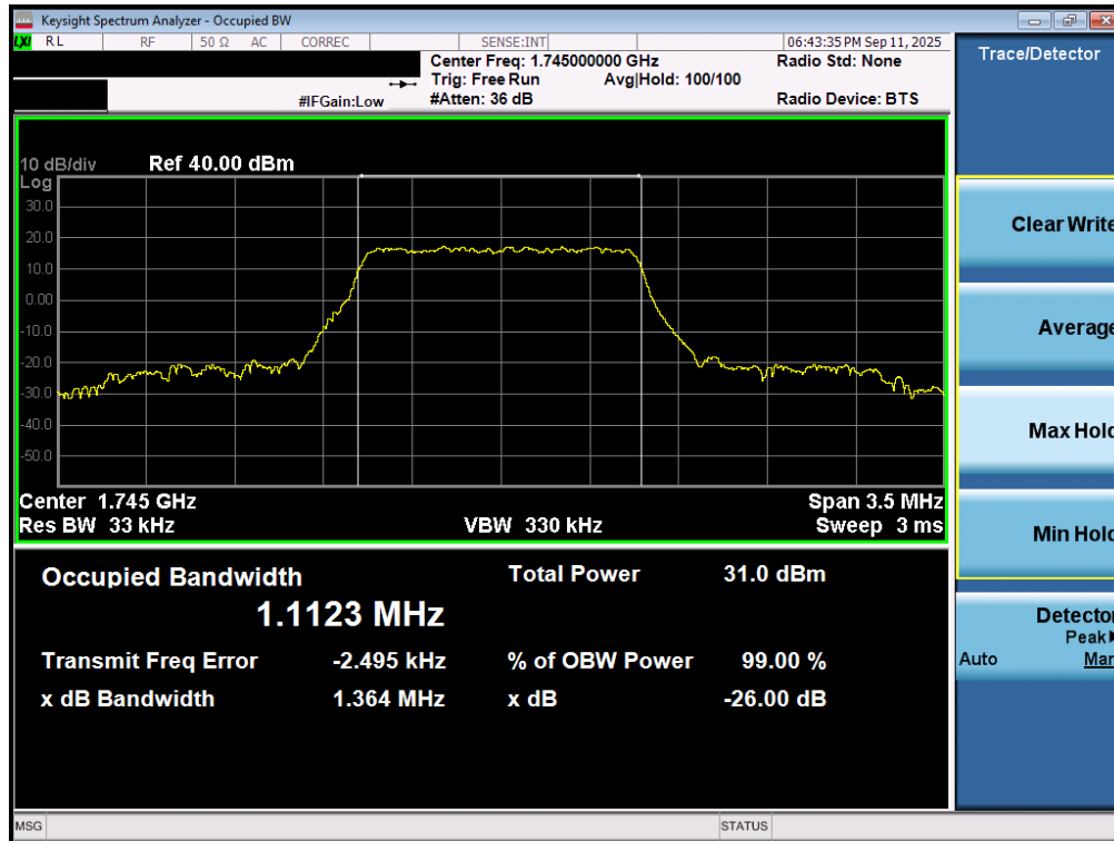
Plot 7-79. Occupied Bandwidth Plot (LTE Band 66/4 - 1.4MHz QPSK - Full RB - ANT2)
