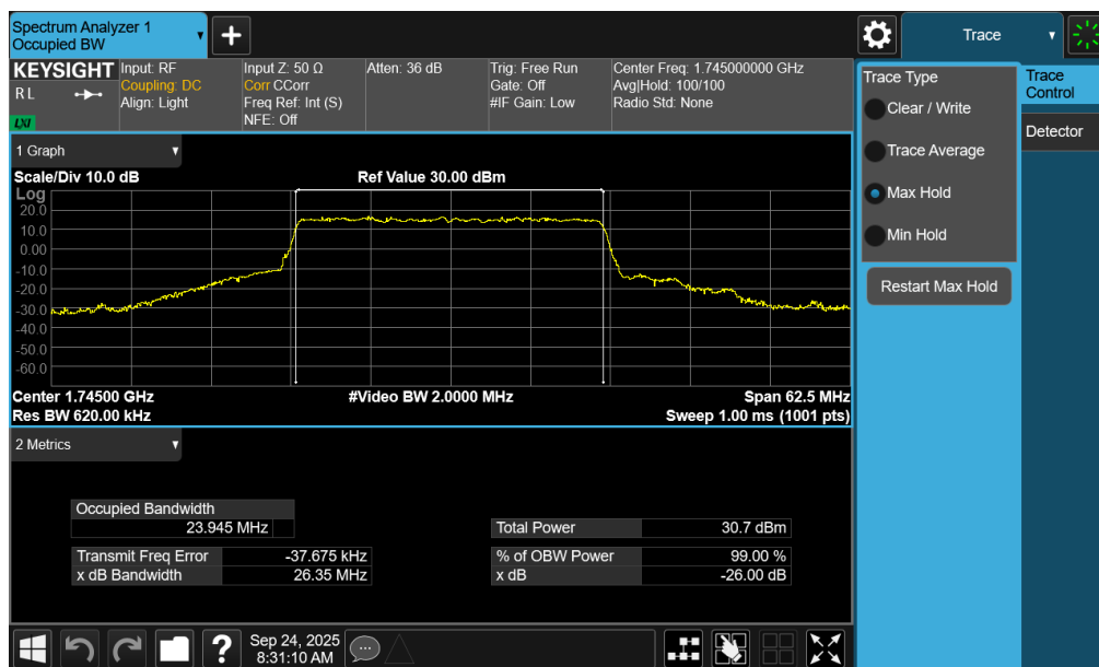
Plot 7-42. Occupied Bandwidth Plot (NR Band n66 - 25.0MHz CP-OFDM QPSK - Full RB – ANT1)
