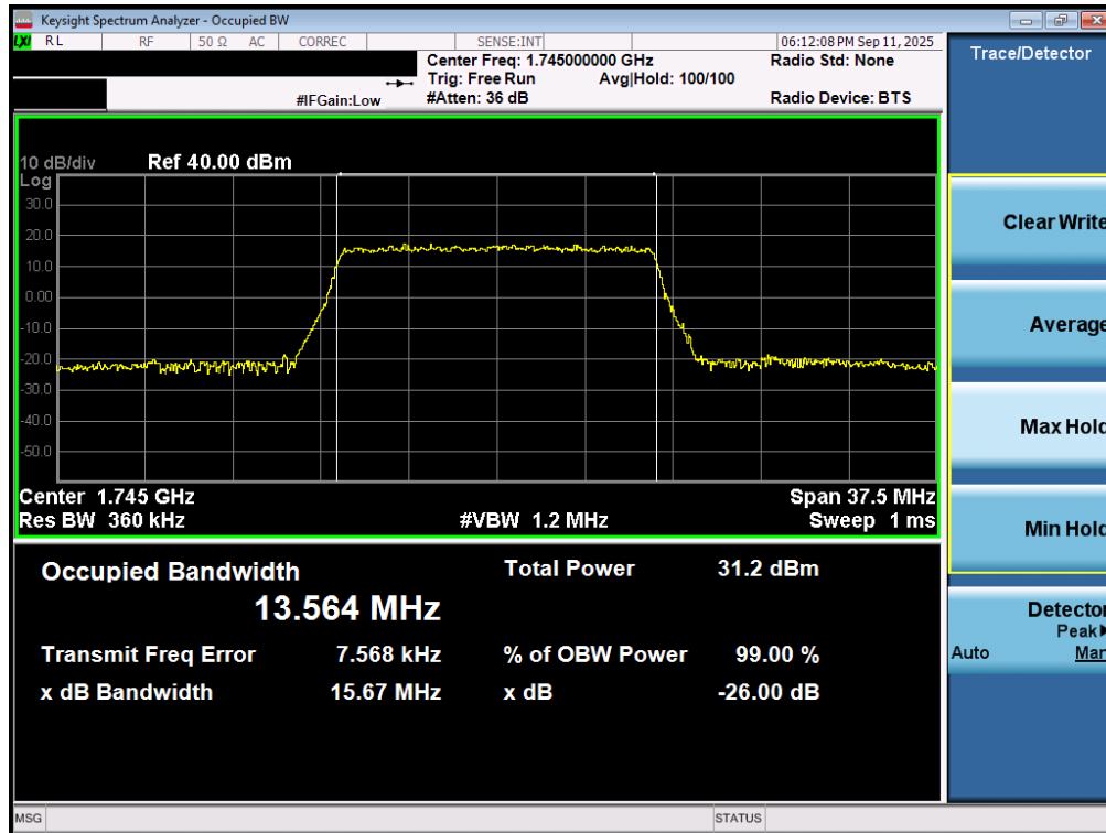
Plot 7-71. Occupied Bandwidth Plot (LTE Band 66/4 - 15MHz QPSK - Full RB - ANT2)
