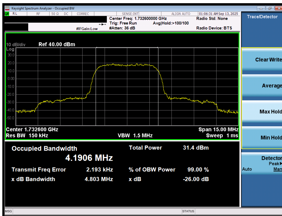
Plot 7-56. Occupied Bandwidth Plot (WCDMA, Ch. 1413 – ANT2)
