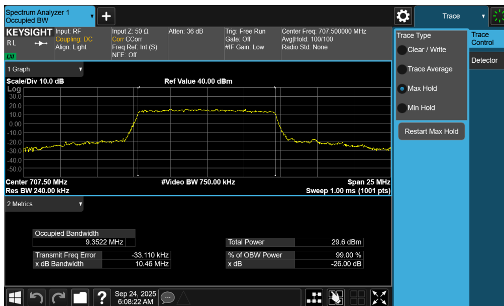
Plot 7-31. Occupied Bandwidth Plot (NR Band n12 - 10MHz CP-OFDM 16-QAM - Full RB – ANT1)
