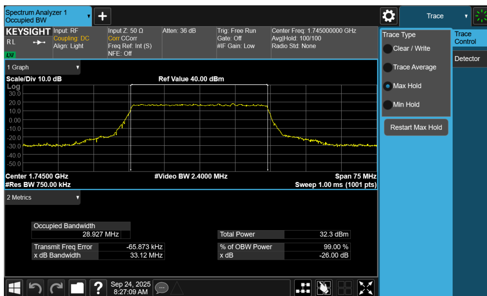
Plot 7-39. Occupied Bandwidth Plot (NR Band n66 - 30.0MHz CP-OFDM QPSK - Full RB – ANT1)
