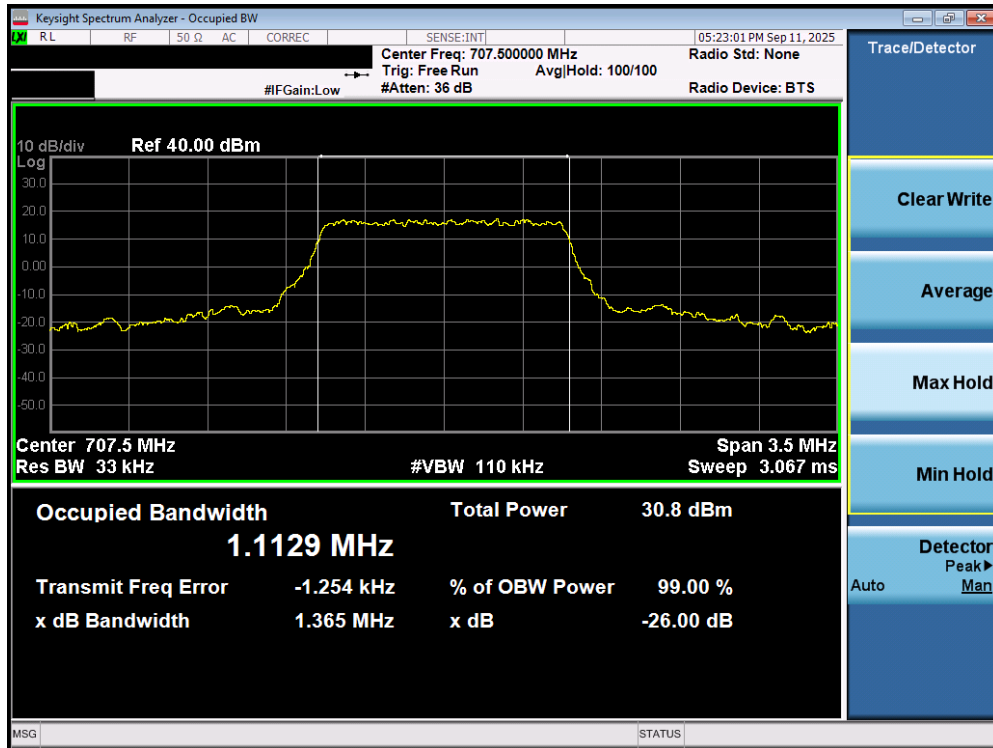
Plot 7-63. Occupied Bandwidth Plot (LTE Band 12 – 1.4MHz QPSK - Full RB – ANT2)
