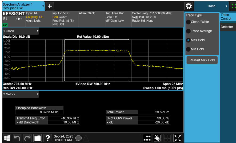
Plot 7-30. Occupied Bandwidth Plot (NR Band n12 - 10MHz CP-OFDM QPSK - Full RB – ANT1)
