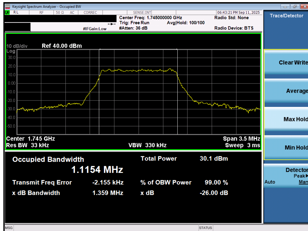
Plot 7-80. Occupied Bandwidth Plot (LTE Band 66/4 - 1.4MHz 16-QAM - Full RB - ANT2)
