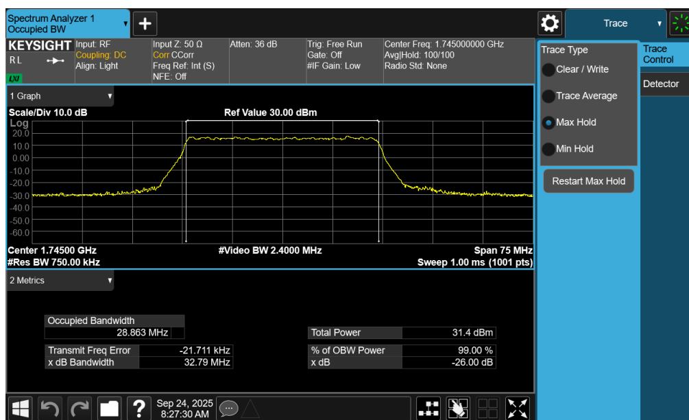
Plot 7-40. Occupied Bandwidth Plot (NR Band n66 - 30.0MHz CP-OFDM 16QAM - Full RB – ANT1)
