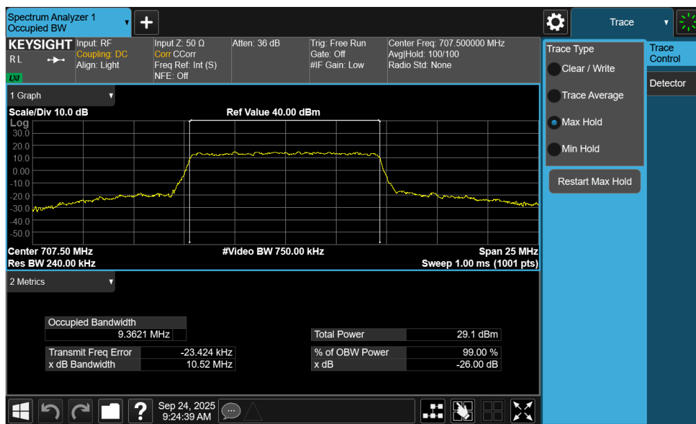
Plot 7-86. Occupied Bandwidth Plot (NR Band n12 - 10MHz CP-OFDM 16-QAM - Full RB – ANT2)
