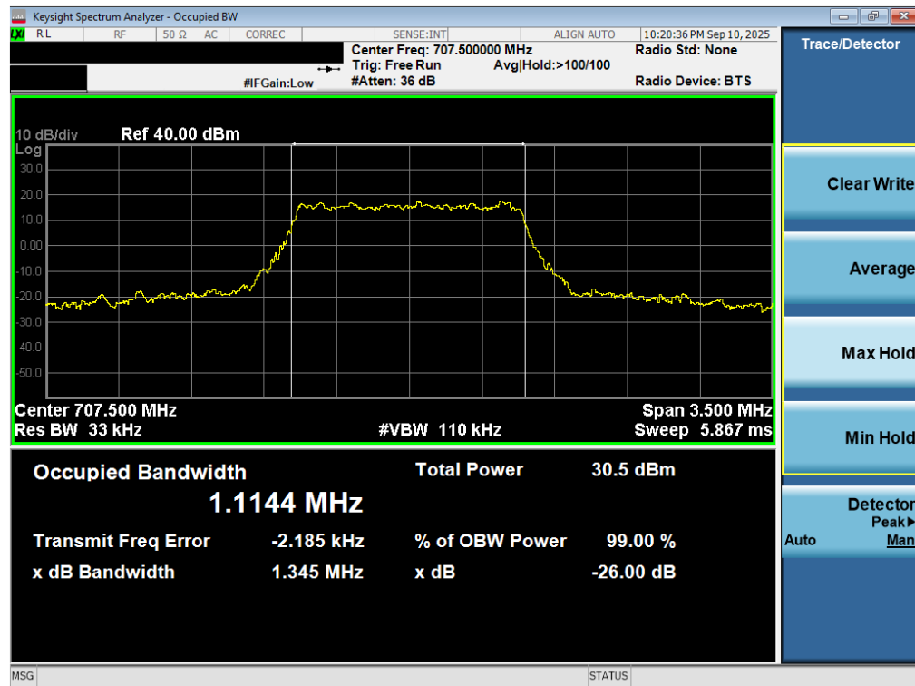
Plot 7-9. Occupied Bandwidth Plot (LTE Band 12 – 1.4MHz 16-QAM - Full RB – ANT1)
