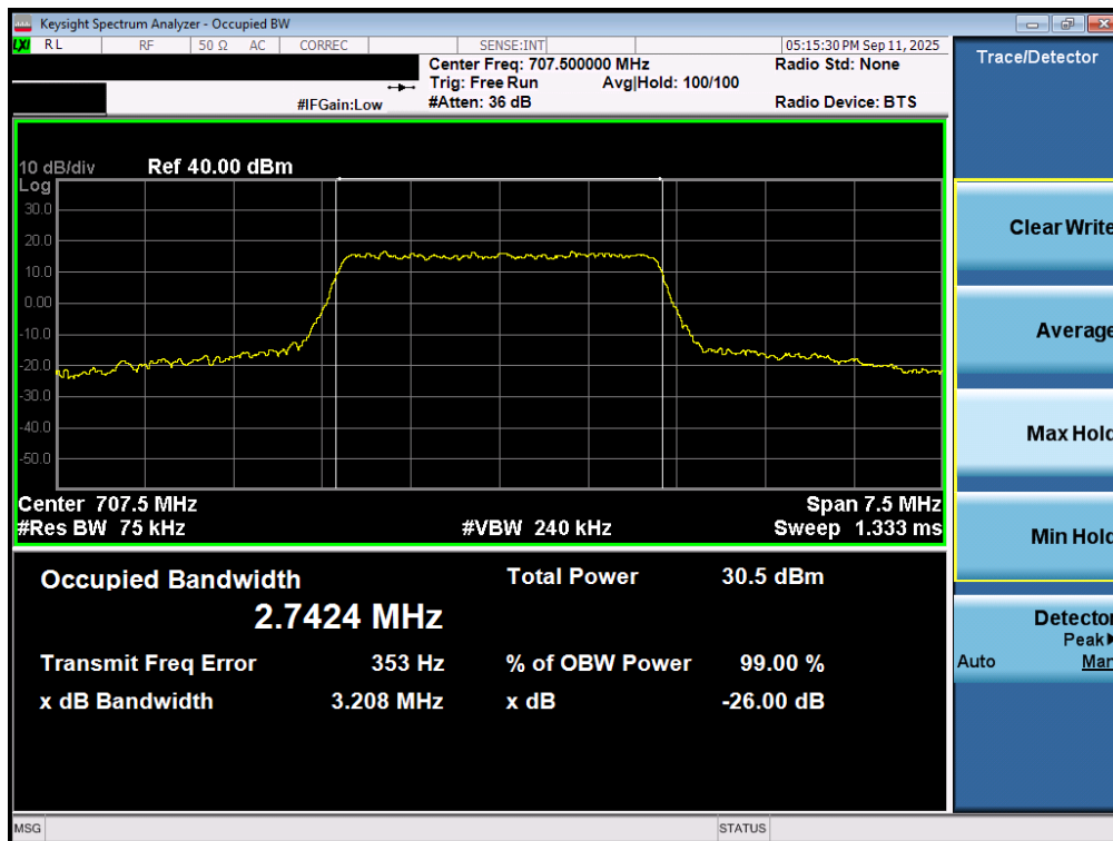
Plot 7-62. Occupied Bandwidth Plot (LTE Band 12 - 3MHz 16-QAM - Full RB – ANT2)
