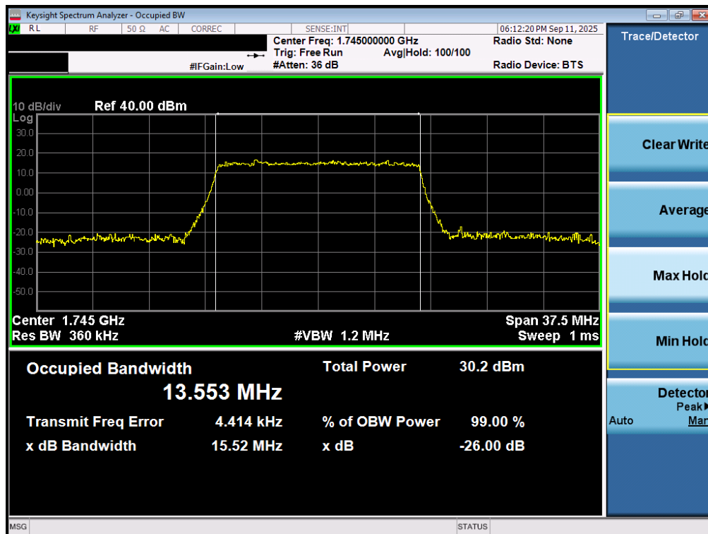
Plot 7-72. Occupied Bandwidth Plot (LTE Band 66/4 - 15MHz 16-QAM - Full RB - ANT2)
