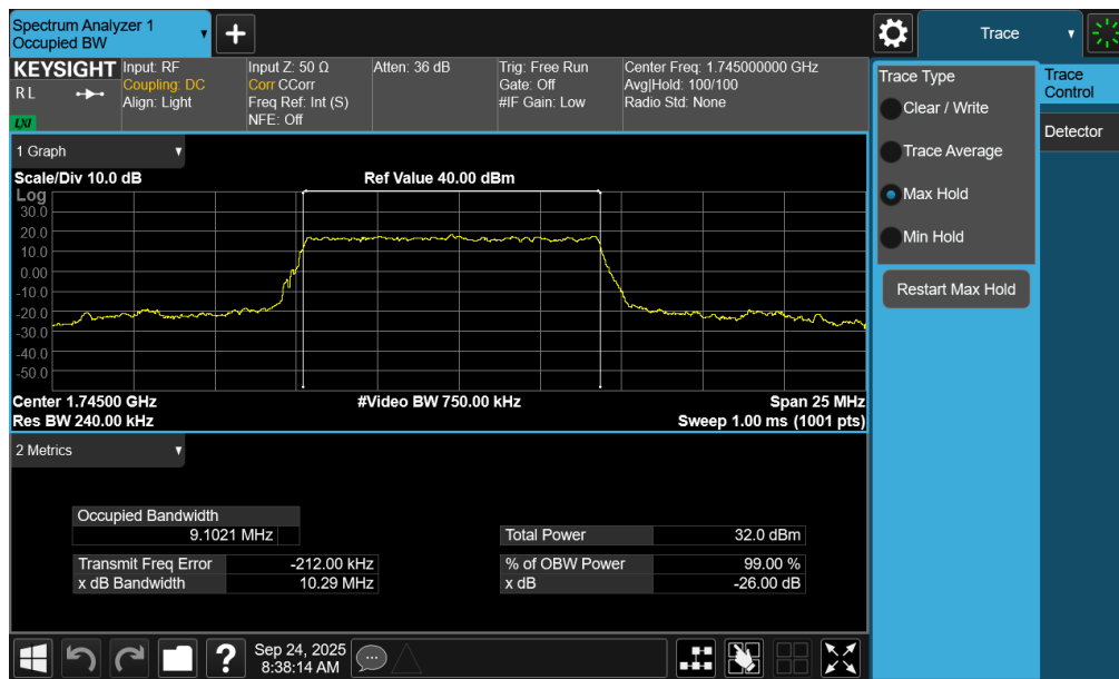
Plot 7-50. Occupied Bandwidth Plot (NR Band n66 - 10.0MHz DFT-s-OFDM BPSK - Full RB – ANT1)
