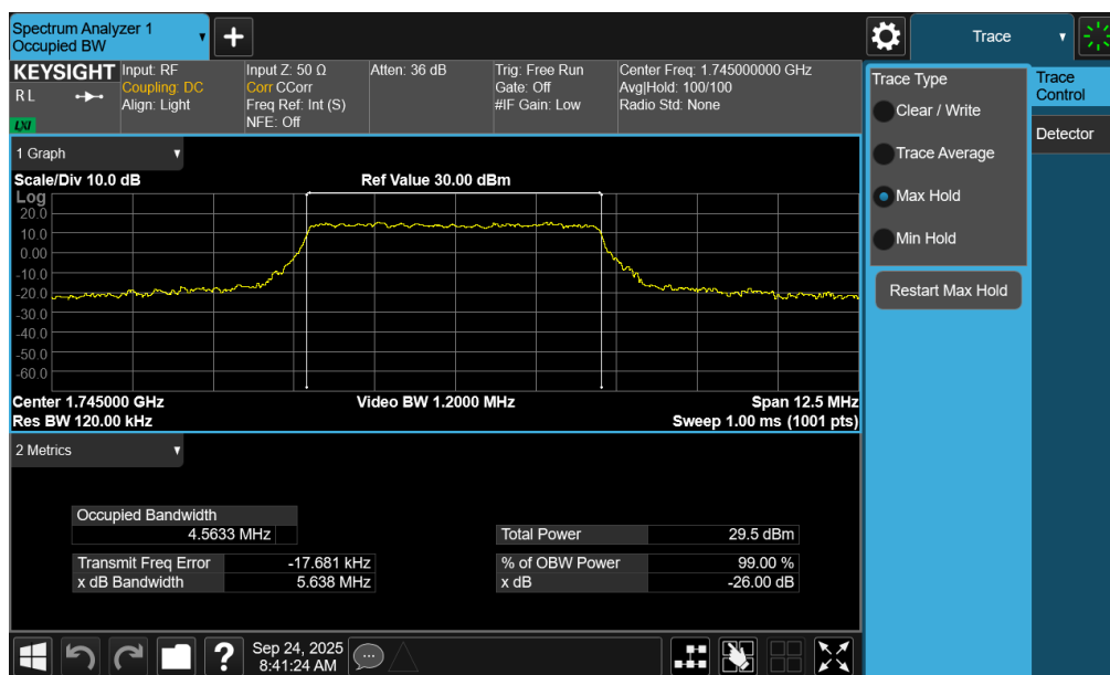
Plot 7-55. Occupied Bandwidth Plot (NR Band n66 - 5.0MHz CP-OFDM 16QAM - Full RB – ANT1)
