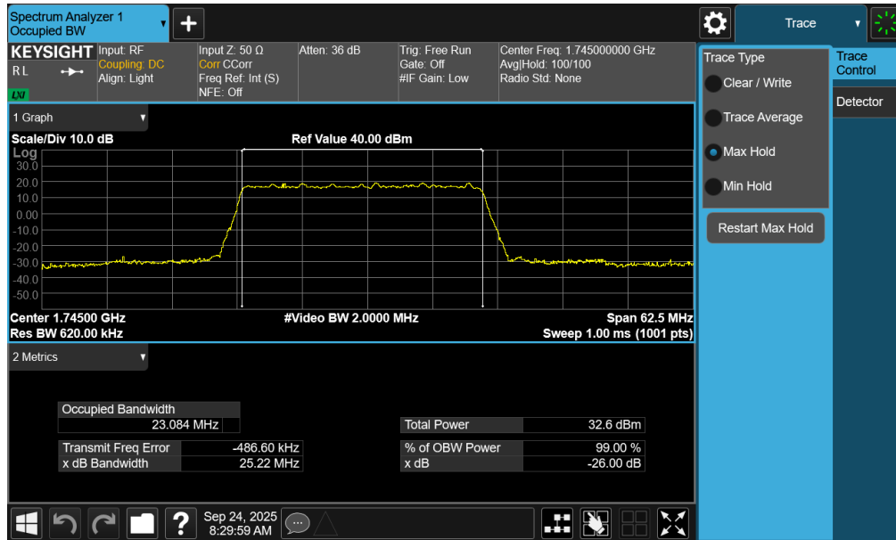
Plot 7-41. Occupied Bandwidth Plot (NR Band n66 - 25.0MHz DFT-s-OFDM BPSK - Full RB – ANT1)
