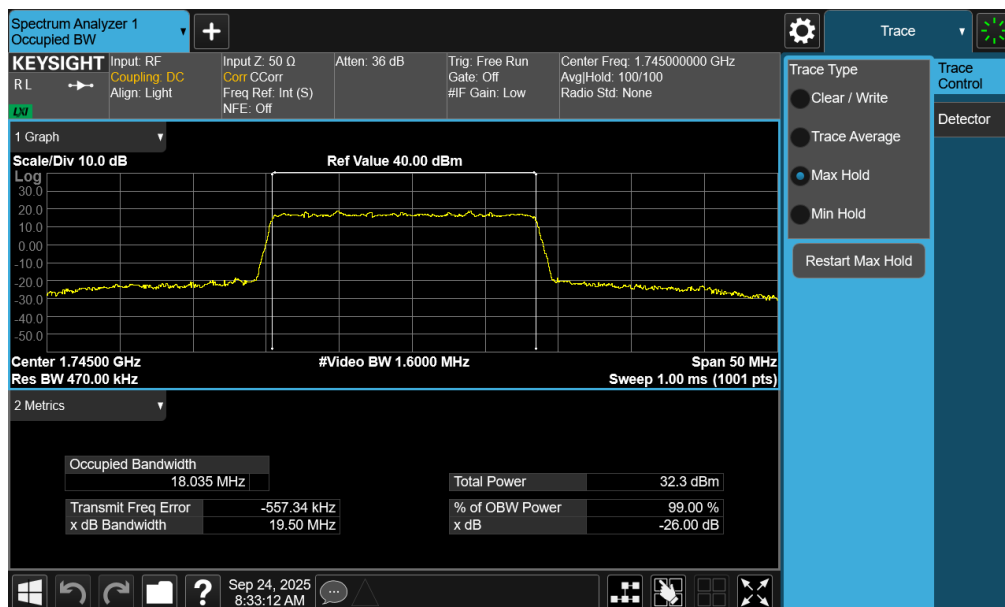
Plot 7-44. Occupied Bandwidth Plot (NR Band n66 - 20.0MHz DFT-s-OFDM BPSK - Full RB – ANT1)
