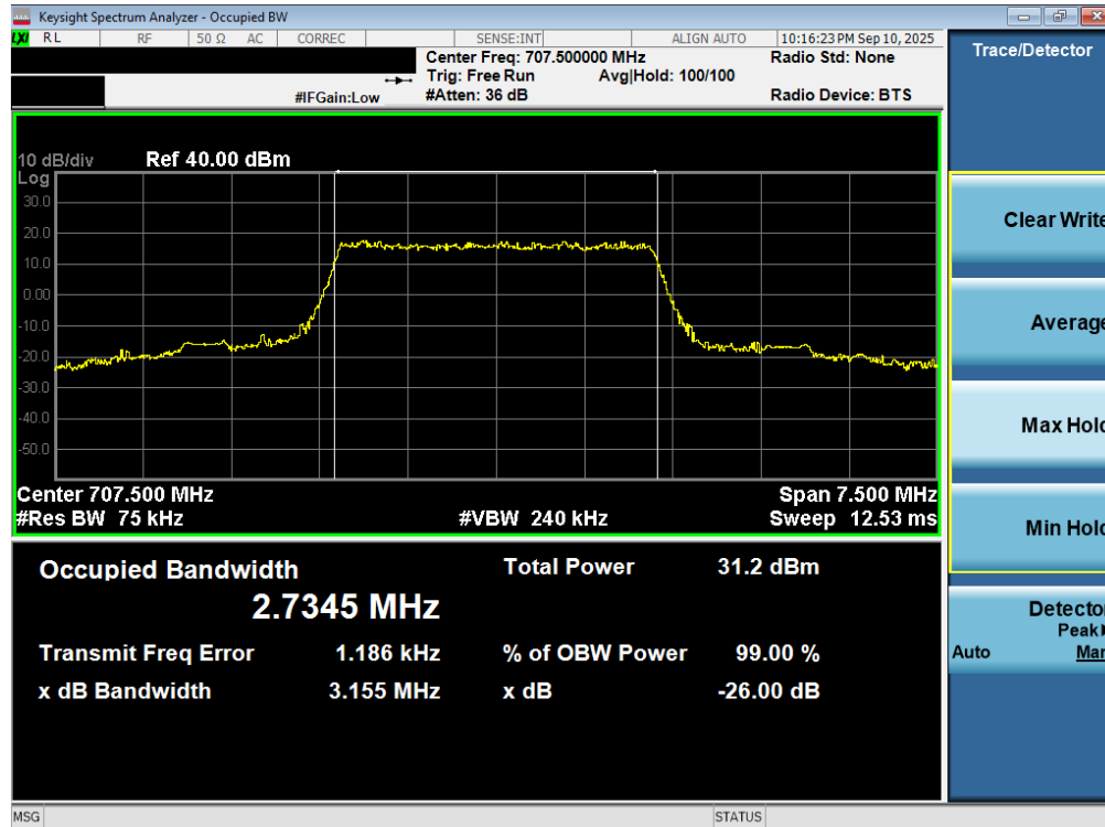
Plot 7-6. Occupied Bandwidth Plot (LTE Band 12 - 3MHz QPSK - Full RB – ANT1)
