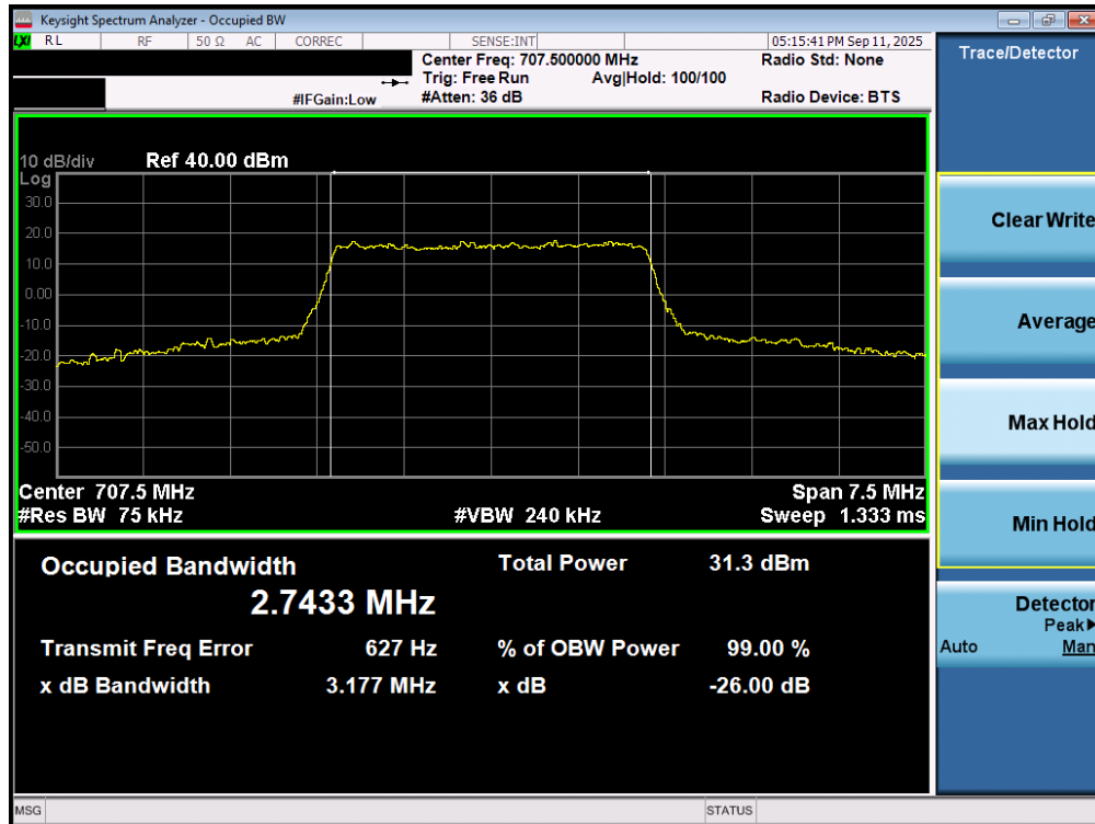
Plot 7-61. Occupied Bandwidth Plot (LTE Band 12 - 3MHz QPSK - Full RB – ANT2)
