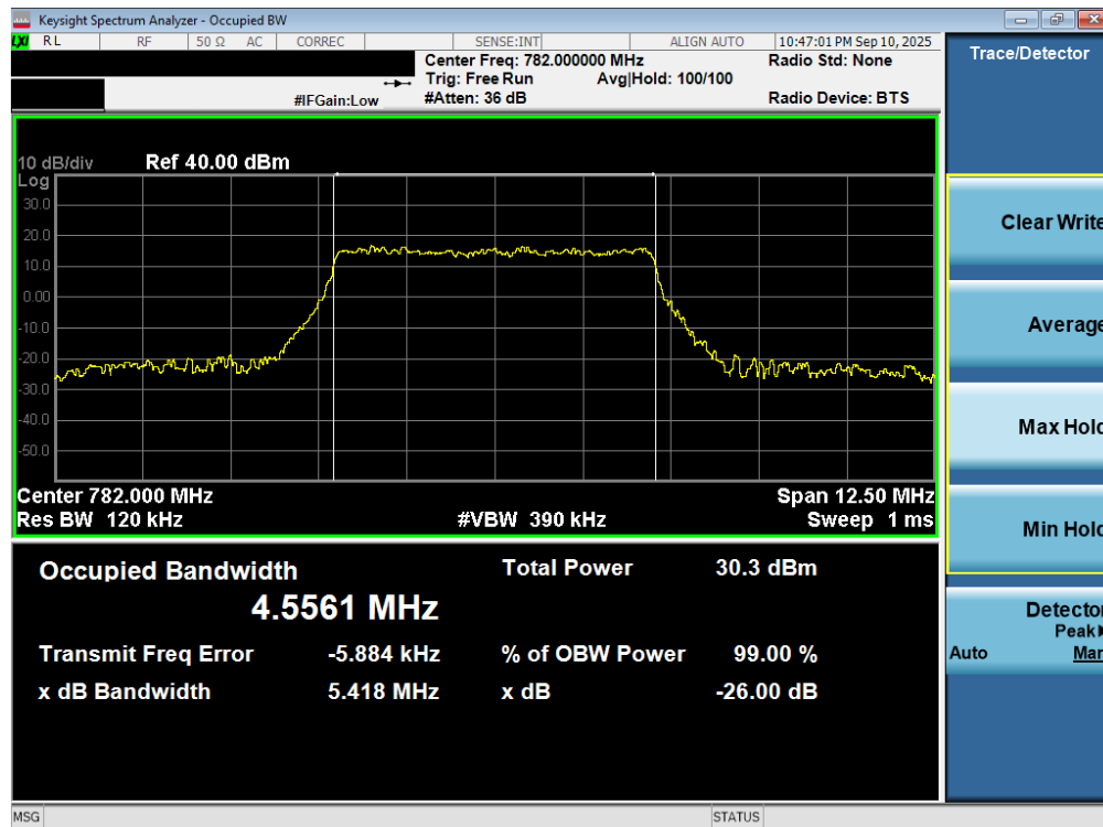
Plot 7-13. Occupied Bandwidth Plot (LTE Band 13 - 5MHz 16-QAM - Full RB – ANT1)
