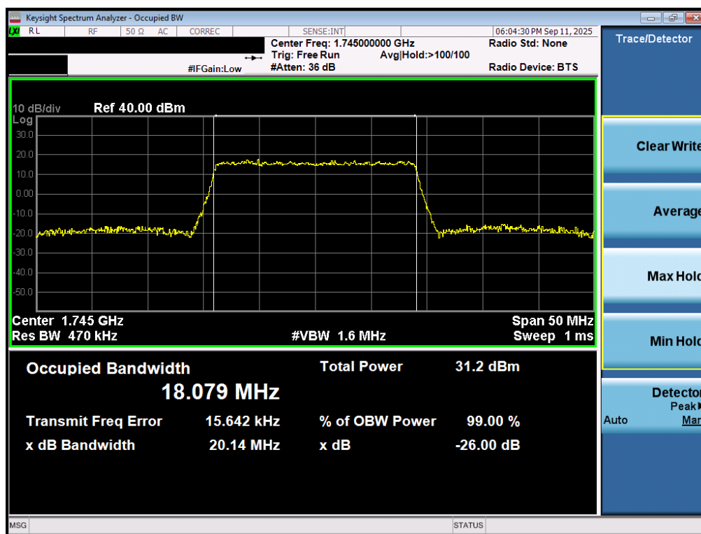
Plot 7-69. Occupied Bandwidth Plot (LTE Band 66/4 - 20MHz QPSK - Full RB - ANT2)
