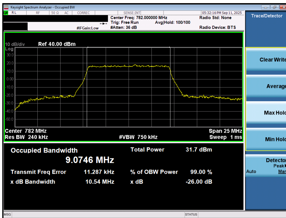
Plot 7-65. Occupied Bandwidth Plot (LTE Band 13 - 10MHz QPSK - Full RB – ANT2)
