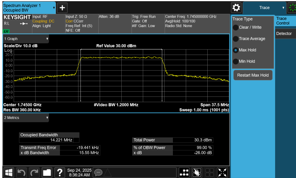
Plot 7-49. Occupied Bandwidth Plot (NR Band n66 - 15.0MHz CP-OFDM 16QAM - Full RB – ANT1)
