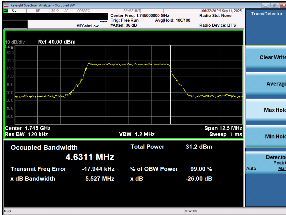
Plot 7-75. Occupied Bandwidth Plot (LTE Band 66/4 - 5MHz QPSK - Full RB - ANT2)
