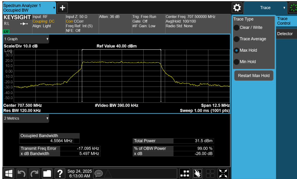
Plot 7-32. Occupied Bandwidth Plot (NR Band n12 - 5MHz DFT-s-OFDM BPSK - Full RB – ANT1)
