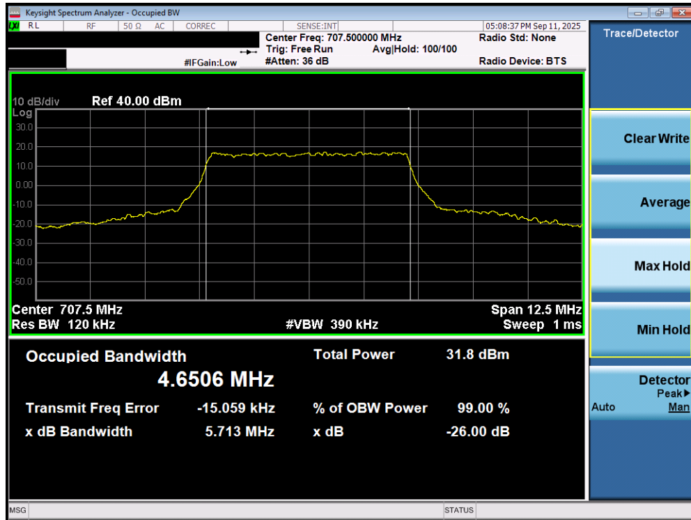
Plot 7-59. Occupied Bandwidth Plot (LTE Band 12/17 - 5MHz QPSK - Full RB - ANT2)
