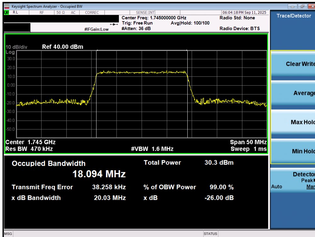
Plot 7-70. Occupied Bandwidth Plot (LTE Band 66/4 - 20MHz 16-QAM - Full RB - ANT2)
