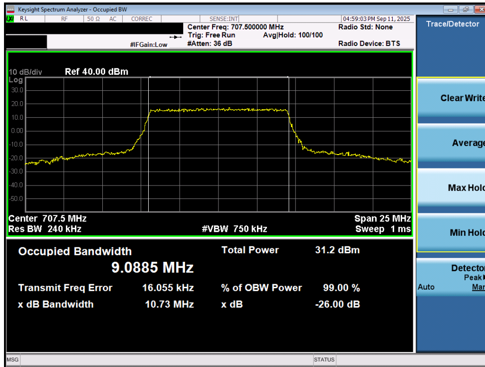
Plot 7-57. Occupied Bandwidth Plot (LTE Band 12/17 - 10MHz QPSK - Full RB – ANT2)
