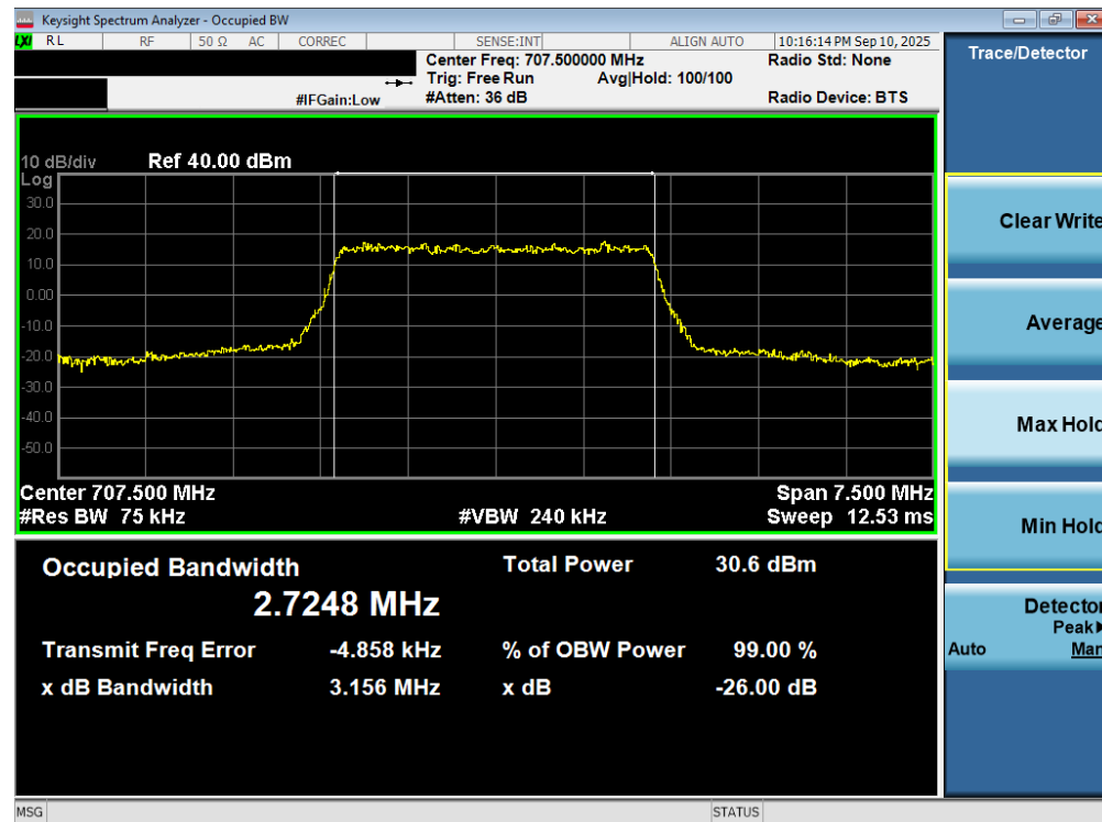
Plot 7-7. Occupied Bandwidth Plot (LTE Band 12 - 3MHz 16-QAM - Full RB – ANT1)
