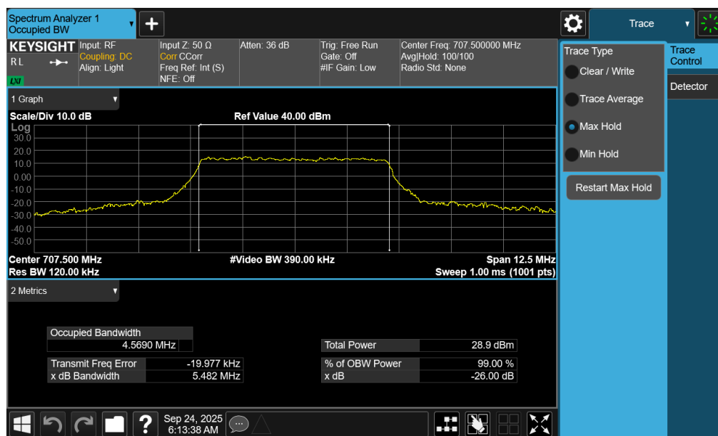
Plot 7-34. Occupied Bandwidth Plot (NR Band n12 - 5MHz CP-OFDM 16-QAM - Full RB – ANT1)
