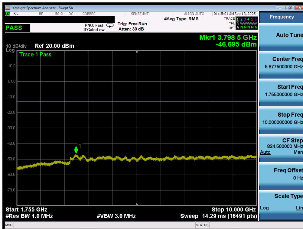
Plot 7-130. Conducted Spurious Plot (WCDMA-AWS - 5MHz QPSK - 1 RB – Low Channel)
