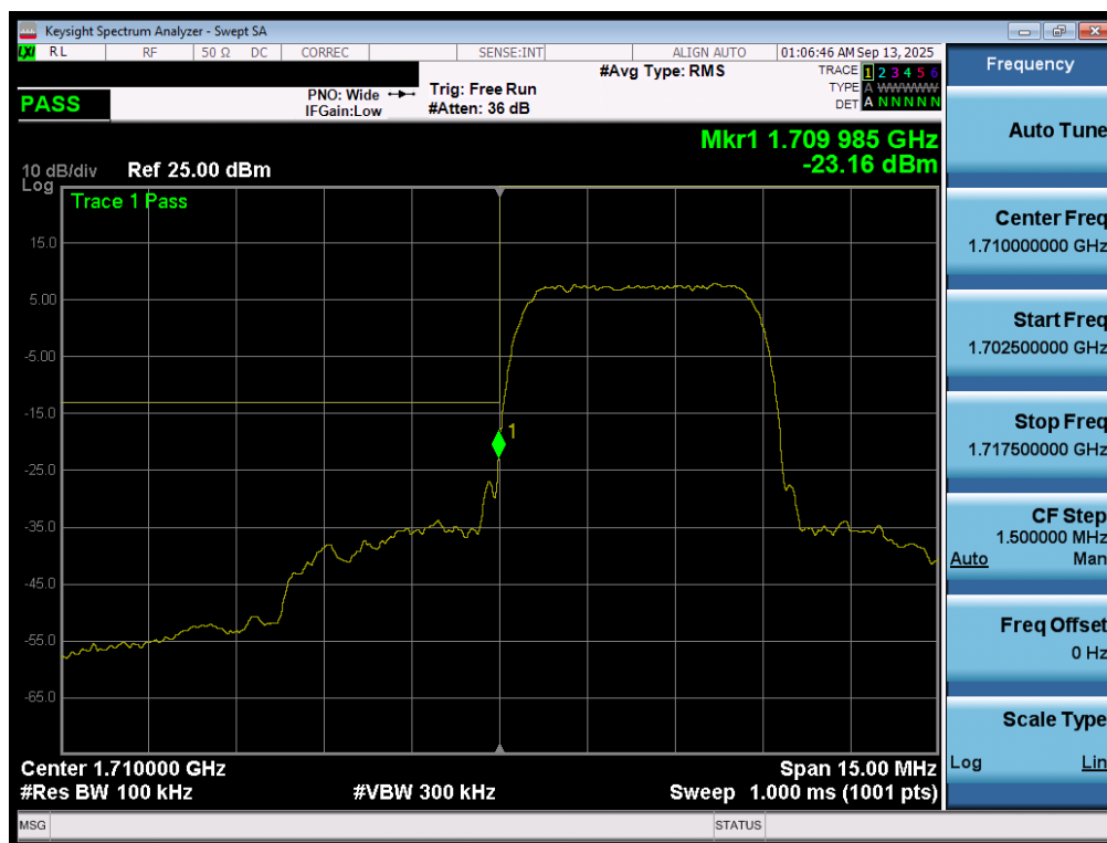
Plot 7-169. Lower Band Edge Plot (WCDMA AWS – Ch. 1312 – ANT2)
