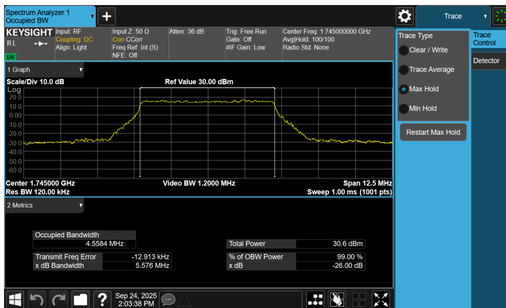
Plot 7-109. Occupied Bandwidth Plot (NR Band n66 - 5.0MHz CP-OFDM QPSK - Full RB – ANT2)
