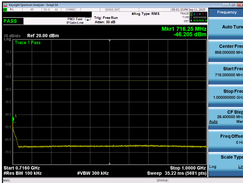
Plot 7-133. Conducted Spurious Plot (LTE Band 12/17 - 10MHz QPSK - 1 RB - Low Channel - ANT2)
