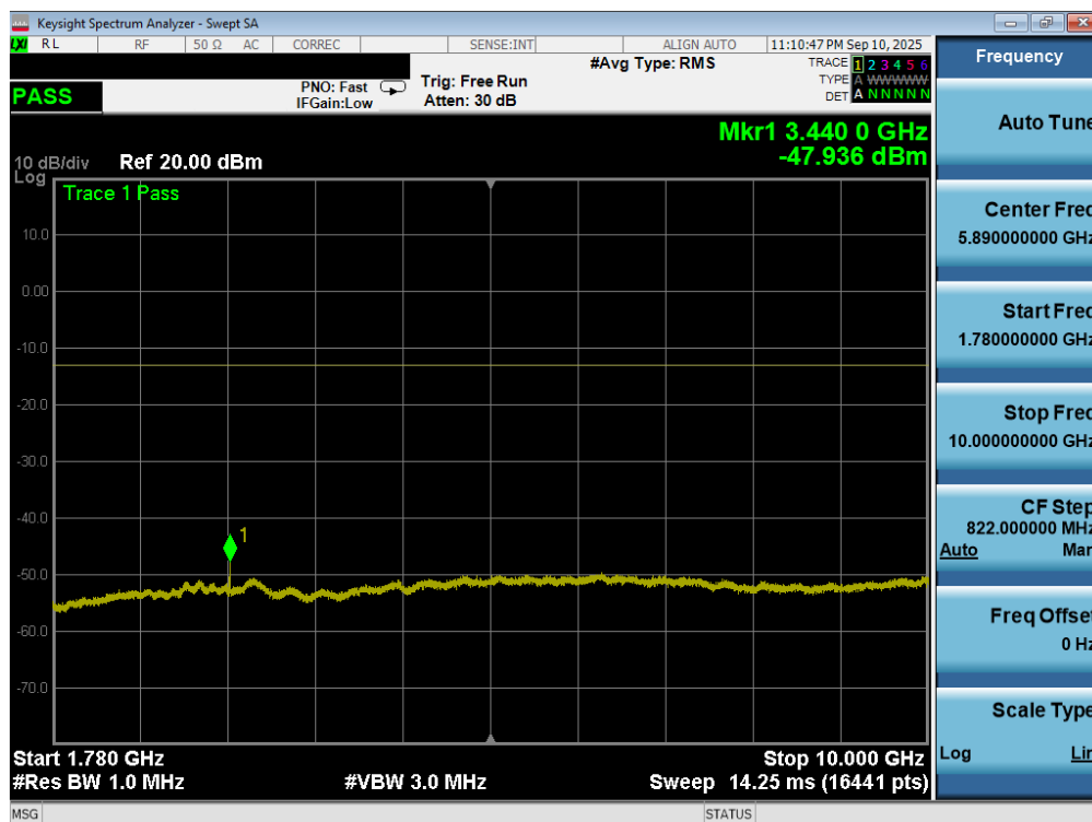
Plot 7-124. Conducted Spurious Plot (LTE Band 66/4 - 20MHz QPSK - 1 RB – Low Channel)
