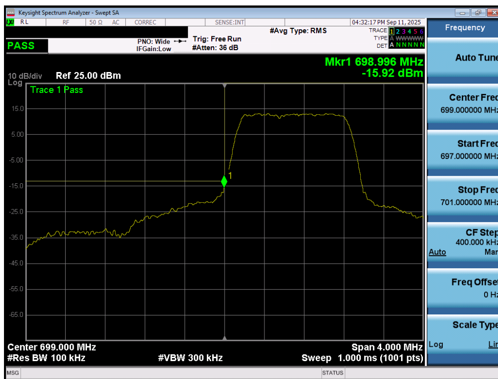
Plot 7-151. Lower Band Edge Plot (LTE Band 12/17 – 1.4MHz QPSK – Full RB - ANT1)
