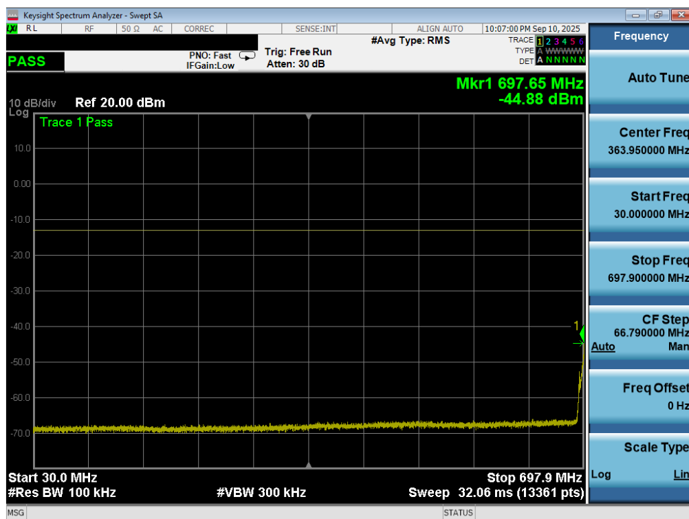
Plot 7-114. Conducted Spurious Plot (LTE Band 12/17 - 10MHz QPSK - 1 RB - Low Channel - ANT1)
