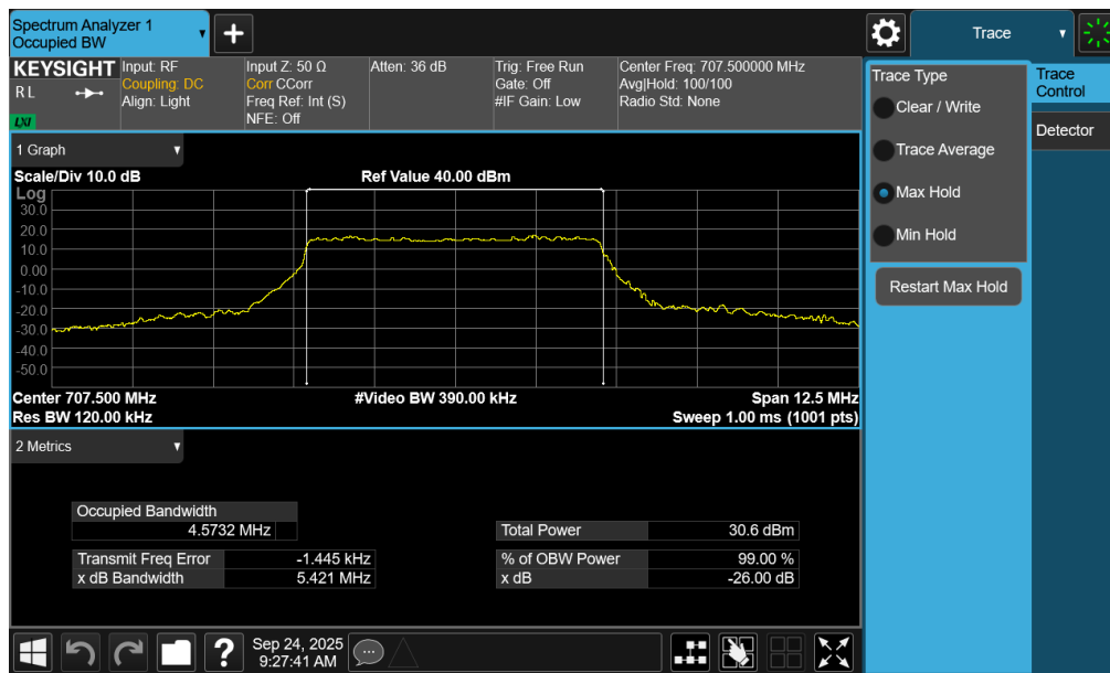
Plot 7-88. Occupied Bandwidth Plot (NR Band n12 - 5MHz CP-OFDM QPSK - Full RB – ANT2)
