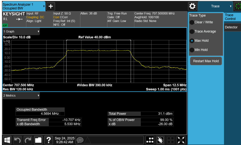
Plot 7-87. Occupied Bandwidth Plot (NR Band n12 - 5MHz DFT-s-OFDM BPSK - Full RB – ANT2)
