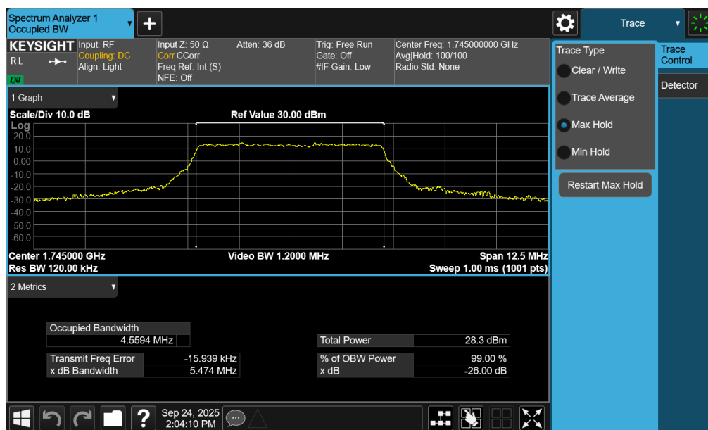
Plot 7-110. Occupied Bandwidth Plot (NR Band n66 - 5.0MHz CP-OFDM 16QAM - Full RB – ANT2)
