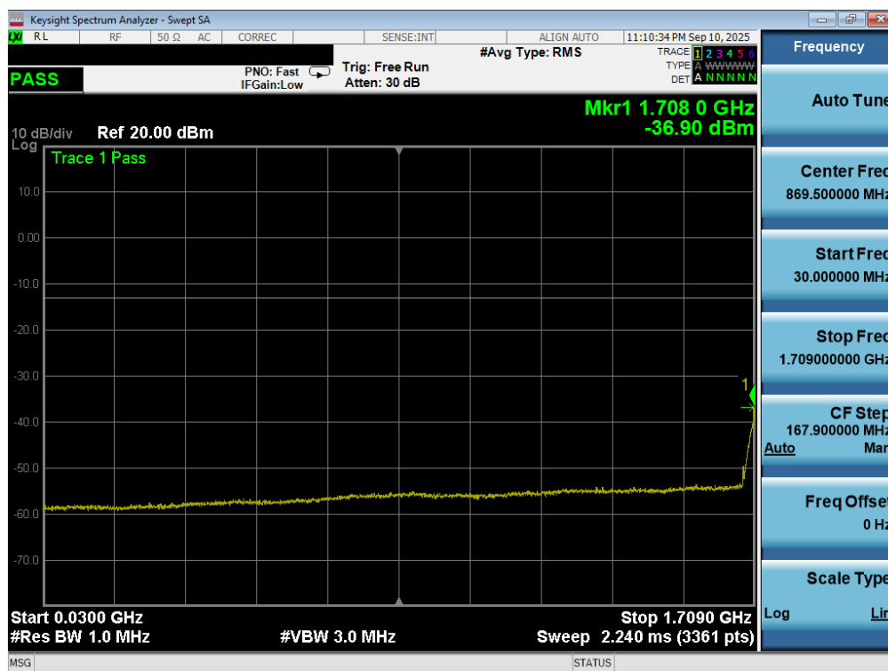
Plot 7-123. Conducted Spurious Plot (LTE Band 66/4 - 20MHz QPSK - 1 RB – Low Channel)
