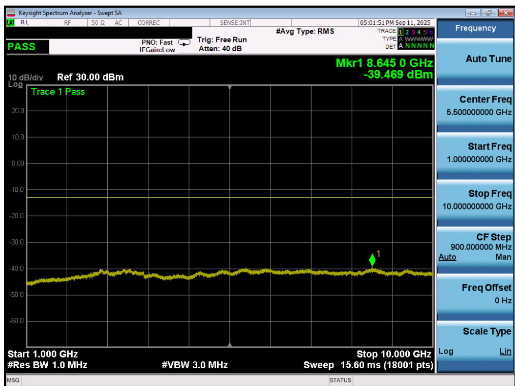
Plot 7-134. Conducted Spurious Plot (LTE Band 12/17 - 10MHz QPSK - 1 RB - Low Channel - ANT2)
