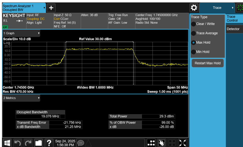
Plot 7-101. Occupied Bandwidth Plot (NR Band n66 - 20.0MHz CP-OFDM 16QAM - Full RB – ANT2)
