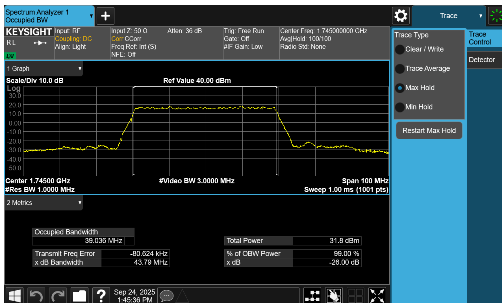
Plot 7-90. Occupied Bandwidth Plot (NR Band n66 - 40.0MHz DFT-s-OFDM BPSK - Full RB – ANT2)
