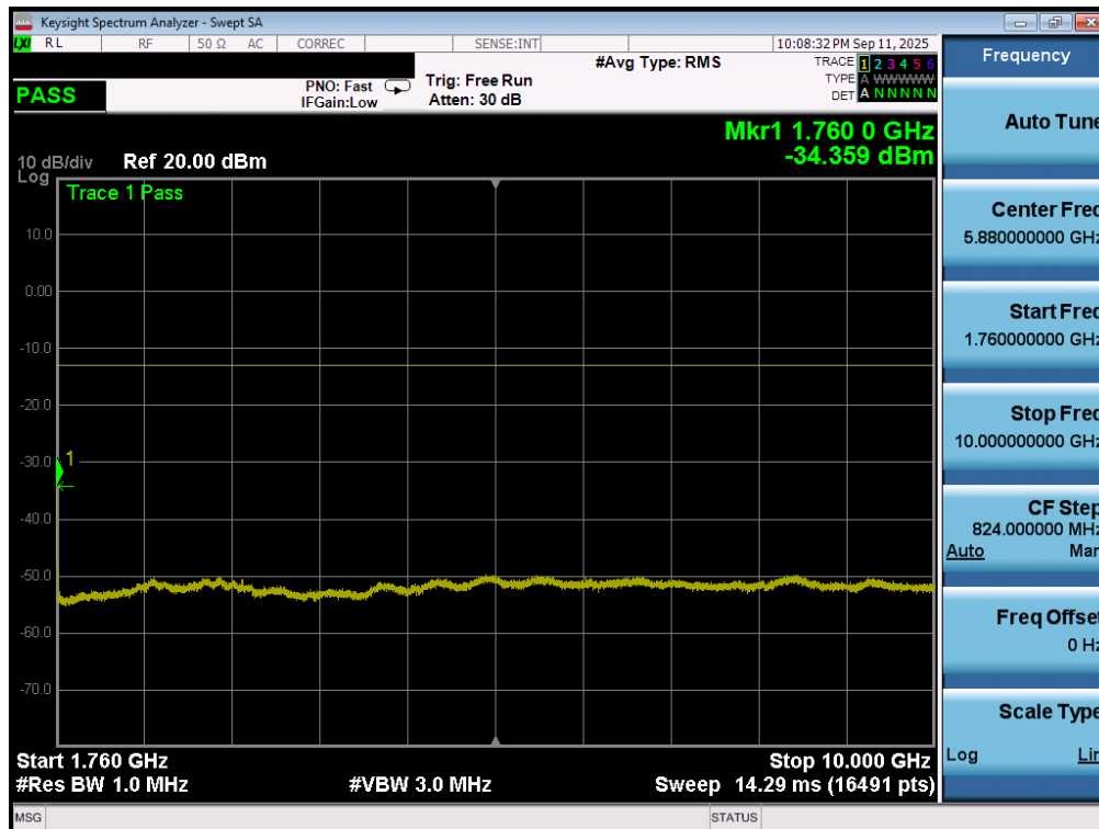
Plot 7-112. Conducted Spurious Plot (WCDMA-AWS - 5MHz QPSK - 1 RB – High Channel)
