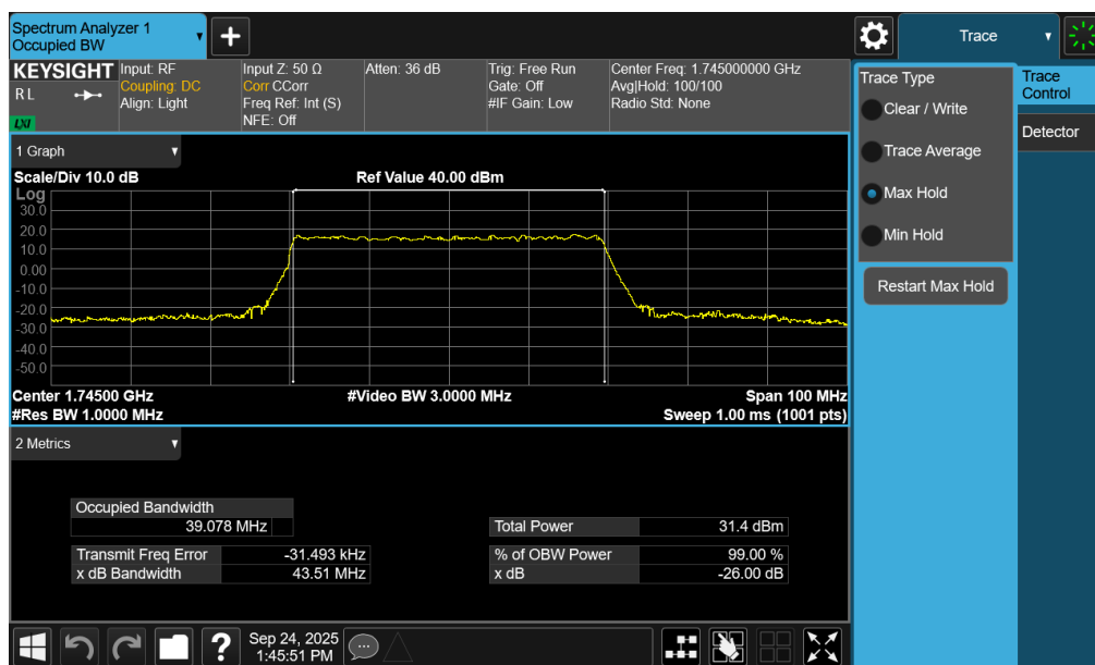
Plot 7-91. Occupied Bandwidth Plot (NR Band n66 - 40.0MHz CP-OFDM QPSK - Full RB – ANT2)
