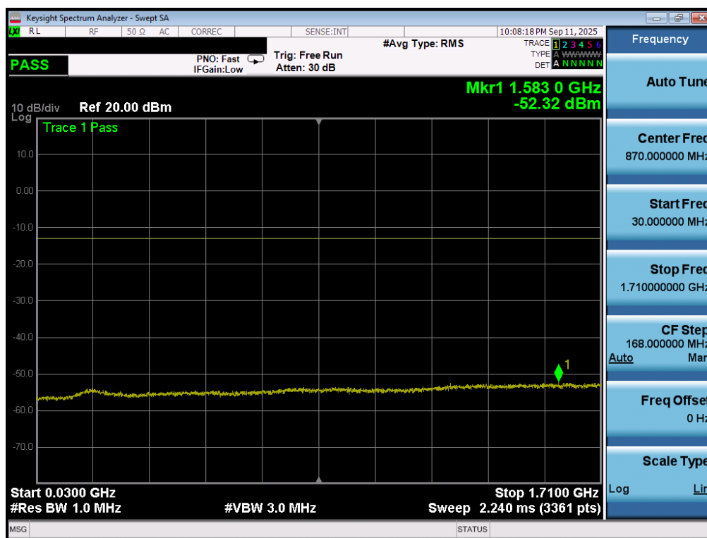
Plot 7-111. Conducted Spurious Plot (WCDMA-AWS - 5MHz QPSK - 1 RB – High Channel)
