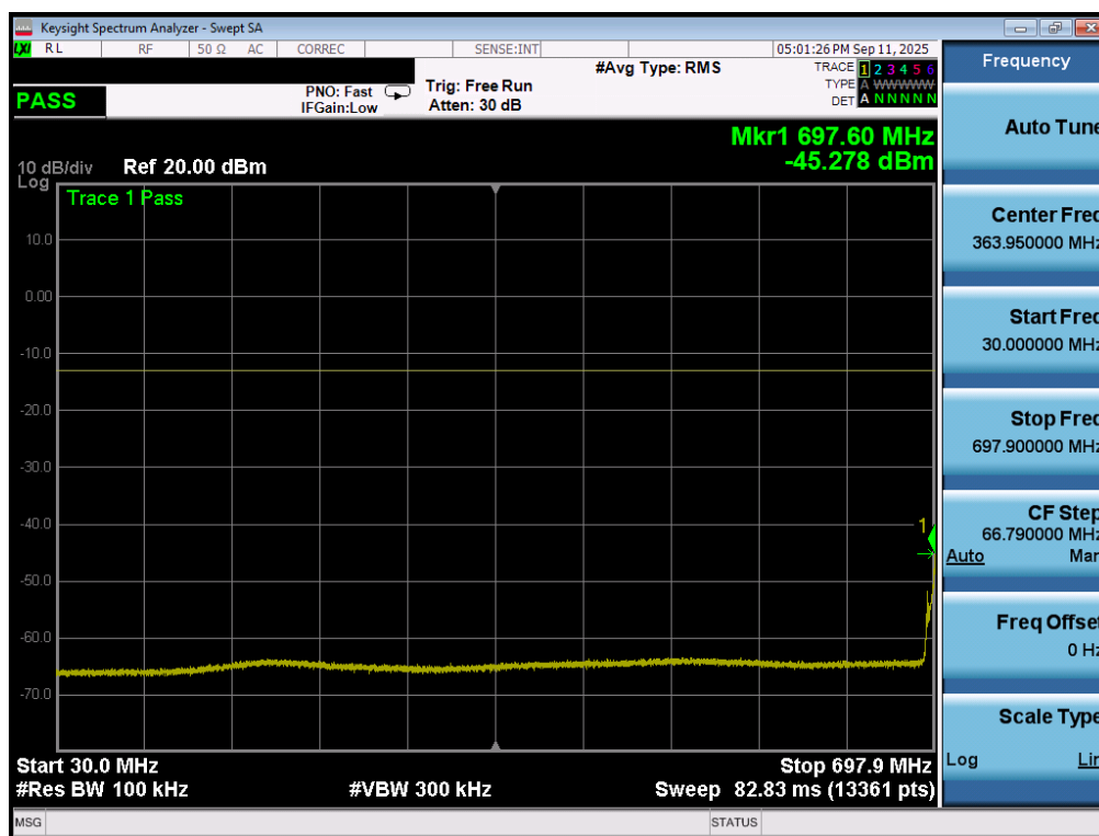
Plot 7-132. Conducted Spurious Plot (LTE Band 12/17 - 10MHz QPSK - 1 RB - Low Channel - ANT2)
