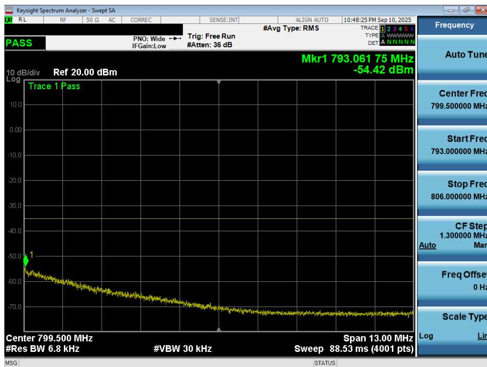
Plot 7-156. Upper Emission Mask Plot (LTE Band 13 - 5MHz QPSK – Full RB - ANT1)
