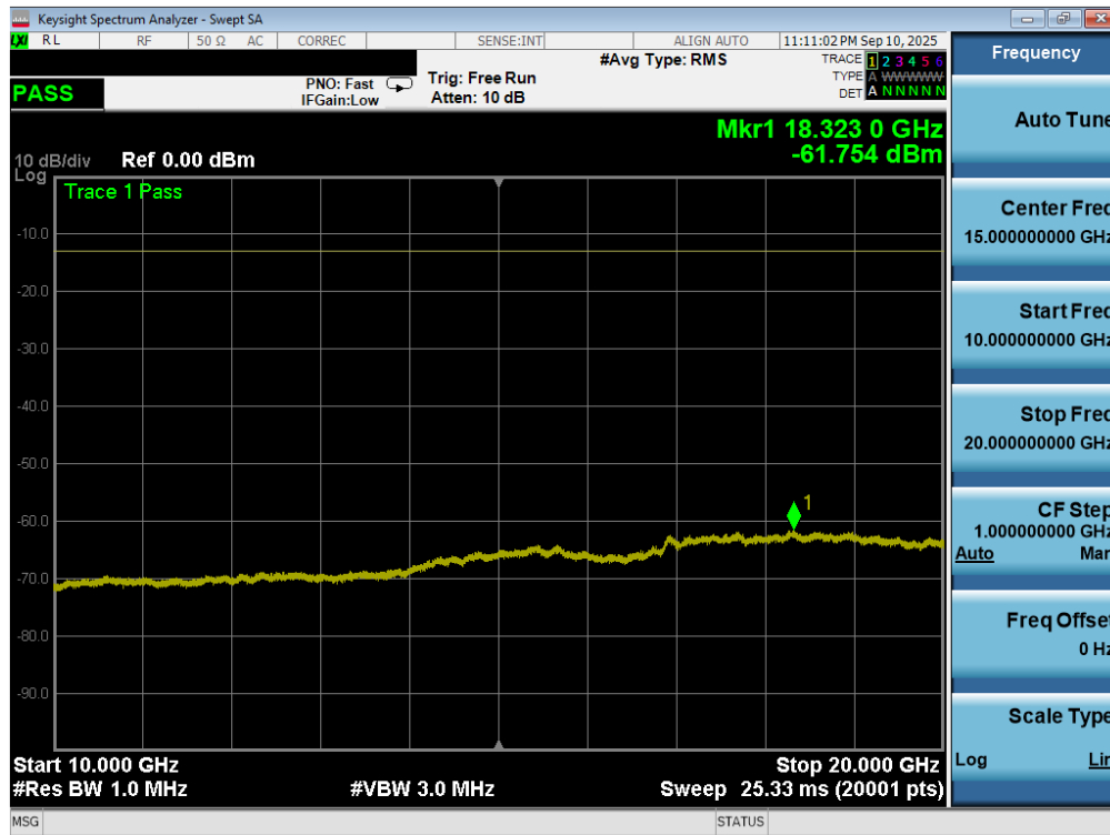
Plot 7-125. Conducted Spurious Plot (LTE Band 66/4 - 20MHz QPSK - 1 RB – Low Channel)
