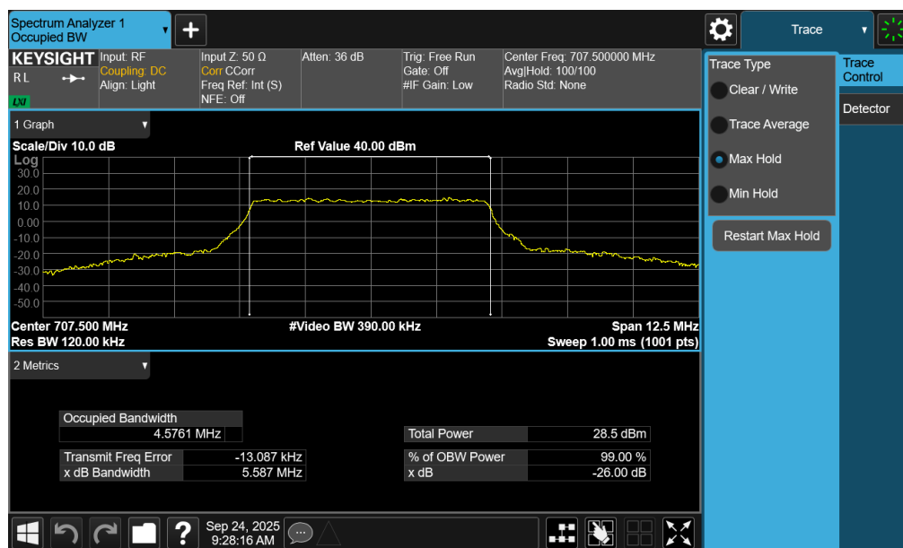
Plot 7-89. Occupied Bandwidth Plot (NR Band n12 - 5MHz CP-OFDM 16-QAM - Full RB – ANT2)
