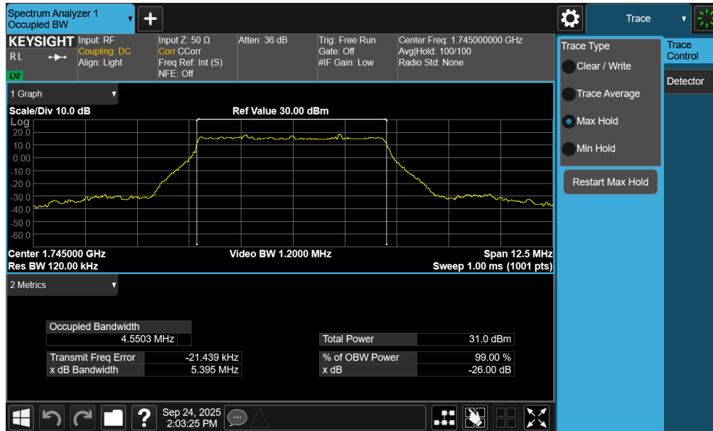
Plot 7-108. Occupied Bandwidth Plot (NR Band n66 - 5.0MHz DFT-s-OFDM BPSK - Full RB – ANT2)
