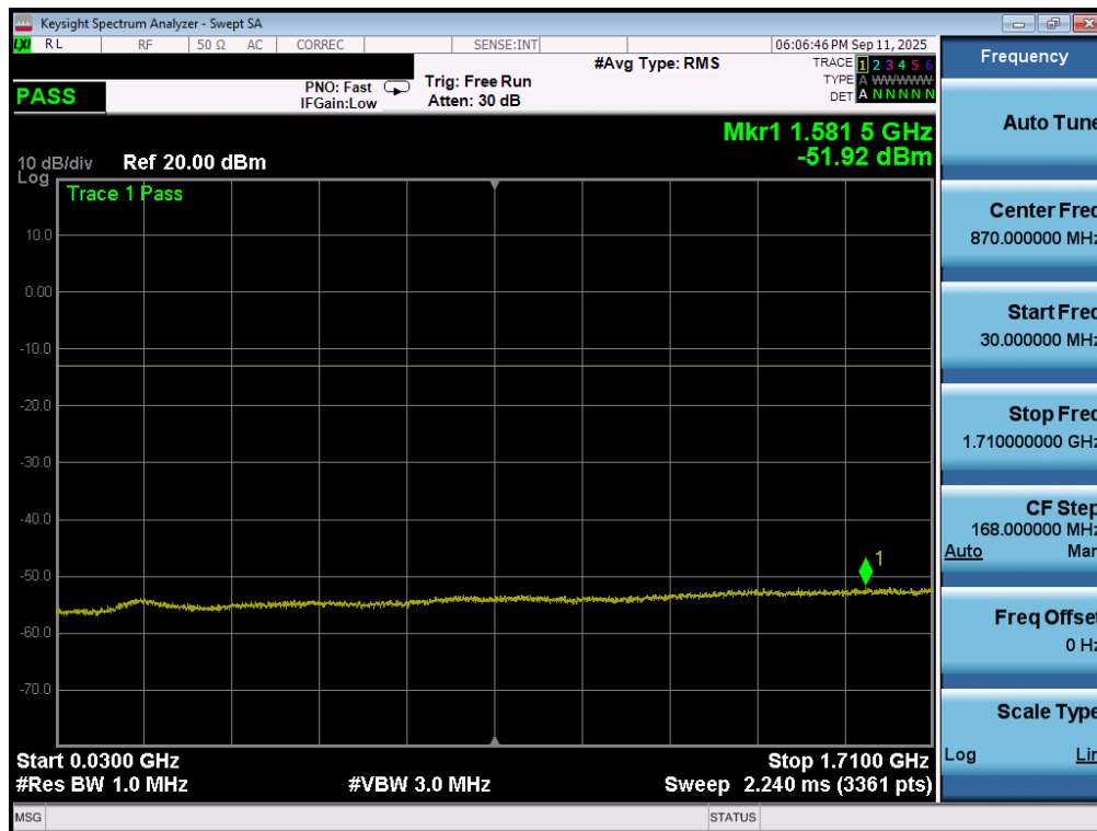
Plot 7-141. Conducted Spurious Plot (LTE Band 66/4 - 20MHz QPSK - 1 RB – High Channel)
