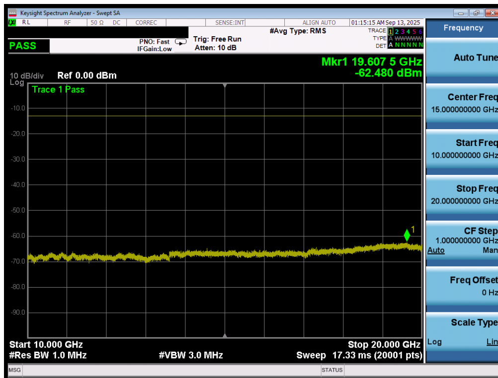
Plot 7-131. Conducted Spurious Plot (WCDMA-AWS - 5MHz QPSK - 1 RB – Low Channel)
