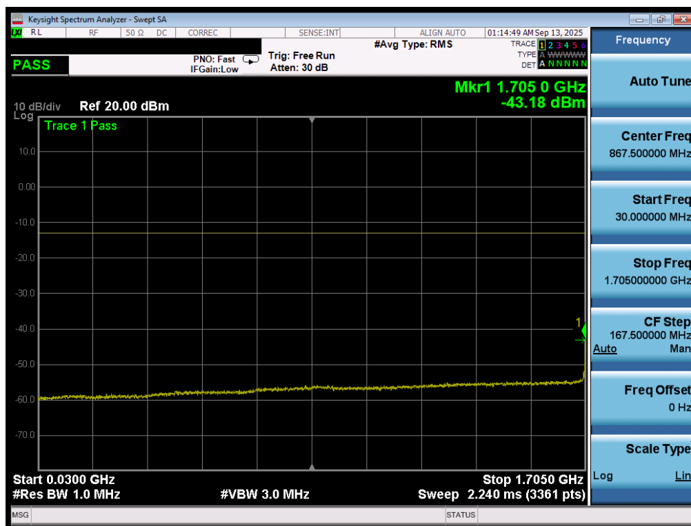
Plot 7-129. Conducted Spurious Plot (WCDMA-AWS - 5MHz QPSK - 1 RB – Low Channel)
