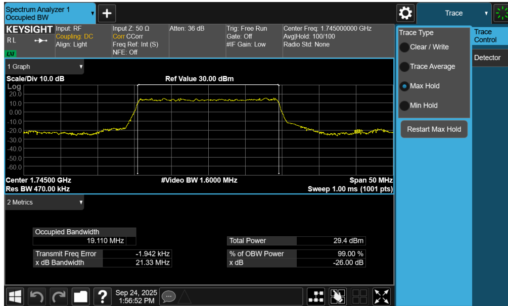
Plot 7-100. Occupied Bandwidth Plot (NR Band n66 - 20.0MHz CP-OFDM QPSK - Full RB – ANT2)
