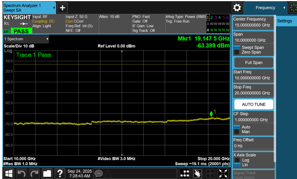
Plot 7-128. Conducted Spurious Plot (NR Band n66 - 40MHz - 1 RB - High Channel - ANT1)
