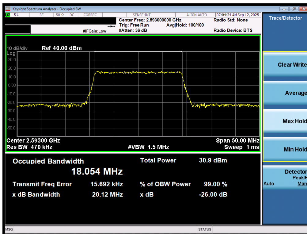
Plot 7-9. Occupied Bandwidth Plot (LTE Band 41(PC3) - 20MHz QPSK - Full RB - Ant1)
