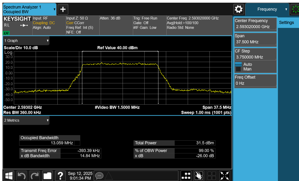
Plot 7-60. Occupied Bandwidth Plot (NR Band n41 PC3 – 15MHz \pi/2 BPSK – Full RB – Ant1)
