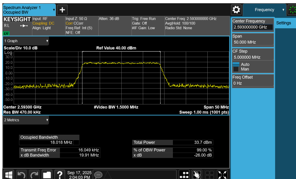
Plot 7-17. Occupied Bandwidth Plot (LTE Band 41(PC2) - 20MHz QPSK - Full RB - Ant2)
