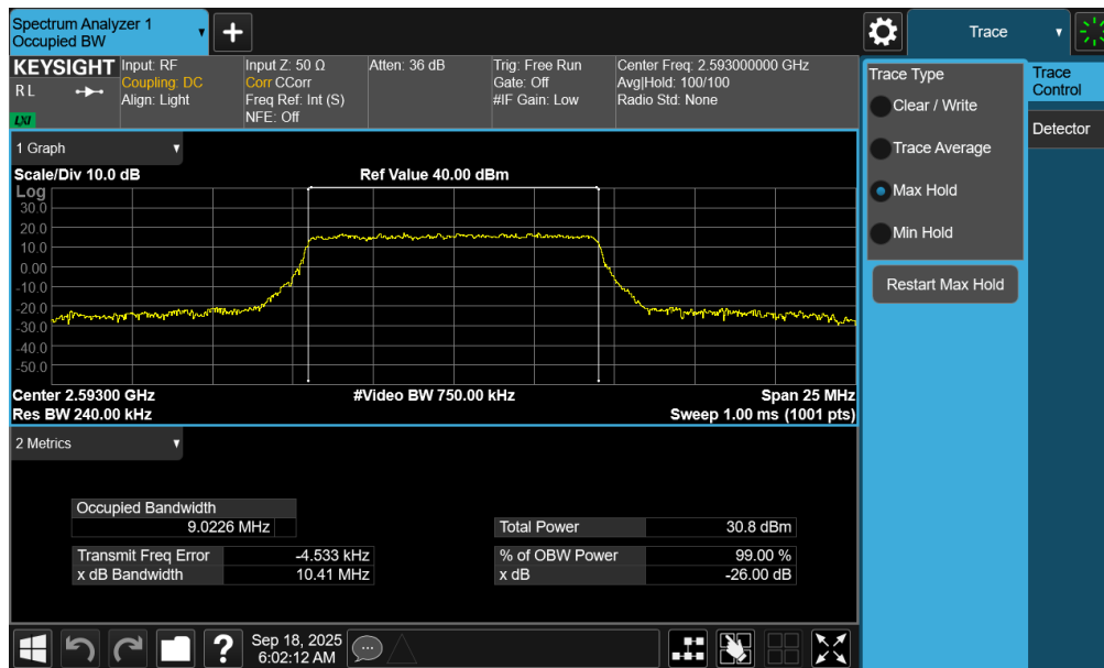
Plot 7-29. Occupied Bandwidth Plot (LTE Band 41(PC3) - 10MHz QPSK - Full RB - Ant2)
