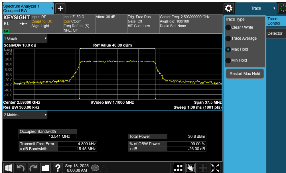
Plot 7-27. Occupied Bandwidth Plot (LTE Band 41(PC3) - 15MHz QPSK - Full RB - Ant2)
