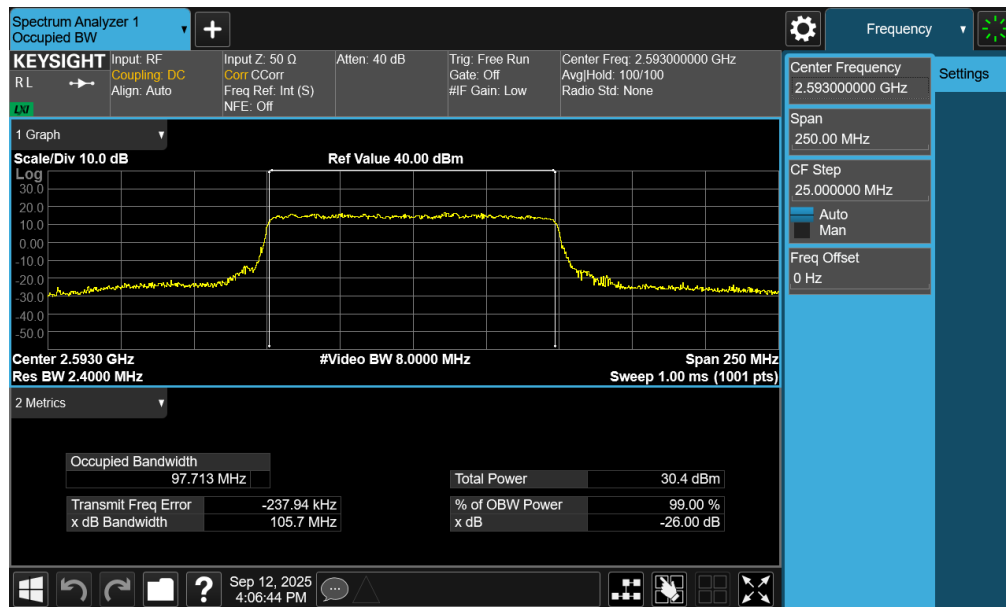
Plot 7-35. Occupied Bandwidth Plot (NR Band n41 PC3 – 100MHz 16-QAM – Full RB – Ant1)
