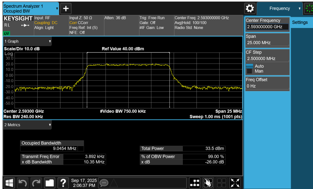
Plot 7-21. Occupied Bandwidth Plot (LTE Band 41(PC2) - 10MHz QPSK - Full RB - Ant2)
