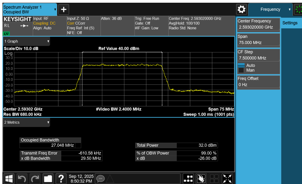
Plot 7-54. Occupied Bandwidth Plot (NR Band n41 PC3 – 30MHz \pi/2 BPSK – Full RB – Ant1)
