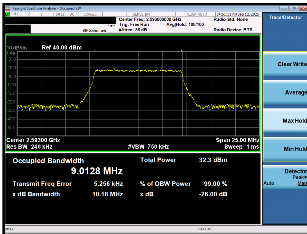
Plot 7-6. Occupied Bandwidth Plot (LTE Band 41(PC2) - 10MHz 16-QAM - Full RB - Ant1)
