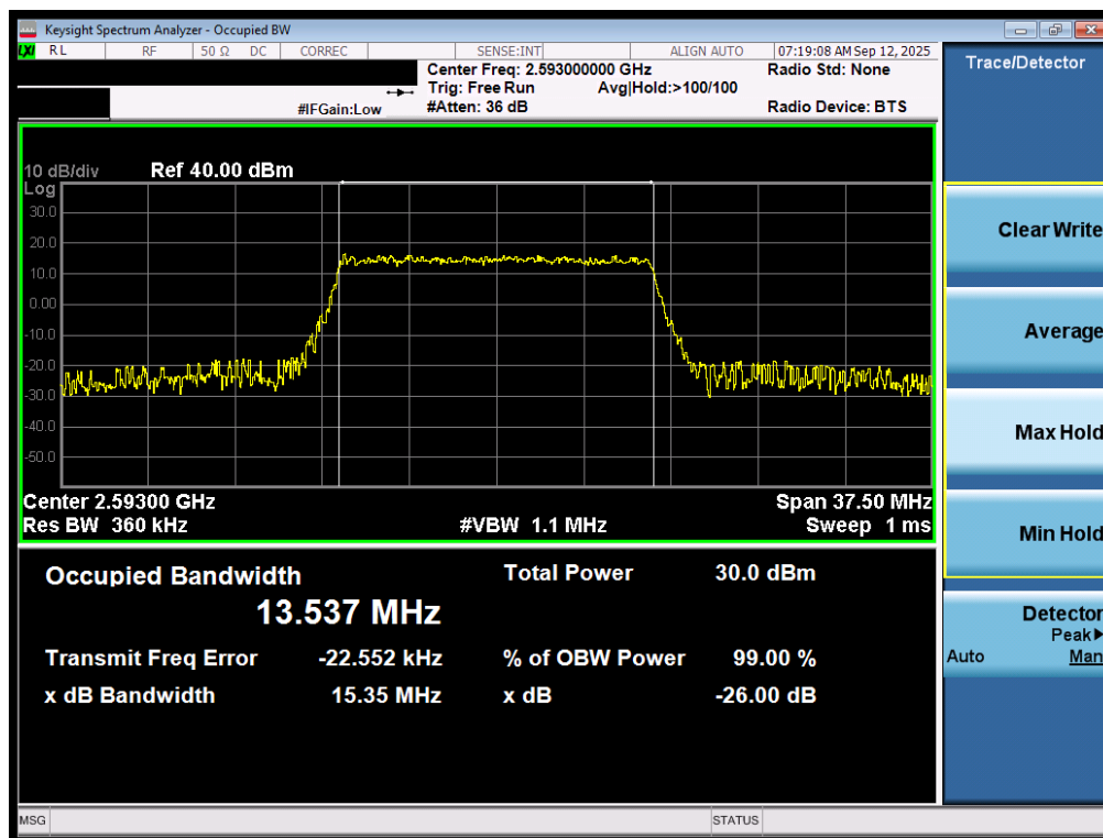
Plot 7-12. Occupied Bandwidth Plot (LTE Band 41(PC3) - 15MHz 16-QAM - Full RB - Ant1)
