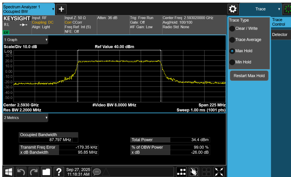
Plot 7-71. Occupied Bandwidth Plot (NR Band n41 PC3 – 90MHz 16-QAM – Full RB – Ant2)
