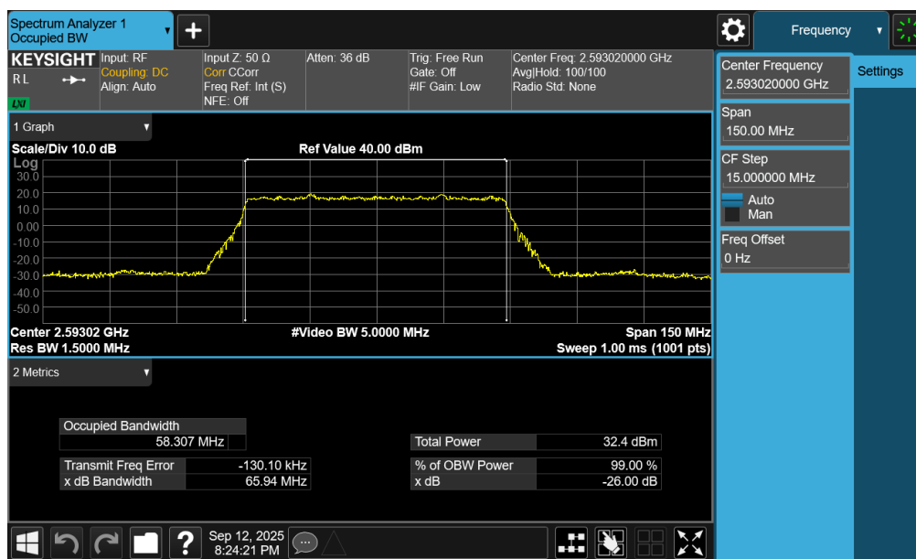
Plot 7-45. Occupied Bandwidth Plot (NR Band n41 PC3 – 60MHz \pi/2 BPSK – Full RB – Ant1)
