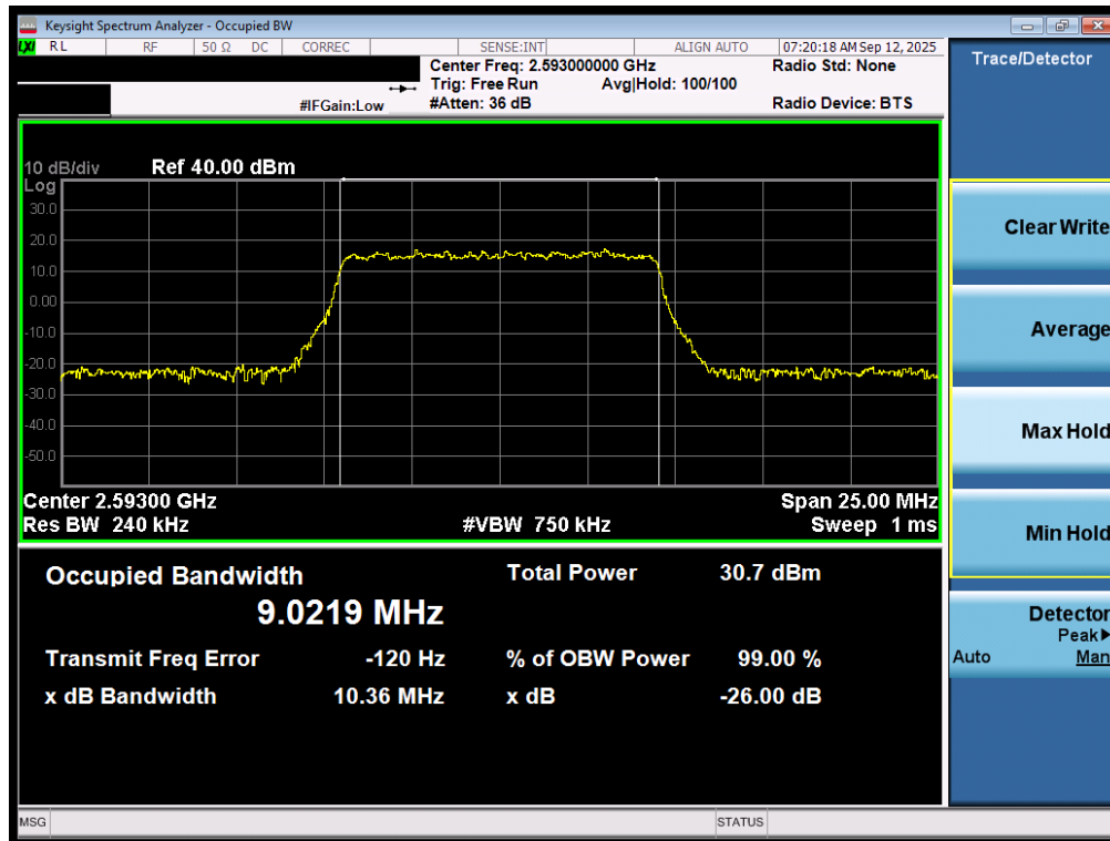
Plot 7-13. Occupied Bandwidth Plot (LTE Band 41(PC3) - 10MHz QPSK - Full RB - Ant1)
