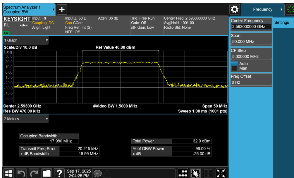
Plot 7-18. Occupied Bandwidth Plot (LTE Band 41(PC2) - 20MHz 16-QAM - Full RB - Ant2)
