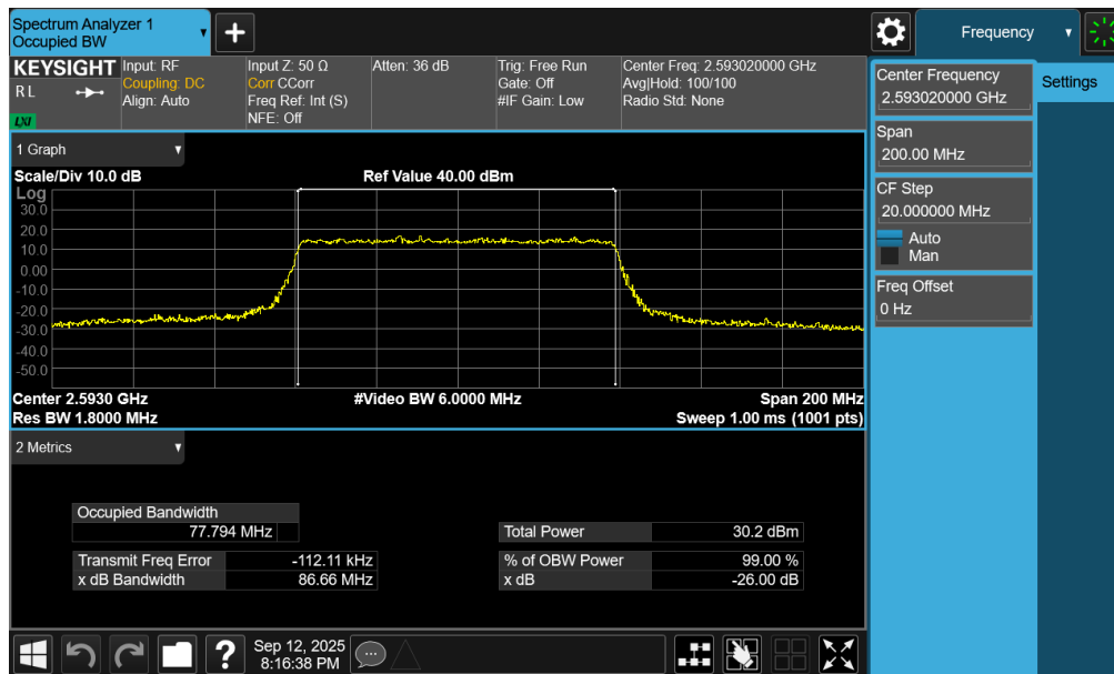
Plot 7-41. Occupied Bandwidth Plot (NR Band n41 PC3 – 80MHz 16-QAM – Full RB – Ant1)
