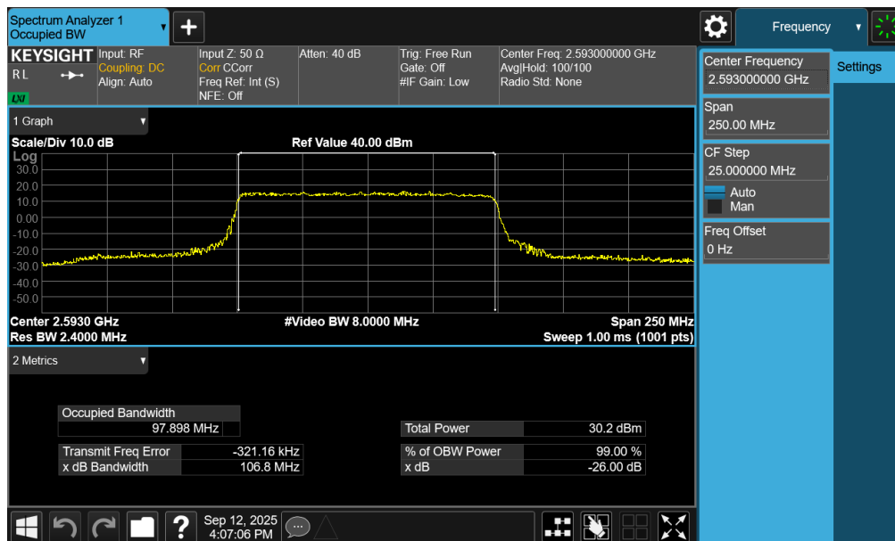
Plot 7-34. Occupied Bandwidth Plot (NR Band n41 PC3 – 100MHz QPSK – Full RB – Ant1)
