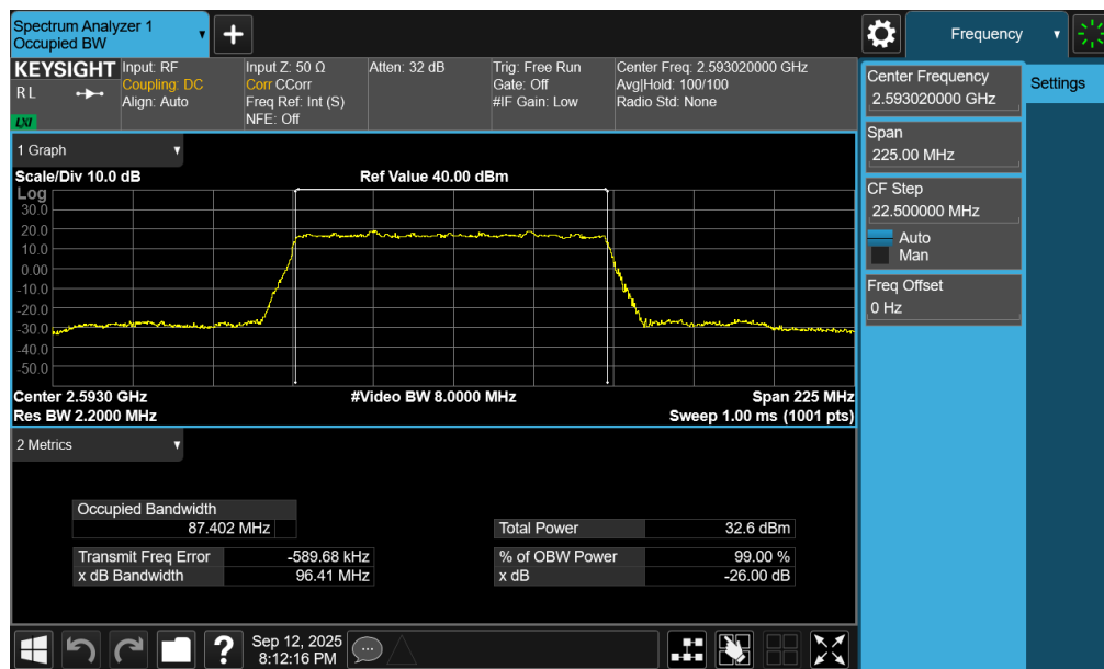
Plot 7-36. Occupied Bandwidth Plot (NR Band n41 PC3 – 90MHz \pi/2 BPSK – Full RB – Ant1)
