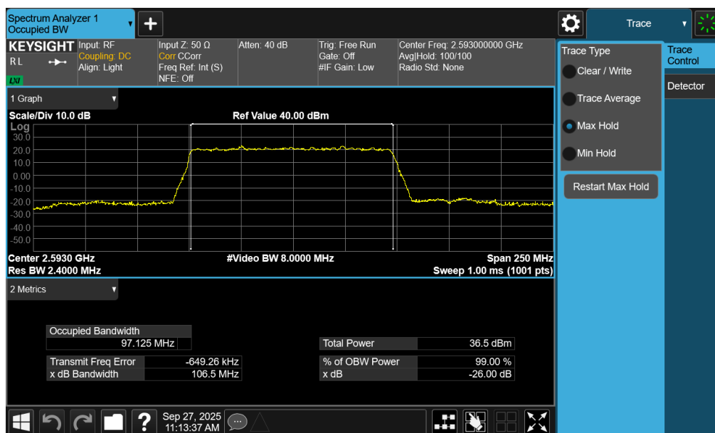
Plot 7-66. Occupied Bandwidth Plot (NR Band n41 PC3 – 100MHz \pi/2 BPSK – Full RB – Ant2)
