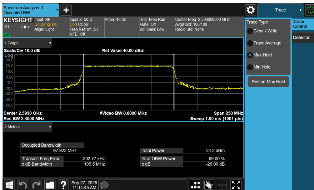
Plot 7-67. Occupied Bandwidth Plot (NR Band n41 PC3 – 100MHz QPSK – Full RB – Ant2)
