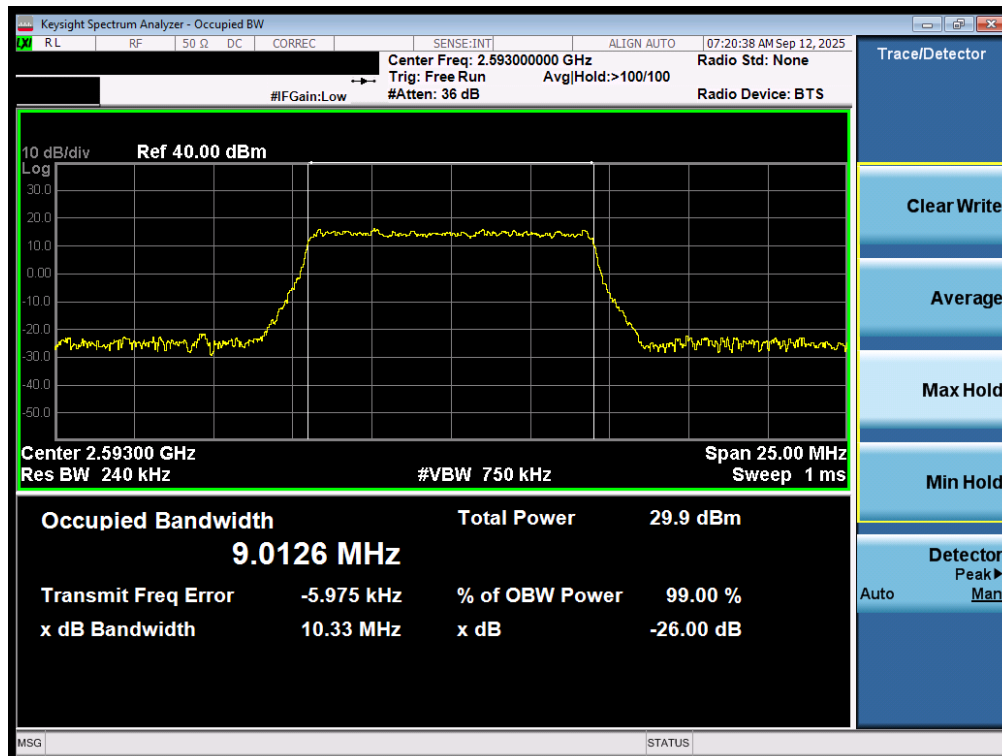
Plot 7-14. Occupied Bandwidth Plot (LTE Band 41(PC3) - 10MHz 16-QAM - Full RB - Ant1)
