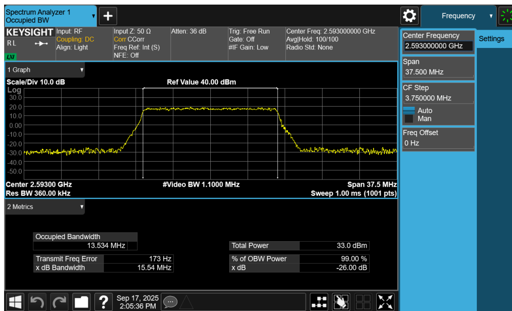
Plot 7-20. Occupied Bandwidth Plot (LTE Band 41(PC2) - 15MHz 16-QAM - Full RB - Ant2)
