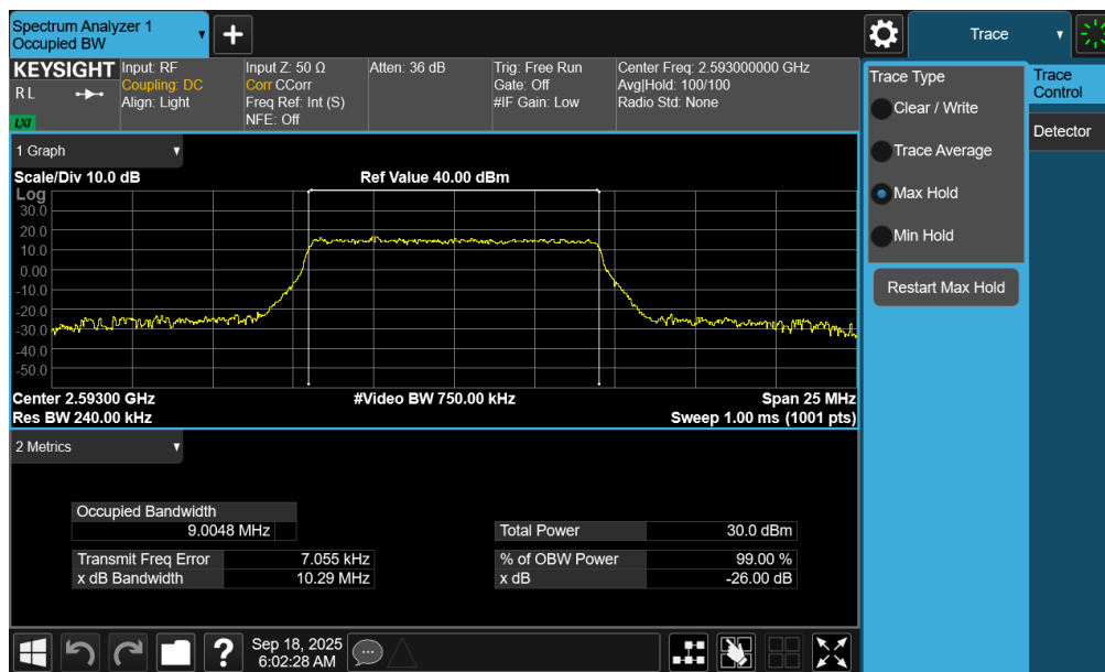
Plot 7-30. Occupied Bandwidth Plot (LTE Band 41(PC3) - 10MHz 16-QAM - Full RB - Ant2)
