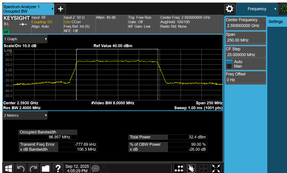
Plot 7-33. Occupied Bandwidth Plot (NR Band n41 PC3 – 100MHz \pi/2 BPSK – Full RB – Ant1)
