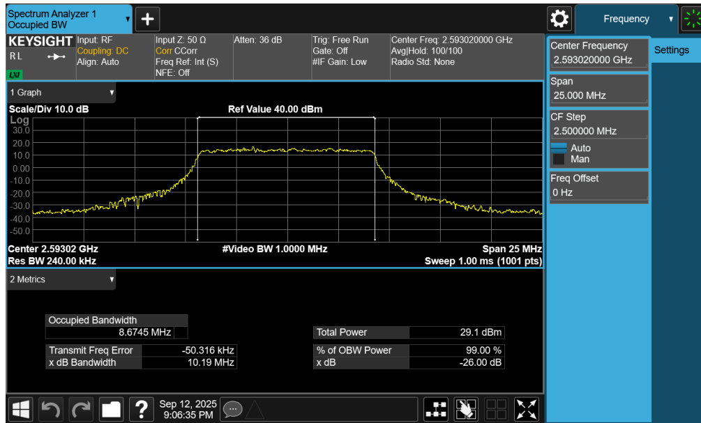
Plot 7-65. Occupied Bandwidth Plot (NR Band n41 PC3 – 10MHz 16-QAM – Full RB – Ant1)
