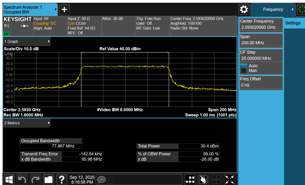
Plot 7-40. Occupied Bandwidth Plot (NR Band n41 PC3 – 80MHz QPSK – Full RB – Ant1)
