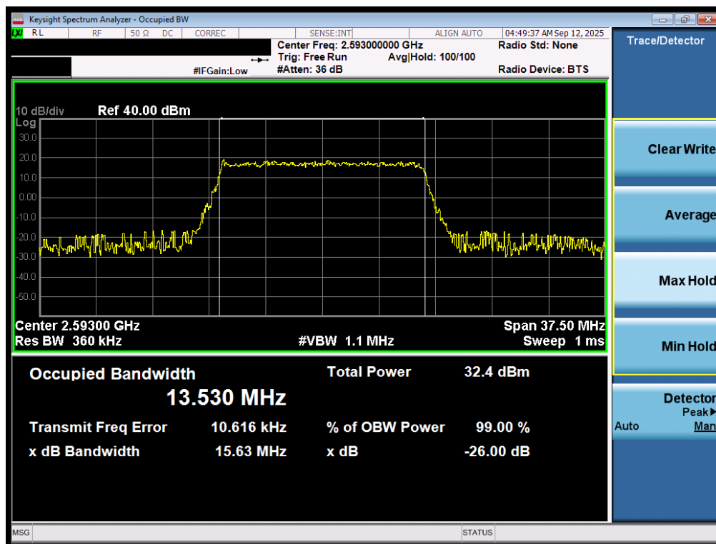
Plot 7-4. Occupied Bandwidth Plot (LTE Band 41(PC2) - 15MHz 16-QAM - Full RB - Ant1)
