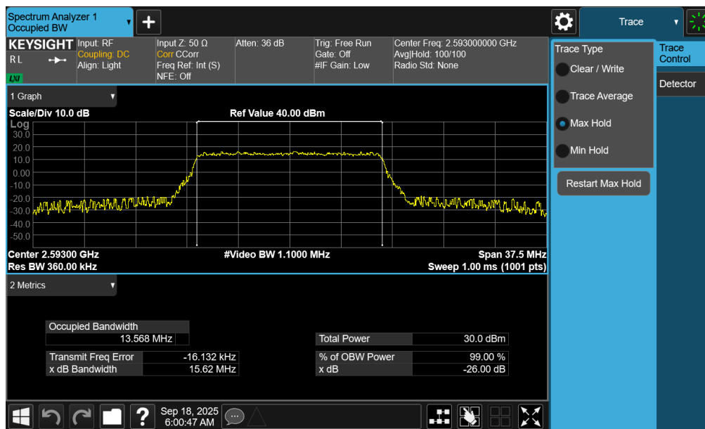
Plot 7-28. Occupied Bandwidth Plot (LTE Band 41(PC3) - 15MHz 16-QAM - Full RB - Ant2)
