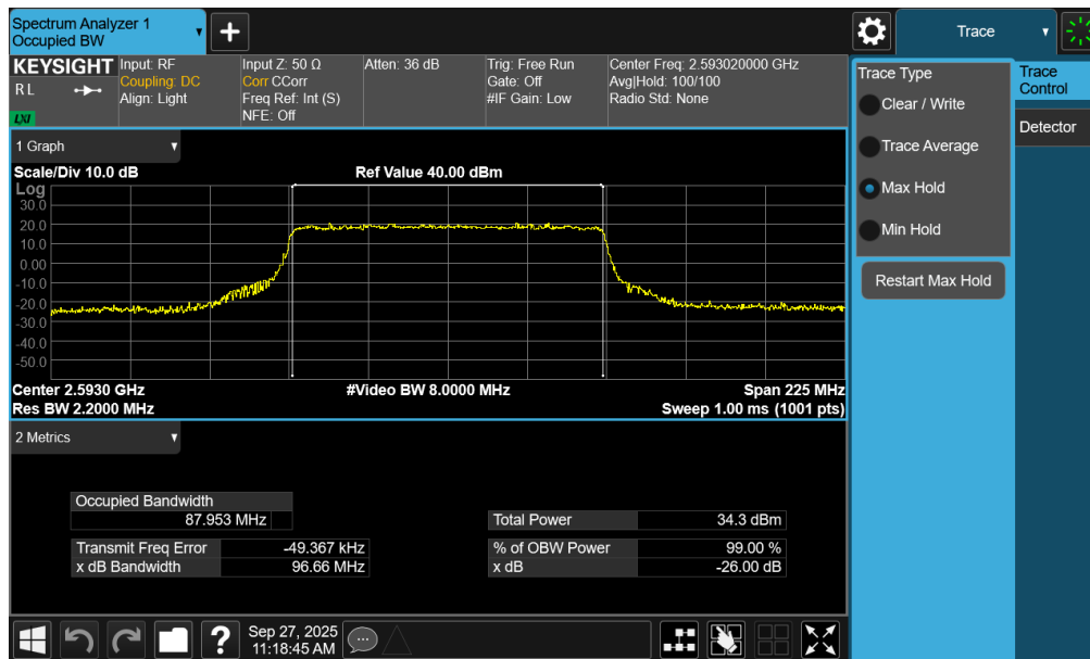
Plot 7-70. Occupied Bandwidth Plot (NR Band n41 PC3 – 90MHz QPSK – Full RB – Ant2)
