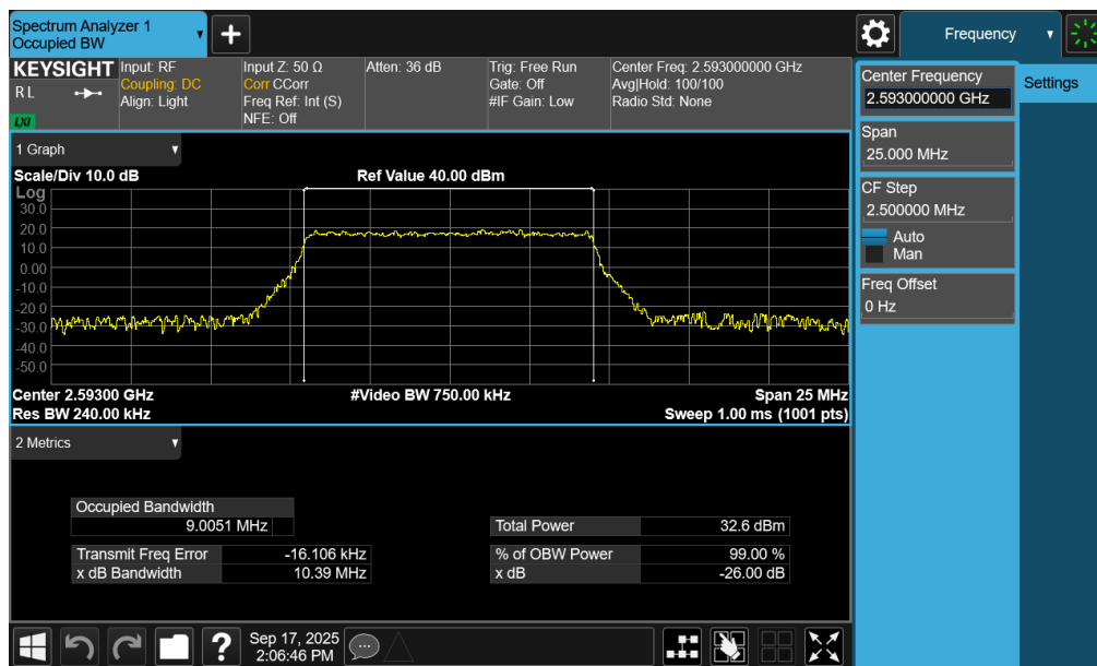
Plot 7-22. Occupied Bandwidth Plot (LTE Band 41(PC2) - 10MHz 16-QAM - Full RB - Ant2)
