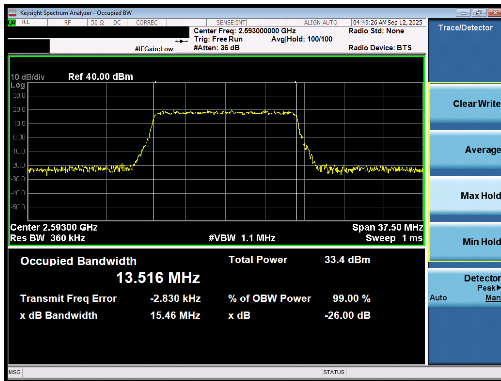
Plot 7-3. Occupied Bandwidth Plot (LTE Band 41(PC2) - 15MHz QPSK - Full RB - Ant1)
