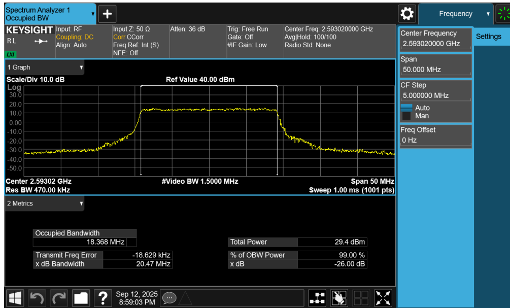
Plot 7-59. Occupied Bandwidth Plot (NR Band n41 PC3 – 20MHz 16-QAM – Full RB – Ant1)
