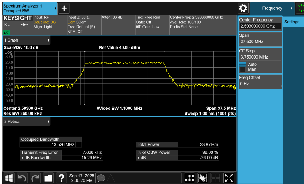
Plot 7-19. Occupied Bandwidth Plot (LTE Band 41(PC2) - 15MHz QPSK - Full RB - Ant2)
