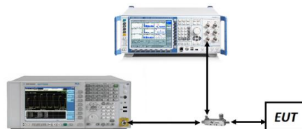
Figure 7-1. Test Instrument & Measurement Setup – Online Mode
