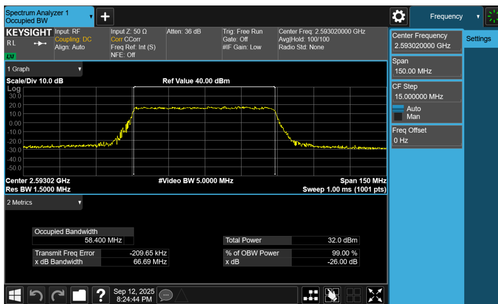
Plot 7-46. Occupied Bandwidth Plot (NR Band n41 PC3 – 60MHz QPSK – Full RB – Ant1)
