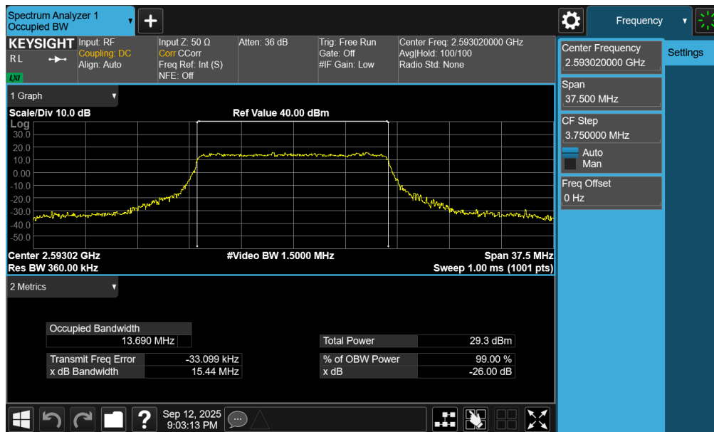
Plot 7-61. Occupied Bandwidth Plot (NR Band n41 PC3 – 15MHz QPSK – Full RB – Ant1)
