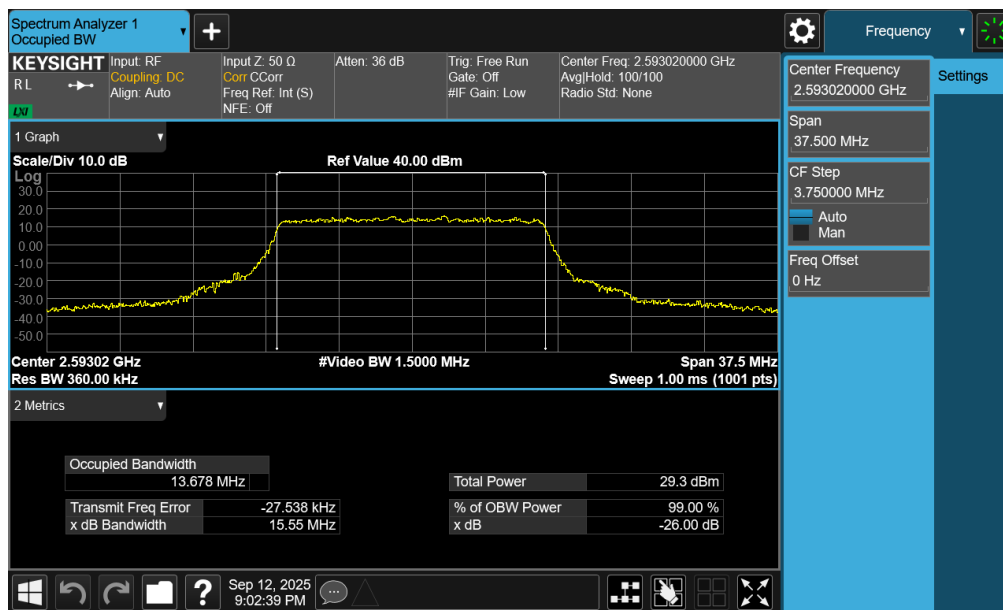
Plot 7-62. Occupied Bandwidth Plot (NR Band n41 PC3 – 15MHz 16-QAM – Full RB – Ant1)
