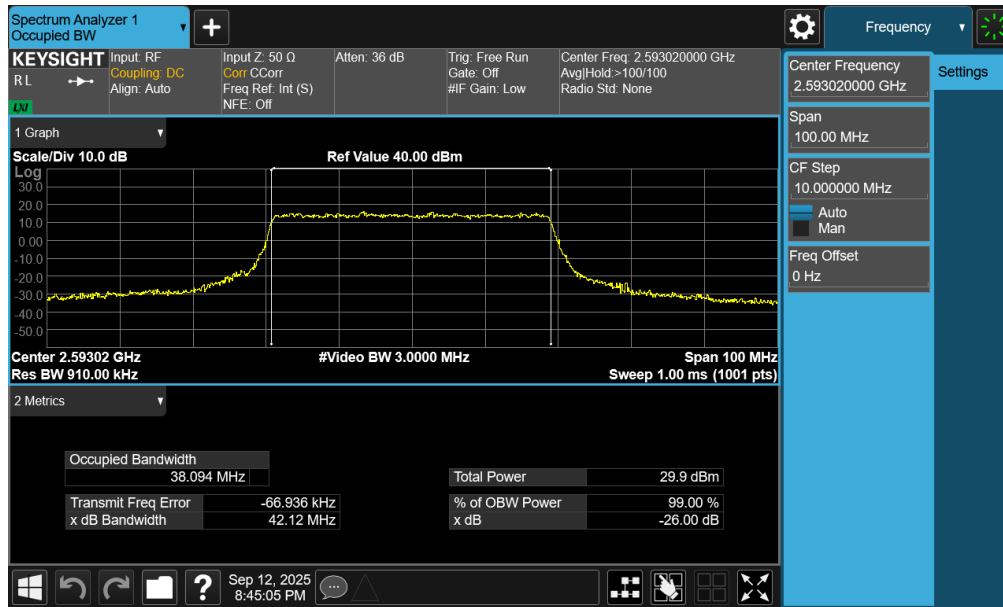
Plot 7-53. Occupied Bandwidth Plot (NR Band n41 PC3 – 40MHz 16-QAM – Full RB – Ant1)
