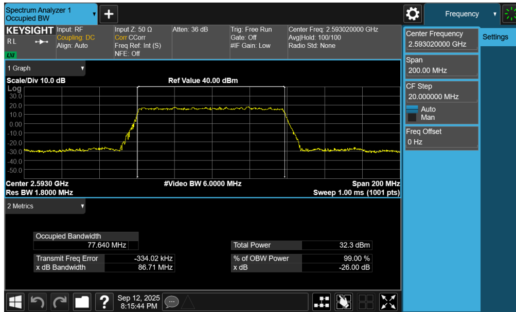
Plot 7-39. Occupied Bandwidth Plot (NR Band n41 PC3 – 80MHz \pi/2 BPSK – Full RB – Ant1)
