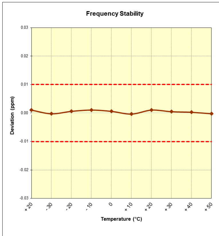
Figure 7-3. Frequency Stability Plot
