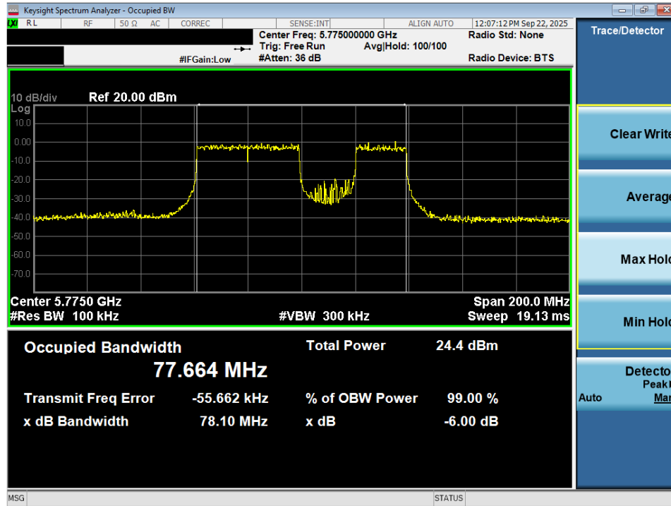
Plot 7-48. 6dB Bandwidth Plot MIMO ANT2 (80MHz BW 802.11be (20MHz Puncture) (UNII Band 3) – Ch. 155)
