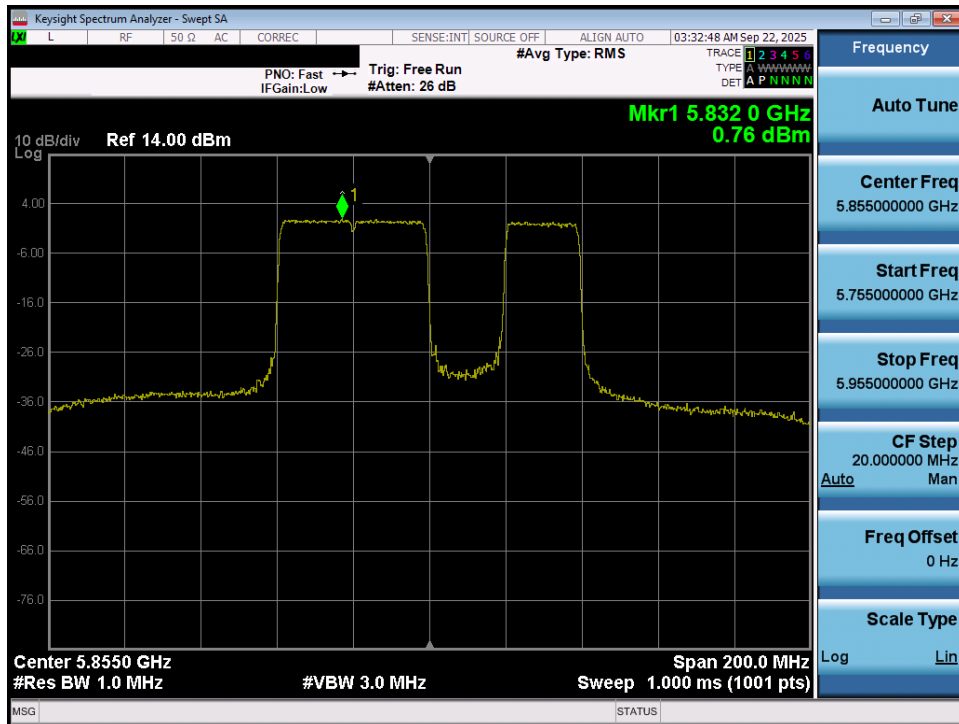
Plot 7-87. Power Spectral Density Plot MIMO ANT1 (80MHz BW 802.11be (UNII Band 3/4) – Ch. 171)
