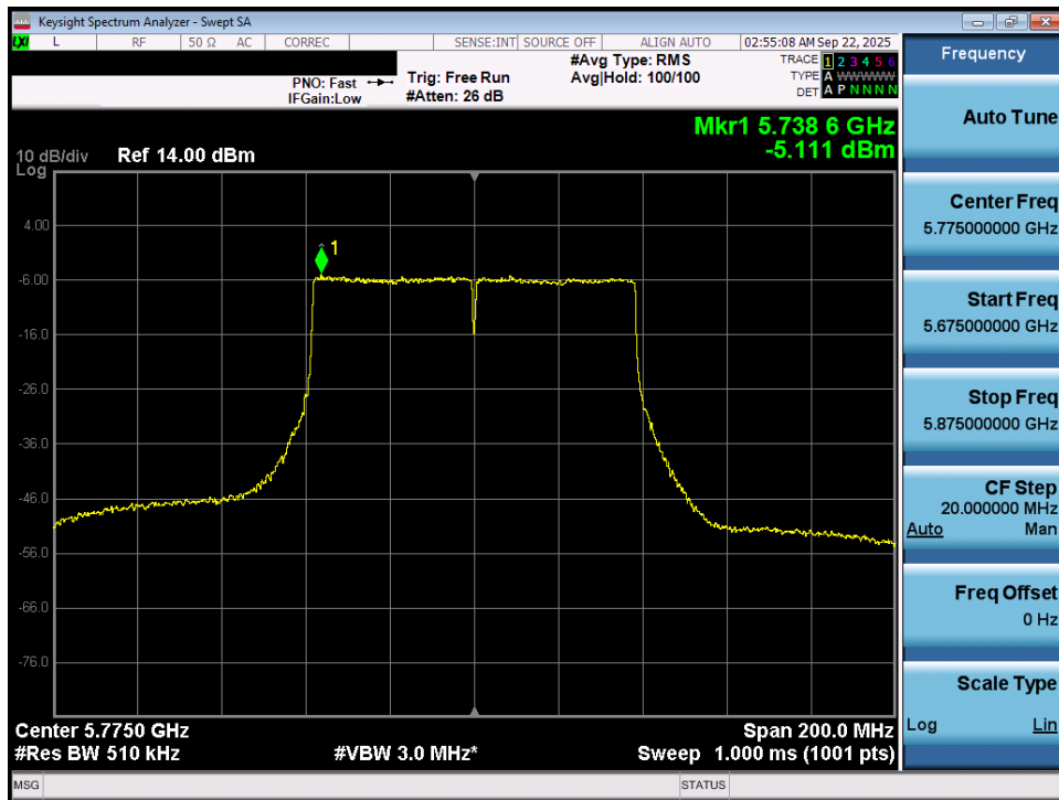
Plot 7-77. Power Spectral Density Plot MIMO ANT1 (80MHz BW 802.11ac (UNII Band 3) – Ch. 155)
