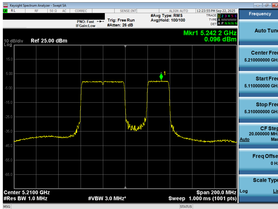
Plot 7-98. Power Spectral Density Plot MIMO ANT2 (80MHz BW 802.11be (20MHz Puncture) (UNII Band 1) – Ch. 42)
