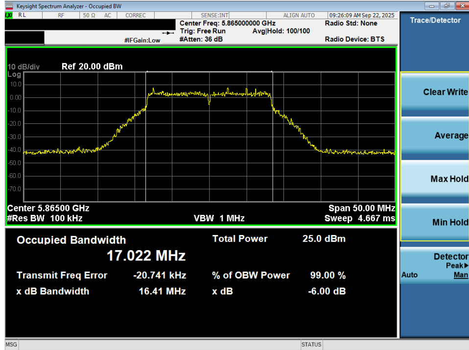
Plot 7-50. 6dB Bandwidth Plot MIMO ANT2 (802.11a (UNII Band 4) – Ch. 173)
