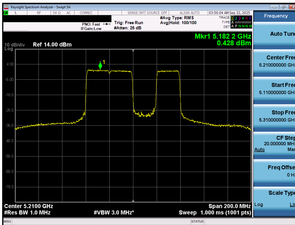
Plot 7-68. Power Spectral Density Plot MIMO ANT1 (80MHz BW 802.11be (20MHz Puncture) (UNII Band 1) – Ch. 42)
