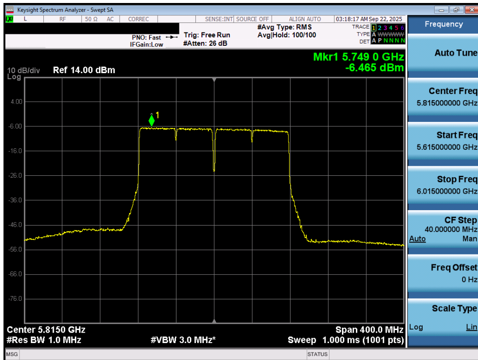
Plot 7-88. Power Spectral Density Plot MIMO ANT1 (160MHz BW 802.11ac (UNII Band 3/4) – Ch. 163)
