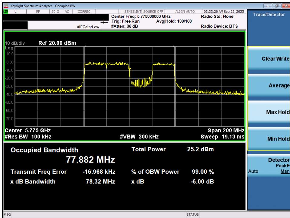
Plot 7-30. 6dB Bandwidth Plot MIMO ANT1 (80MHz BW 802.11be (20MHz Puncture) (UNII Band 3) – Ch. 155)
