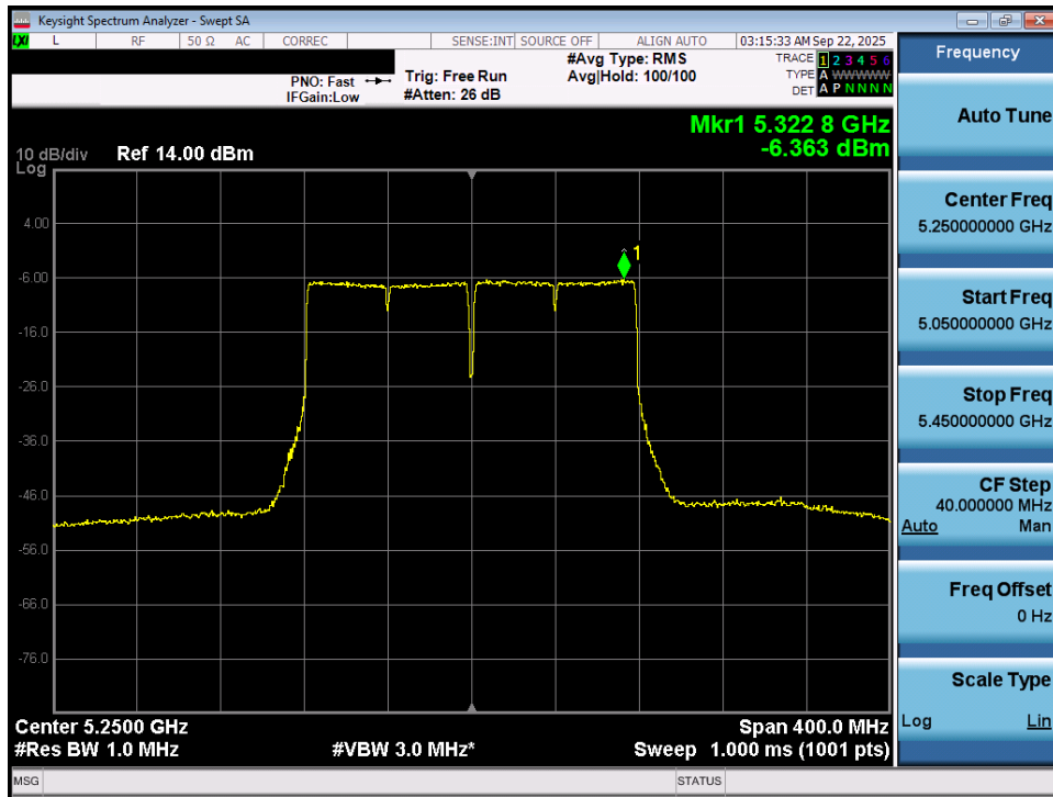
Plot 7-69. Power Spectral Density Plot MIMO ANT1 (160MHz BW 802.11ac (UNII Band 1/2A) – Ch. 50)
