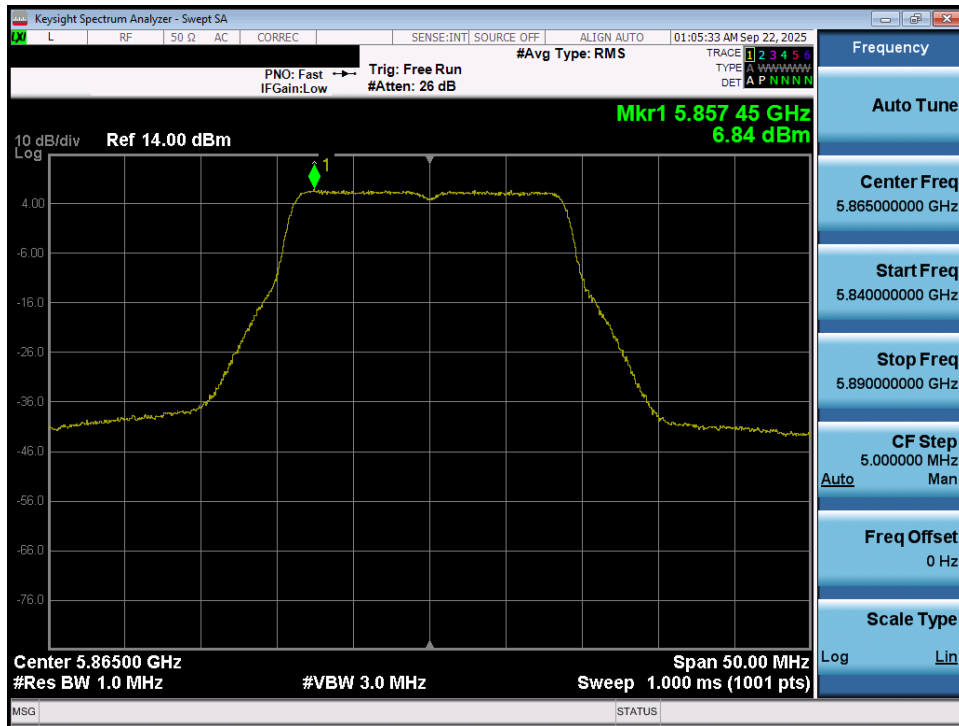
Plot 7-81. Power Spectral Density Plot MIMO ANT1 (20MHz BW 802.11n (UNII Band 4) – Ch. 173)
