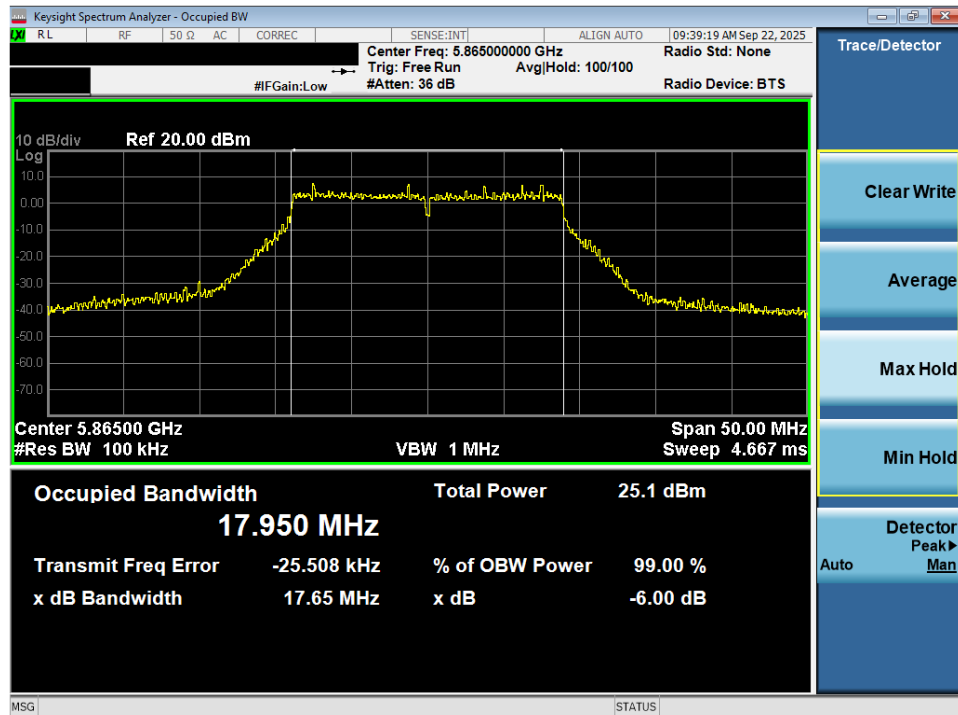
Plot 7-51. 6dB Bandwidth Plot MIMO ANT2 (20MHz BW 802.11n (UNII Band 4) – Ch. 173)
