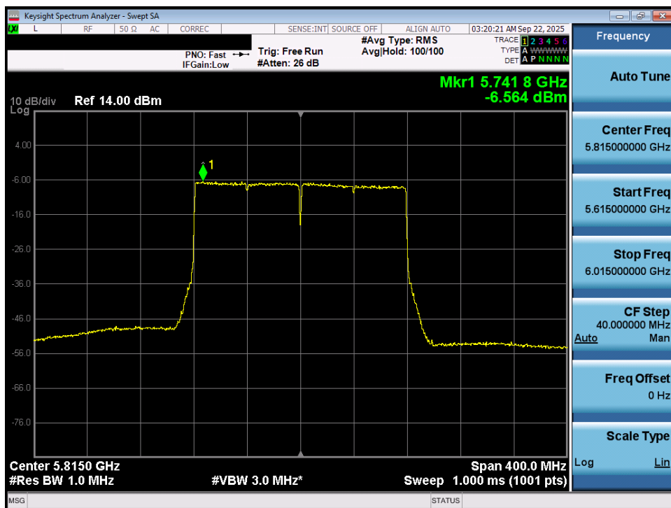
Plot 7-89. Power Spectral Density Plot MIMO ANT1 (160MHz BW 802.11be (UNII Band 3/4) – Ch. 163)
