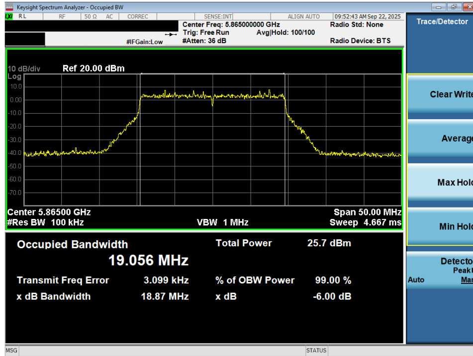
Plot 7-52. 6dB Bandwidth Plot MIMO ANT2 (20MHz BW 802.11be (UNII Band 4) – Ch. 173)
