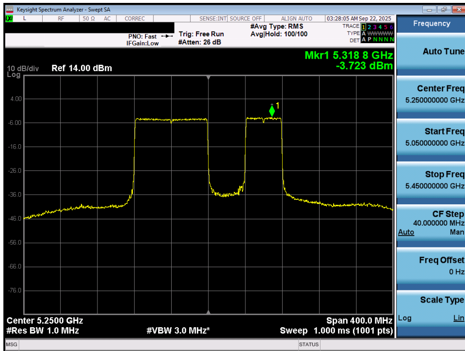
Plot 7-70. Power Spectral Density Plot MIMO ANT1 (160MHz BW 802.11be (40MHz Puncture) (UNII Band 1/2A) – Ch. 50)
