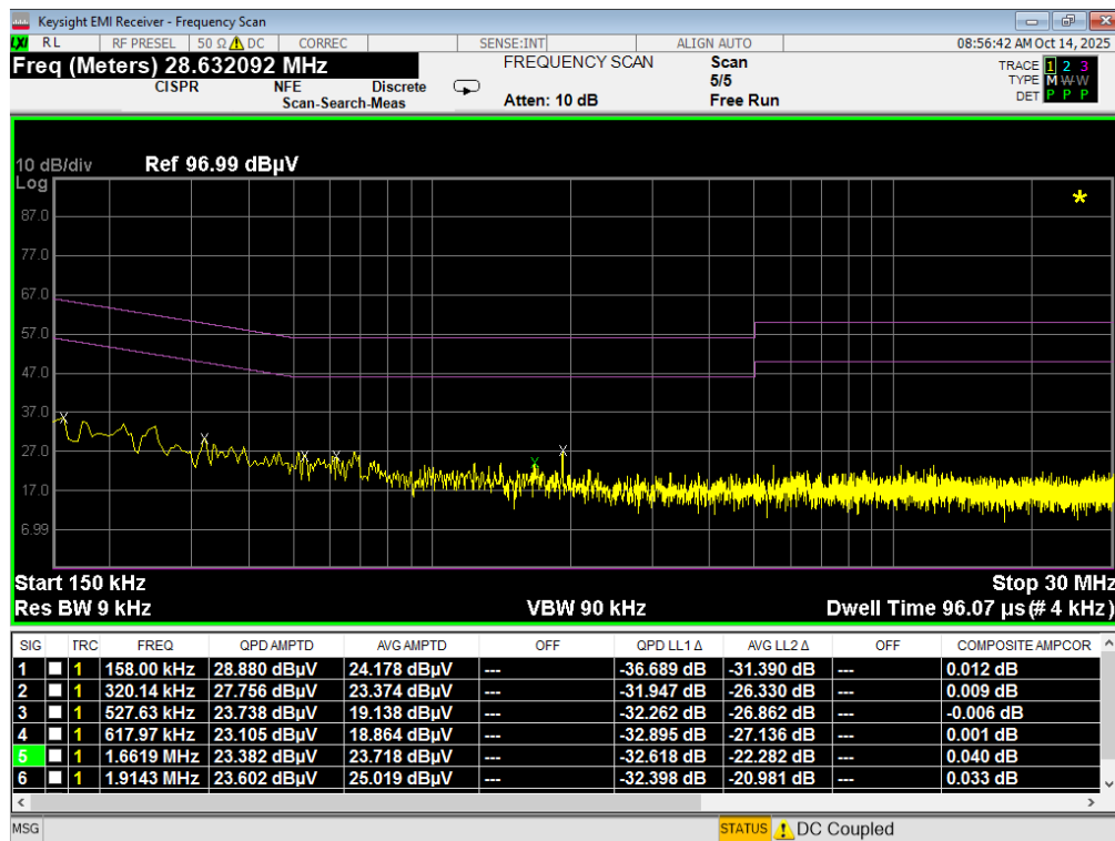
Plot 7-205. Line Conducted Plot with 802.11a UNII Band 2A (N) with WCP
