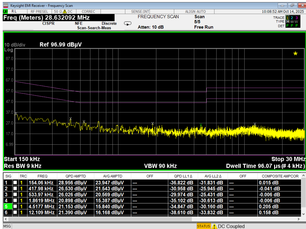
Plot 7-211. Line Conducted Plot with 802.11a UNII Band 4 (N) with WCP
