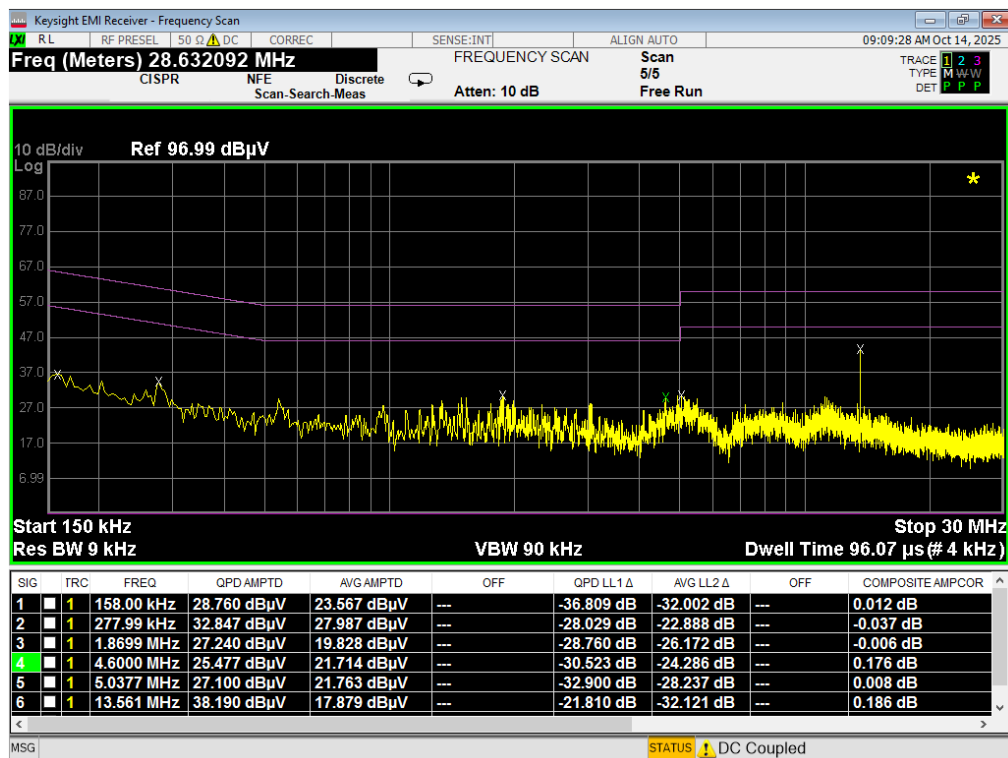
Plot 7-207. Line Conducted Plot with 802.11a UNII Band 2C (N) with WCP
