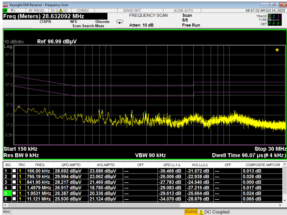
Plot 7-203. Line Conducted Plot with 802.11a UNII Band 1 (N) with WCP
