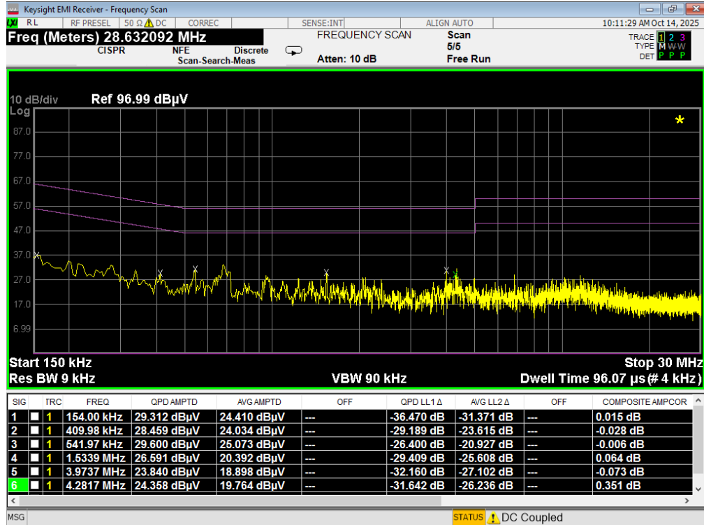
Plot 7-210. Line Conducted Plot with 802.11a UNII Band 4 (L1) with WCP
