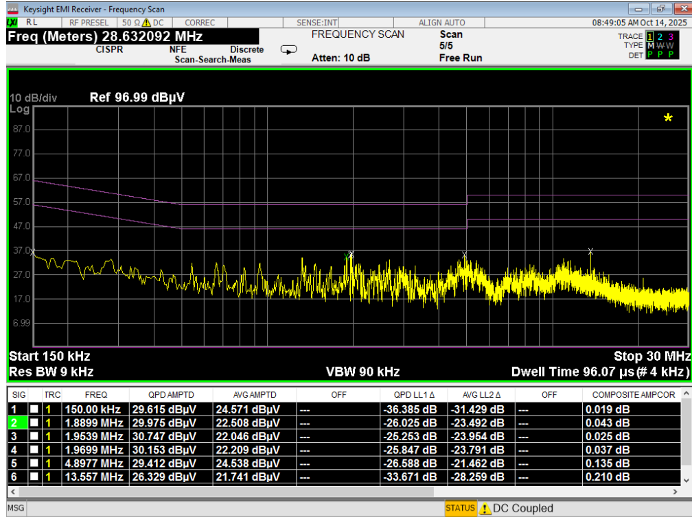
Plot 7-202. Line Conducted Plot with 802.11a UNII Band 1 (L1) with WCP
