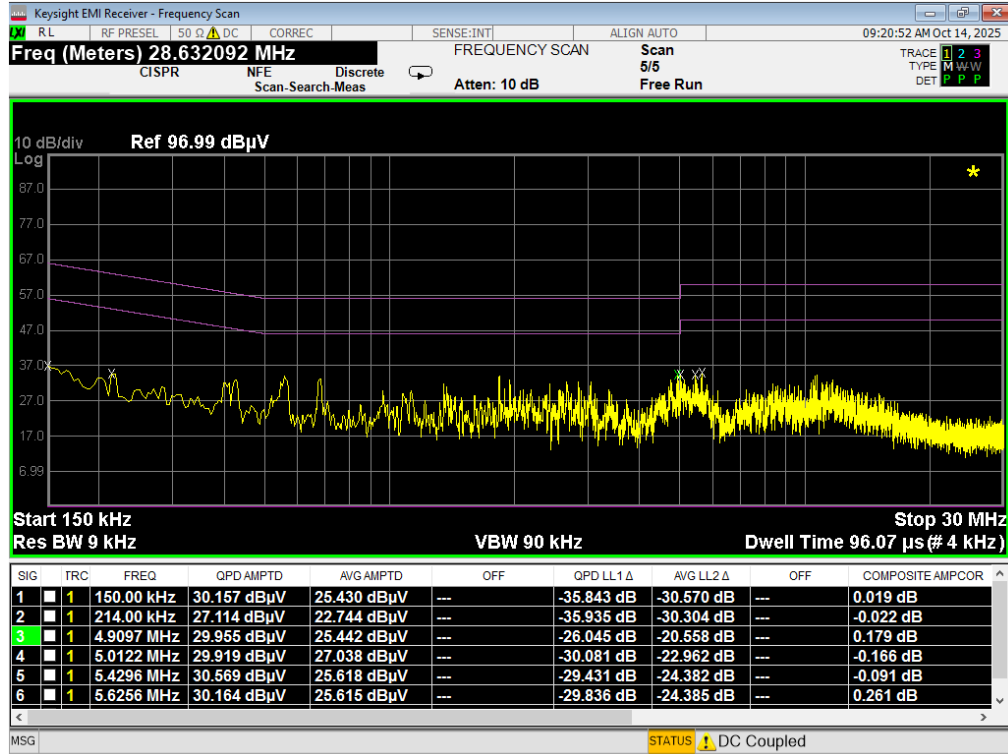
Plot 7-208. Line Conducted Plot with 802.11a UNII Band 3 (L1) with WCP
