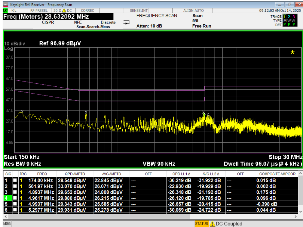
Plot 7-206. Line Conducted Plot with 802.11a UNII Band 2C (L1) with WCP
