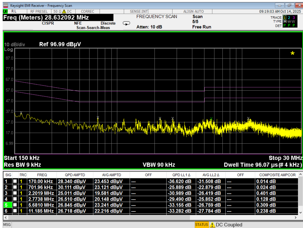
Plot 7-209. Line Conducted Plot with 802.11a UNII Band 3 (N) with WCP
