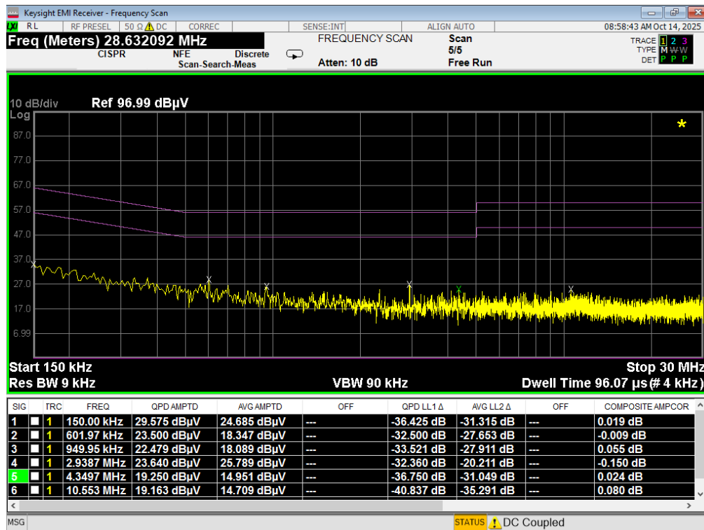
Plot 7-204. Line Conducted Plot with 802.11a UNII Band 2A (L1) with WCP
