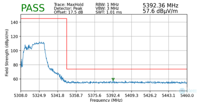
Plot 7-143. Radiated Upper Band Edge Plot MIMO (Peak – UNII Band 2A – 106+26 Tones)
