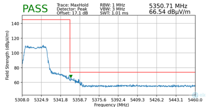
Plot 7-153. Radiated Upper Band Edge Plot MIMO (Peak – UNII Band 2A – 242 Tones)
