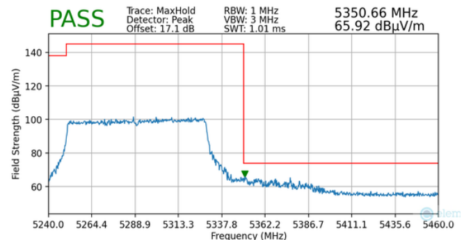
Plot 7-183. Radiated Upper Band Edge Plot MIMO (Peak – UNII Band 2A – 996 Tones)
