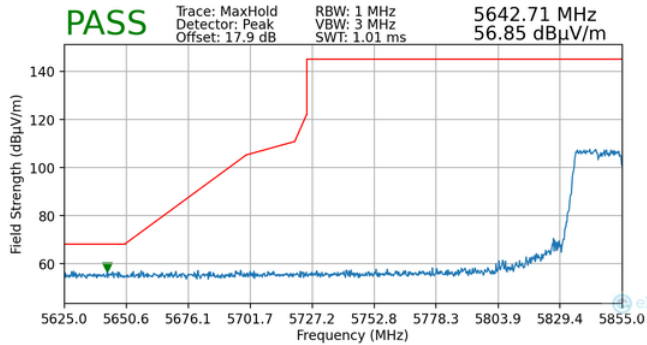
Plot 7-157. Radiated Lower Band Edge Plot MIMO (Peak - UNII Band 4 - 242 Tones)
