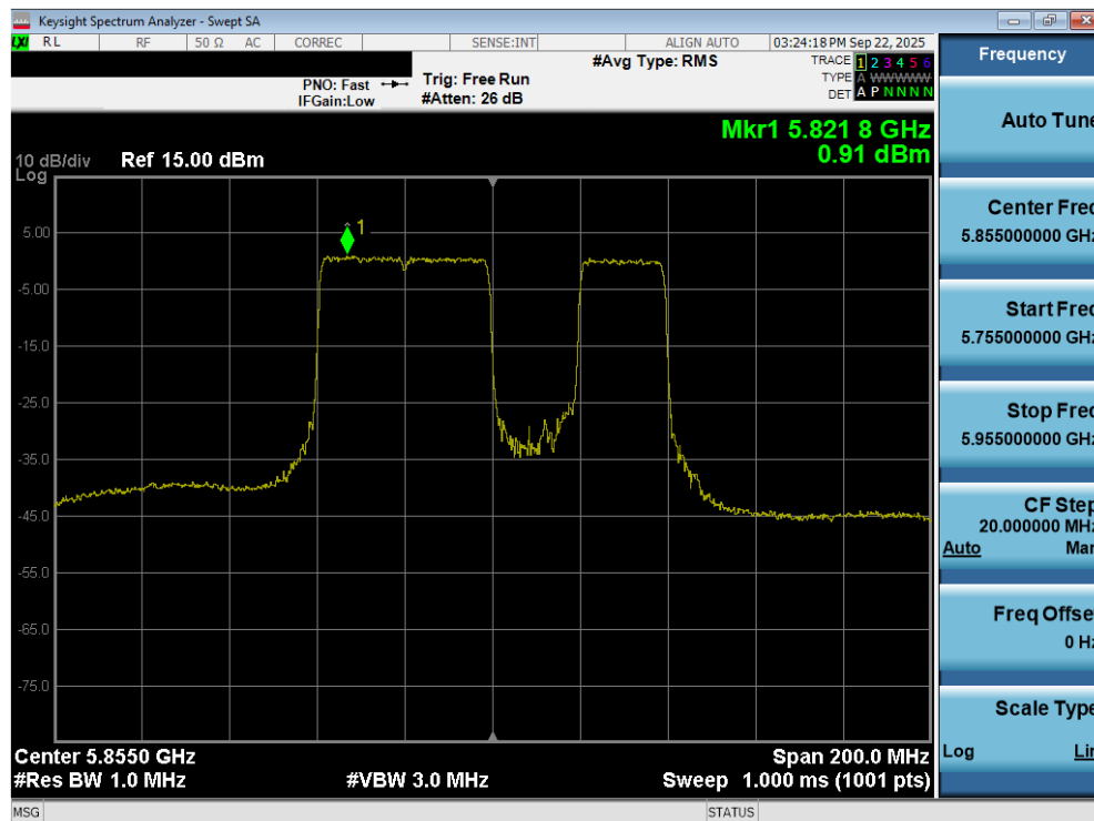
Plot 7-112. Power Spectral Density Plot MIMO ANT2 (80MHz BW 802.11be – 484+242 Tones (UNII Band 3/4) – Ch. 171)
