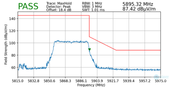
Plot 7-169. Radiated Upper Band Edge Plot MIMO (Peak - UNII Band 4 - 484 Tones)
