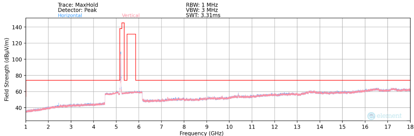
Plot 7-123. Radiated Spurious Plot above 1GHz MIMO (802.11ax – UNII 1 Ch. 40)
