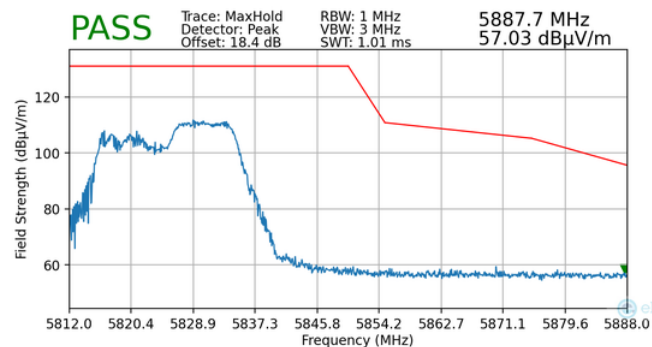
Plot 7-136. Radiated Upper Band Edge Plot MIMO (Peak – UNII Band 3 – 106 Tones)
