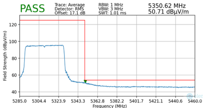
Plot 7-162. Radiated Upper Band Edge Plot MIMO (Average – UNII Band 2A – 484 Tones)
