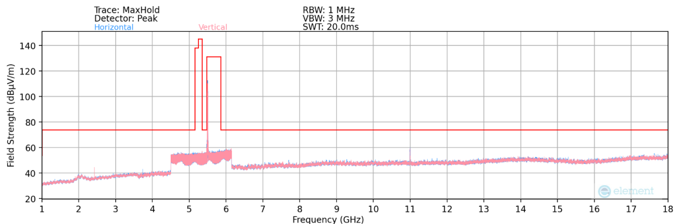
Plot 7-121. Radiated Spurious Plot above 1GHz MIMO (802.11ax – MRU 52+26 Tones)
