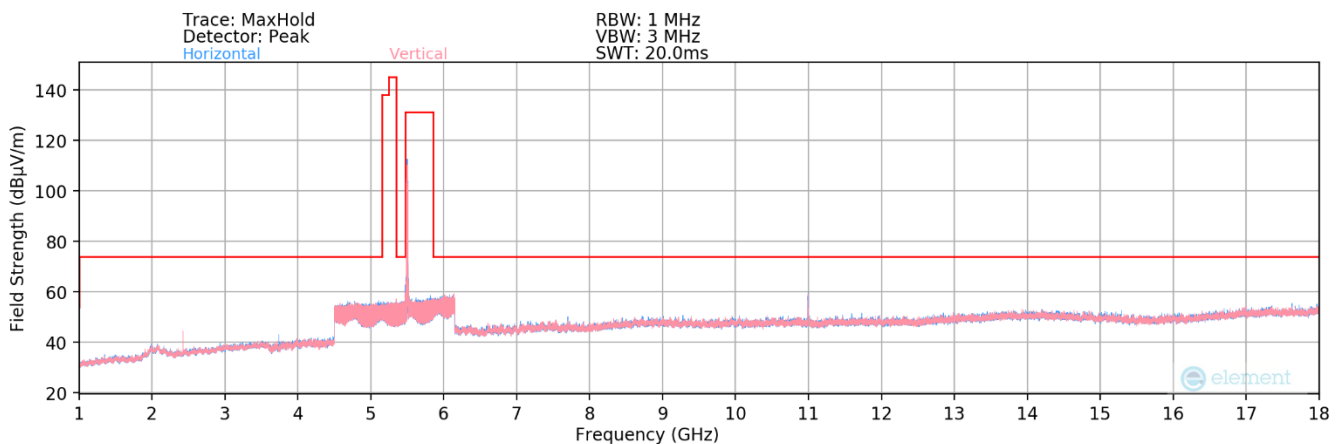
Plot 7-116. Radiated Spurious Plot above 1GHz MIMO (802.11ax – UNII 2C Ch. 100)
