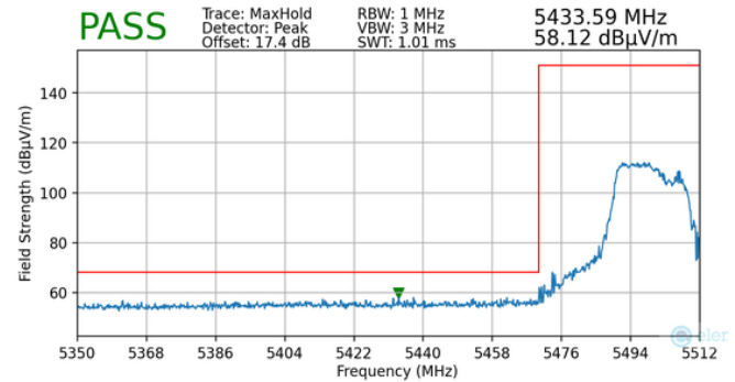
Plot 7-145. Radiated Lower Band Edge Plot MIMO (Peak – UNII Band 2C – 106+26 Tones)
