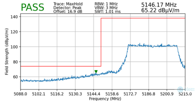
Plot 7-161. Radiated Lower Band Edge Plot MIMO (Peak – UNII Band 1 – 484 Tones)
