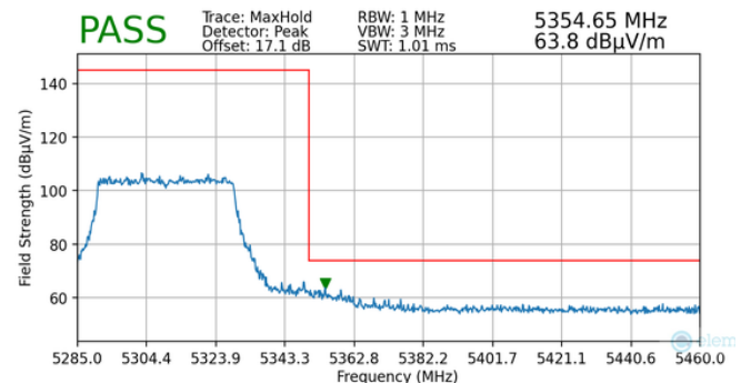
Plot 7-163. Radiated Upper Band Edge Plot MIMO (Peak – UNII Band 2A – 484 Tones)
