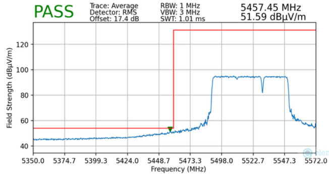
Plot 7-174. Radiated Lower Band Edge Plot MIMO (Average – UNII Band 2C – 484+242 Tones)
