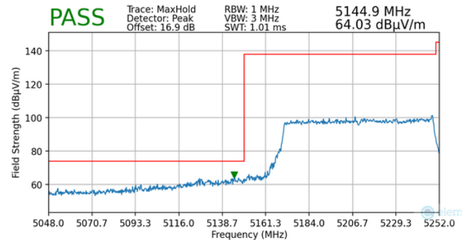
Plot 7-181. Radiated Lower Band Edge Plot MIMO (Peak – UNII Band 1 – 996 Tones)
