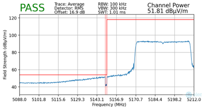
Plot 7-160. Radiated Lower Band Edge Plot MIMO (Average – UNII Band 1 – 484 Tones)
