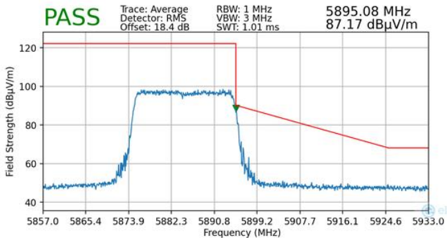
Plot 7-158. Radiated Upper Band Edge Plot MIMO (Average - UNII Band 4 - 242 Tones)
