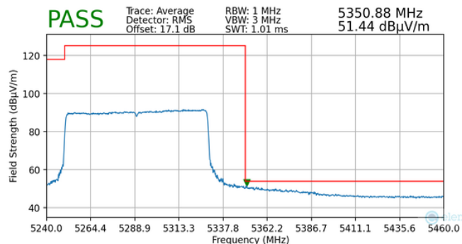
Plot 7-182. Radiated Upper Band Edge Plot MIMO (Average – UNII Band 2A – 996 Tones)
