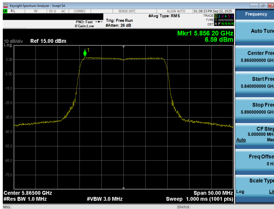
Plot 7-102. Power Spectral Density Plot MIMO ANT2 (20MHz BW 802.11be – 242 Tones (UNII Band 4) – Ch. 173)
