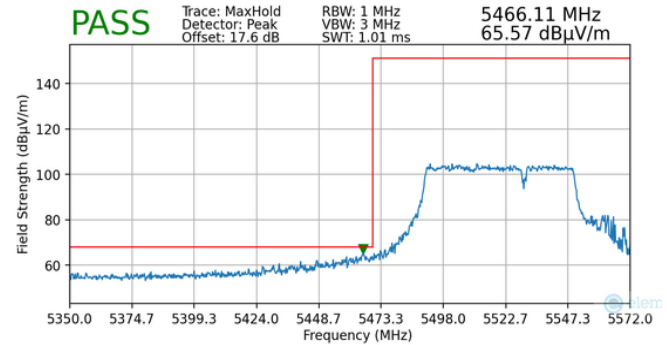
Plot 7-175. Radiated Lower Band Edge Plot MIMO (Peak – UNII Band 2C – 484+242 Tones)
