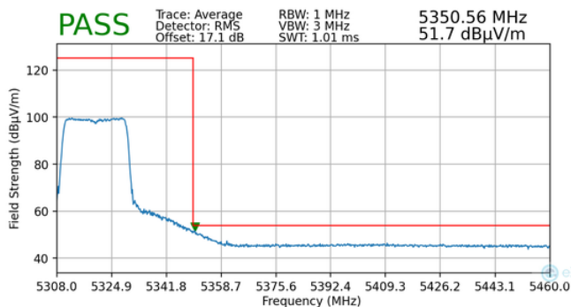
Plot 7-152. Radiated Upper Band Edge Plot MIMO (Average – UNII Band 2A – 242 Tones)
