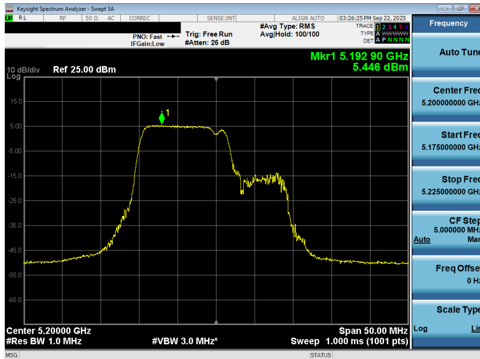
Plot 7-106. Power Spectral Density Plot MIMO ANT2 (20MHz BW 802.11be – 52+26 Tones (UNII Band 1) – Ch. 40)
