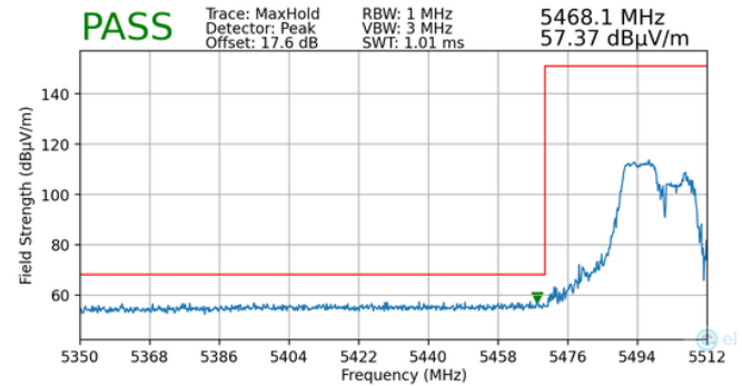
Plot 7-135. Radiated Lower Band Edge Plot MIMO (Peak – UNII Band 2C – 106 Tones)
