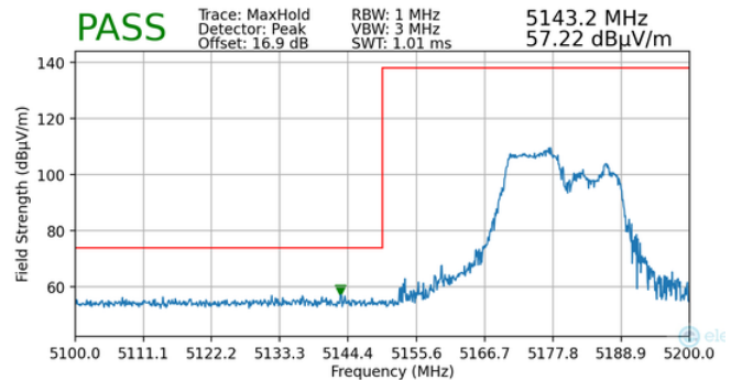
Plot 7-131. Radiated Lower Band Edge Plot MIMO (Peak – UNII Band 1 – 106 Tones)
