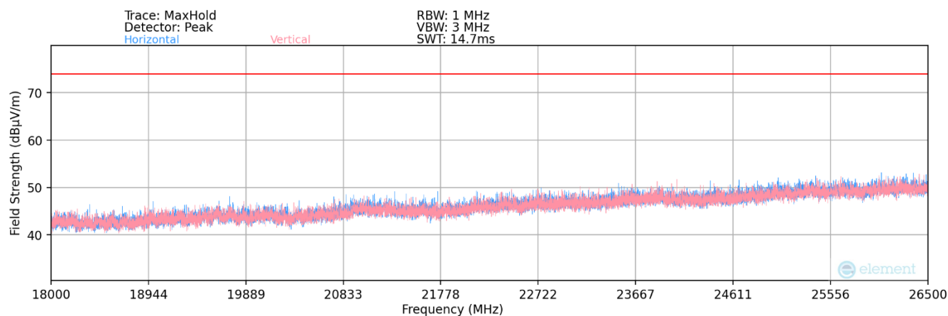
Plot 7-119. Radiated Spurious Plot 18GHz - 26.5GHz (802.11ax)
