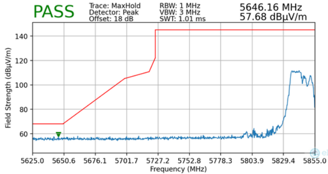
Plot 7-137. Radiated Lower Band Edge Plot MIMO (Peak – UNII Band 4 – 106 Tones)
