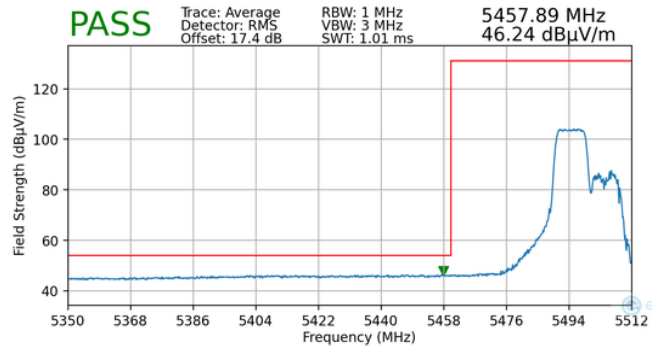
Plot 7-134. Radiated Lower Band Edge Plot MIMO (Average – UNII Band 2C – 106 Tones)
