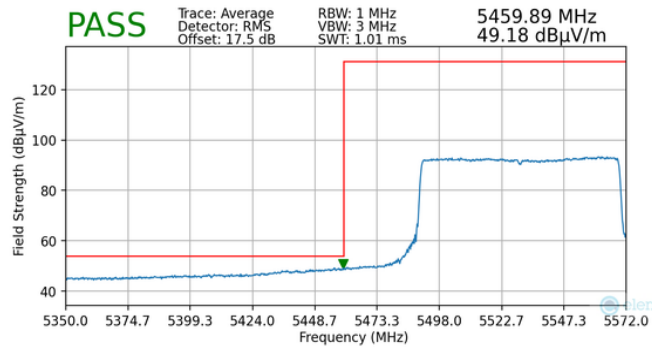
Plot 7-184. Radiated Lower Band Edge Plot MIMO (Average – UNII Band 2C – 996 Tones)
