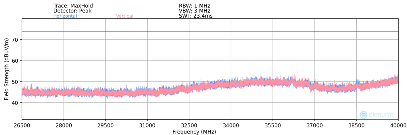
Plot 7-129. Radiated Spurious Plot 26.5GHz - 40GHz (802.11ax)
