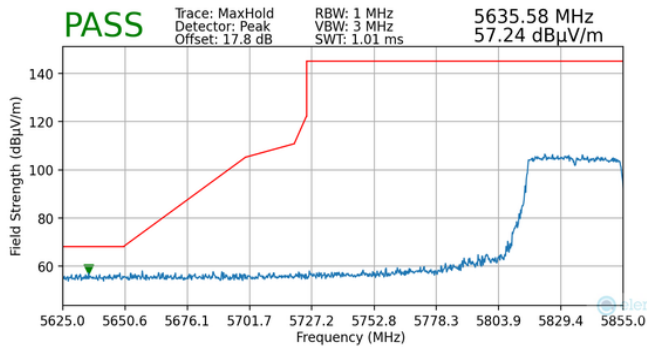
Plot 7-167. Radiated Lower Band Edge Plot MIMO (Peak - UNII Band 4 - 484 Tones)
