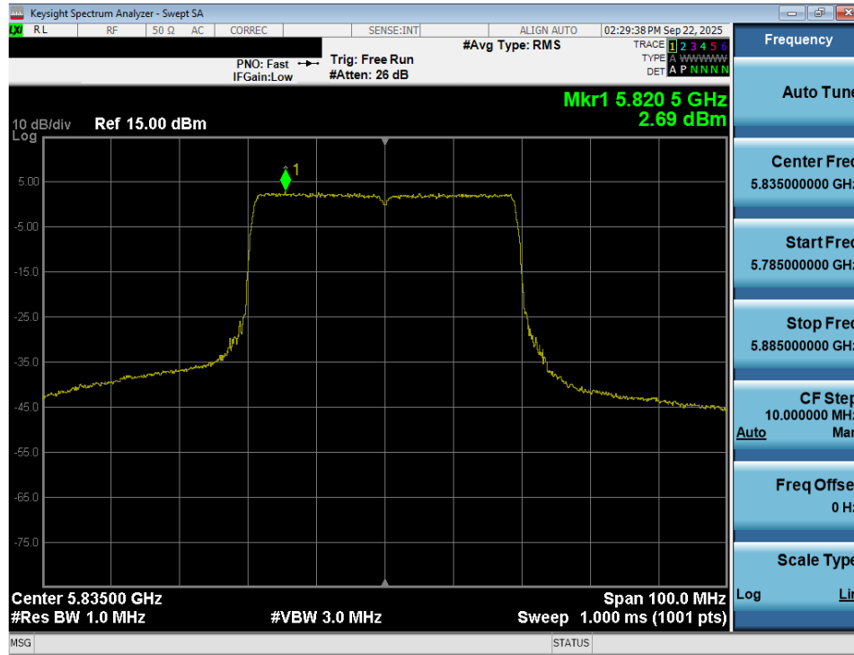
Plot 7-103. Power Spectral Density Plot MIMO ANT2 (40MHz BW 802.11be – 484 Tones (UNII Band 3/4) – Ch. 167)
