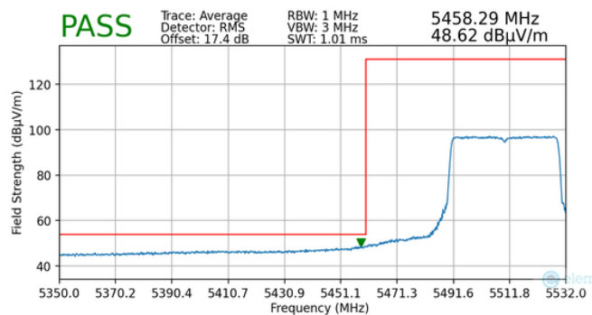
Plot 7-164. Radiated Lower Band Edge Plot MIMO (Average - UNII Band 2C - 484 Tones)
