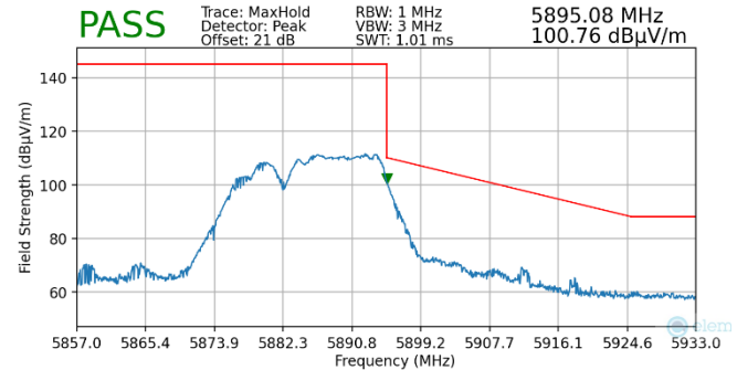
Plot 7-149. Radiated Upper Band Edge Plot MIMO (Peak - UNII Band 4 - 106+26 Tones)
