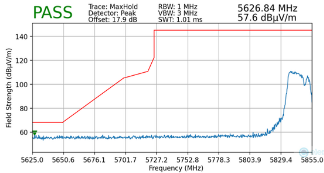
Plot 7-147. Radiated Lower Band Edge Plot MIMO (Peak - UNII Band 4 - 106+26 Tones)
