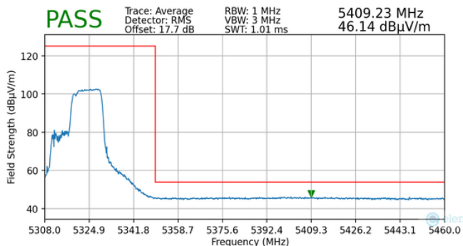
Plot 7-142. Radiated Upper Band Edge Plot MIMO (Average – UNII Band 2A – 106+26 Tones)
