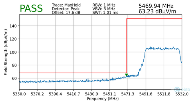
Plot 7-165. Radiated Lower Band Edge Plot MIMO (Peak - UNII Band 2C - 484 Tones)
