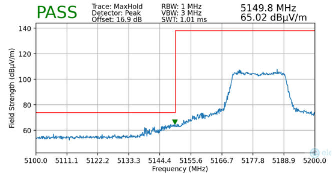
Plot 7-151. Radiated Lower Band Edge Plot MIMO (Peak – UNII Band 1 – 242 Tones)
