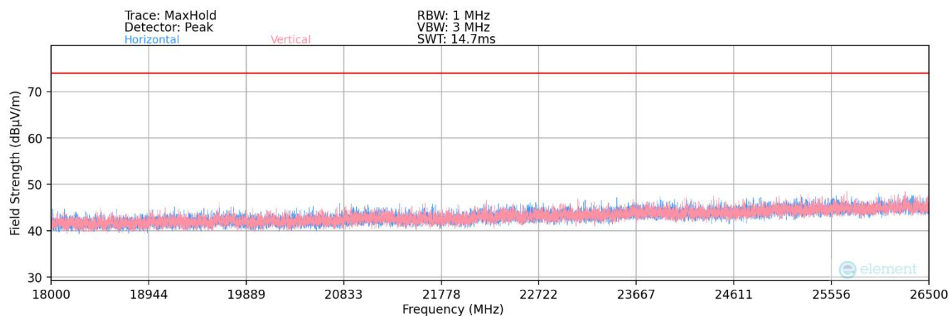
Plot 7-128. Radiated Spurious Plot 18GHz - 26.5GHz (802.11ax)
