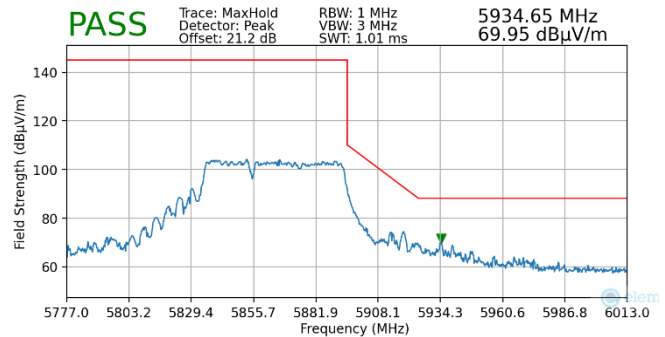
Plot 7-179. Radiated Upper Band Edge Plot MIMO (Peak - UNII Band 3/4 - 484+242 Tones)
