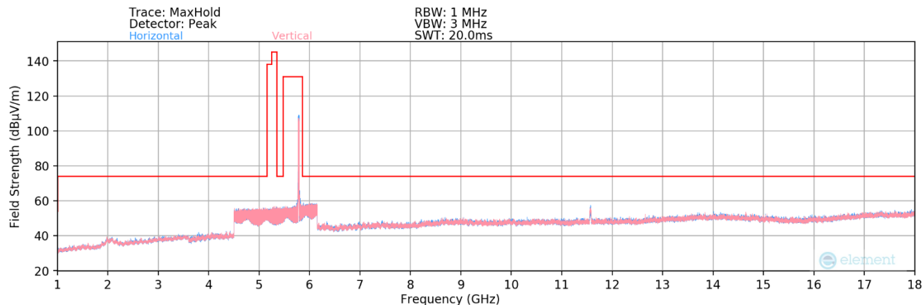
Plot 7-126. Radiated Spurious Plot above 1GHz MIMO (802.11ax – UNII 3 Ch. 157)
