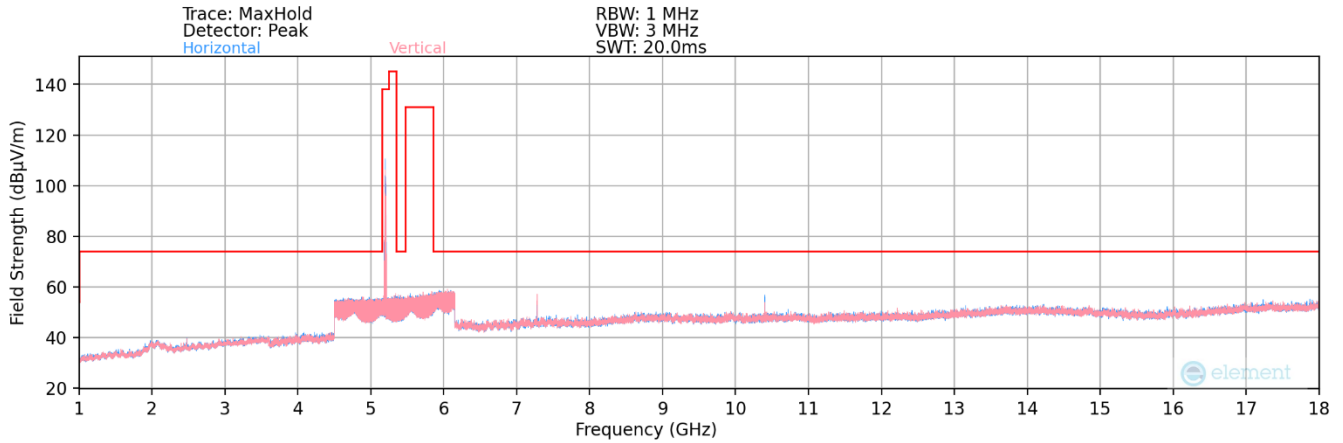
Plot 7-114. Radiated Spurious Plot above 1GHz MIMO (802.11ax – UNII 1 Ch. 40)
