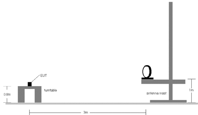
Figure 7-5. Radiated Test Setup < 30MHz
