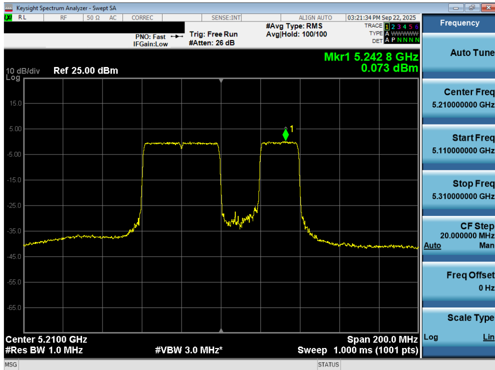
Plot 7-107. Power Spectral Density Plot MIMO ANT2 (80MHz BW 802.11be – 484+242 Tones (UNII Band 1) – Ch. 42)
