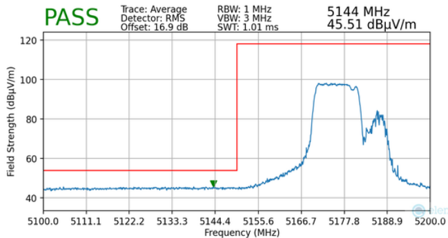
Plot 7-140. Radiated Lower Band Edge Plot MIMO (Average – UNII Band 1 – 106+26 Tones)
