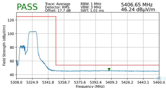
Plot 7-132. Radiated Upper Band Edge Plot MIMO (Average – UNII Band 2A – 106 Tones)
