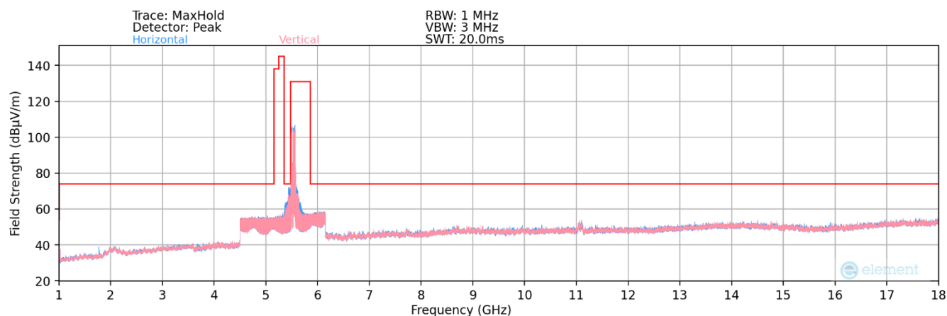
Plot 7-122. Radiated Spurious Plot above 1GHz MIMO (802.11ax – MRU 484+242 Tones)
