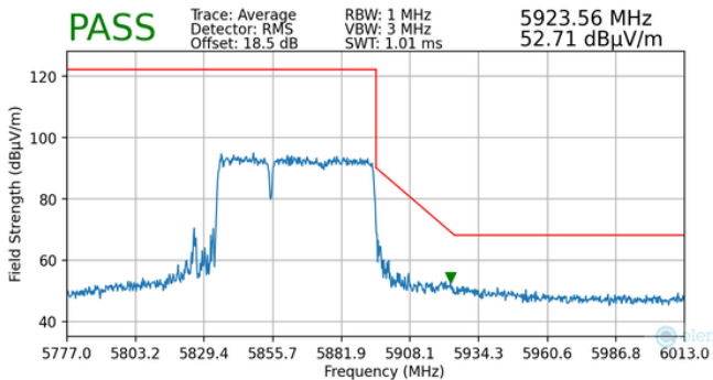
Plot 7-178. Radiated Upper Band Edge Plot MIMO (Average - UNII Band 3/4 - 484+242 Tones)
