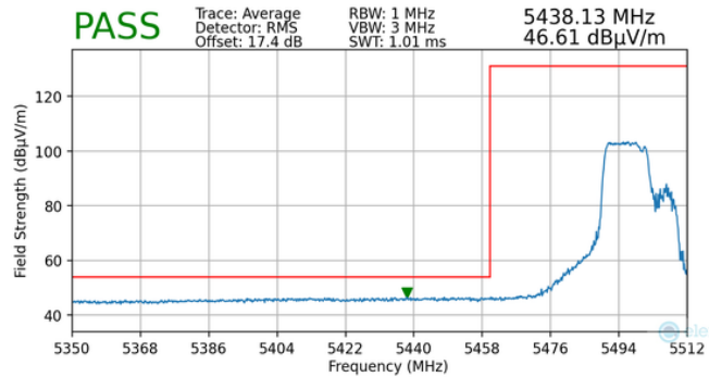
Plot 7-144. Radiated Lower Band Edge Plot MIMO (Average – UNII Band 2C – 106+26 Tones)
