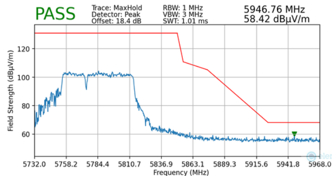
Plot 7-176. Radiated Upper Band Edge Plot MIMO (Peak – UNII Band 3 – 484+242 Tones)
