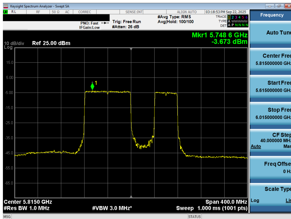
Plot 7-113. Power Spectral Density Plot MIMO ANT2 (160MHz BW 802.11be – 996+484 Tones (UNII Band 3/4) – Ch. 163)
