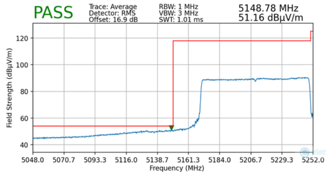
Plot 7-180. Radiated Lower Band Edge Plot MIMO (Average – UNII Band 1 – 996 Tones)
