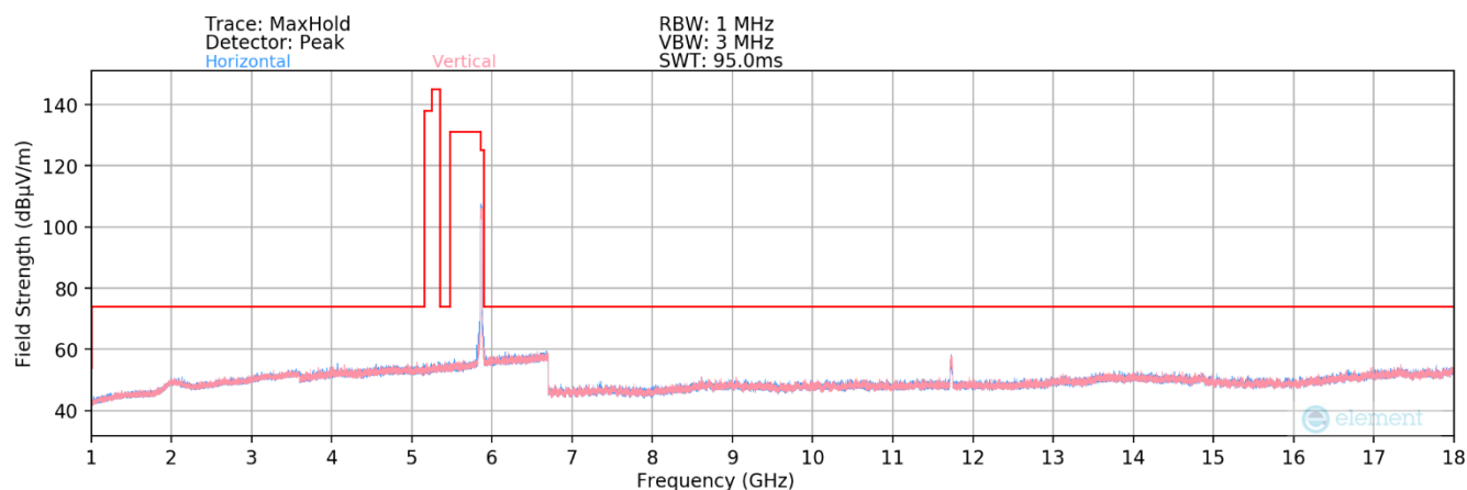
Plot 7-127. Radiated Spurious Plot above 1GHz MIMO (802.11ax – UNII 4 Ch. 173)
