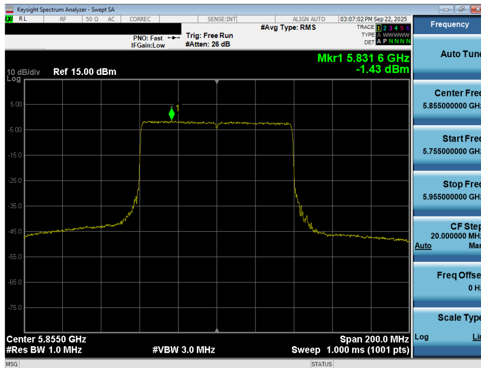
Plot 7-104. Power Spectral Density Plot MIMO ANT2 (80MHz BW 802.11be – 996 Tones (UNII Band 3/4) – Ch. 171)
