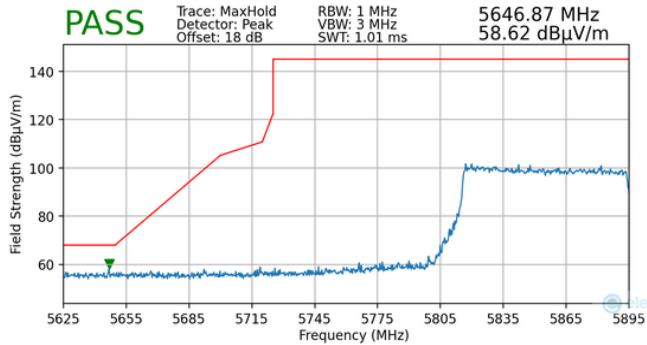
Plot 7-187. Radiated Lower Band Edge Plot MIMO (Peak - UNII Band 3/4 - 996 Tones)
