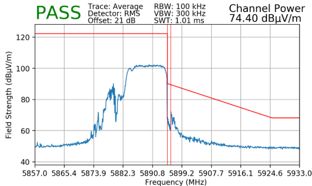
Plot 7-148. Radiated Upper Band Edge Plot MIMO (Average - UNII Band 4 - 106+26 Tones)
