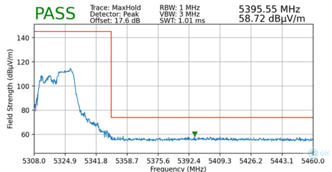
Plot 7-133. Radiated Upper Band Edge Plot MIMO (Peak – UNII Band 2A – 106 Tones)
