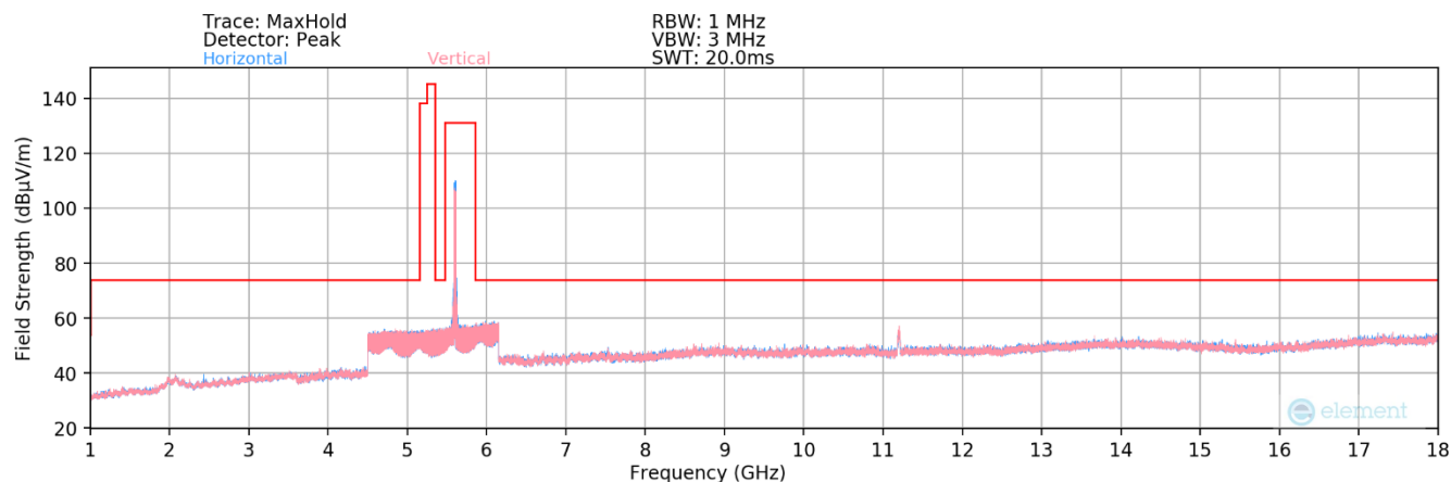
Plot 7-125. Radiated Spurious Plot above 1GHz MIMO (802.11ax – UNII 2C Ch. 120)
