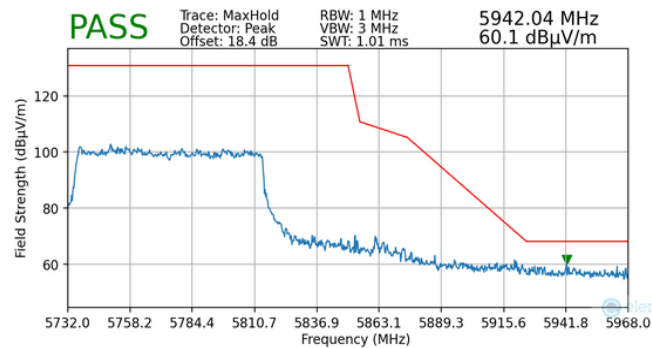
Plot 7-186. Radiated Upper Band Edge Plot MIMO (Peak – UNII Band 3 – 996 Tones)
