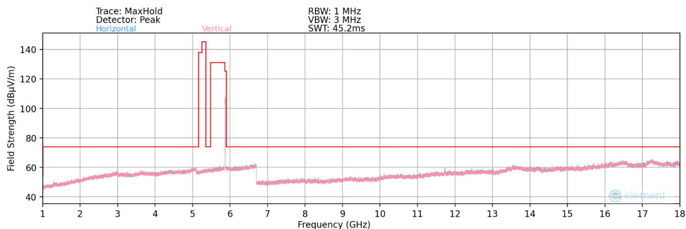
Plot 7-118. Radiated Spurious Plot above 1GHz MIMO (802.11ax – UNII 4 Ch. 173)
