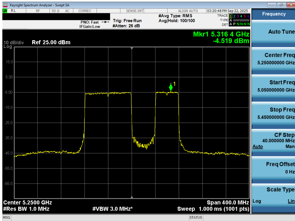
Plot 7-108. Power Spectral Density Plot MIMO ANT2 (160MHz BW 802.11be – 996+484 Tones (UNII Band 1/2A) – Ch. 50)
