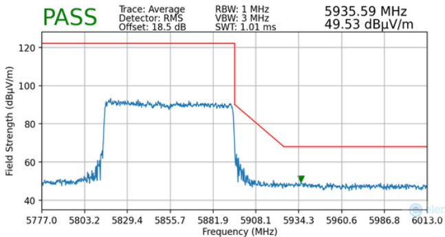
Plot 7-188. Radiated Upper Band Edge Plot MIMO (Average - UNII Band 3/4 - 996 Tones)
