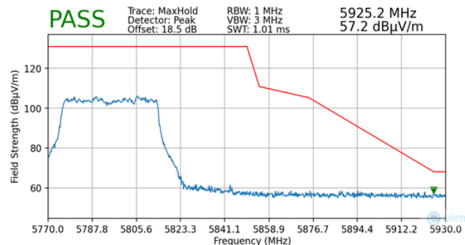
Plot 7-166. Radiated Upper Band Edge Plot MIMO (Peak - UNII Band 3 - 484 Tones)
