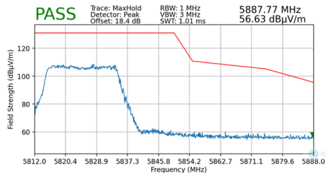
Plot 7-156. Radiated Upper Band Edge Plot MIMO (Peak – UNII Band 3 – 242 Tones)
