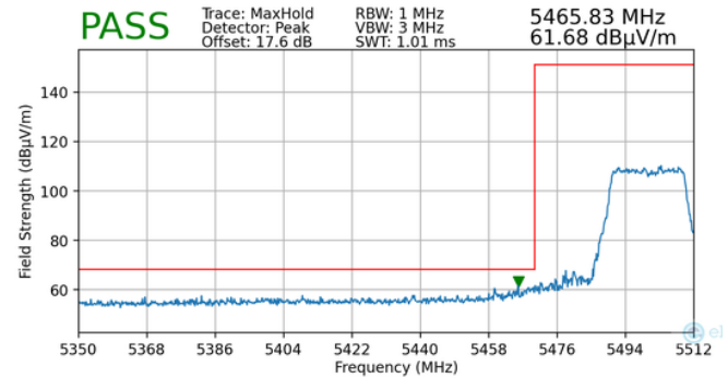
Plot 7-155. Radiated Lower Band Edge Plot MIMO (Peak – UNII Band 2C – 242 Tones)
