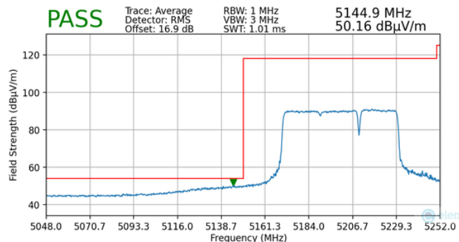
Plot 7-170. Radiated Lower Band Edge Plot MIMO (Average – UNII Band 1 – 484+242 Tones)
