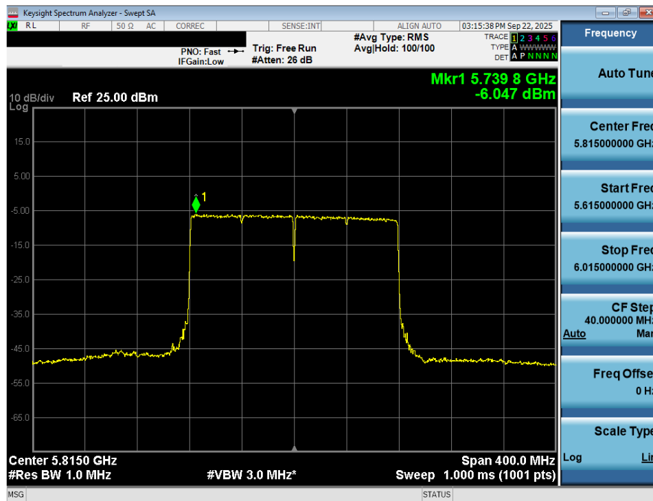
Plot 7-105. Power Spectral Density Plot MIMO ANT2 (160MHz BW 802.11be – 996*2 Tones (UNII Band 3/4) – Ch. 163)
