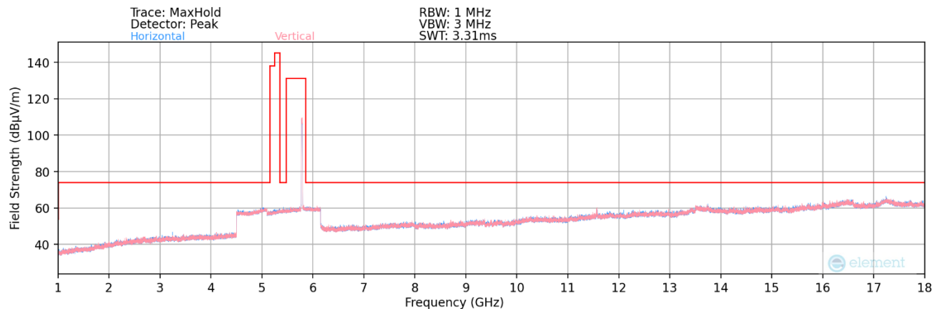
Plot 7-117. Radiated Spurious Plot above 1GHz MIMO (802.11ax – UNII 3 Ch. 157)
