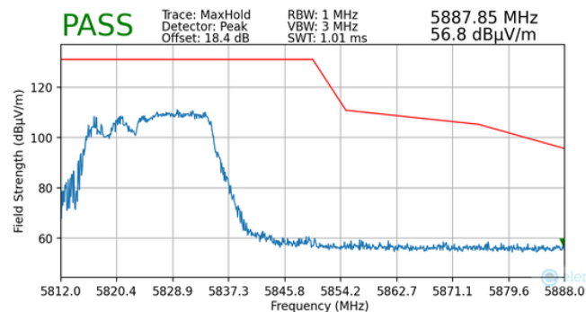
Plot 7-146. Radiated Upper Band Edge Plot MIMO (Peak – UNII Band 3 – 106+26 Tones)
