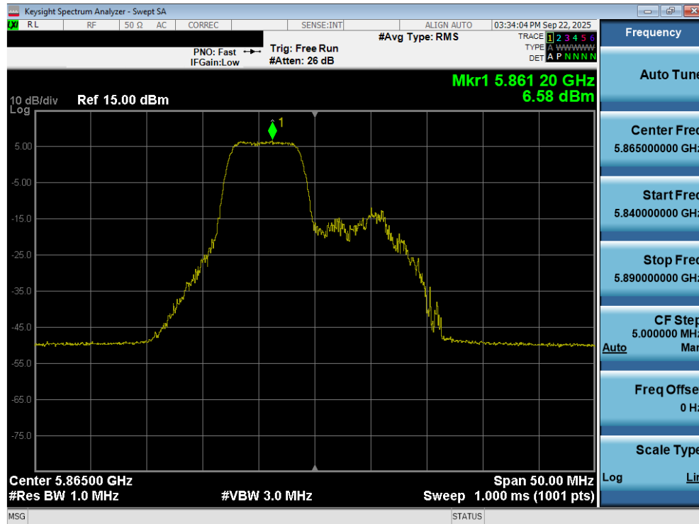
Plot 7-111. Power Spectral Density Plot MIMO ANT2 (20MHz BW 802.11be – 52+26 Tones (UNII Band 4) – Ch. 173)
