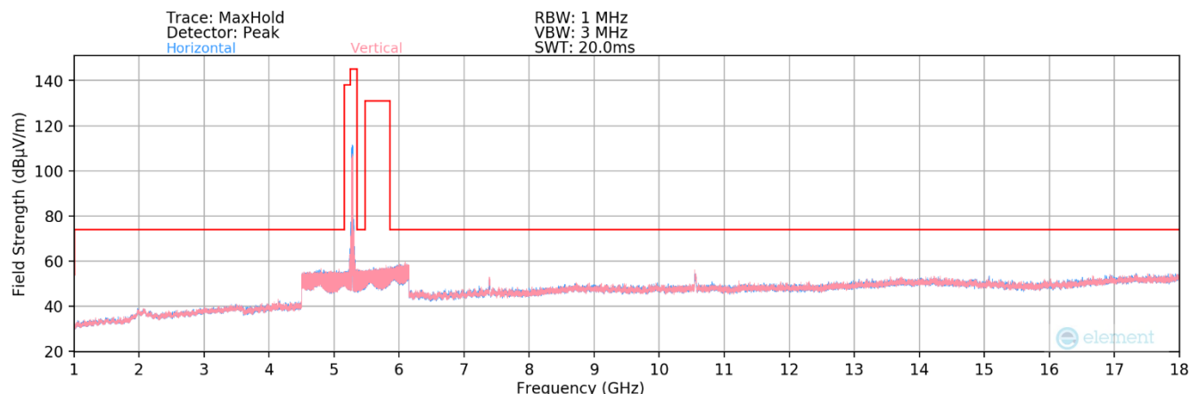
Plot 7-124. Radiated Spurious Plot above 1GHz MIMO (802.11ax – UNII 2A Ch. 56)
