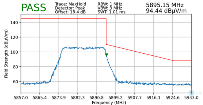
Plot 7-159. Radiated Upper Band Edge Plot MIMO (Peak - UNII Band 4 - 242 Tones)
