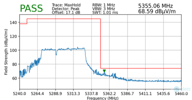
Plot 7-173. Radiated Upper Band Edge Plot MIMO (Peak – UNII Band 2A – 484+242 Tones)
