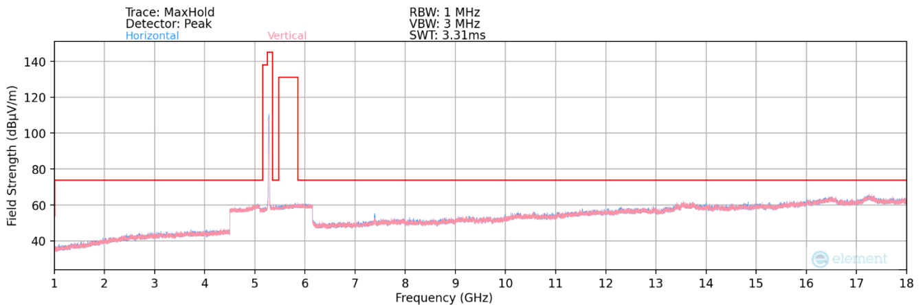
Plot 7-115. Radiated Spurious Plot above 1GHz MIMO (802.11ax – UNII 2A Ch. 56)
