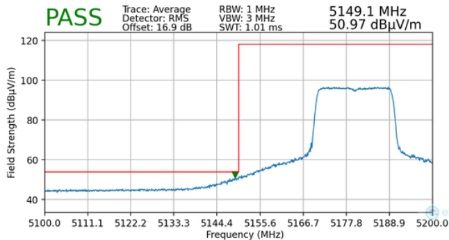
Plot 7-150. Radiated Lower Band Edge Plot MIMO (Average – UNII Band 1 – 242 Tones)
