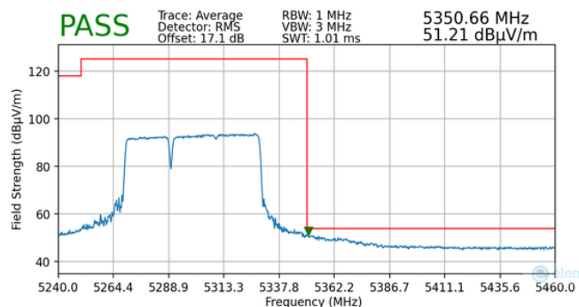
Plot 7-172. Radiated Upper Band Edge Plot MIMO (Average – UNII Band 2A – 484+242 Tones)
