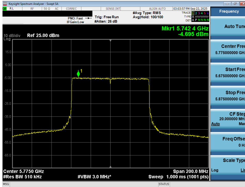
Plot 7-101. Power Spectral Density Plot MIMO ANT2 (80MHz BW 802.11be – 996 Tones (UNII Band 3) – Ch. 155)
