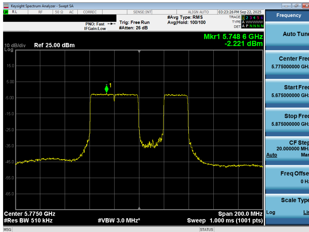
Plot 7-110. Power Spectral Density Plot MIMO ANT2 (80MHz BW 802.11be – 484+242 Tones (UNII Band 3) – Ch. 155)
