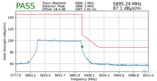
Plot 7-189. Radiated Upper Band Edge Plot MIMO (Peak - UNII Band 3/4 - 996 Tones)
