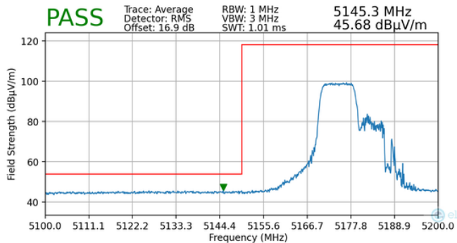
Plot 7-130. Radiated Lower Band Edge Plot MIMO (Average – UNII Band 1 – 106 Tones)
