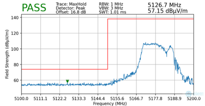
Plot 7-141. Radiated Lower Band Edge Plot MIMO (Peak – UNII Band 1 – 106+26 Tones)
