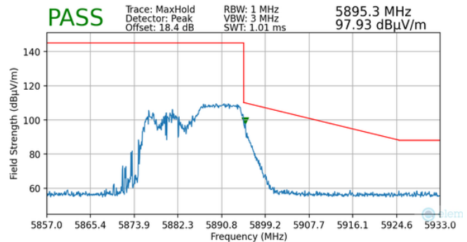
Plot 7-139. Radiated Upper Band Edge Plot MIMO (Peak – UNII Band 4 – 106 Tones)
