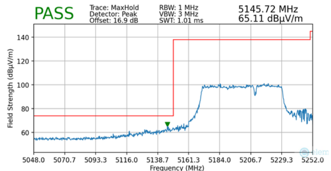
Plot 7-171. Radiated Lower Band Edge Plot MIMO (Peak – UNII Band 1 – 484+242 Tones)
