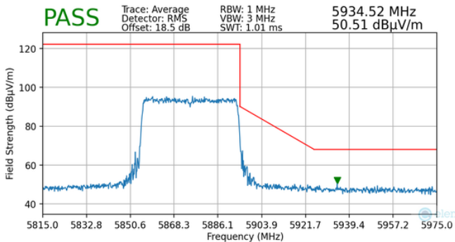
Plot 7-168. Radiated Upper Band Edge Plot MIMO (Average - UNII Band 4 - 484 Tones)
