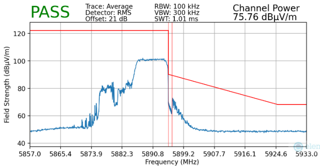
Plot 7-138. Radiated Upper Band Edge Plot MIMO (Average – UNII Band 4 – 106 Tones)
