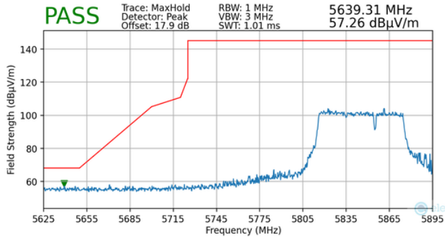
Plot 7-177. Radiated Lower Band Edge Plot MIMO (Peak - UNII Band 3/4 - 484+242 Tones)
