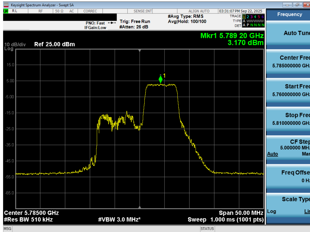
Plot 7-109. Power Spectral Density Plot MIMO ANT2 (20MHz BW 802.11be – 52+26 Tones (UNII Band 3) – Ch. 157)
