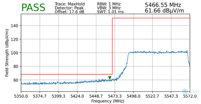
Plot 7-185. Radiated Lower Band Edge Plot MIMO (Peak – UNII Band 2C – 996 Tones)
