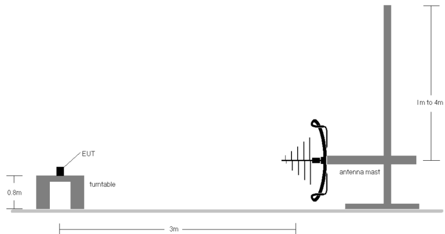
Figure 7-6. Radiated Test Setup < 1GHz
