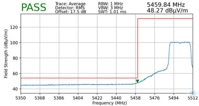
Plot 7-154. Radiated Lower Band Edge Plot MIMO (Average – UNII Band 2C – 242 Tones)
