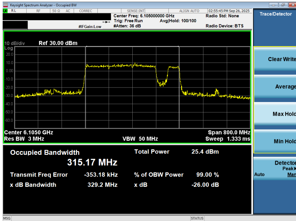
Plot 7-36. 26dB Bandwidth Plot MIMO ANT2 (320MHz 802.11be (UNII Band 5) – Ch. 31) – 40MHz Punctured – SP
