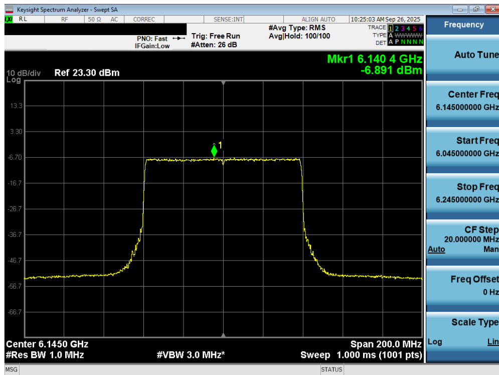
Plot 7-58. Power Spectral Density Plot MIMO ANT2 (80MHz 802.11ax/be (UNII Band 5) – Ch. 39) - LPI
