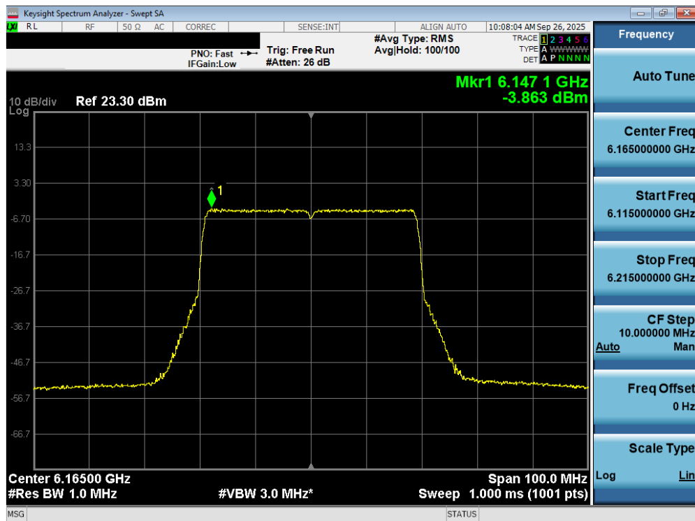
Plot 7-57. Power Spectral Density Plot MIMO ANT2 (40MHz 802.11ax/be (UNII Band 5) – Ch. 43) - LPI
