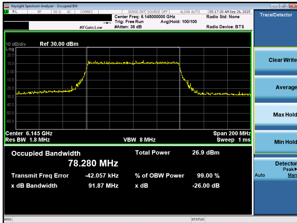
Plot 7-13. 26dB Bandwidth Plot MIMO ANT1 (80MHz 802.11ax/be (UNII Band 5) – Ch. 39) – SP
