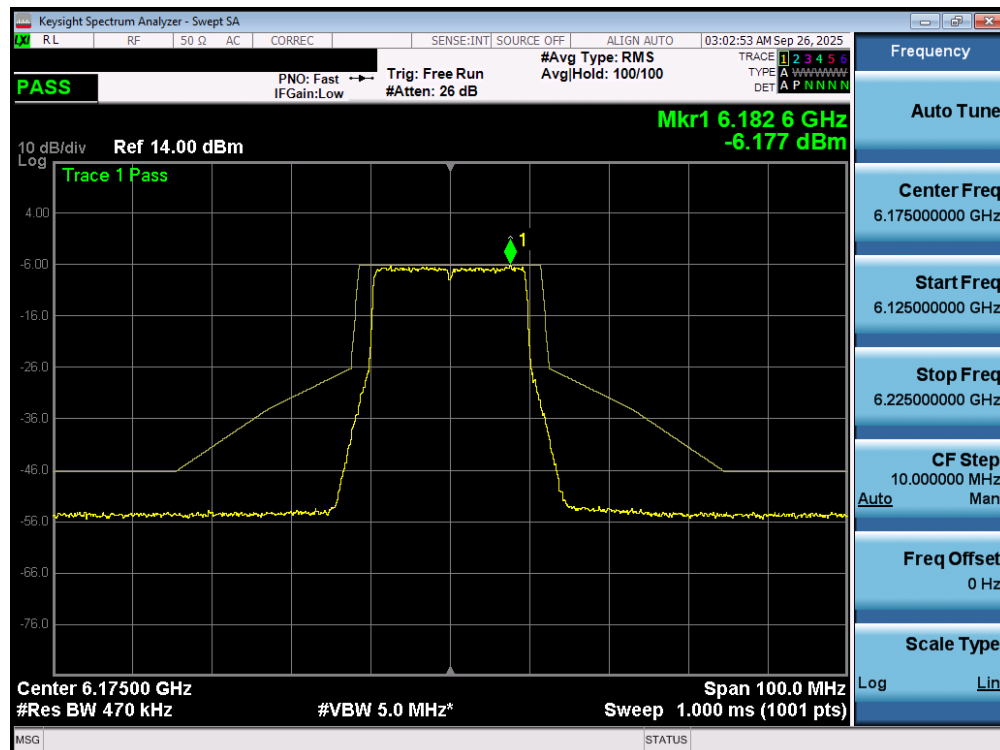
Plot 7-74. In Band Emissions Plot MIMO ANT1 (20MHz 802.11ax/be (UNII Band 5) – Ch. 45) - LPI
