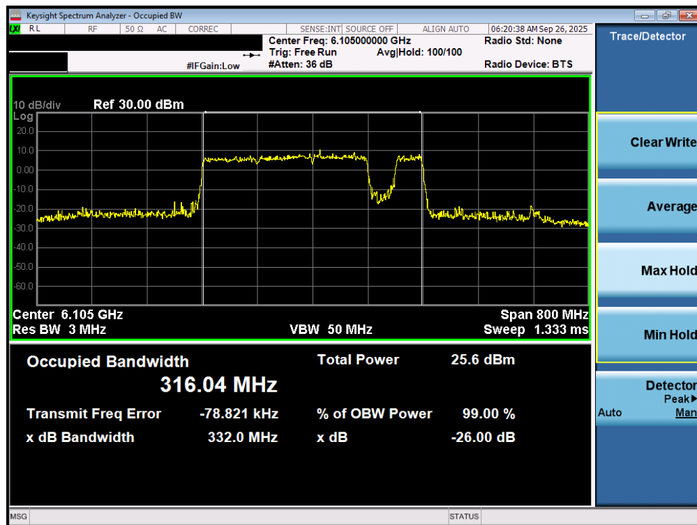
Plot 7-18. 26dB Bandwidth Plot MIMO ANT1 (320MHz 802.11be (UNII Band 5) – Ch. 31) – 40MHz Punctured – SP
