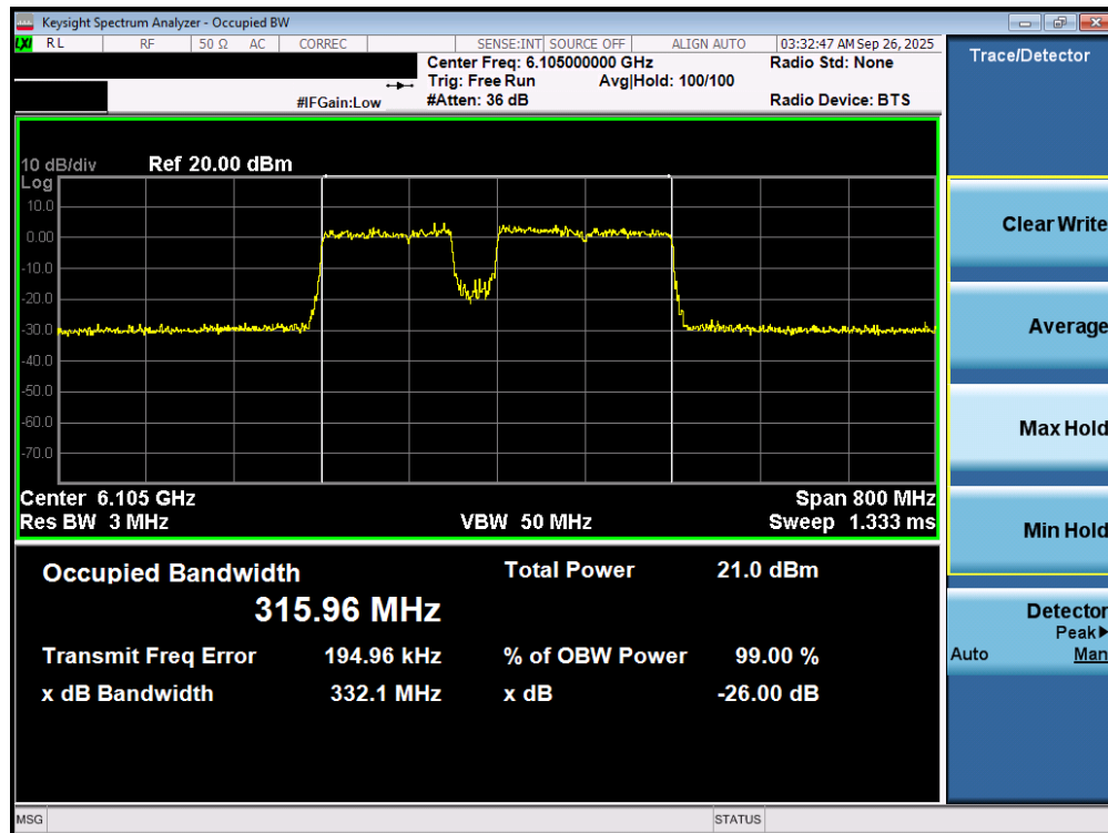
Plot 7-9. 26dB Bandwidth Plot MIMO ANT1 (320MHz 802.11be (UNII Band 5) – Ch. 31) – 40MHz Punctured – LPI
