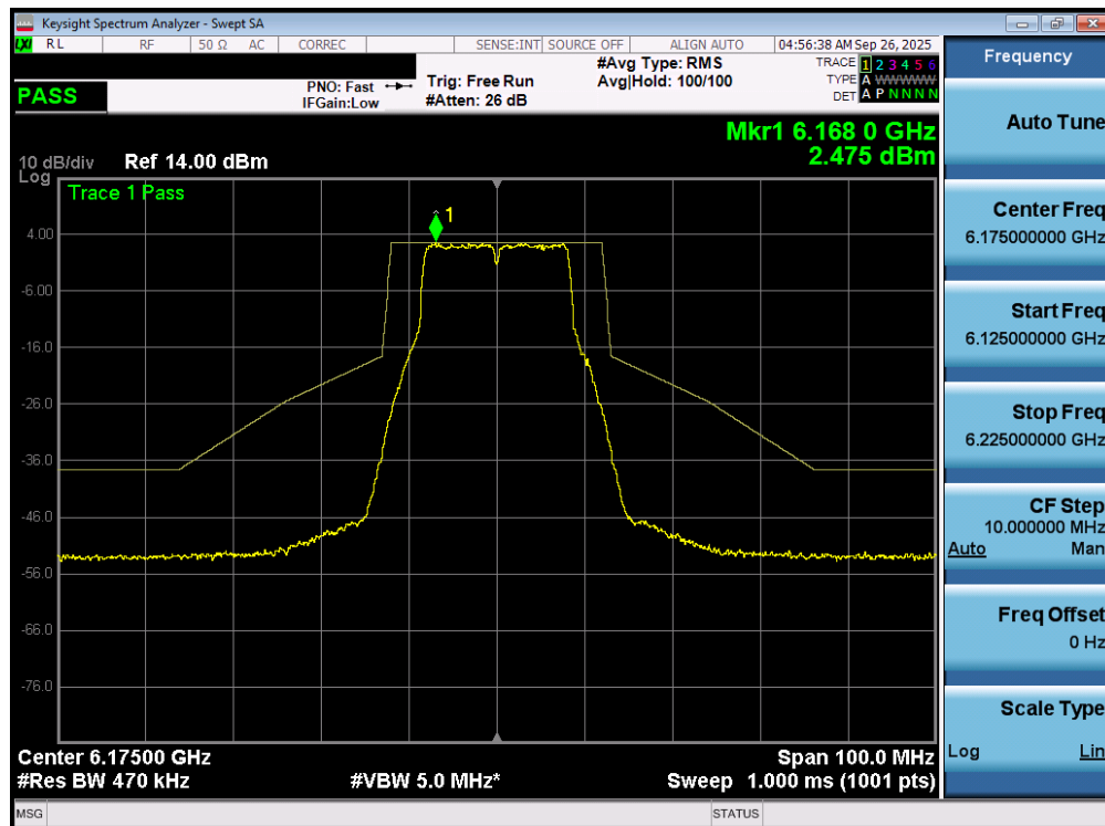
Plot 7-82. In Band Emissions Plot MIMO ANT1 (20MHz 802.11a (UNII Band 5) – Ch. 45) - SP
