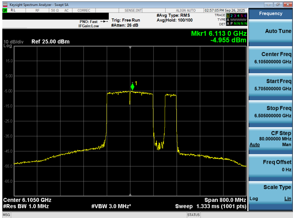
Plot 7-72. Power Spectral Density Plot MIMO ANT2 (320MHz 802.11be (UNII Band 5) – Ch. 31) – 120MHz Punctured – SP
