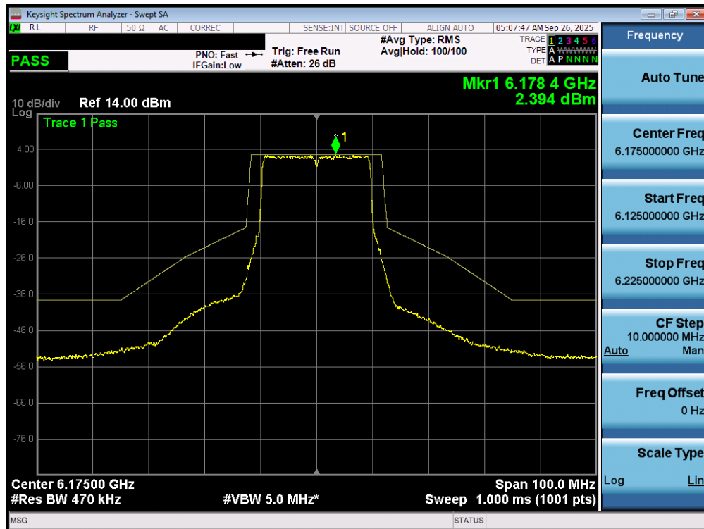
Plot 7-83. In Band Emissions Plot MIMO ANT1 (20MHz 802.11ax/be (UNII Band 5) – Ch. 45) - SP
