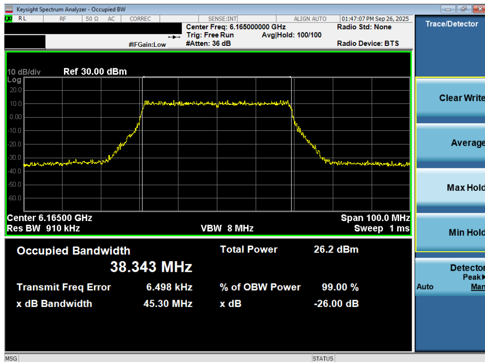
Plot 7-30. 26dB Bandwidth Plot MIMO ANT2 (40MHz 802.11ax/be (UNII Band 5) – Ch. 43) - SP
