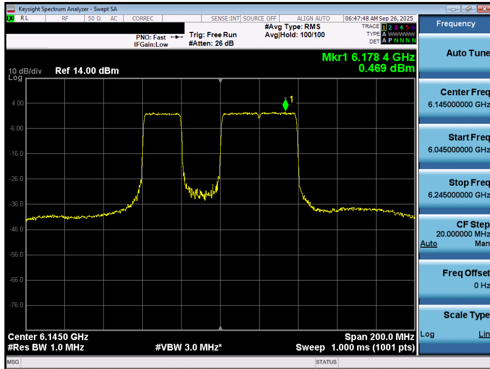
Plot 7-52. Power Spectral Density Plot MIMO ANT1 (80MHz 802.11be (UNII Band 5) – Ch. 39) – 20MHz Punctured - SP
