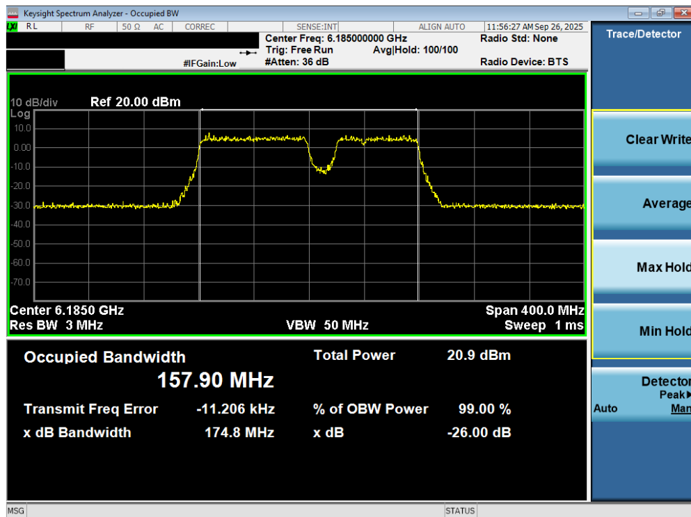
Plot 7-26. 26dB Bandwidth Plot MIMO ANT2 (160MHz 802.11be (UNII Band 5) – Ch. 47) – 20MHz Punctured - LPI
