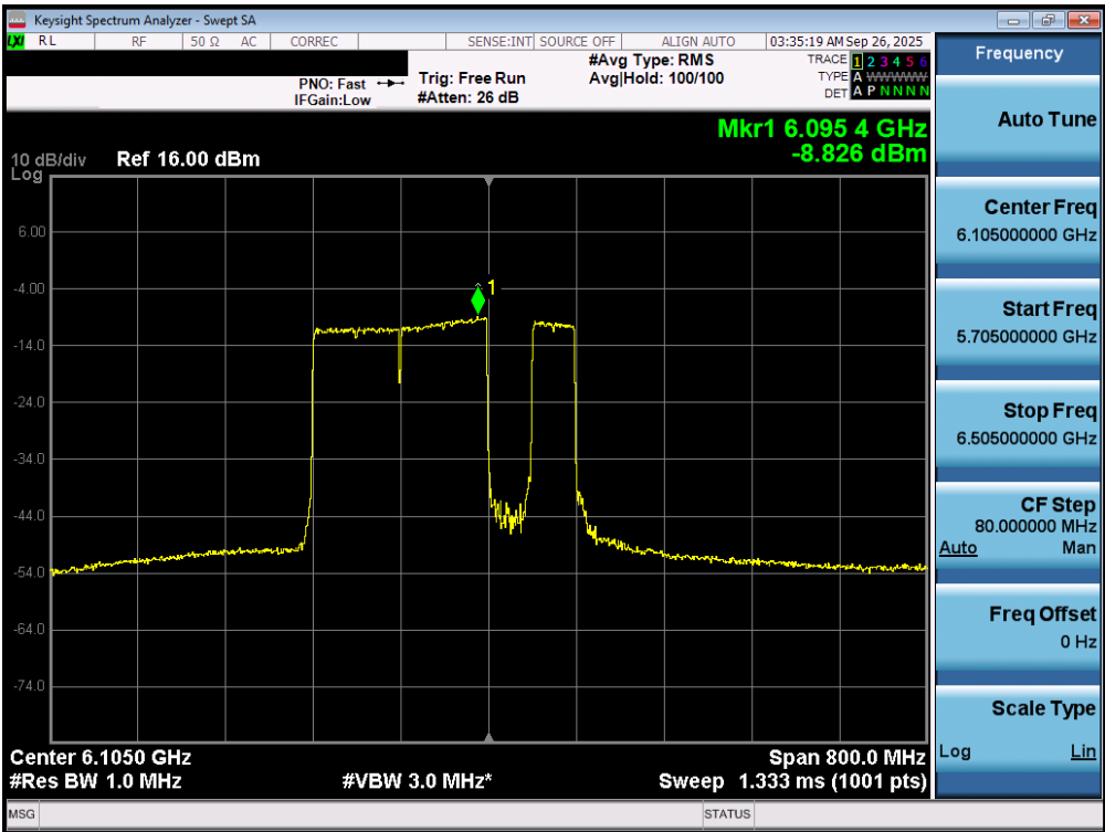
Plot 7-45. Power Spectral Density Plot MIMO ANT1 (320MHz 802.11be (UNII Band 5) – Ch. 31) – 120MHz Punctured – LPI
