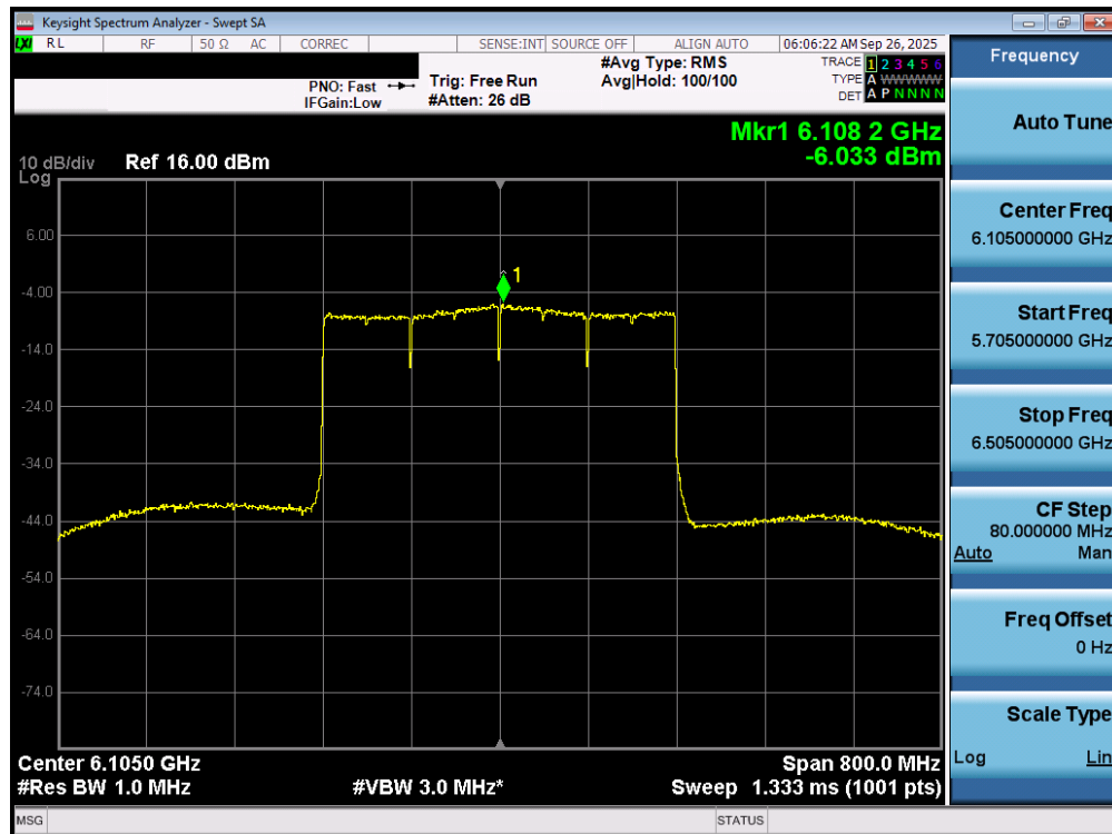
Plot 7-51. Power Spectral Density Plot MIMO ANT1 (320MHz 802.11be (UNII Band 5) – Ch. 31) - SP
