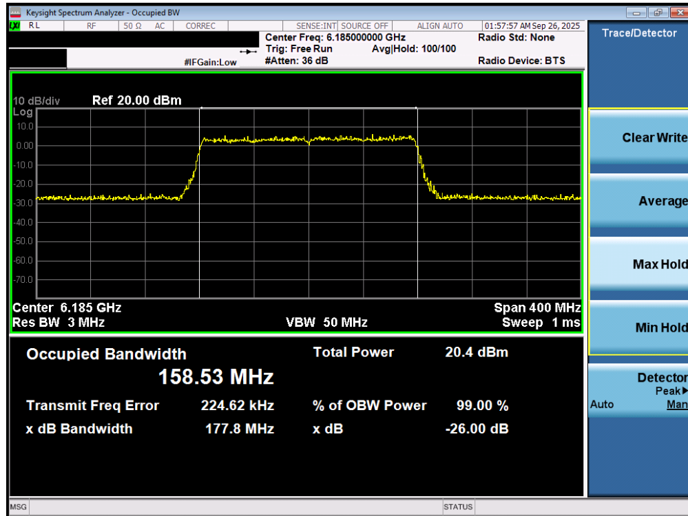
Plot 7-5. 26dB Bandwidth Plot MIMO ANT1 (160MHz 802.11ax/be (UNII Band 5) – Ch. 47) - LPI
