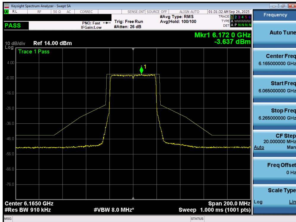
Plot 7-75. In Band Emissions Plot MIMO ANT1 (40MHz 802.11ax/be (UNII Band 5) – Ch. 43) - LPI
