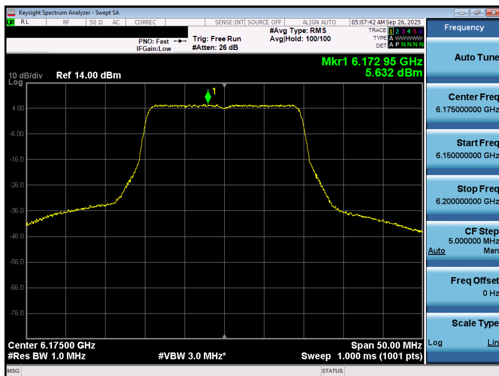
Plot 7-47. Power Spectral Density Plot MIMO ANT1 (20MHz 802.11ax/be (UNII Band 5) – Ch. 45) - SP
