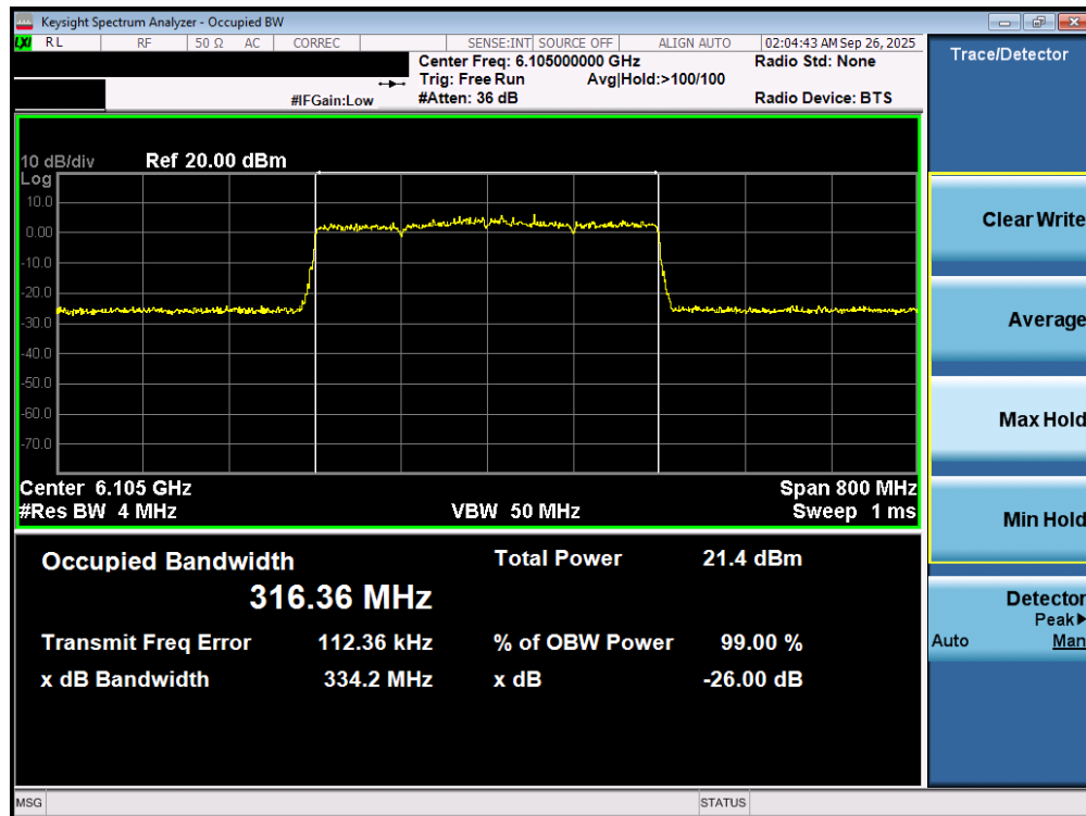
Plot 7-6. 26dB Bandwidth Plot MIMO ANT1 (320MHz 802.11be (UNII Band 5) – Ch. 31) - LPI
