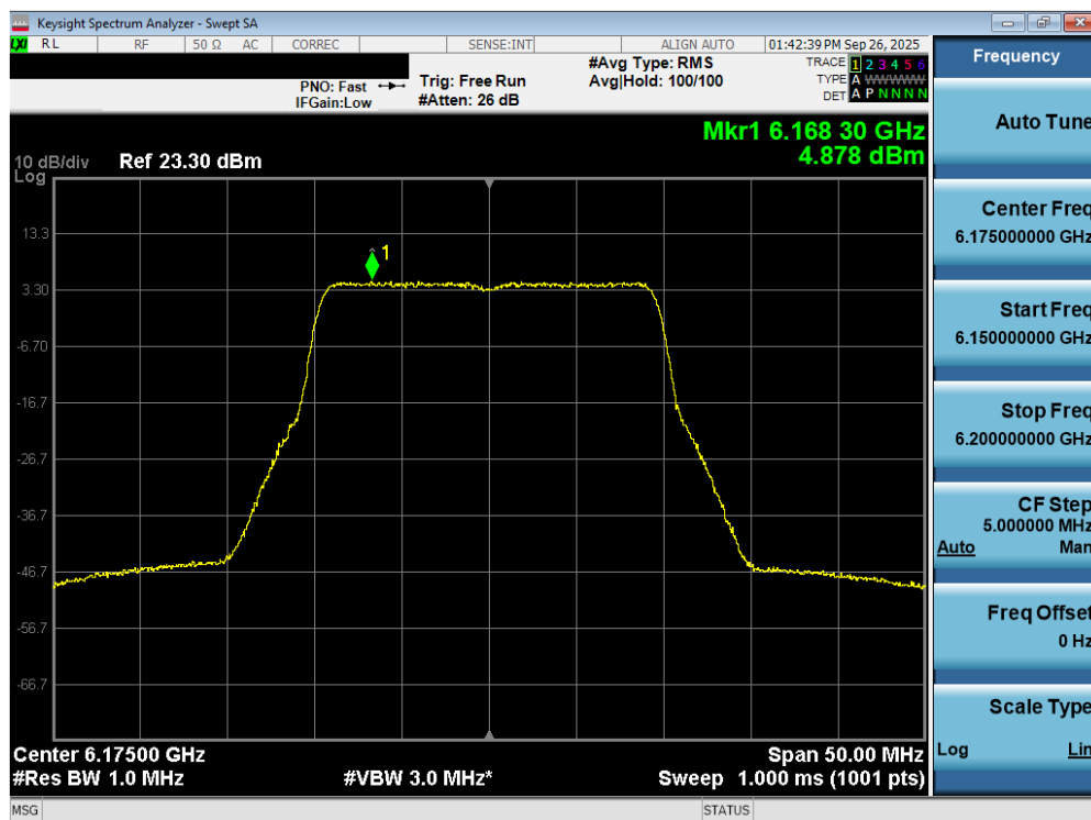
Plot 7-65. Power Spectral Density Plot MIMO ANT2 (20MHz 802.11ax/be (UNII Band 5) – Ch. 45) - SP
