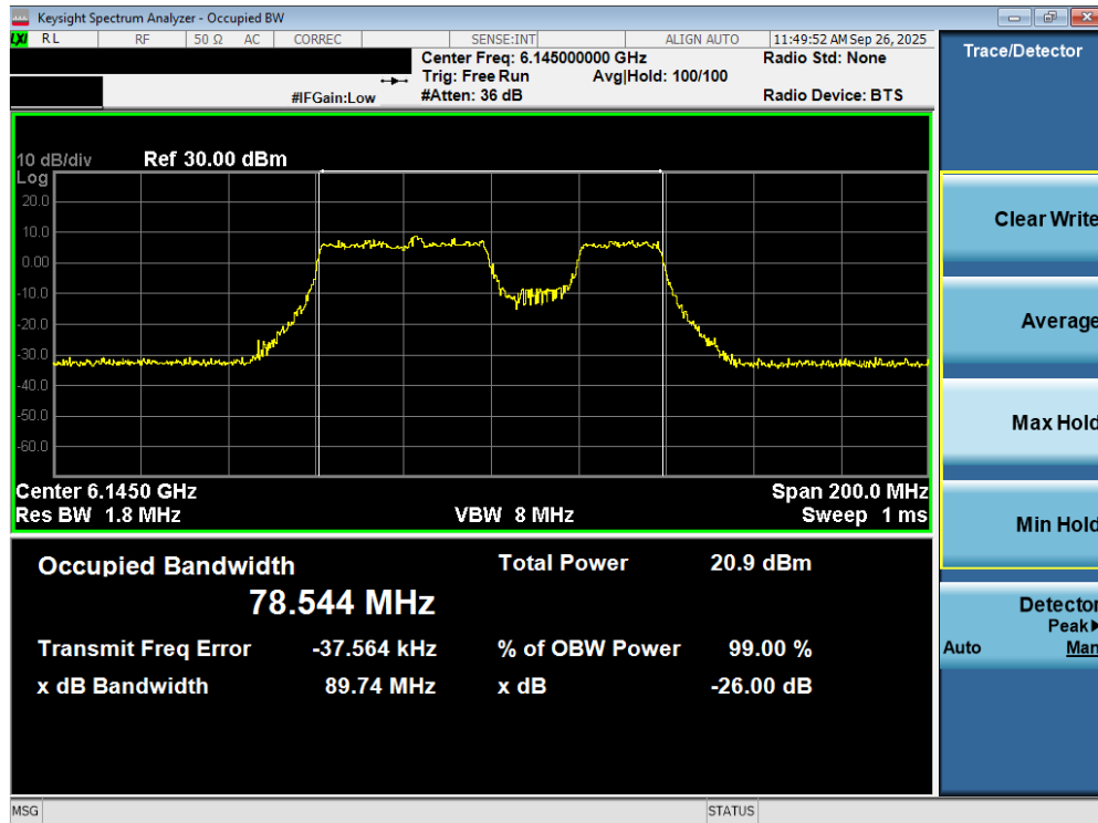
Plot 7-25. 26dB Bandwidth Plot MIMO ANT2 (80MHz 802.11be (UNII Band 5) – Ch. 39) – 20MHz Punctured - LPI
