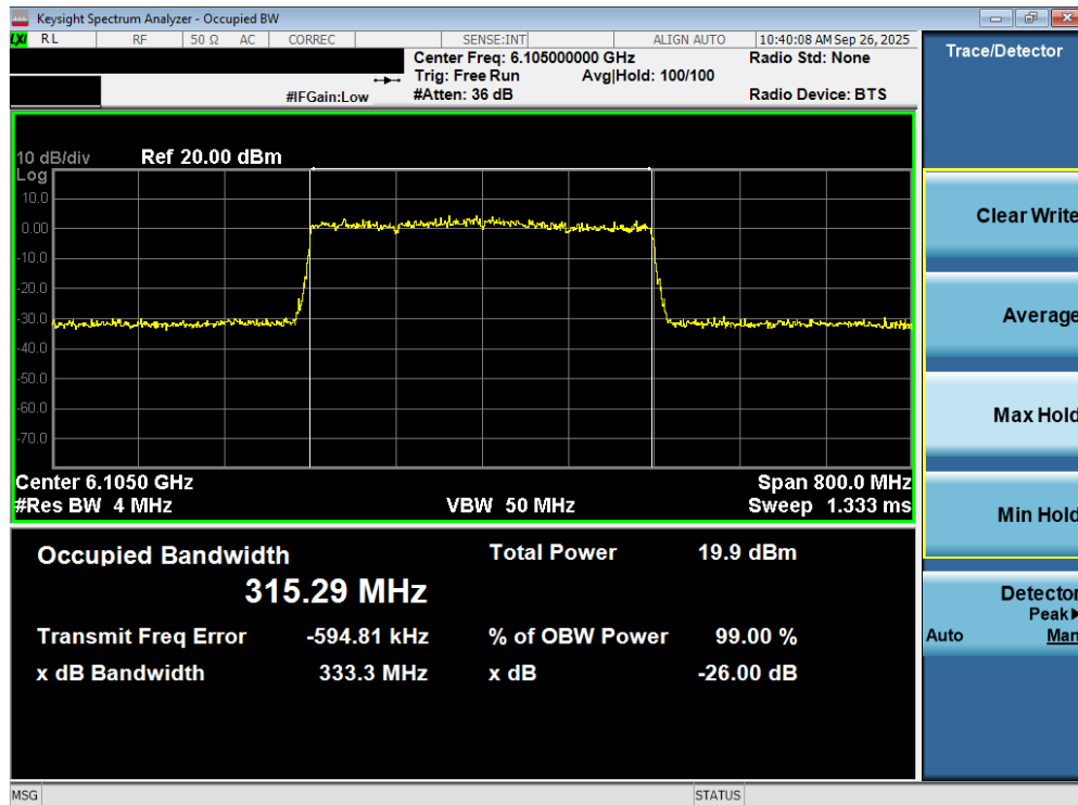
Plot 7-24. 26dB Bandwidth Plot MIMO ANT2 (320MHz 802.11be (UNII Band 5) – Ch. 31) – LPI
