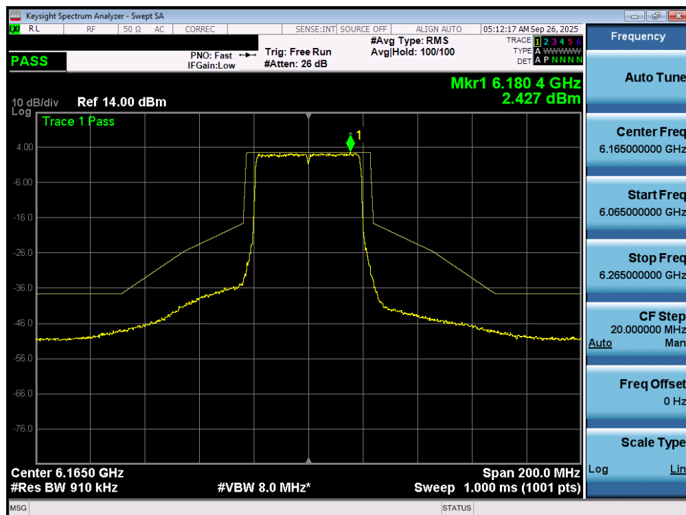
Plot 7-84. In Band Emissions Plot MIMO ANT1 (40MHz 802.11ax/be (UNII Band 5) – Ch. 43) - SP
