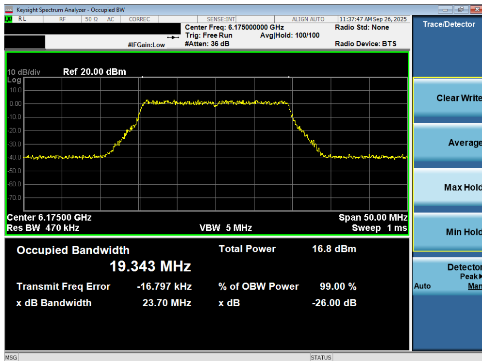
Plot 7-20. 26dB Bandwidth Plot MIMO ANT2 (20MHz 802.11ax/be (UNII Band 5) – Ch. 45) - LPI
