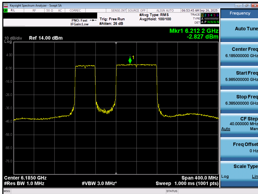
Plot 7-53. Power Spectral Density Plot MIMO ANT1 (160MHz 802.11be (UNII Band 5) – Ch. 47) – 40MHz Punctured - SP
