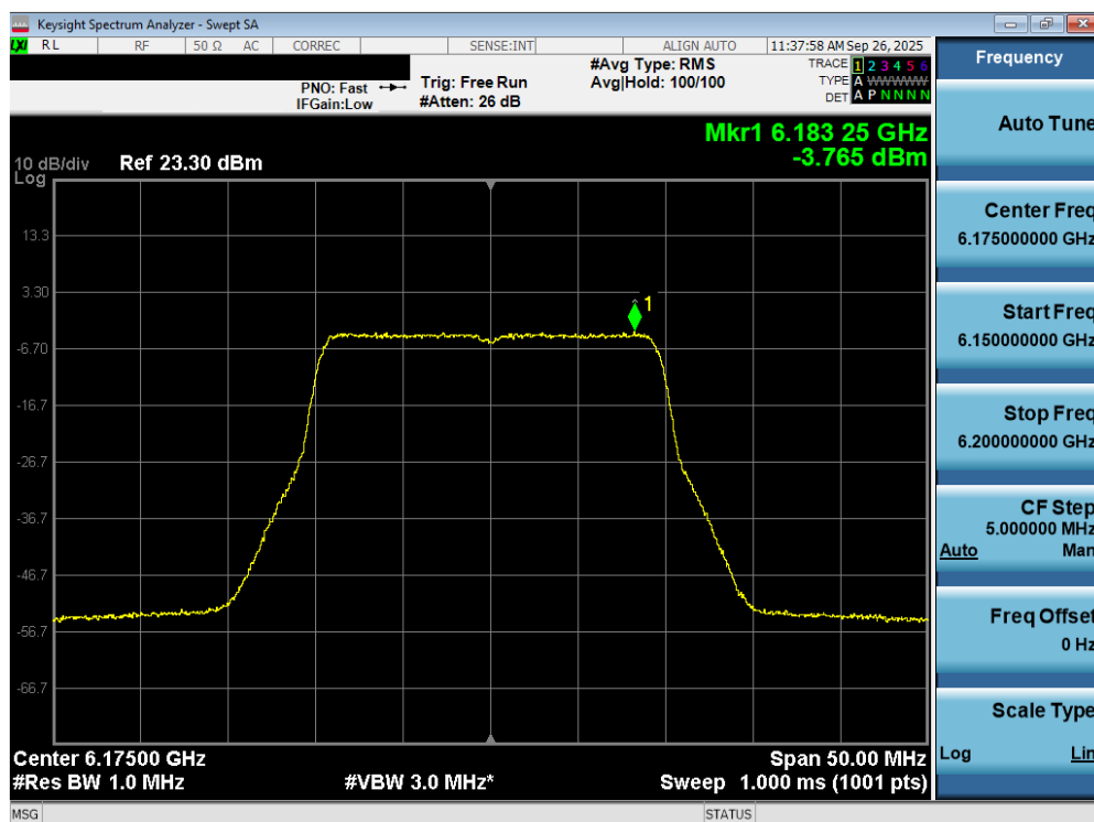
Plot 7-56. Power Spectral Density Plot MIMO ANT2 (20MHz 802.11ax/be (UNII Band 5) – Ch. 45) - LPI
