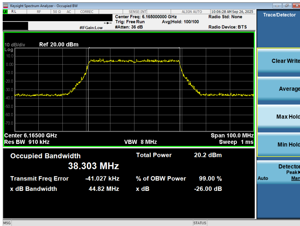
Plot 7-21. 26dB Bandwidth Plot MIMO ANT2 (40MHz 802.11ax/be (UNII Band 5) – Ch. 43) - LPI
