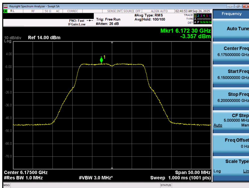
Plot 7-37. Power Spectral Density Plot MIMO ANT1 (20MHz 802.11a (UNII Band 5) – Ch. 45) - LPI
