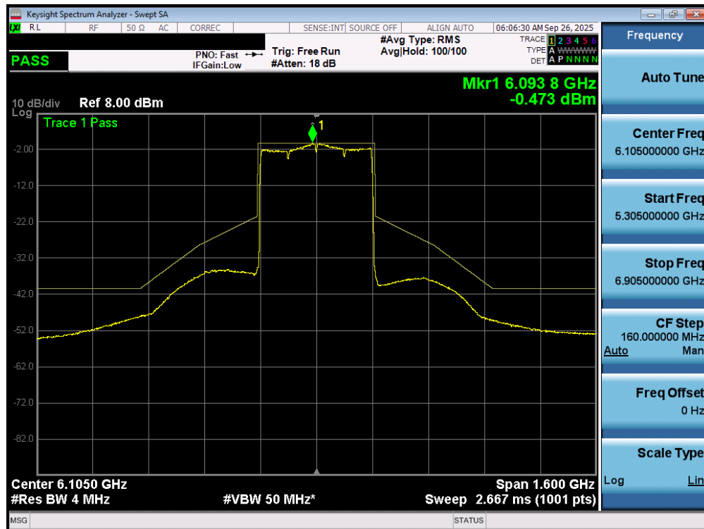
Plot 7-87. In Band Emissions Plot MIMO ANT1 (320MHz 802.11be (UNII Band 5) – Ch. 31) - SP
