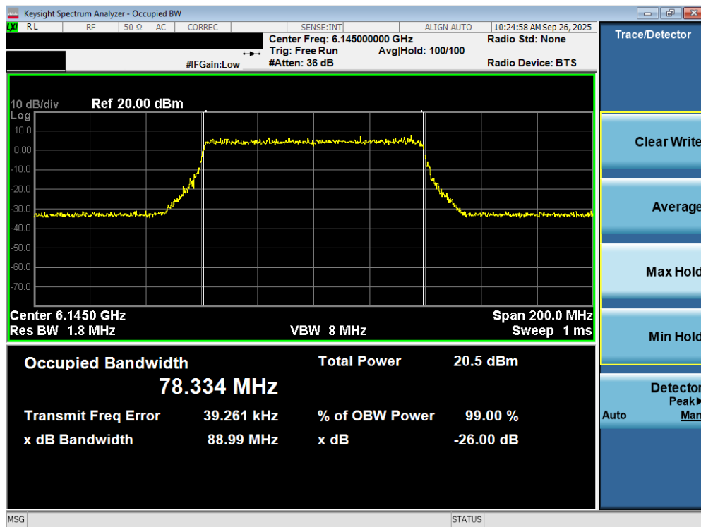
Plot 7-22. 26dB Bandwidth Plot MIMO ANT2 (80MHz 802.11ax/be (UNII Band 5) – Ch. 39) - LPI
