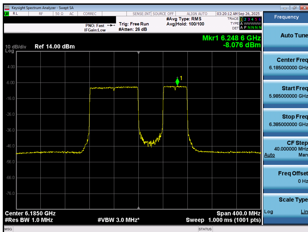
Plot 7-44. Power Spectral Density Plot MIMO ANT1 (160MHz 802.11be (UNII Band 5) – Ch. 47) – 40MHz Punctured - LPI
