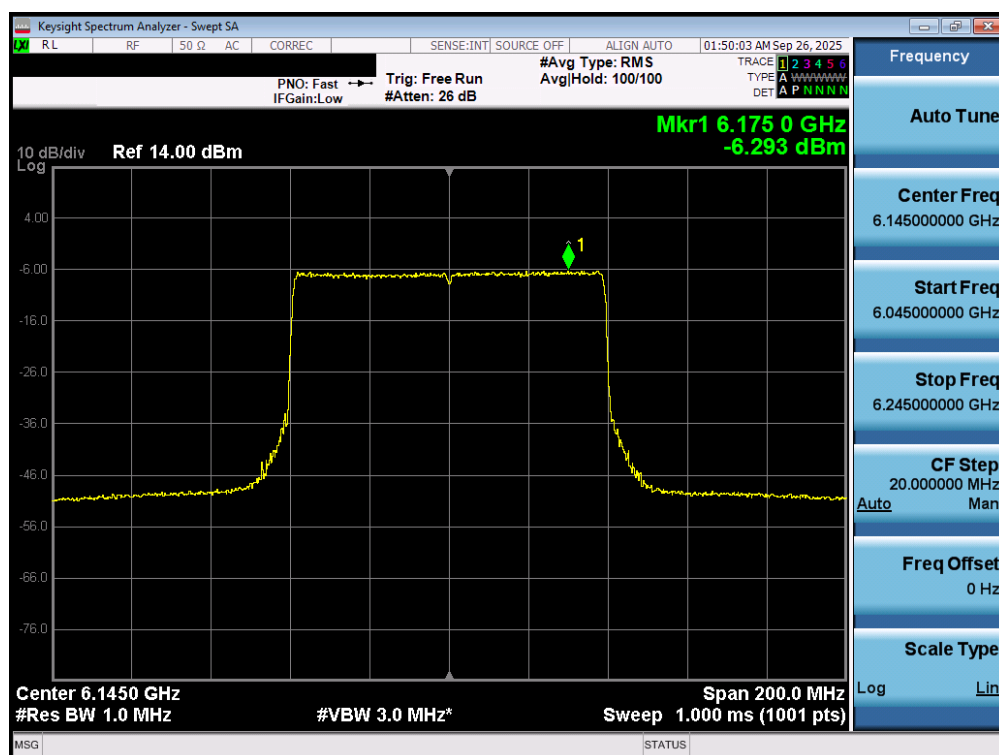
Plot 7-40. Power Spectral Density Plot MIMO ANT1 (80MHz 802.11ax/be (UNII Band 5) – Ch. 39) - LPI
