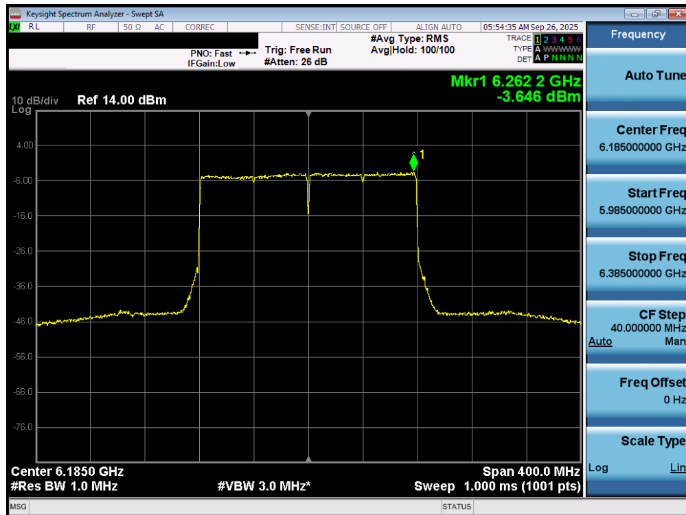
Plot 7-50. Power Spectral Density Plot MIMO ANT1 (160MHz 802.11ax/be (UNII Band 5) – Ch. 47) - SP
