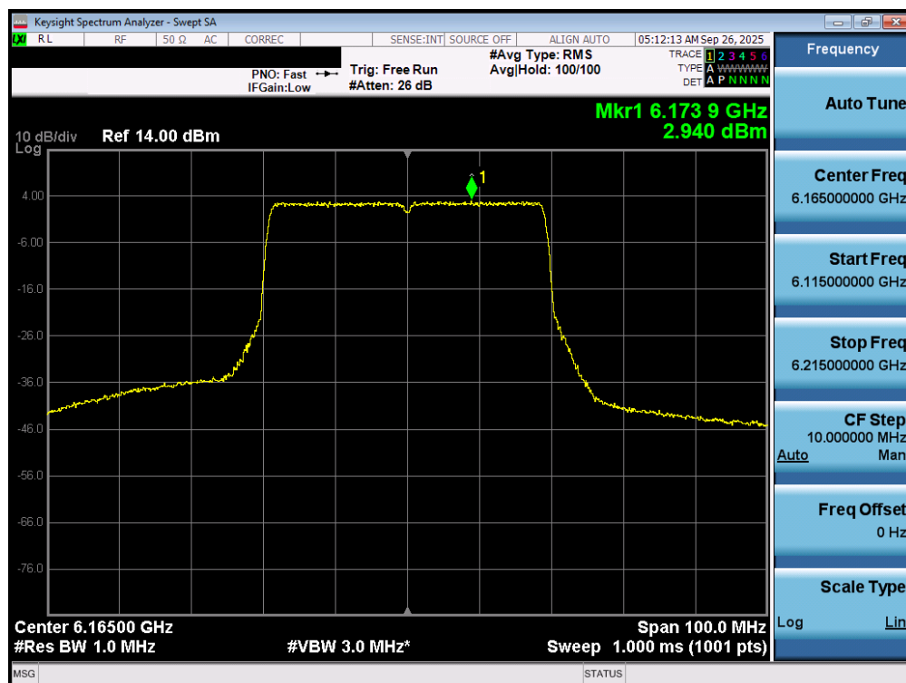
Plot 7-48. Power Spectral Density Plot MIMO ANT1 (40MHz 802.11ax/be (UNII Band 5) – Ch. 43) – SP
