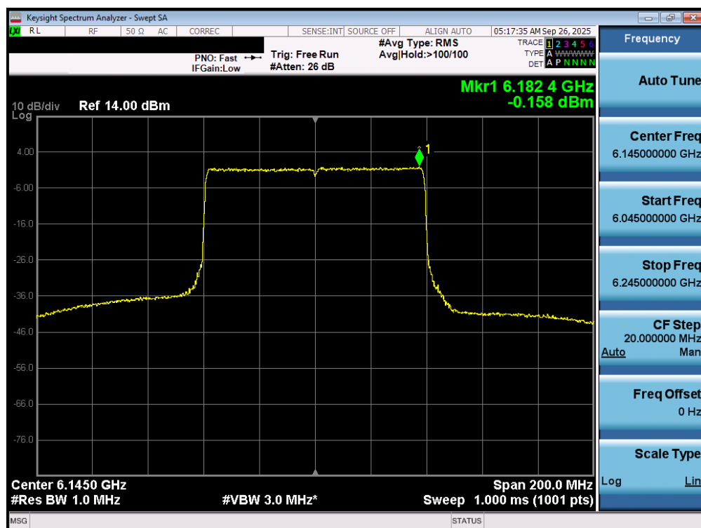
Plot 7-49. Power Spectral Density Plot MIMO ANT1 (80MHz 802.11ax/be (UNII Band 5) – Ch. 39) – SP
