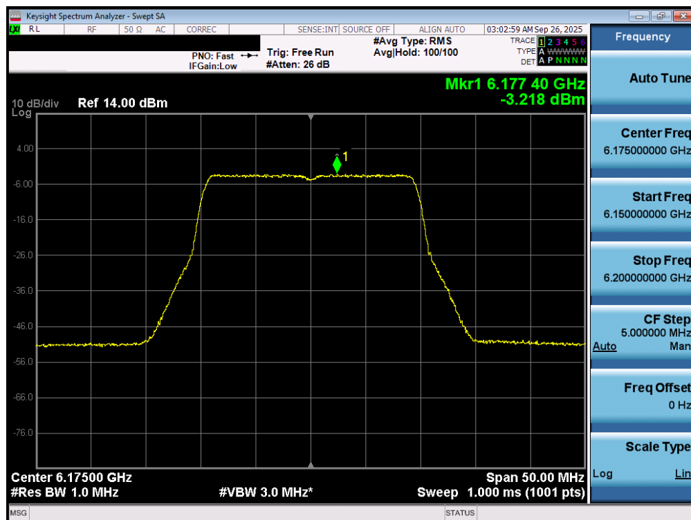
Plot 7-38. Power Spectral Density Plot MIMO ANT1 (20MHz 802.11ax/be (UNII Band 5) – Ch. 45) - LPI
