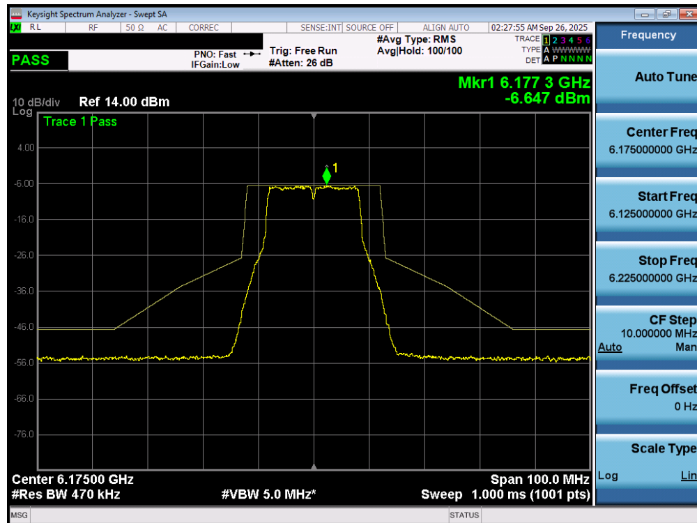
Plot 7-73. In Band Emissions Plot MIMO ANT1 (20MHz 802.11a (UNII Band 5) – Ch. 45) - LPI
