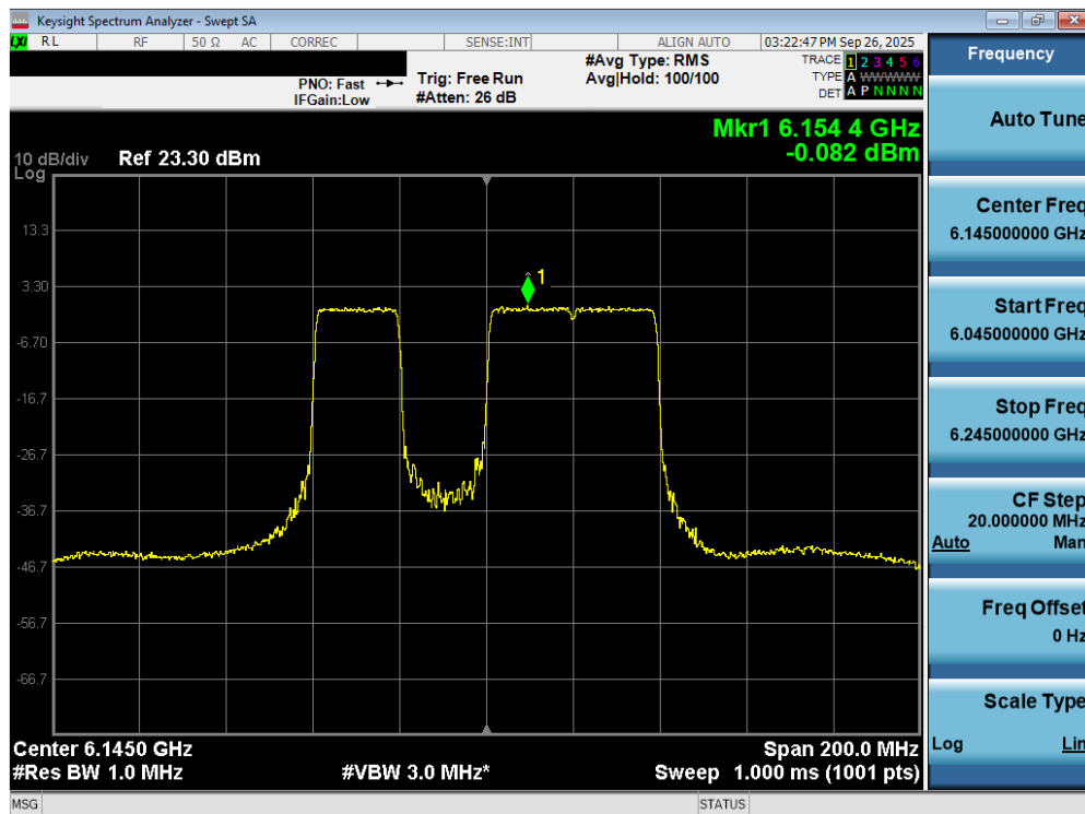
Plot 7-70. Power Spectral Density Plot MIMO ANT2 (80MHz 802.11be (UNII Band 5) – Ch. 39) – 20MHz Punctured - SP
