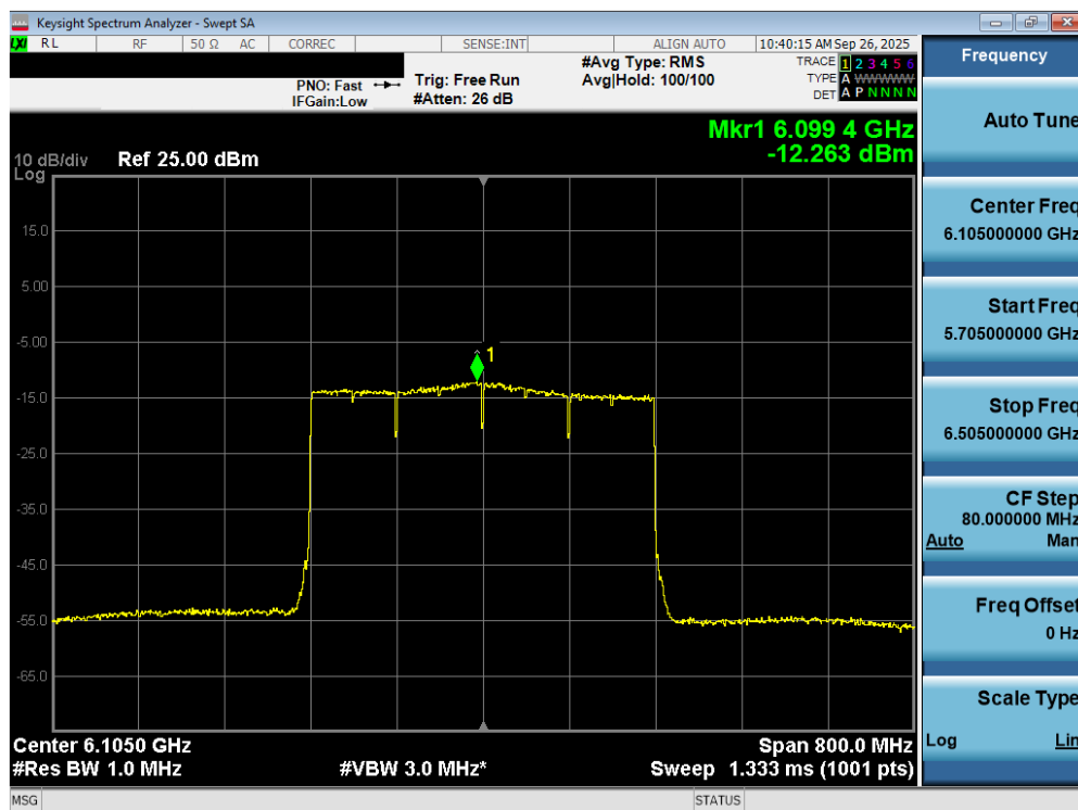
Plot 7-60. Power Spectral Density Plot MIMO ANT2 (320MHz 802.11be (UNII Band 5) – Ch. 31) - LPI
