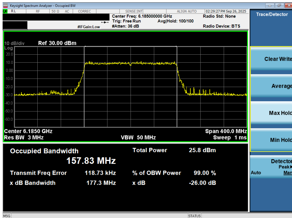
Plot 7-32. 26dB Bandwidth Plot MIMO ANT2 (160MHz 802.11ax/be (UNII Band 5) – Ch. 47) - SP
