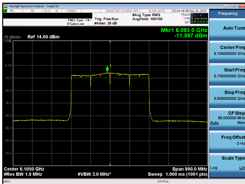
Plot 7-42. Power Spectral Density Plot MIMO ANT1 (320MHz 802.11be (UNII Band 5) – Ch. 31) - LPI
