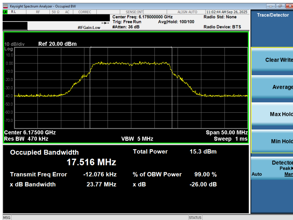
Plot 7-19. 26dB Bandwidth Plot MIMO ANT2 (20MHz 802.11a (UNII Band 5) – Ch. 45) - LPI
