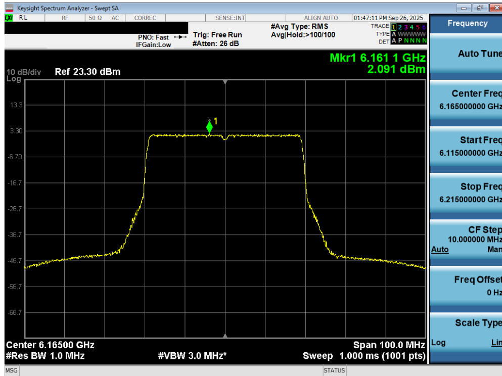
Plot 7-66. Power Spectral Density Plot MIMO ANT2 (40MHz 802.11ax/be (UNII Band 5) – Ch. 43) - SP
