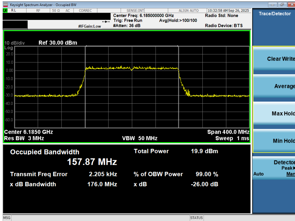
Plot 7-23. 26dB Bandwidth Plot MIMO ANT2 (160MHz 802.11ax/be (UNII Band 5) – Ch. 47) – LPI
