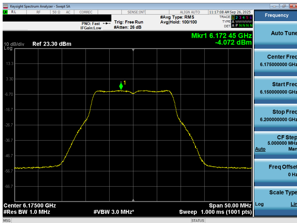
Plot 7-55. Power Spectral Density Plot MIMO ANT2 (20MHz 802.11a (UNII Band 5) – Ch. 45) - LPI
