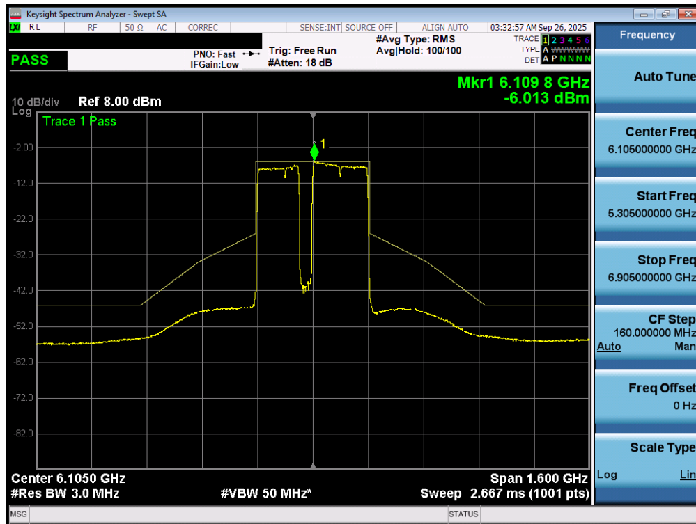
Plot 7-81. In Band Emissions Plot MIMO ANT1 (320MHz 802.11be (UNII Band 5) – Ch. 31) – 40MHz Punctured – LPI
