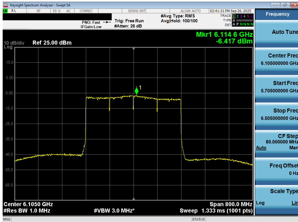
Plot 7-69. Power Spectral Density Plot MIMO ANT2 (320MHz 802.11be (UNII Band 5) – Ch. 31) - SP
