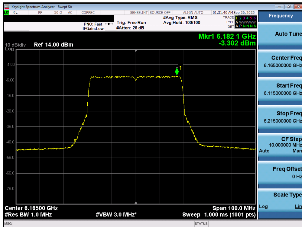
Plot 7-39. Power Spectral Density Plot MIMO ANT1 (40MHz 802.11ax/be (UNII Band 5) – Ch. 43) - LPI
