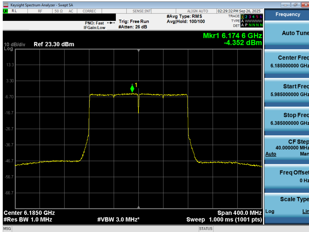
Plot 7-68. Power Spectral Density Plot MIMO ANT2 (160MHz 802.11ax/be (UNII Band 5) – Ch. 47) - SP
