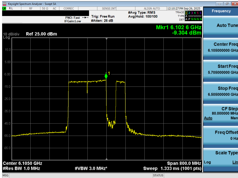
Plot 7-63. Power Spectral Density Plot MIMO ANT2 (320MHz 802.11be (UNII Band 5) – Ch. 31) – 120MHz Punctured – LPI
