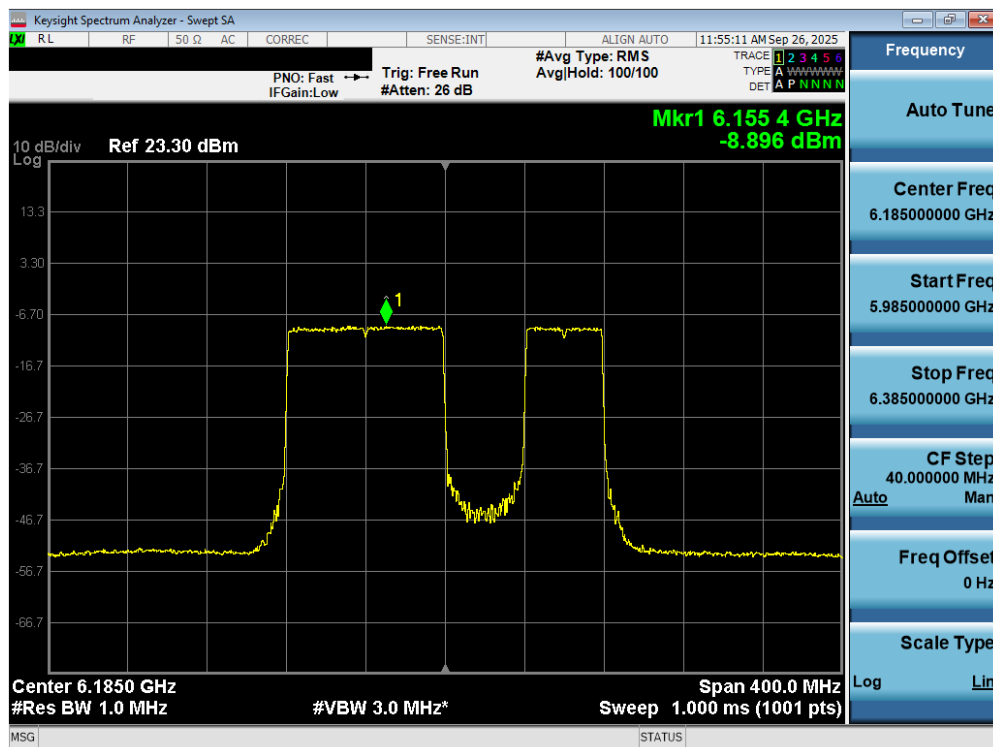
Plot 7-62. Power Spectral Density Plot MIMO ANT2 (160MHz 802.11be (UNII Band 5) – Ch. 47) – 40MHz Punctured - LPI
