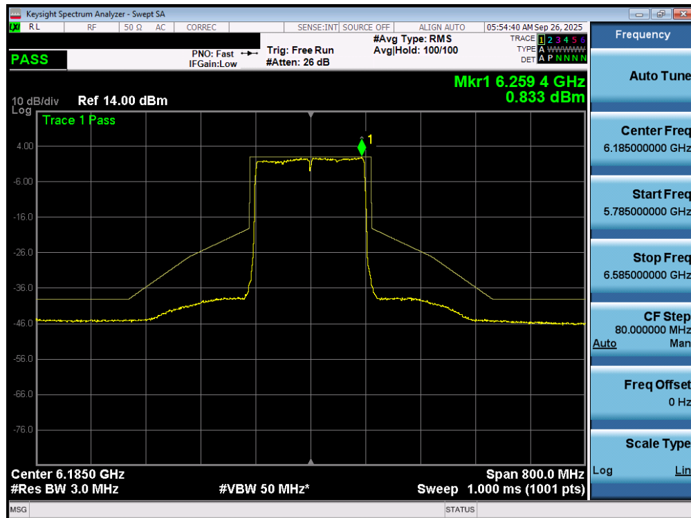
Plot 7-86. In Band Emissions Plot MIMO ANT1 (160MHz 802.11ax/be (UNII Band 5) – Ch. 47) - SP
