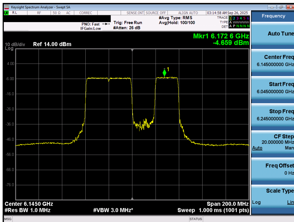
Plot 7-43. Power Spectral Density Plot MIMO ANT1 (80MHz 802.11be (UNII Band 5) – Ch. 39) – 20MHz Punctured - LPI
