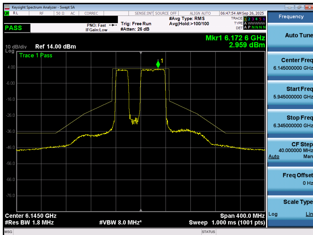
Plot 7-88. In Band Emissions Plot MIMO ANT1 (80MHz 802.11be (UNII Band 5) – Ch. 39) – 20MHz Punctured - SP
