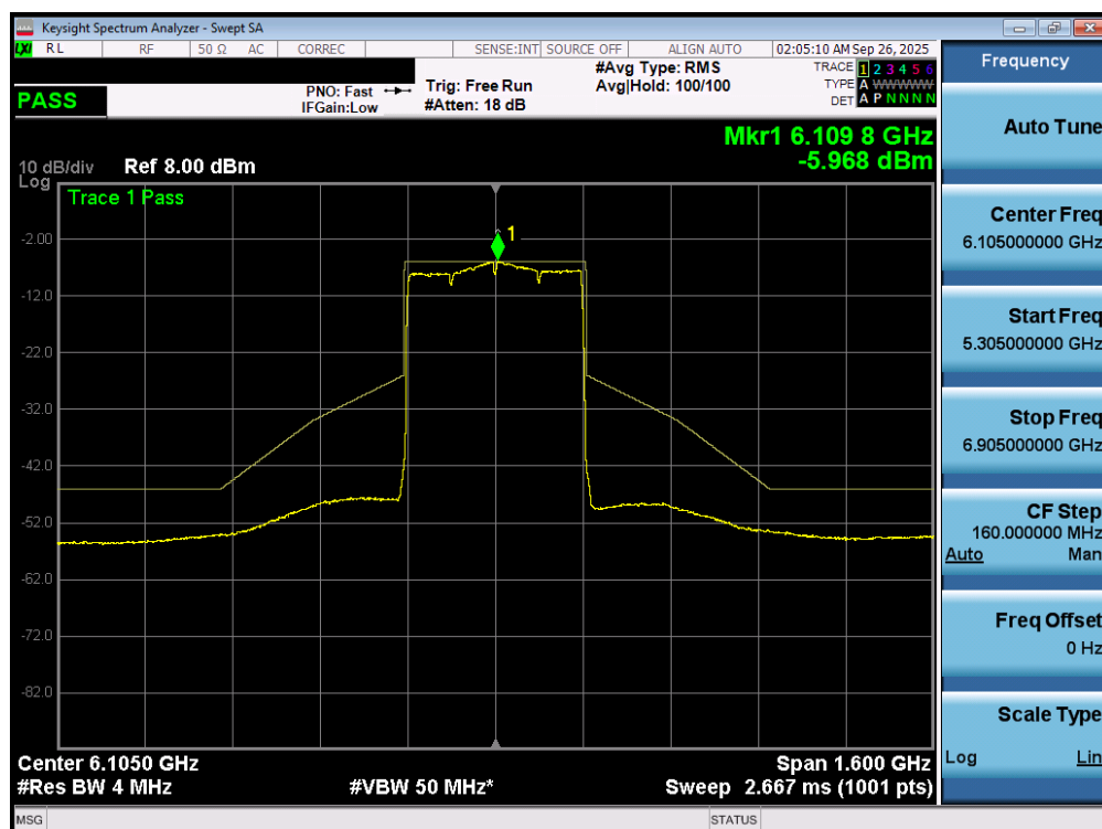
Plot 7-78. In Band Emissions Plot MIMO ANT1 (320MHz 802.11be (UNII Band 5) – Ch. 31) - LPI
