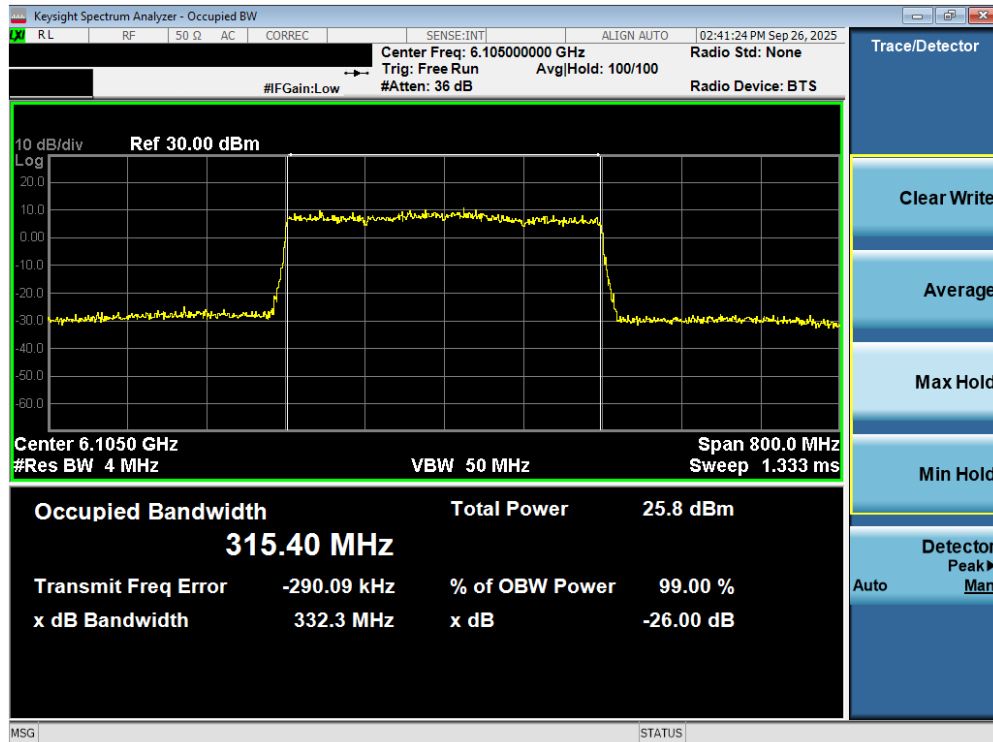
Plot 7-33. 26dB Bandwidth Plot MIMO ANT2 (320MHz 802.11be (UNII Band 5) – Ch. 31) - SP
