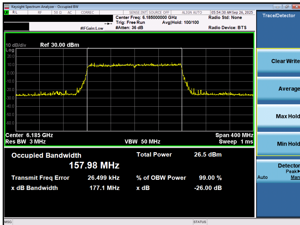
Plot 7-14. 26dB Bandwidth Plot MIMO ANT1 (160MHz 802.11ax/be (UNII Band 5) – Ch. 47) – SP
