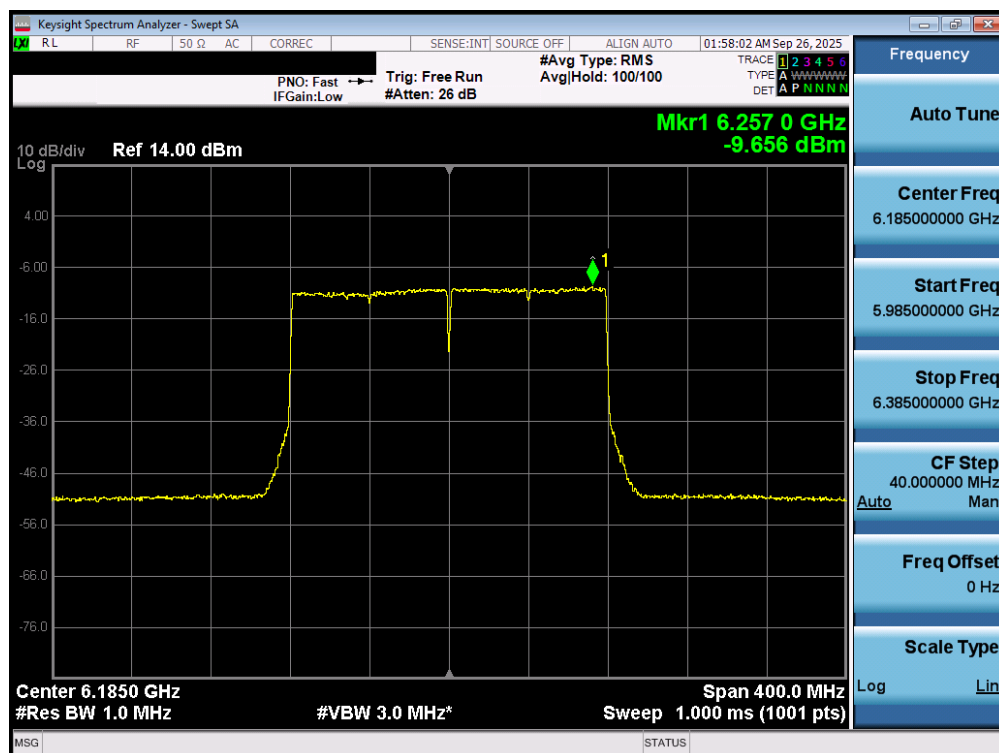
Plot 7-41. Power Spectral Density Plot MIMO ANT1 (160MHz 802.11ax/be (UNII Band 5) – Ch. 47) - LPI
