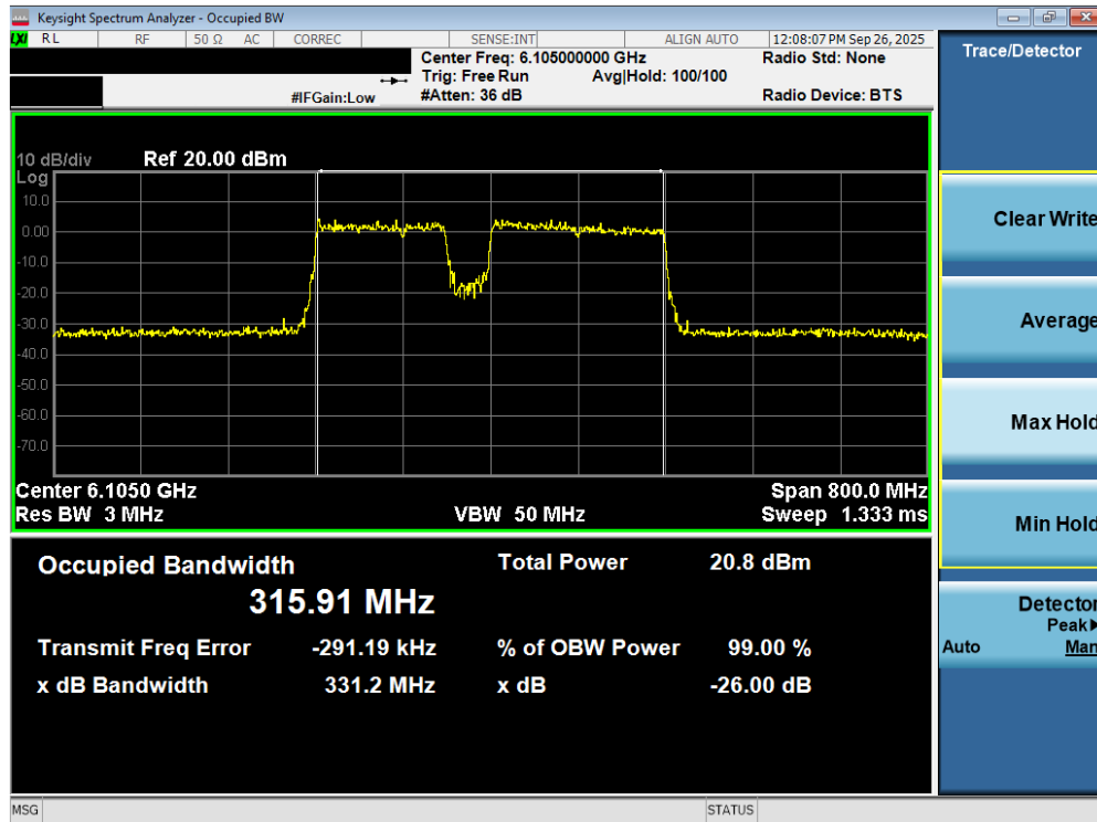
Plot 7-27. 26dB Bandwidth Plot MIMO ANT2 (320MHz 802.11be (UNII Band 5) – Ch. 31) – 40MHz Punctured – LPI
