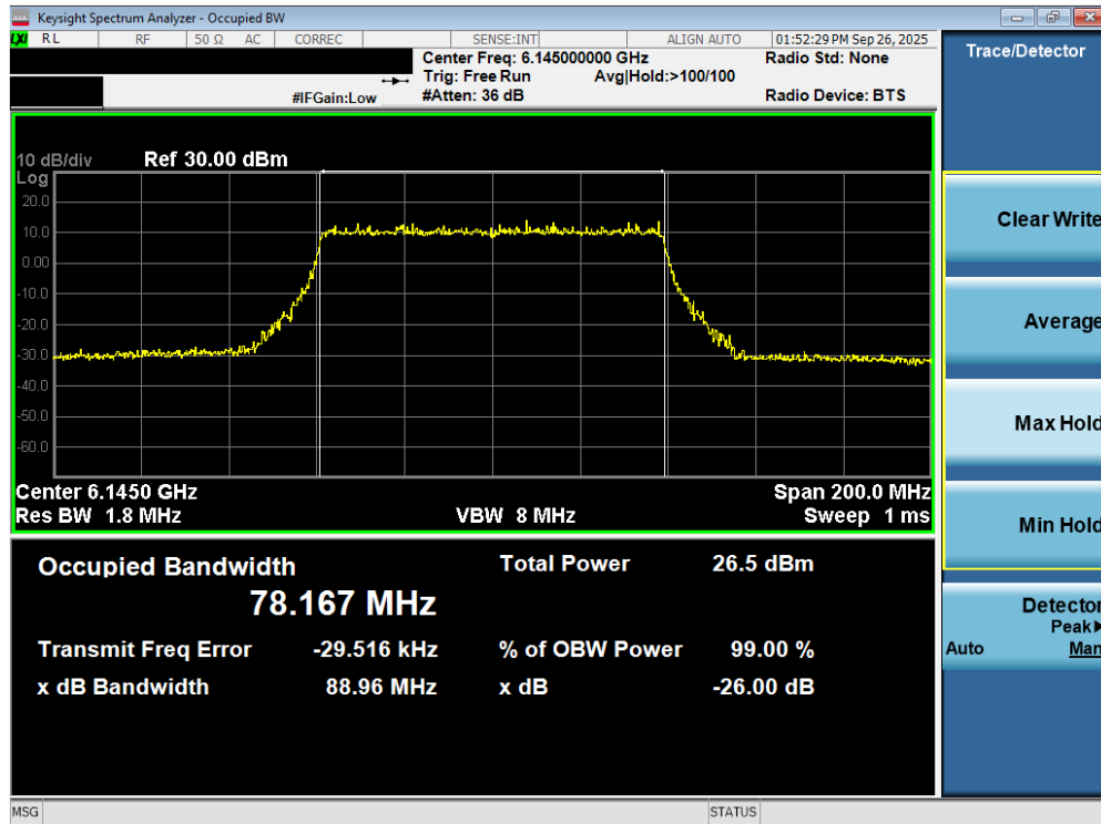
Plot 7-31. 26dB Bandwidth Plot MIMO ANT2 (80MHz 802.11ax/be (UNII Band 5) – Ch. 39) - SP
