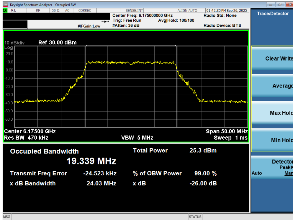
Plot 7-29. 26dB Bandwidth Plot MIMO ANT2 (20MHz 802.11ax/be (UNII Band 5) – Ch. 45) - SP
