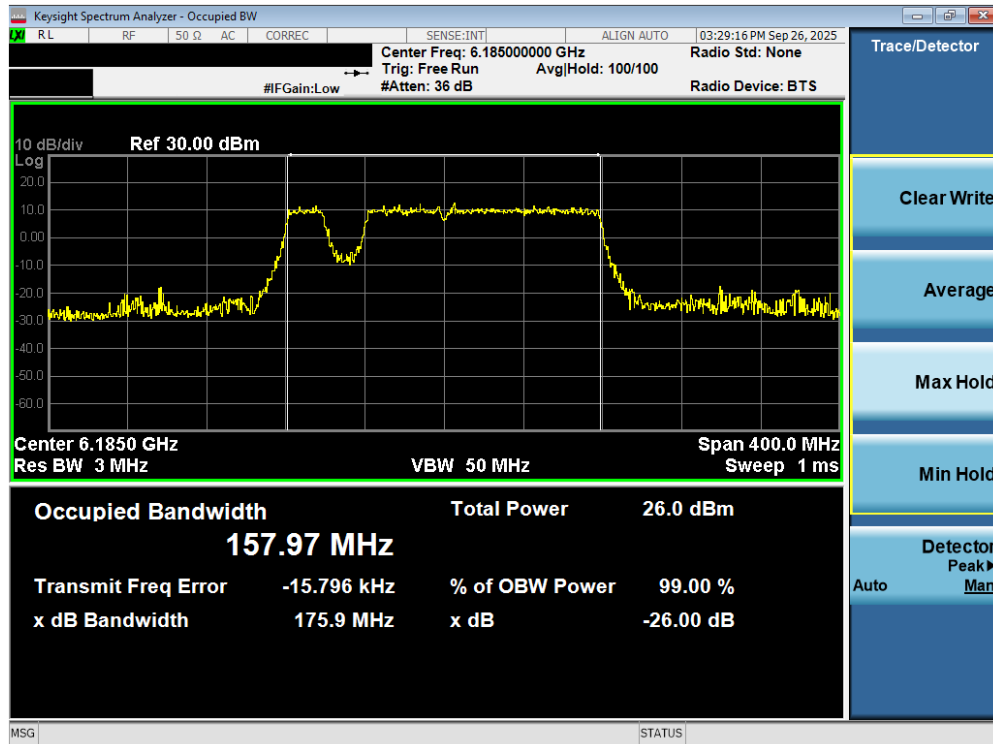
Plot 7-35. 26dB Bandwidth Plot MIMO ANT2 (160MHz 802.11be (UNII Band 5) – Ch. 47) – 20MHz Punctured - SP
