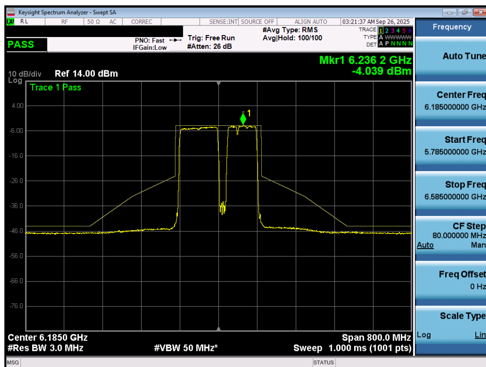
Plot 7-80. In Band Emissions Plot MIMO ANT1 (160MHz 802.11be (UNII Band 5) – Ch. 47) – 20MHz Punctured - LPI
