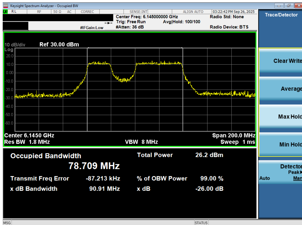
Plot 7-34. 26dB Bandwidth Plot MIMO ANT2 (80MHz 802.11be (UNII Band 5) – Ch. 39) – 20MHz Punctured - SP
