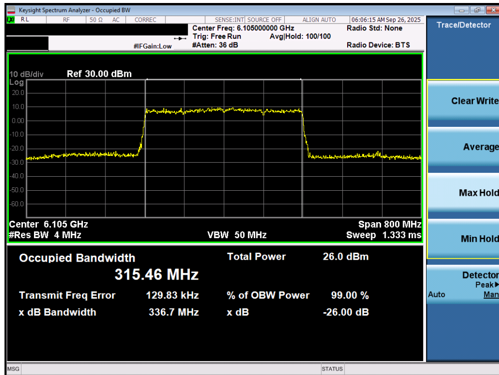
Plot 7-15. 26dB Bandwidth Plot MIMO ANT1 (320MHz 802.11be (UNII Band 5) – Ch. 31) – SP
