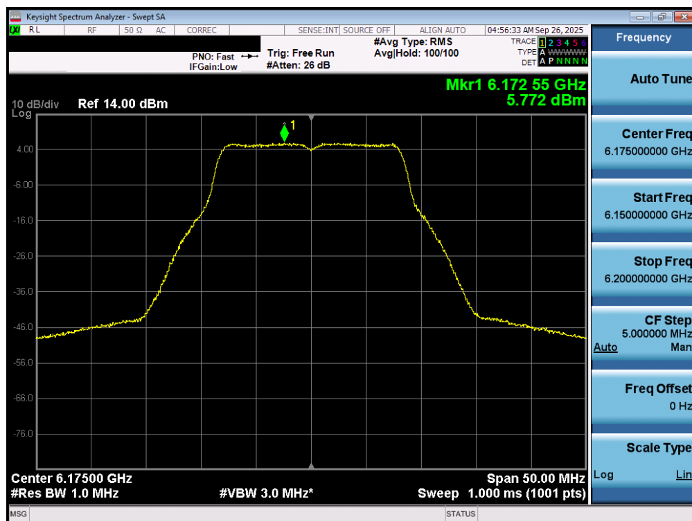
Plot 7-46. Power Spectral Density Plot MIMO ANT1 (20MHz 802.11a (UNII Band 5) – Ch. 45) - SP
