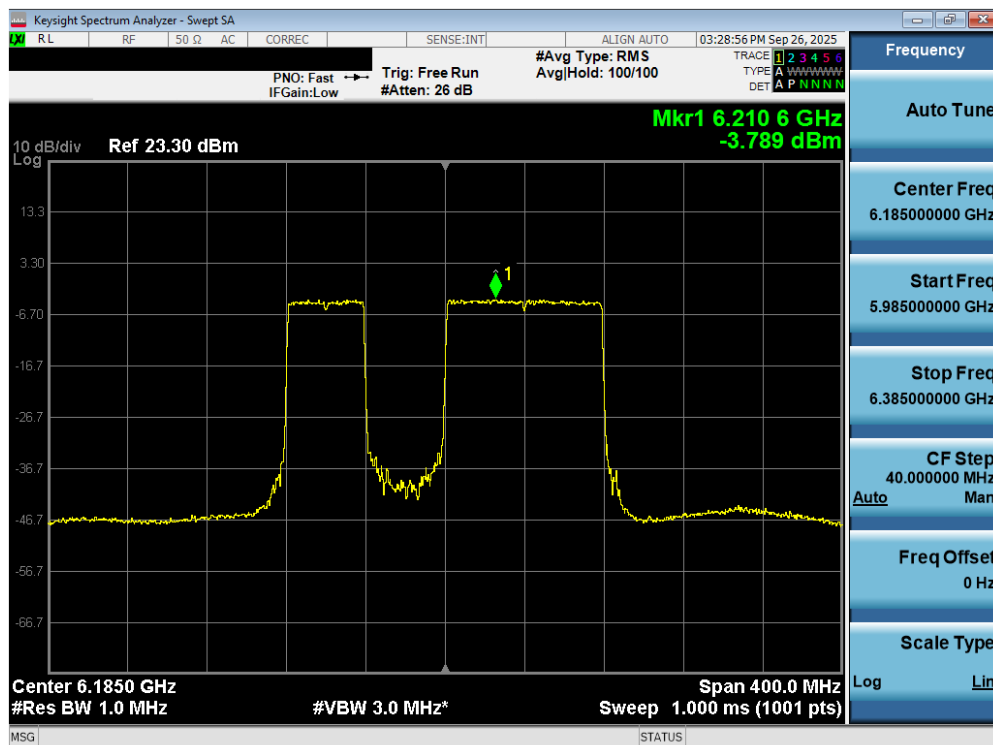
Plot 7-71. Power Spectral Density Plot MIMO ANT2 (160MHz 802.11be (UNII Band 5) – Ch. 47) – 40MHz Punctured - SP
