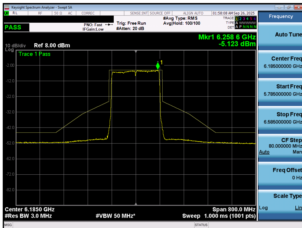
Plot 7-77. In Band Emissions Plot MIMO ANT1 (160MHz 802.11ax/be (UNII Band 5) – Ch. 47) - LPI
