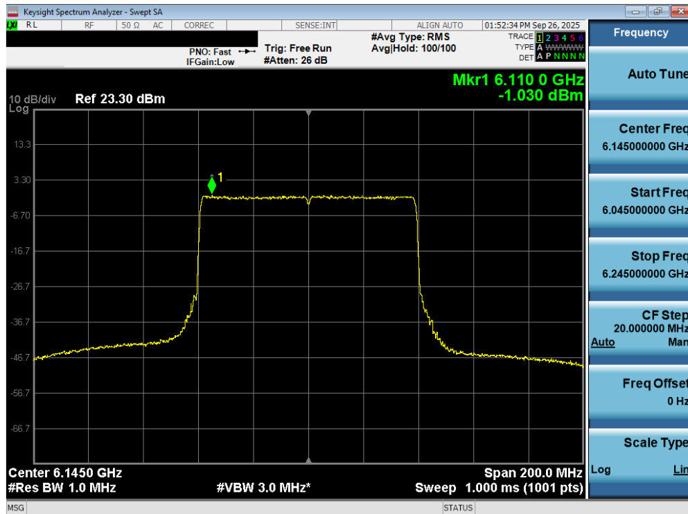
Plot 7-67. Power Spectral Density Plot MIMO ANT2 (80MHz 802.11ax/be (UNII Band 5) – Ch. 39) - SP
