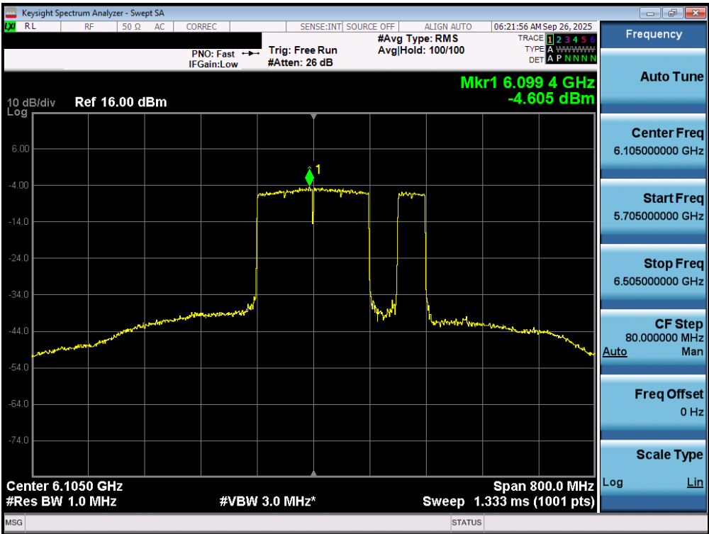
Plot 7-54. Power Spectral Density Plot MIMO ANT1 (320MHz 802.11be (UNII Band 5) – Ch. 31) – 120MHz Punctured – SP
