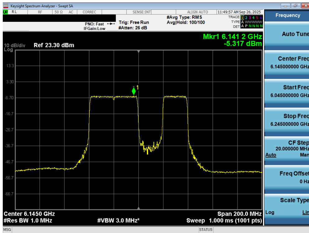
Plot 7-61. Power Spectral Density Plot MIMO ANT2 (80MHz 802.11be (UNII Band 5) – Ch. 39) – 20MHz Punctured - LPI
