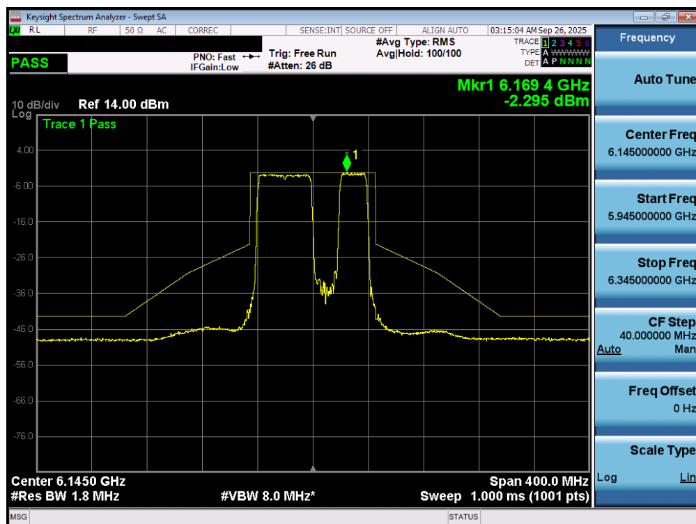
Plot 7-79. In Band Emissions Plot MIMO ANT1 (80MHz 802.11be (UNII Band 5) – Ch. 39) – 20MHz Punctured - LPI
