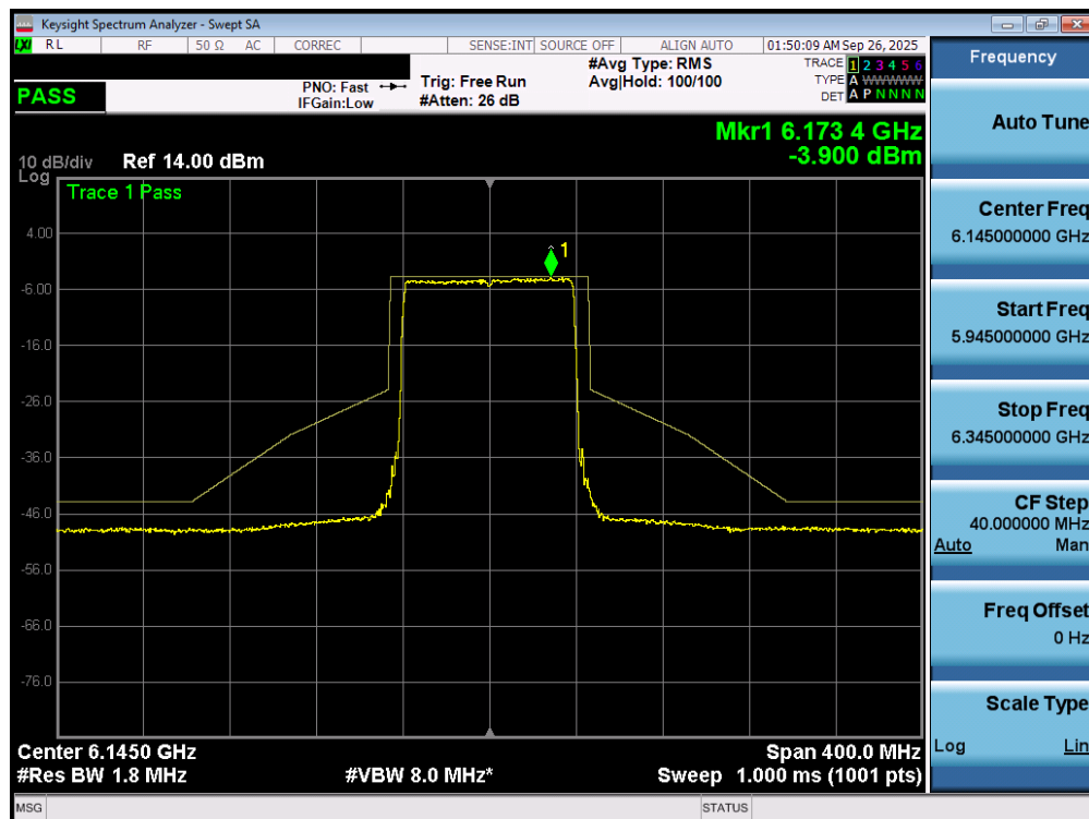
Plot 7-76. In Band Emissions Plot MIMO ANT1 (80MHz 802.11ax/be (UNII Band 5) – Ch. 39) - LPI/SP
