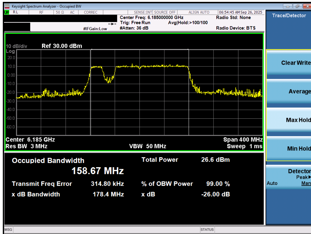
Plot 7-17. 26dB Bandwidth Plot MIMO ANT1 (160MHz 802.11be (UNII Band 5) – Ch. 47) – 20MHz Punctured – SP
