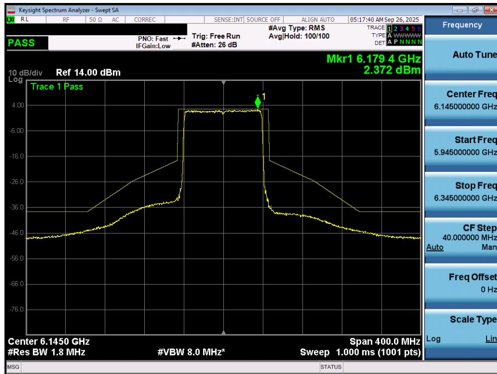
Plot 7-85. In Band Emissions Plot MIMO ANT1 (80MHz 802.11ax/be (UNII Band 5) – Ch. 39) – SP/SP
