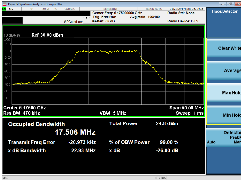
Plot 7-28. 26dB Bandwidth Plot MIMO ANT2 (20MHz 802.11a (UNII Band 5) – Ch. 45) - SP
