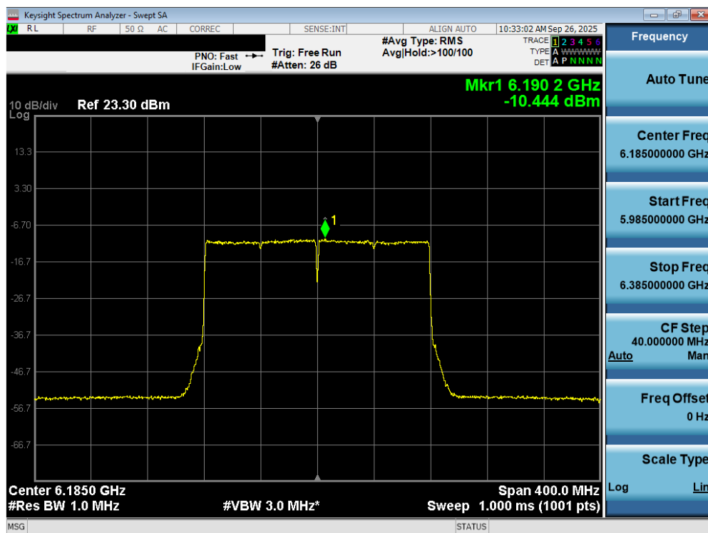
Plot 7-59. Power Spectral Density Plot MIMO ANT2 (160MHz 802.11ax/be (UNII Band 5) – Ch. 47) - LPI
