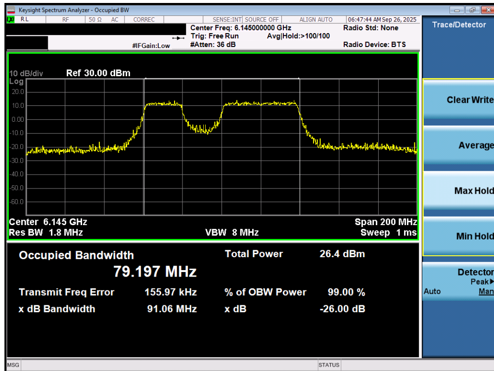
Plot 7-16. 26dB Bandwidth Plot MIMO ANT1 (80MHz 802.11be (UNII Band 5) – Ch. 39) – 20MHz Punctured - SP
