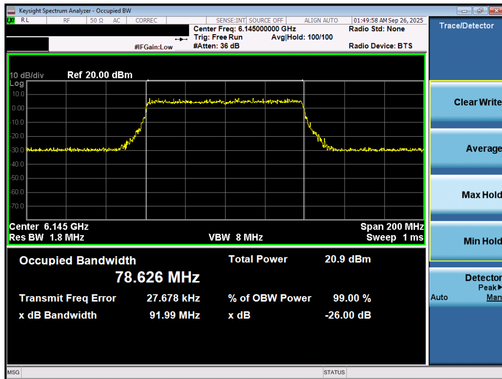
Plot 7-4. 26dB Bandwidth Plot MIMO ANT1 (80MHz 802.11ax/be (UNII Band 5) – Ch. 39) - LPI
