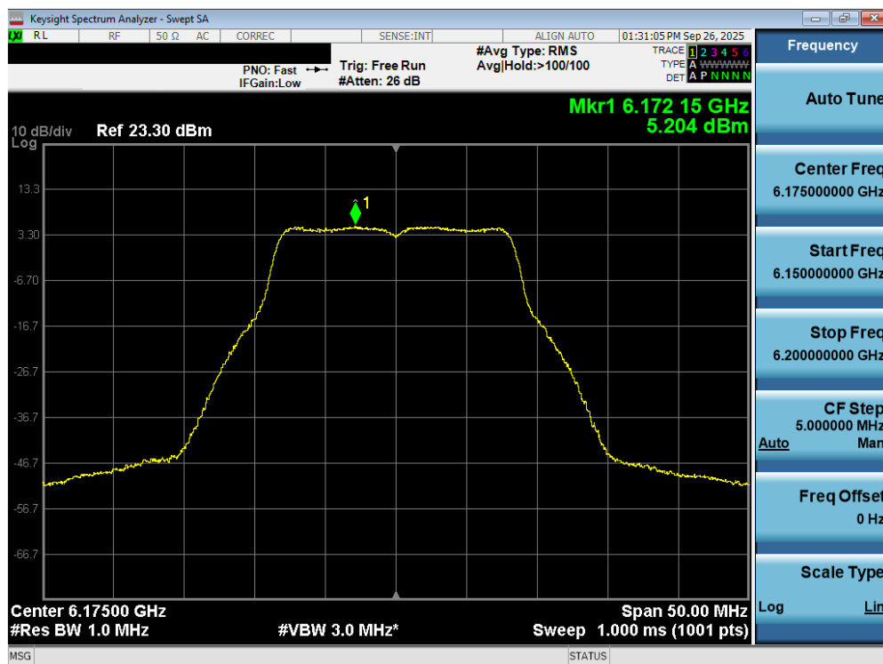
Plot 7-64. Power Spectral Density Plot MIMO ANT2 (20MHz 802.11a (UNII Band 5) – Ch. 45) - SP
