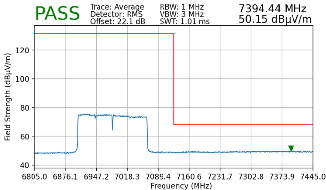
Plot 7-102. Radiated Upper Band Edge Plot MIMO (Average – UNII Band 8)
