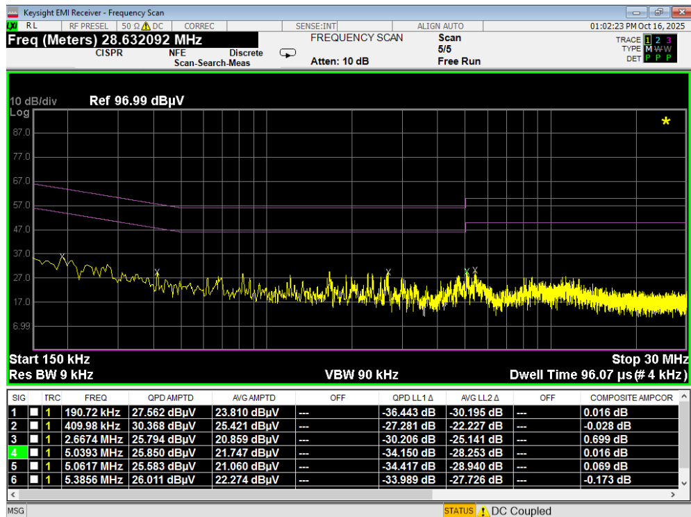
Plot 7-121. Line Conducted Plot with 802.11a UNII Band 7 (N)
