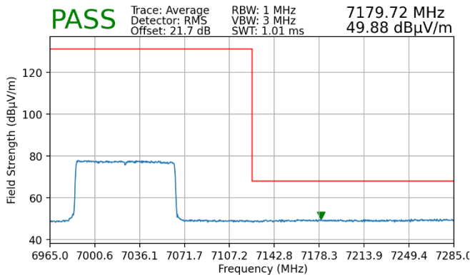
Plot 7-94. Radiated Upper Band Edge Plot MIMO (Average – UNII Band 8)
