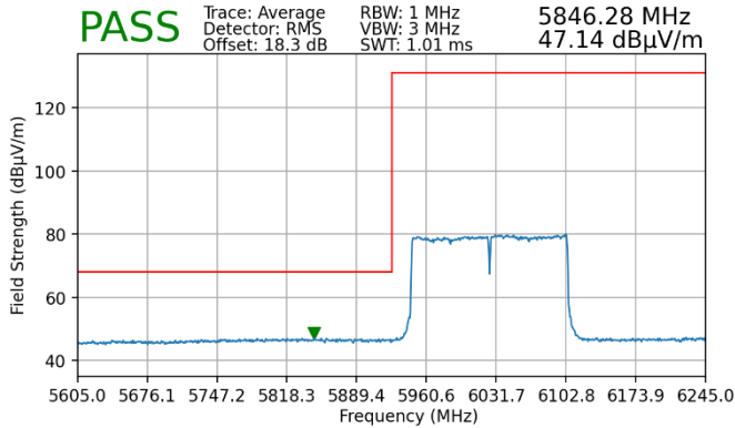
Plot 7-100. Radiated Lower Band Edge Plot MIMO (Average – UNII Band 5)
