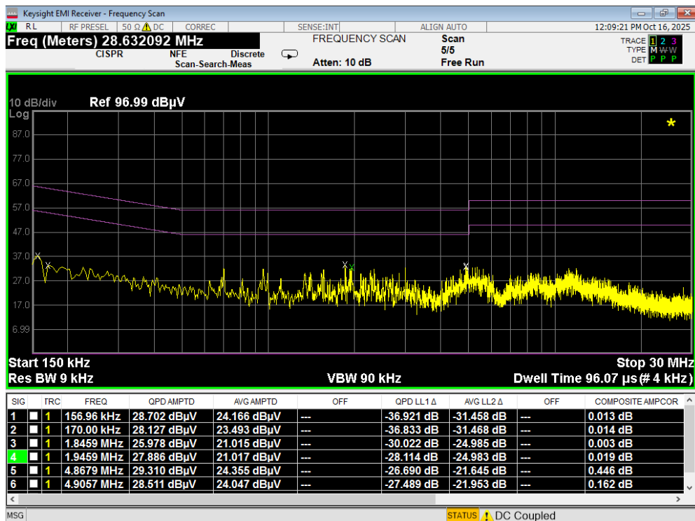
Plot 7-125. Line Conducted Plot with 802.11a UNII Band 5 (N) with WCP
