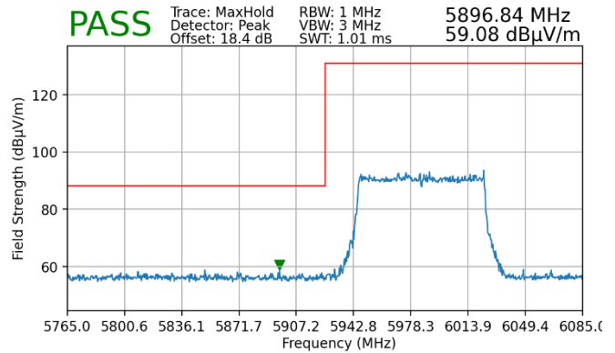
Plot 7-93. Radiated Lower Band Edge Plot MIMO (Peak – UNII Band 5)
