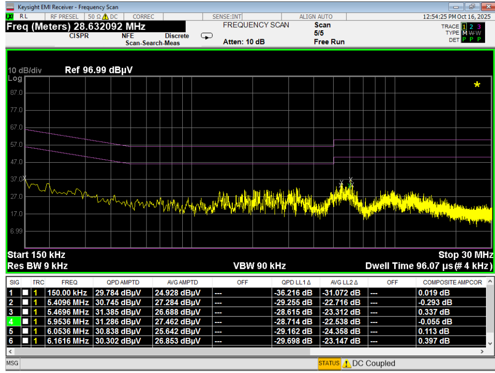
Plot 7-118. Line Conducted Plot with 802.11a UNII Band 6 (L1)
