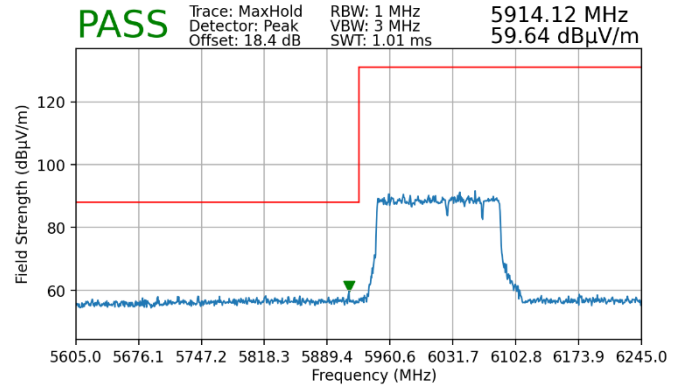
Plot 7-105. Radiated Lower Band Edge Plot MIMO (Peak – UNII Band 5)
