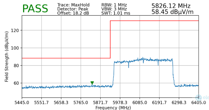
Plot 7-109. Radiated Lower Band Edge Plot MIMO (Peak – UNII Band 5)
