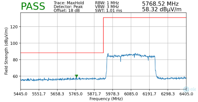
Plot 7-113. Radiated Lower Band Edge Plot MIMO (Peak – UNII Band 5)
