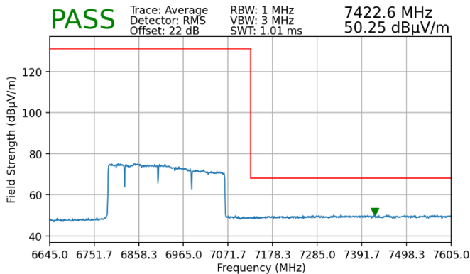
Plot 7-114. Radiated Upper Band Edge Plot MIMO (Average – UNII Band 8)
