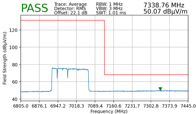
Plot 7-106. Radiated Upper Band Edge Plot MIMO (Average – UNII Band 8)
