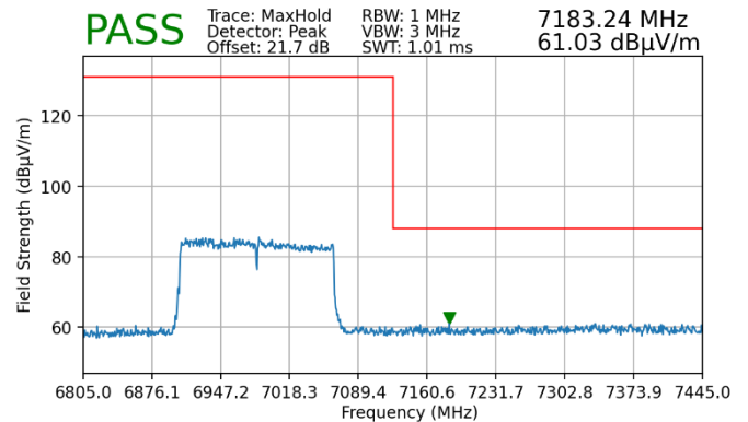
Plot 7-103. Radiated Upper Band Edge Plot MIMO (Peak – UNII Band 8)
