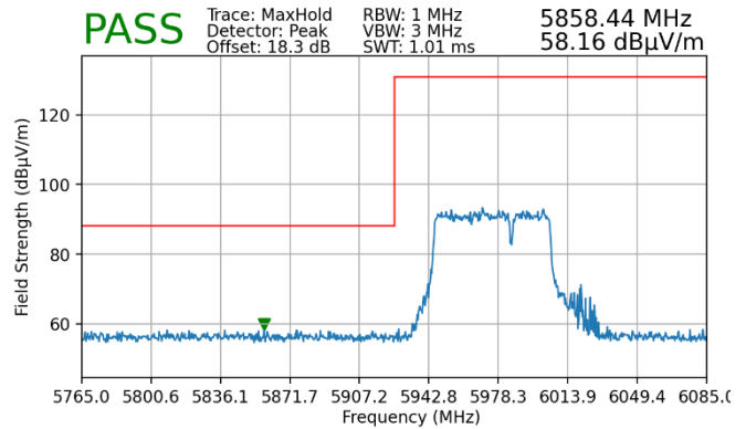
Plot 7-97. Radiated Lower Band Edge Plot MIMO (Peak – UNII Band 5)
