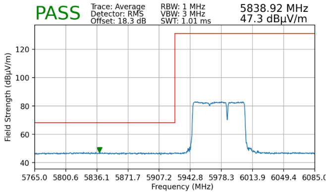
Plot 7-96. Radiated Lower Band Edge Plot MIMO (Average – UNII Band 5)
