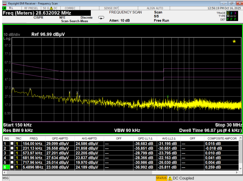
Plot 7-126. Line Conducted Plot with 802.11a UNII Band 6 (L1) with WCP
