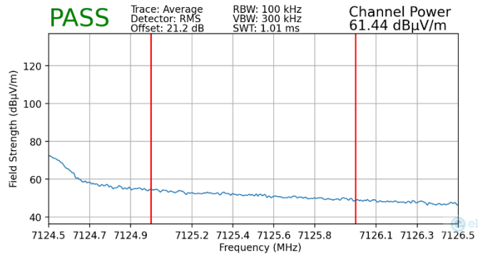
Plot 7-86. Radiated Upper Band Edge Plot MIMO (Average – UNII Band 8)
