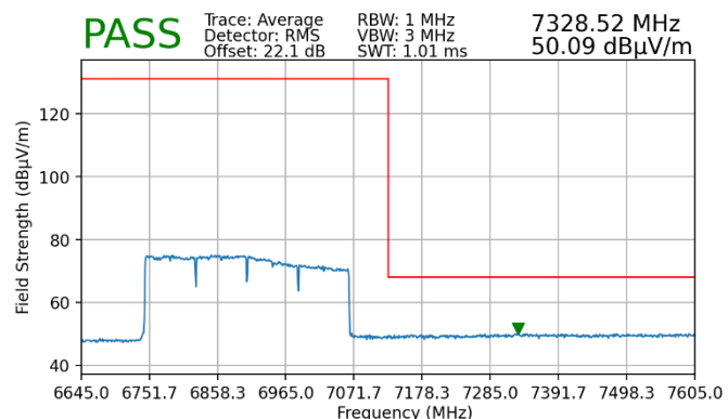
Plot 7-110. Radiated Upper Band Edge Plot MIMO (Average – UNII Band 8)
