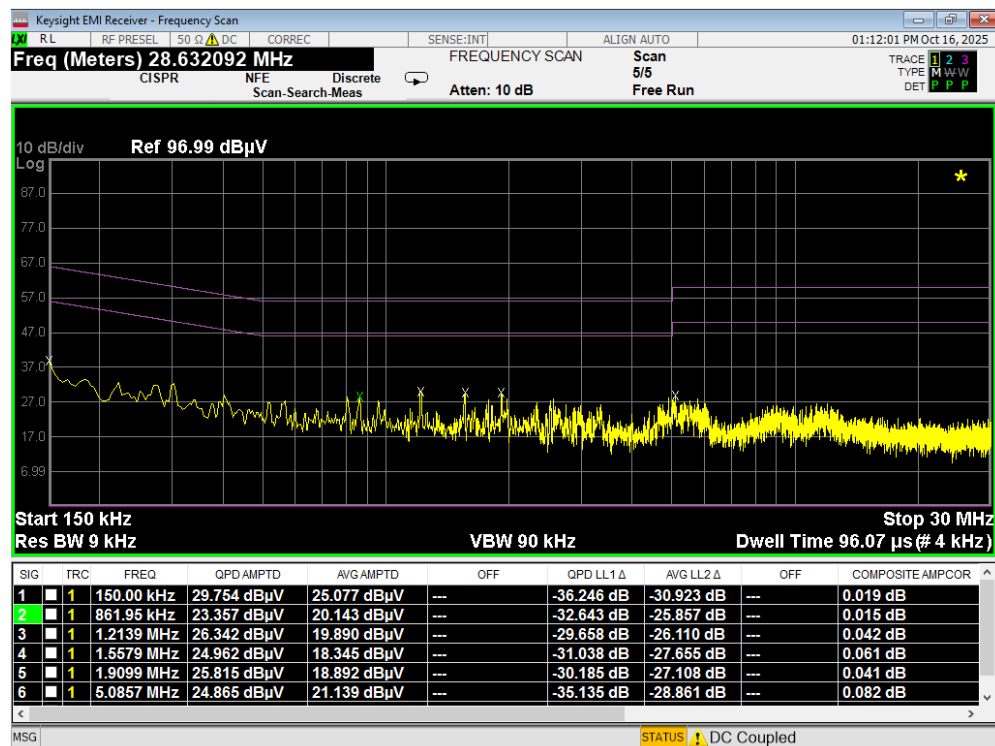
Plot 7-123. Line Conducted Plot with 802.11a UNII Band 8 (N)
