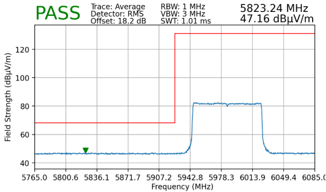
Plot 7-92. Radiated Lower Band Edge Plot MIMO (Average – UNII Band 5)
