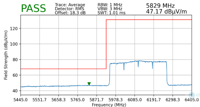
Plot 7-108. Radiated Lower Band Edge Plot MIMO (Average – UNII Band 5)
