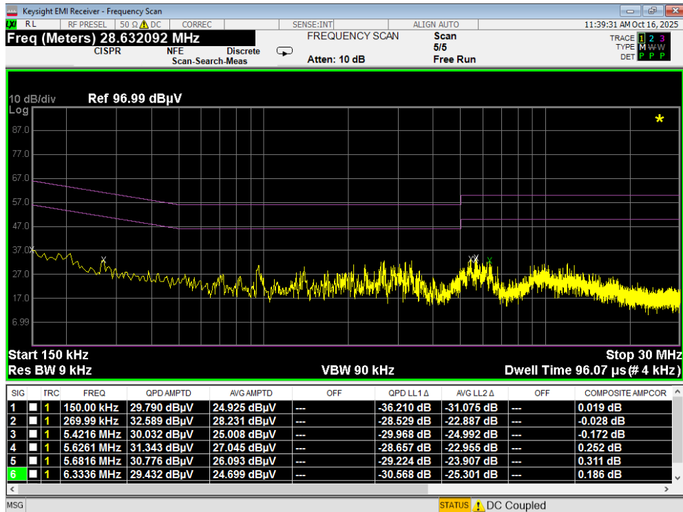
Plot 7-116. Line Conducted Plot with 802.11a UNII Band 5 (L1)
