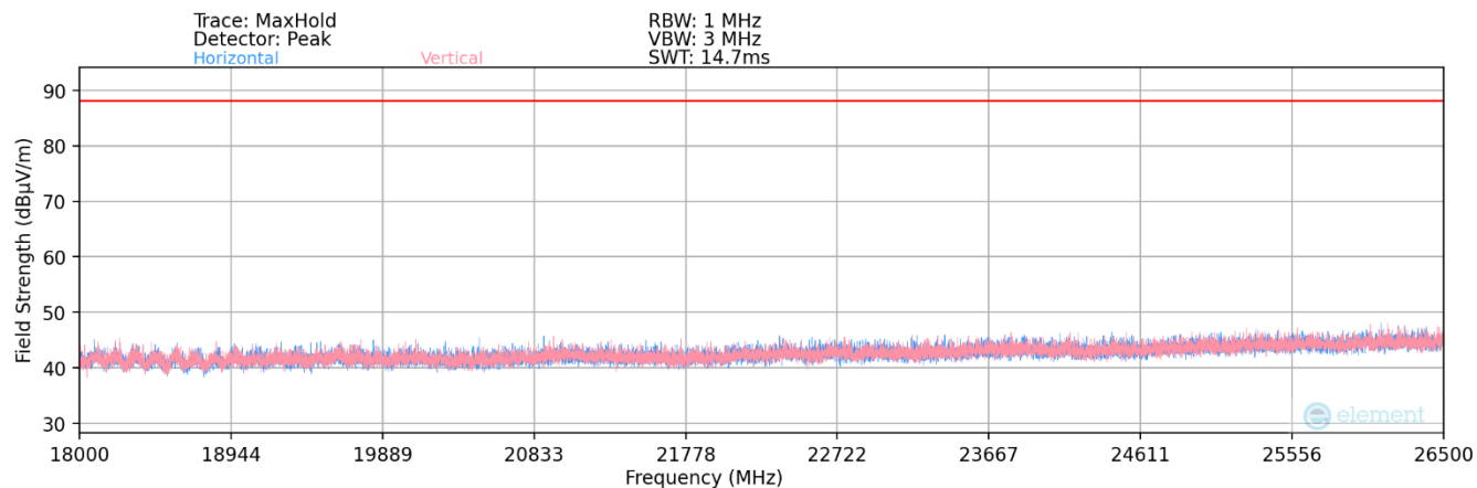
Plot 7-82. Radiated Spurious Plot 18GHz - 26.5GHz (802.11a) – Ch.149
