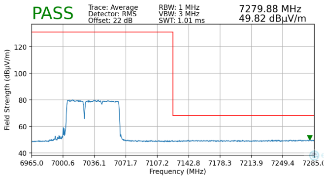
Plot 7-98. Radiated Upper Band Edge Plot MIMO (Average – UNII Band 8)
