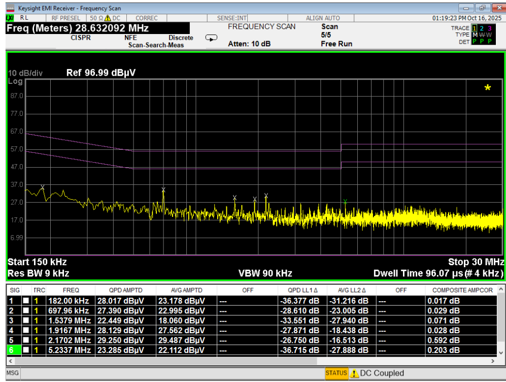
Plot 7-130. Line Conducted Plot with 802.11a UNII Band 8 (L1) with WCP
