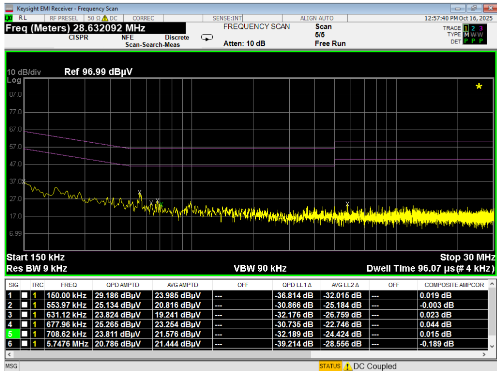
Plot 7-127. Line Conducted Plot with 802.11a UNII Band 6 (N) with WCP
