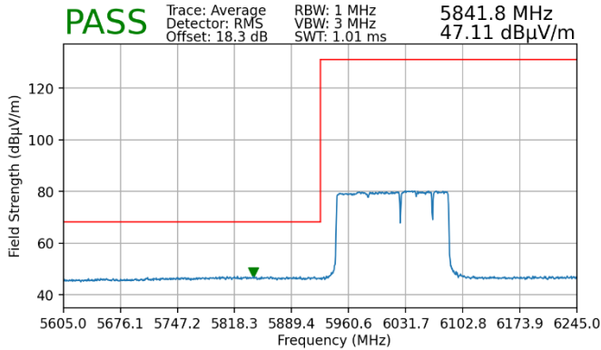
Plot 7-104. Radiated Lower Band Edge Plot MIMO (Average – UNII Band 5)
