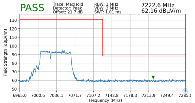
Plot 7-99. Radiated Upper Band Edge Plot MIMO (Peak – UNII Band 8)
