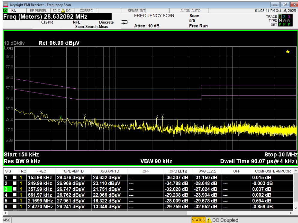
Plot 7-128. Line Conducted Plot with 802.11a UNII Band 7 (L1) with WCP
