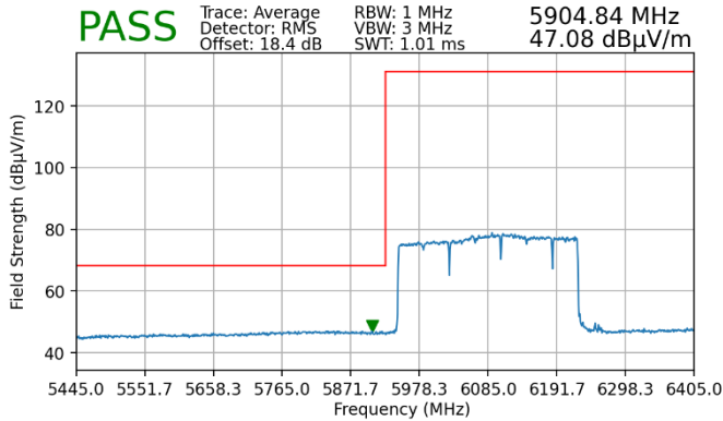
Plot 7-112. Radiated Lower Band Edge Plot MIMO (Average – UNII Band 5)
