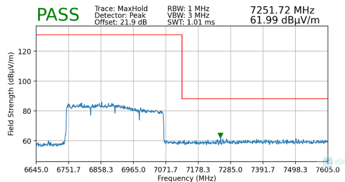
Plot 7-111. Radiated Upper Band Edge Plot MIMO (Peak – UNII Band 8)
