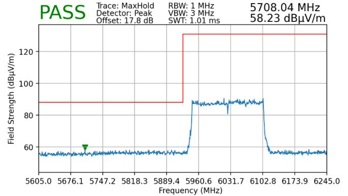
Plot 7-101. Radiated Lower Band Edge Plot MIMO (Peak – UNII Band 5)
