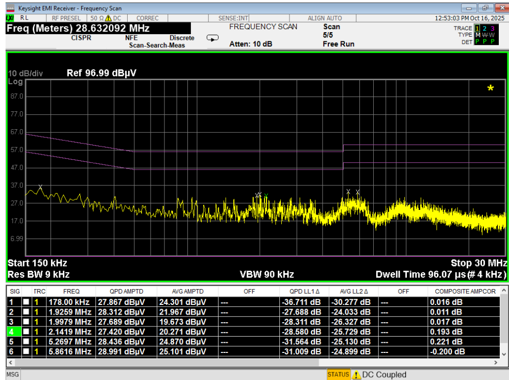
Plot 7-119. Line Conducted Plot with 802.11a UNII Band 6 (N)
