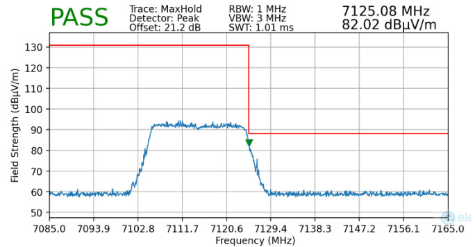
Plot 7-87. Radiated Upper Band Edge Plot MIMO (Peak – UNII Band 8)
