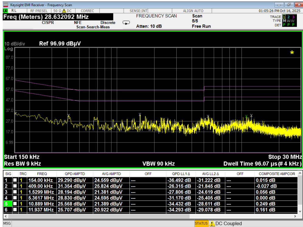
Plot 7-120. Line Conducted Plot with 802.11a UNII Band 7 (L1)
