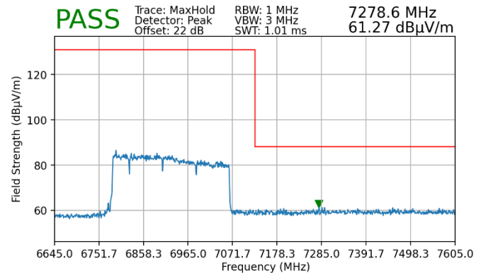
Plot 7-115. Radiated Upper Band Edge Plot MIMO (Peak – UNII Band 8)
