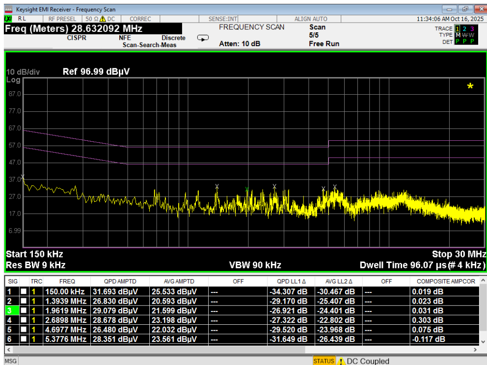
Plot 7-117. Line Conducted Plot with 802.11a UNII Band 5 (N)
