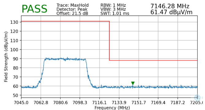
Plot 7-91. Radiated Upper Band Edge Plot MIMO (Peak – UNII Band 8)
