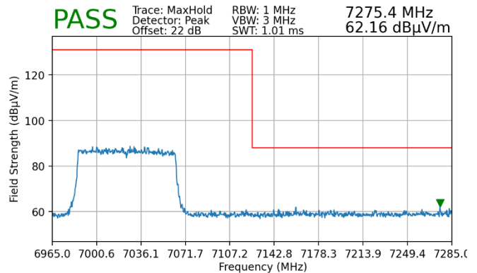
Plot 7-95. Radiated Upper Band Edge Plot MIMO (Peak – UNII Band 8)
