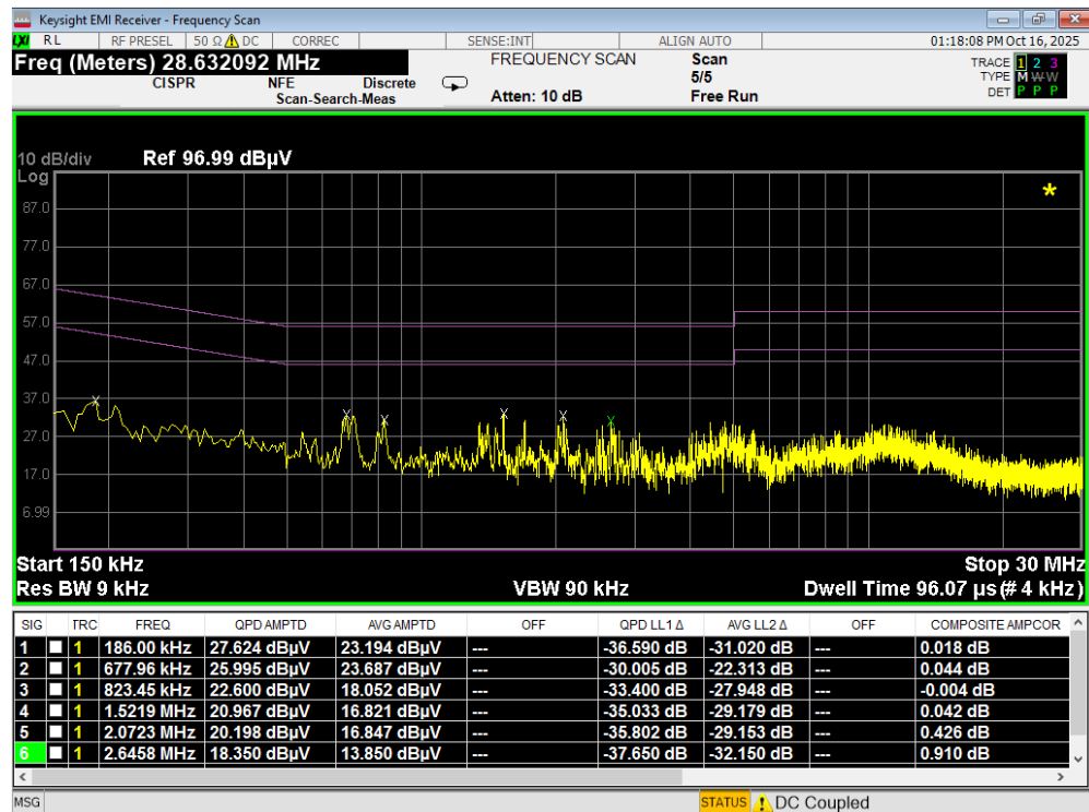
Plot 7-131. Line Conducted Plot with 802.11a UNII Band 8 (N) with WCP
