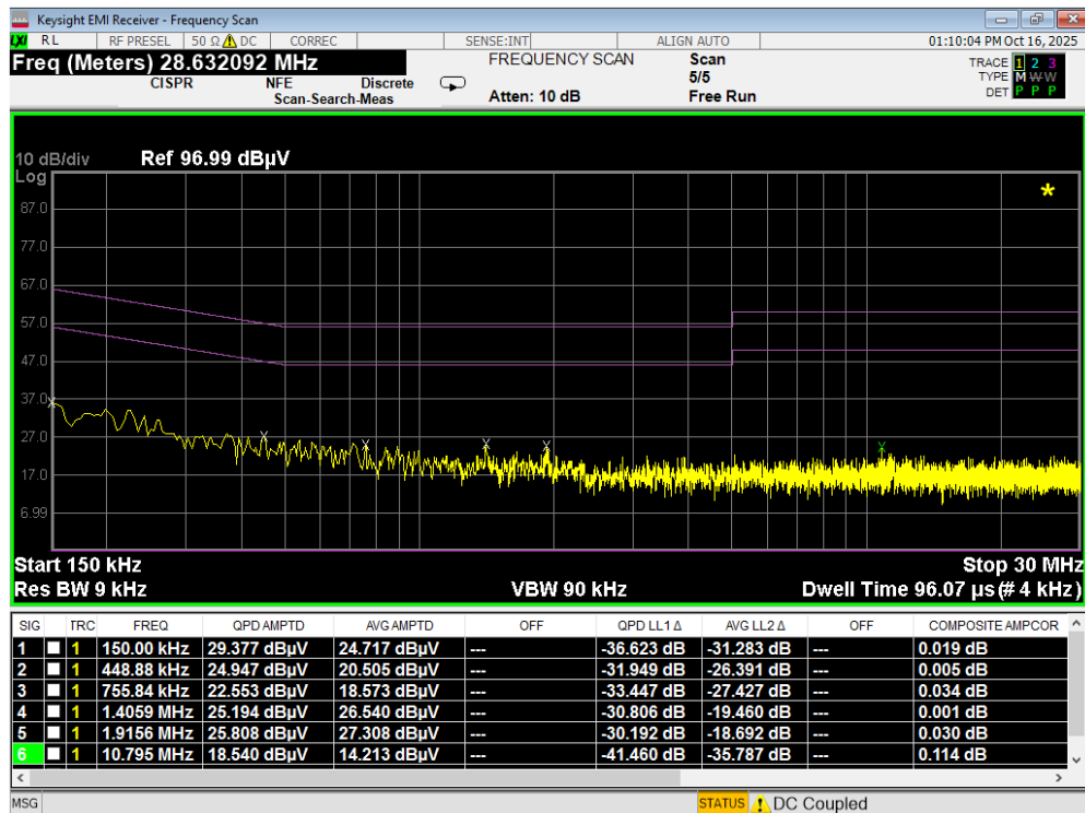
Plot 7-129. Line Conducted Plot with 802.11a UNII Band 7 (N) with WCP
