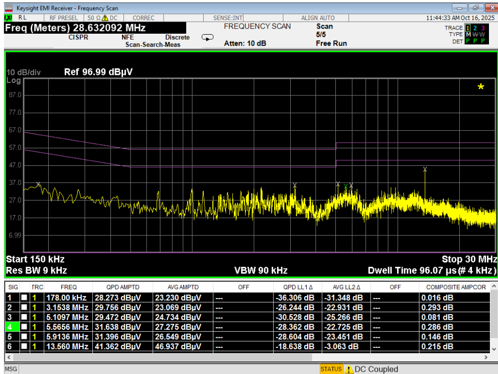
Plot 7-124. Line Conducted Plot with 802.11a UNII Band 5 (L1) with WCP
