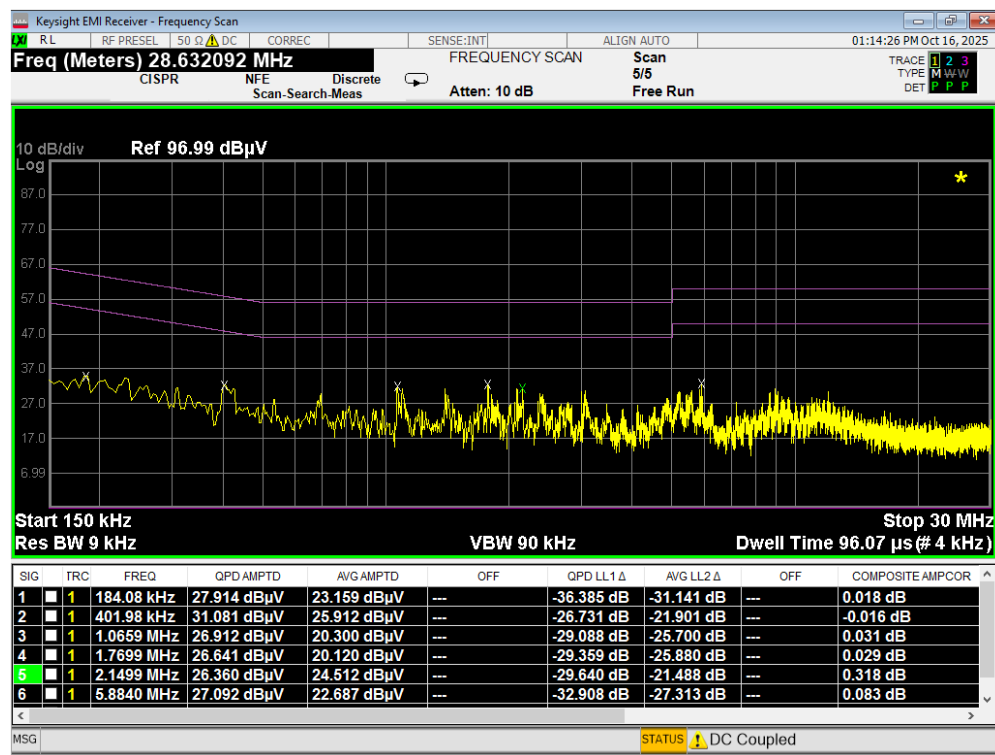
Plot 7-122. Line Conducted Plot with 802.11a UNII Band 8 (L1)
