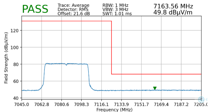
Plot 7-90. Radiated Upper Band Edge Plot MIMO (Average – UNII Band 8)
