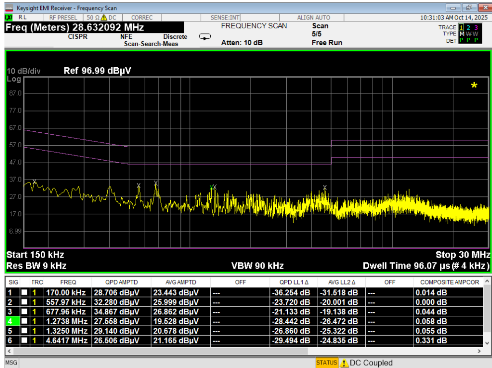
Plot 7-183. Line Conducted Plot with 802.11a UNII Band 5 (L1) with WCP
