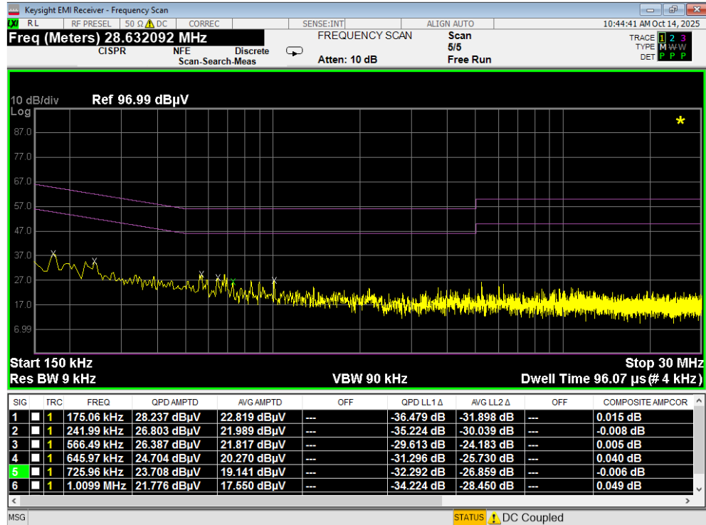
Plot 7-185. Line Conducted Plot with 802.11a UNII Band 6 (L1) with WCP
