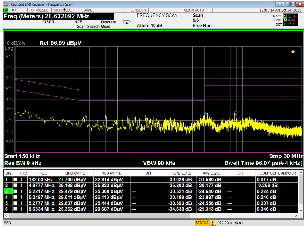
Plot 7-189. Line Conducted Plot with 802.11a UNII Band 8 (L1) with WCP
