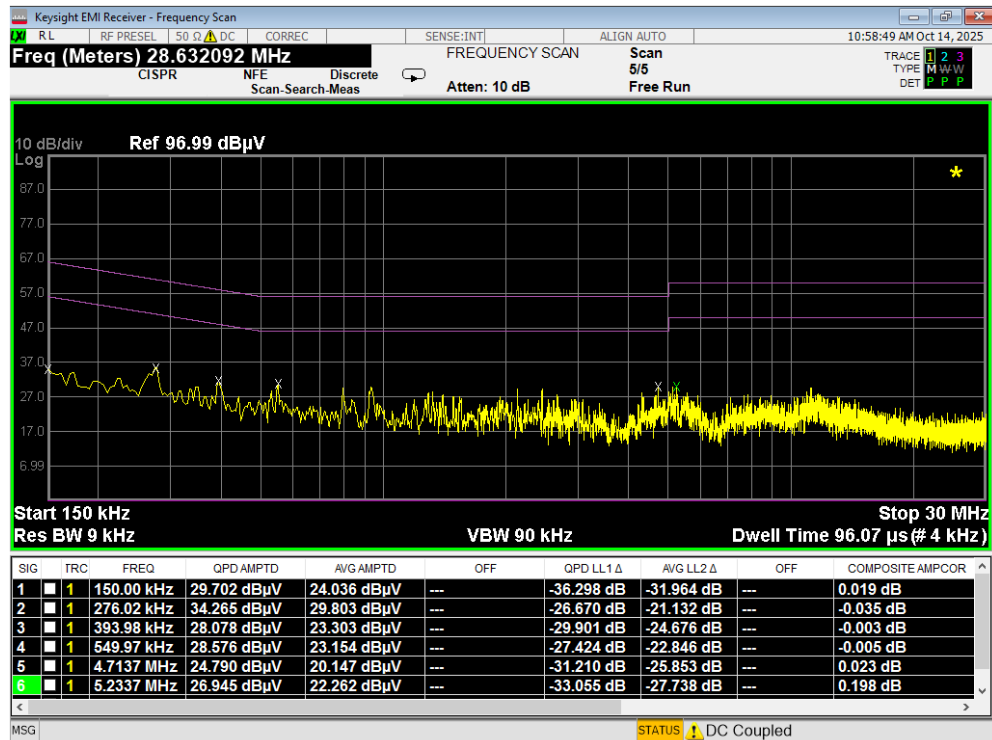
Plot 7-190. Line Conducted Plot with 802.11a UNII Band 8 (N) with WCP
