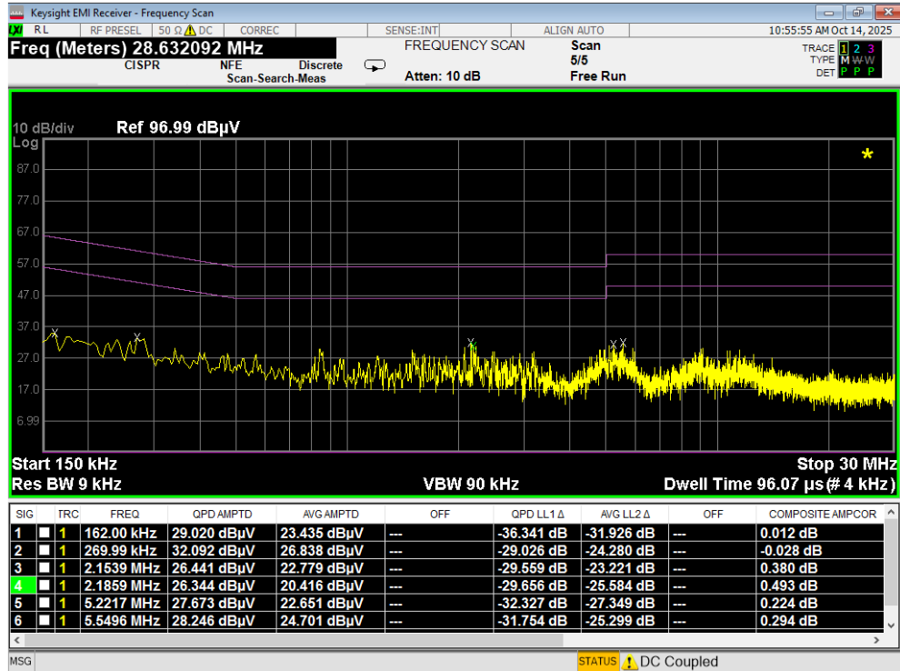
Plot 7-181. Line Conducted Plot with 802.11a UNII Band 8 (L1)
