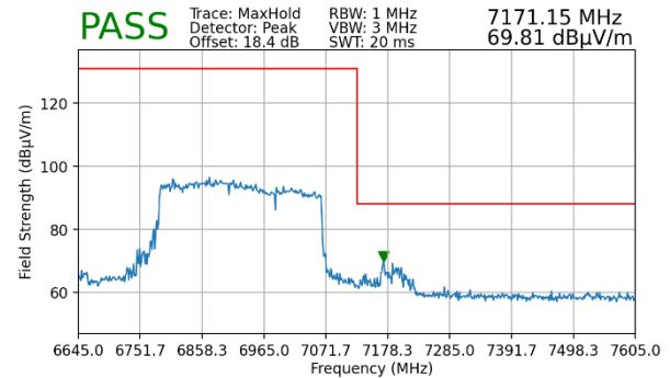
Plot 7-174. Radiated Upper Band Edge Plot MIMO (Peak – UNII Band 8)
