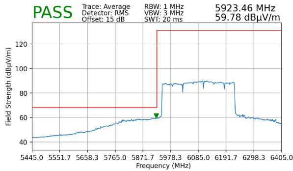
Plot 7-171. Radiated Lower Band Edge Plot MIMO (Average – UNII Band 5)
