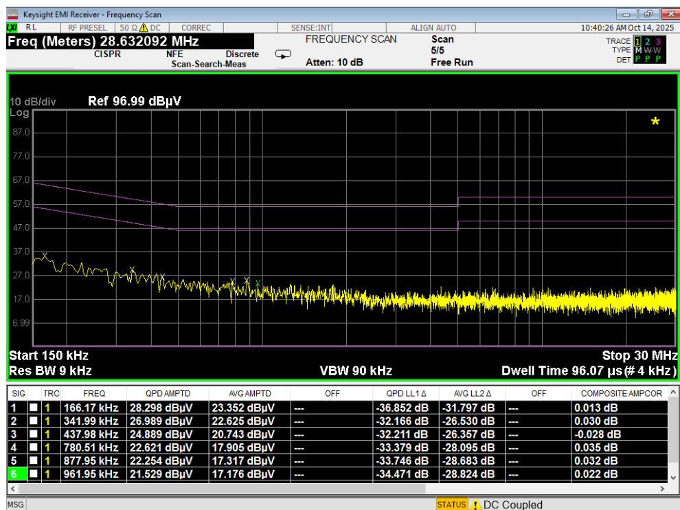
Plot 7-178. Line Conducted Plot with 802.11a UNII Band 6 (N)
