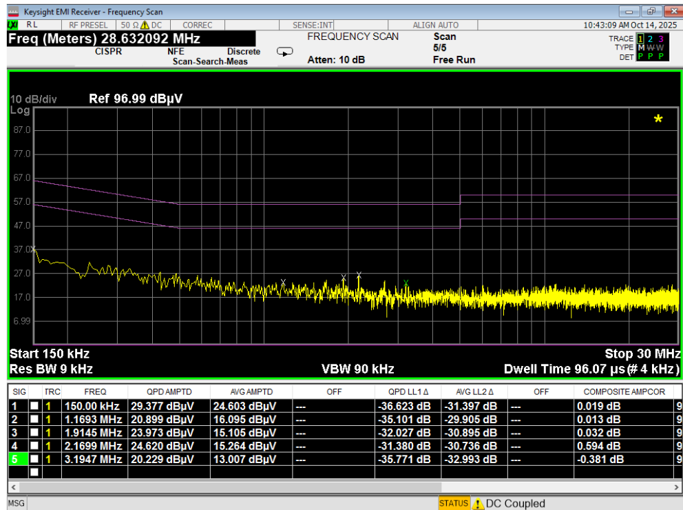
Plot 7-186. Line Conducted Plot with 802.11a UNII Band 6 (N) with WCP
