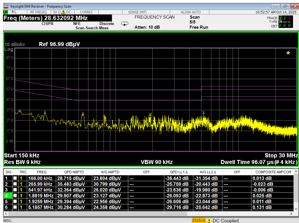
Plot 7-187. Line Conducted Plot with 802.11a UNII Band 7 (L1) with WCP
