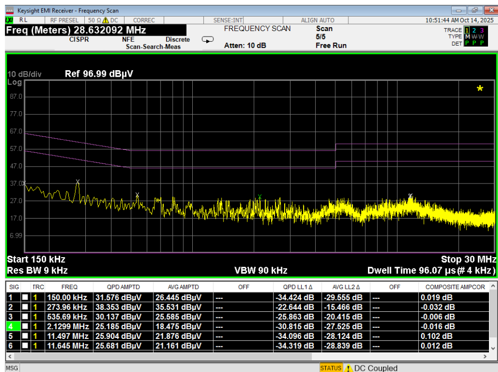
Plot 7-188. Line Conducted Plot with 802.11a UNII Band 7 (N) with WCP
