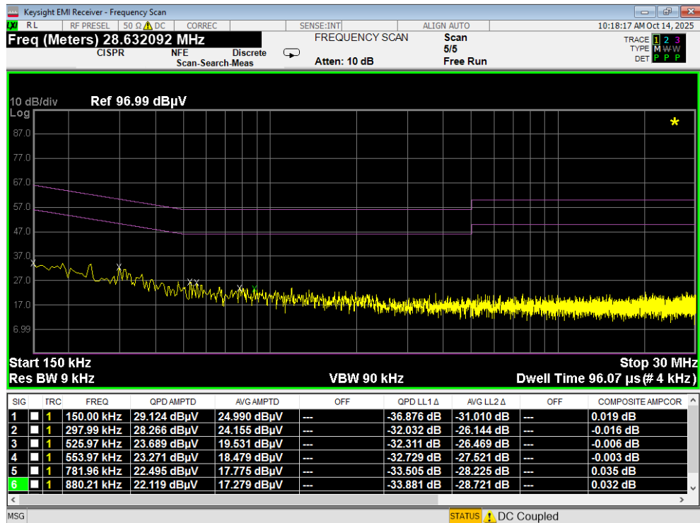
Plot 7-176. Line Conducted Plot with 802.11a UNII Band 5 (N)
