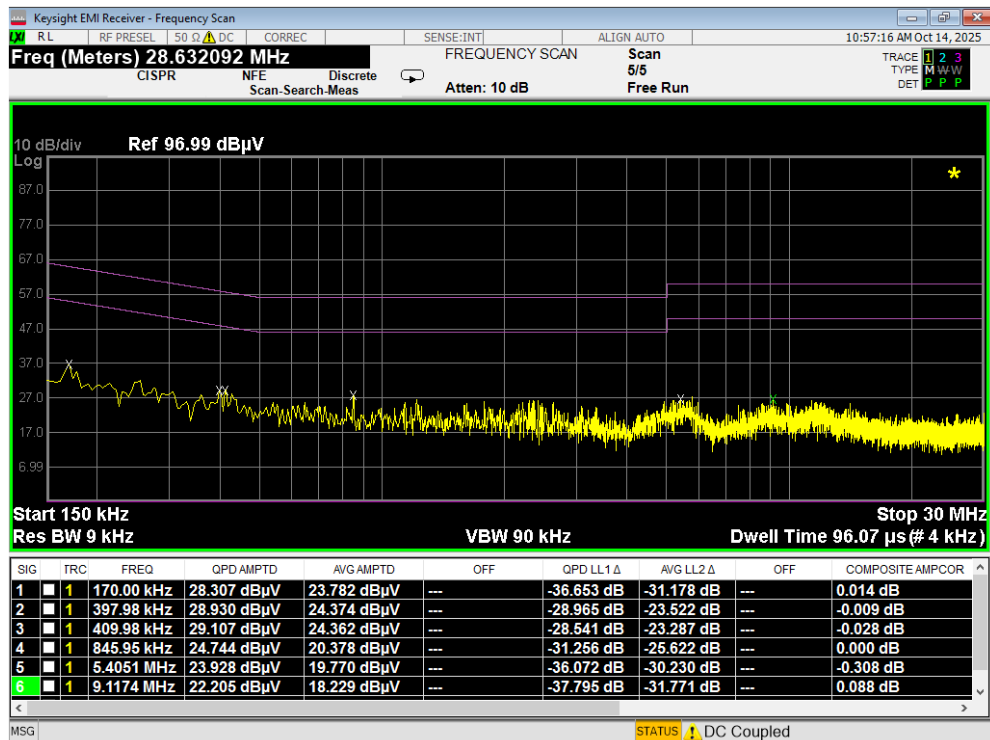
Plot 7-182. Line Conducted Plot with 802.11a UNII Band 8 (N)
