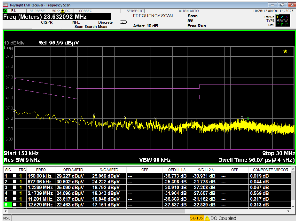
Plot 7-184. Line Conducted Plot with 802.11a UNII Band 5 (N) with WCP
