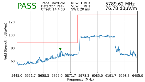
Plot 7-172. Radiated Lower Band Edge Plot MIMO (Peak – UNII Band 5)
