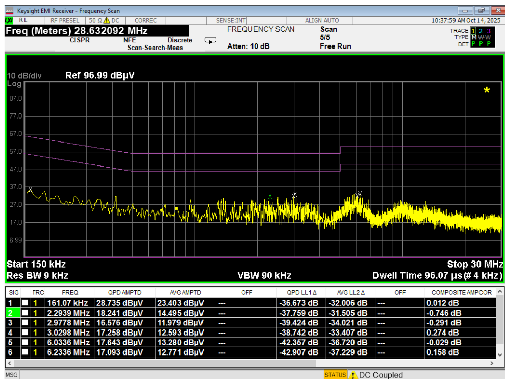
Plot 7-177. Line Conducted Plot with 802.11a UNII Band 6 (L1)
