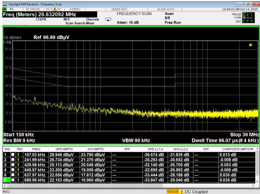
Plot 7-180. Line Conducted Plot with 802.11a UNII Band 7 (N)
