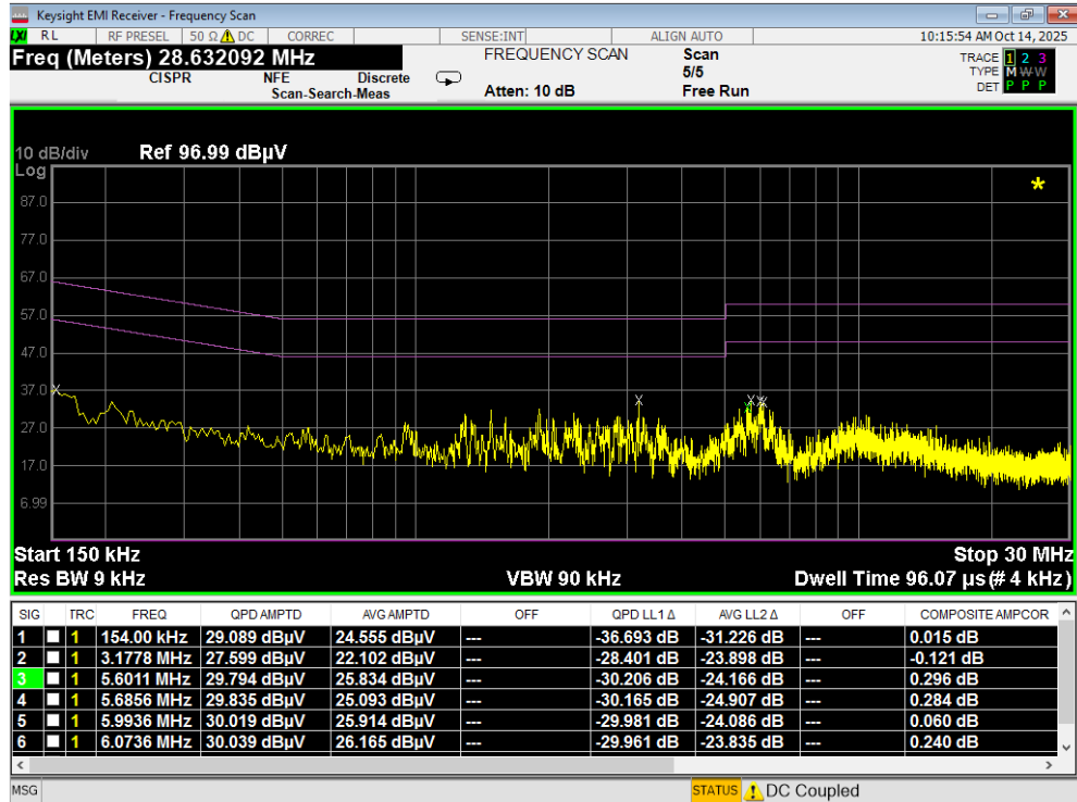
Plot 7-175. Line Conducted Plot with 802.11a UNII Band 5 (L1)
