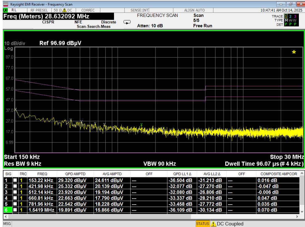
Plot 7-179. Line Conducted Plot with 802.11a UNII Band 7 (L1)
