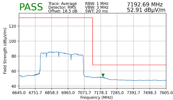
Plot 7-173. Radiated Upper Band Edge Plot MIMO (Average – UNII Band 8)
