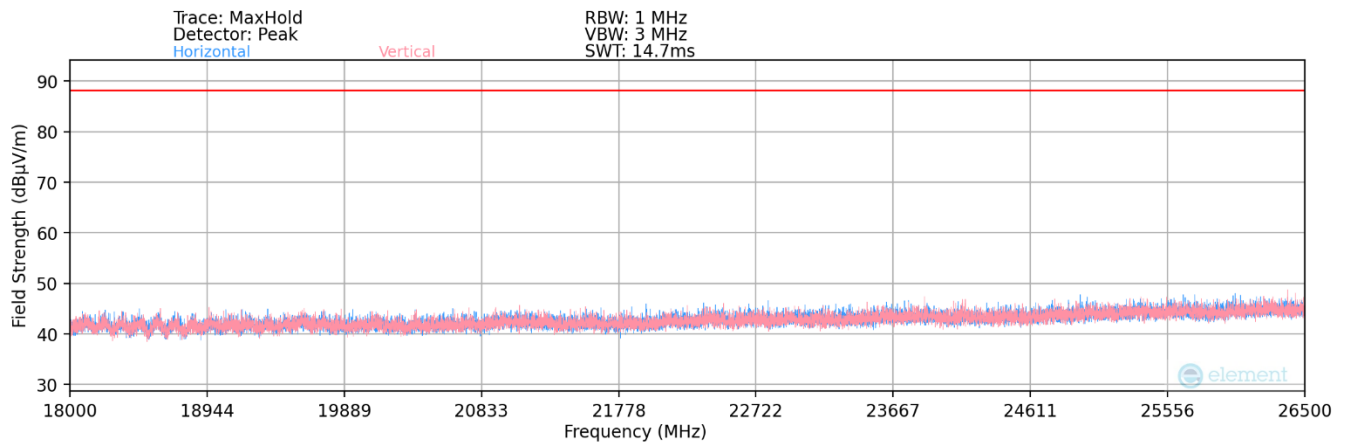
Plot 7-179. Radiated Spurious Plot 18GHz - 26.5GHz (802.11ax) – Ch.149
