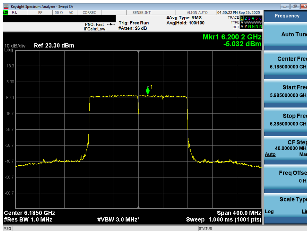
Plot 7-111. Power Spectral Density Plot MIMO ANT2 (160MHz 802.11ax/be (Full Tones) (UNII Band 5) – Ch. 47) - SP
