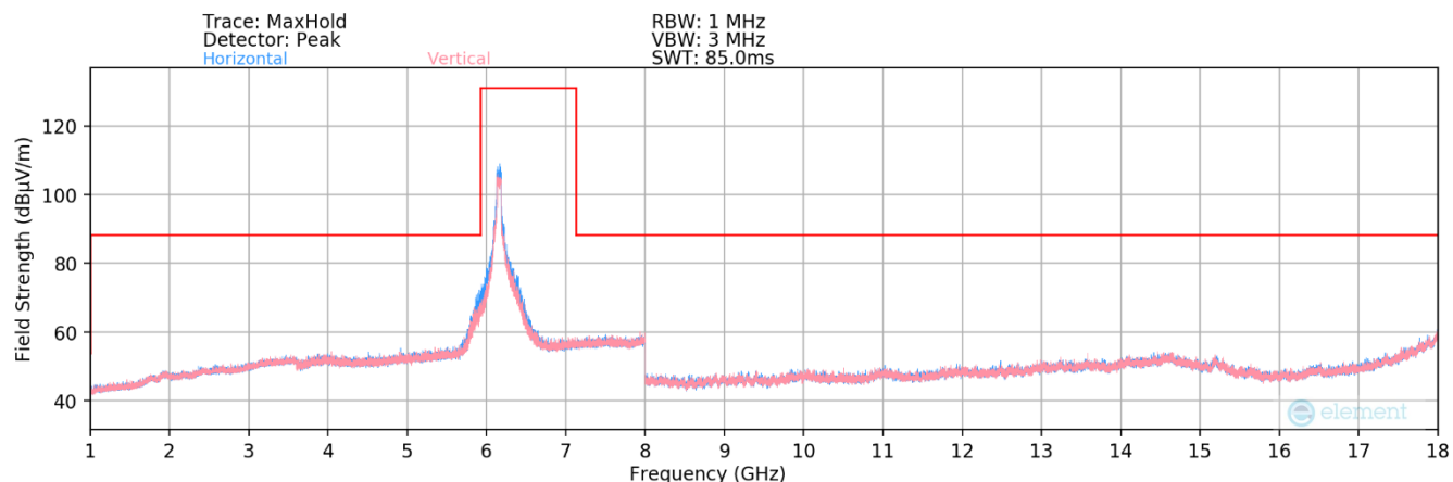
Plot 7-182. Radiated Spurious Plot 1GHz – 18GHz MIMO (802.11be – UNII Band 5 Ch. 39) – 484+242 Tones
