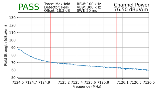
Plot 7-186. Radiated Lower Band Edge Plot MIMO (Peak – UNII Band 8 – 106T)
