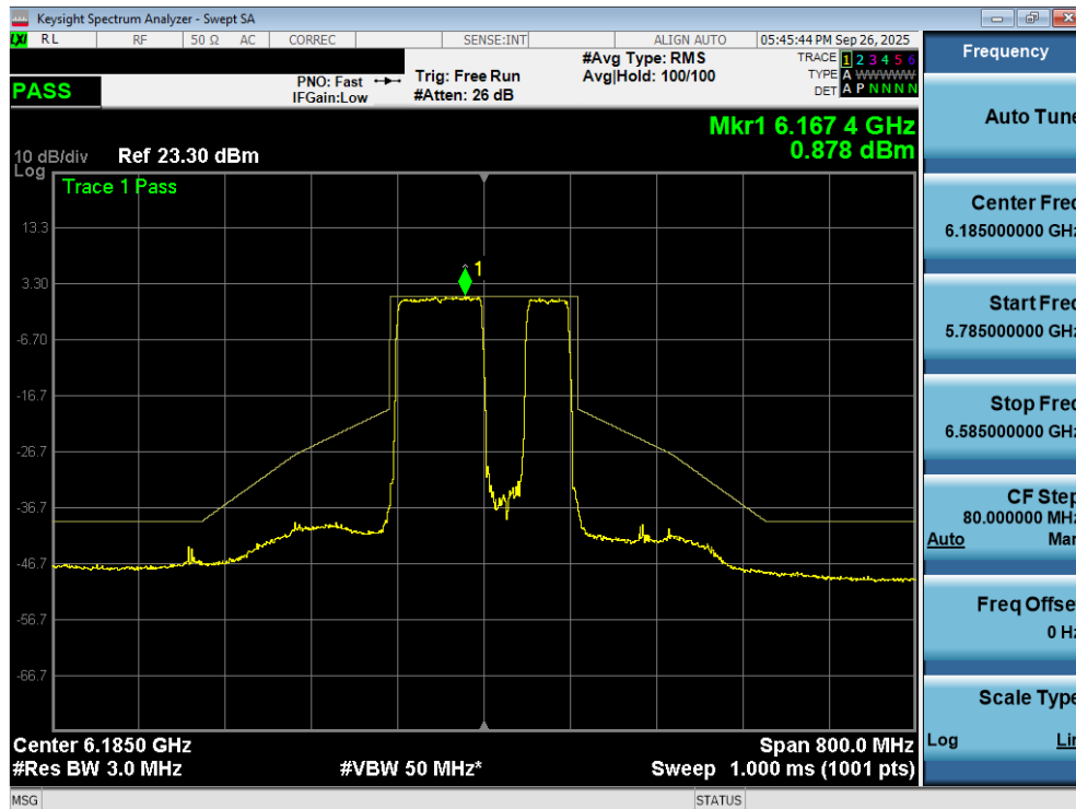
Plot 7-157. In Band Emissions Plot MIMO ANT2 (160MHz 802.11be (996+484 Tones) (UNII Band 5) – Ch. 47) SP
