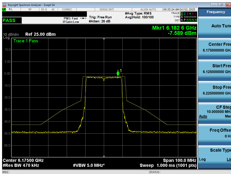
Plot 7-159. In Band Emissions Plot MIMO ANT2 (20MHz 802.11ax/be (Full Tones) (UNII Band 5) – Ch. 45) - LPI
