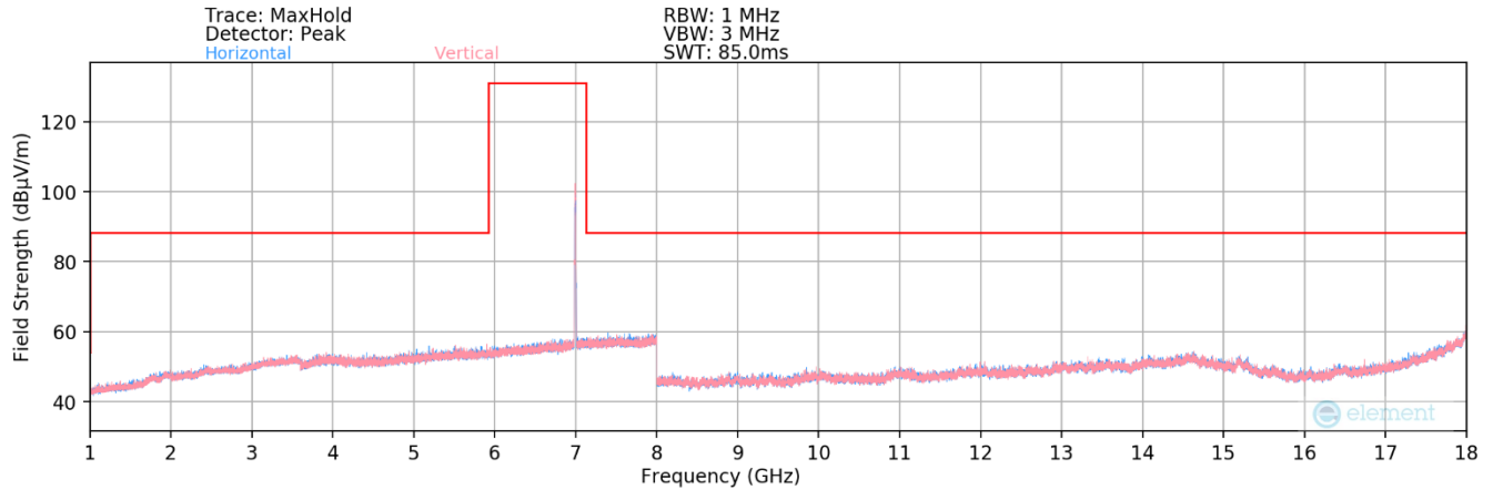
Plot 7-172. Radiated Spurious Plot 1GHz – 18GHz MIMO (802.11ax – U Band 8 Ch. 209)
