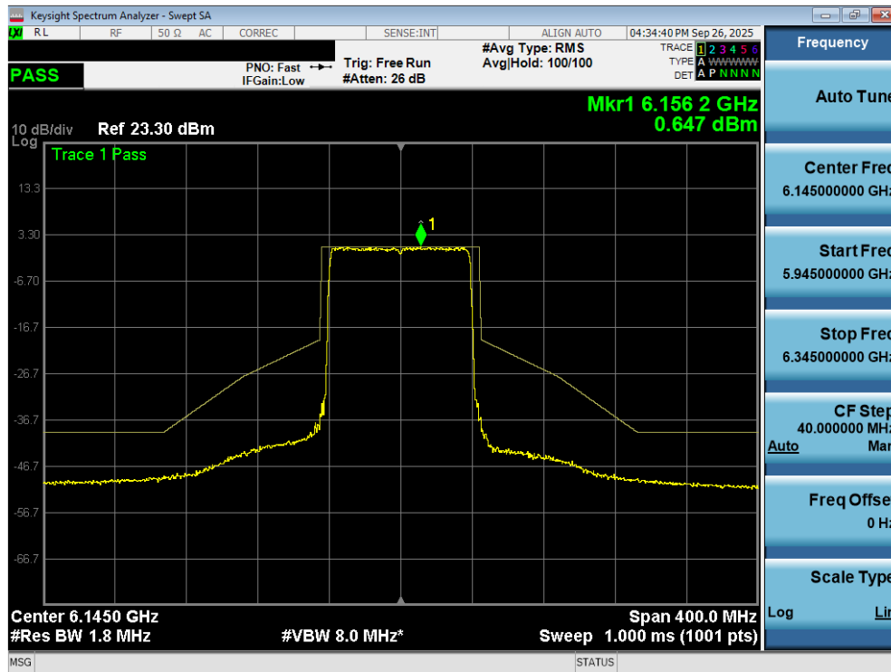
Plot 7-166. In Band Emissions Plot MIMO ANT2 (80MHz 802.11ax/be (Full Tones) (UNII Band 5) – Ch. 39) – SP
