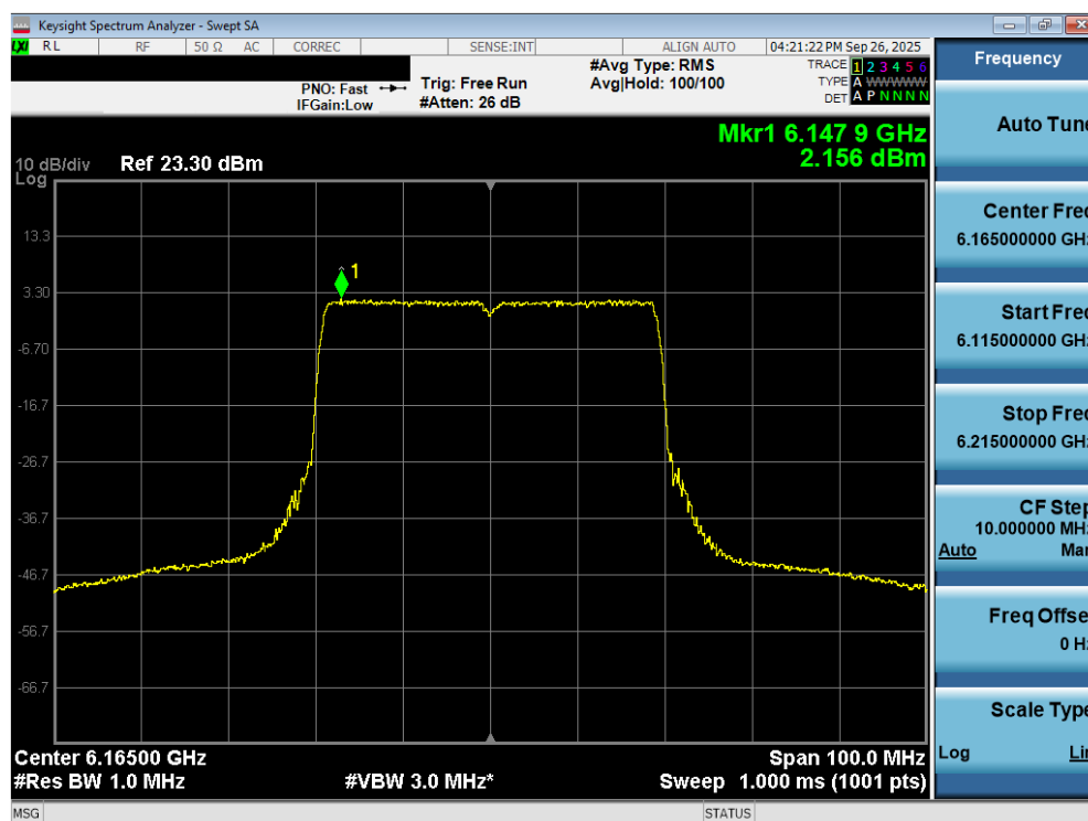
Plot 7-109. Power Spectral Density Plot MIMO ANT2 (40MHz 802.11ax/be (Full Tones) (UNII Band 5) – Ch. 43) – SP
