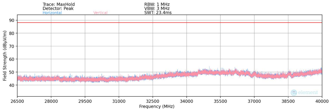
Plot 7-180. Radiated Spurious Plot 26.5GHz - 40GHz (802.11ax) – Ch.149
