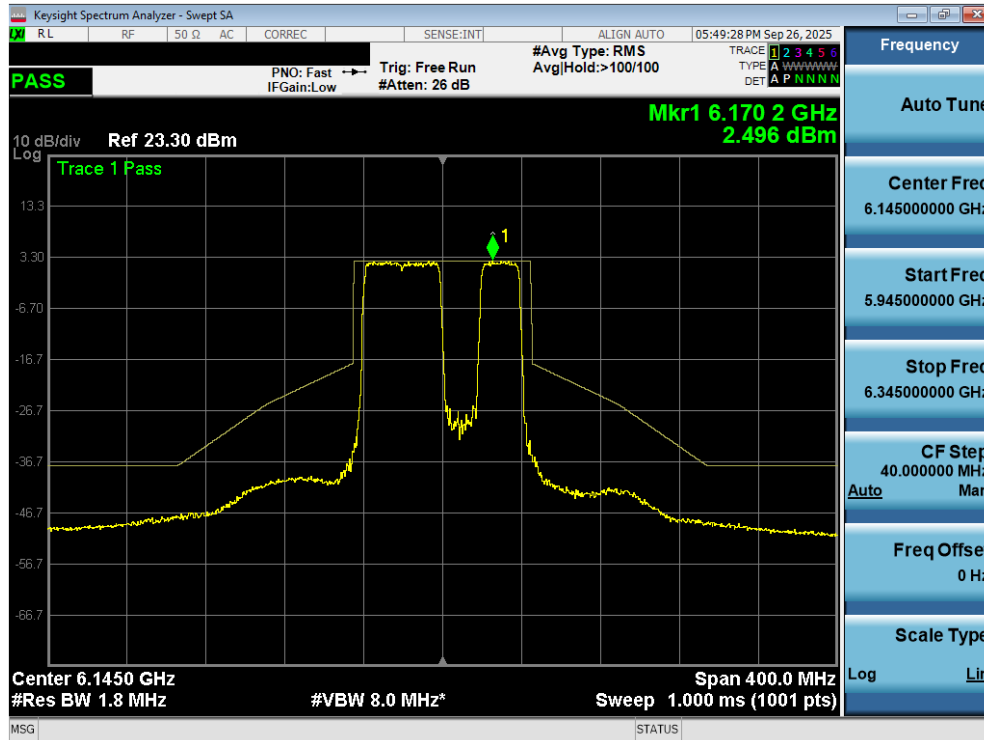
Plot 7-156. In Band Emissions Plot MIMO ANT2 (80MHz 802.11be (484+242 Tones) (UNII Band 5) – Ch. 39) SP
