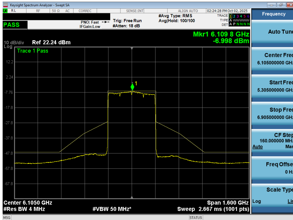
Plot 7-163. In Band Emissions Plot MIMO ANT2 (320MHz 802.11be (Full Tones) (UNII Band 5) – Ch. 31) - LPI
