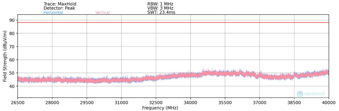
Plot 7-174. Radiated Spurious Plot 26.5GHz - 40GHz (802.11ax) – Ch.149
