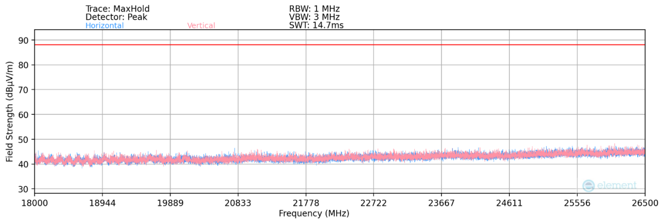
Plot 7-173. Radiated Spurious Plot 18GHz - 26.5GHz (802.11ax) – Ch.149
