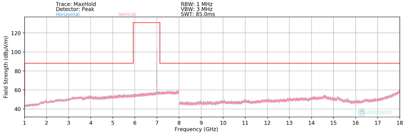
Plot 7-178. Radiated Spurious Plot 1GHz – 18GHz MIMO (802.11ax – U Band 8 Ch. 209)
