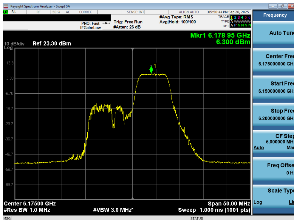
Plot 7-99. Power Spectral Density Plot MIMO ANT2 (20MHz 802.11be (52+26 Tones) (UNII Band 5) – Ch. 45) – SP
