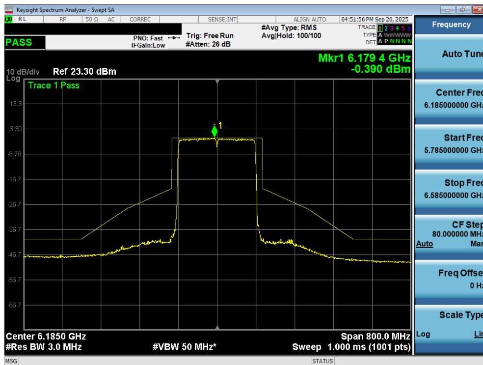
Plot 7-167. In Band Emissions Plot MIMO ANT2 (160MHz 802.11ax/be (Full Tones) (UNII Band 5) – Ch. 47) - SP
