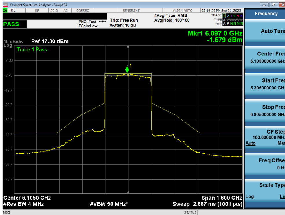
Plot 7-168. In Band Emissions Plot MIMO ANT2 (320MHz 802.11be (Full Tones) (UNII Band 5) – Ch. 31) - SP
