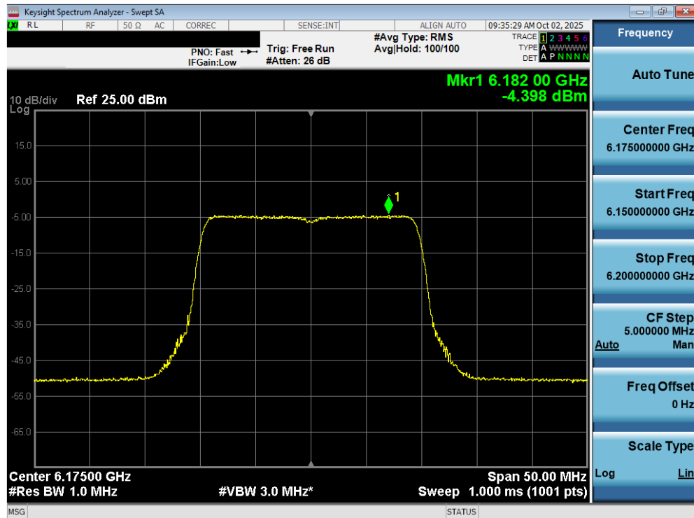
Plot 7-103. Power Spectral Density Plot MIMO ANT2 (20MHz 802.11ax/be (Full Tones) (UNII Band 5) – Ch. 45) - LPI
