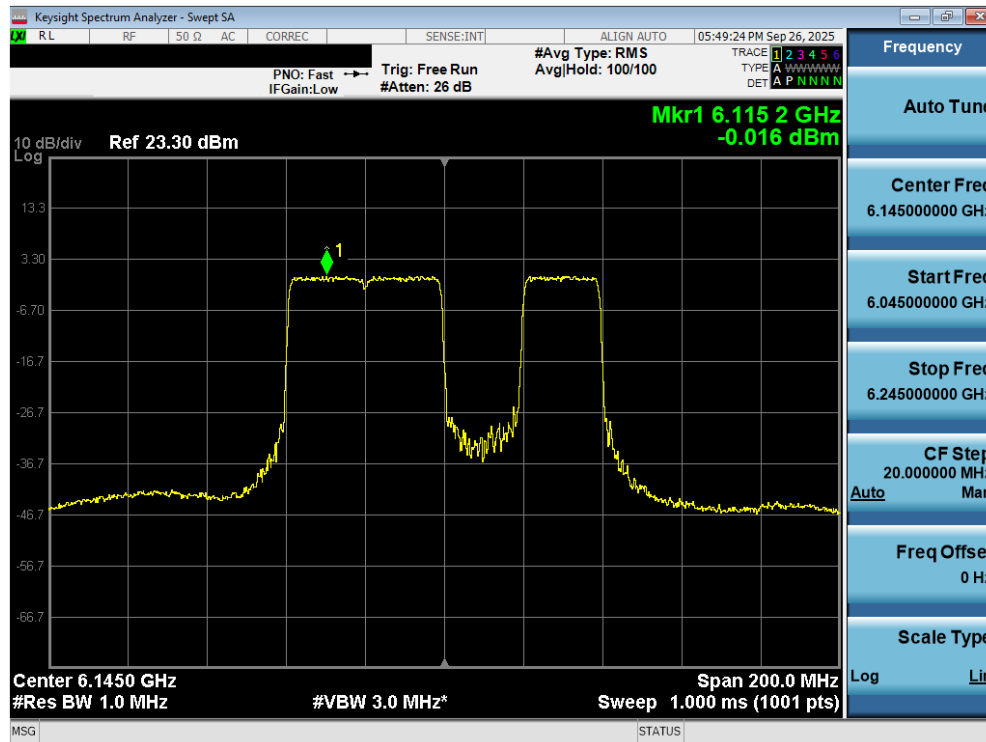
Plot 7-100. Power Spectral Density Plot MIMO ANT2 (80MHz 802.11be (484+242 Tones) (UNII Band 5) – Ch. 39) SP
