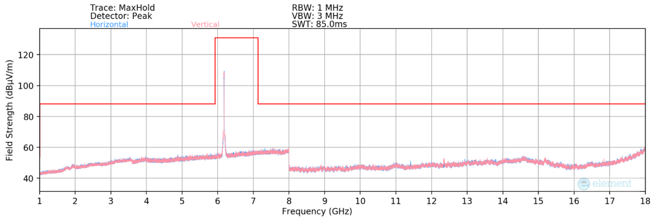
Plot 7-175. Radiated Spurious Plot 1GHz – 18GHz MIMO (802.11ax – UNII Band 5 Ch. 45)
