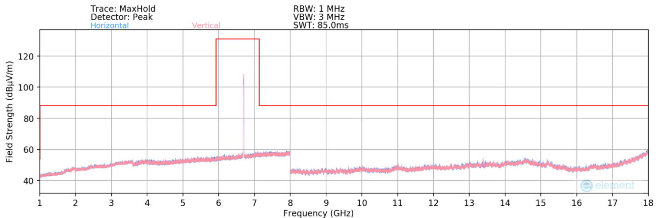
Plot 7-171. Radiated Spurious Plot 1GHz – 18GHz MIMO (802.11ax – UNII Band 7 Ch. 149)
