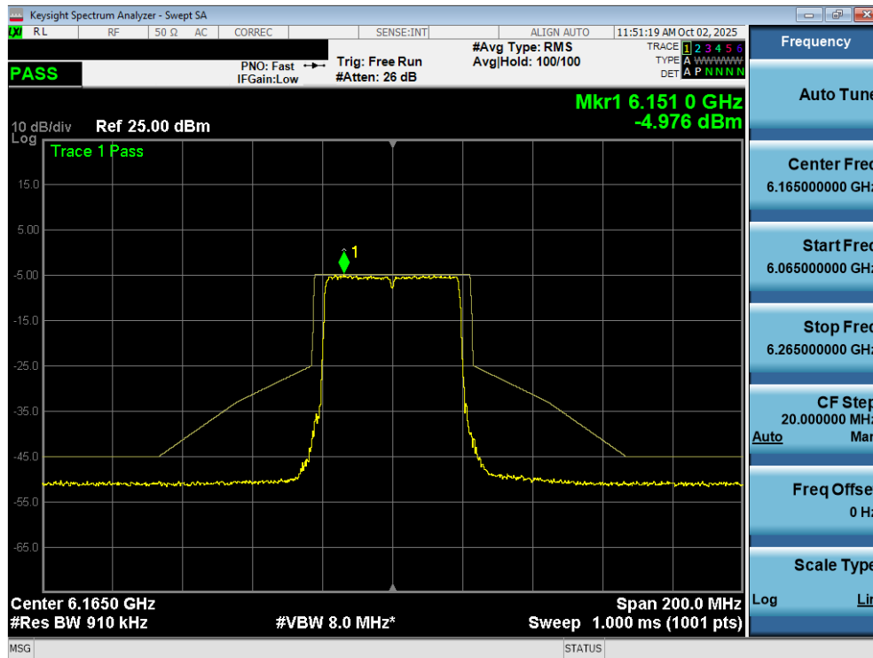
Plot 7-160. In Band Emissions Plot MIMO ANT2 (40MHz 802.11ax/be (Full Tones) (UNII Band 5) – Ch. 43) - LPI
