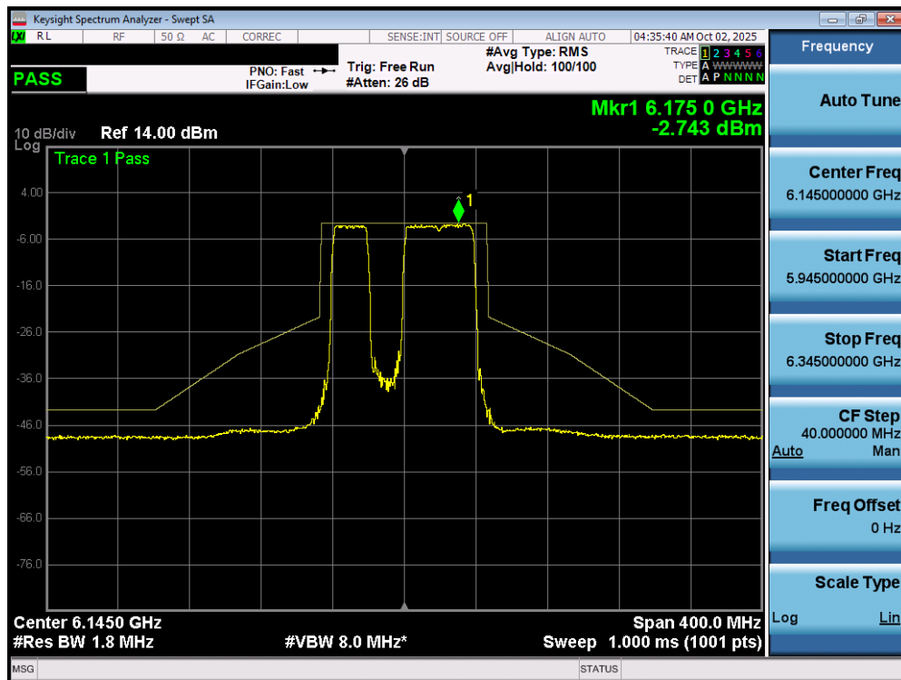
Plot 7-119. In Band Emissions Plot MIMO ANT1 (80MHz 802.11be (484+242 Tones) (UNII Band 5) – Ch. 39) LPI
