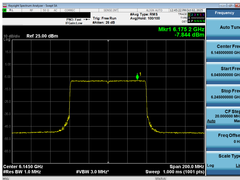
Plot 7-105. Power Spectral Density Plot MIMO ANT2 (80MHz 802.11ax/be (Full Tones) (UNII Band 5) – Ch. 39) - LPI
