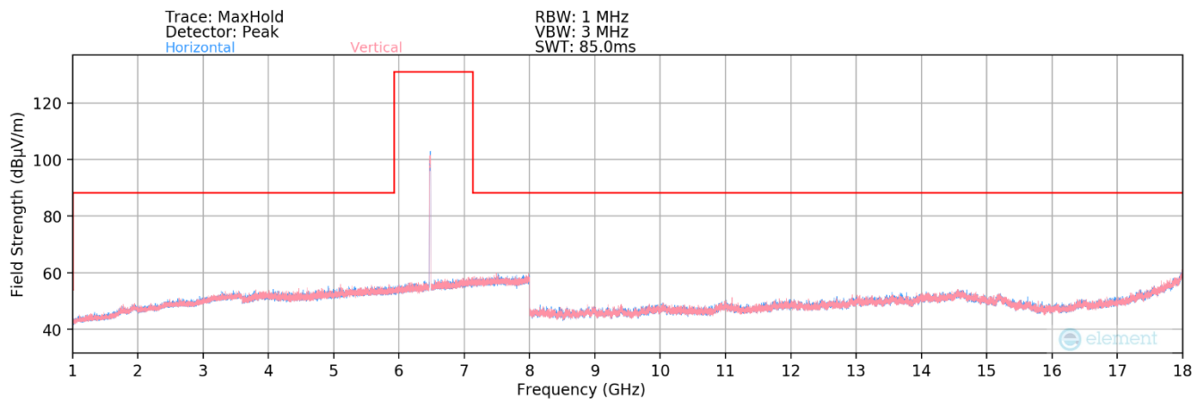
Plot 7-170. Radiated Spurious Plot 1GHz – 18GHz MIMO (802.11ax – UNII Band 6 Ch. 105)
