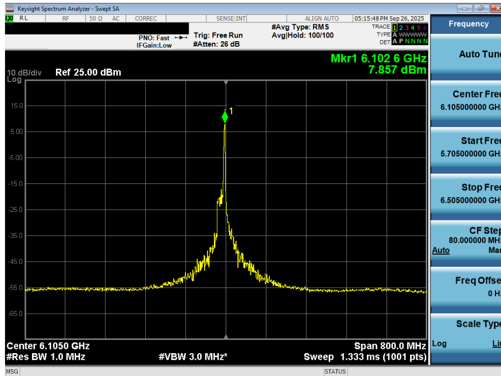
Plot 7-98. Power Spectral Density Plot MIMO ANT2 (320MHz 802.11be (26 Tones) (UNII Band 5) – Ch. 31) - SP
