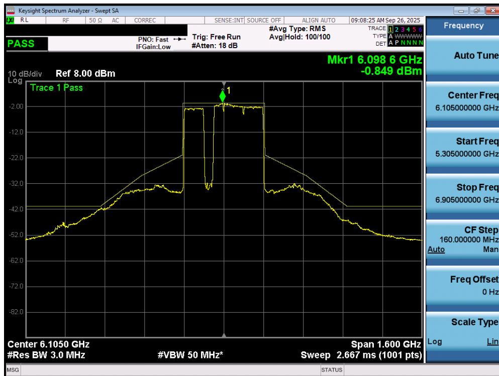
Plot 7-130. In Band Emissions Plot MIMO ANT1 (320MHz 802.11be (3*996+484 Tones) (UNII Band 5) – Ch. 31) SP
