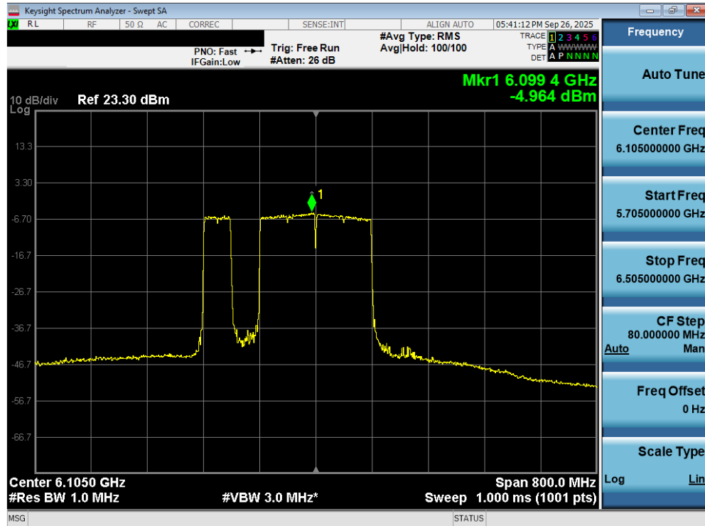
Plot 7-102. Power Spectral Density Plot MIMO ANT2 (320MHz 802.11be (2*996+484 Tones) (UNII Band 5) – Ch. 31) SP
