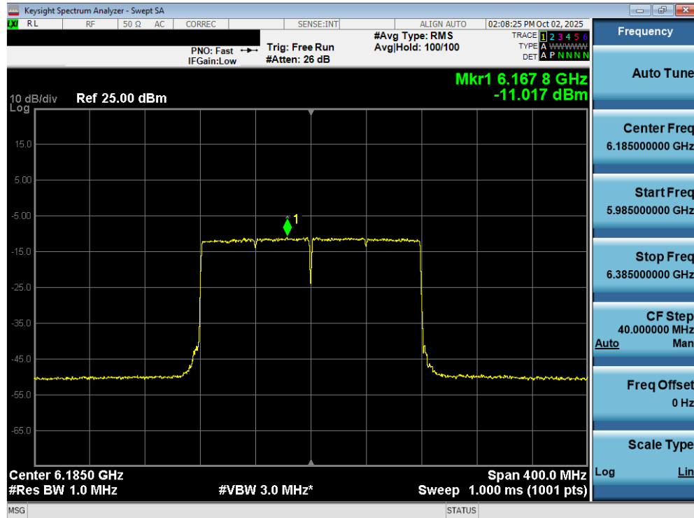
Plot 7-106. Power Spectral Density Plot MIMO ANT2 (160MHz 802.11ax/be (Full Tones) (UNII Band 5) – Ch. 47) - LPI
