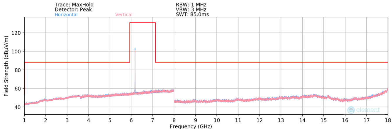
Plot 7-181. Radiated Spurious Plot 1GHz – 18GHz MIMO (802.11be – UNII Band 5 Ch. 45) – 52+26 Tones
