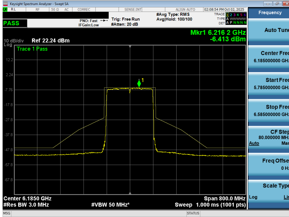
Plot 7-162. In Band Emissions Plot MIMO ANT2 (160MHz 802.11ax/be (Full Tones) (UNII Band 5) – Ch. 47) - LPI
