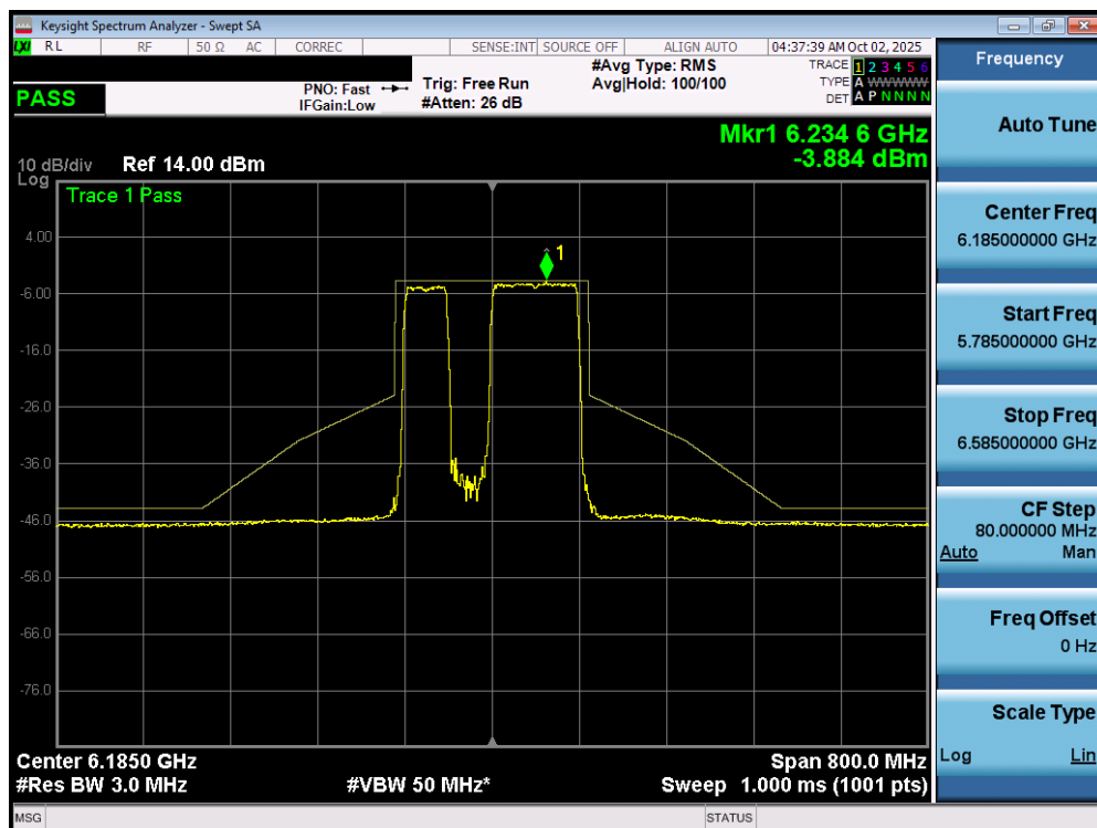
Plot 7-120. In Band Emissions Plot MIMO ANT1 (160MHz 802.11be (996+484 Tones) (UNII Band 5) – Ch. 47) LPI
