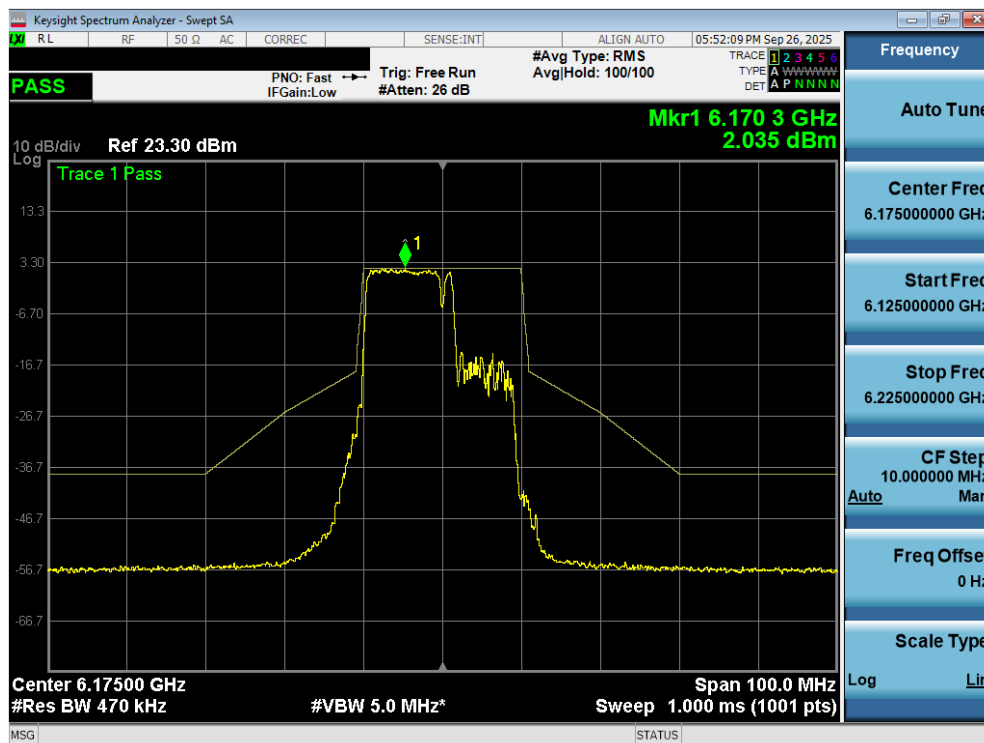
Plot 7-155. In Band Emissions Plot MIMO ANT2 (20MHz 802.11be (106+26 Tones) (UNII Band 5) – Ch. 45) - SP
