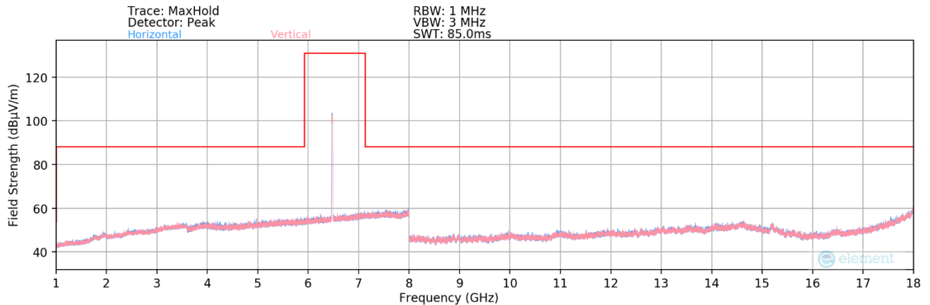
Plot 7-176. Radiated Spurious Plot 1GHz – 18GHz MIMO (802.11ax – UNII Band 6 Ch. 105)
