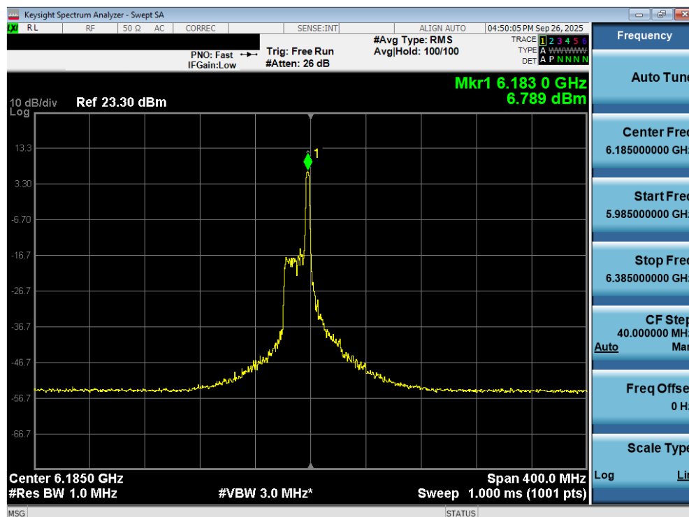
Plot 7-97. Power Spectral Density Plot MIMO ANT2 (160MHz 802.11ax/be (26 Tones) (UNII Band 5) – Ch. 47) - SP
