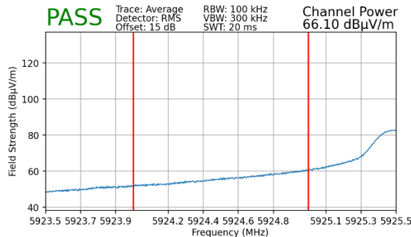
Plot 7-183. Radiated Lower Band Edge Plot MIMO (Average – UNII Band 5 – 106T)
