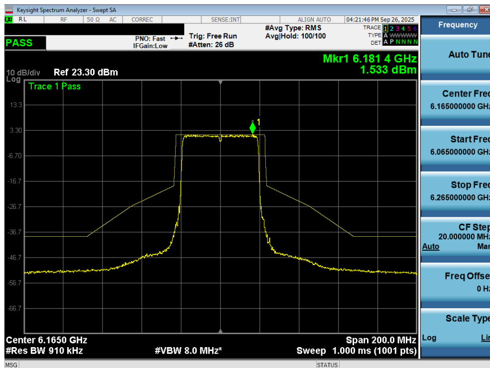
Plot 7-165. In Band Emissions Plot MIMO ANT2 (40MHz 802.11ax/be (Full Tones) (UNII Band 5) – Ch. 43) – SP
