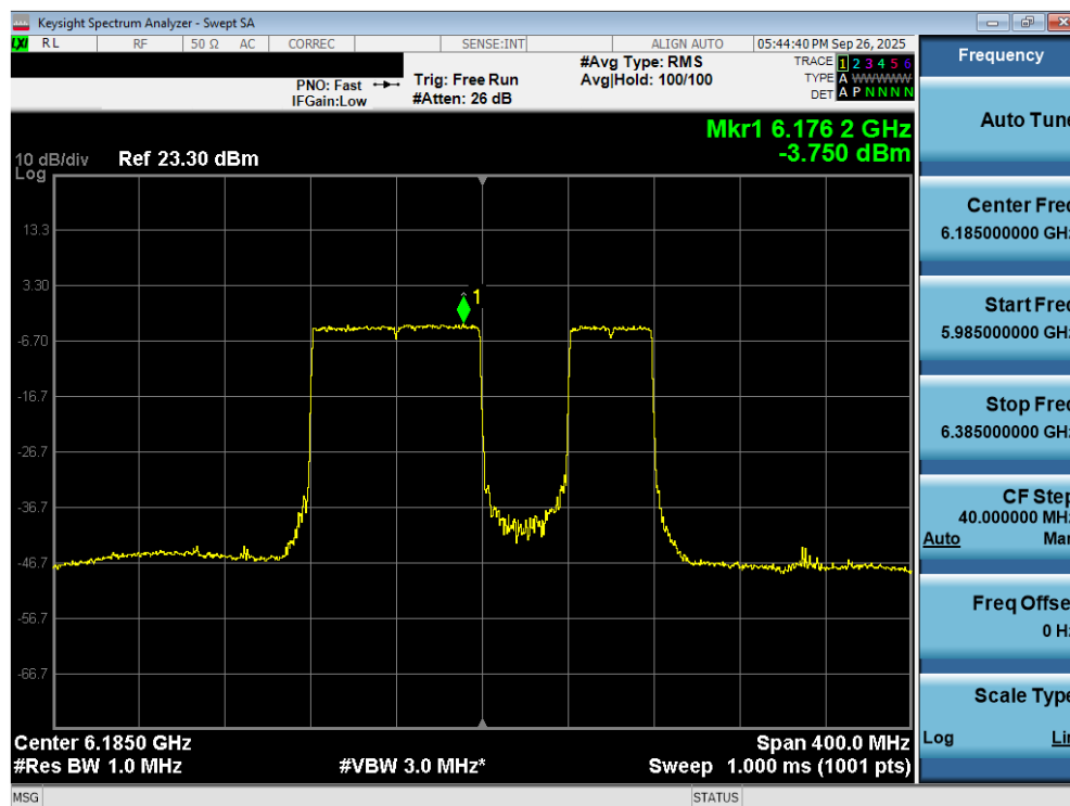
Plot 7-101. Power Spectral Density Plot MIMO ANT2 (160MHz 802.11be (996+484 Tones) (UNII Band 5) – Ch. 47) SP
