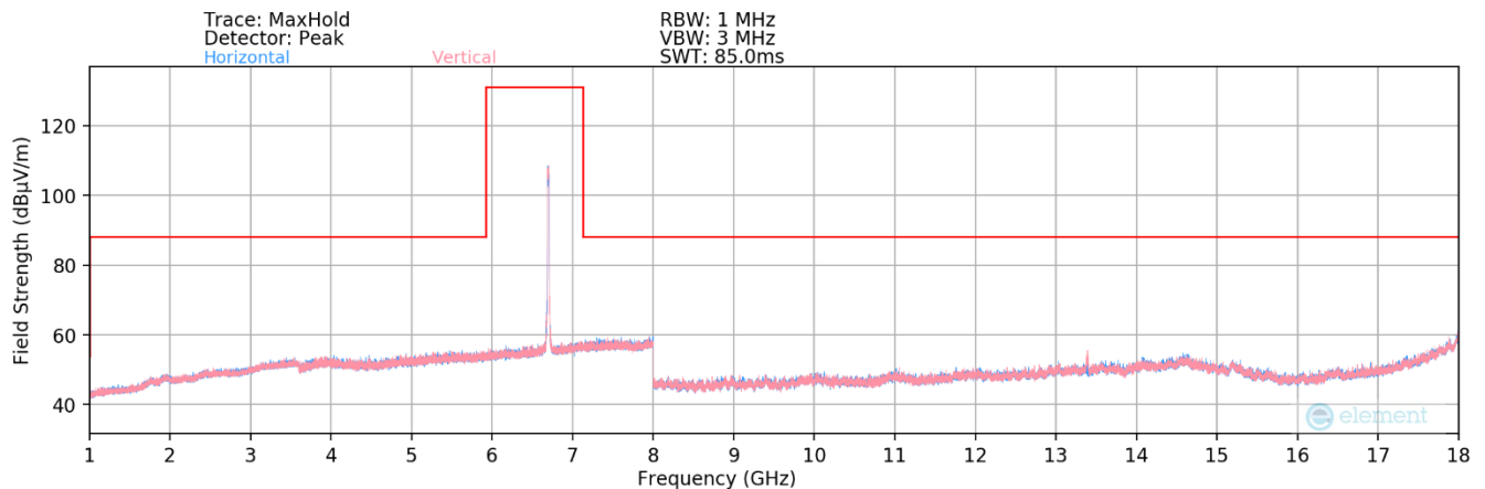
Plot 7-177. Radiated Spurious Plot 1GHz – 18GHz MIMO (802.11ax – UNII Band 7 Ch. 149)
