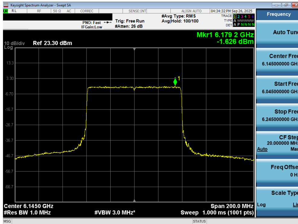
Plot 7-110. Power Spectral Density Plot MIMO Ant2 (80MHz 802.11ax/be (Full Tones) (UNII Band 5) – Ch. 39) - SP
