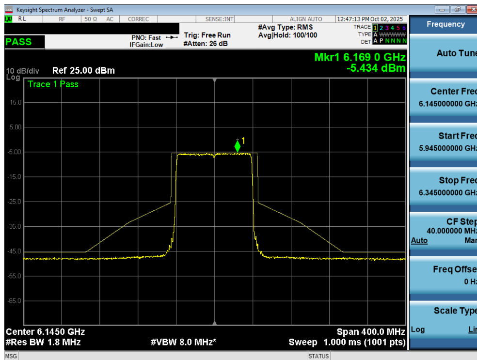
Plot 7-161. In Band Emissions Plot MIMO ANT2 (80MHz 802.11ax/be (Full Tones) (UNII Band 5) – Ch. 39) - LPI
