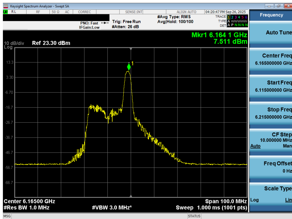
Plot 7-95. Power Spectral Density Plot MIMO ANT2 (40MHz 802.11ax/be (26 Tones) (UNII Band 5) – Ch. 43) - SP
