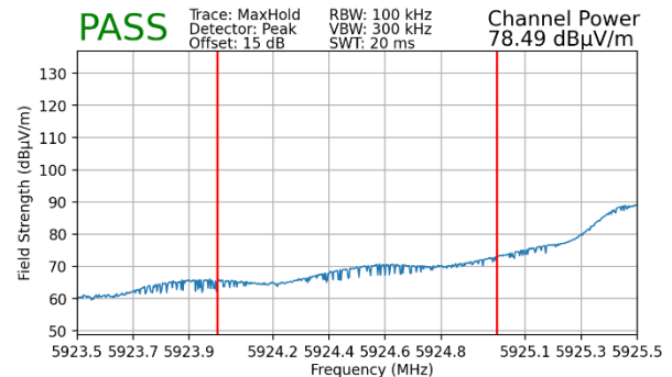
Plot 7-184. Radiated Lower Band Edge Plot MIMO (Peak – UNII Band 5 – 106T)
