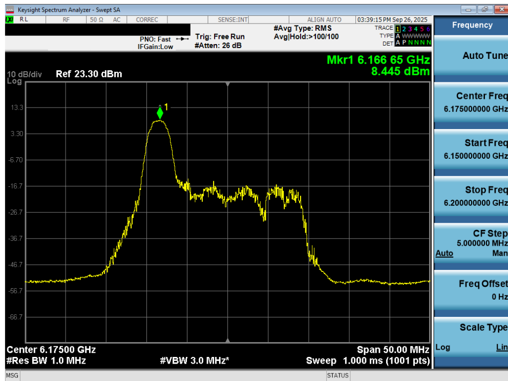
Plot 7-94. Power Spectral Density Plot MIMO ANT2 (20MHz 802.11ax/be (26 Tones) (UNII Band 5) – Ch. 45) - SP
