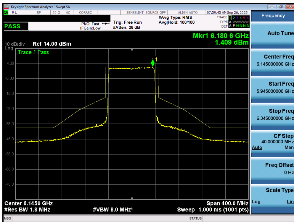
Plot 7-138. In Band Emissions Plot MIMO ANT1 (80MHz 802.11ax/be (Full Tones) (UNII Band 5) – Ch. 39) – SP
