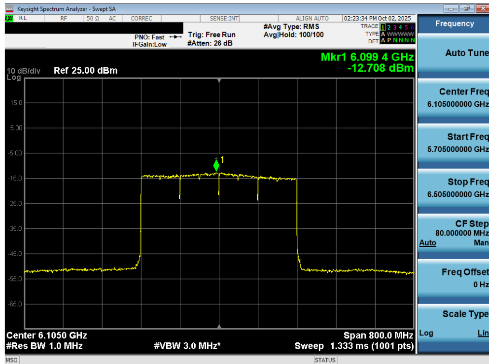
Plot 7-107. Power Spectral Density Plot MIMO ANT2 (320MHz 802.11be (Full Tones) (UNII Band 5) – Ch. 31) - LPI
