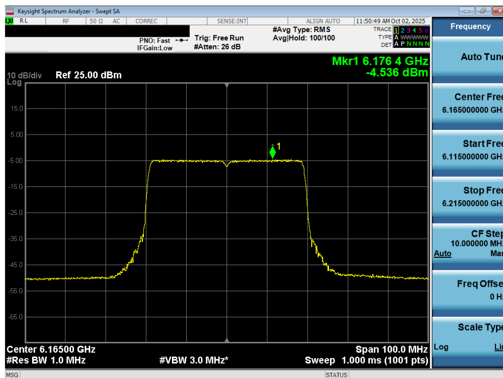
Plot 7-104. Power Spectral Density Plot MIMO ANT2 (40MHz 802.11ax/be (Full Tones) (UNII Band 5) – Ch. 43) - LPI
