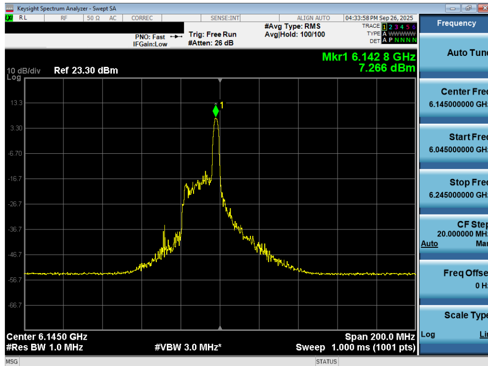
Plot 7-96. Power Spectral Density Plot MIMO ANT2 (80MHz 802.11ax/be (26 Tones) (UNII Band 5) – Ch. 39) – SP
