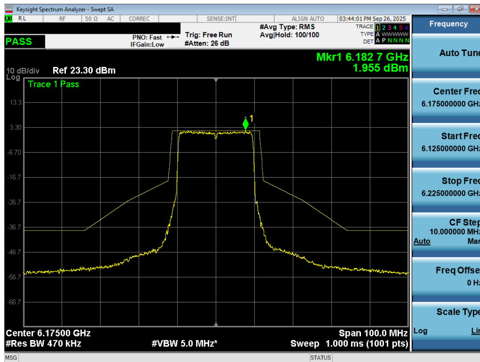
Plot 7-164. In Band Emissions Plot MIMO ANT2 (20MHz 802.11ax/be (Full Tones) (UNII Band 5) – Ch. 45) - SP
