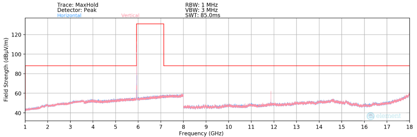
Plot 7-169. Radiated Spurious Plot 1GHz – 18GHz MIMO (802.11ax – UNII Band 5 Ch. 2)
