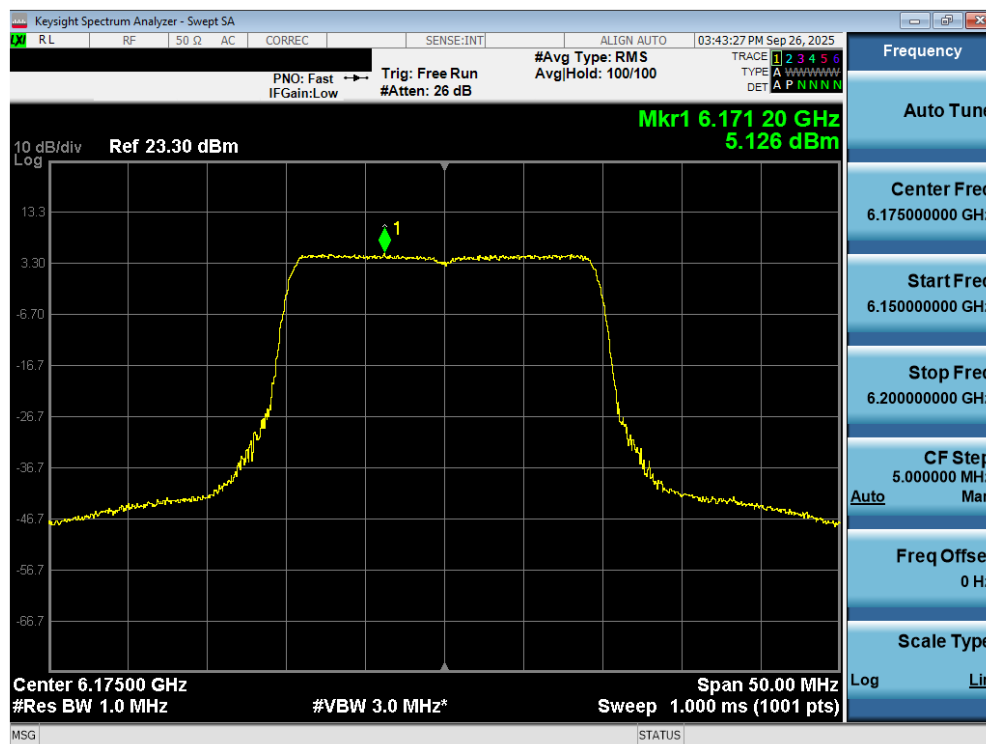
Plot 7-108. Power Spectral Density Plot MIMO ANT2 (20MHz 802.11ax/be (Full Tones) (UNII Band 5) – Ch. 45) - SP
