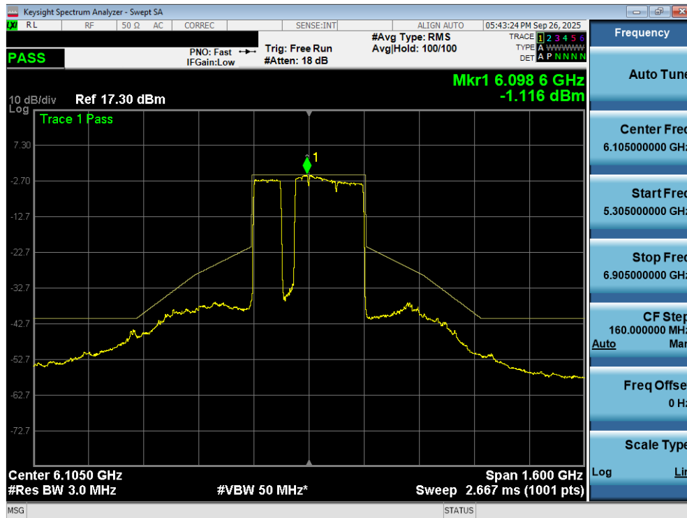
Plot 7-158. In Band Emissions Plot MIMO ANT2 (320MHz 802.11be (3*996+484 Tones) (UNII Band 5) – Ch. 31) SP
