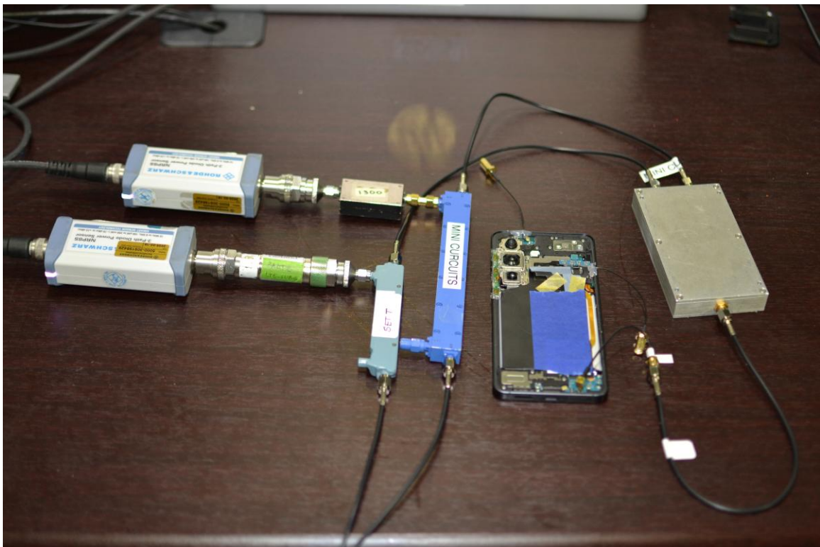
Test Setup Photo 6 – Conducted Test Setup (Figure 5.2-1d)
