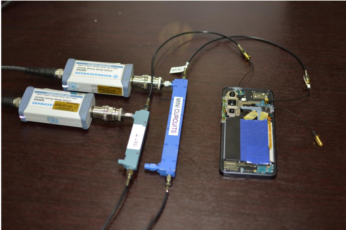
Test Setup Photo 5 – Conducted Test Setup (Figure 5.2-1c)
