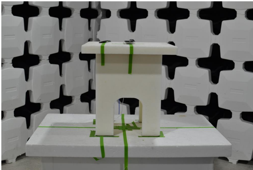
Figure 4. Test Setup – with WCP – 1GHz-40GHz
