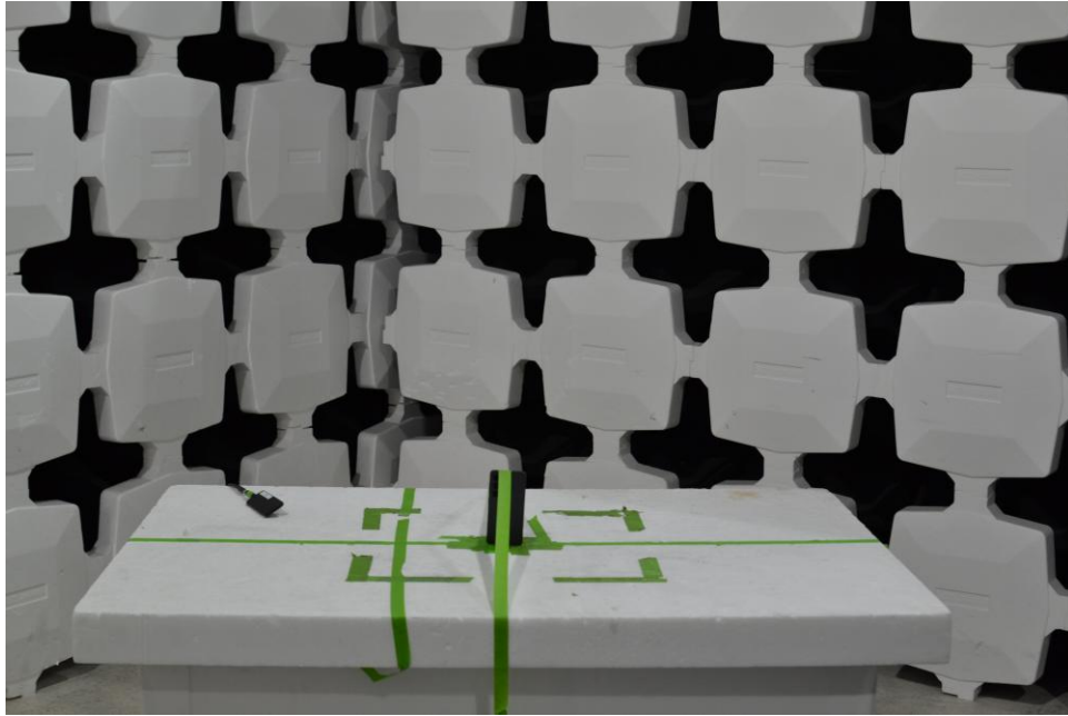
Figure 7. Test Setup – Z Position – 30MHz-1GHz
