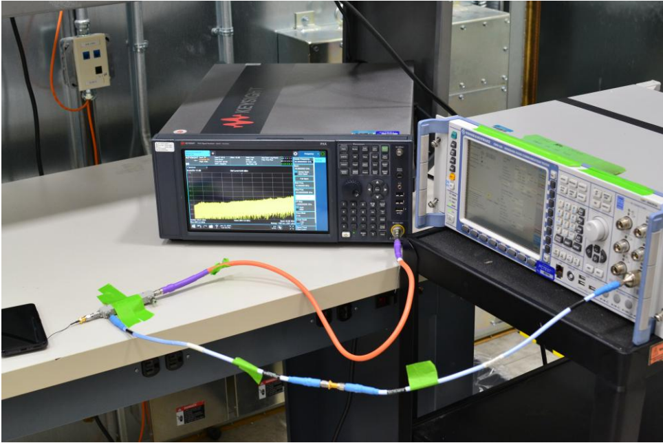
Figure 9. Conducted Test Setup – Online mode
