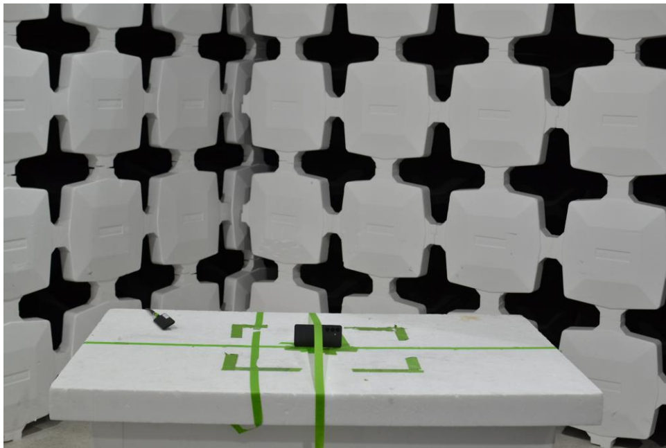
Figure 6. Test Setup – Y Position – 30MHz-1GHz
