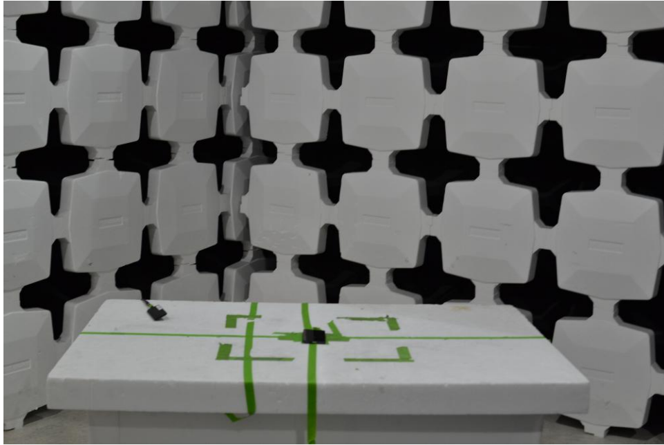
Figure 5. Test Setup – X Position – 30MHz-1GHz
