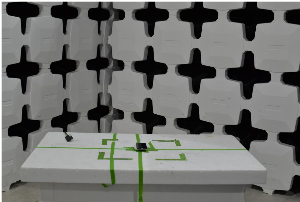
Figure 8. Test Setup – with WCP – 30MHz-1GHz
