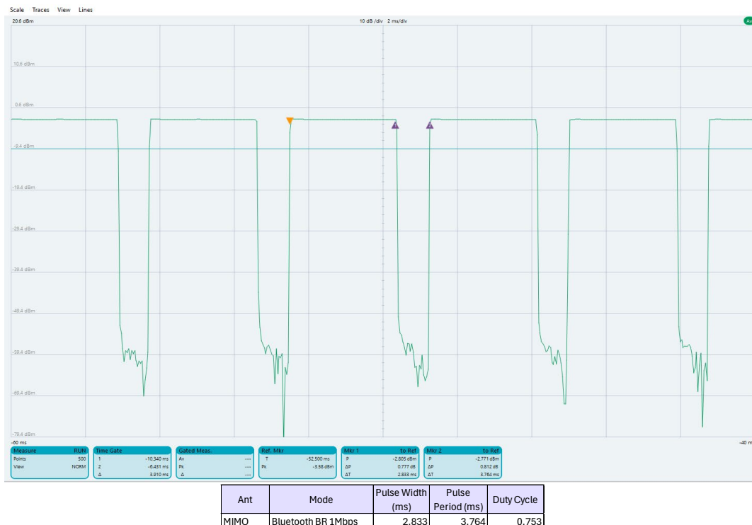
Figure 2-5 2.4 GHz Bluetooth MIMO (G&I) Duty Cycle Plot and Calculation
