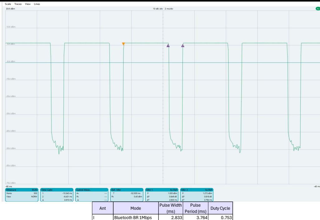
Figure 2-4 2.4 GHz Bluetooth Ant I Duty Cycle Plot and Calculation
