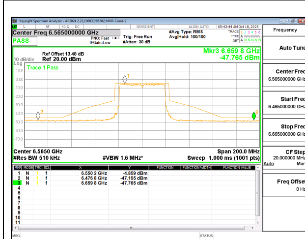
6565 MHz CHAIN 0
