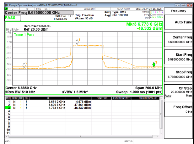
6685 MHz CHAIN 1
