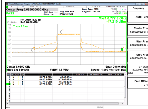
6685 MHz CHAIN 0
