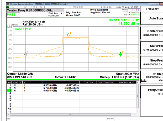
6845 MHz CHAIN 0
