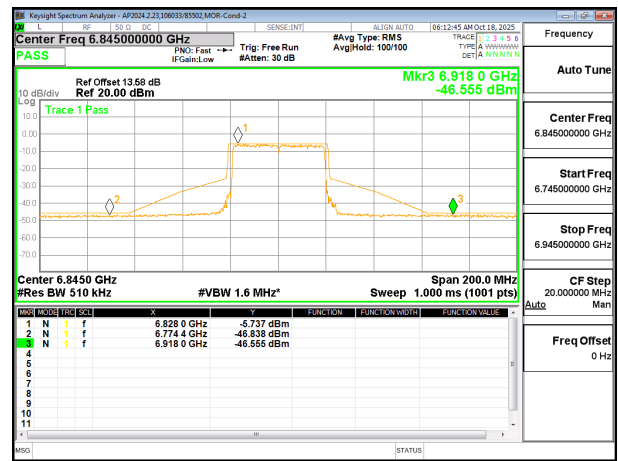
6845 MHz CHAIN 1
