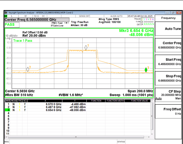
6565 MHz CHAIN 1
