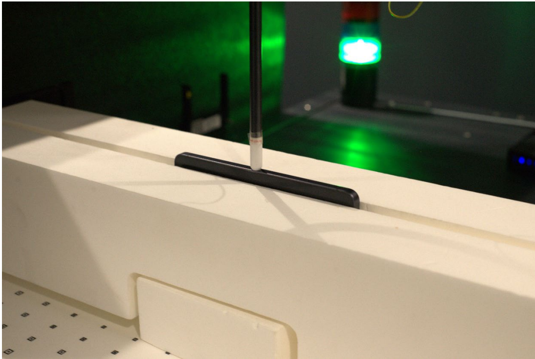
Figure 26 PD Test Setup – Body– Left Edge 2mm
