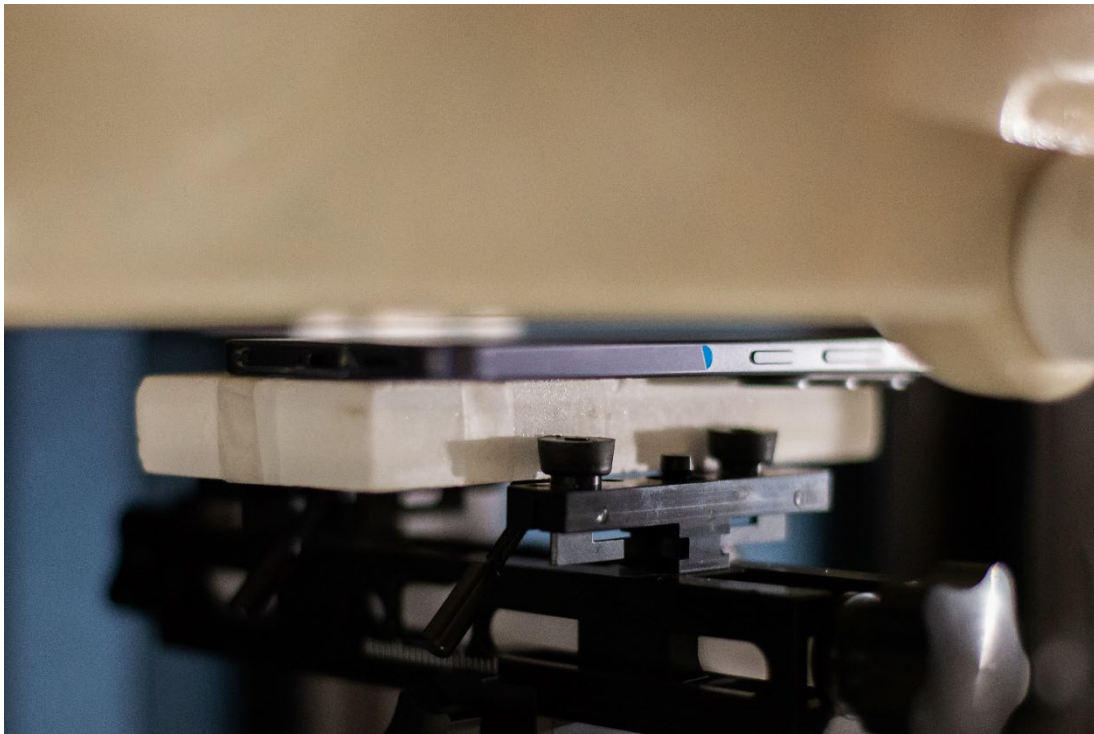
Figure 11 SAR Test Setup – Body-worn/Hotspot – Front 5mm
