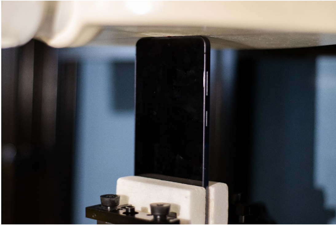
Figure 15 SAR Test Setup – Phablet – Top 0mm
