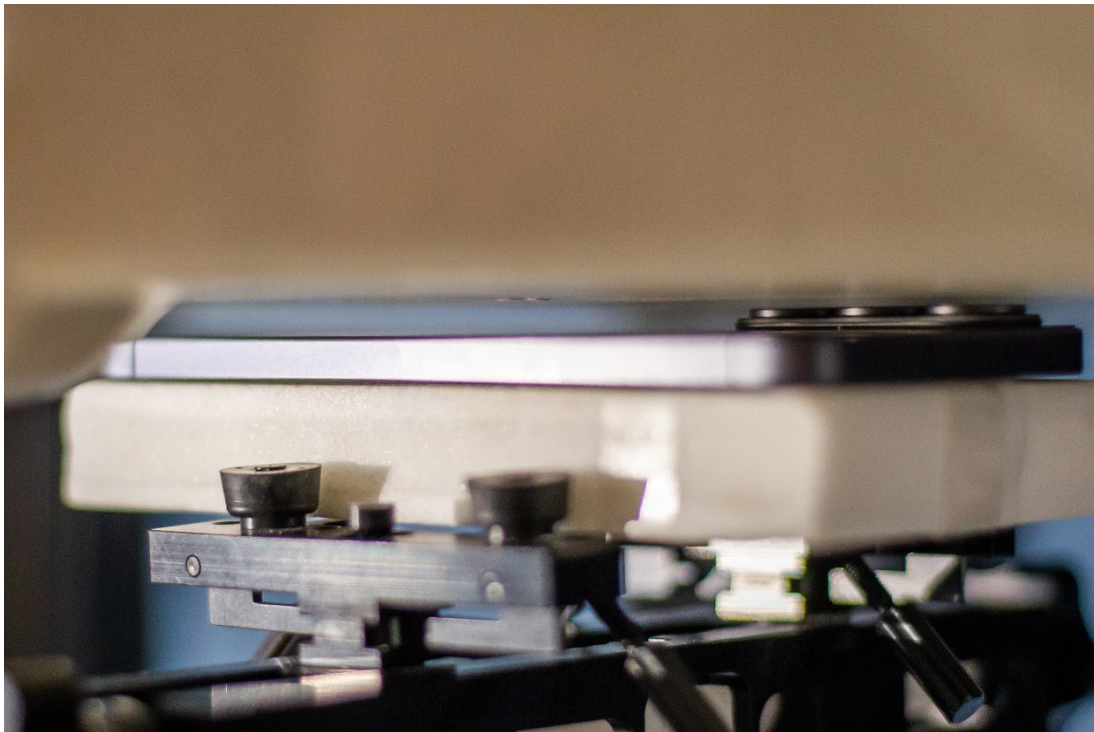
Figure 6 SAR Test Setup – Body-worn/Hotspot – Back 5mm
