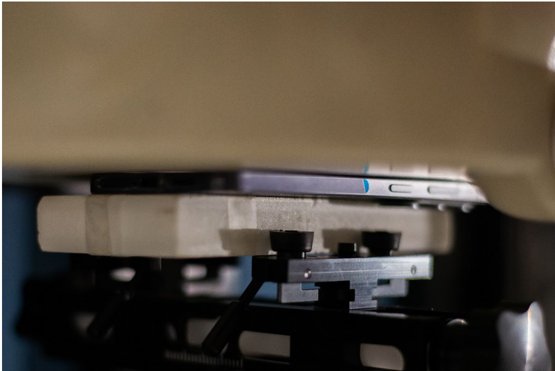
Figure 12 SAR Test Setup – Phablet – Front 0mm
