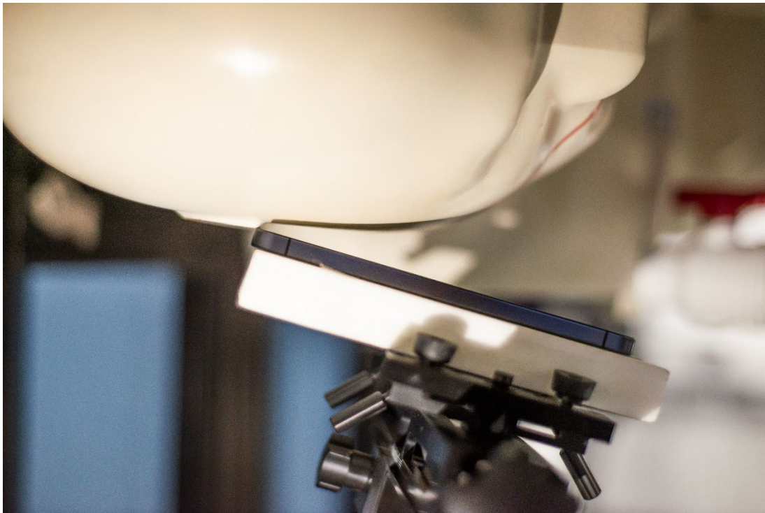
Figure 3 SAR Test Setup – Head – Right Tilt 0mm
