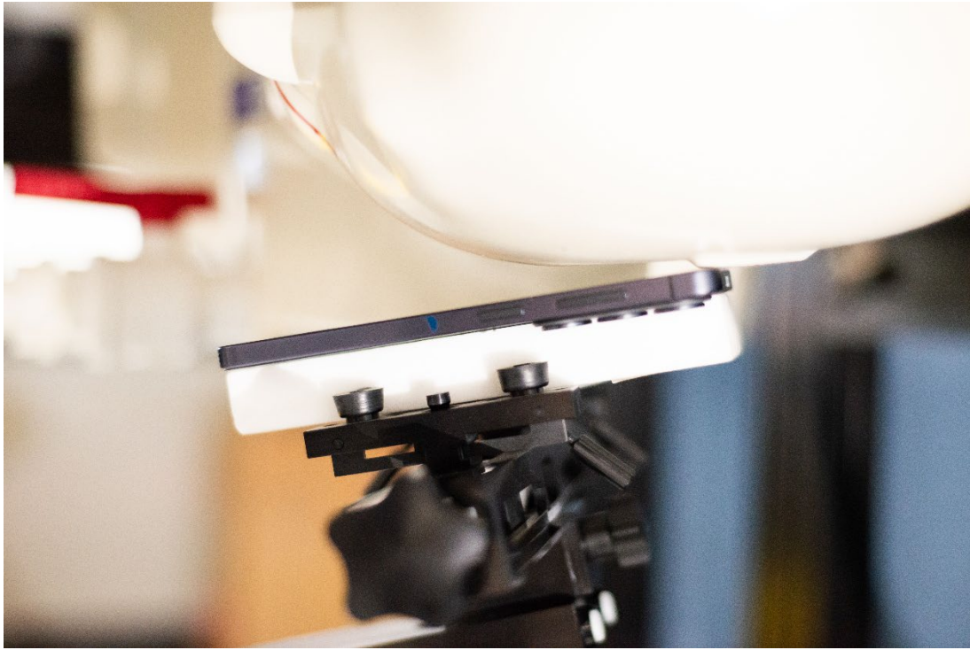
Figure 5 SAR Test Setup – Head – Left Tilt 0mm
