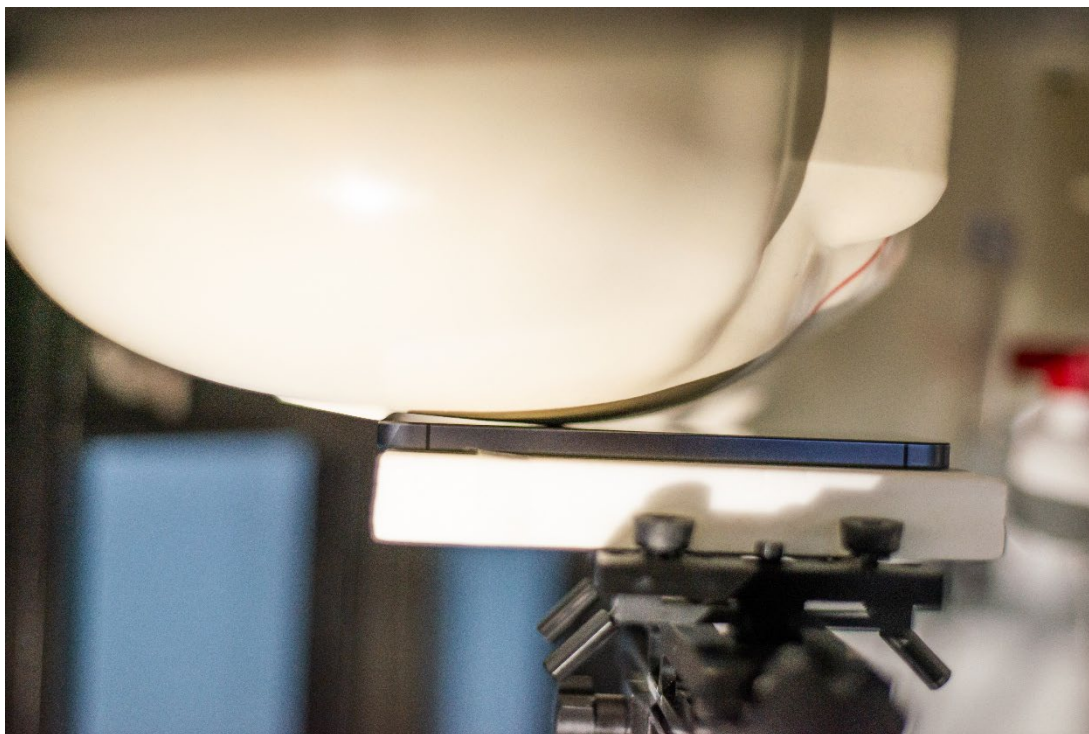
Figure 2 SAR Test Setup – Head – Right Cheek 0mm
