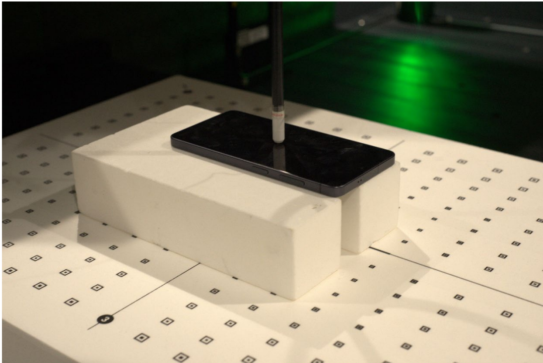
Figure 24 PD Test Setup – Body/Head– Front 2mm
