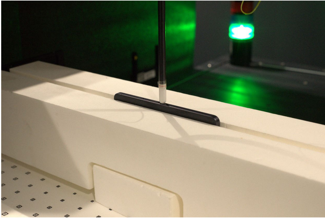
Figure 27 PD Test Setup – Body– Right Edge 2mm
