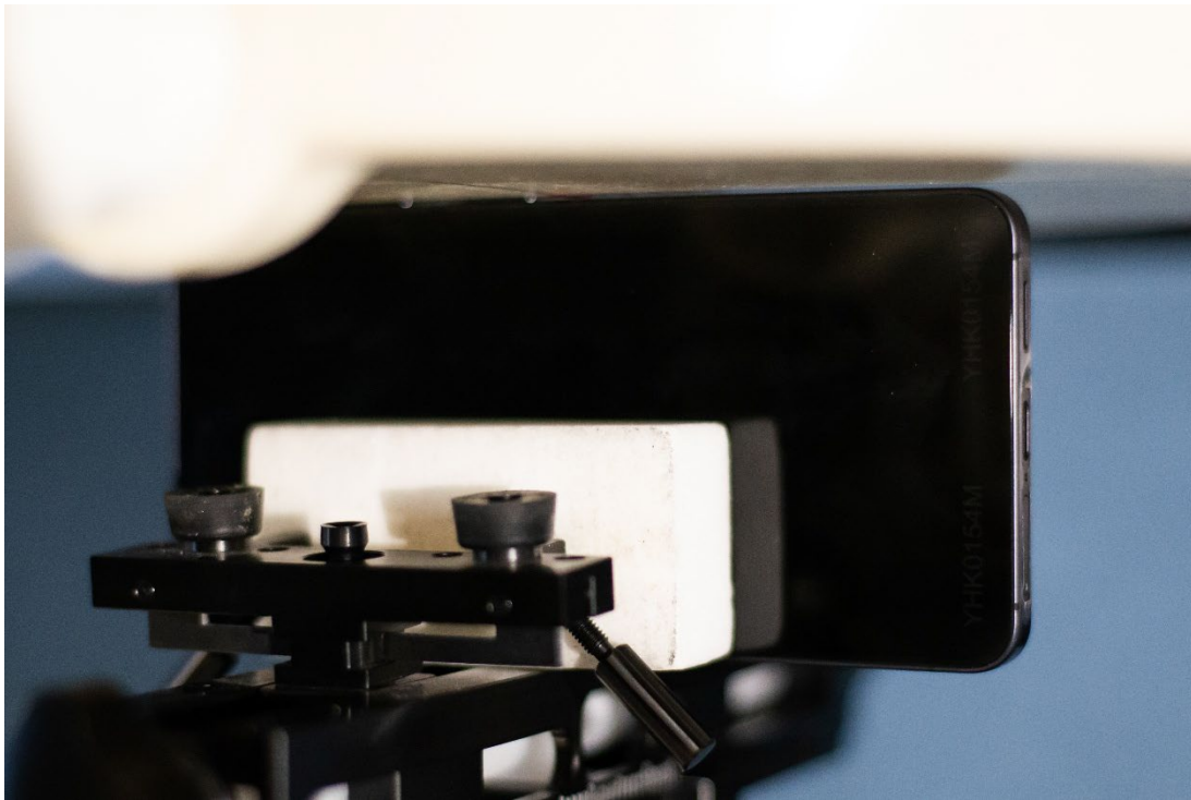
Figure 19 SAR Test Setup – Phablet – Right 0mm
