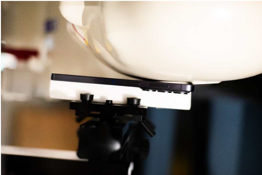
Figure 4 SAR Test Setup – Head – Left Cheek 0mm
