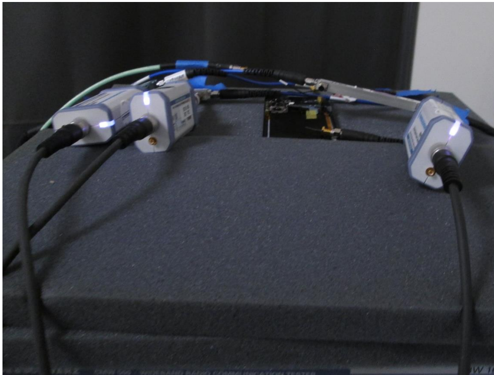
Figure 3 TAS Test Setup – Conducted Power Test Setup with Three Ports: System Continuity
