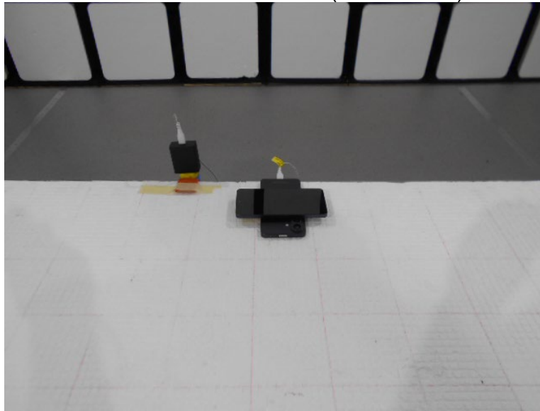
WPT RADIATED EMISSIONS SETUP (30-1000MHz)
