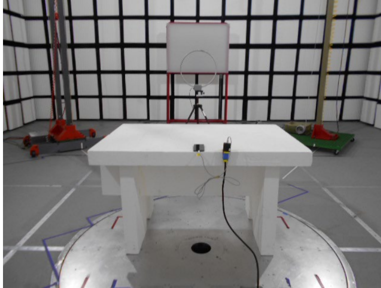
6 WLAN, NFC RADIATED EMISSIONS SETUP (<30MHz)
