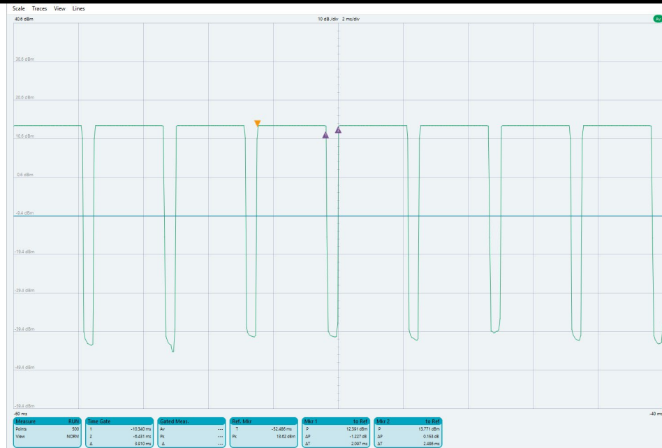
Figure 2-5 2.4 GHz Bluetooth LE MIMO (G&I) Duty Cycle Plot and Calculation
