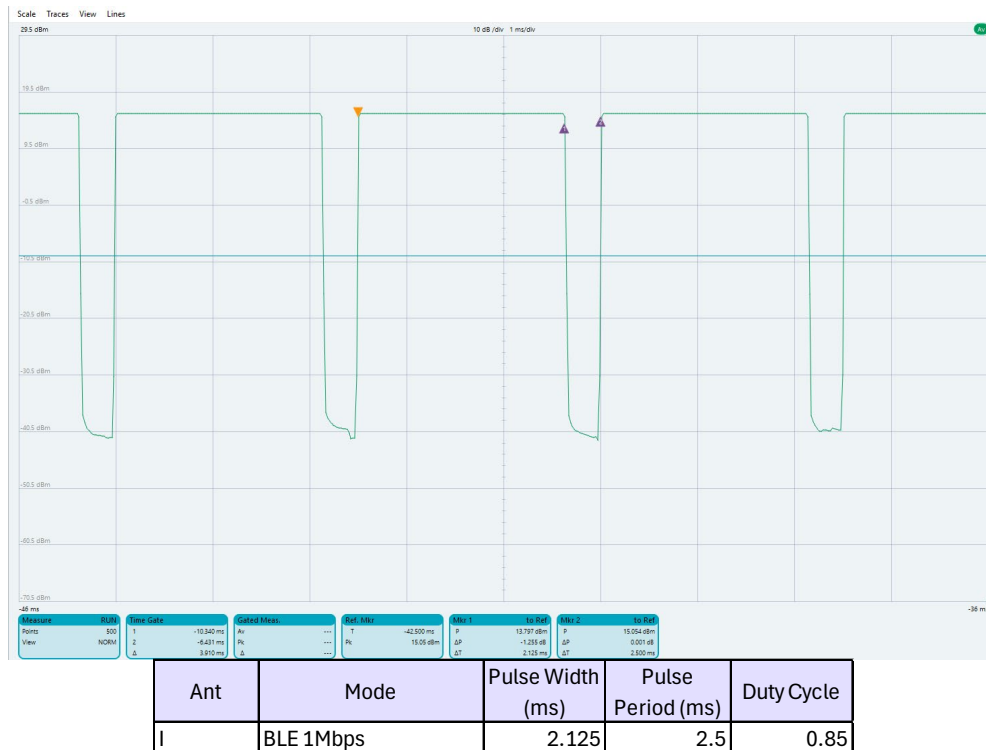
Figure 2-4 2.4 GHz Bluetooth LE Ant I Duty Cycle Plot and Calculation
