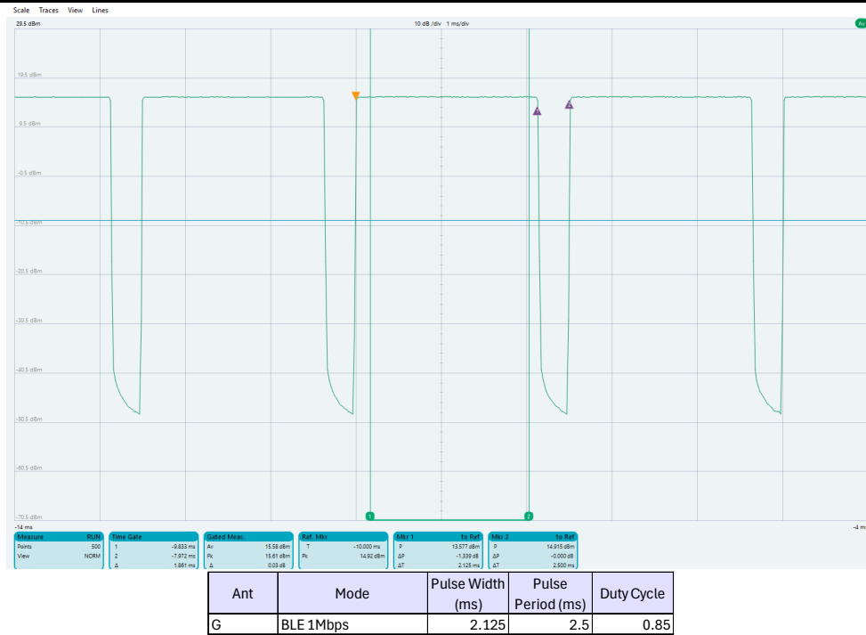
Figure 2-3 2.4 GHz Bluetooth LE Ant G Duty Cycle Plot and Calculation
