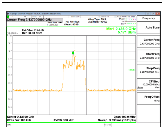
IN-BAND REFERENCE LEVEL ANTENNA 2
