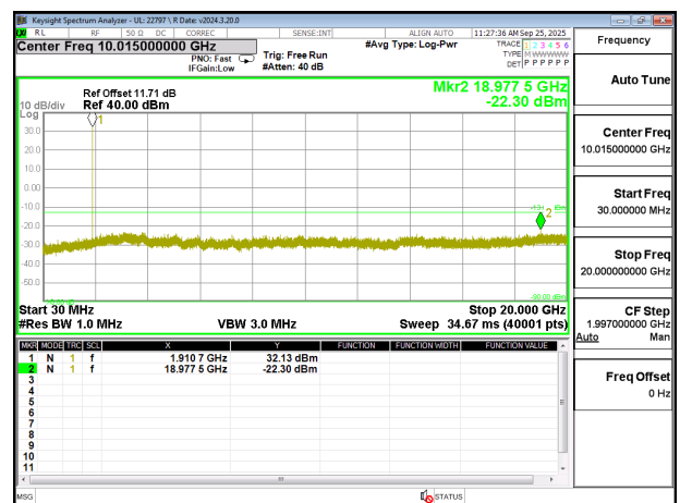
GSM1900 EGPRS HIGH Channel
