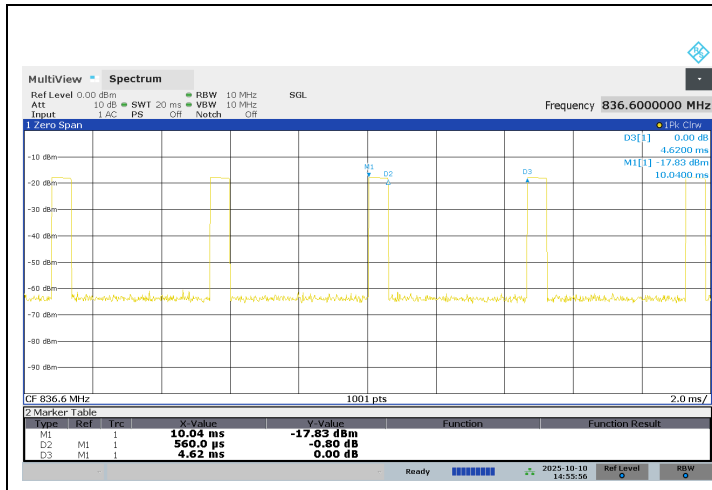
DUTY CYCLE GSM850 – 1 Time Slot
