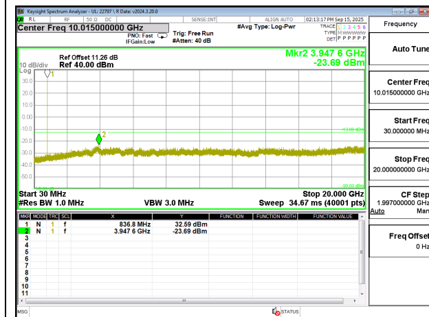
GSM850 GPRS MID Channel
