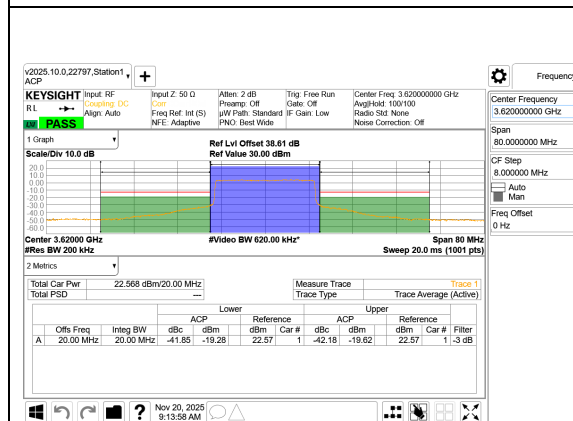
LTE B48 20MHz QPSK Mid Channel RB100-0
