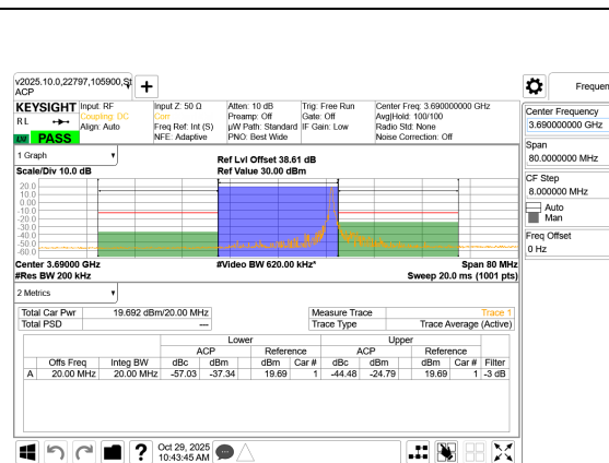
LTE B48 20MHz QPSK High Channel RB1-99
