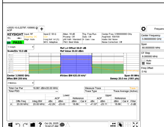
LTE B48 20MHz QPSK Low Channel RB100-0
