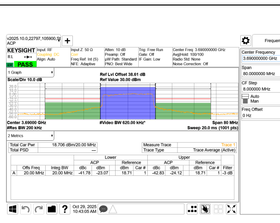
LTE B48 20MHz QPSK High Channel RB100-0
