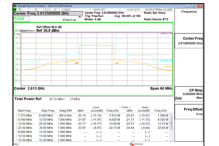
LTE B38 15MHz QPSK High Channel RB75-0
