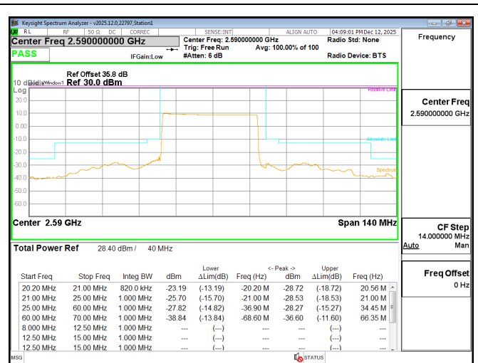
5G NR N38 40MHz BPSK Low Channel RB100-0
