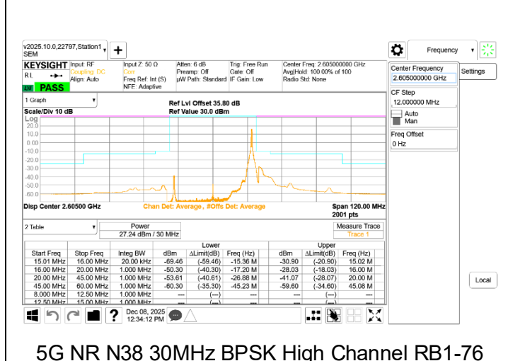
5G NR N38 30MHz BPSK High Channel RB1-76
