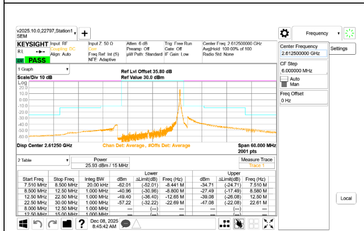
LTE B38 15MHz QPSK High Channel RB1-74
