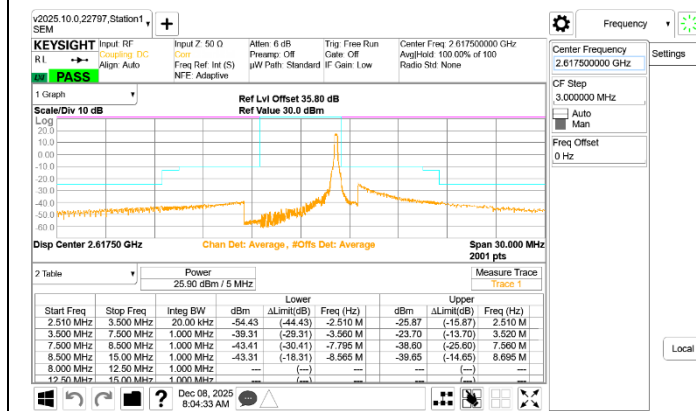
LTE B38 5MHz QPSK High Channel RB1-24
