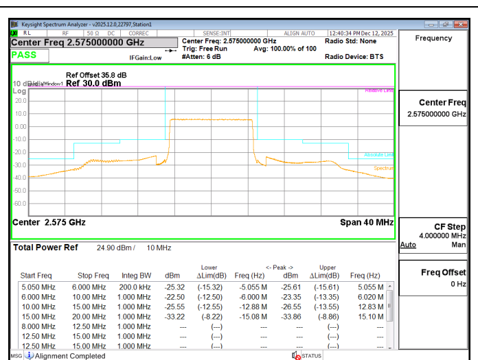
LTE B38 10MHz QPSK Low Channel RB50-0
