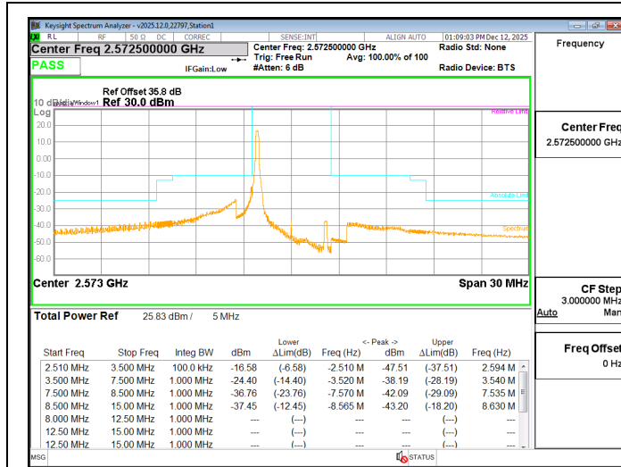
LTE B38 5MHz QPSK Low Channel RB1-0
