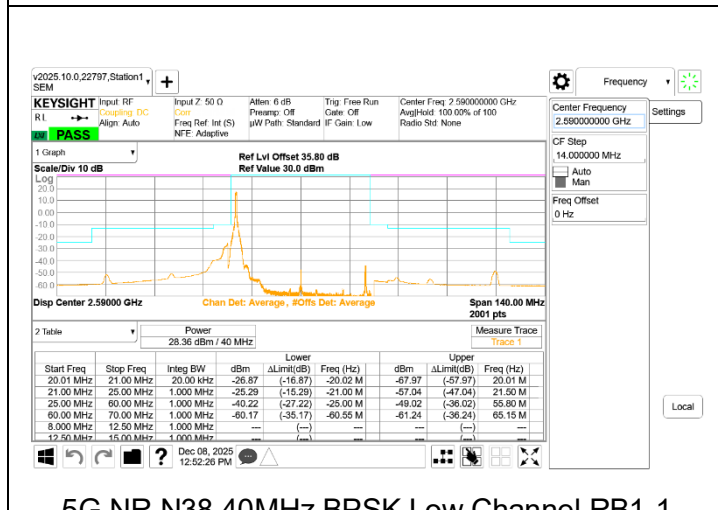
5G NR N38 40MHz BPSK Low Channel RB1-1
