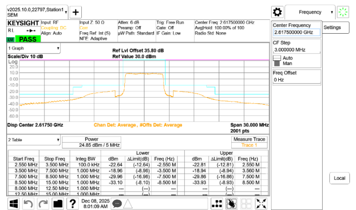
LTE B38 5MHz QPSK High Channel RB25-0
