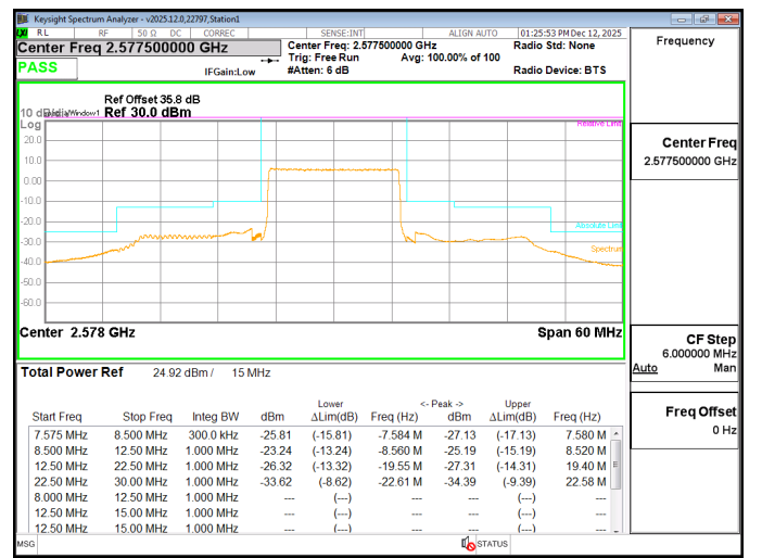
LTE B38 15MHz QPSK Low Channel RB75-0
