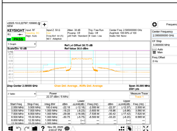
LTE B41 5MHz QPSK Middle Channel RB25-0
