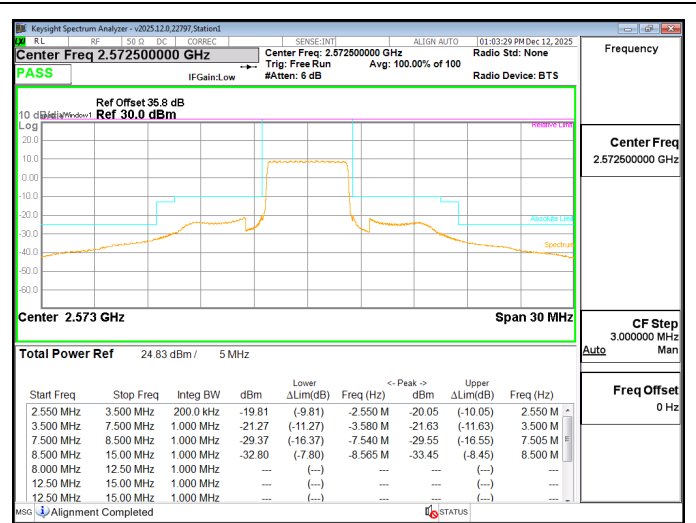
LTE B38 5MHz QPSK Low Channel RB25-0
