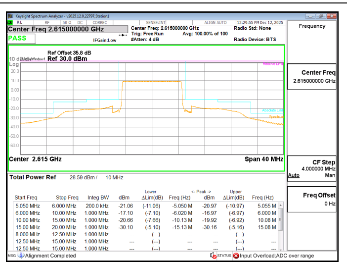
LTE B38 10MHz QPSK High Channel RB50-0
