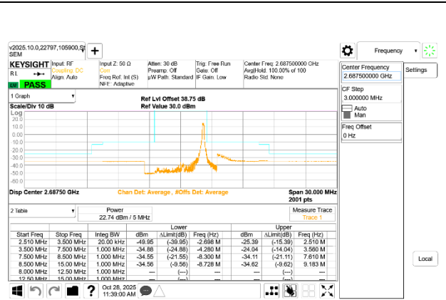
LTE B41 5MHz QPSK High Channel RB1-24
