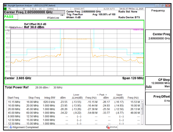
5G NR N38 30MHz BPSK High Channel RB75-0
