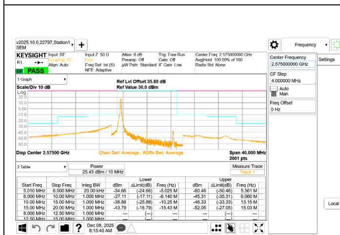
LTE B38 10MHz QPSK Low Channel RB1-0
