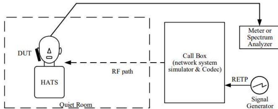
Figure 3.4 Volume Control Test Setup
