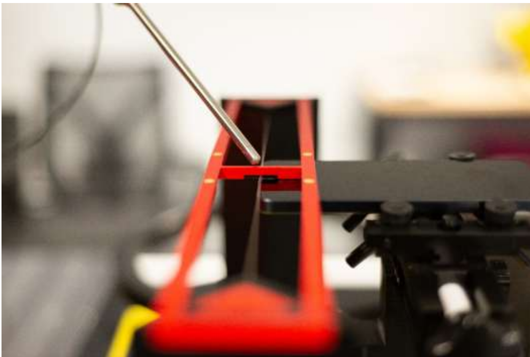
Figure D.2 HAC T-Coil Test Setup Photos 2
