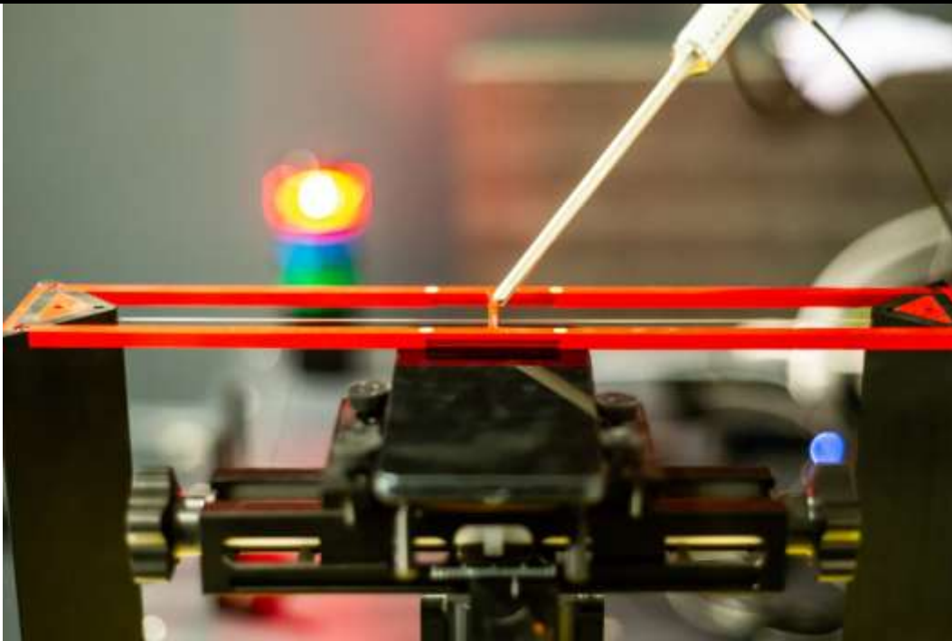
Figure D.1 HAC T-Coil Test Setup Photos 1
