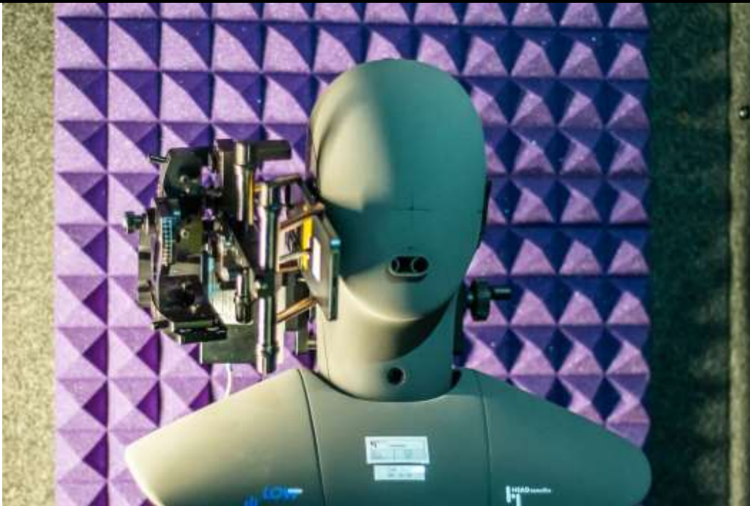
Figure D.1 HAC Volume Control Test Setup Photos 1
