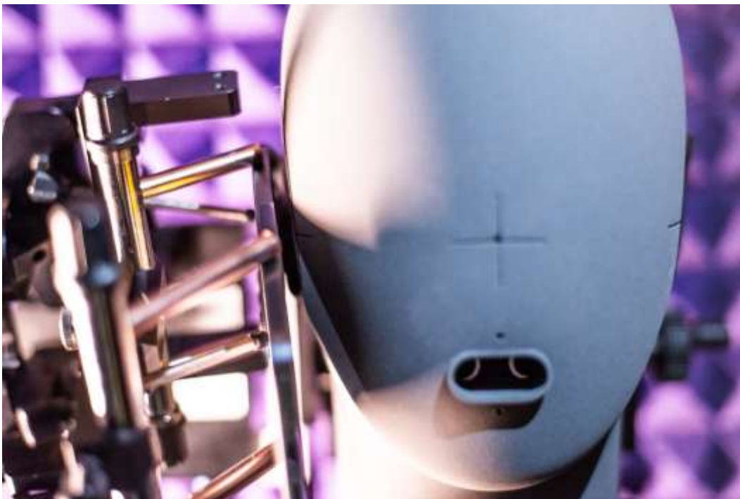
Figure D.2 HAC Volume Control Test Setup Photos 2
