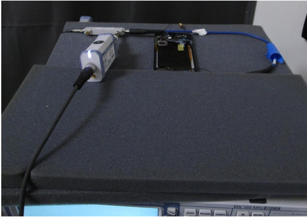
Figure 1 TAS Test Setup – Conducted Power Test Setup with Single Port
