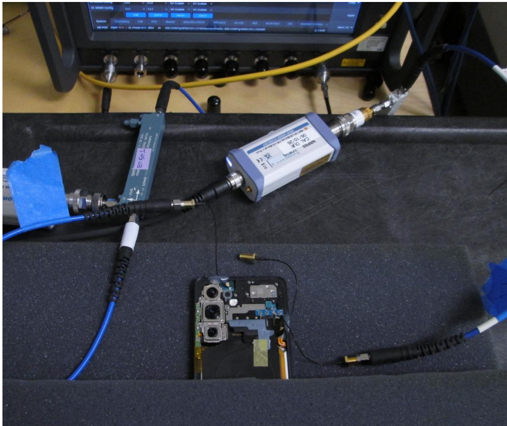
Figure 3 TAS Test Setup – Conducted Power Test Setup with Two Ports: ENDC
