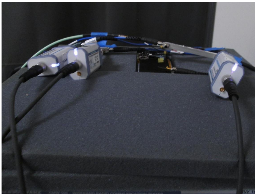
Figure 4 TAS Test Setup – Conducted Power Test Setup with Three Ports: System Continuity
