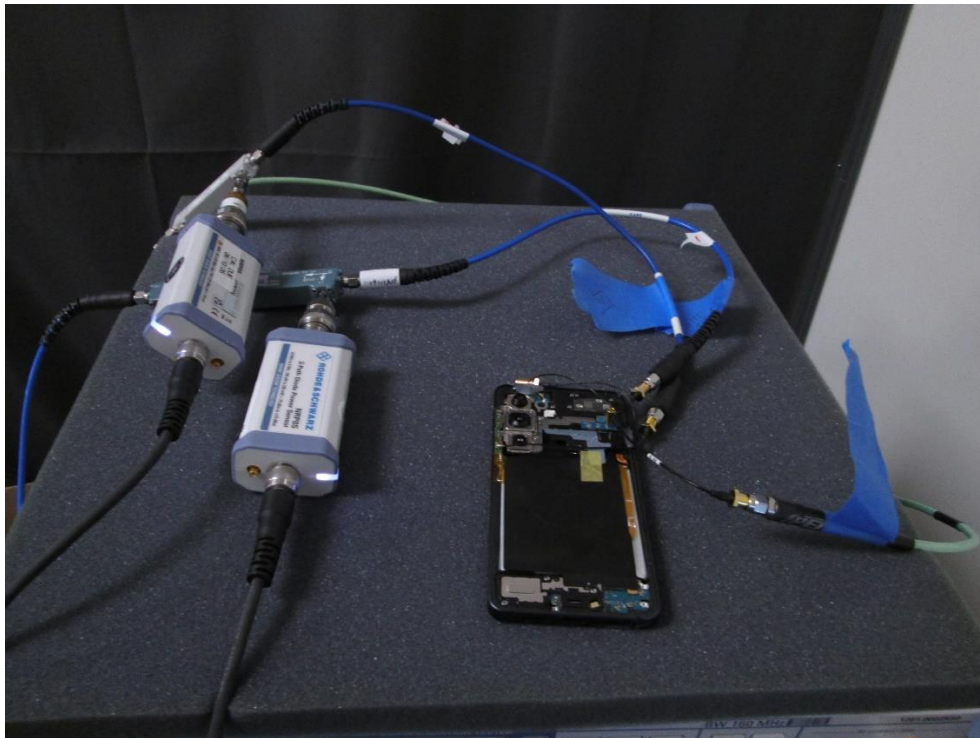
Figure 2 TAS Test Setup – Conducted Power Test Setup with Two Ports
