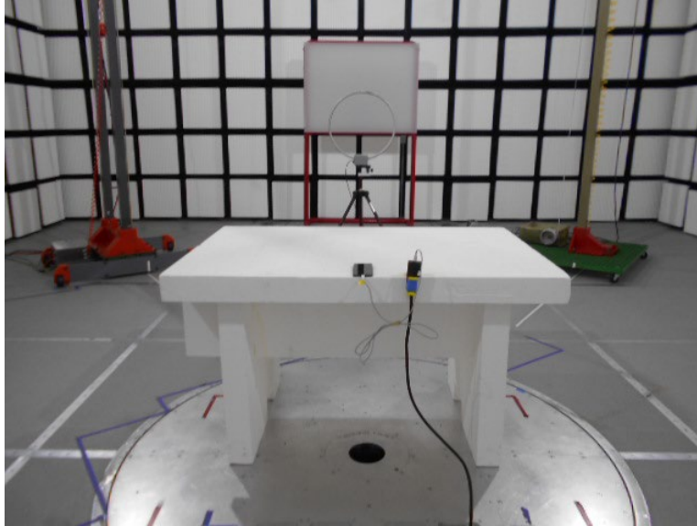
BT C0/BLE C0/5 WLAN/6 WLAN RADIATED EMISSIONS SETUP (<30MHz)
