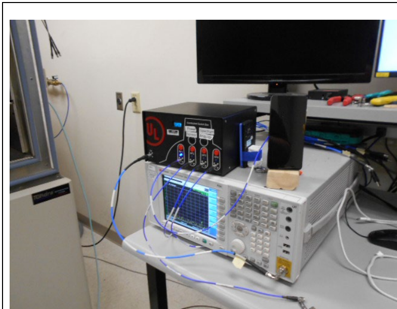
BT, BLE, 2.4/5/6 WLAN CONDUCTED SETUP
