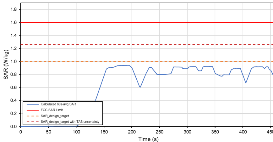
Total Time-Averaged SAR Test Sequence B Tech: LTE, Band 5
