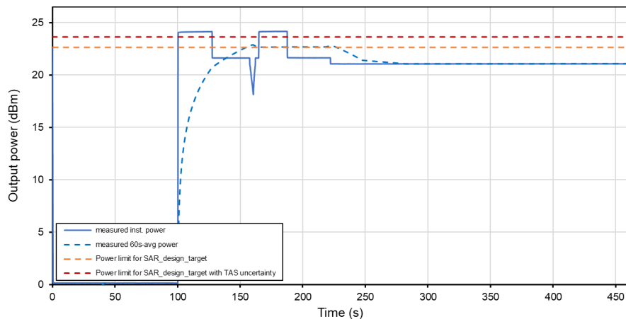
Time-Averaged Conducted Power Test Sequence A Tech: WCDMA, Band 5
