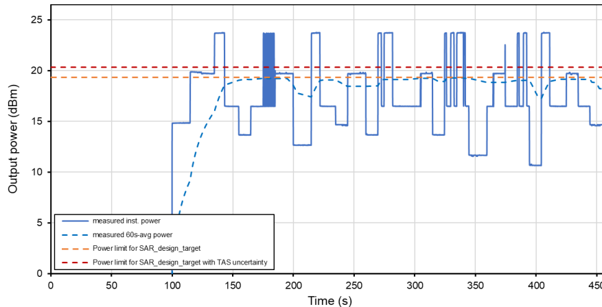
Time-Averaged Conducted Power Test Sequence B Tech: NR, Band n5
