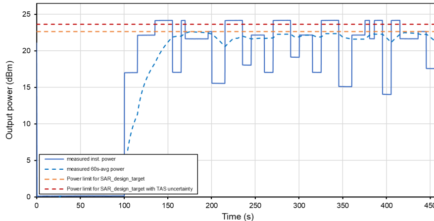
Time-Averaged Conducted Power Test Sequence B Tech: WCDMA, Band 5
