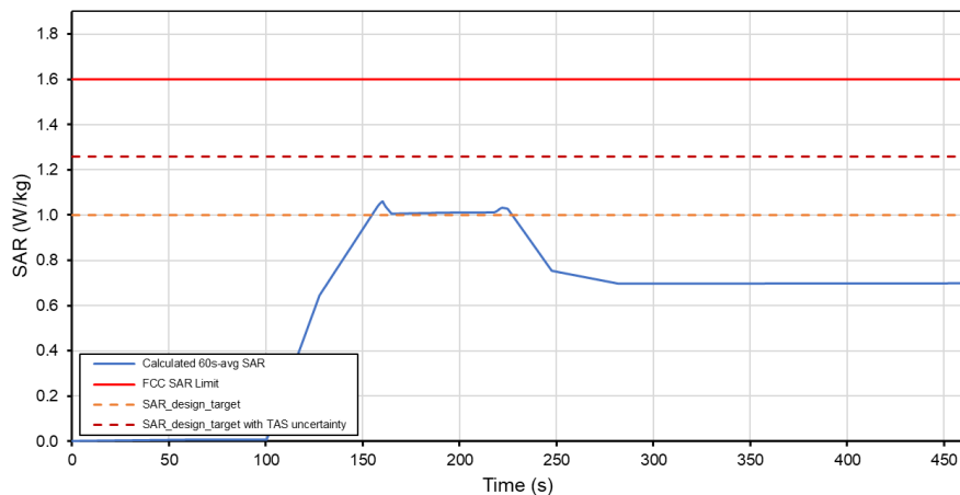
Total Time-Averaged SAR Test Sequence A Tech: WCDMA, Band 5
