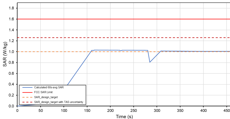
Total Time-Averaged SAR Test Sequence A Tech: LTE, Band 41
