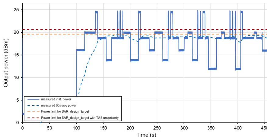
Time-Averaged Conducted Power Test Sequence B Tech: GSM, Band 850
