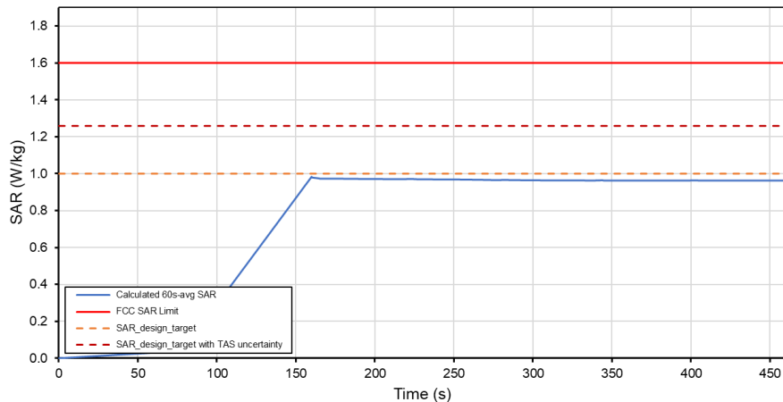
Total Time-Averaged SAR Test Sequence A Tech: NR, Band 77
