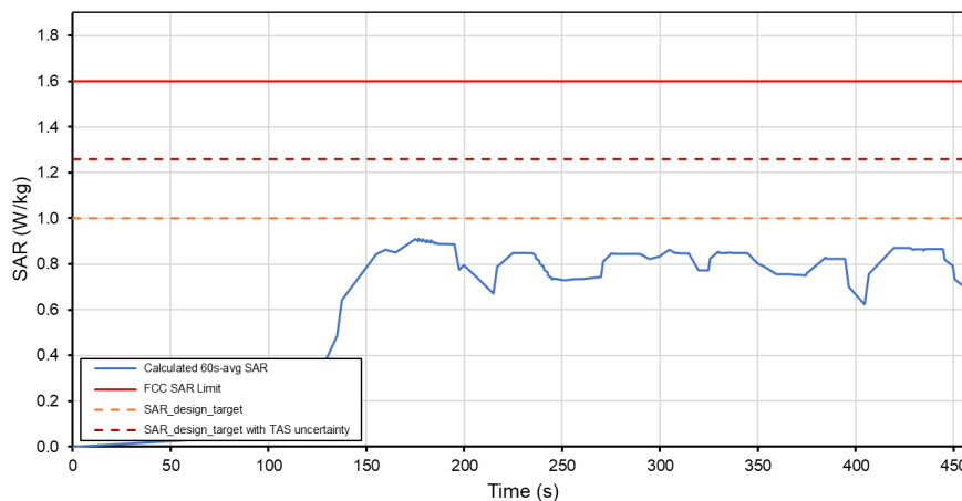
Total Time-Averaged SAR Test Sequence B Tech: NR, Band 77
