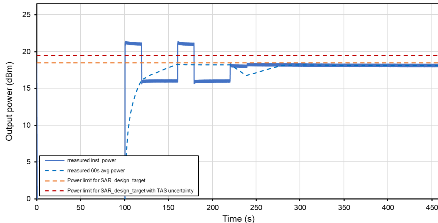
Time-Averaged Conducted Power Test Sequence A Tech: GSM, Band 1900
