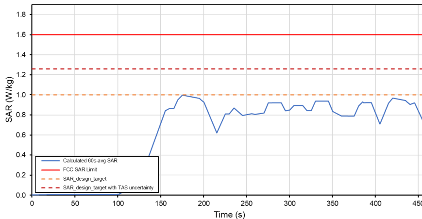
Total Time-Averaged SAR Test Sequence B Tech: WCDMA, Band 5
