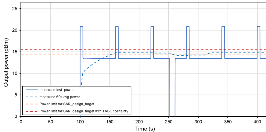
Time-Averaged Conducted Power Dropped Connection Tech: NR, Band 77
