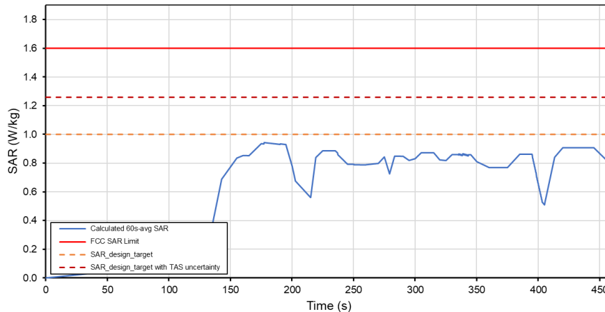
Total Time-Averaged SAR Test Sequence B Tech: LTE, Band 41
