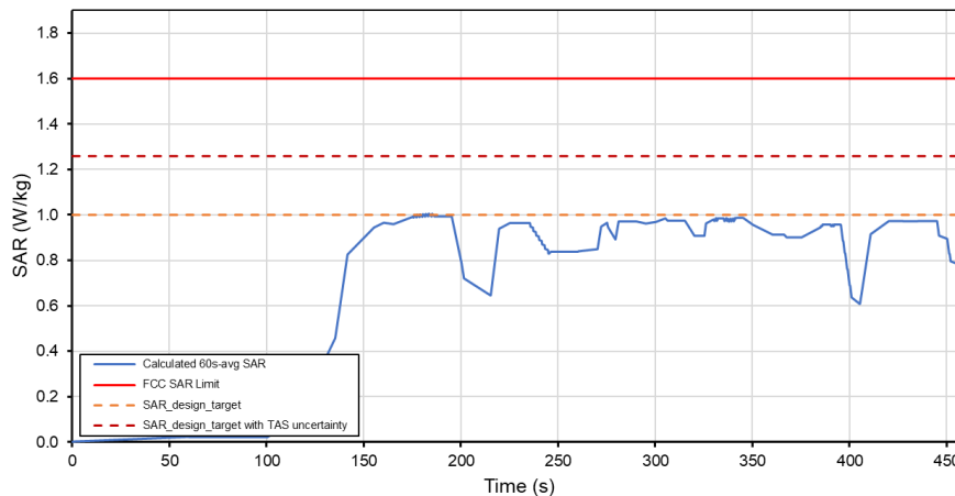
Total Time-Averaged SAR Test Sequence B Tech: WCDMA, Band 2
