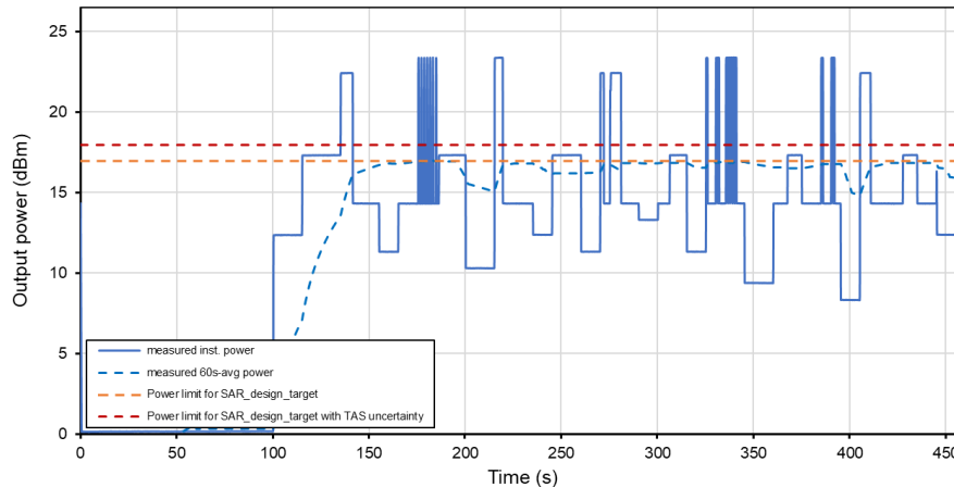
Time-Averaged Conducted Power Test Sequence B Tech: WCDMA, Band 2
