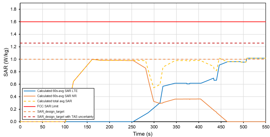
Total Time-Averaged SAR Exposure Switching Tech: LTE, Band 5 / NR Band n66
