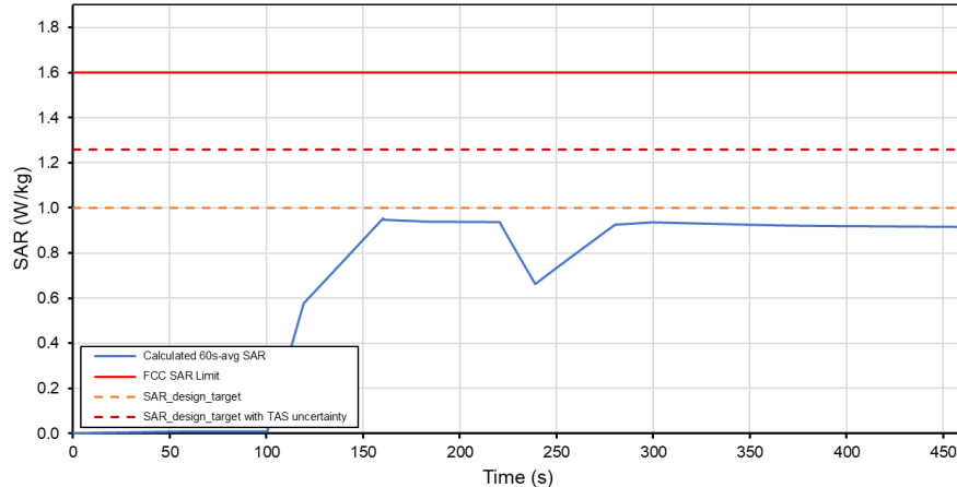
Total Time-Averaged SAR Test Sequence A Tech: GSM, Band 1900
