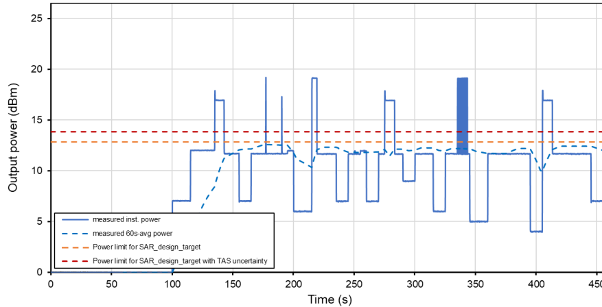
Time-Averaged Conducted Power Test Sequence B Tech: LTE, Band 41 PC3
