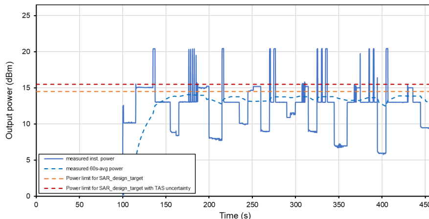
Time-Averaged Conducted Power Test Sequence B Tech: NR, Band 77
