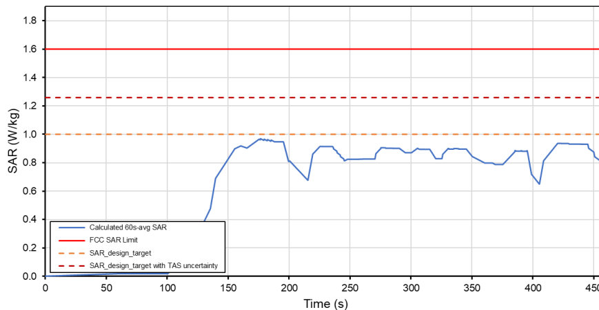
Total Time-Averaged SAR Test Sequence B Tech: GSM, Band 850
