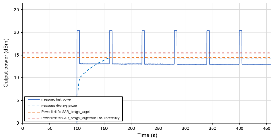
Time-Averaged Conducted Power Test Sequence A Tech: NR, Band 77
