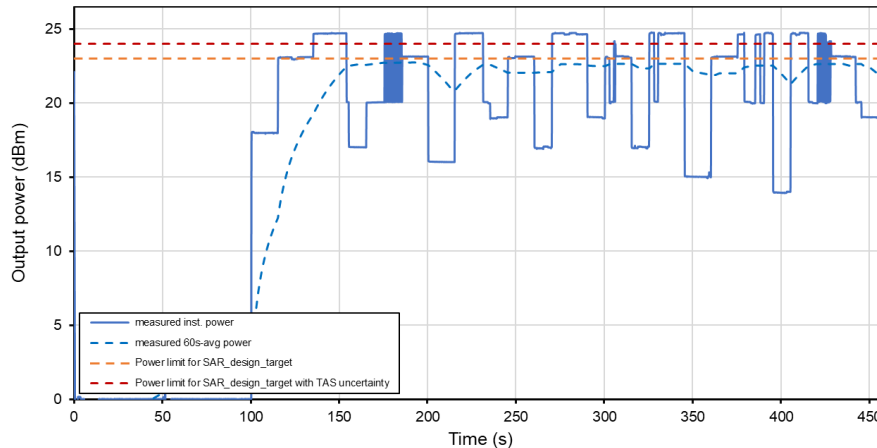
Time-Averaged Conducted Power Test Sequence B Tech: LTE, Band 5
