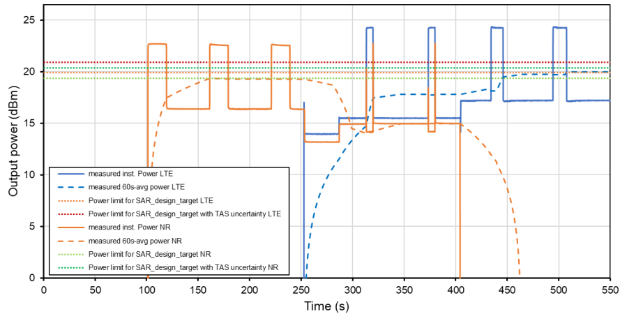
Time-Averaged Conducted Power SAR Exposure Switching Tech: LTE, Band 5 / NR Band n66
