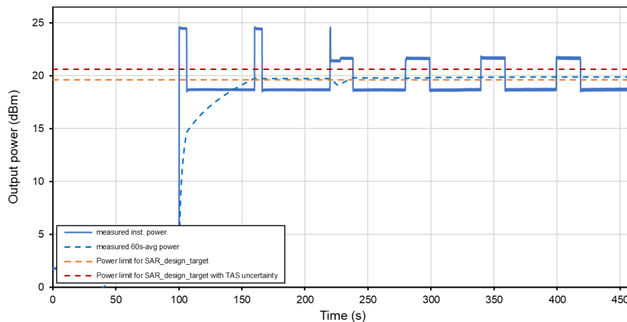
Time-Averaged Conducted Power Test Sequence A Tech: GSM, Band 850
