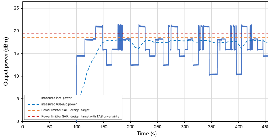
Time-Averaged Conducted Power Test Sequence B Tech: GSM, Band 1900
