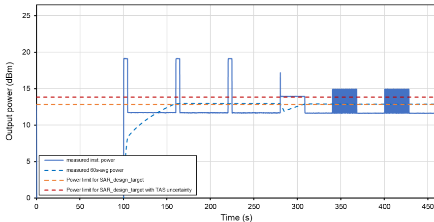
Time-Averaged Conducted Power Test Sequence A Tech: LTE, Band 41 PC3
