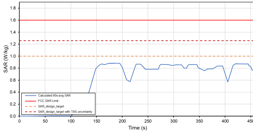
Total Time-Averaged SAR Test Sequence B Tech: GSM, Band 1900
