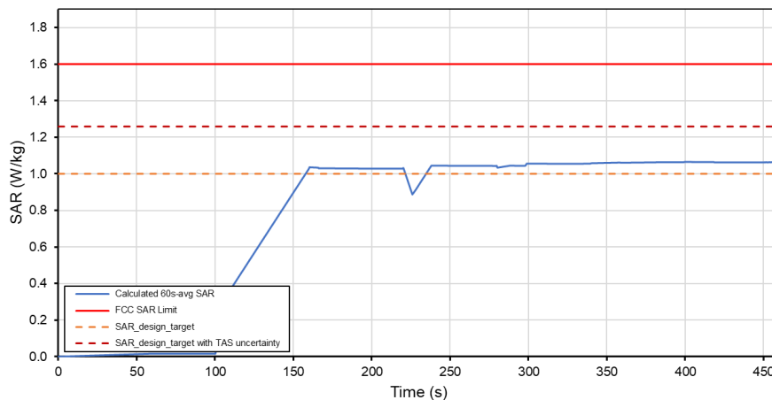
Total Time-Averaged SAR Test Sequence A Tech: GSM, Band 850
