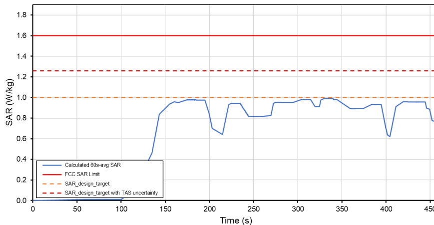
Total Time-Averaged SAR Test Sequence B Tech: NR, Band n5
