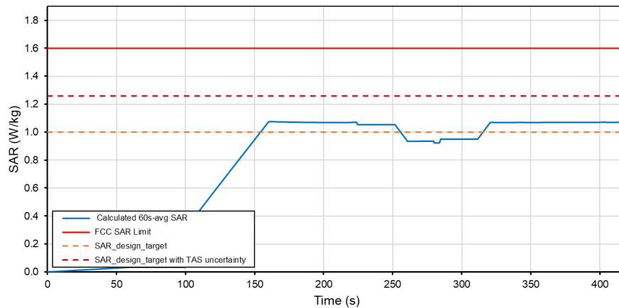
Total Time-Averaged SAR Dropped Connection Tech: NR, Band 77
