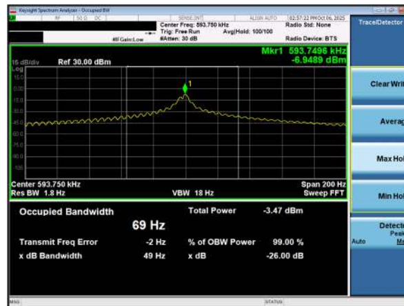
Figure 1-1 Digitizer Occupied Bandwidth
