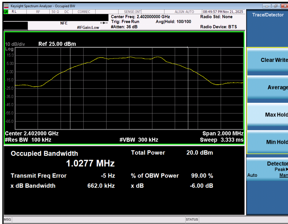
Plot 7-25. 6dB Bandwidth Plot (Bluetooth (LE), 1Mbps – Ch. 37) – Dual Ant 1
