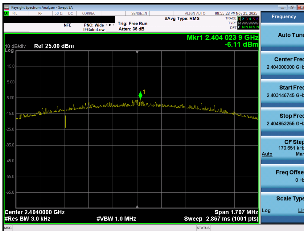
Plot 7-100. Power Spectral Density Plot (Bluetooth (LE), 2Mbps – Ch. 0) – Dual Ant 1
