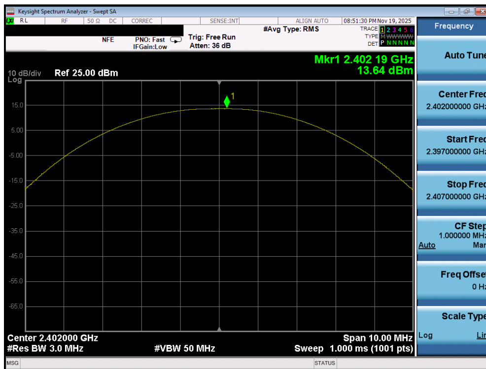
Plot 7-61. Peak Power Plot (Bluetooth (LE), 1Mbps – Ch. 37) – Dual Ant 1
