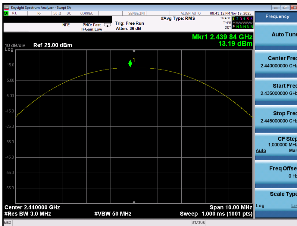
Plot 7-68. Peak Power Plot (Bluetooth (LE), 1Mbps – Ch. 17) – Dual Ant 2
