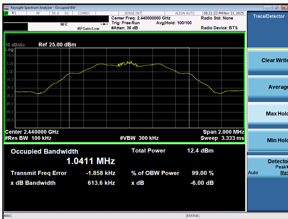
Plot 7-2. 6dB Bandwidth Plot (Bluetooth (LE), 125kbps – Ch. 17) – Ant 1
