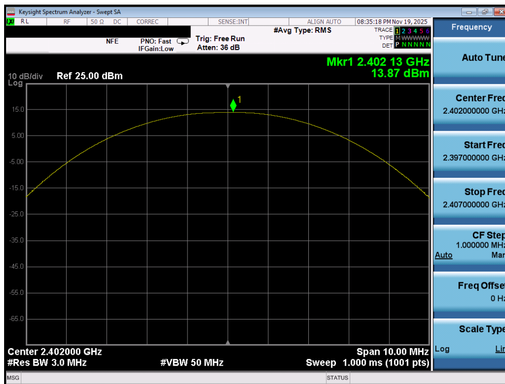
Plot 7-67. Peak Power Plot (Bluetooth (LE), 1Mbps – Ch. 37) – Dual Ant 2
