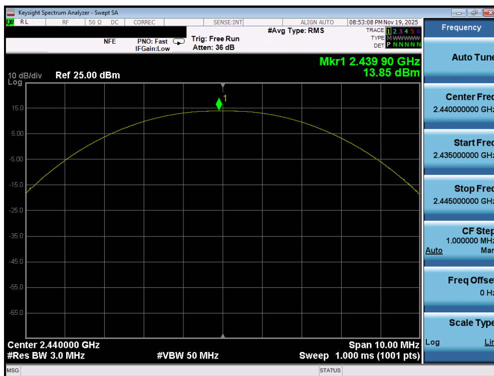
Plot 7-62. Peak Power Plot (Bluetooth (LE), 1Mbps – Ch. 17) – Dual Ant 1
