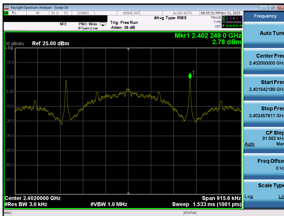
Plot 7-73. Power Spectral Density Plot (Bluetooth (LE), 125kbps – Ch. 37) – Ant 1
