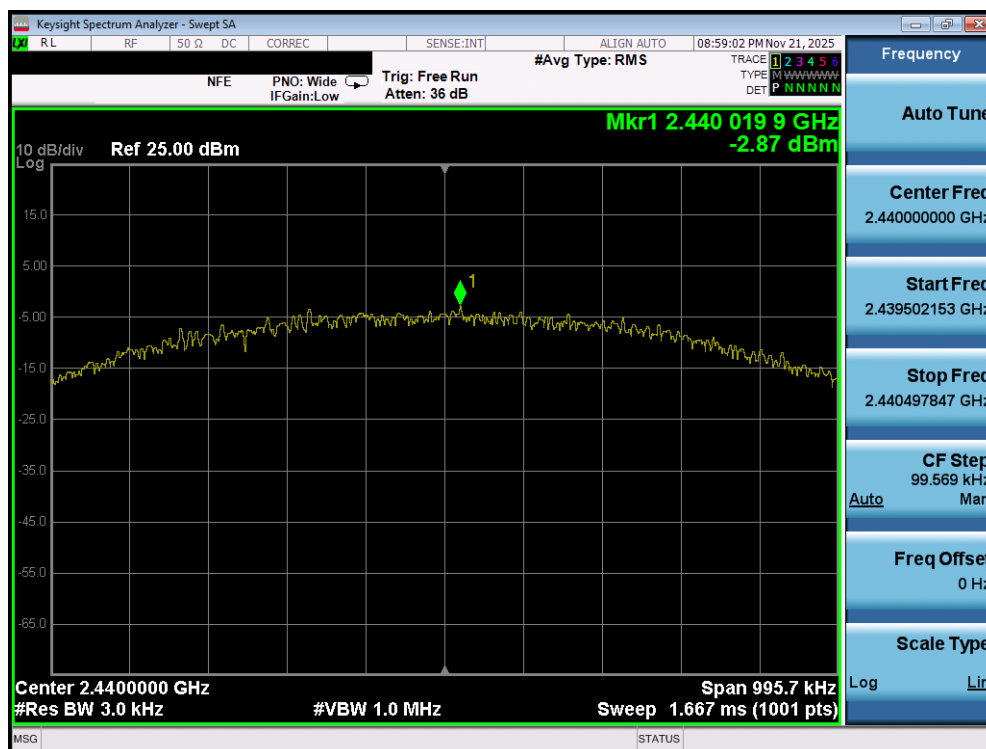
Plot 7-98. Power Spectral Density Plot (Bluetooth (LE), 1Mbps – Ch. 17) – Dual Ant 1
