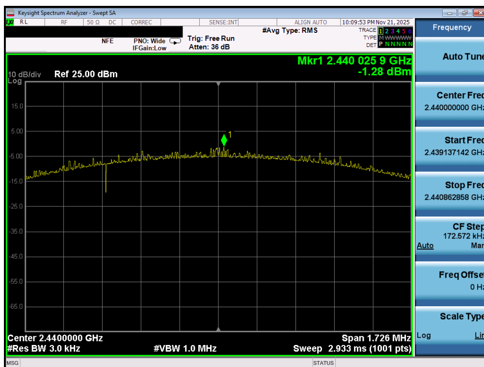
Plot 7-95. Power Spectral Density Plot (Bluetooth (LE), 2Mbps – Ch. 17) – Ant 2
