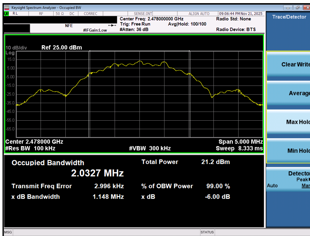
Plot 7-30. 6dB Bandwidth Plot (Bluetooth (LE), 2Mbps – Ch. 36) – Dual Ant 1
