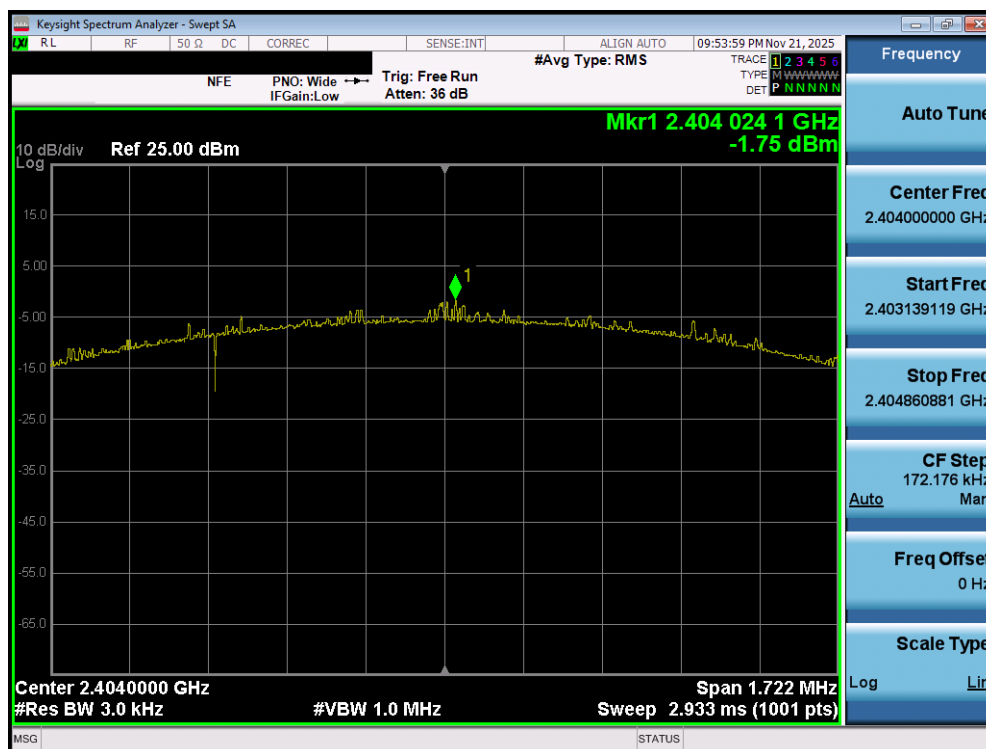
Plot 7-94. Power Spectral Density Plot (Bluetooth (LE), 2Mbps – Ch. 0) – Ant 2
