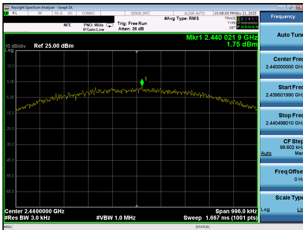
Plot 7-92. Power Spectral Density Plot (Bluetooth (LE), 1Mbps – Ch. 17) – Ant 2
