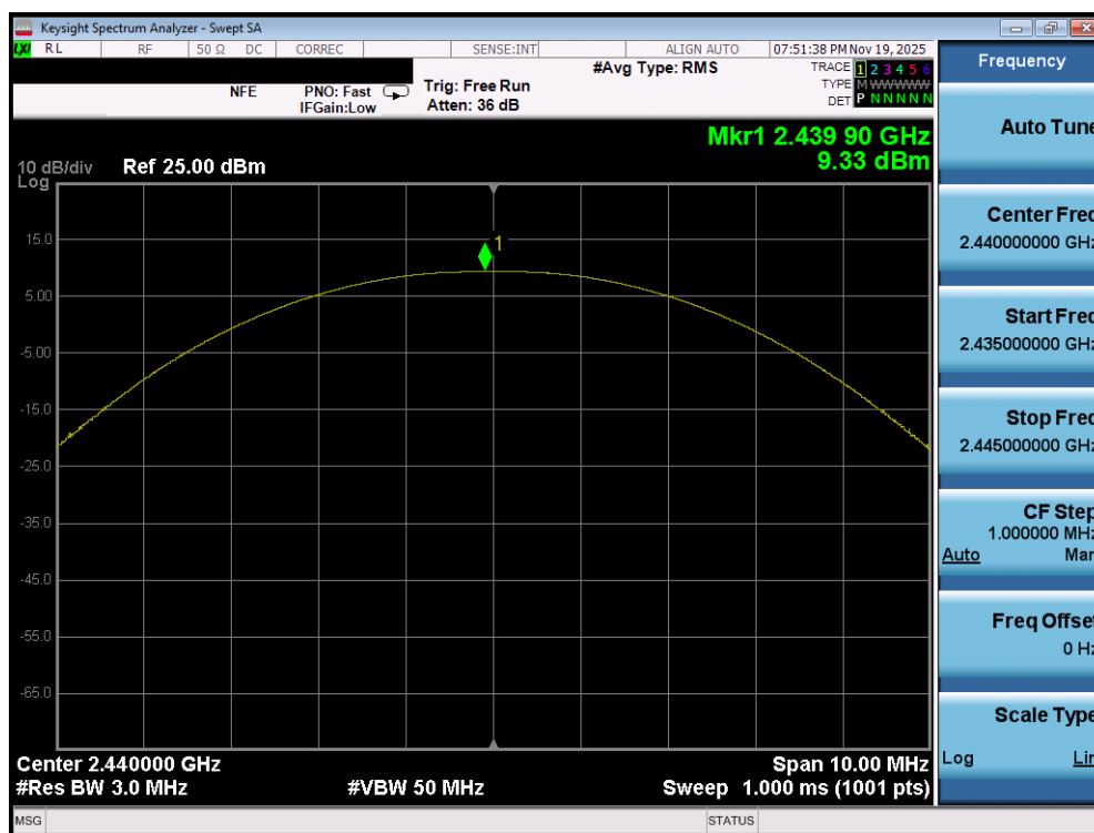
Plot 7-38. Peak Power Plot (Bluetooth (LE), 125kbps – Ch. 17) – Ant 1
