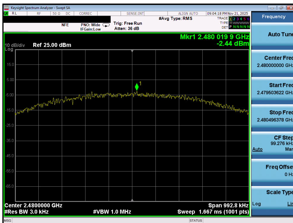
Plot 7-99. Power Spectral Density Plot (Bluetooth (LE), 1Mbps – Ch. 39) – Dual Ant 1
