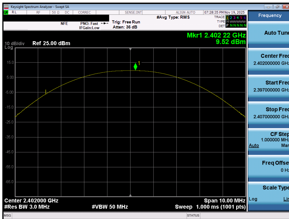
Plot 7-37. Peak Power Plot (Bluetooth (LE), 125kbps – Ch. 37) – Ant 1
