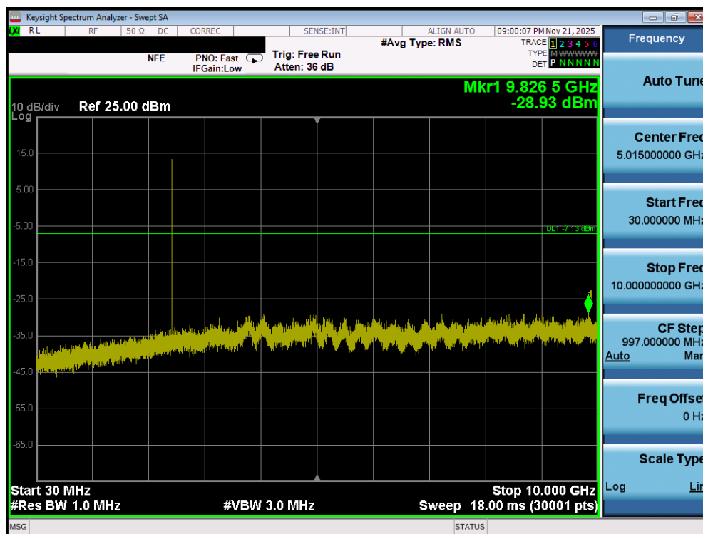
Plot 7-147. Conducted Spurious Plot (Bluetooth (LE), 1Mbps – Ch. 17) – Dual Ant 1
