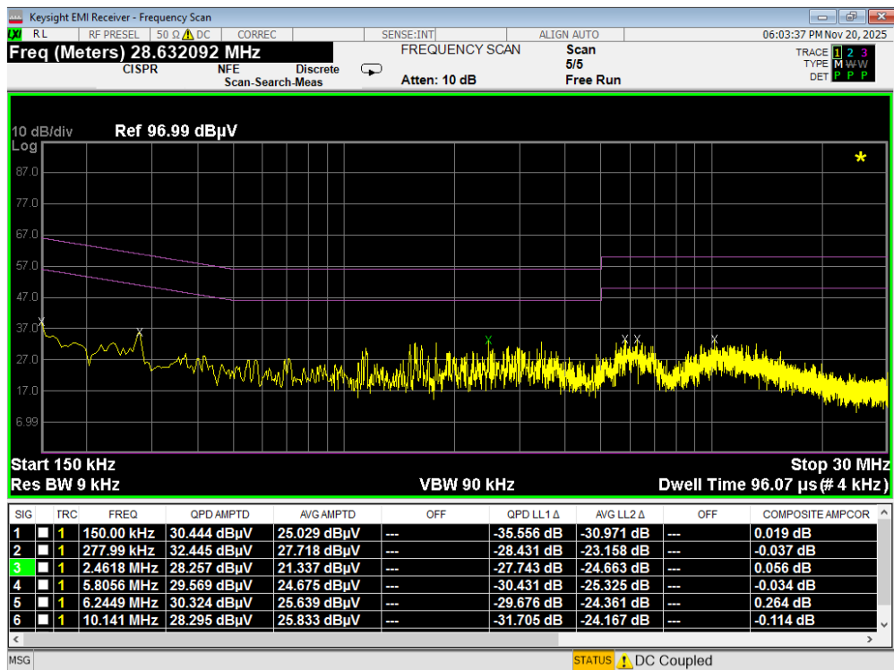
Plot 7-179. Line Conducted Plot with Bluetooth LE (N)
