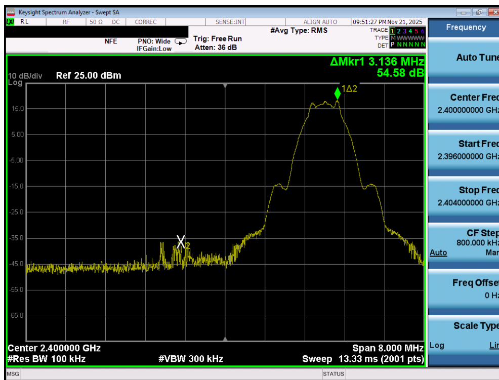
Plot 7-121. Band Edge Plot (Bluetooth (LE), 1Mbps – Ch. 37) – Ant 2
