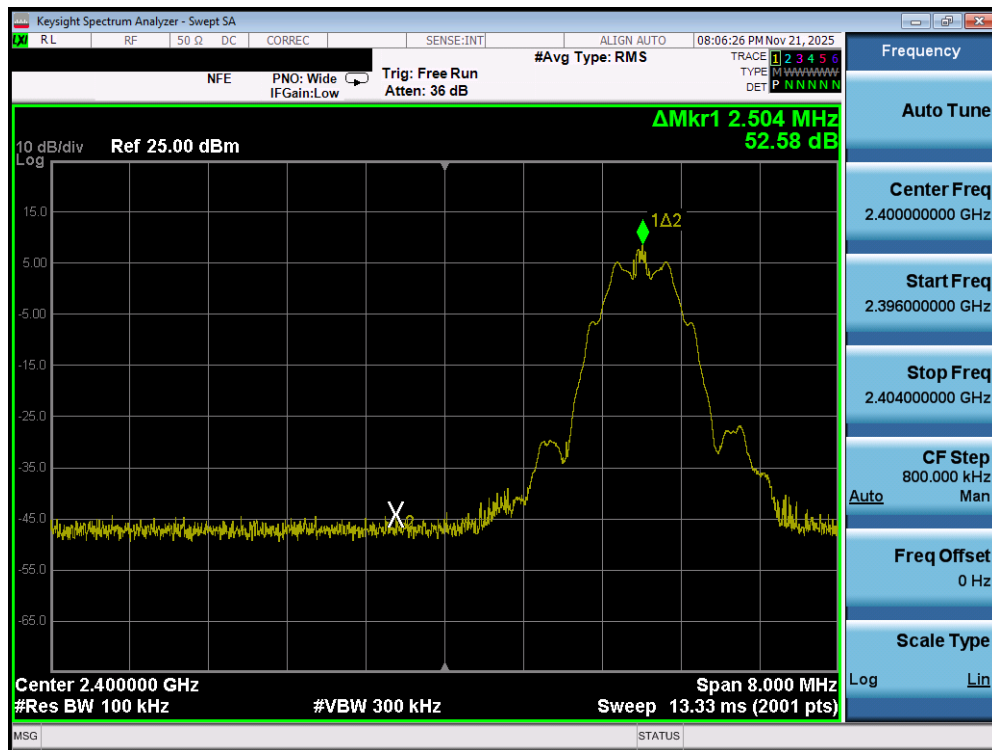
Plot 7-109. Band Edge Plot (Bluetooth (LE), 125kbps – Ch. 37) – Ant 1
