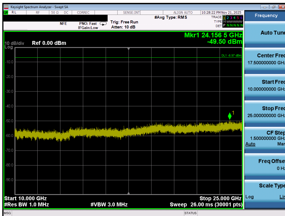
Plot 7-152. Conducted Spurious Plot (Bluetooth (LE), 1Mbps – Ch. 37) – Dual Ant 2
