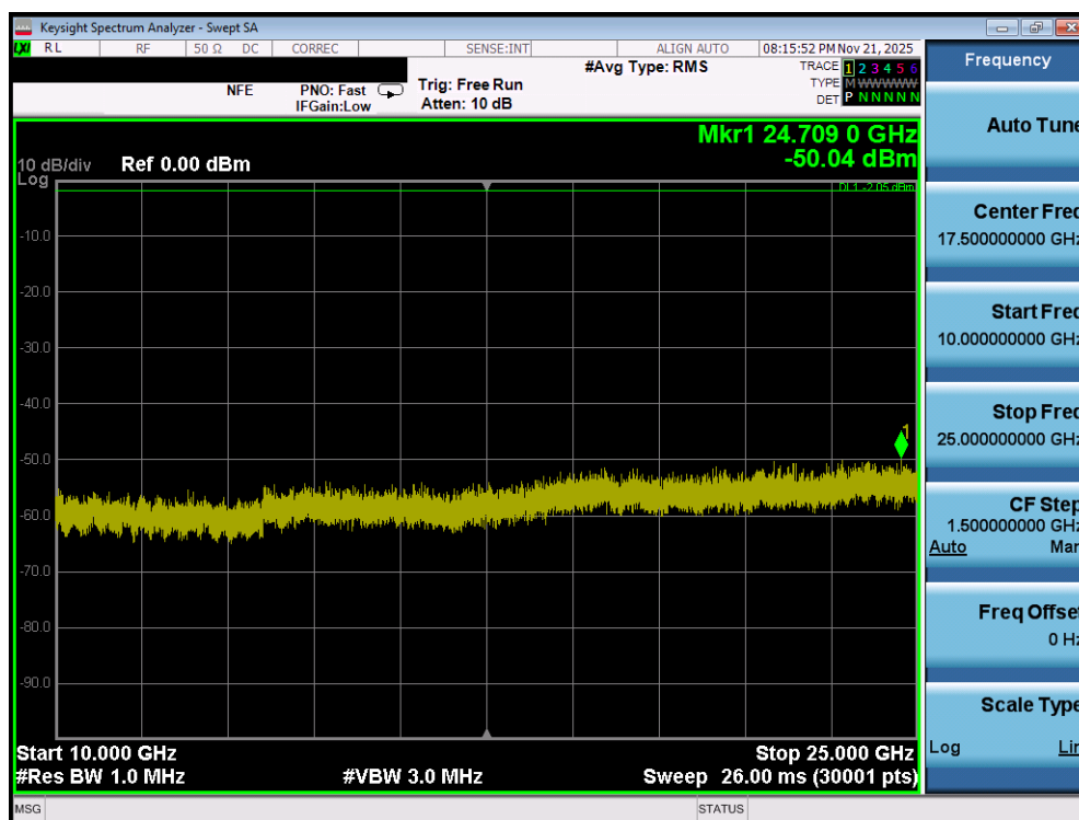
Plot 7-134. Conducted Spurious Plot (Bluetooth (LE), 1Mbps – Ch. 37) – Ant 1
