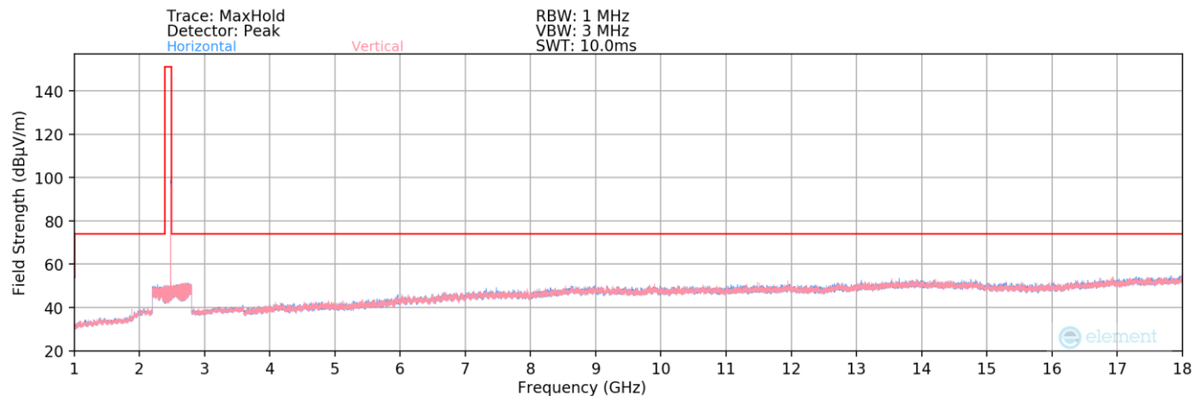
Plot 7-163. Radiated Spurious Plot above 1GHz (Bluetooth (LE) – Ch. 39) – Ant 2
