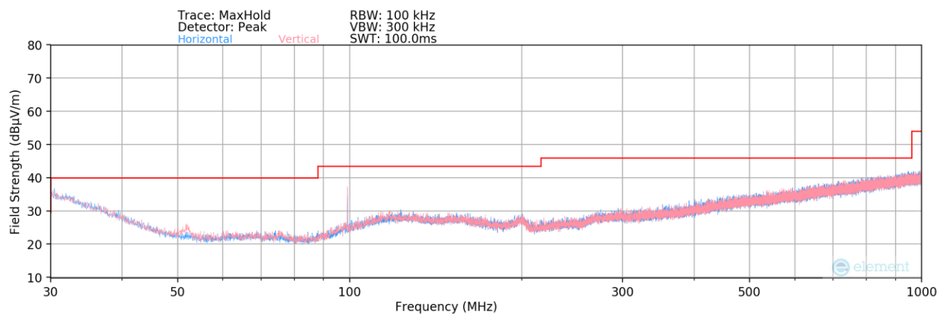
Plot 7-176. Radiated Spurious Plot below 1GHz – Ant 2
