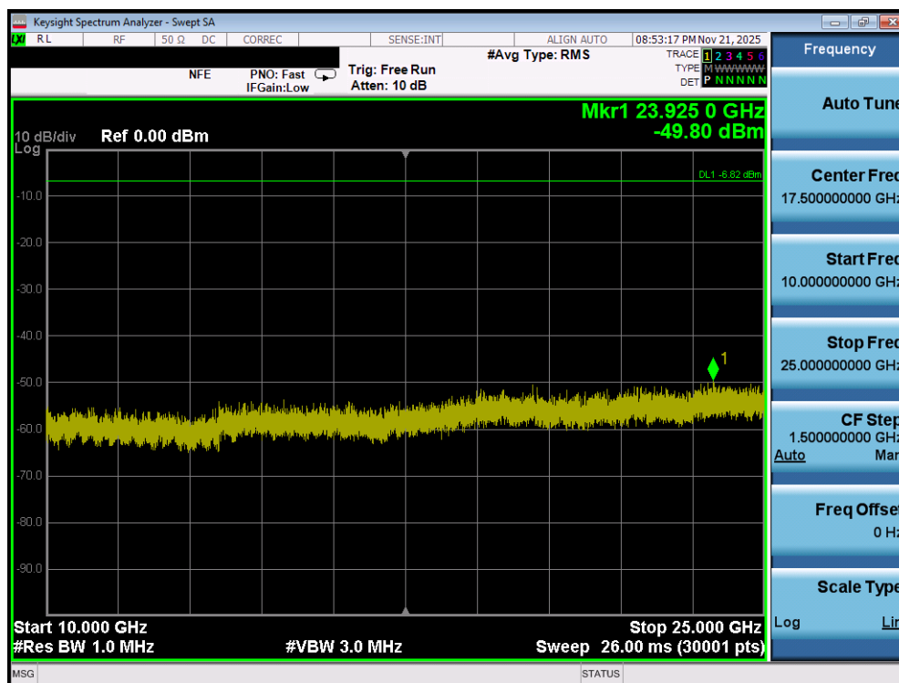
Plot 7-146. Conducted Spurious Plot (Bluetooth (LE), 1Mbps – Ch. 37) – Dual Ant 1
