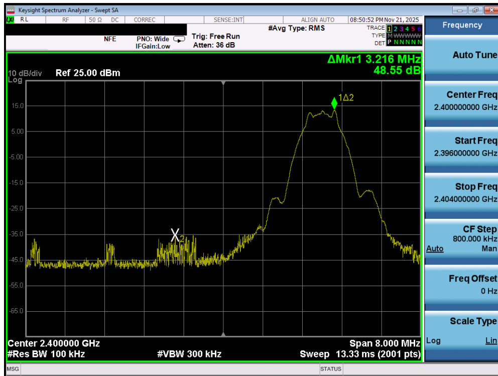
Plot 7-125. Band Edge Plot (Bluetooth (LE), 1Mbps – Ch. 37) – Dual Ant 1
