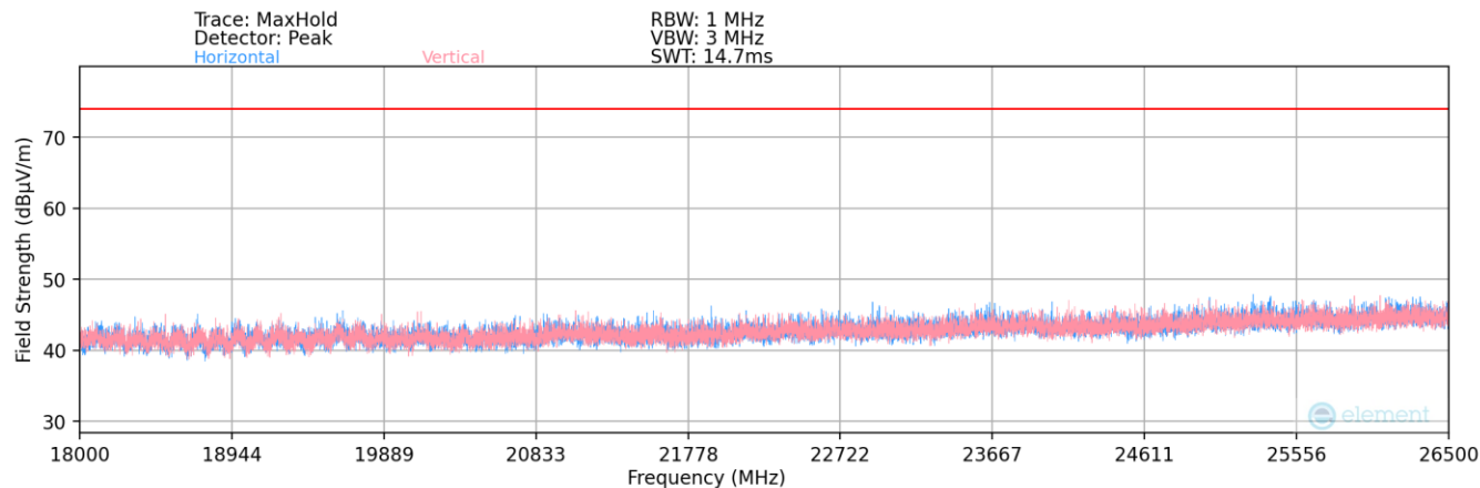
Plot 7-168. Radiated Spurious Plot above 18GHz (Bluetooth (LE) – Ch. 17) – Dual
