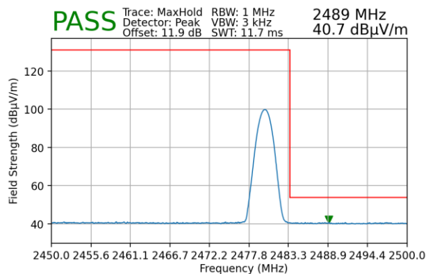
Plot 7-173. Radiated Restricted Upper Band Edge Measurement (Average) – Dual
