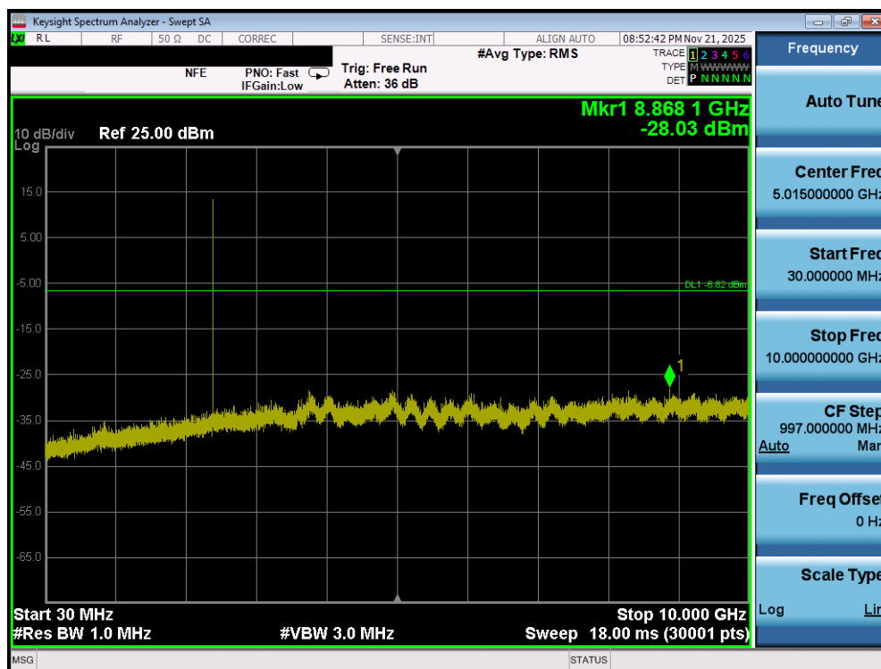
Plot 7-145. Conducted Spurious Plot (Bluetooth (LE), 1Mbps – Ch. 37) – Dual Ant 1
