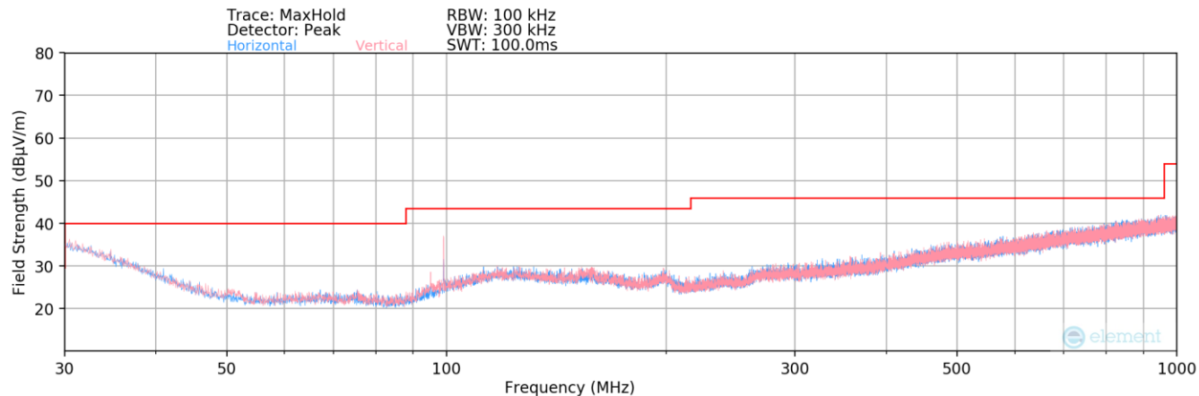
Plot 7-175. Radiated Spurious Plot below 1GHz – Ant 1
