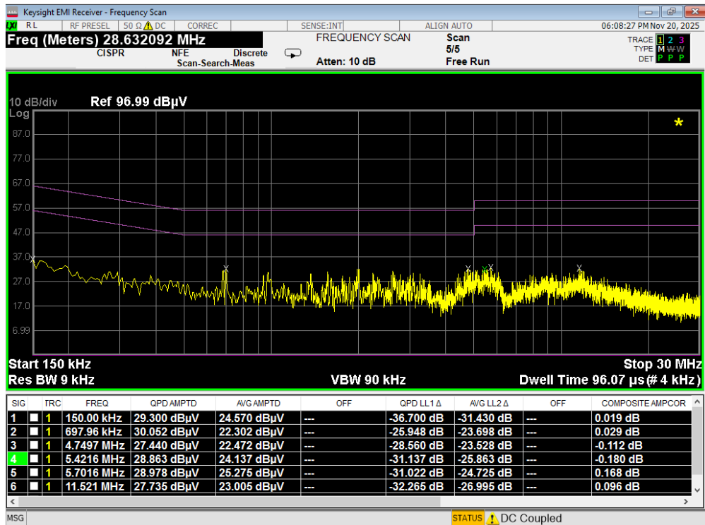
Plot 7-181. Line Conducted Plot with Bluetooth LE (N) - WCP
