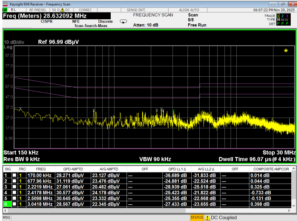
Plot 7-180. Line Conducted Plot with Bluetooth LE (L1) - WCP
