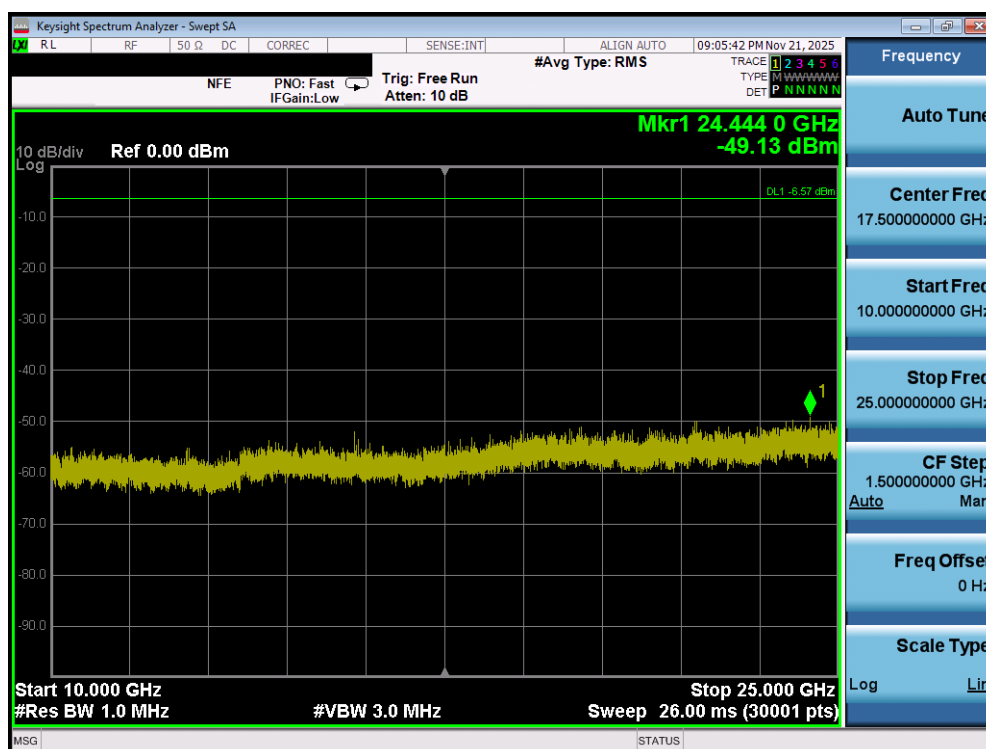
Plot 7-150. Conducted Spurious Plot (Bluetooth (LE), 1Mbps – Ch. 39) – Dual Ant 1
