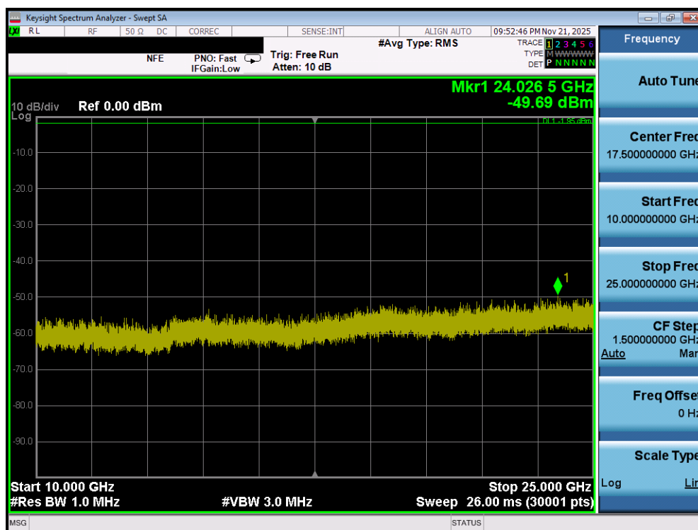
Plot 7-140. Conducted Spurious Plot (Bluetooth (LE), 1Mbps – Ch. 37) – Ant 2
