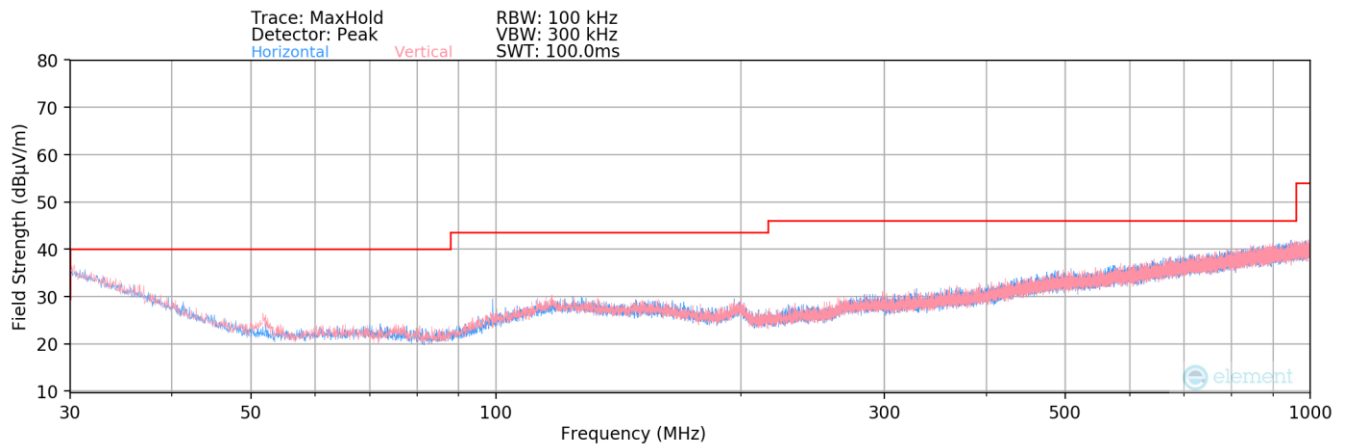
Plot 7-177. Radiated Spurious Plot below 1GHz – Dual
