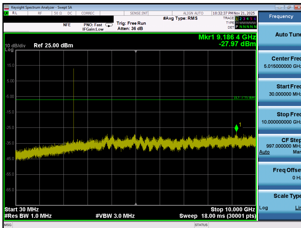
Plot 7-153. Conducted Spurious Plot (Bluetooth (LE), 1Mbps – Ch. 17) – Dual Ant 2
