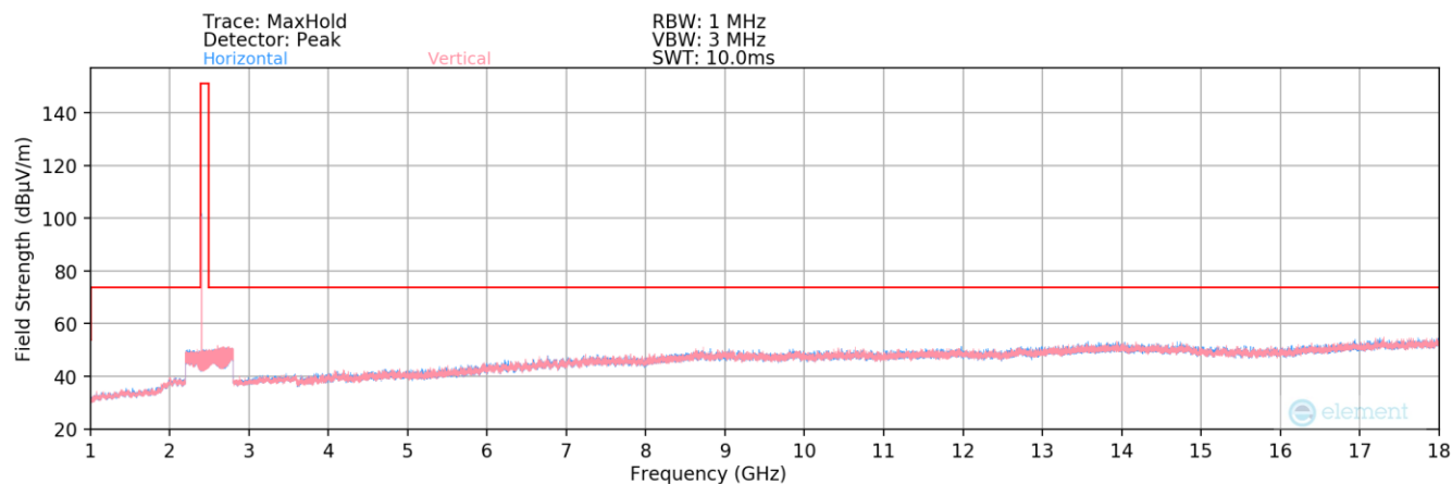
Plot 7-161. Radiated Spurious Plot above 1GHz (Bluetooth (LE) – Ch. 37) – Ant 2
