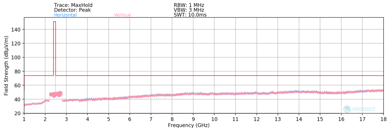
Plot 7-167. Radiated Spurious Plot above 1GHz (Bluetooth (LE) – Ch. 39) – Dual
