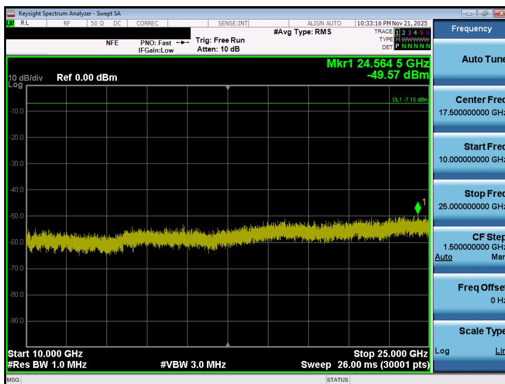
Plot 7-154. Conducted Spurious Plot (Bluetooth (LE), 1Mbps – Ch. 17) – Dual Ant 2
