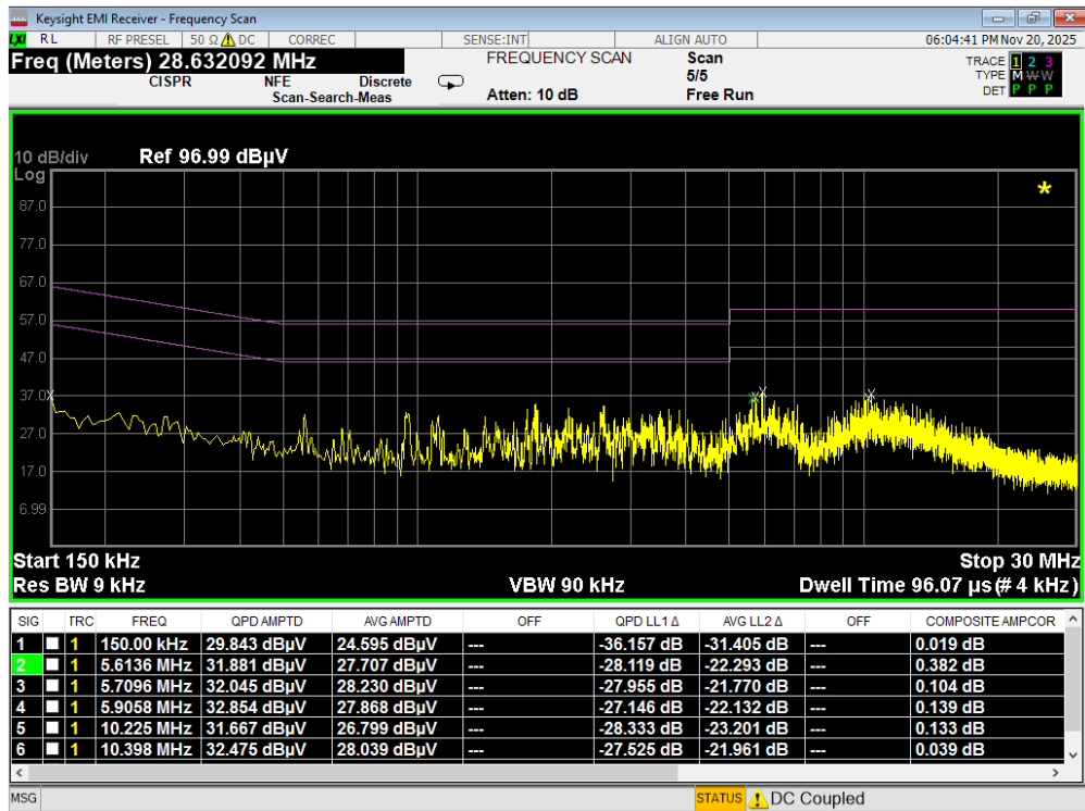
Plot 7-178. Line Conducted Plot with Bluetooth LE (L1)
