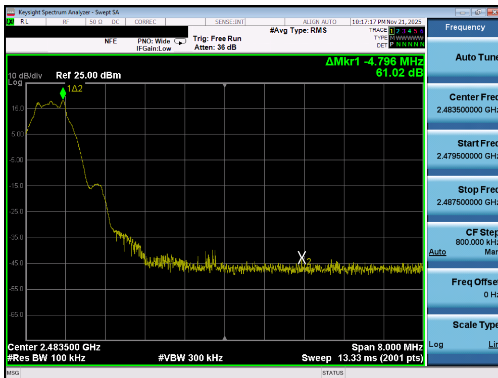
Plot 7-122. Band Edge Plot (Bluetooth (LE), 1Mbps – Ch. 39) – Ant 2
