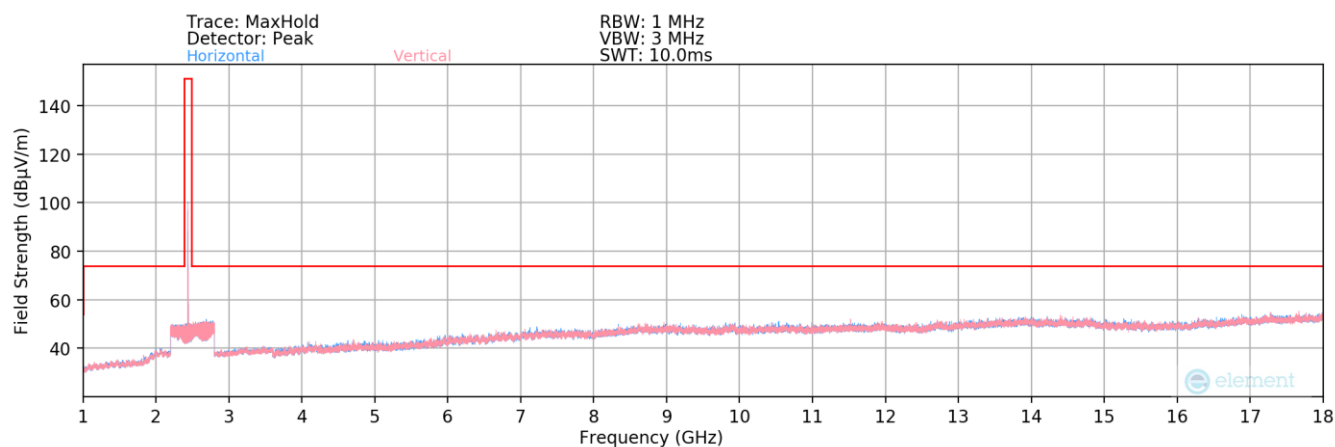
Plot 7-166. Radiated Spurious Plot above 1GHz (Bluetooth (LE) – Ch. 17) – Dual
