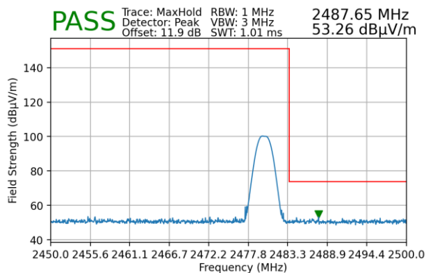
Plot 7-174. Radiated Restricted Upper Band Edge Measurement (Peak) – Dual
