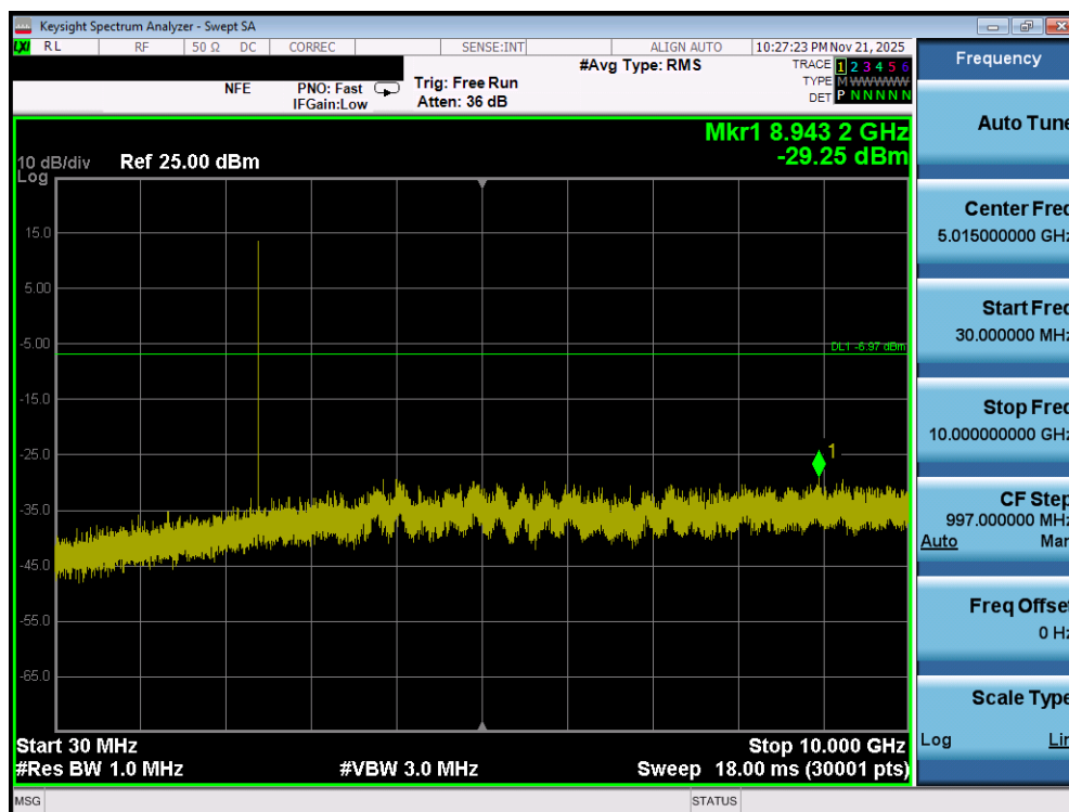
Plot 7-151. Conducted Spurious Plot (Bluetooth (LE), 1Mbps – Ch. 37) – Dual Ant 2
