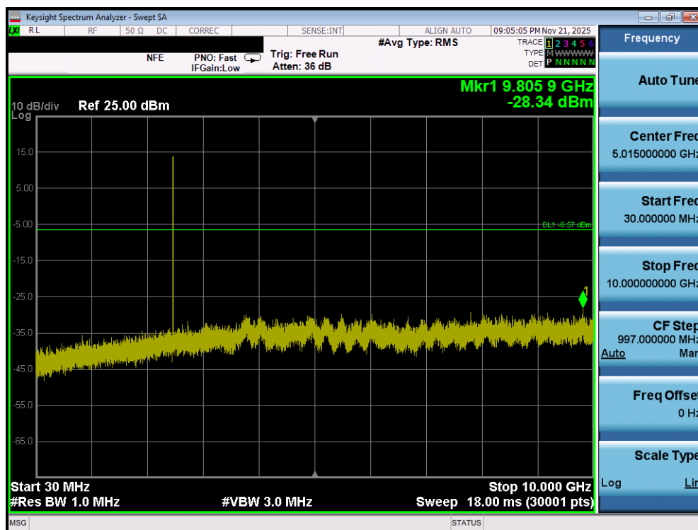
Plot 7-149. Conducted Spurious Plot (Bluetooth (LE), 1Mbps – Ch. 39) – Dual Ant 1
