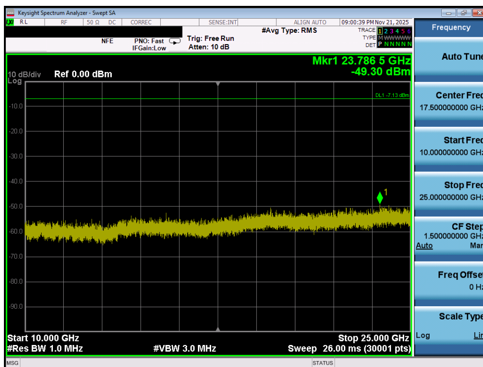
Plot 7-148. Conducted Spurious Plot (Bluetooth (LE), 1Mbps – Ch. 17) – Dual Ant 1
