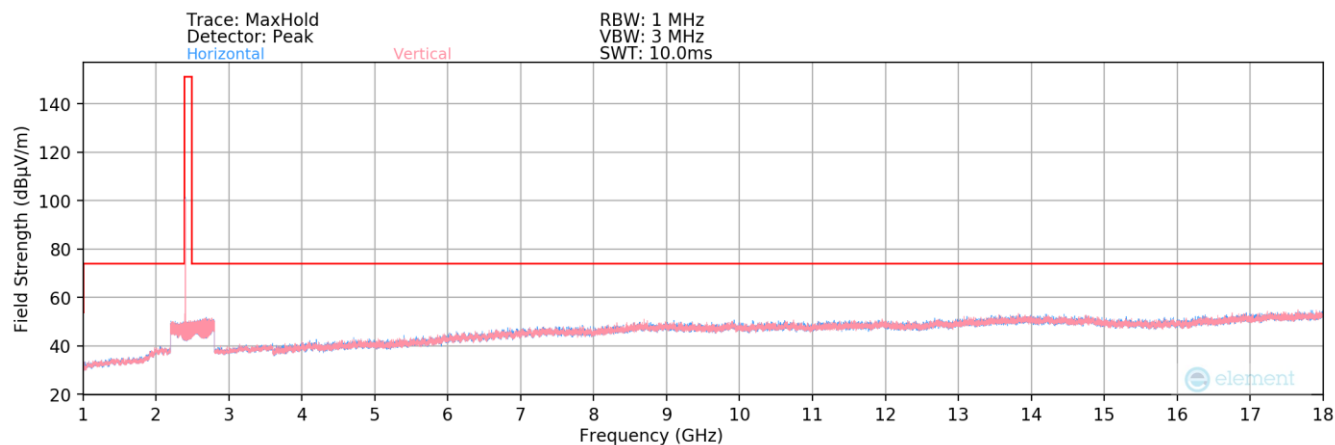
Plot 7-165. Radiated Spurious Plot above 1GHz (Bluetooth (LE) – Ch. 37) – Dual
