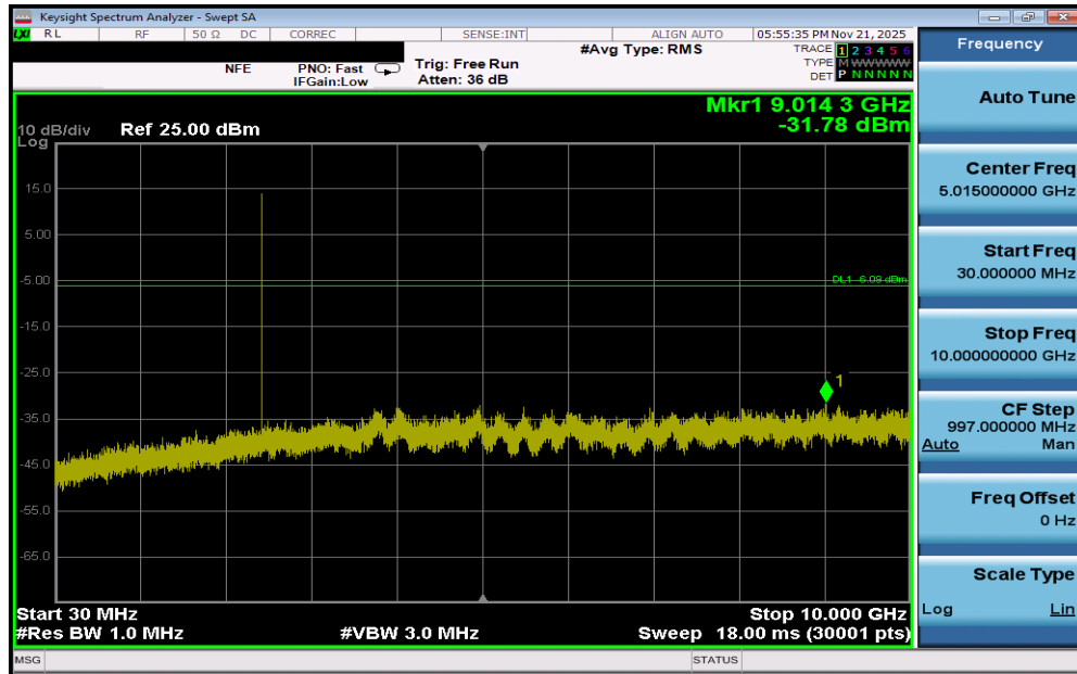
Plot 7-155. Conducted Spurious Plot (Bluetooth, 1Mbps – Ch. 39) – Dual Ant 1
