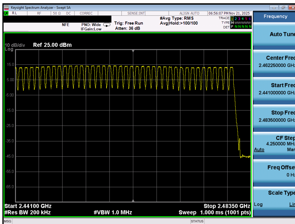
Plot 7-140. High End Spectrum Channel Hopping Plot (Bluetooth) – Dual Ant 2
