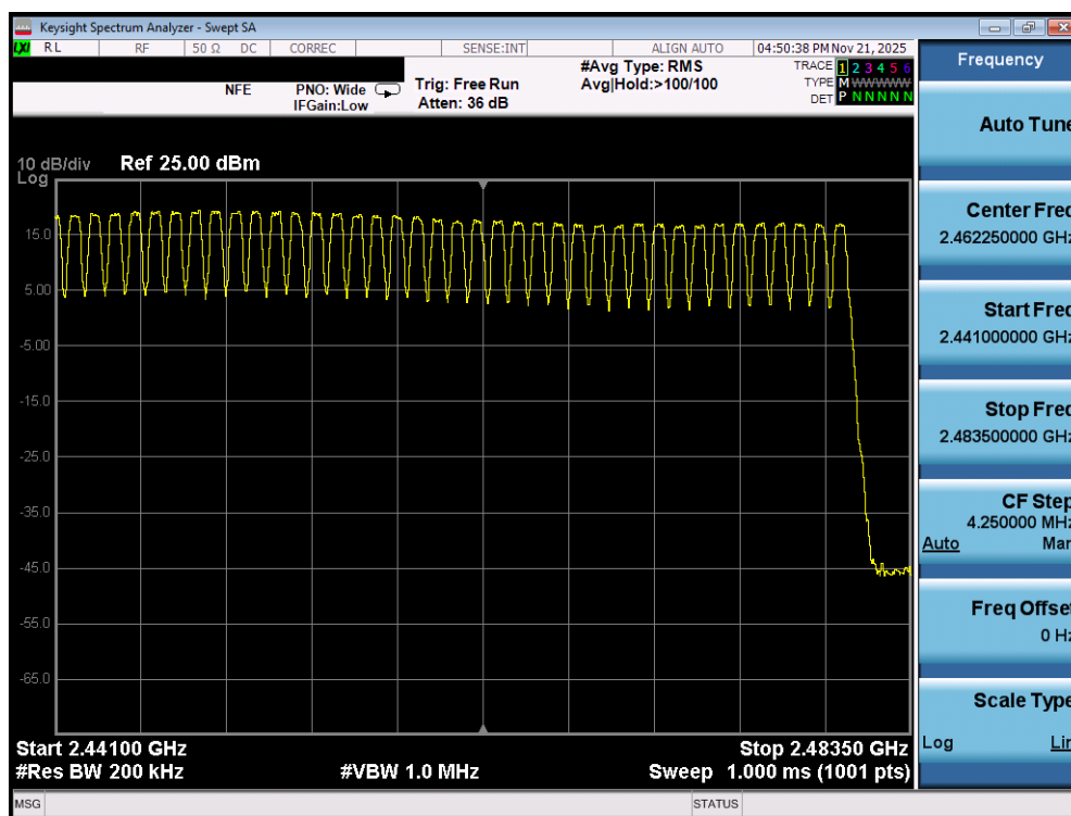
Plot 7-134. High End Spectrum Channel Hopping Plot (Bluetooth) – Ant 1
