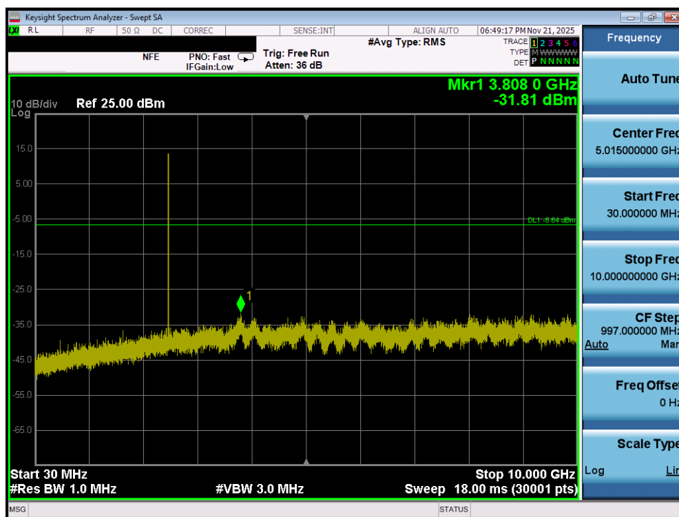
Plot 7-163. Conducted Spurious Plot (Bluetooth, 1Mbps – Ch. 78) – Dual Ant 2
