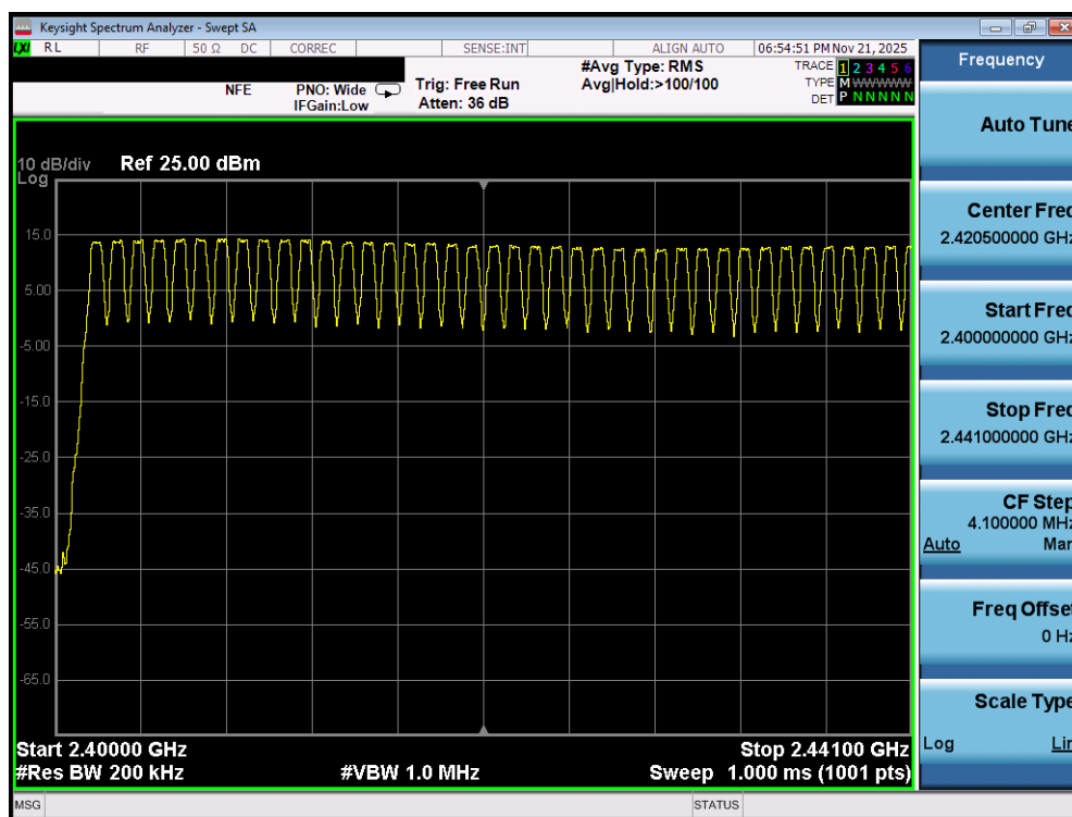
Plot 7-139. Low End Spectrum Channel Hopping Plot (Bluetooth) – Dual Ant 2
