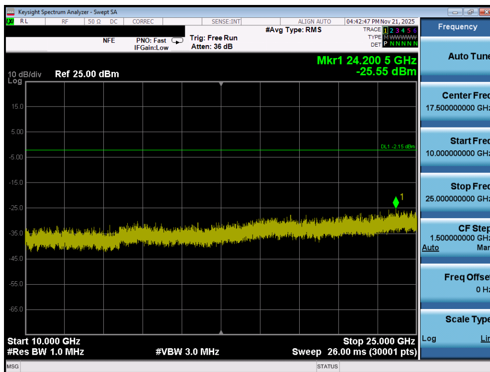
Plot 7-152. Conducted Spurious Plot (Bluetooth, 1Mbps – Ch. 78) – Ant 2
