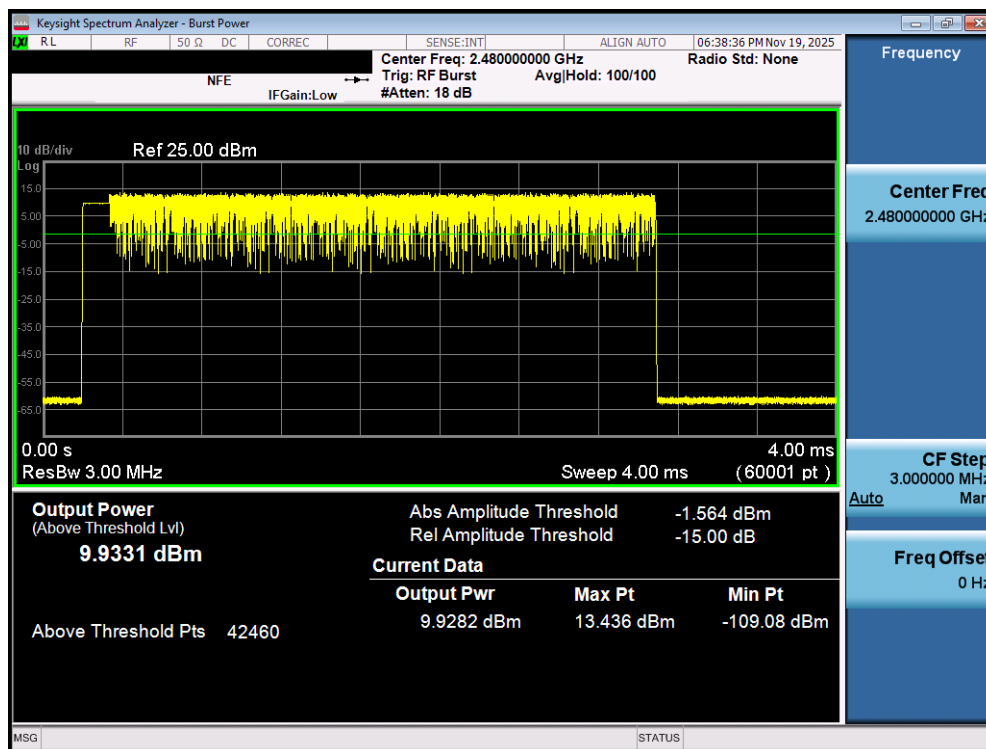
Plot 7-108. Average Conducted Power (3Mbps - Ch. 78) - Dual Ant 2
