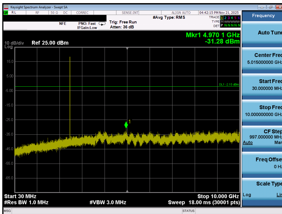
Plot 7-151. Conducted Spurious Plot (Bluetooth, 1Mbps – Ch. 78) – Ant 2
