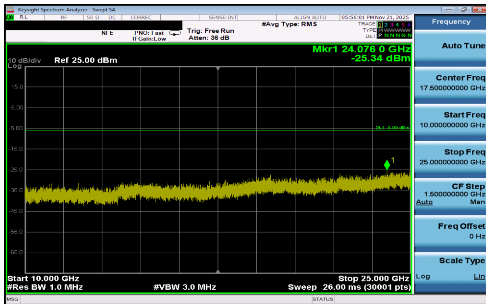
Plot 7-156. Conducted Spurious Plot (Bluetooth, 1Mbps – Ch. 39) – Dual Ant 1
