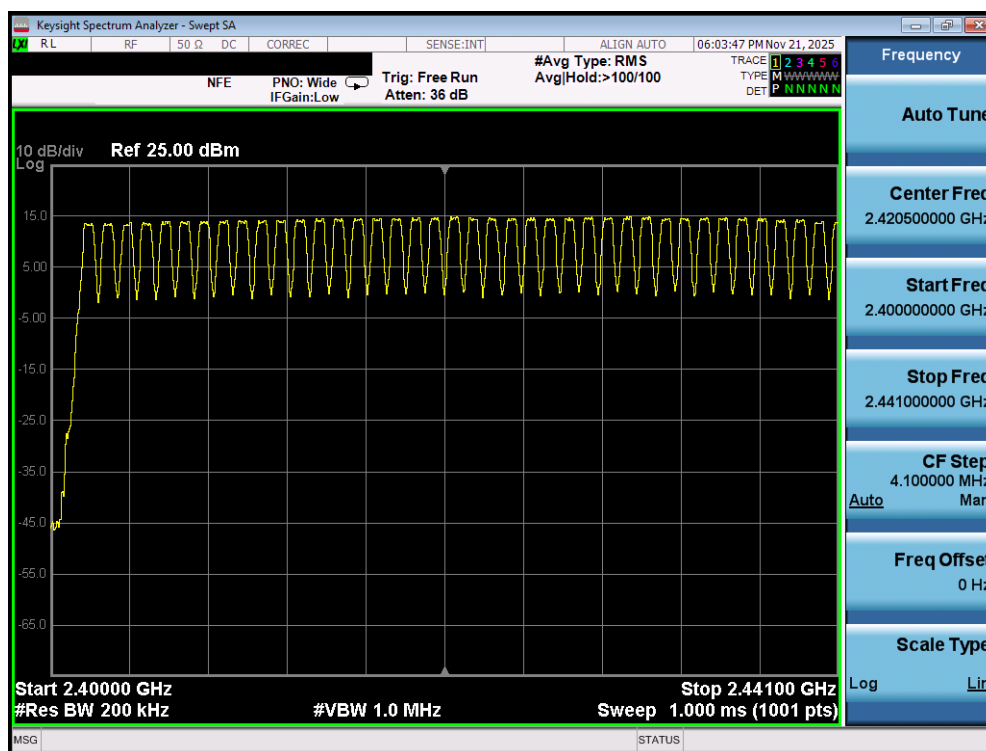
Plot 7-137. Low End Spectrum Channel Hopping Plot (Bluetooth) – Dual Ant 1
