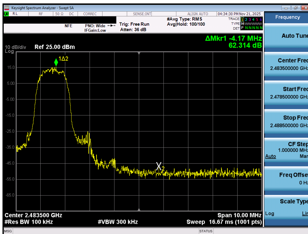
Plot 7-110. Band Edge Plot (Bluetooth with Hopping Disabled, 3 Mbps – Ch. 78) – Ant 1
