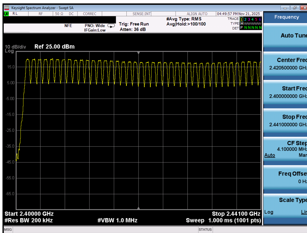
Plot 7-133. Low End Spectrum Channel Hopping Plot (Bluetooth) – Ant 1
