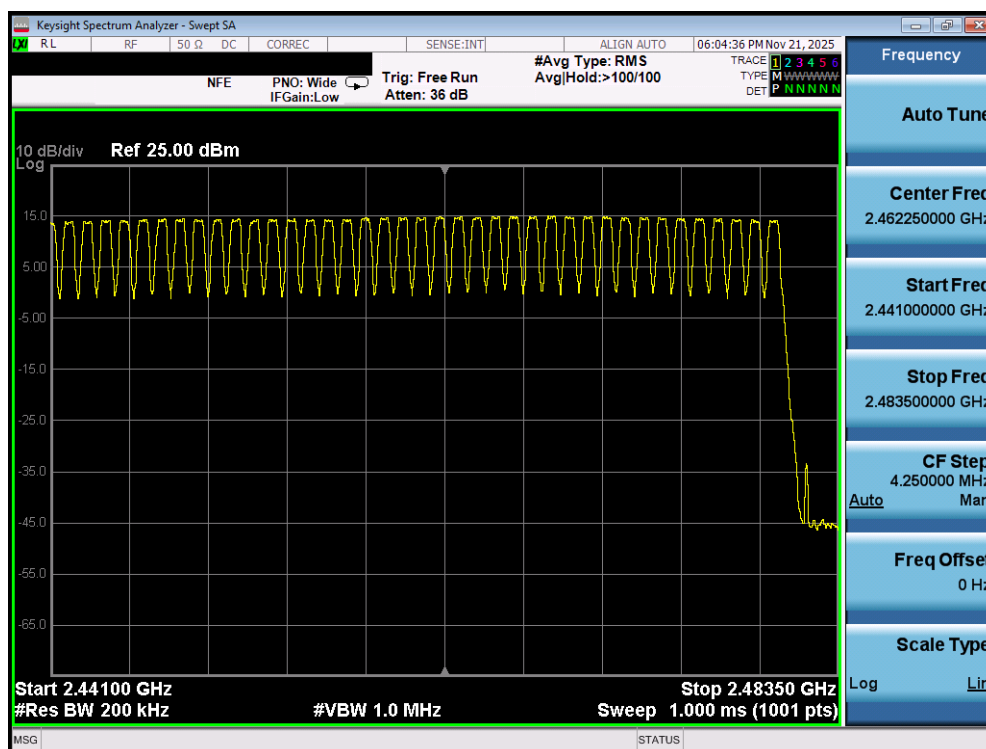
Plot 7-138. High End Spectrum Channel Hopping Plot (Bluetooth) – Dual Ant 1
