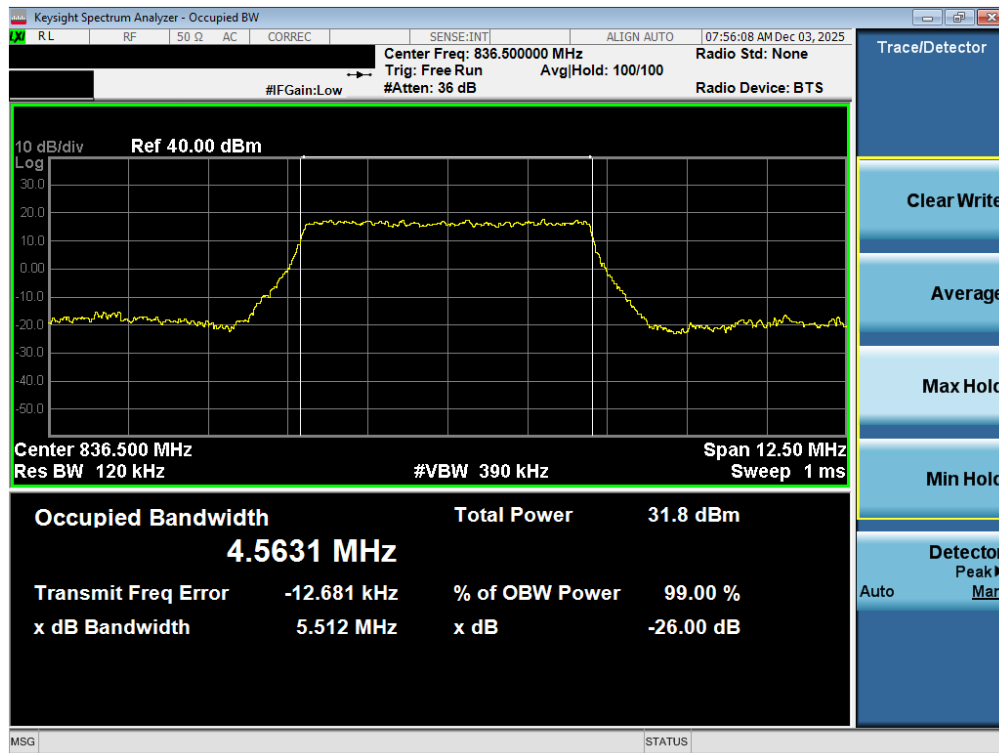
Plot 7-30. Occupied Bandwidth Plot (LTE Band 26/5 - 5MHz QPSK - Full RB - Ant2)
