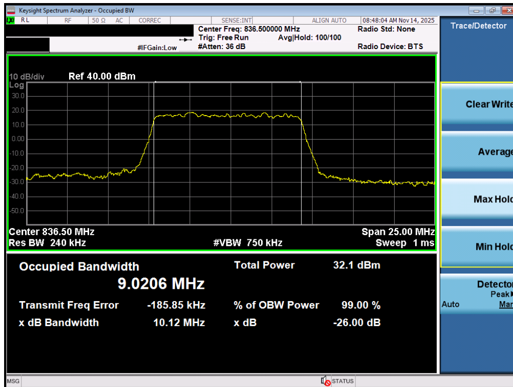
Plot 7-42. Occupied Bandwidth Plot (NR Band n26/5 - 10MHz \pi/2 BPSK - Full RB - Ant2)
