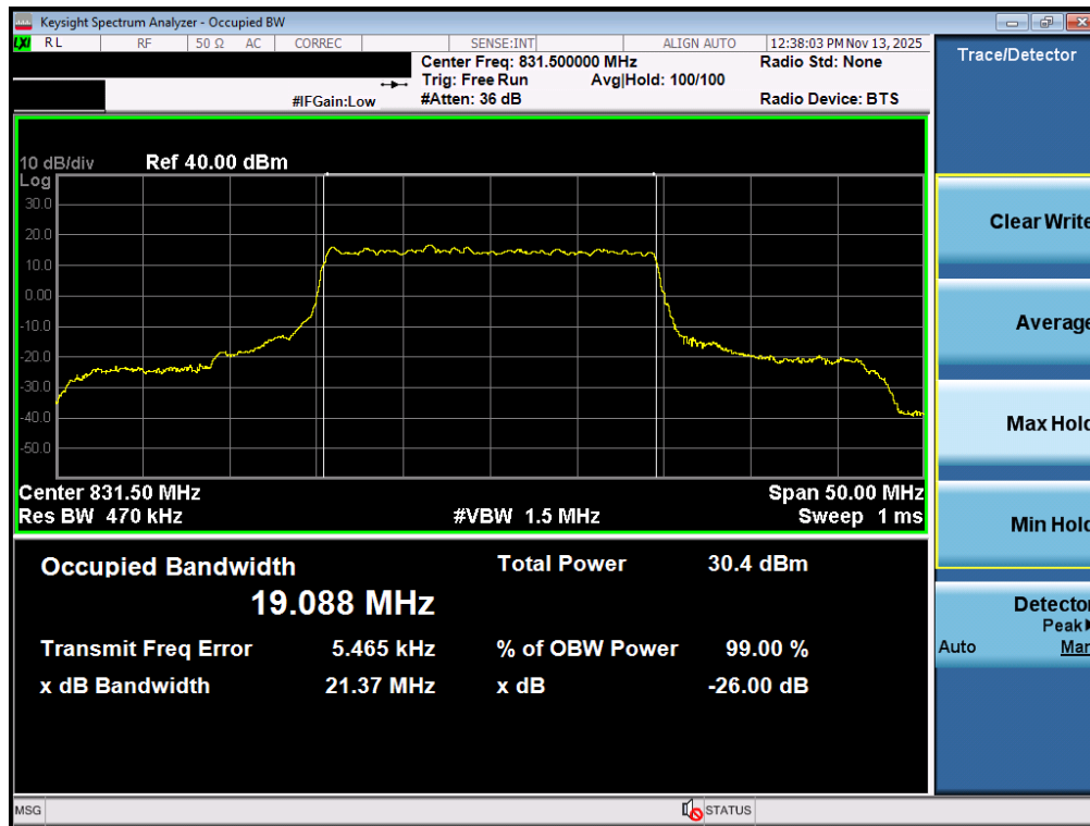
Plot 7-13. Occupied Bandwidth Plot (NR Band n26/5 - 20MHz 16-QAM - Full RB - Ant1)
