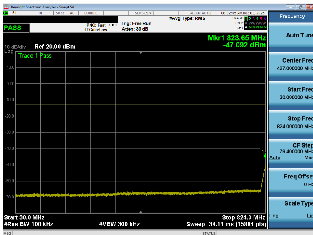
Plot 7-90. Conducted Spurious Plot (LTE Band 26/5 - 15MHz QPSK - 1 RB - Mid Channel – Ant2)
