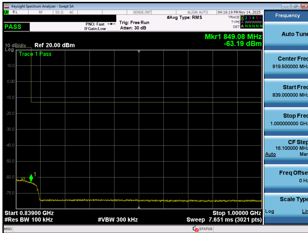
Plot 7-64. Conducted Spurious Plot (NR Band n26/5 - 20.0MHz - 1 RB - Mid Channel - Ant1)
