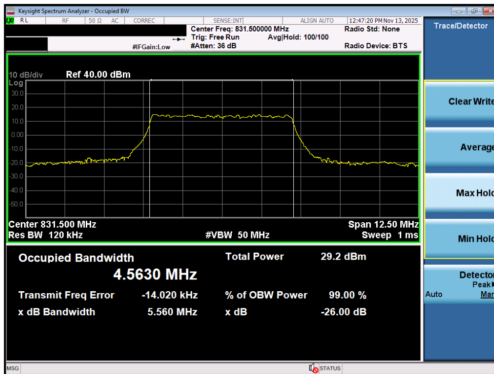
Plot 7-22. Occupied Bandwidth Plot (NR Band n26/5 - 5MHz 16-QAM - Full RB - Ant1)
