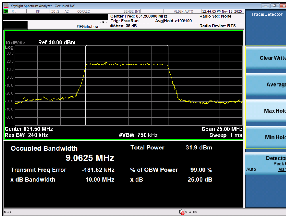
Plot 7-17. Occupied Bandwidth Plot (NR Band n26/5 - 10MHz \pi/2 BPSK - Full RB - Ant1)
