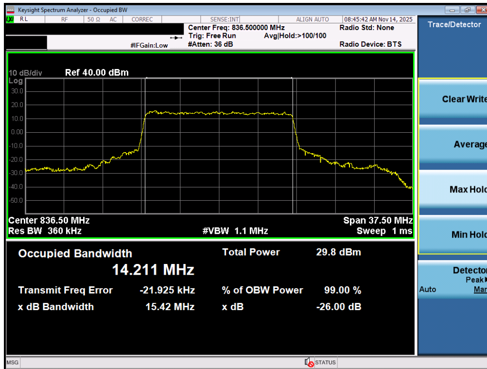
Plot 7-40. Occupied Bandwidth Plot (NR Band n26/5 - 15MHz QPSK - Full RB - Ant2)
