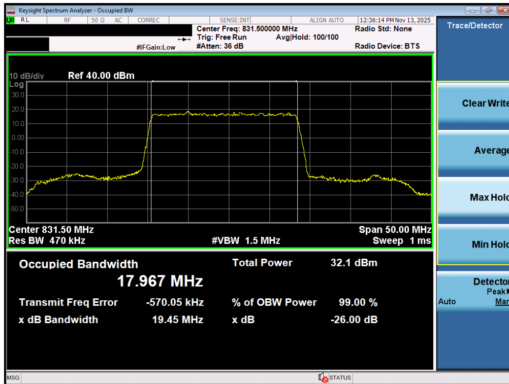
Plot 7-11. Occupied Bandwidth Plot (NR Band n26/5 - 20MHz \pi/2 BPSK - Full RB - Ant1)
