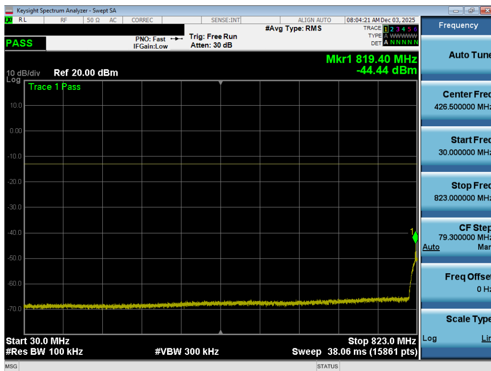
Plot 7-87. Conducted Spurious Plot (LTE Band 26/5 - 15MHz QPSK – 1 RB - Low Channel – Ant2)
