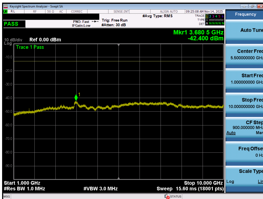
Plot 7-101. Conducted Spurious Plot (NR Band n26/5 - 20.0MHz - 1 RB - Mid Channel - Ant2)
