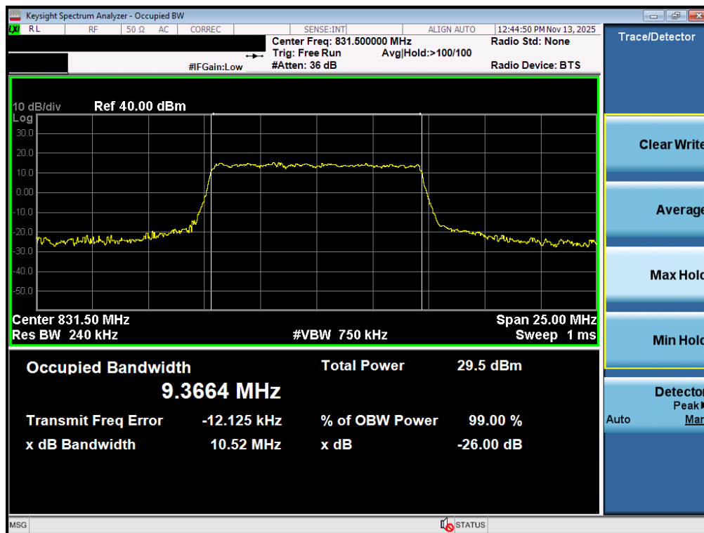
Plot 7-19. Occupied Bandwidth Plot (NR Band n26/5 - 10MHz 16-QAM - Full RB - Ant1)
