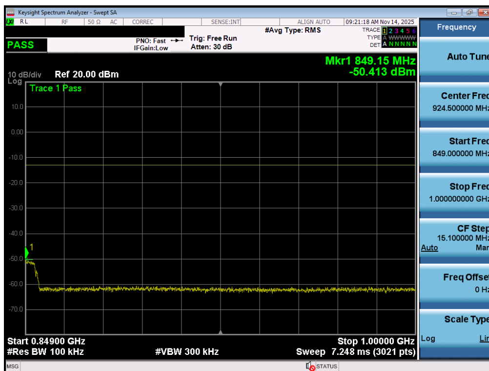
Plot 7-97. Conducted Spurious Plot (NR Band n26/5 - 20.0MHz - 1 RB - Low Channel - Ant2)
