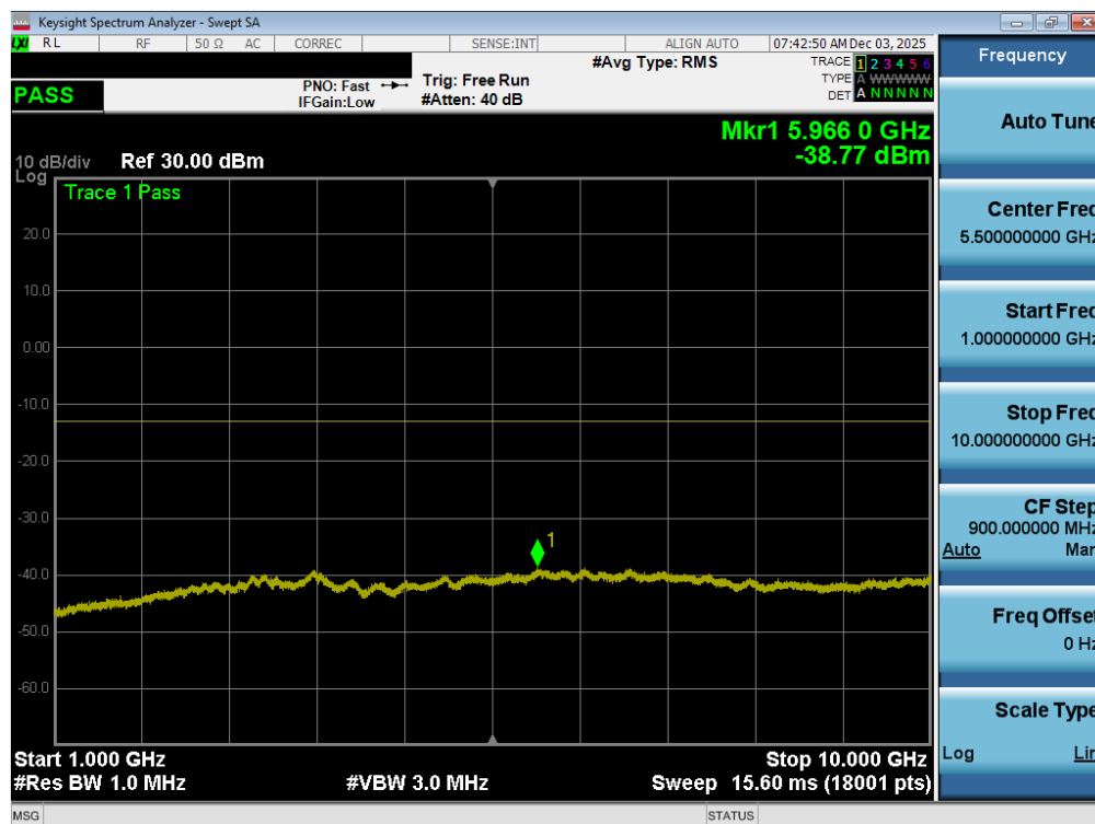
Plot 7-59. Conducted Spurious Plot (LTE Band 26/5 - 15MHz QPSK - 1 RB - High Channel – Ant1)
