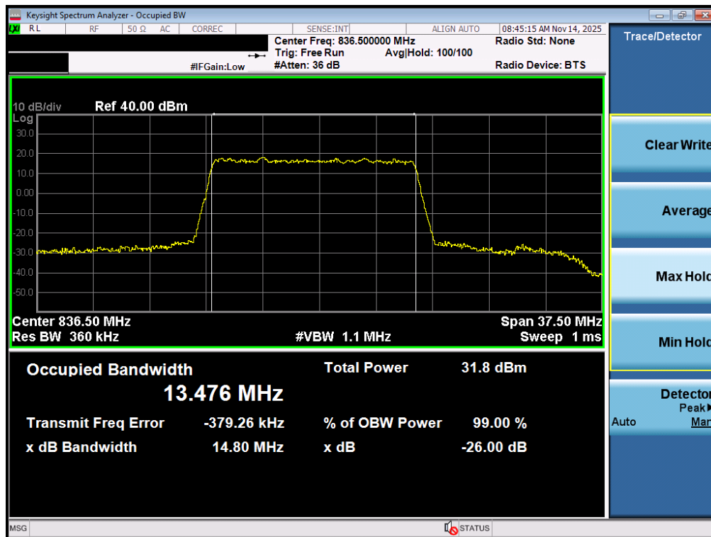
Plot 7-39. Occupied Bandwidth Plot (NR Band n26/5 - 15MHz \pi/2 BPSK - Full RB - Ant2)
