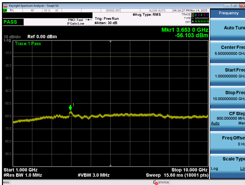
Plot 7-65. Conducted Spurious Plot (NR Band n26/5 - 20.0MHz - 1 RB - Mid Channel - Ant1)
