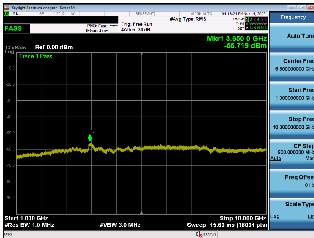
Plot 7-68. Conducted Spurious Plot (NR Band n26/5 - 20.0MHz - 1 RB - High Channel - Ant1)
