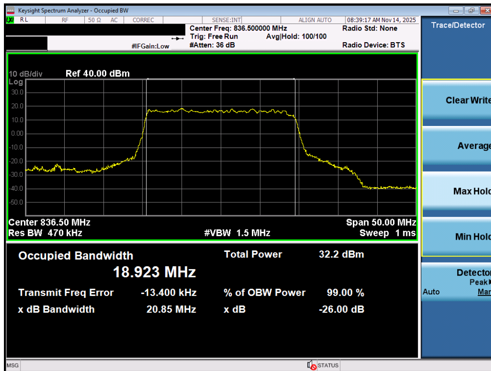
Plot 7-37. Occupied Bandwidth Plot (NR Band n26/5 - 20MHz QPSK - Full RB - Ant2)
