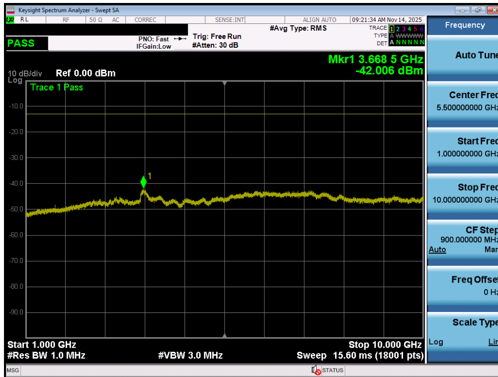
Plot 7-98. Conducted Spurious Plot (NR Band n26/5 - 20.0MHz - 1 RB - Low Channel - Ant2)
