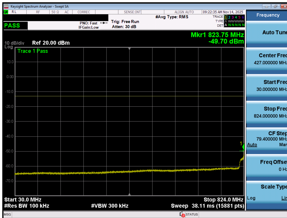
Plot 7-99. Conducted Spurious Plot (NR Band n26/5 - 20.0MHz - 1 RB - Mid Channel - Ant2)
