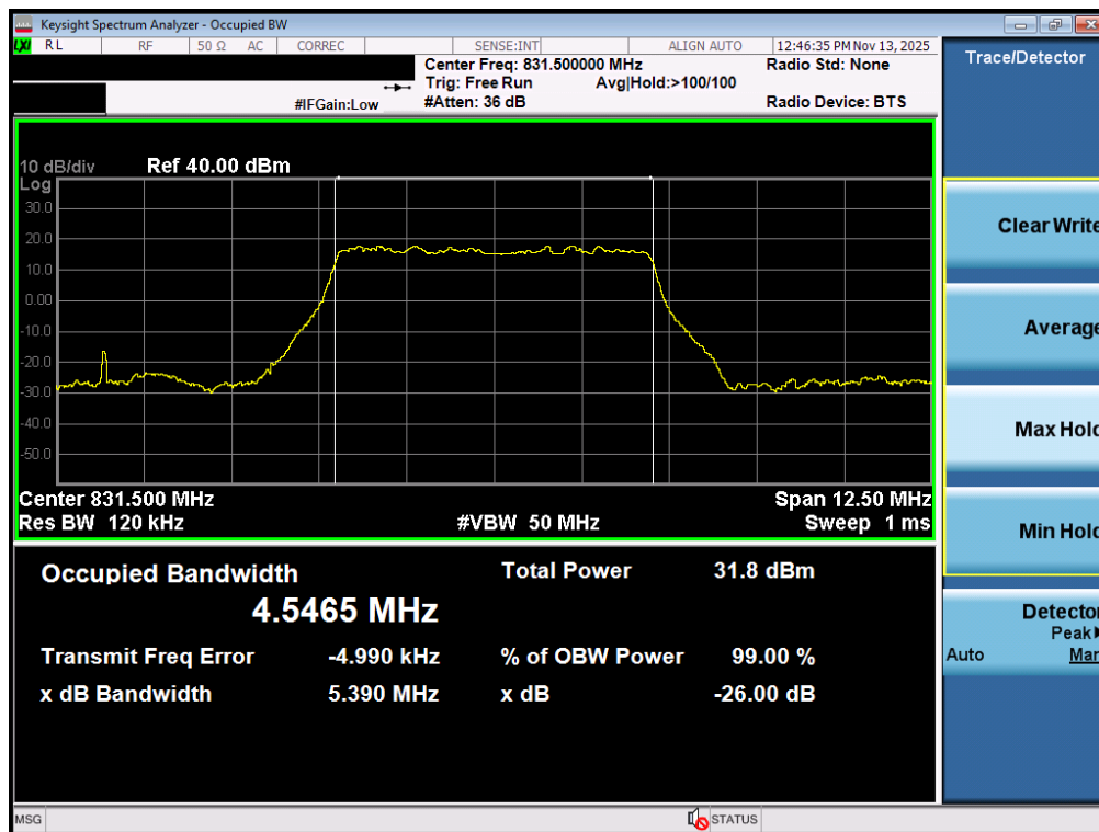
Plot 7-20. Occupied Bandwidth Plot (NR Band n26/5 - 5MHz \pi/2 BPSK - Full RB - Ant1)
