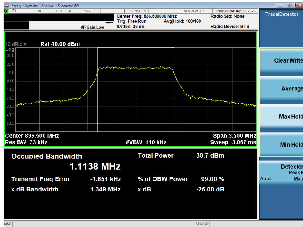
Plot 7-35. Occupied Bandwidth Plot (LTE Band 26/5 - 1.4MHz 16-QAM - Full RB - Ant2)
