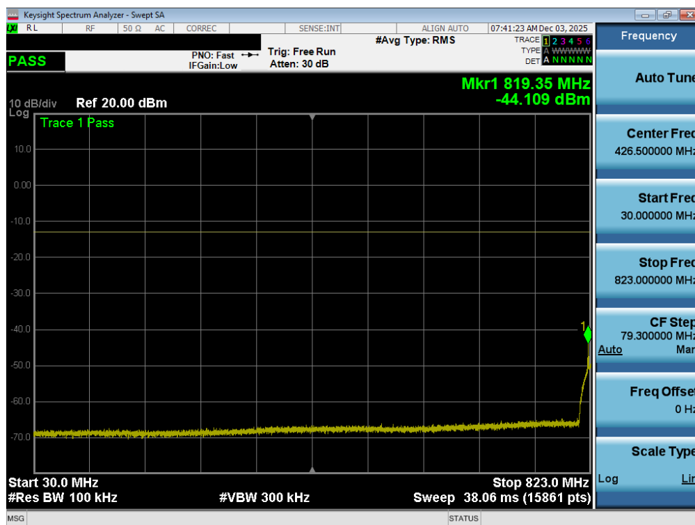
Plot 7-51. Conducted Spurious Plot (LTE Band 26/5 - 15MHz QPSK – 1 RB - Low Channel – Ant1)
