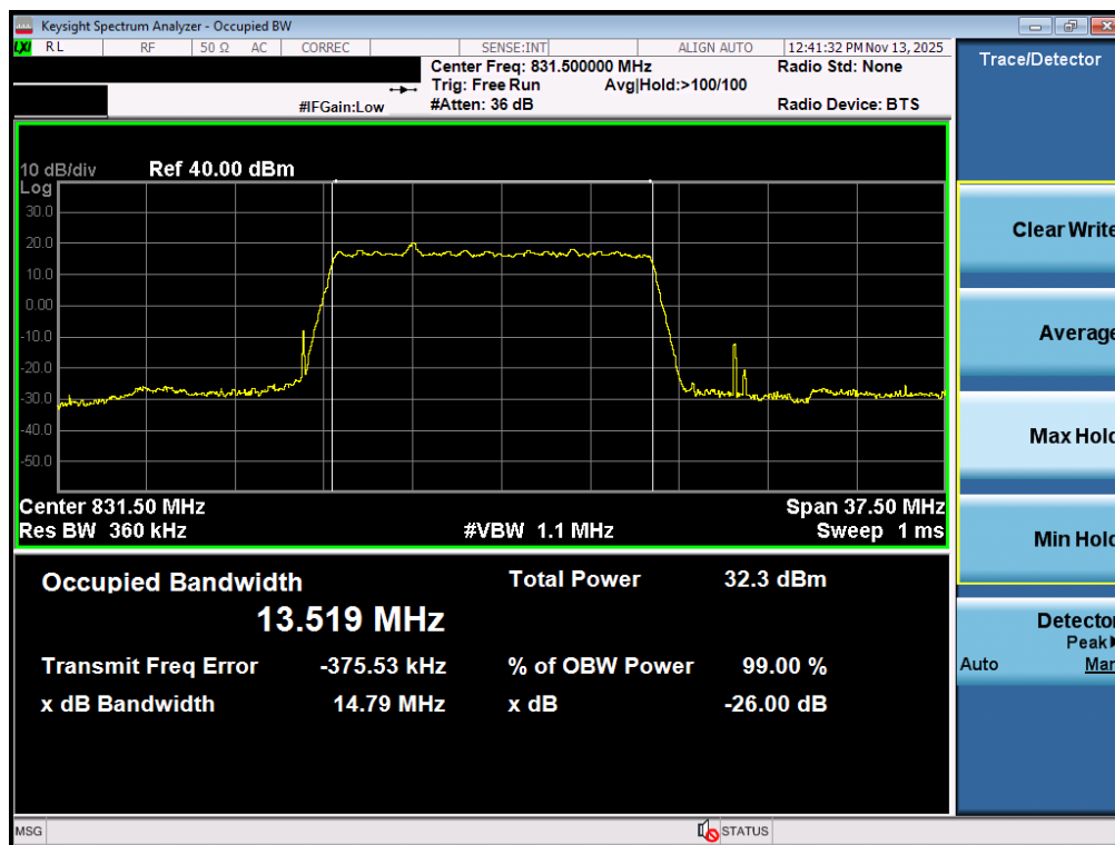
Plot 7-14. Occupied Bandwidth Plot (NR Band n26/5 - 15MHz \pi/2 BPSK - Full RB - Ant1)
