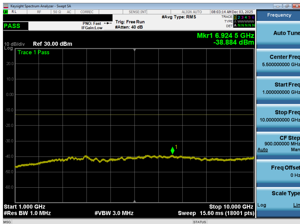
Plot 7-92. Conducted Spurious Plot (LTE Band 26/5 - 15MHz QPSK - 1 RB - Mid Channel – Ant2)
