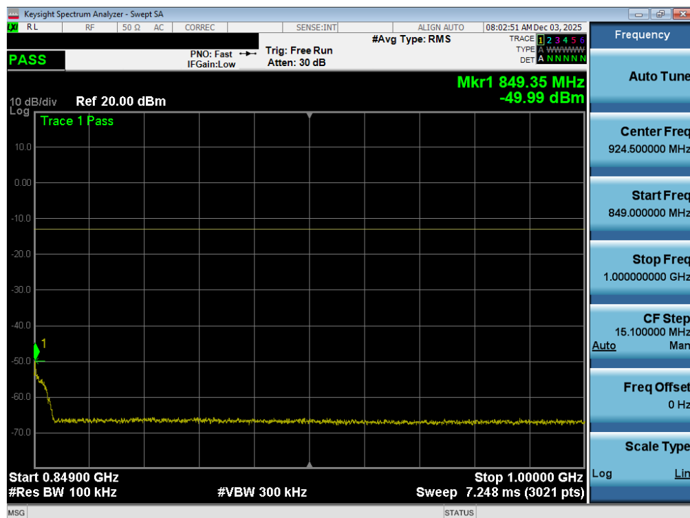
Plot 7-91. Conducted Spurious Plot (LTE Band 26/5 - 15MHz QPSK - 1 RB - Mid Channel – Ant2)
