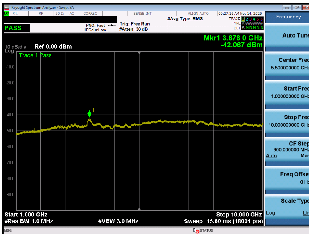
Plot 7-104. Conducted Spurious Plot (NR Band n26/5 - 20.0MHz - 1 RB - High Channel - Ant2)
