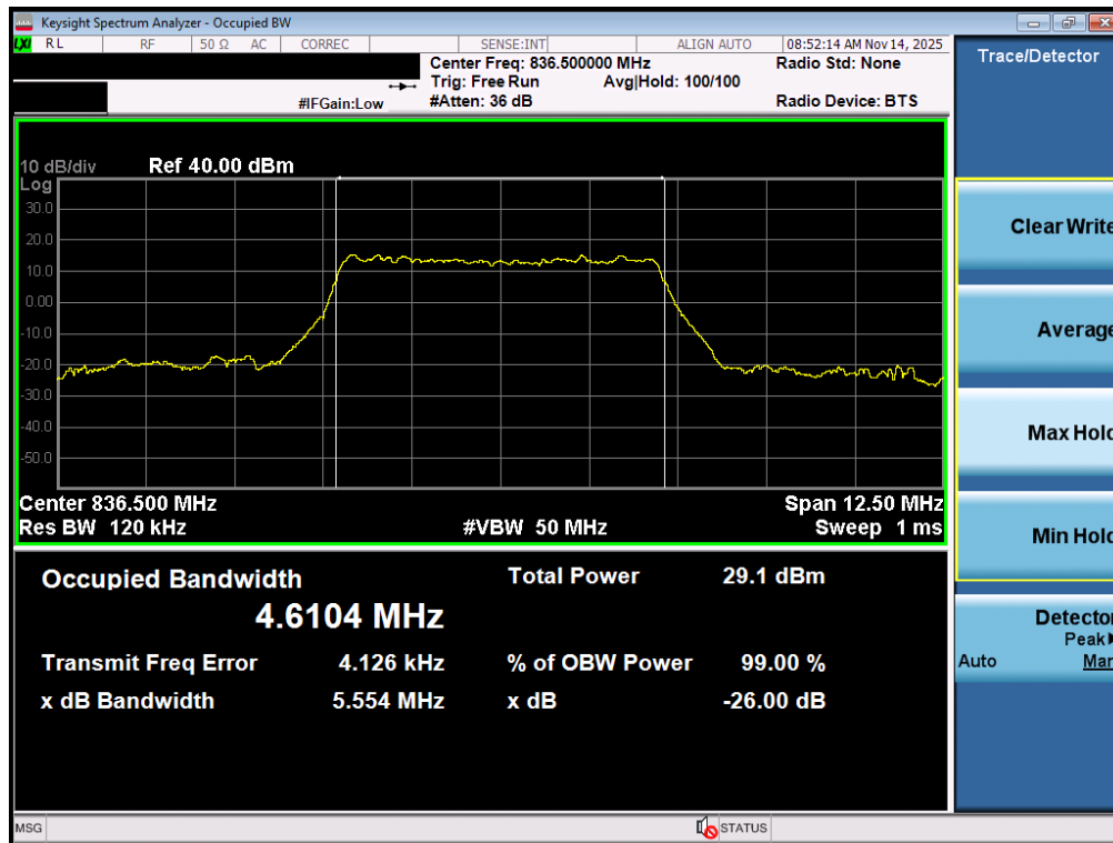
Plot 7-46. Occupied Bandwidth Plot (NR Band n26/5 - 5MHz QPSK - Full RB - Ant2)
