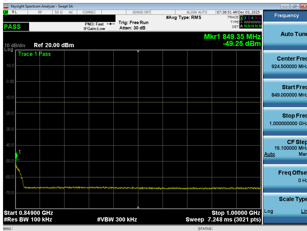
Plot 7-55. Conducted Spurious Plot (LTE Band 26/5 - 15MHz QPSK - 1 RB - Mid Channel – Ant1)
