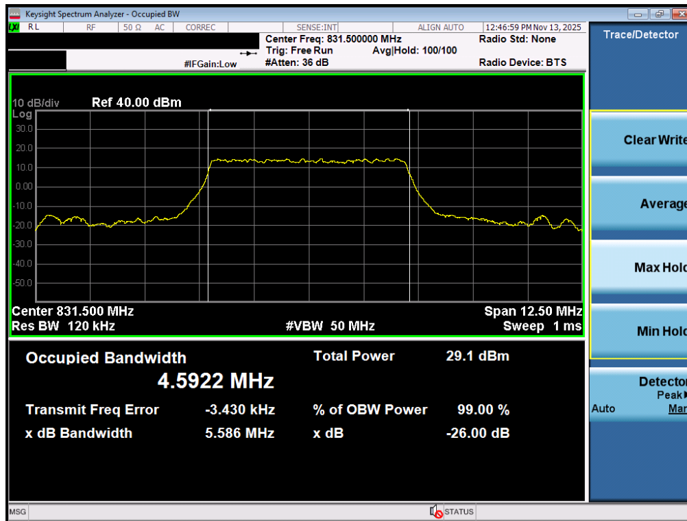
Plot 7-21. Occupied Bandwidth Plot (NR Band n26/5 - 5MHz QPSK - Full RB - Ant1)
