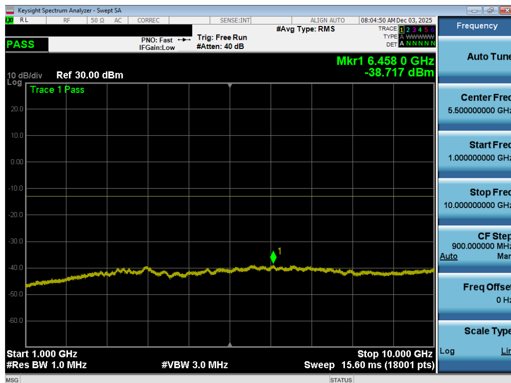
Plot 7-89. Conducted Spurious Plot (LTE Band 26/5 - 15MHz QPSK - 1 RB - Low Channel – Ant2)
