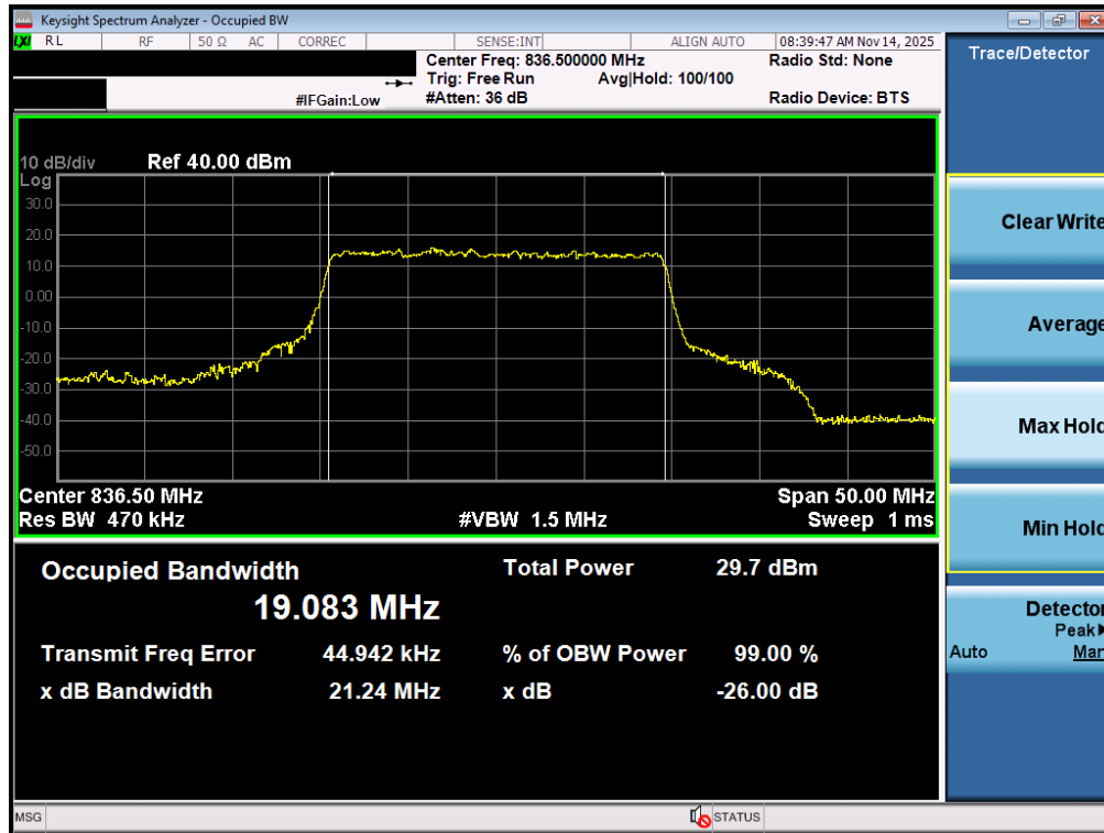
Plot 7-38. Occupied Bandwidth Plot (NR Band n26/5 - 20MHz 16-QAM - Full RB - Ant2)
