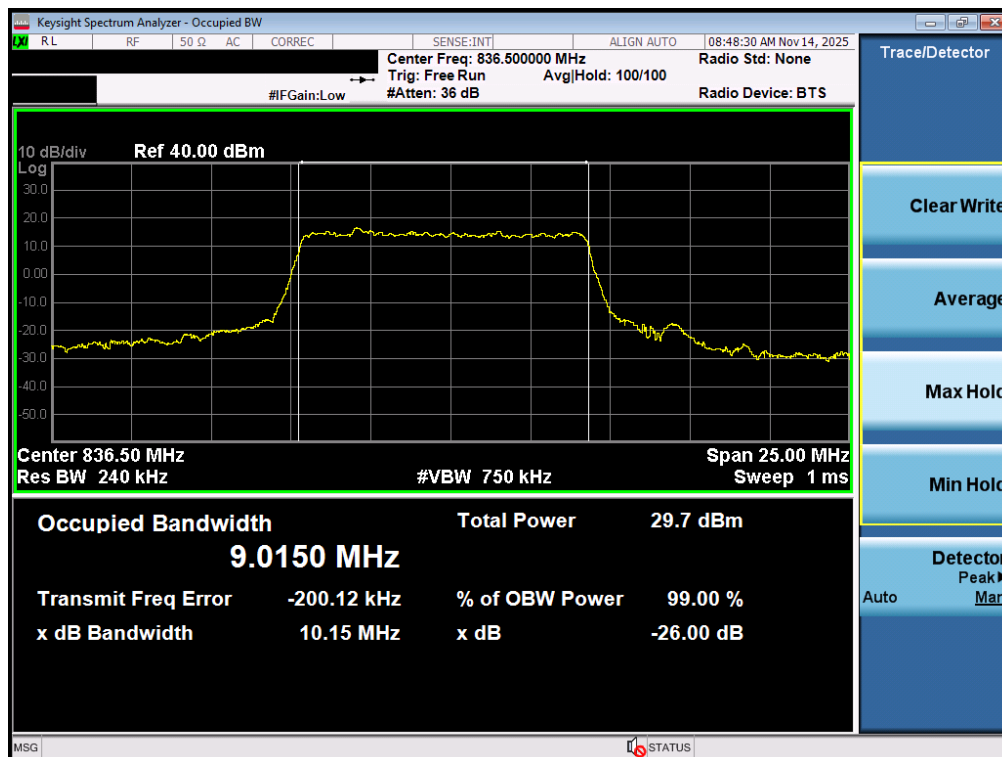
Plot 7-43. Occupied Bandwidth Plot (NR Band n26/5 - 10MHz QPSK - Full RB - Ant2)
