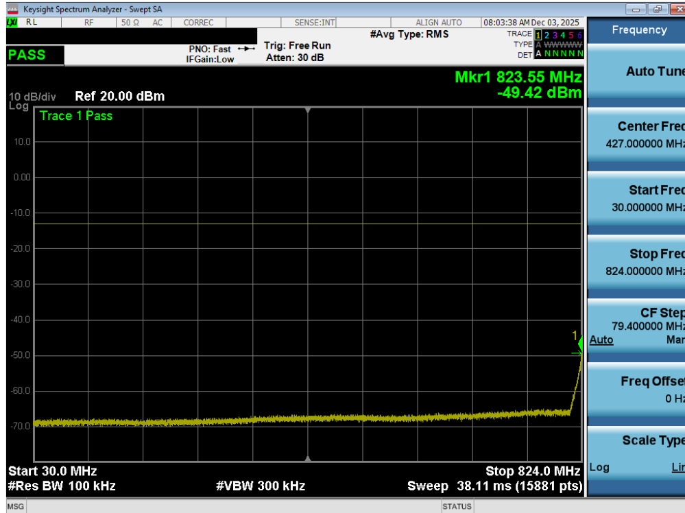
Plot 7-93. Conducted Spurious Plot (LTE Band 26/5 - 15MHz QPSK - 1 RB - High Channel – Ant2)
