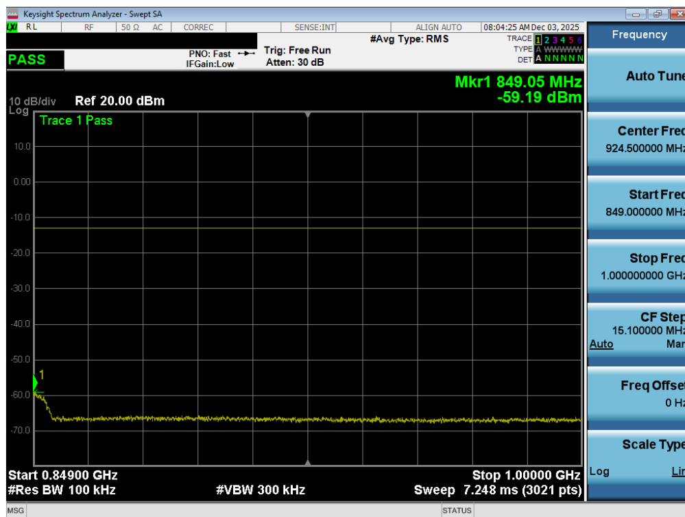
Plot 7-88. Conducted Spurious Plot (LTE Band 26/5 - 15MHz QPSK - 1 RB - Low Channel – Ant2)
