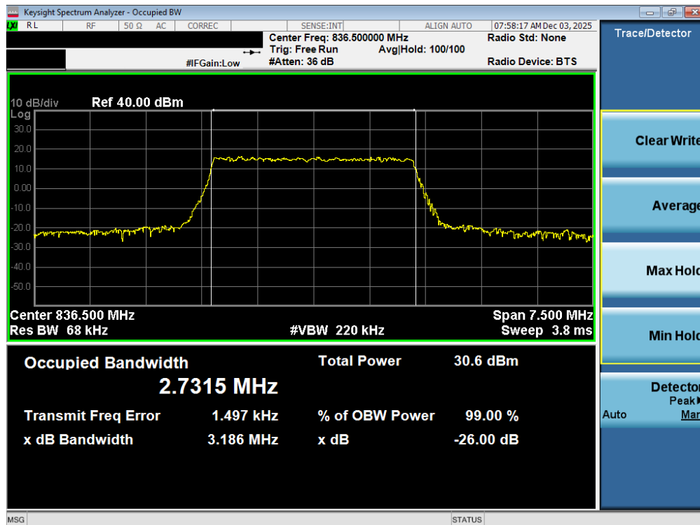
Plot 7-33. Occupied Bandwidth Plot (LTE Band 26/5 - 3MHz 16-QAM - Full RB - Ant2)
