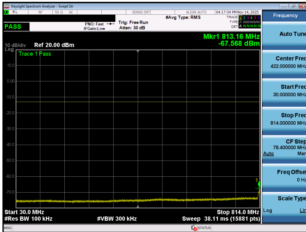
Plot 7-66. Conducted Spurious Plot (NR Band n26/5 - 20.0MHz - 1 RB - High Channel - Ant1)
