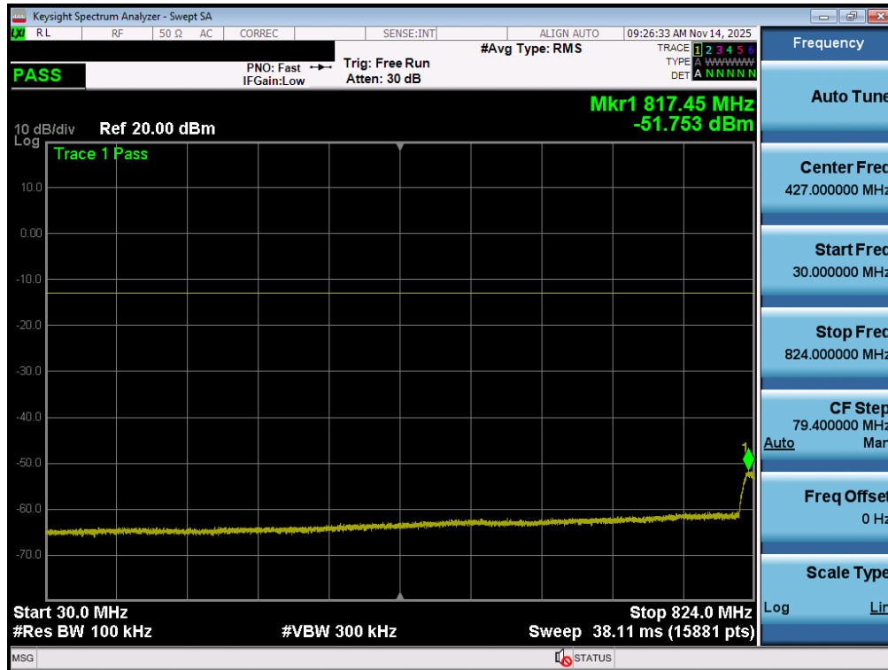
Plot 7-102. Conducted Spurious Plot (NR Band n26/5 - 20.0MHz - 1 RB - High Channel - Ant2)
