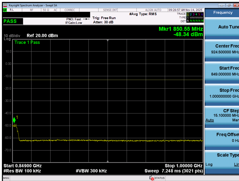
Plot 7-103. Conducted Spurious Plot (NR Band n26/5 - 20.0MHz - 1 RB - High Channel - Ant2)
