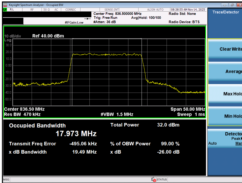
Plot 7-36. Occupied Bandwidth Plot (NR Band n26/5 - 20MHz \pi/2 BPSK - Full RB - Ant2)
