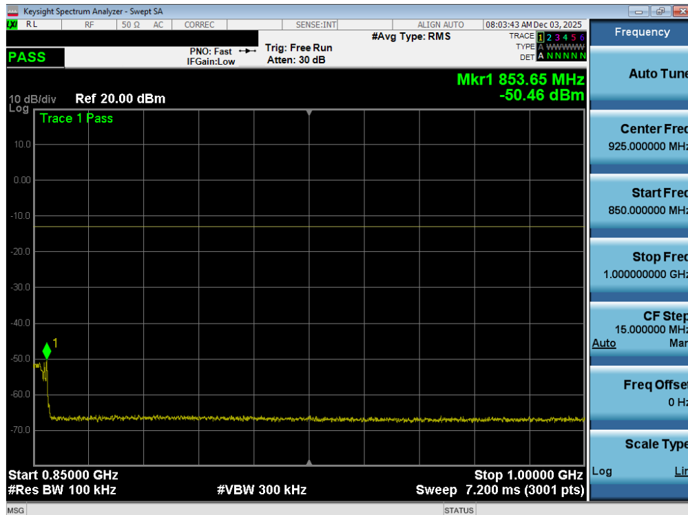
Plot 7-94. Conducted Spurious Plot (LTE Band 26/5 - 15MHz QPSK - 1 RB - High Channel – Ant2)
