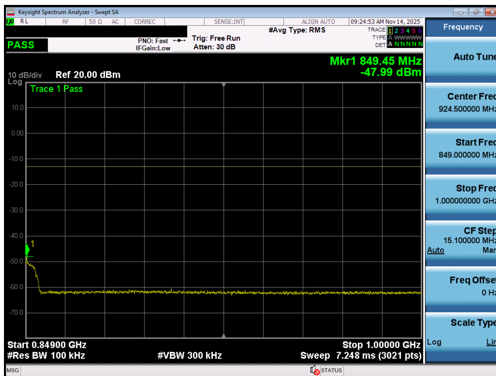
Plot 7-100. Conducted Spurious Plot (NR Band n26/5 - 20.0MHz - 1 RB - Mid Channel - Ant2)
