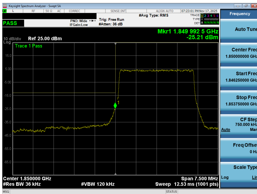
Plot 7-88. Lower Band Edge Plot (LTE Band 25/2 - 3MHz QPSK – Full RB - Ant1)
