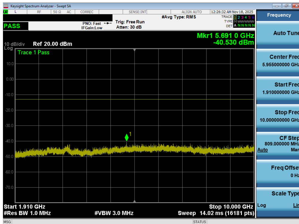
Plot 7-77. Conducted Spurious Plot (GPRS Ch. 661 - Ant1)
