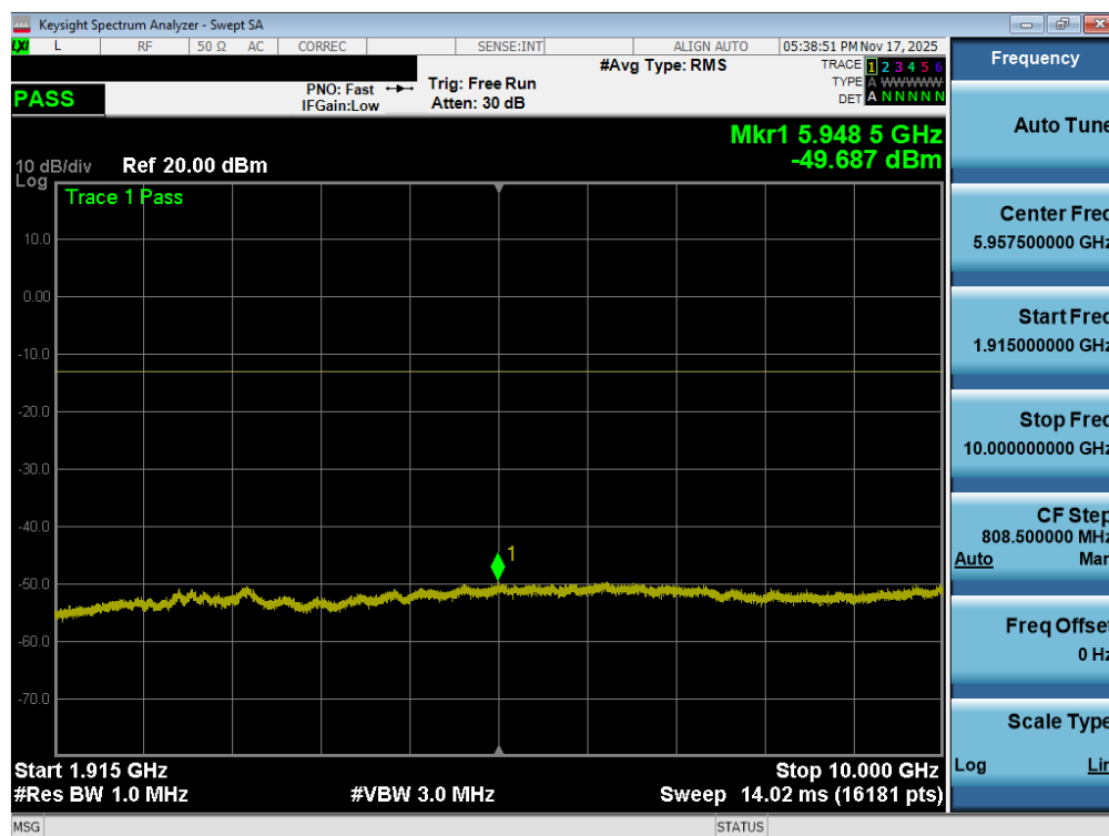
Plot 7-71. Conducted Spurious Plot (LTE Band 25/2 - 20MHz QPSK - 1RB - Low Channel - Ant1)
