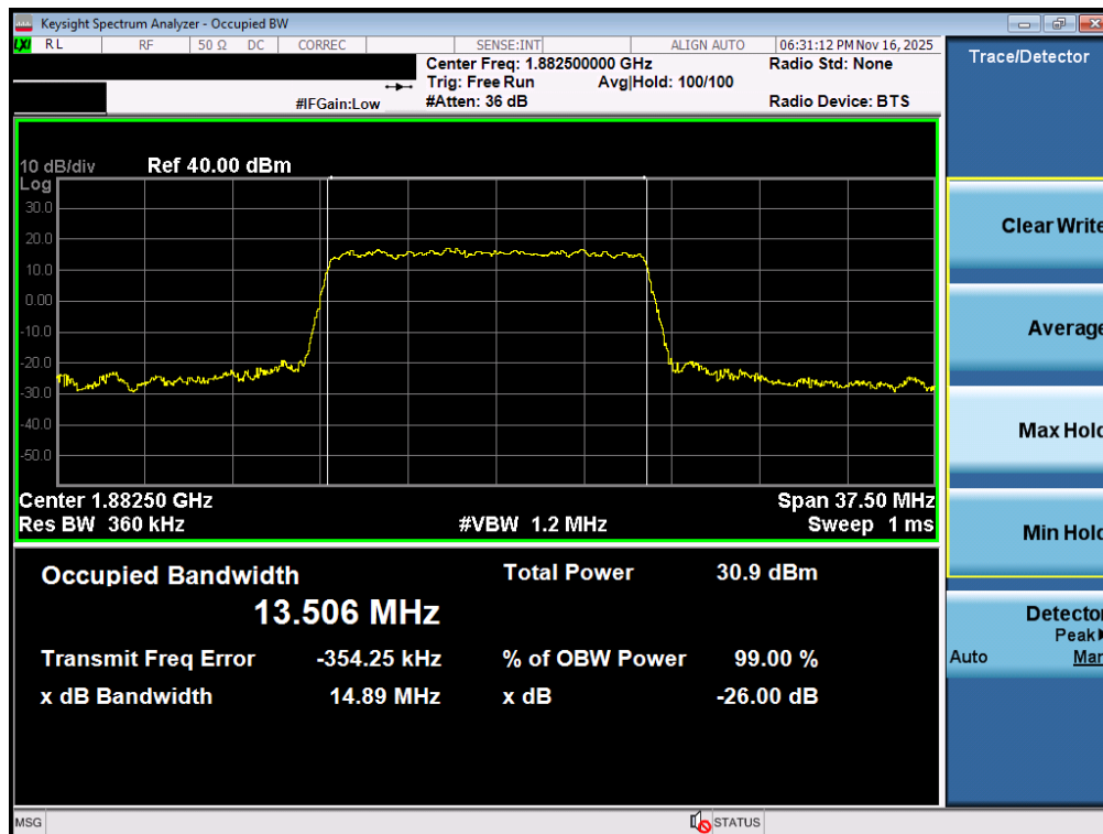
Plot 7-29. Occupied Bandwidth Plot (NR Band n25/2 - 15.0MHz CP-OFDM QPSK - Full RB - ANT1)
