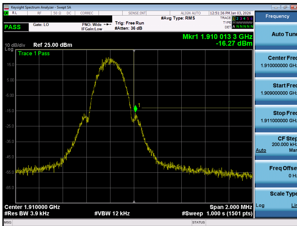
Plot 7-102. Upper Band Edge Plot (GPRS PCS – Ch. 810 - Ant1)
