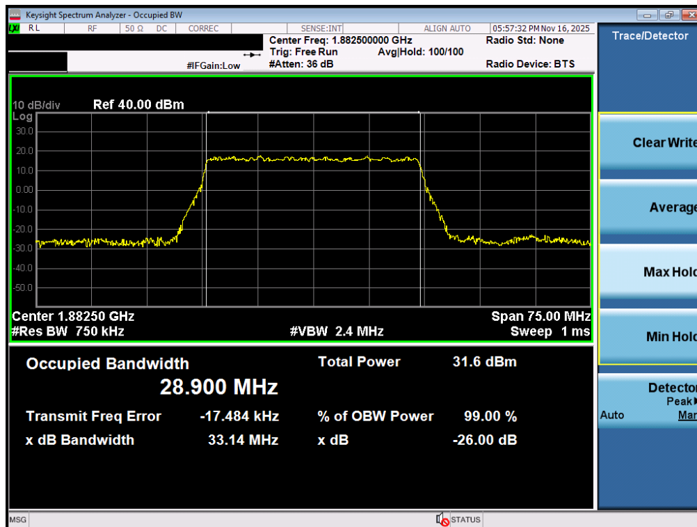
Plot 7-19. Occupied Bandwidth Plot (NR Band n25/2 - 30.0MHz DFT-s-OFDM BPSK - Full RB - ANT1)
