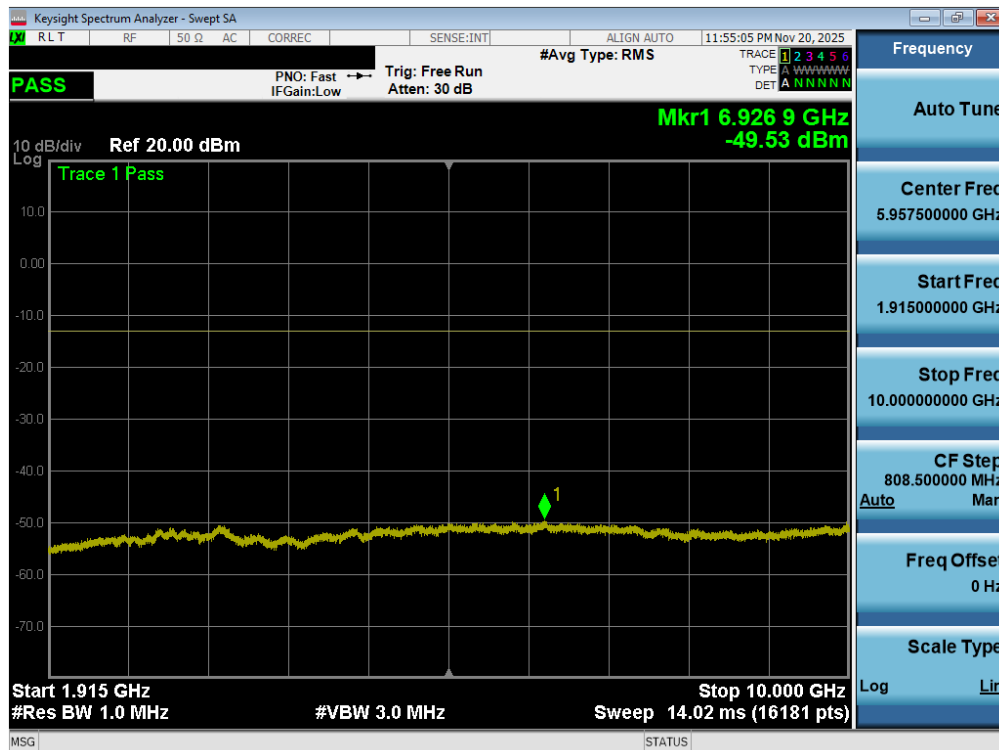
Plot 7-83. Conducted Spurious Plot (LTE Band 25/2 - 20MHz QPSK - 1RB - Low Channel - Ant2)
