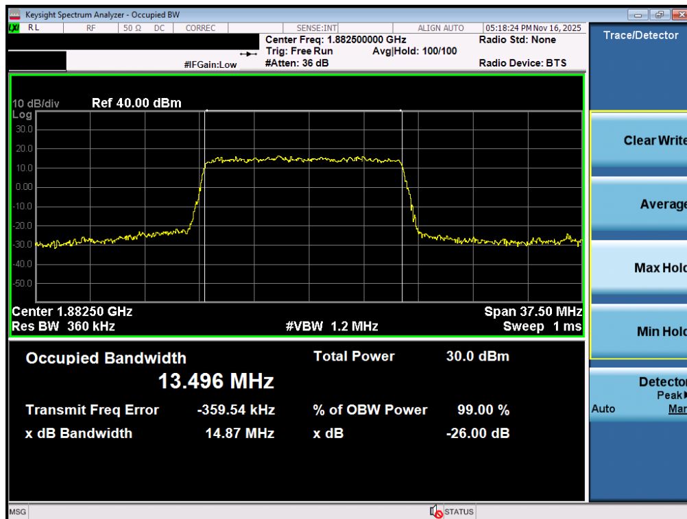
Plot 7-62. Occupied Bandwidth Plot (NR Band n25/2 - 15.0MHz CP-OFDM QPSK - Full RB - ANT2)
