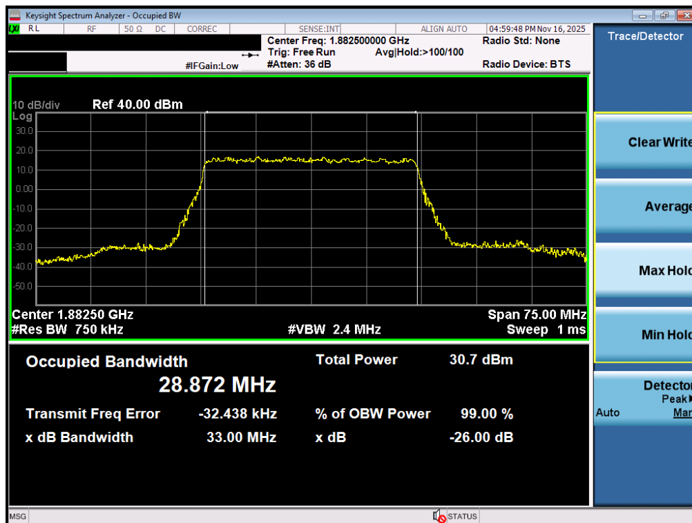
Plot 7-52. Occupied Bandwidth Plot (NR Band n25/2 - 30.0MHz DFT-s-OFDM BPSK - Full RB - ANT2)
