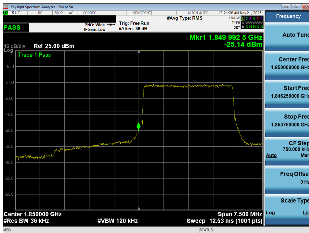
Plot 7-108. Lower Band Edge Plot (LTE Band 25/2 - 3MHz QPSK – Full RB - Ant2)
