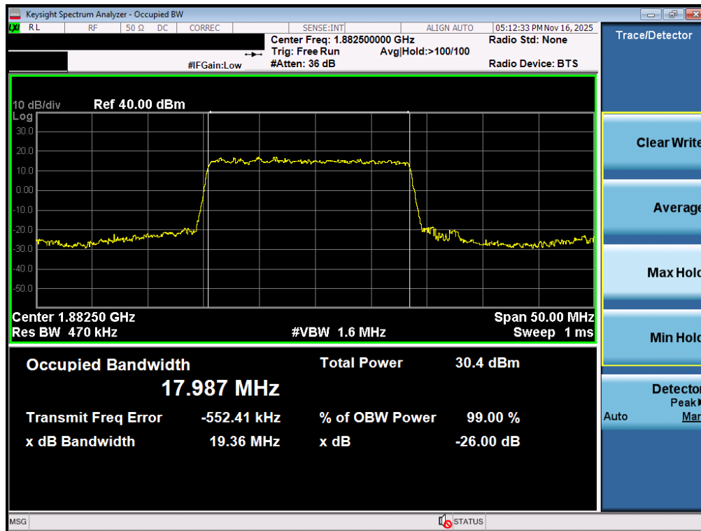
Plot 7-59. Occupied Bandwidth Plot (NR Band n25/2 - 20.0MHz CP-OFDM QPSK - Full RB - ANT2)
