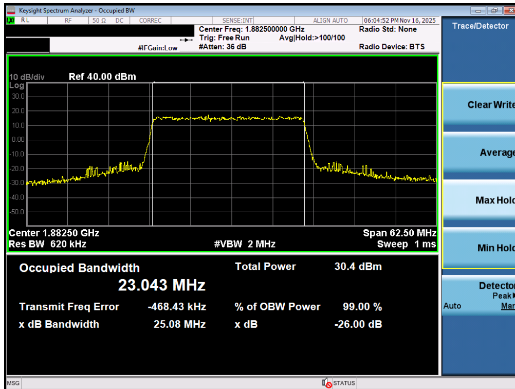
Plot 7-24. Occupied Bandwidth Plot (NR Band n25/2 - 25.0MHz CP-OFDM 16QAM - Full RB - ANT1)
