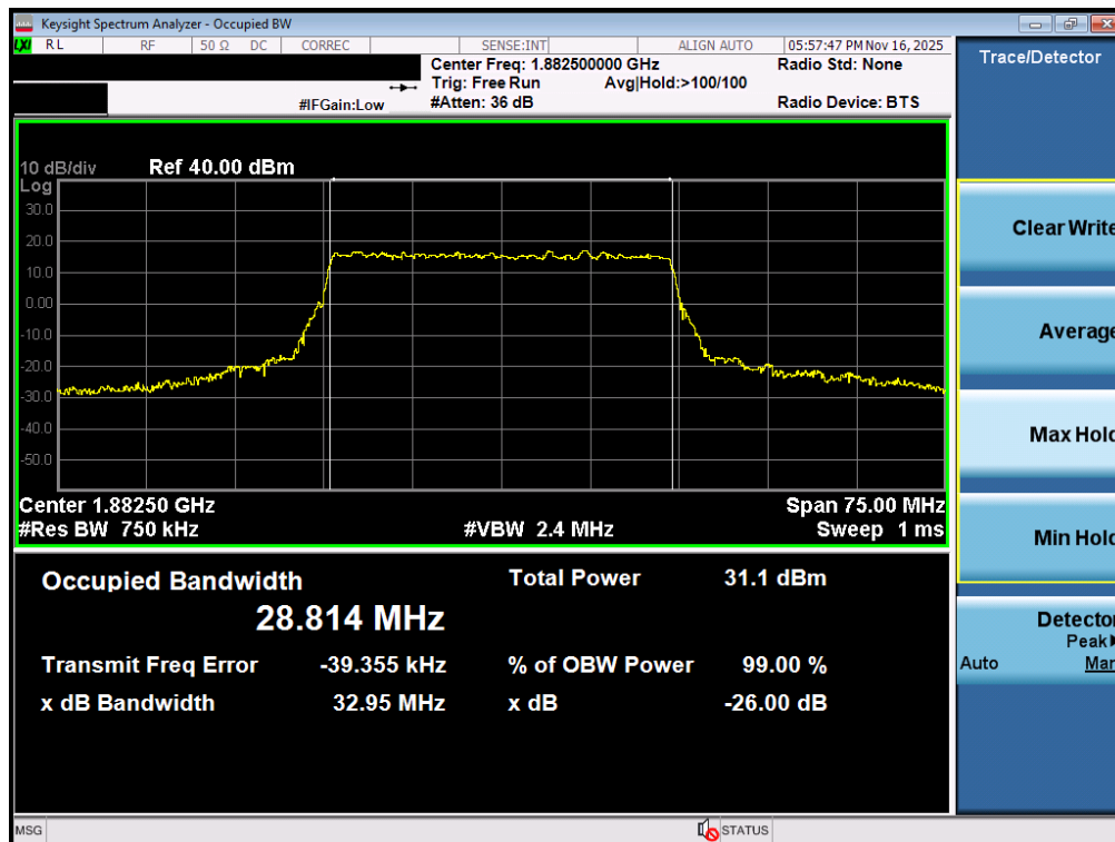
Plot 7-21. Occupied Bandwidth Plot (NR Band n25/2 - 30.0MHz CP-OFDM 16QAM - Full RB - ANT1)
