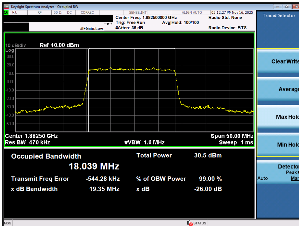
Plot 7-58. Occupied Bandwidth Plot (NR Band n25/2 - 20.0MHz DFT-s-OFDM BPSK - Full RB - ANT2)
