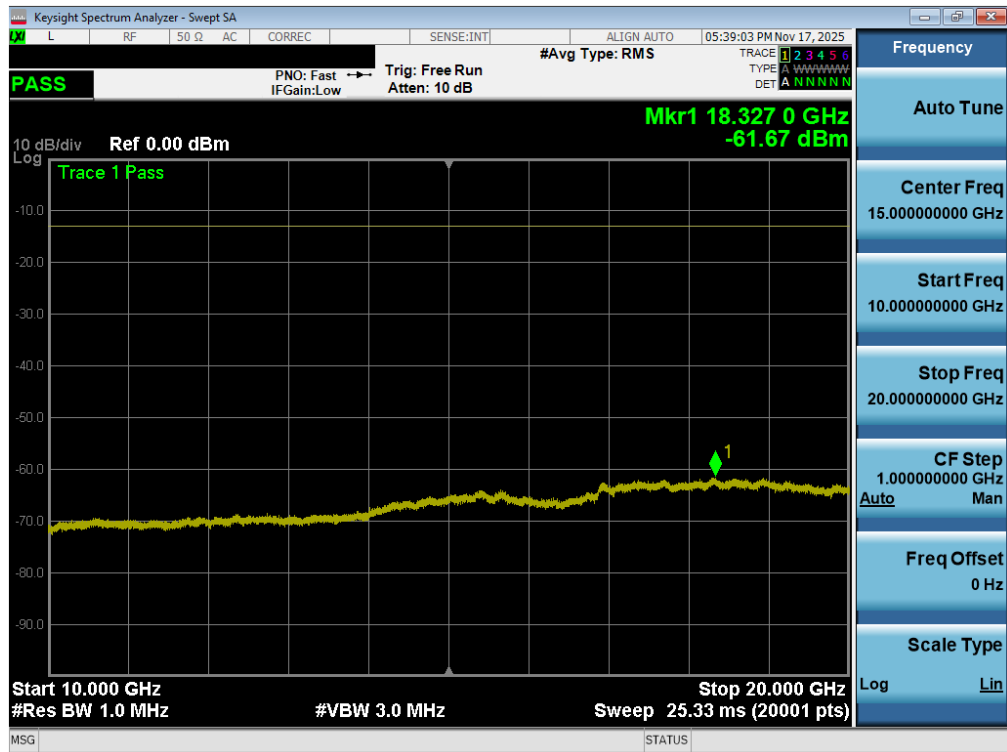
Plot 7-72. Conducted Spurious Plot (LTE Band 25/2 - 20MHz QPSK - 1RB - Low Channel - Ant1)
