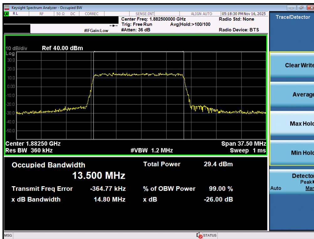
Plot 7-63. Occupied Bandwidth Plot (NR Band n25/2 - 15.0MHz CP-OFDM 16QAM - Full RB - ANT2)
