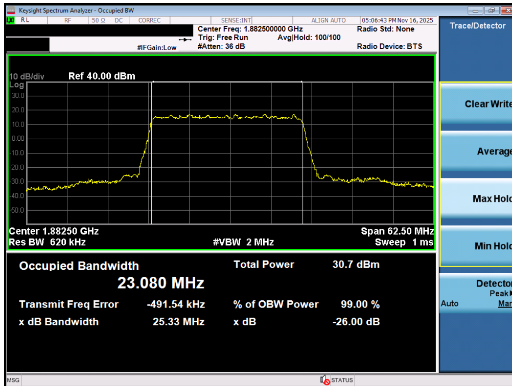
Plot 7-55. Occupied Bandwidth Plot (NR Band n25/2 - 25.0MHz DFT-s-OFDM BPSK - Full RB - ANT2)
