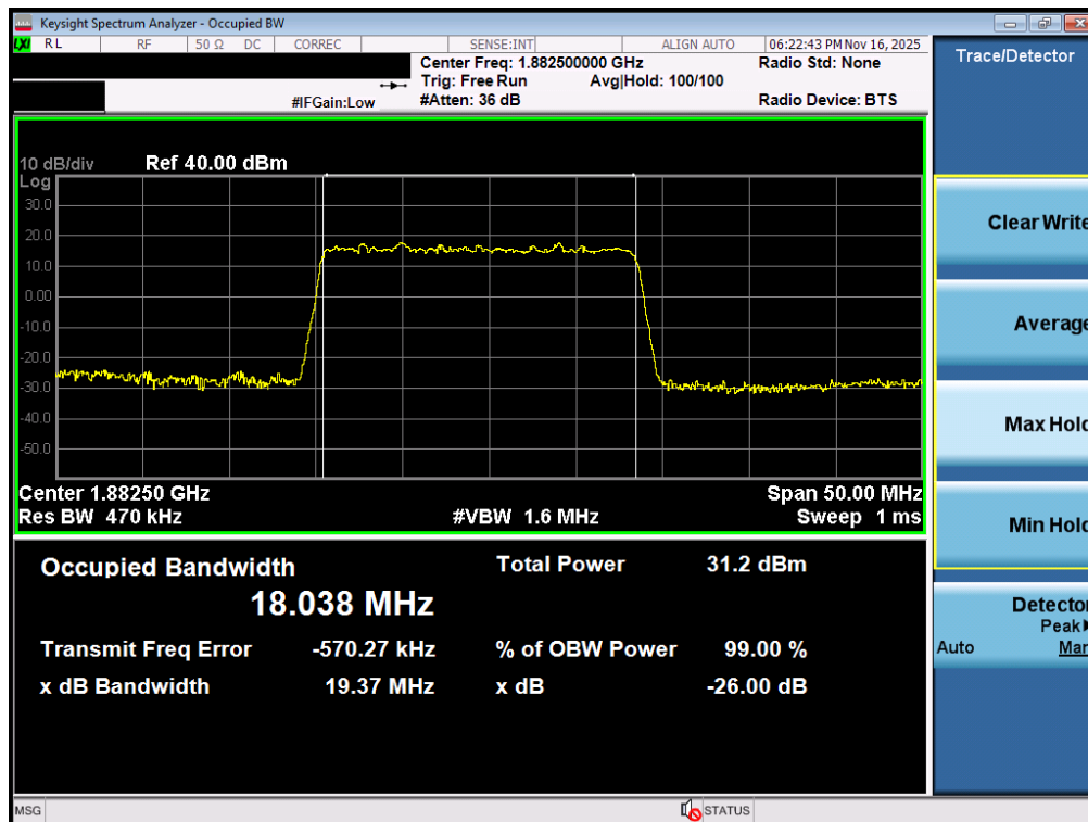
Plot 7-25. Occupied Bandwidth Plot (NR Band n25/2 - 20.0MHz DFT-s-OFDM BPSK - Full RB - ANT1)
