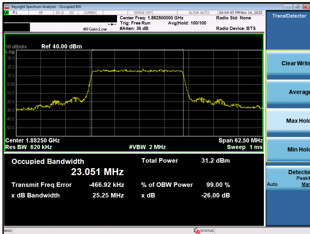
Plot 7-23. Occupied Bandwidth Plot (NR Band n25/2 - 25.0MHz CP-OFDM QPSK - Full RB - ANT1)
