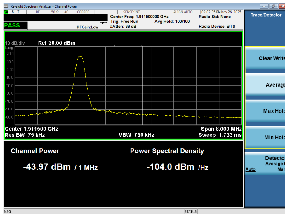
Plot 7-103. Extended Upper Band Edge Plot (GPRS PCS – Ch. 810 - Ant1)
