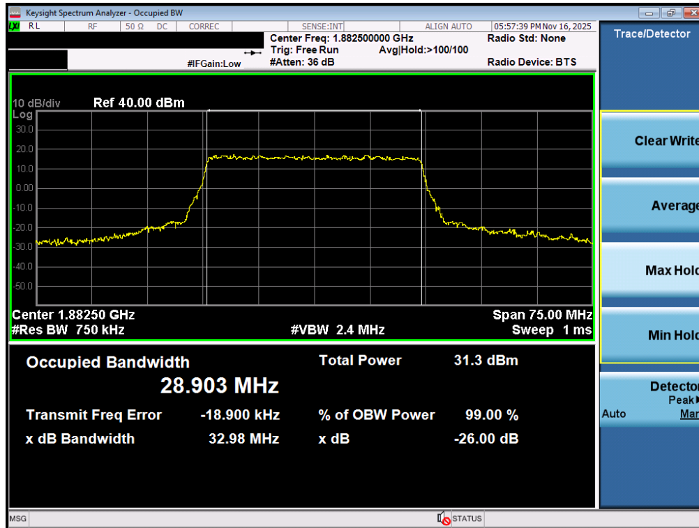
Plot 7-20. Occupied Bandwidth Plot (NR Band n25/2 - 30.0MHz CP-OFDM QPSK - Full RB - ANT1)
