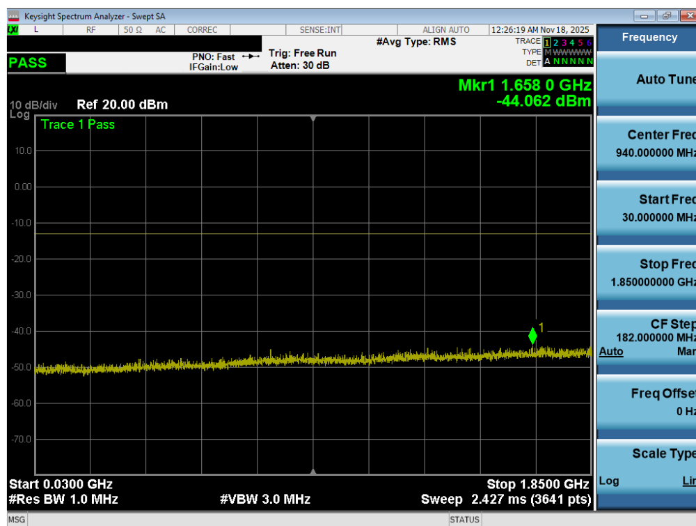
Plot 7-76. Conducted Spurious Plot (GPRS Ch. 661 - Ant1)
