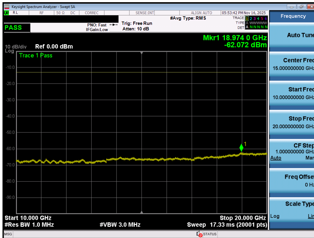
Plot 7-75. Conducted Spurious Plot (NR Band n25/2 - 40.0MHz - 1RB - High Channel - Ant1)
