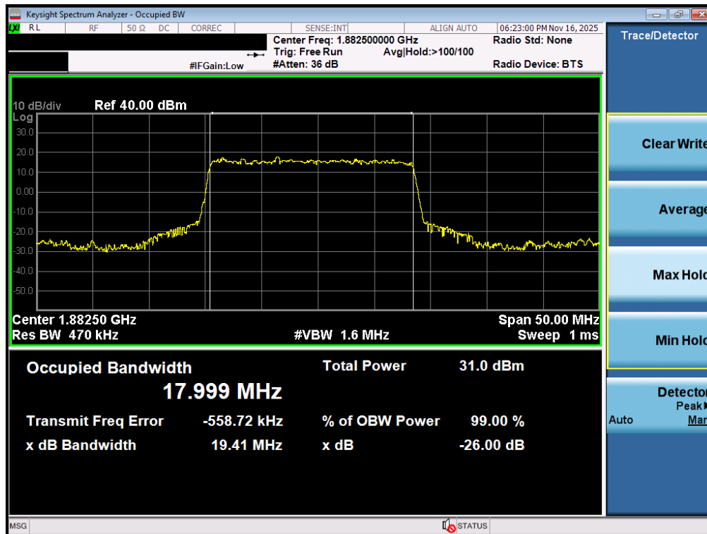
Plot 7-26. Occupied Bandwidth Plot (NR Band n25/2 - 20.0MHz CP-OFDM QPSK - Full RB - ANT1)
