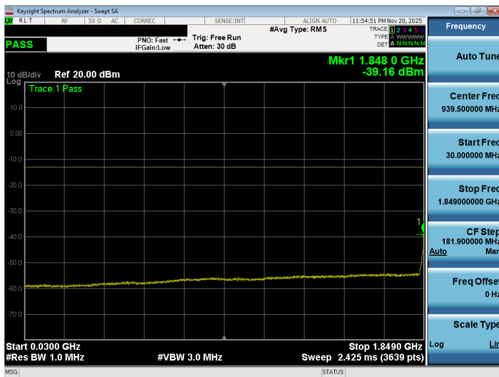
Plot 7-82. Conducted Spurious Plot (LTE Band 25/2 - 20MHz QPSK - 1RB - Low Channel - Ant2)
