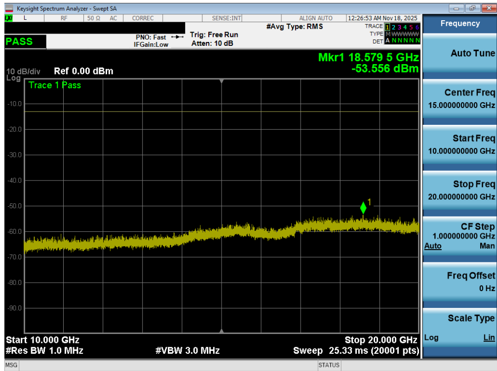
Plot 7-78. Conducted Spurious Plot (GPRS Ch. 661 - Ant1)
