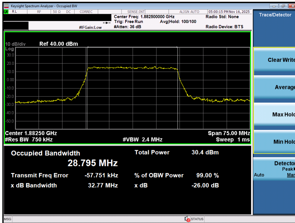
Plot 7-53. Occupied Bandwidth Plot (NR Band n25/2 - 30.0MHz CP-OFDM QPSK - Full RB - ANT2)
