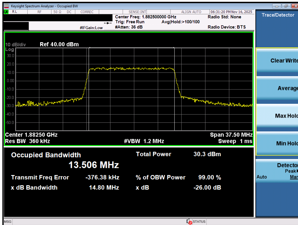
Plot 7-30. Occupied Bandwidth Plot (NR Band n25/2 - 15.0MHz CP-OFDM 16QAM - Full RB - ANT1)
