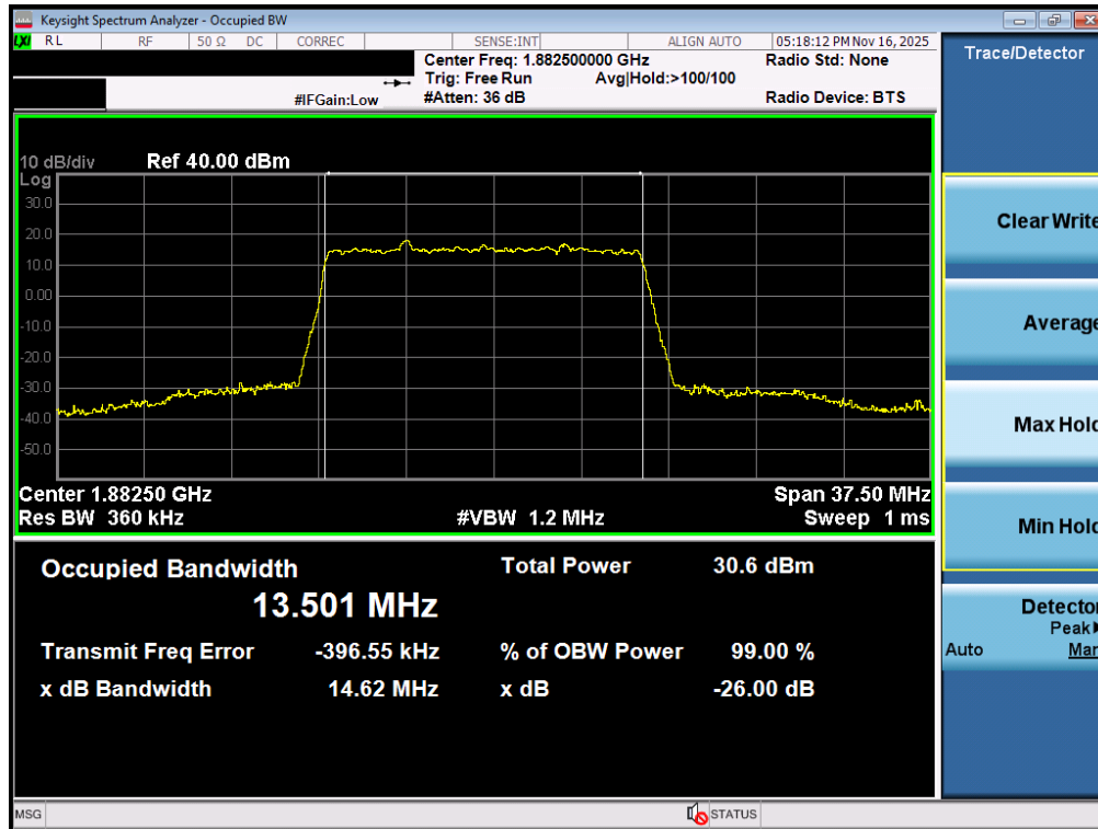
Plot 7-61. Occupied Bandwidth Plot (NR Band n25/2 - 15.0MHz DFT-s-OFDM BPSK - Full RB - ANT2)
