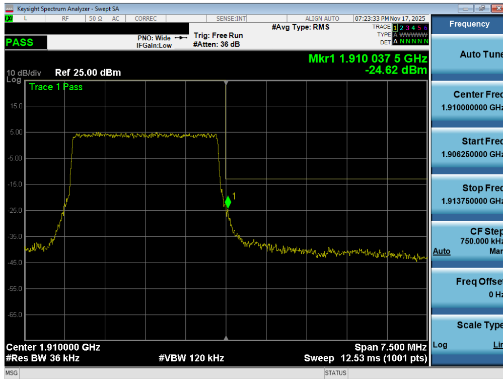
Plot 7-90. Upper Band Edge Plot (LTE Band 2 - 3MHz QPSK – Full RB - Ant1)
