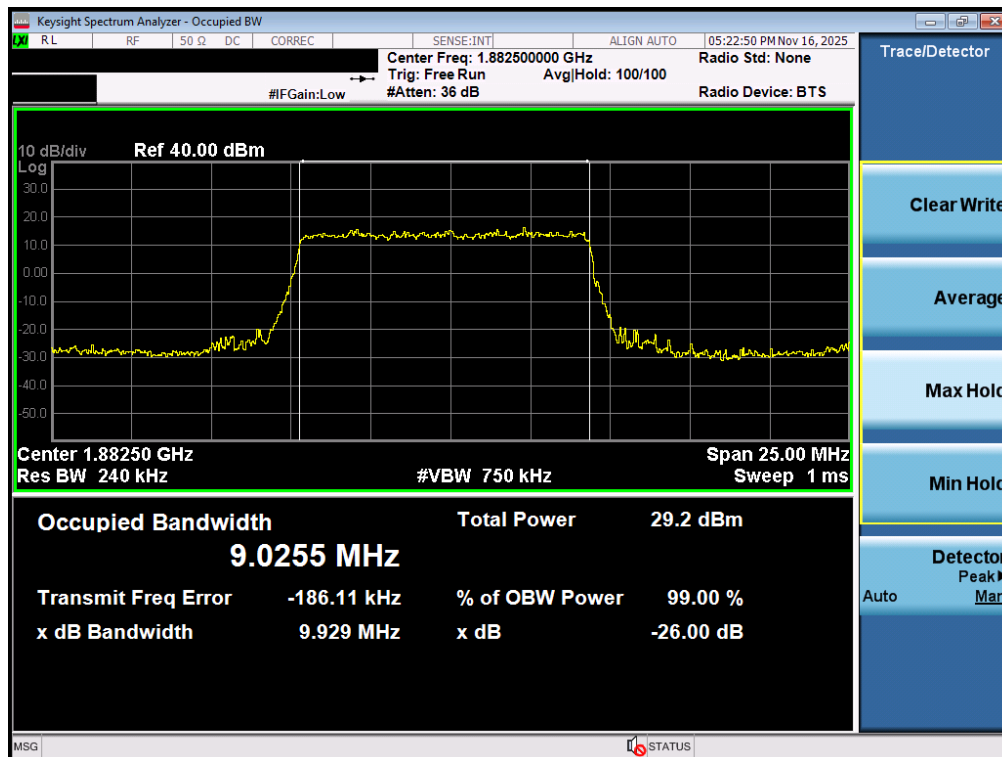
Plot 7-66. Occupied Bandwidth Plot (NR Band n25/2 - 10.0MHz CP-OFDM 16QAM - Full RB - ANT2)
