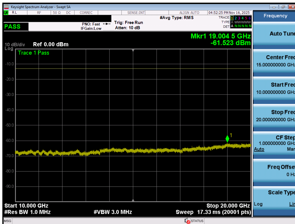
Plot 7-87. Conducted Spurious Plot (NR Band n25/2 - 40.0MHz - 1RB - Low Channel - Ant2)
