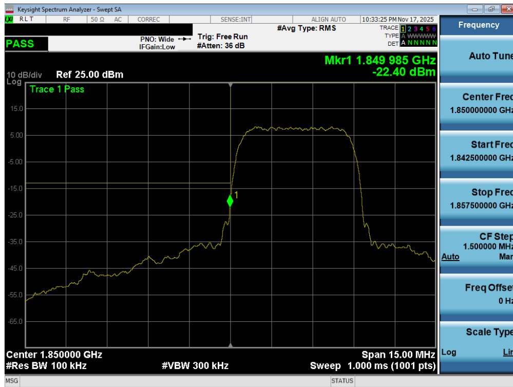
Plot 7-104. Lower Band Edge Plot (WCDMA PCS – Ch. 9262 - Ant1)
