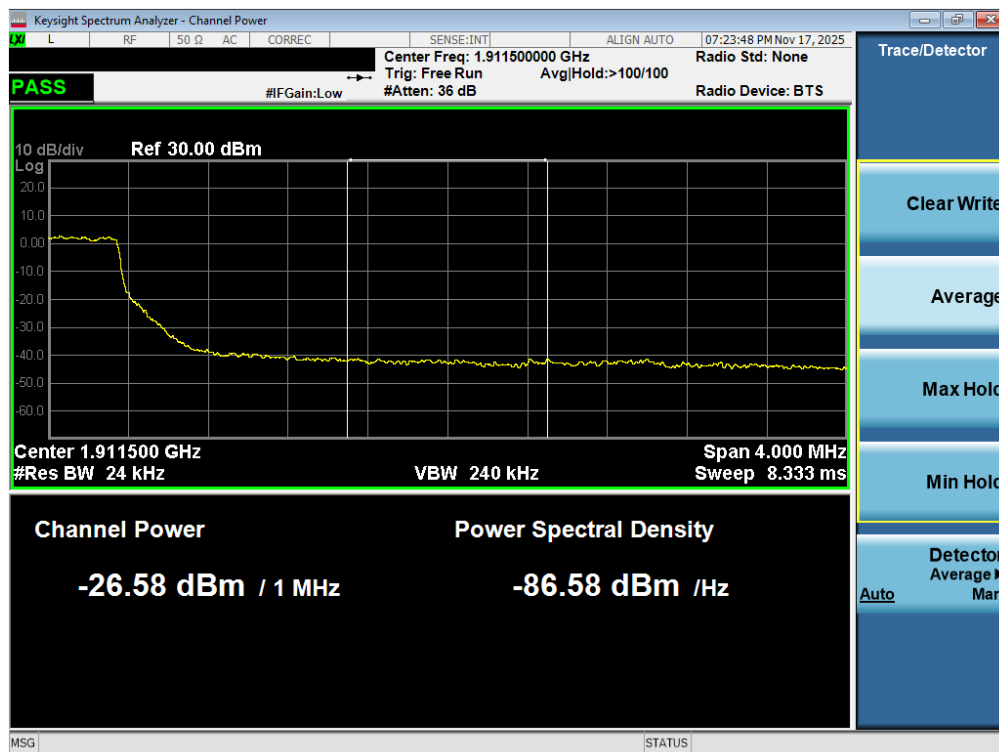
Plot 7-91. Extended Upper Band Edge Plot (LTE Band 2 - 3MHz QPSK – Full RB - Ant1)
