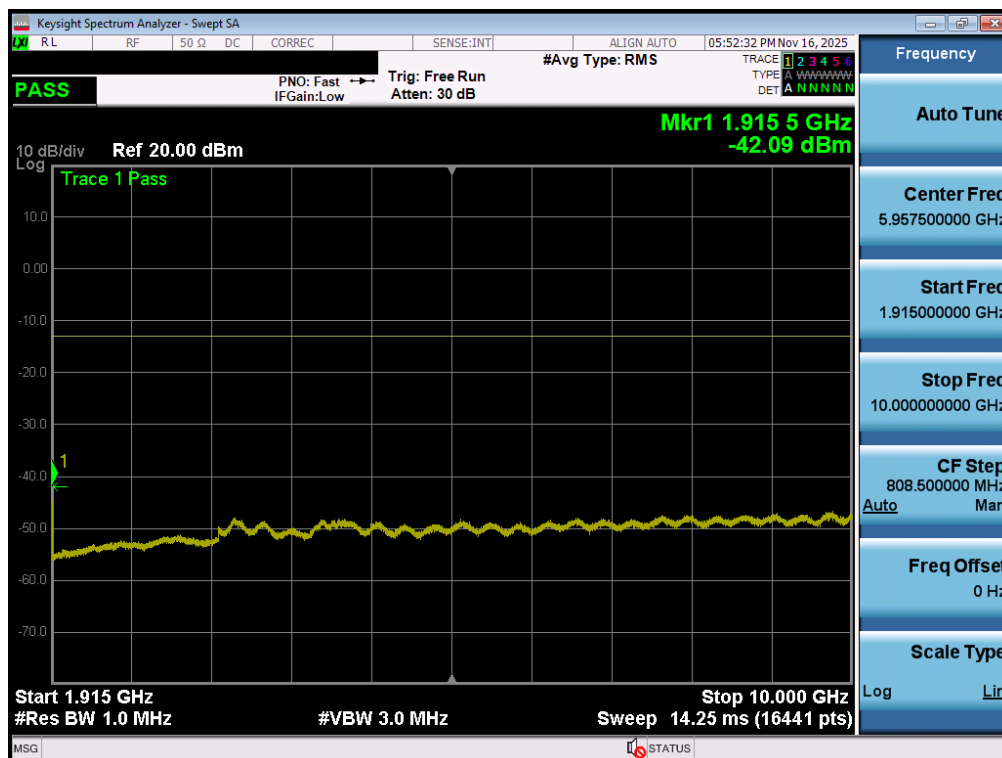
Plot 7-74. Conducted Spurious Plot (NR Band n25/2 - 40.0MHz - 1RB - High Channel - Ant1)
