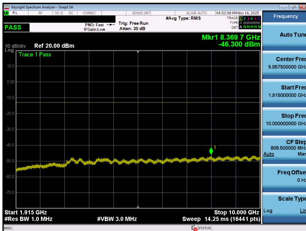
Plot 7-86. Conducted Spurious Plot (NR Band n25/2 - 40.0MHz - 1RB - Low Channel - Ant2)
