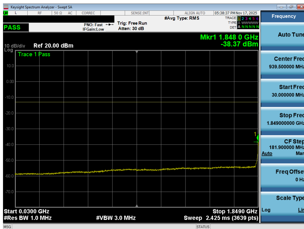
Plot 7-70. Conducted Spurious Plot (LTE Band 25/2 - 20MHz QPSK - 1RB - Low Channel - Ant1)
