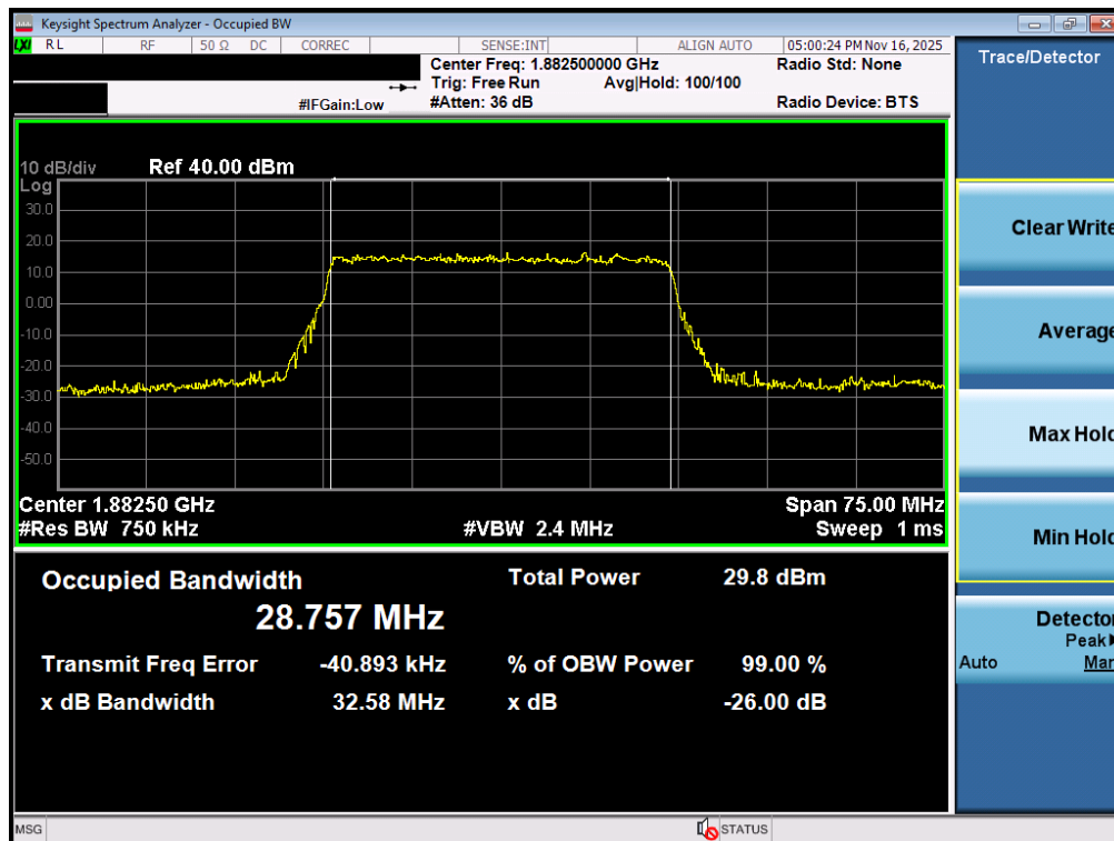
Plot 7-54. Occupied Bandwidth Plot (NR Band n25/2 - 30.0MHz CP-OFDM 16QAM - Full RB - ANT2)
