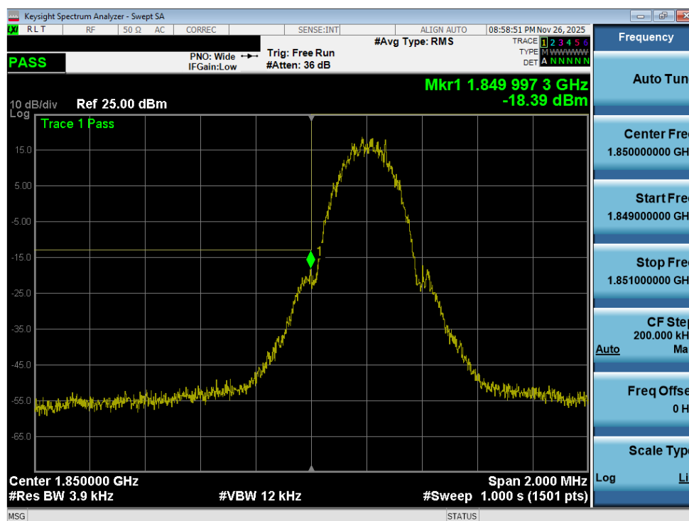
Plot 7-100. Lower Band Edge Plot (GPRS PCS – Ch. 512 - Ant1)
