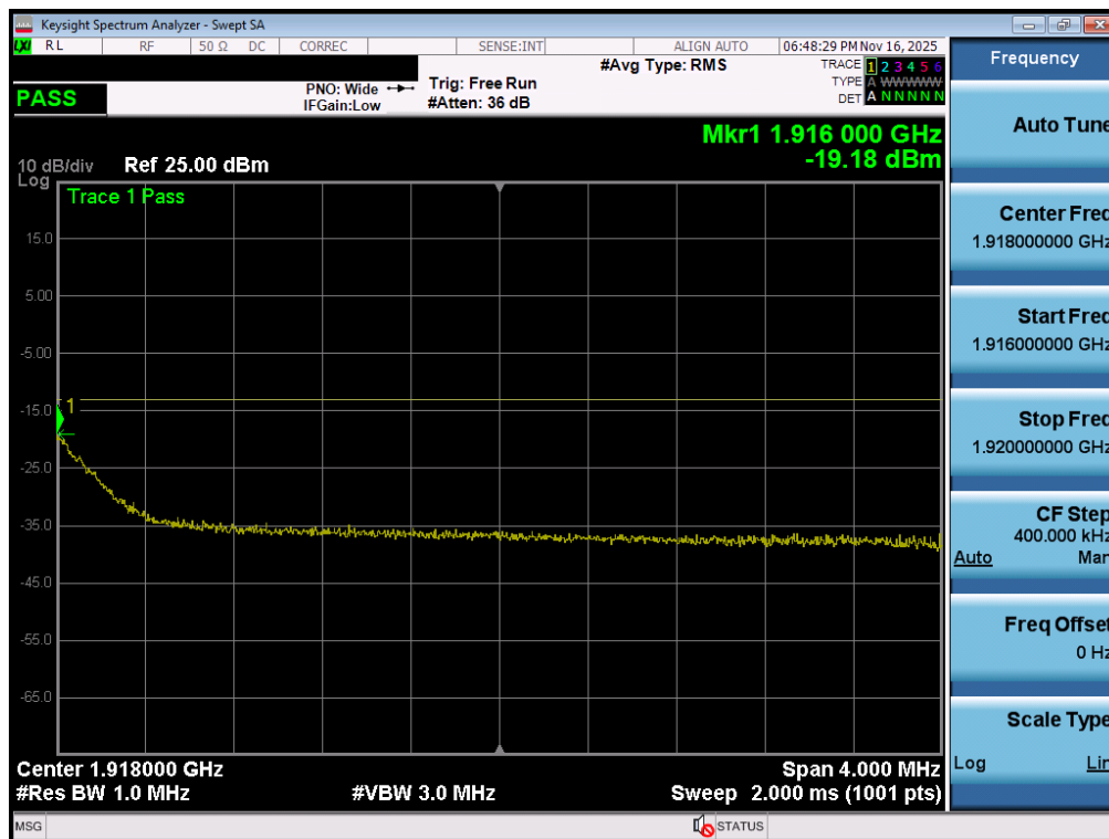
Plot 7-99. Extended Upper Band Edge Plot (NR Band n25 - 10MHz QPSK – Full RB - Ant1)
