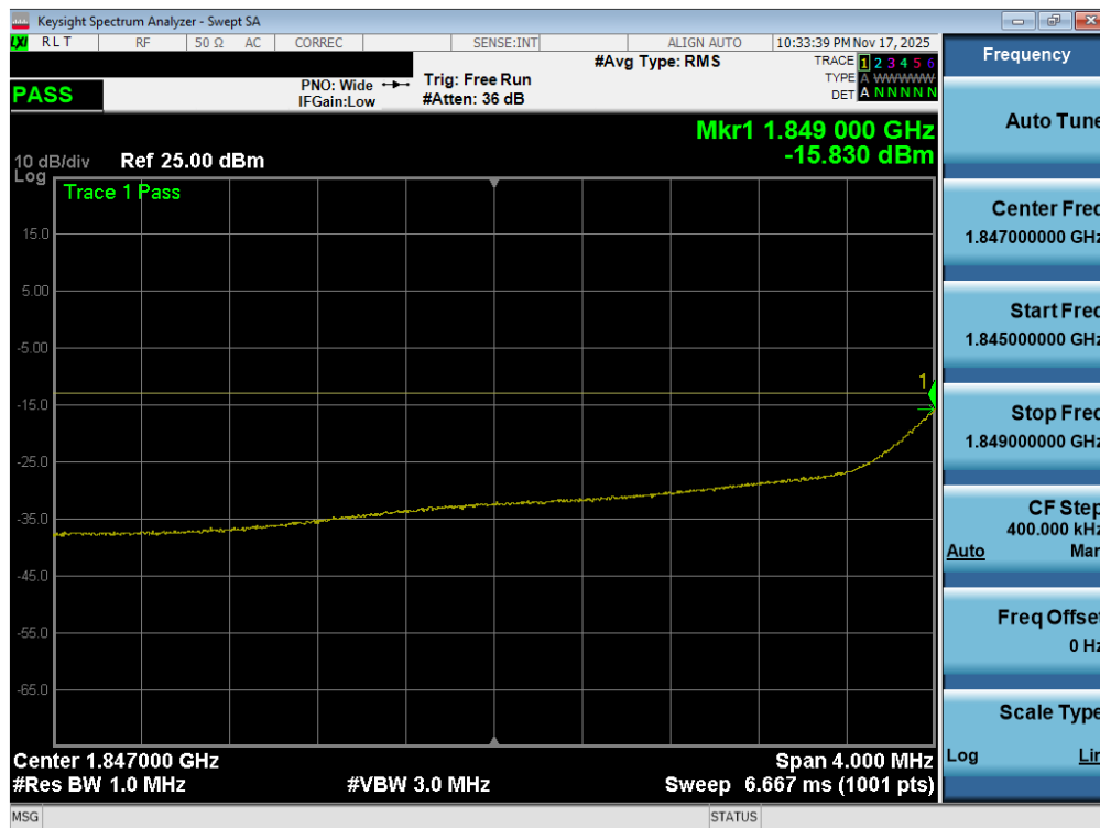
Plot 7-105. Extended Lower Band Edge Plot (WCDMA PCS – Ch. 9262 - Ant1)
