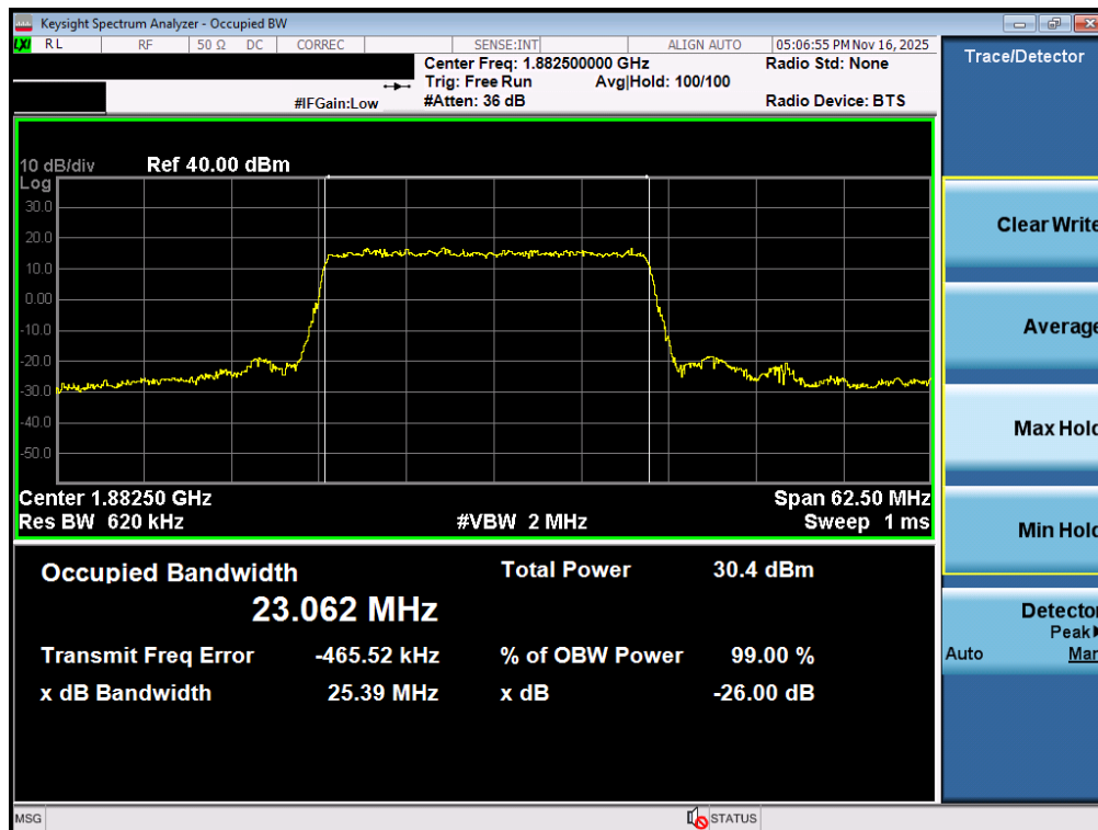
Plot 7-56. Occupied Bandwidth Plot (NR Band n25/2 - 25.0MHz CP-OFDM QPSK - Full RB - ANT2)
