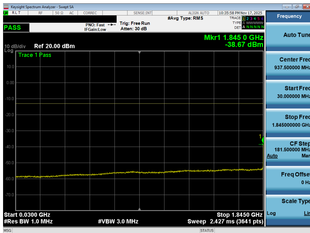
Plot 7-79. Conducted Spurious Plot (WCDMA Ch. 9262 - Ant1)
