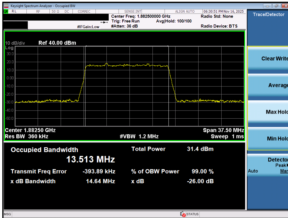
Plot 7-28. Occupied Bandwidth Plot (NR Band n25/2 - 15.0MHz DFT-s-OFDM BPSK - Full RB - ANT1)
