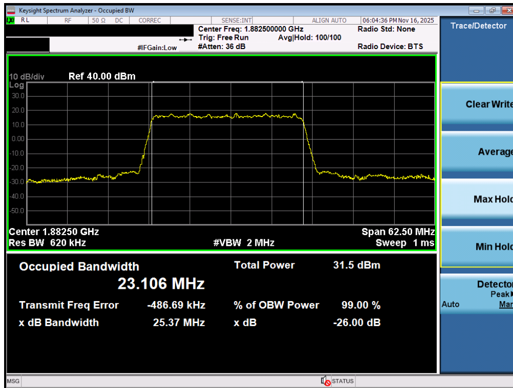
Plot 7-22. Occupied Bandwidth Plot (NR Band n25/2 - 25.0MHz DFT-s-OFDM BPSK - Full RB - ANT1)
