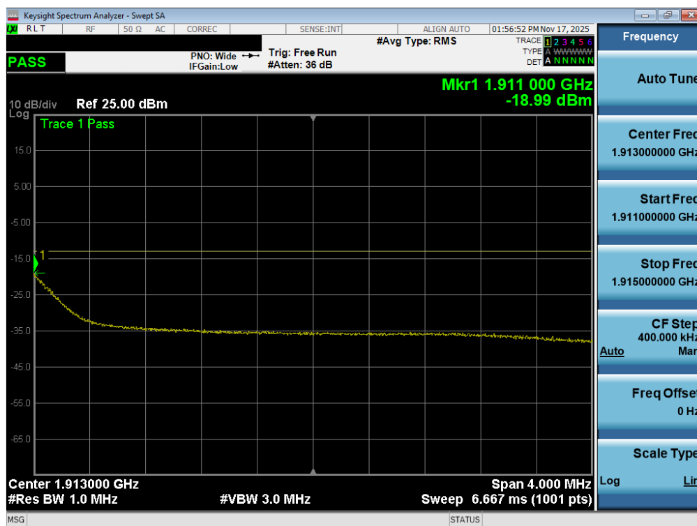
Plot 7-97. Extended Upper Band Edge Plot (NR Band n2 - 10MHz QPSK – Full RB - Ant1)
