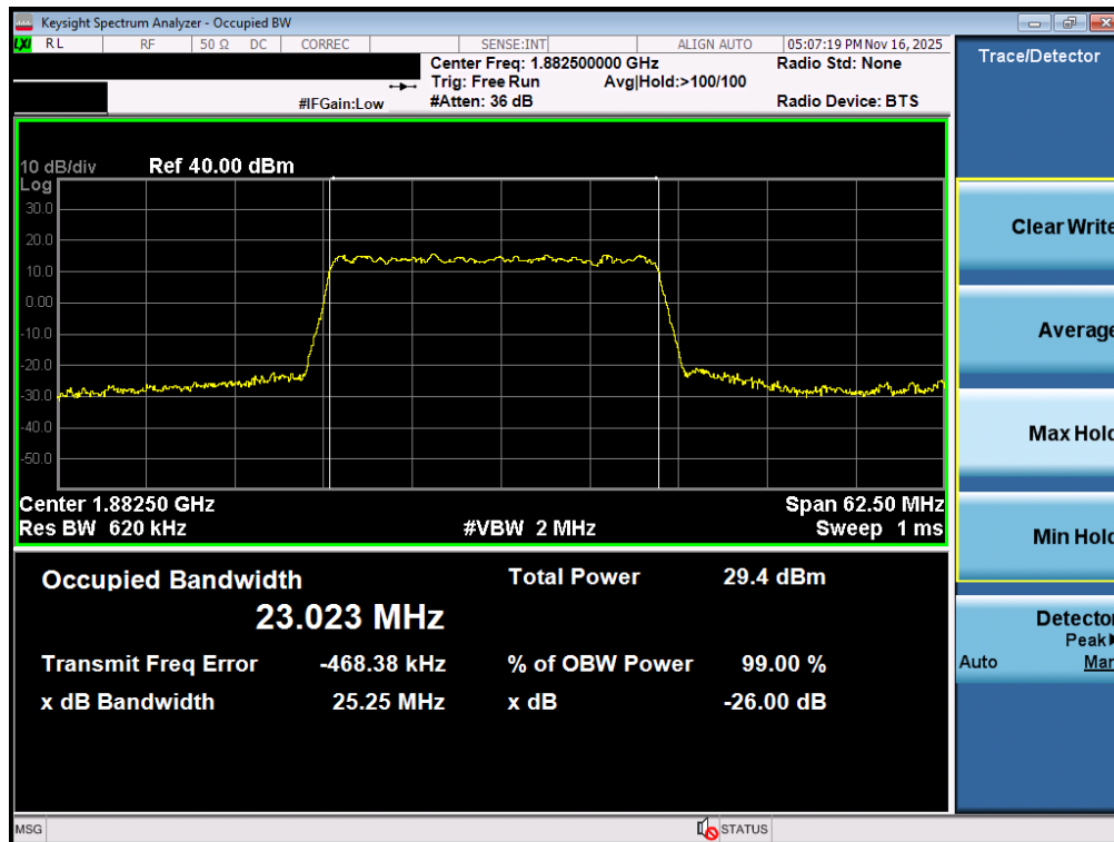
Plot 7-57. Occupied Bandwidth Plot (NR Band n25/2 - 25.0MHz CP-OFDM 16QAM - Full RB - ANT2)
