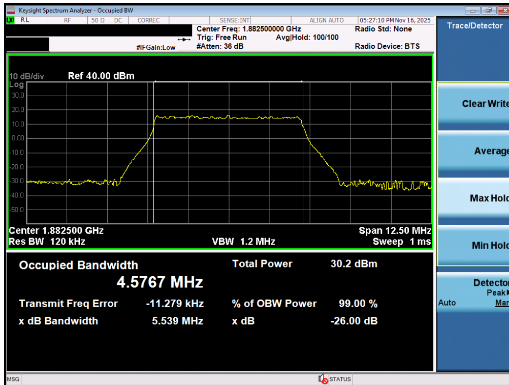
Plot 7-67. Occupied Bandwidth Plot (NR Band n25/2 - 5.0MHz DFT-s-OFDM BPSK - Full RB - ANT2)
