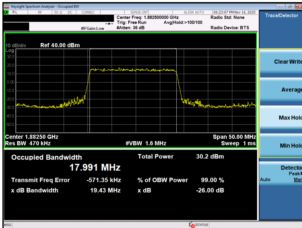
Plot 7-27. Occupied Bandwidth Plot (NR Band n25/2 - 20.0MHz CP-OFDM 16QAM - Full RB - ANT1)
