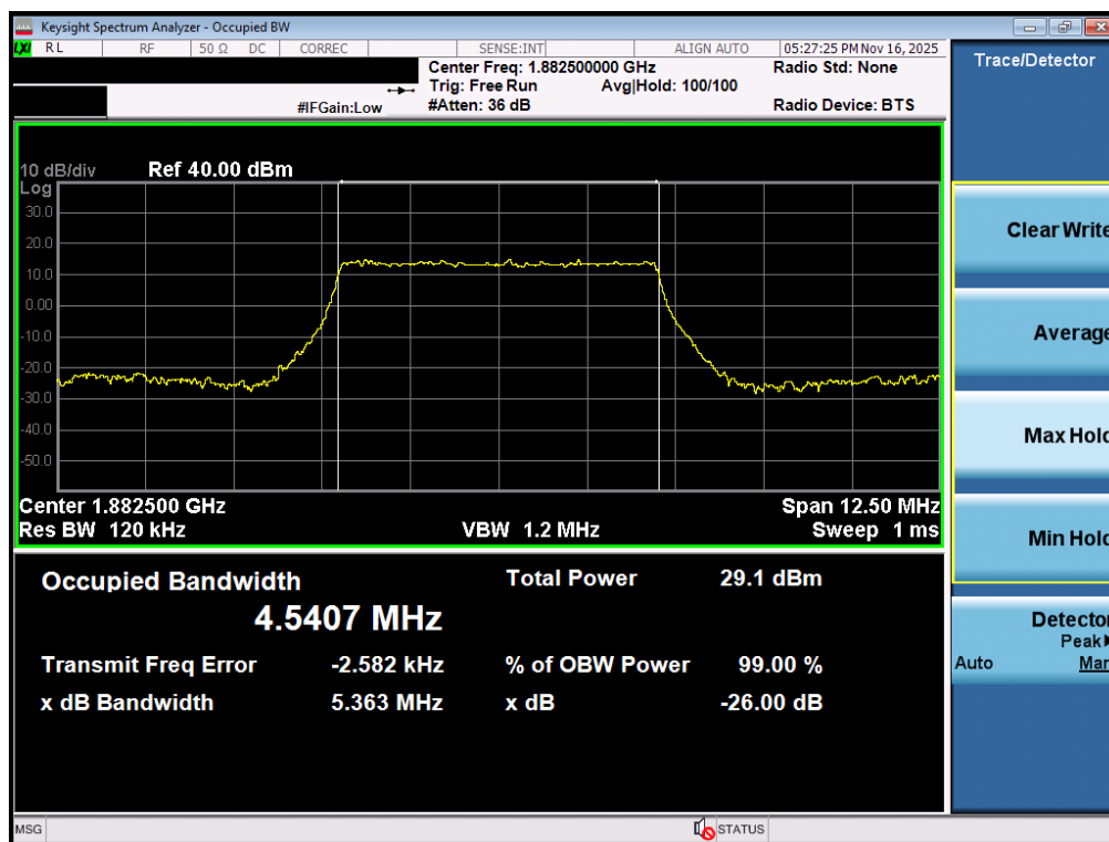
Plot 7-69. Occupied Bandwidth Plot (NR Band n25/2 - 5.0MHz CP-OFDM 16QAM - Full RB - ANT2)
