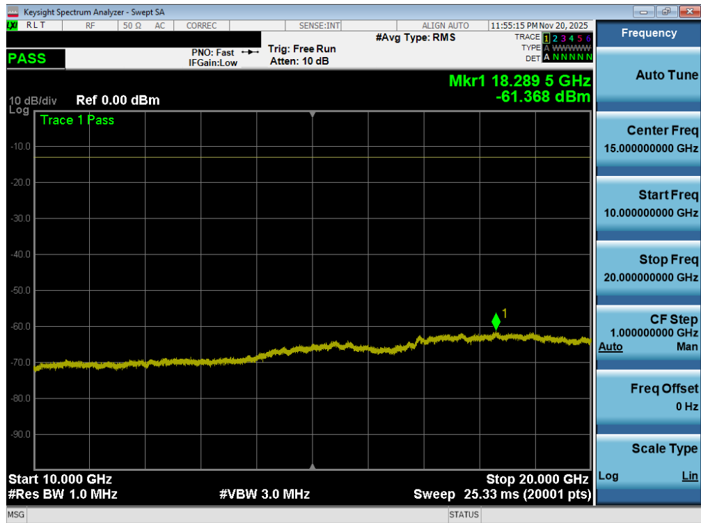
Plot 7-84. Conducted Spurious Plot (LTE Band 25/2 - 20MHz QPSK - 1RB - Low Channel - Ant2)
