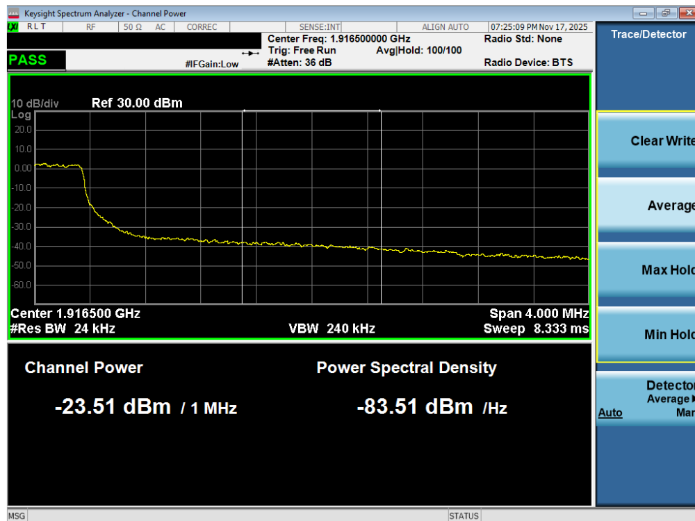
Plot 7-93. Extended Upper Band Edge Plot (LTE Band 25 - 3MHz QPSK – Full RB - Ant1)
