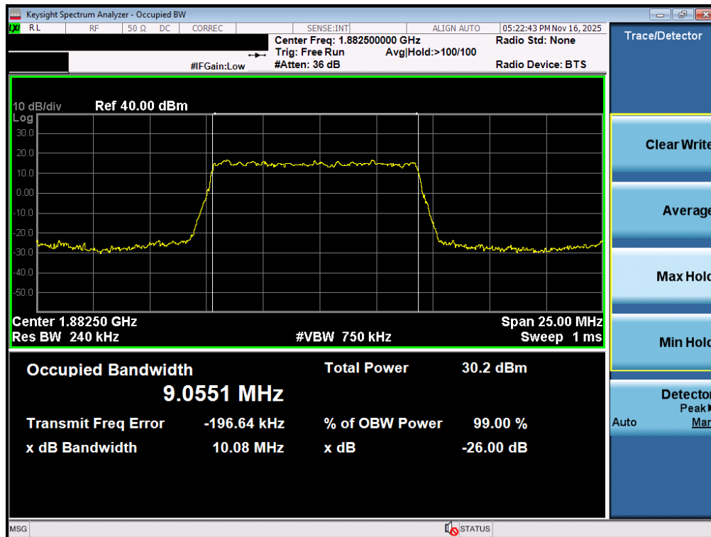
Plot 7-65. Occupied Bandwidth Plot (NR Band n25/2 - 10.0MHz CP-OFDM QPSK - Full RB - ANT2)
