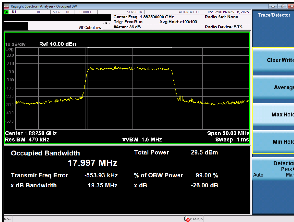
Plot 7-60. Occupied Bandwidth Plot (NR Band n25/2 - 20.0MHz CP-OFDM 16QAM - Full RB - ANT2)
