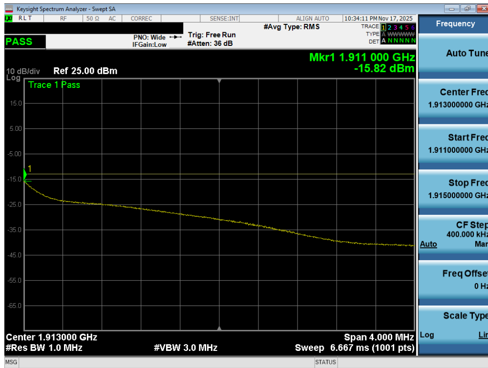
Plot 7-107. Extended Upper Band Edge Plot (WCDMA PCS – Ch. 9538 - Ant1)
