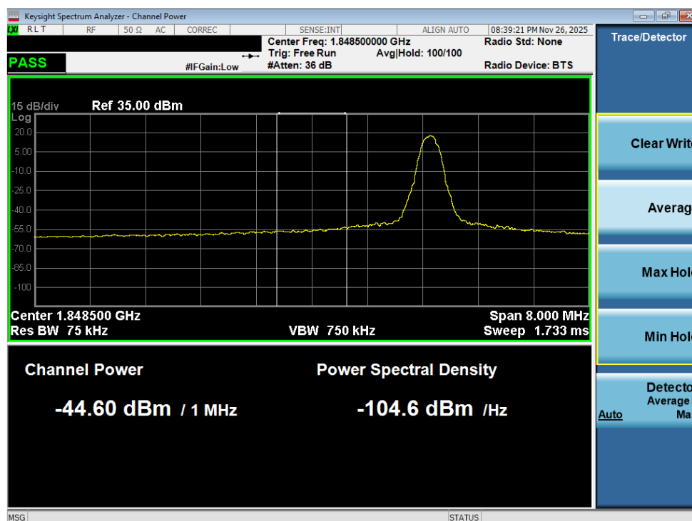
Plot 7-101. Extended Lower Band Edge Plot (GPRS PCS – Ch. 512 - Ant1)
