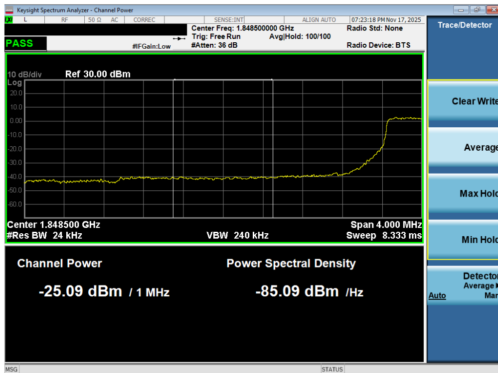
Plot 7-89. Extended Lower Band Edge Plot (LTE Band 25/2 - 3MHz QPSK – Full RB - Ant1)
