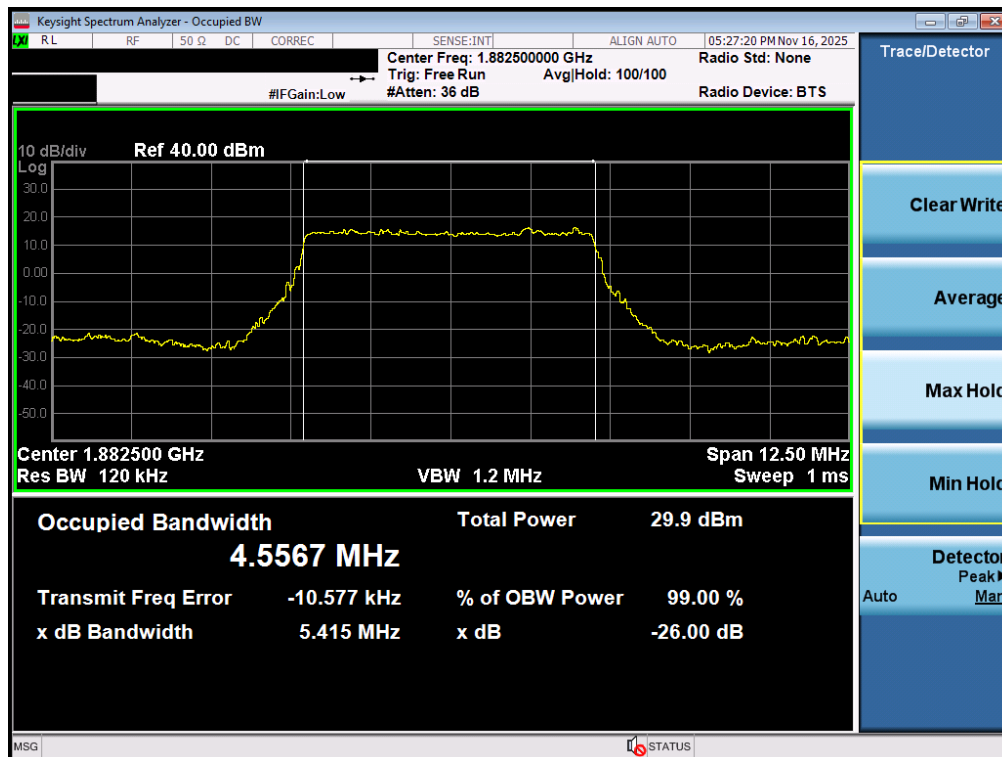
Plot 7-68. Occupied Bandwidth Plot (NR Band n25/2 - 5.0MHz CP-OFDM QPSK - Full RB - ANT2)
