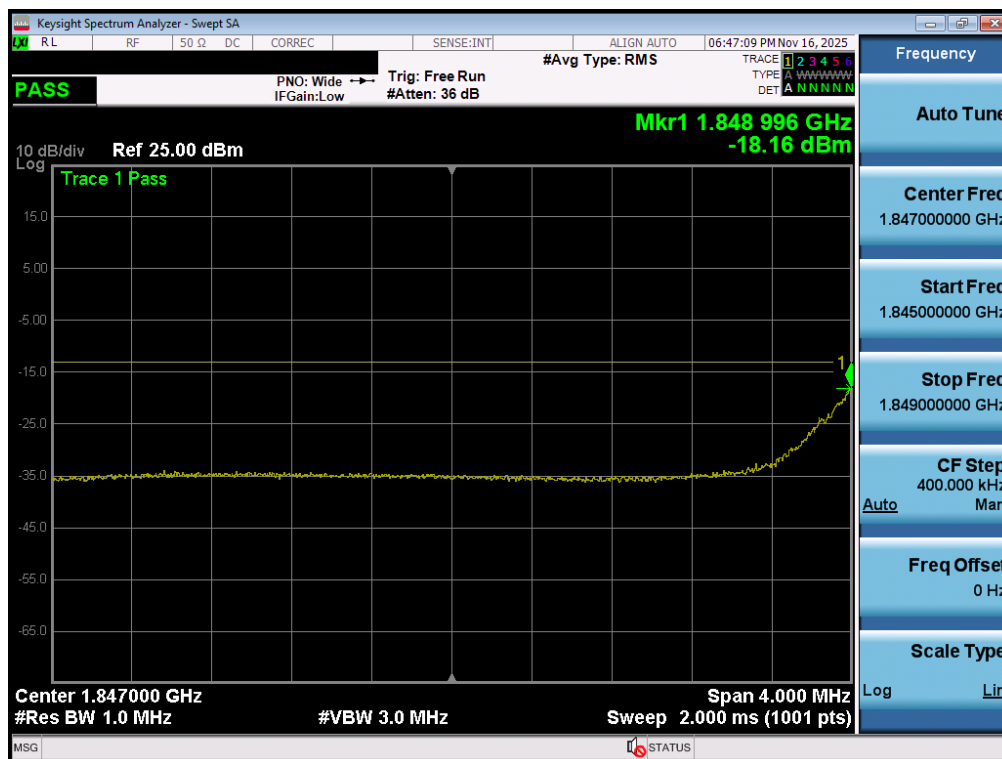
Plot 7-95. Extended Lower Band Edge Plot (NR Band n25/2 - 10MHz QPSK – Full RB - Ant1)
