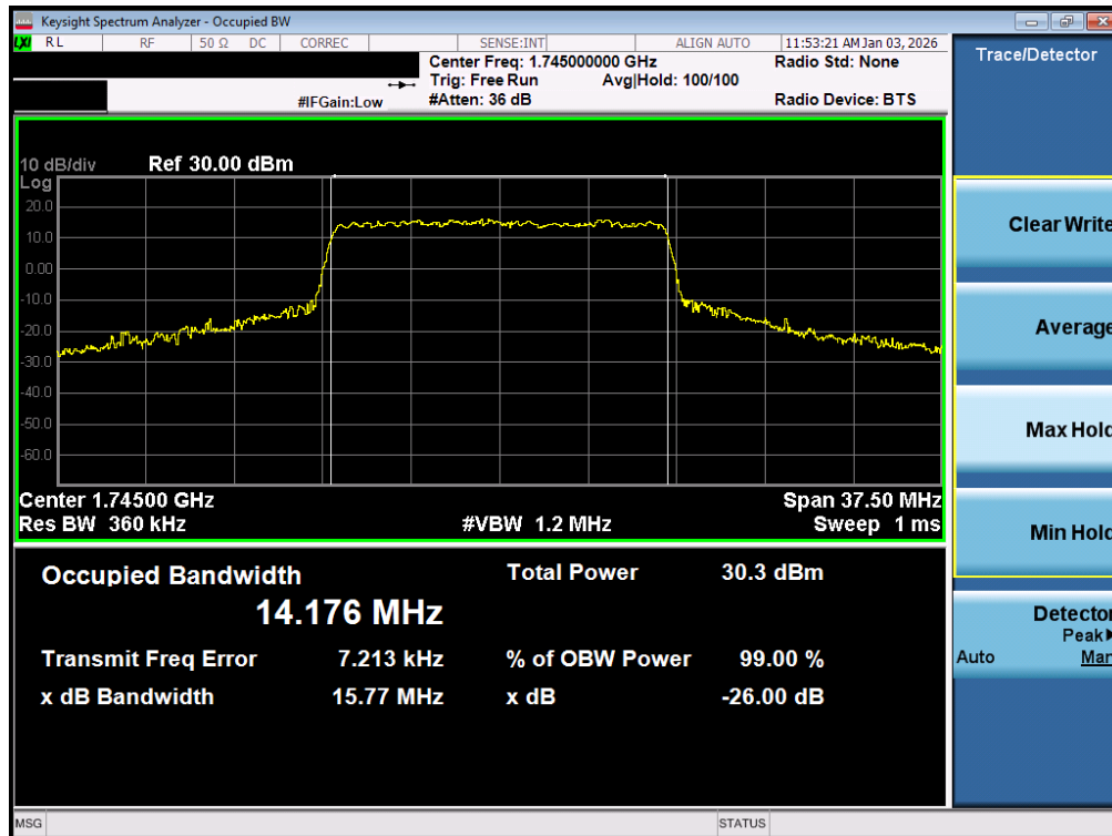
Plot 7-48. Occupied Bandwidth Plot (NR Band n66 - 15.0MHz CP-OFDM QPSK - Full RB – ANT1)
