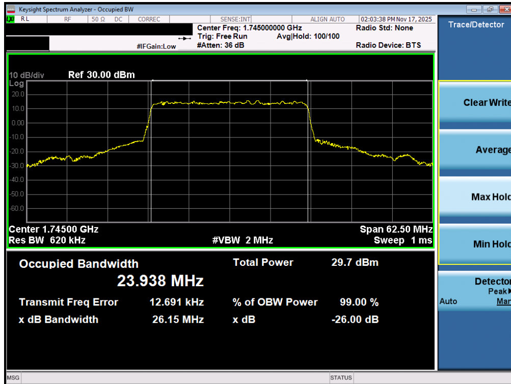
Plot 7-43. Occupied Bandwidth Plot (NR Band n66 - 25.0MHz CP-OFDM 16QAM - Full RB – ANT1)
