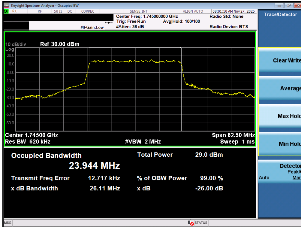
Plot 7-98. Occupied Bandwidth Plot (NR Band n66 - 25.0MHz CP-OFDM 16QAM - Full RB – ANT2)
