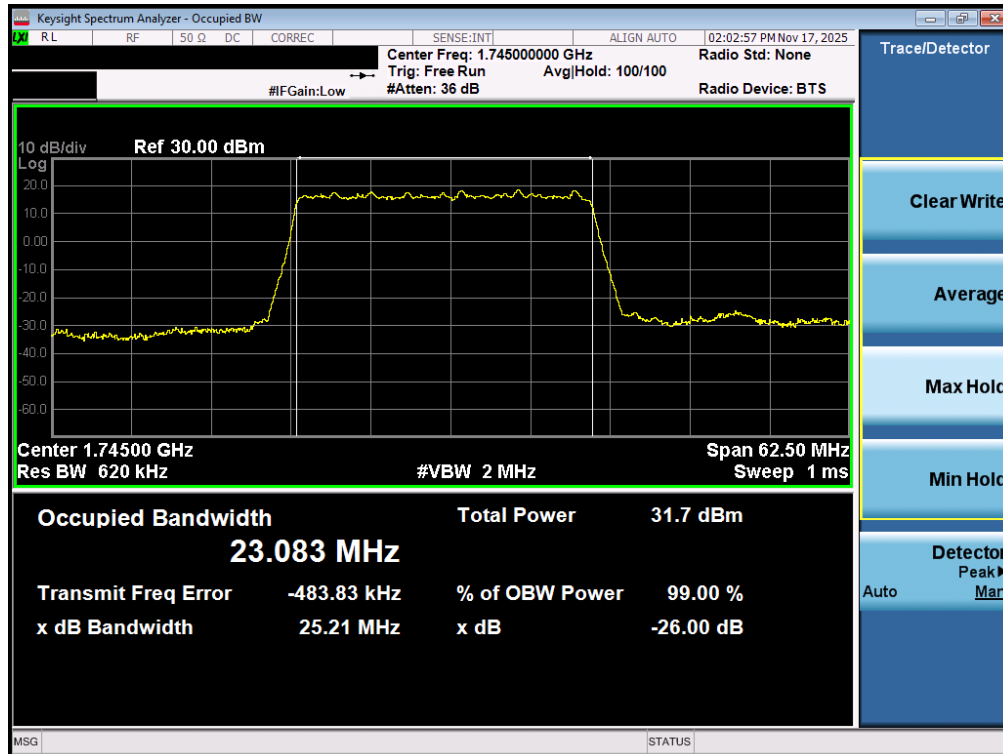
Plot 7-41. Occupied Bandwidth Plot (NR Band n66 - 25.0MHz DFT-s-OFDM BPSK - Full RB – ANT1)
