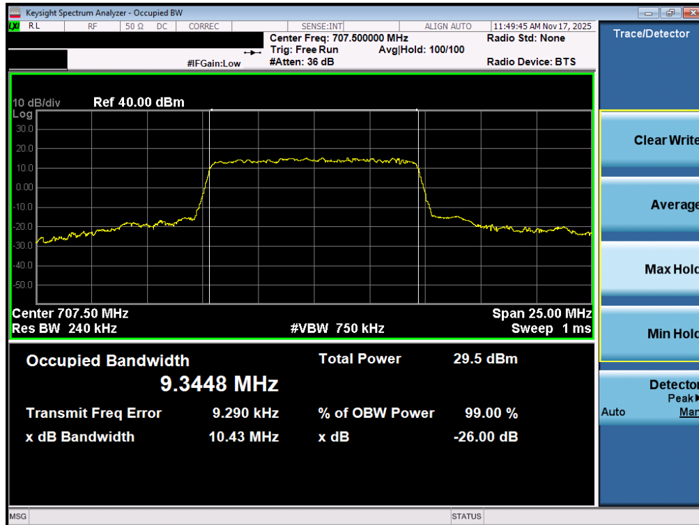
Plot 7-30. Occupied Bandwidth Plot (NR Band n12 - 10MHz CP-OFDM QPSK - Full RB – ANT1)
