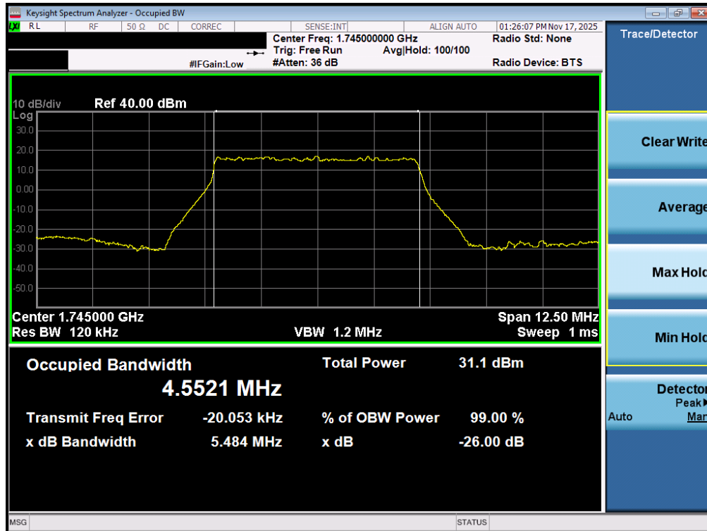
Plot 7-53. Occupied Bandwidth Plot (NR Band n66 - 5.0MHz DFT-s-OFDM BPSK - Full RB – ANT1)
