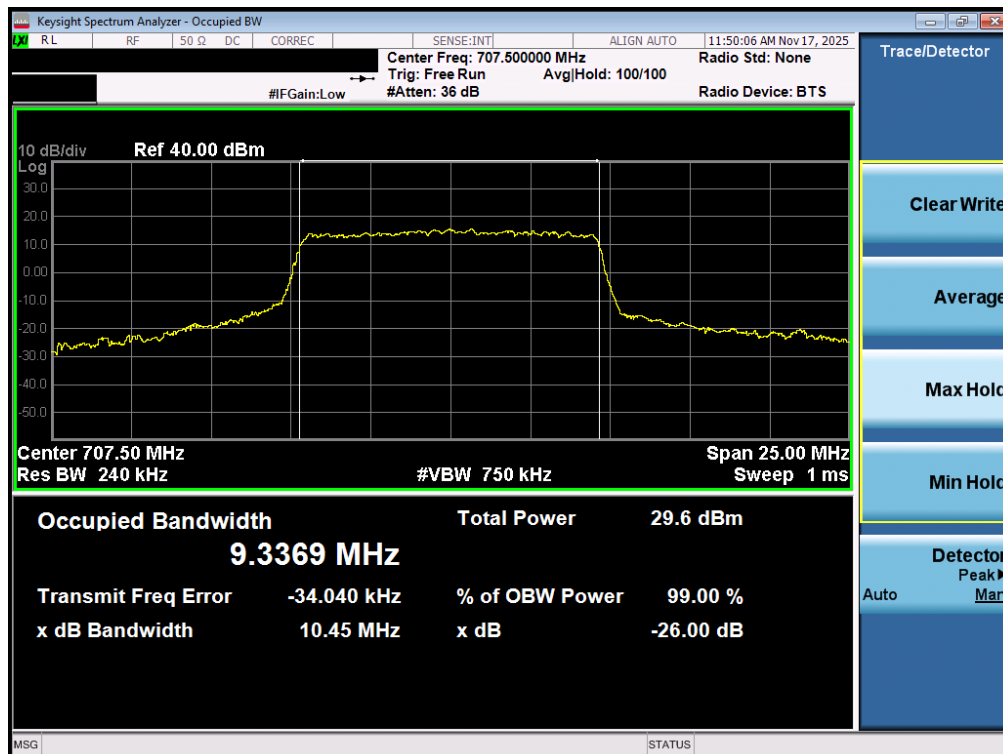
Plot 7-31. Occupied Bandwidth Plot (NR Band n12 - 10MHz CP-OFDM 16-QAM - Full RB – ANT1)
