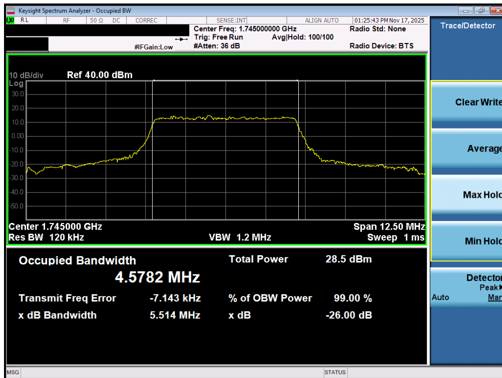
Plot 7-54. Occupied Bandwidth Plot (NR Band n66 - 5.0MHz CP-OFDM QPSK - Full RB – ANT1)
