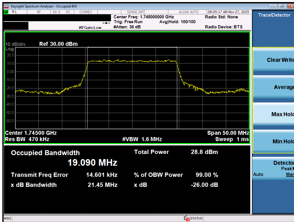
Plot 7-100. Occupied Bandwidth Plot (NR Band n66 - 20.0MHz CP-OFDM QPSK - Full RB – ANT2)
