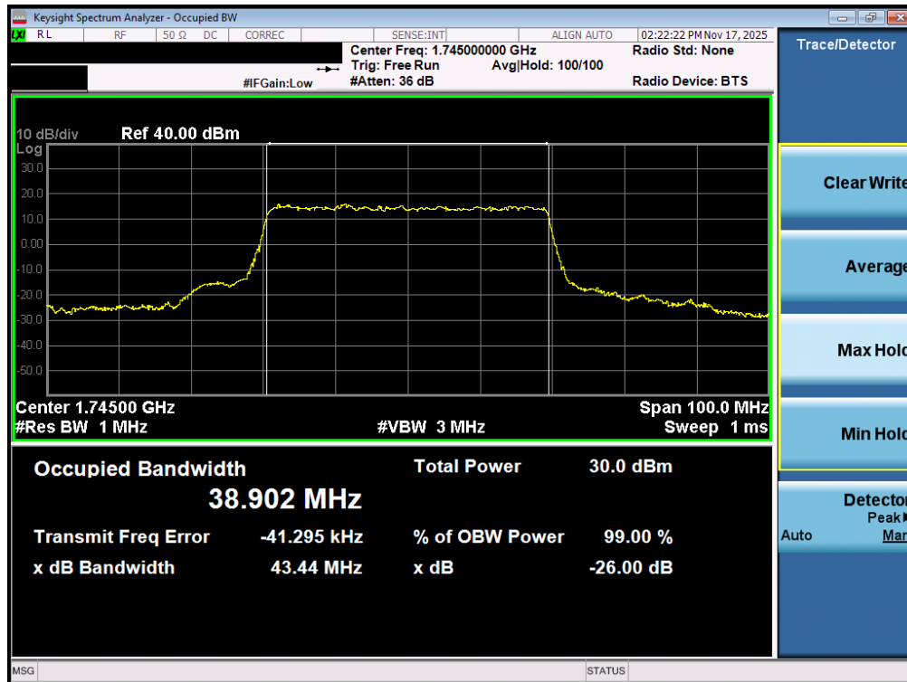
Plot 7-36. Occupied Bandwidth Plot (NR Band n66 - 40.0MHz CP-OFDM QPSK - Full RB – ANT1)
