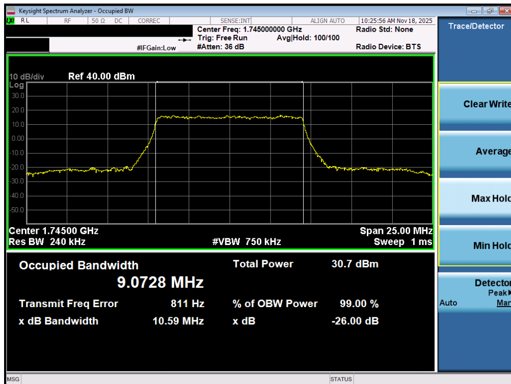
Plot 7-74. Occupied Bandwidth Plot (LTE Band 66/4 - 10MHz 16-QAM - Full RB - ANT2)
