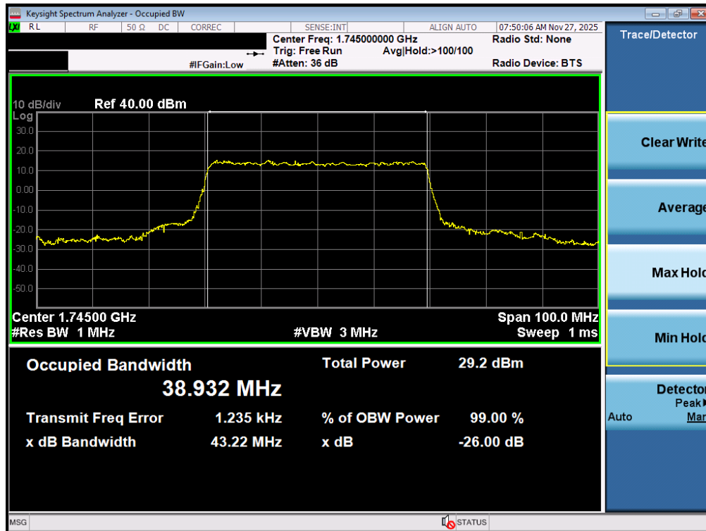
Plot 7-91. Occupied Bandwidth Plot (NR Band n66 - 40.0MHz CP-OFDM QPSK - Full RB – ANT2)
