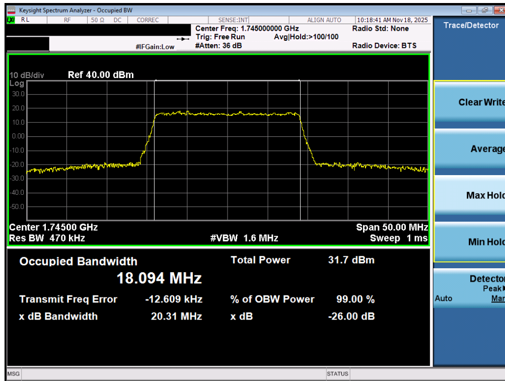
Plot 7-69. Occupied Bandwidth Plot (LTE Band 66/4 - 20MHz QPSK - Full RB - ANT2)
