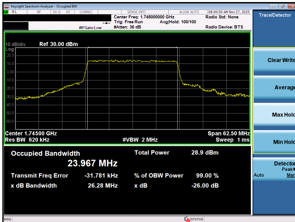
Plot 7-97. Occupied Bandwidth Plot (NR Band n66 - 25.0MHz CP-OFDM QPSK - Full RB – ANT2)
