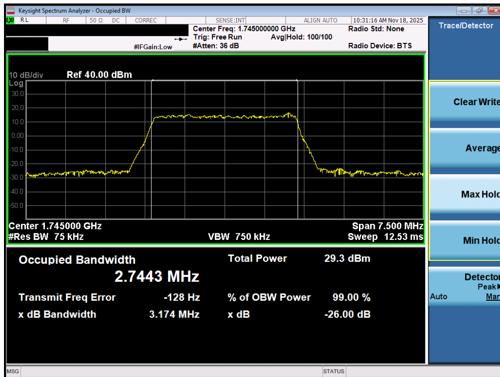
Plot 7-78. Occupied Bandwidth Plot (LTE Band 66/4 - 3MHz 16-QAM - Full RB - ANT2)
