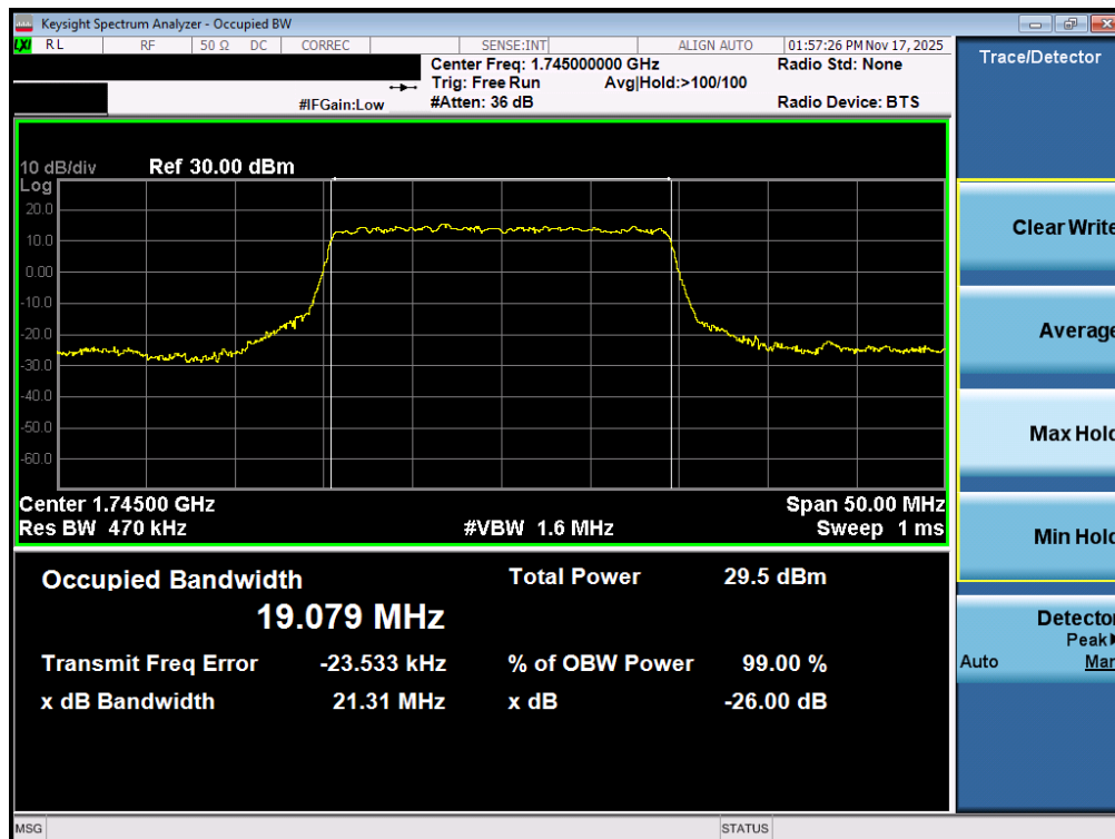
Plot 7-46. Occupied Bandwidth Plot (NR Band n66 - 20.0MHz CP-OFDM 16QAM - Full RB – ANT1)
