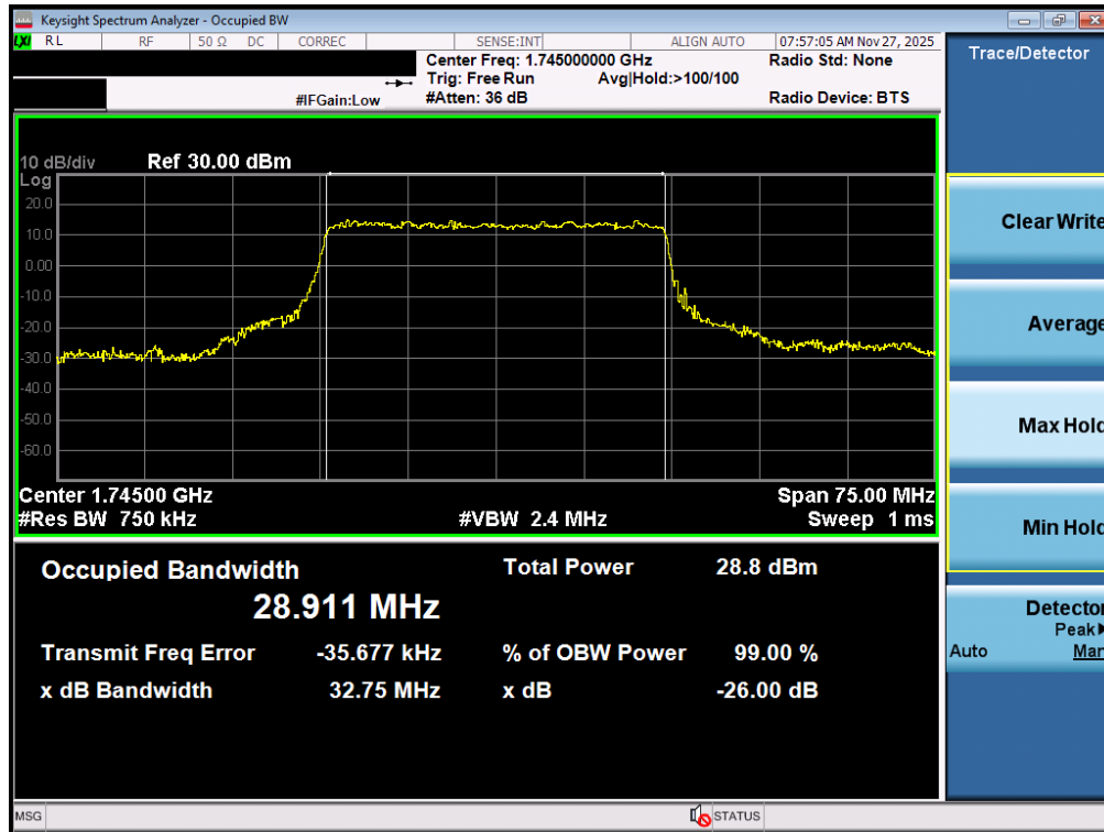
Plot 7-94. Occupied Bandwidth Plot (NR Band n66 - 30.0MHz CP-OFDM QPSK - Full RB – ANT2)
