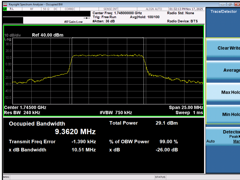
Plot 7-51. Occupied Bandwidth Plot (NR Band n66 - 10.0MHz CP-OFDM QPSK - Full RB – ANT1)
