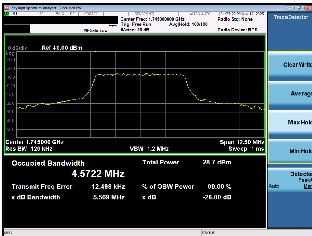
Plot 7-55. Occupied Bandwidth Plot (NR Band n66 - 5.0MHz CP-OFDM 16QAM - Full RB – ANT1)
