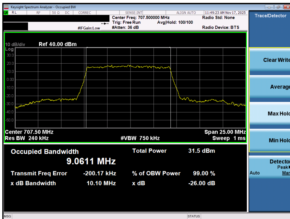
Plot 7-29. Occupied Bandwidth Plot (NR Band n12 - 10MHz DFT-s-OFDM BPSK - Full RB - ANT1)
