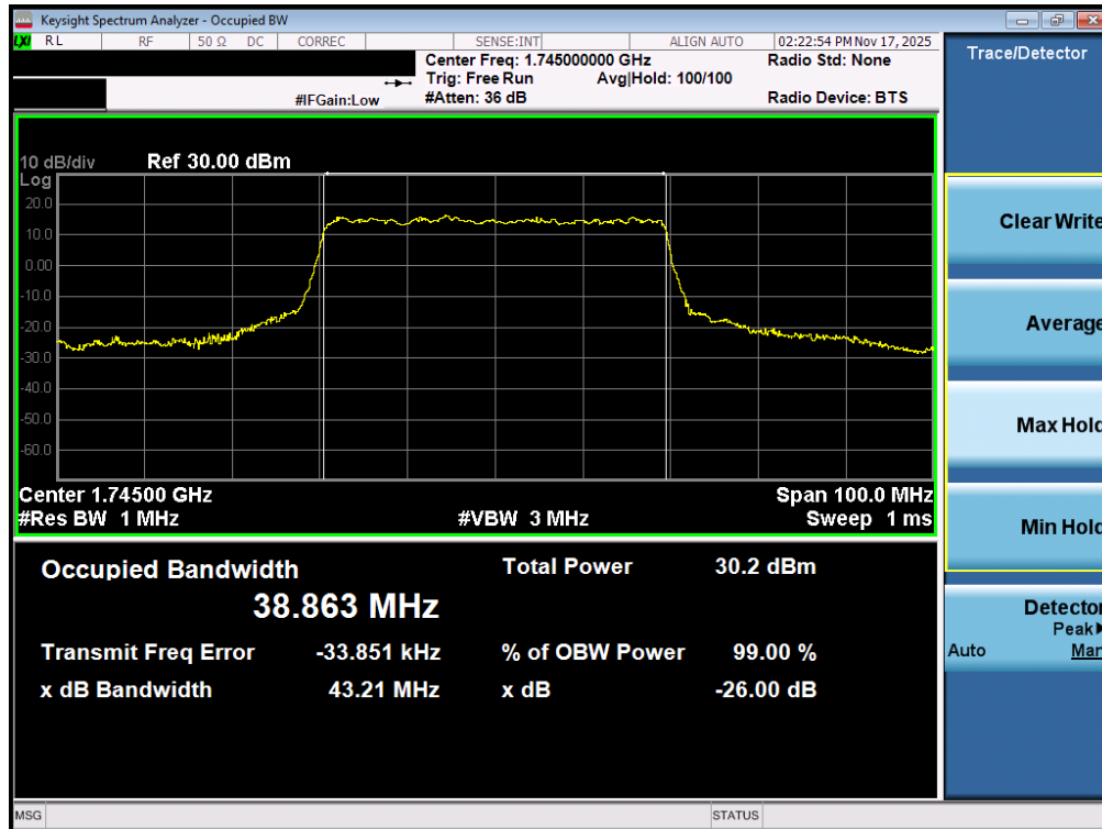
Plot 7-37. Occupied Bandwidth Plot (NR Band n66 - 40.0MHz CP-OFDM 16QAM - Full RB – ANT1)
