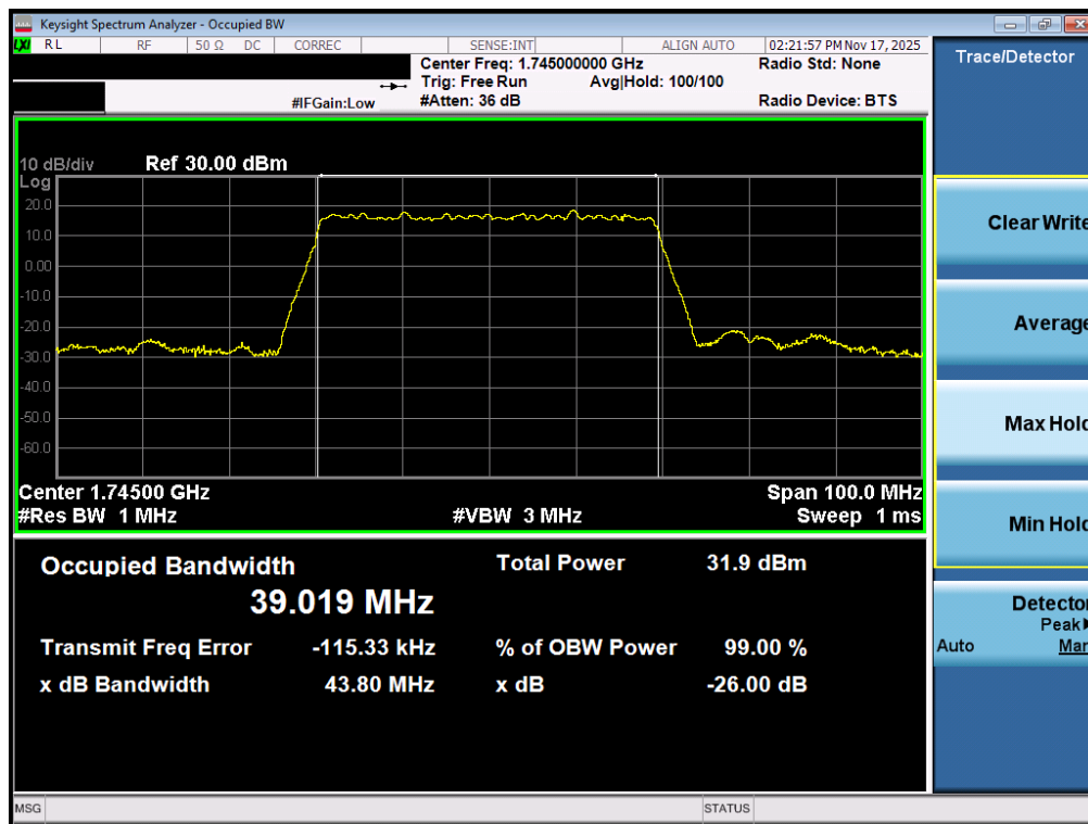
Plot 7-35. Occupied Bandwidth Plot (NR Band n66 - 40.0MHz DFT-s-OFDM BPSK - Full RB – ANT1)
