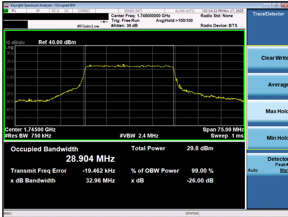
Plot 7-39. Occupied Bandwidth Plot (NR Band n66 - 30.0MHz CP-OFDM QPSK - Full RB – ANT1)
