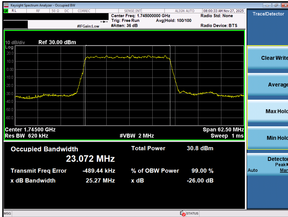
Plot 7-96. Occupied Bandwidth Plot (NR Band n66 - 25.0MHz DFT-s-OFDM BPSK - Full RB – ANT2)
