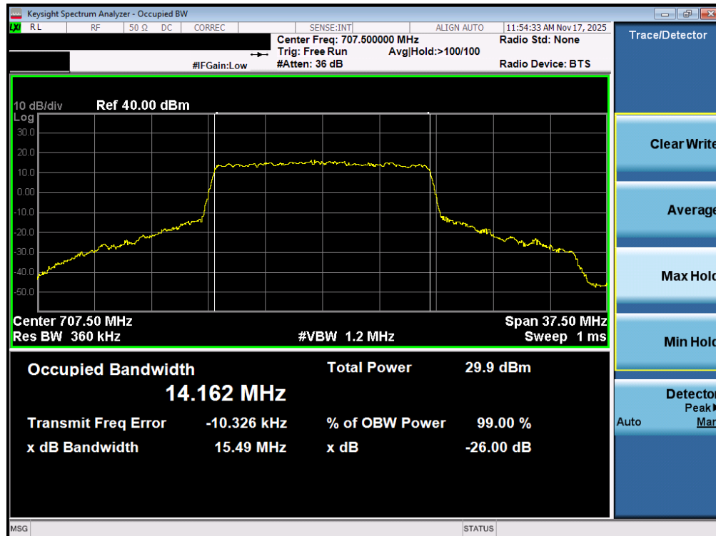
Plot 7-27. Occupied Bandwidth Plot (NR Band n12 - 15MHz QPSK - Full RB – ANT1)
