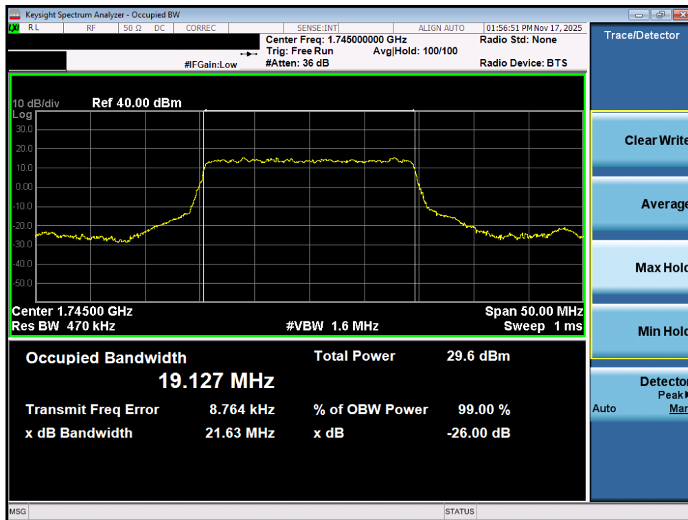
Plot 7-45. Occupied Bandwidth Plot (NR Band n66 - 20.0MHz CP-OFDM QPSK - Full RB – ANT1)
