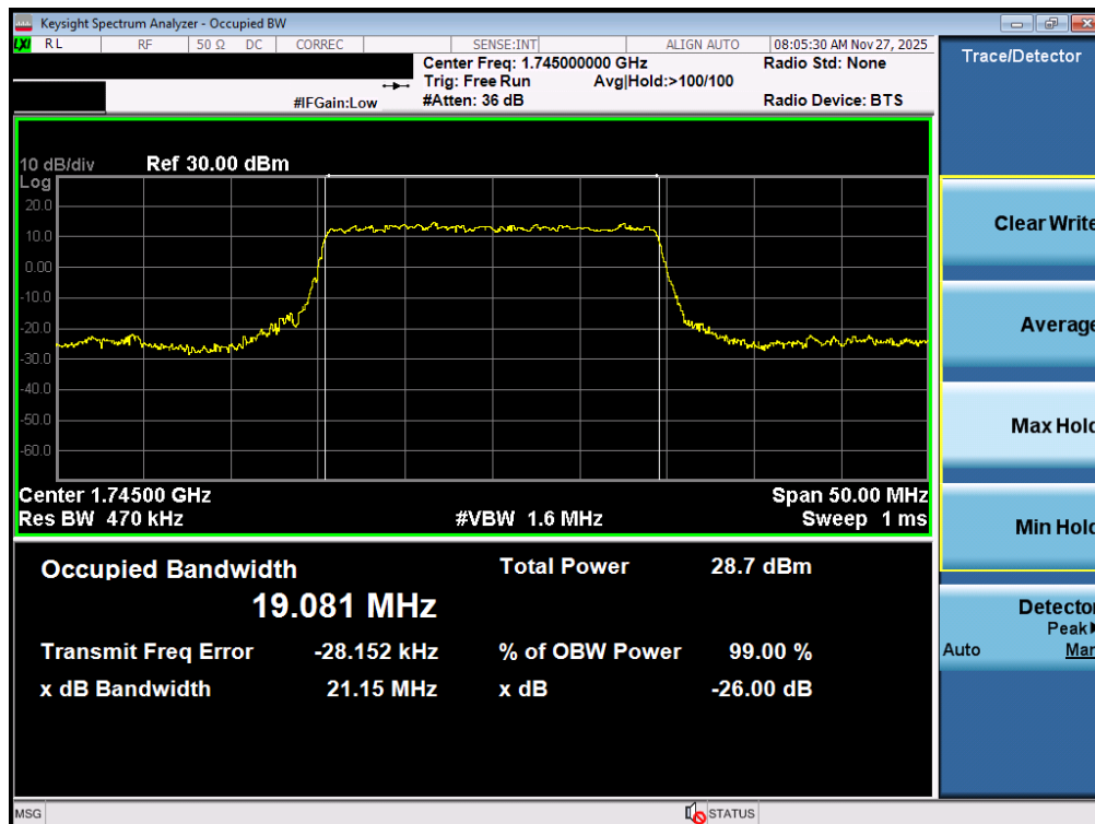
Plot 7-101. Occupied Bandwidth Plot (NR Band n66 - 20.0MHz CP-OFDM 16QAM - Full RB – ANT2)
