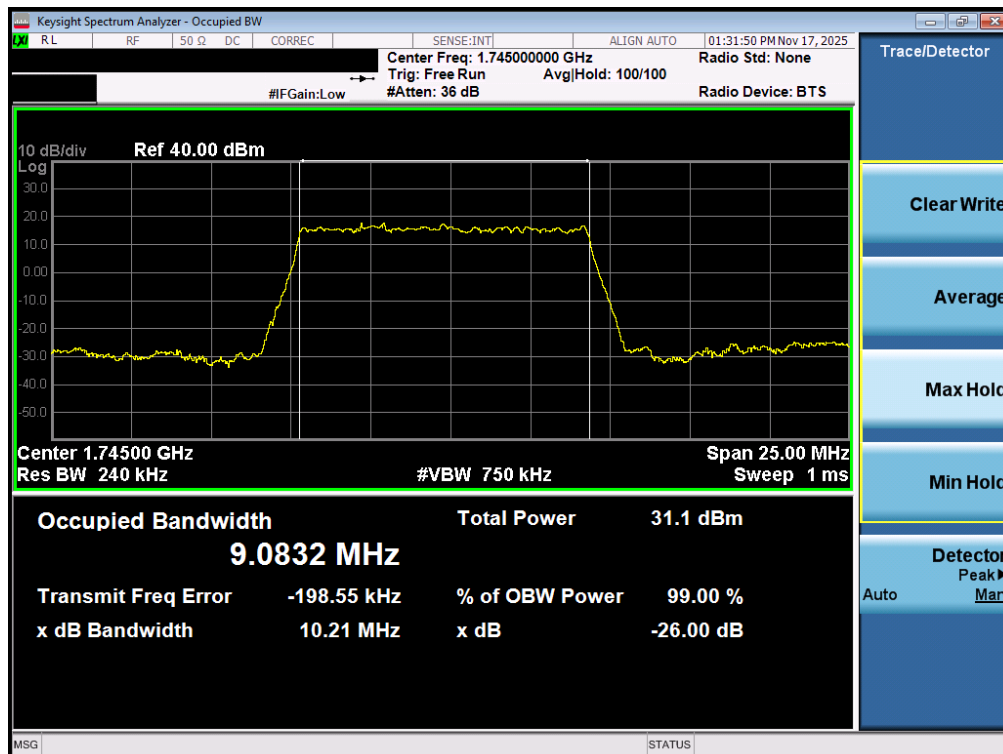
Plot 7-50. Occupied Bandwidth Plot (NR Band n66 - 10.0MHz DFT-s-OFDM BPSK - Full RB – ANT1)
