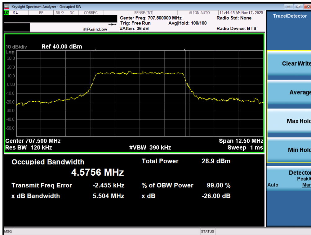
Plot 7-33. Occupied Bandwidth Plot (NR Band n12 - 5MHz CP-OFDM QPSK - Full RB – ANT1)
