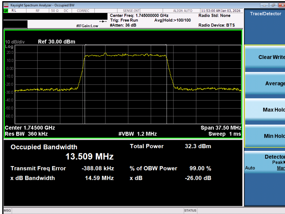
Plot 7-47. Occupied Bandwidth Plot (NR Band n66 - 15.0MHz DFT-s-OFDM BPSK - Full RB – ANT1)
