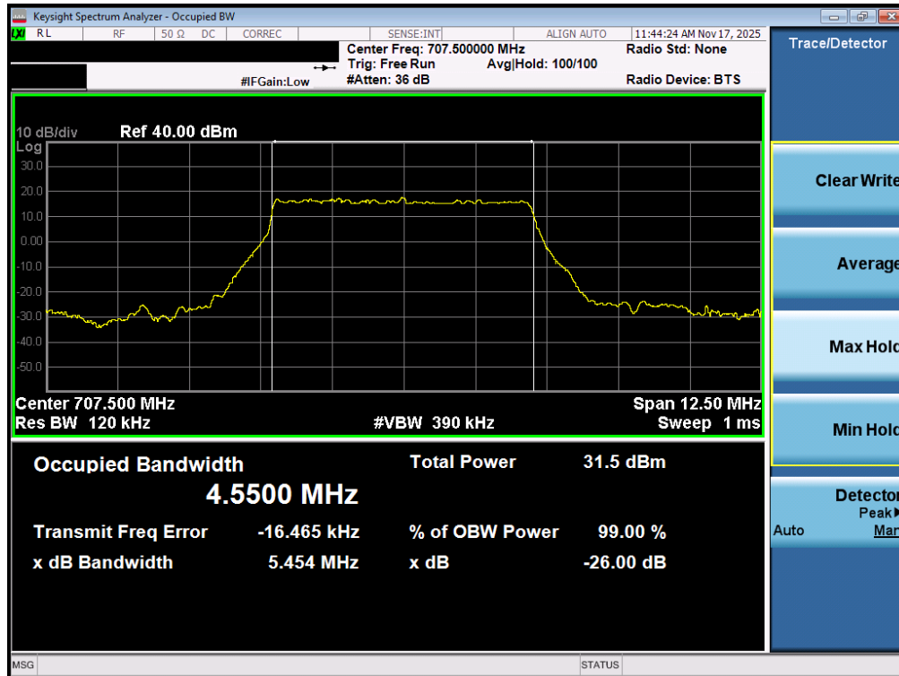
Plot 7-32. Occupied Bandwidth Plot (NR Band n12 - 5MHz DFT-s-OFDM BPSK - Full RB – ANT1)
