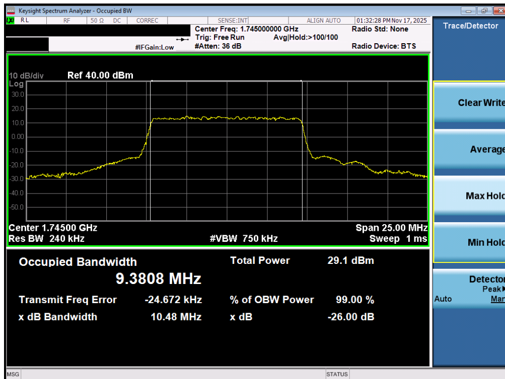
Plot 7-52. Occupied Bandwidth Plot (NR Band n66 - 10.0MHz CP-OFDM 16QAM - Full RB – ANT1)
