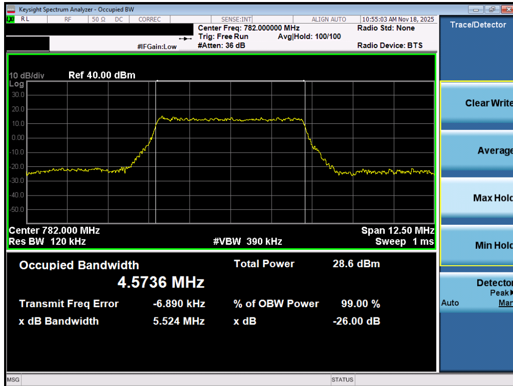
Plot 7-67. Occupied Bandwidth Plot (LTE Band 13 - 5MHz QPSK - Full RB – ANT2)
