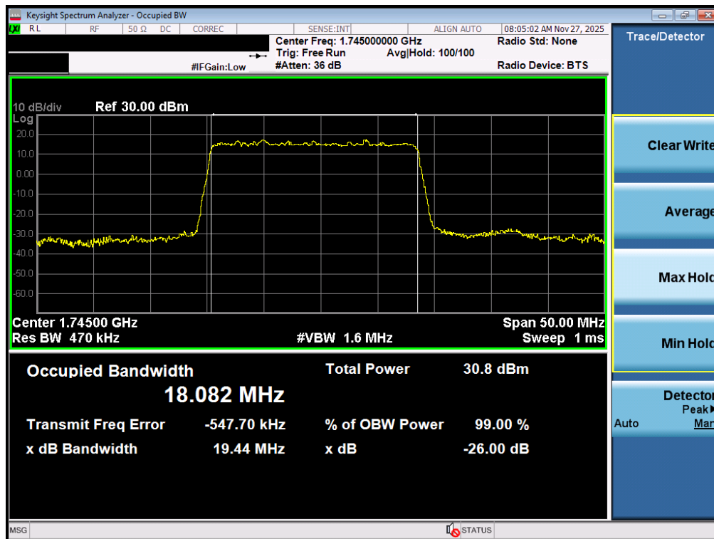
Plot 7-99. Occupied Bandwidth Plot (NR Band n66 - 20.0MHz DFT-s-OFDM BPSK - Full RB – ANT2)
