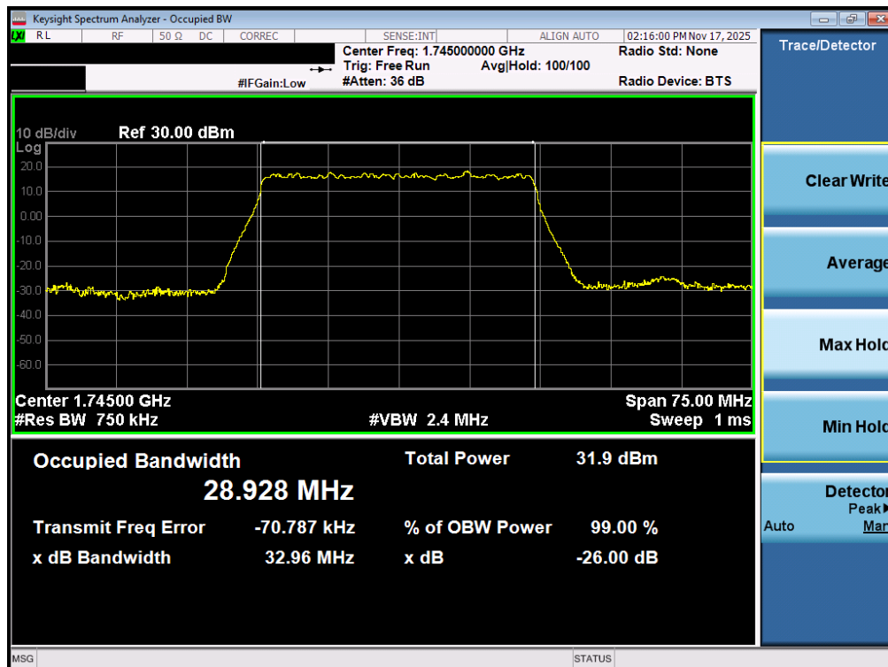
Plot 7-38. Occupied Bandwidth Plot (NR Band n66 - 30.0MHz DFT-s-OFDM BPSK - Full RB – ANT1)
