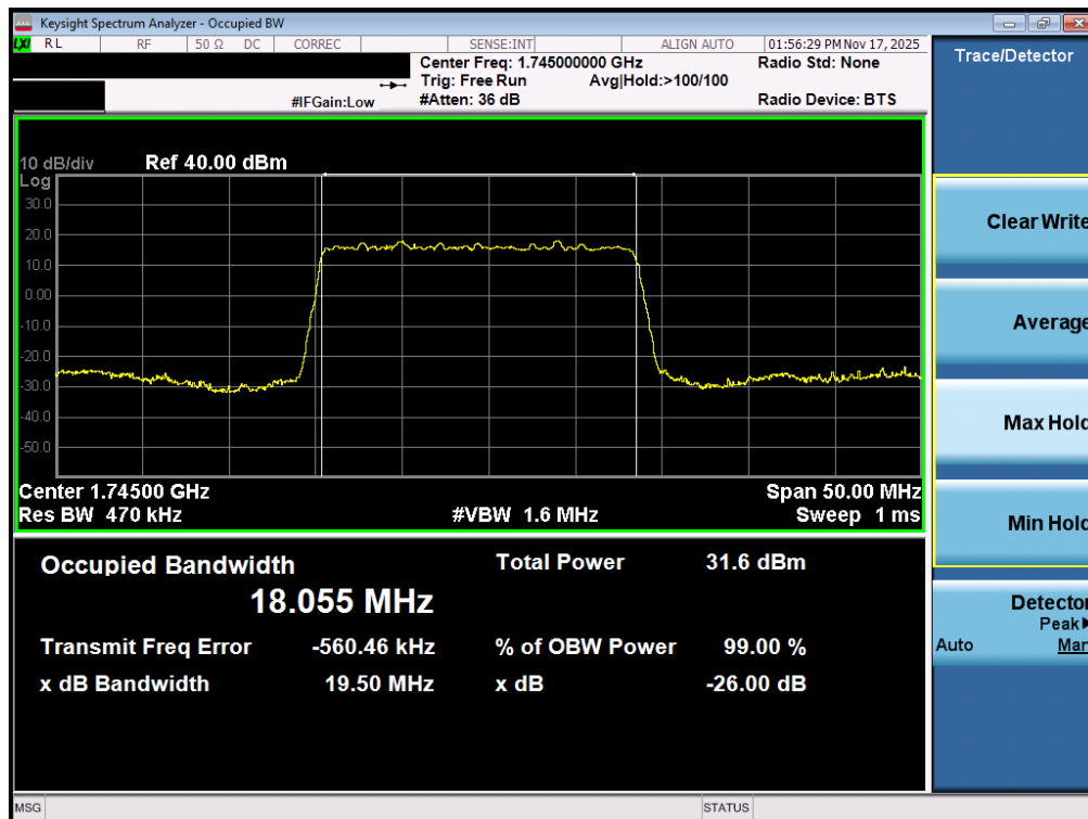
Plot 7-44. Occupied Bandwidth Plot (NR Band n66 - 20.0MHz DFT-s-OFDM BPSK - Full RB – ANT1)
