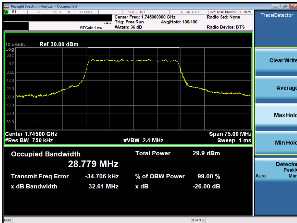
Plot 7-40. Occupied Bandwidth Plot (NR Band n66 - 30.0MHz CP-OFDM 16QAM - Full RB – ANT1)
