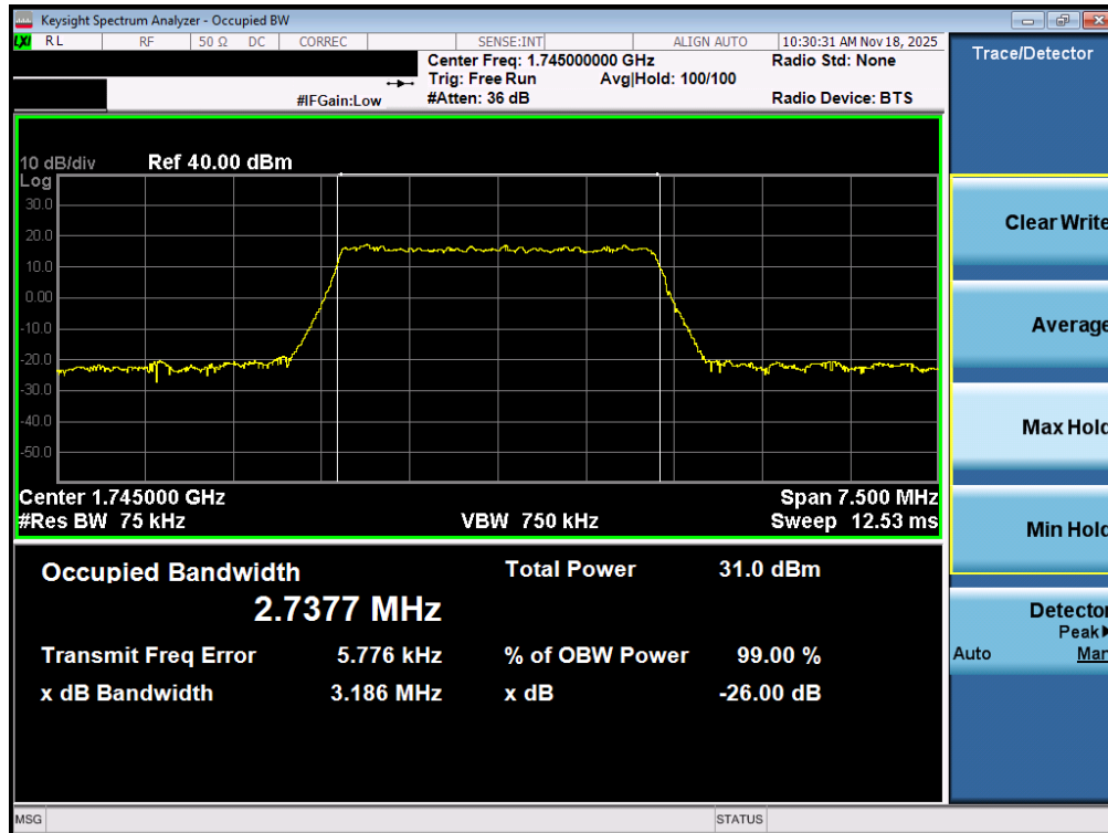
Plot 7-77. Occupied Bandwidth Plot (LTE Band 66/4 - 3MHz QPSK - Full RB - ANT2)
