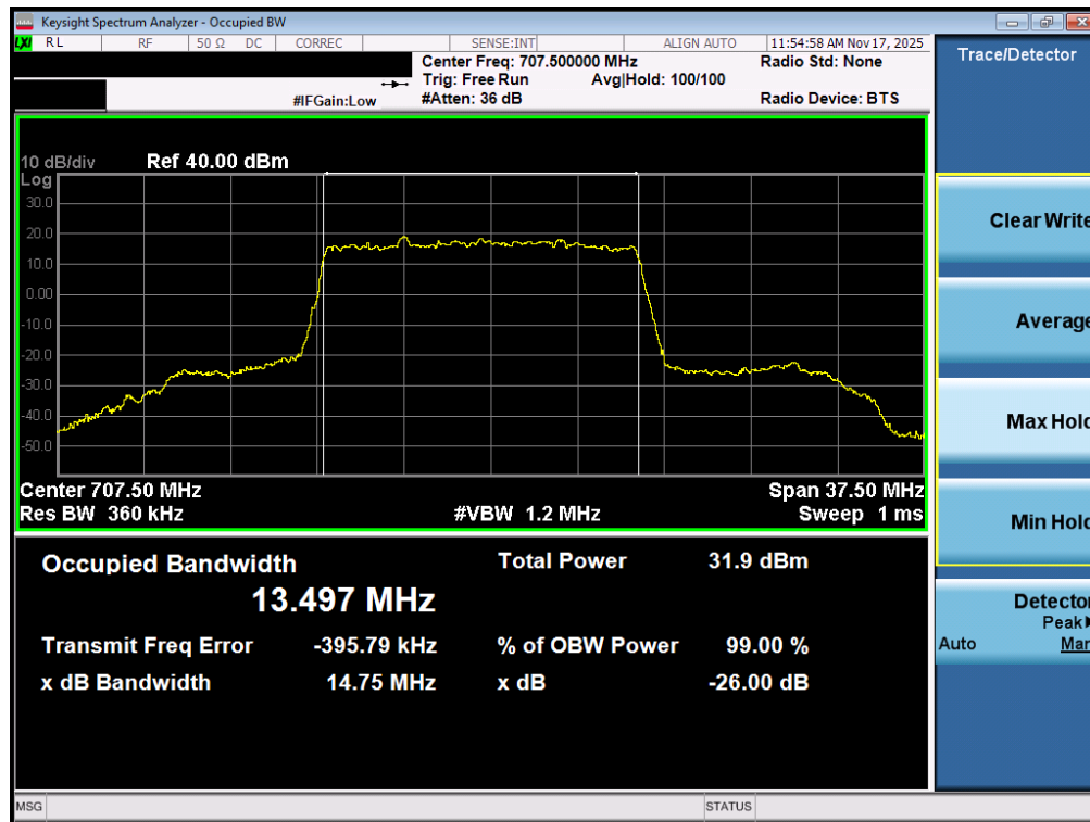
Plot 7-26. Occupied Bandwidth Plot (NR Band n12 - 15MHz DFT-s-OFDM BPSK - Full RB – ANT1)
