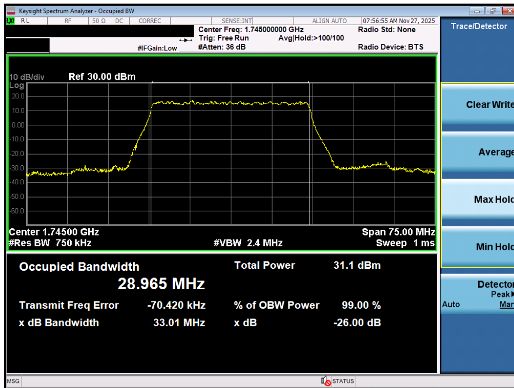
Plot 7-93. Occupied Bandwidth Plot (NR Band n66 - 30.0MHz DFT-s-OFDM BPSK - Full RB - ANT2)
