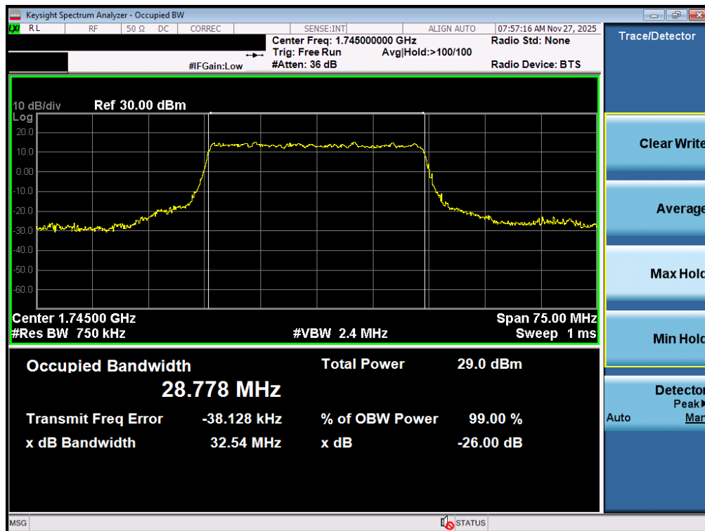
Plot 7-95. Occupied Bandwidth Plot (NR Band n66 - 30.0MHz CP-OFDM 16QAM - Full RB – ANT2)
