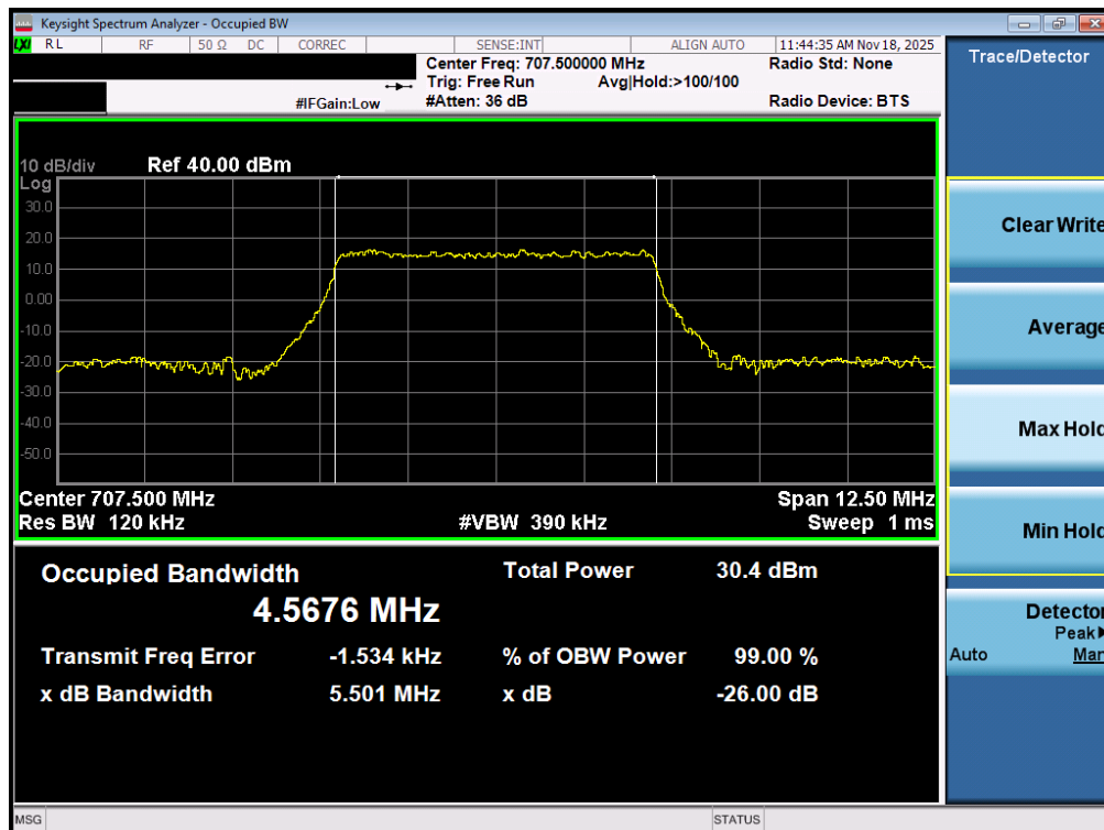
Plot 7-60. Occupied Bandwidth Plot (LTE Band 12/17 - 5MHz 16-QAM - Full RB – ANT2)
