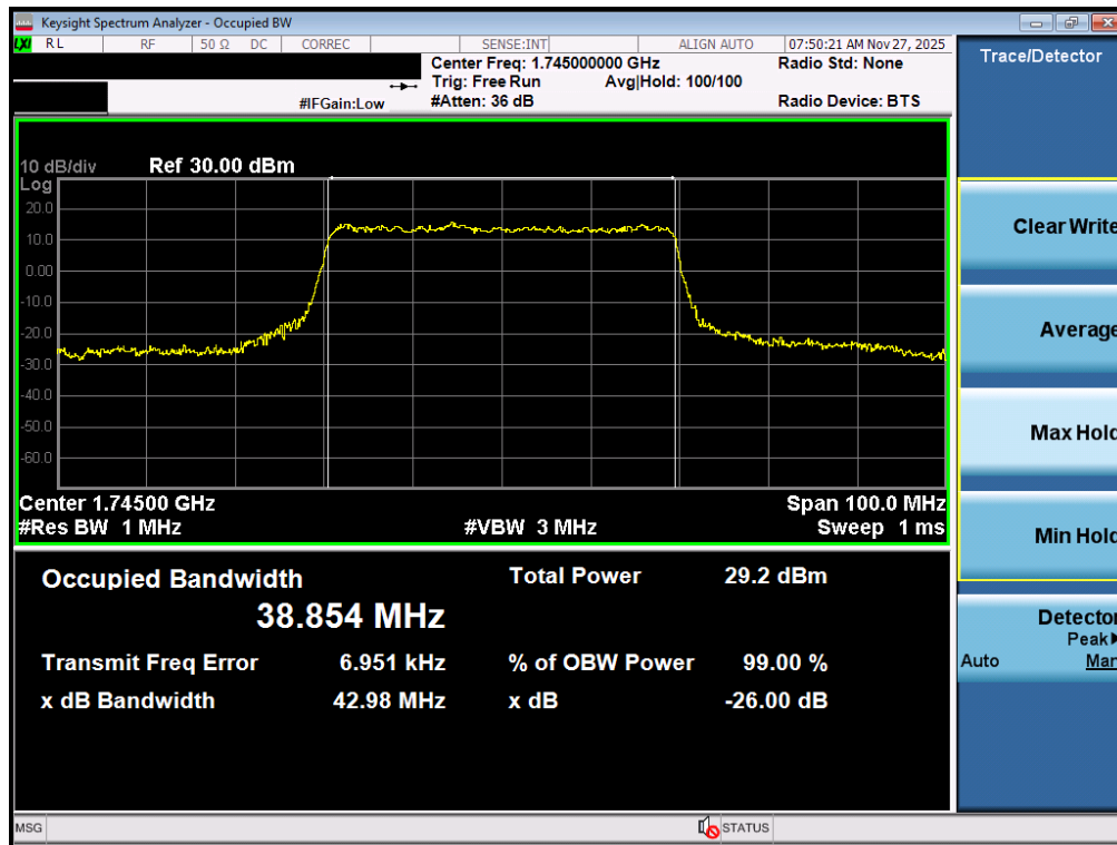
Plot 7-92. Occupied Bandwidth Plot (NR Band n66 - 40.0MHz CP-OFDM 16QAM - Full RB - ANT2)
