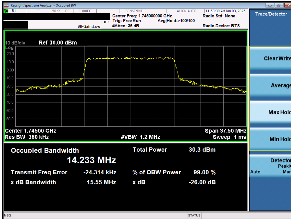
Plot 7-49. Occupied Bandwidth Plot (NR Band n66 - 15.0MHz CP-OFDM 16QAM - Full RB – ANT1)
