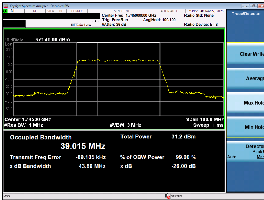
Plot 7-90. Occupied Bandwidth Plot (NR Band n66 - 40.0MHz DFT-s-OFDM BPSK - Full RB – ANT2)
