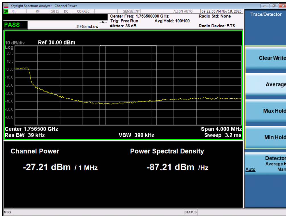
Plot 7-160. Upper Extended Band Edge Plot (LTE Band 4 – 5MHz QPSK – Full RB - ANT1)
