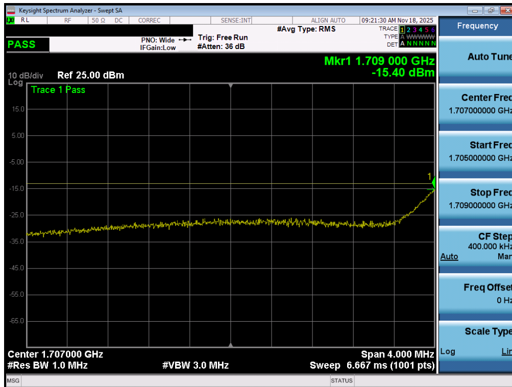
Plot 7-158. Lower Extended Band Edge Plot (LTE Band 66/4 – 5MHz QPSK – Full RB - ANT1)
