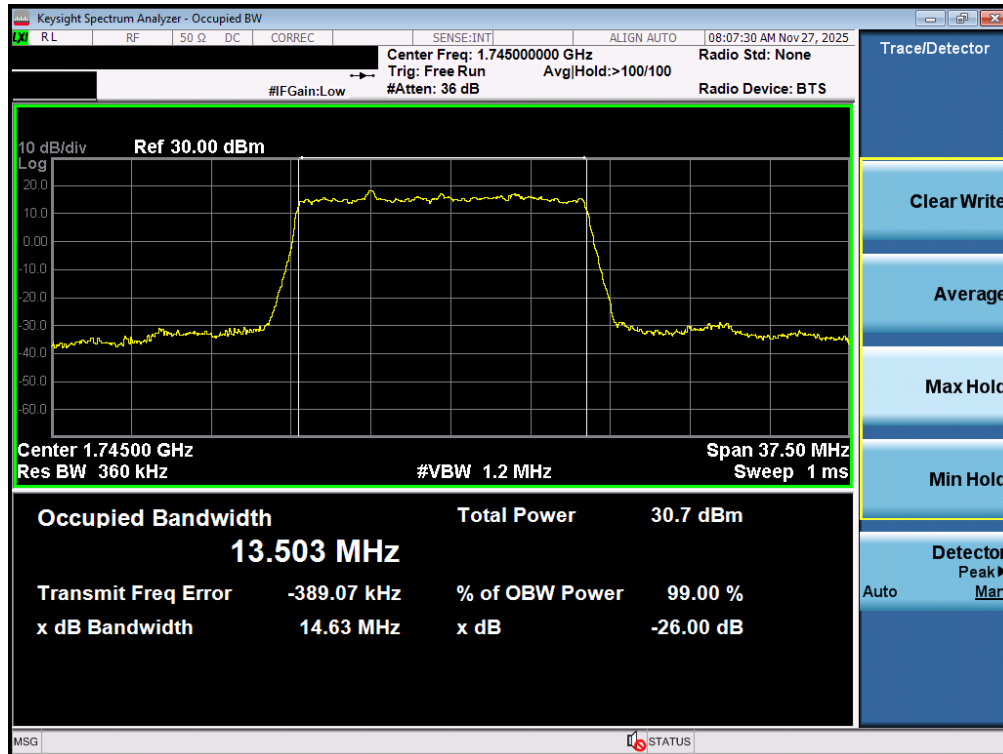
Plot 7-102. Occupied Bandwidth Plot (NR Band n66 - 15.0MHz DFT-s-OFDM BPSK - Full RB – ANT2)
