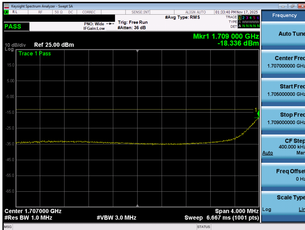
Plot 7-166. Lower Extended Band Edge Plot (NR Band n66 – 10.0MHz - Full RB - ANT1)
