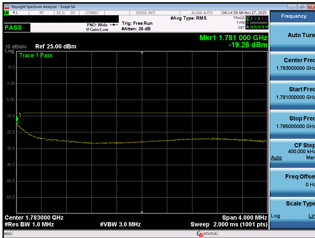
Plot 7-190. Upper Extended Band Edge Plot (NR Band n66 – 10.0MHz - Full RB - ANT2)
