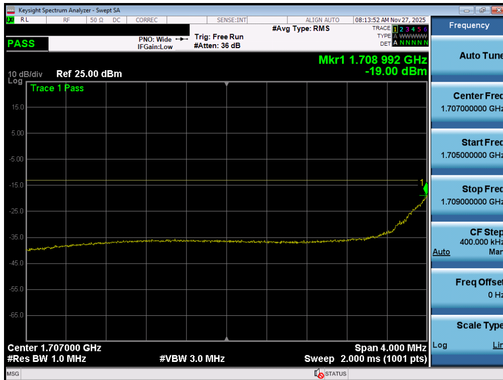
Plot 7-188. Lower Extended Band Edge Plot (NR Band n66 – 10.0MHz - Full RB - ANT2)
