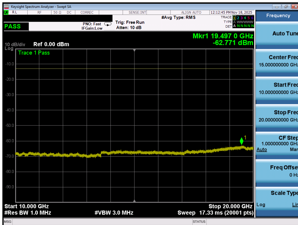
Plot 7-113. Conducted Spurious Plot (WCDMA-AWS - 5MHz QPSK - 1 RB – Low Channel)
