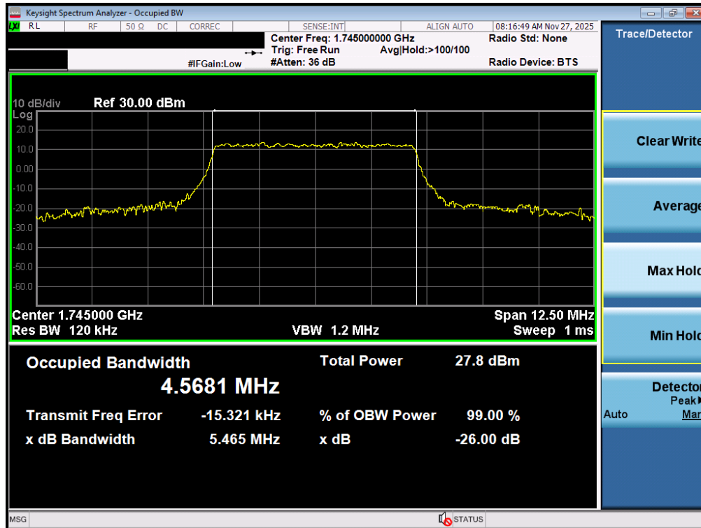
Plot 7-110. Occupied Bandwidth Plot (NR Band n66 - 5.0MHz CP-OFDM 16QAM - Full RB – ANT2)
