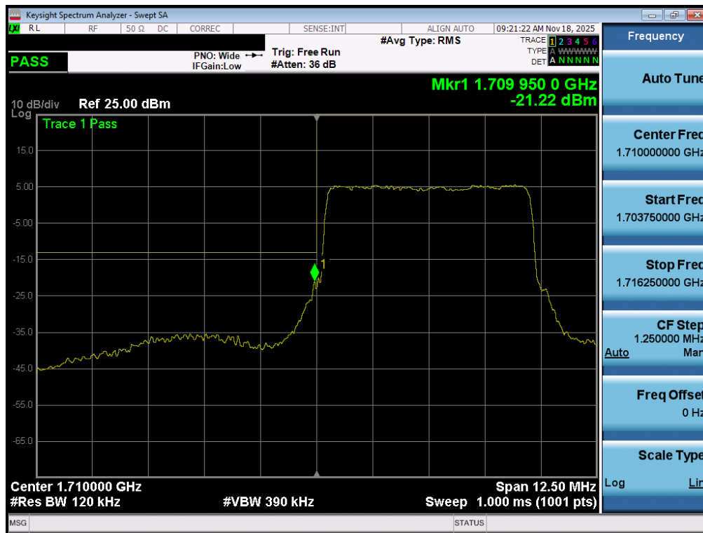
Plot 7-157. Lower Band Edge Plot (LTE Band 66/4 – 5MHz QPSK – Full RB - ANT1)
