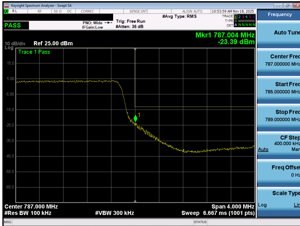
Plot 7-177. Upper Band Edge Plot (LTE Band 13 - 5MHz QPSK – Full RB - ANT2)
