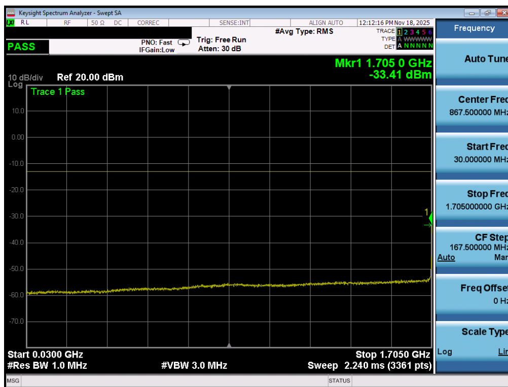
Plot 7-111. Conducted Spurious Plot (WCDMA-AWS - 5MHz QPSK - 1 RB – Low Channel)
