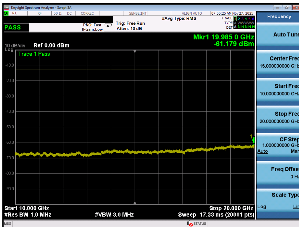
Plot 7-146. Conducted Spurious Plot (NR Band n66 - 40.0MHz - 1 RB - High Channel - ANT2)
