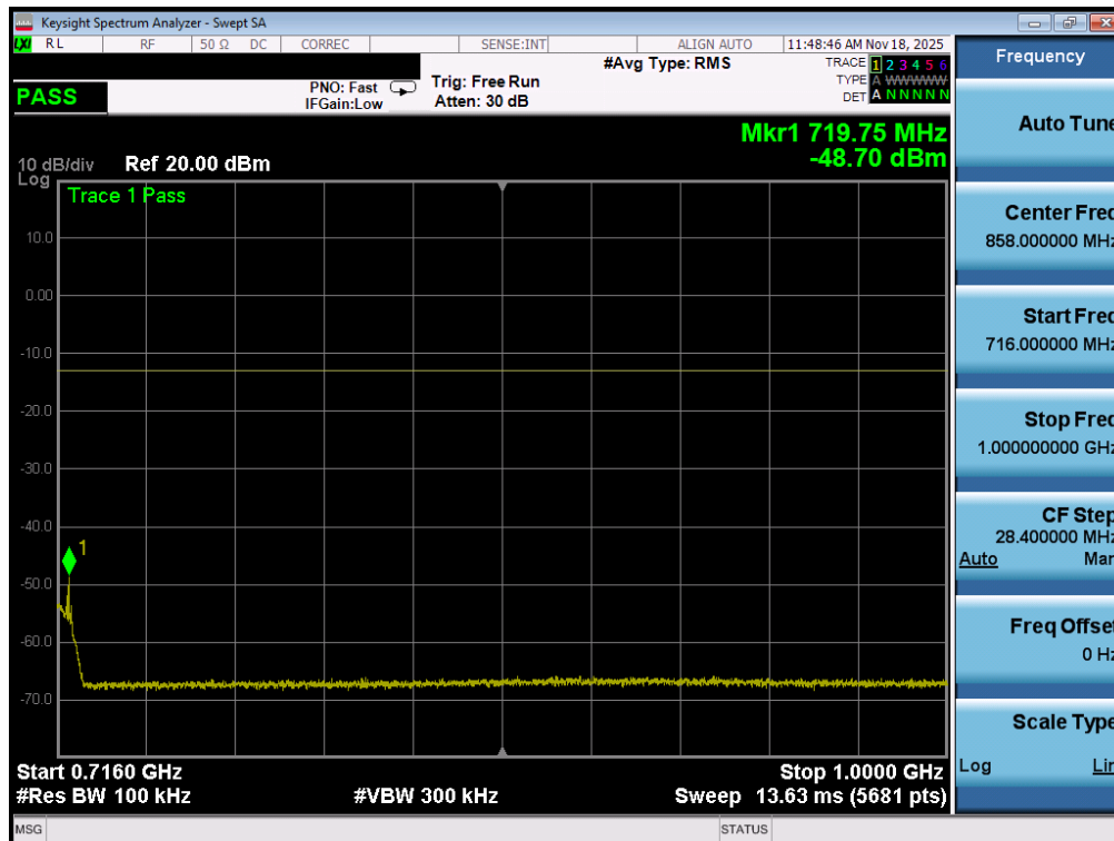
Plot 7-133. Conducted Spurious Plot (LTE Band 12/17 - 10MHz QPSK - 1 RB - Mid Channel - ANT2)
