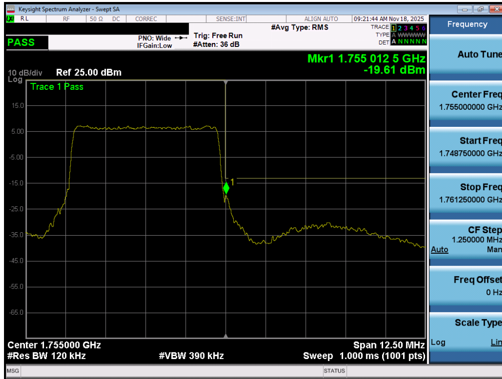
Plot 7-159. Upper Band Edge Plot (LTE Band 4 – 5MHz QPSK – Full RB - ANT1)
