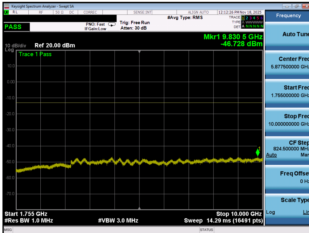
Plot 7-112. Conducted Spurious Plot (WCDMA-AWS - 5MHz QPSK - 1 RB – Low Channel)
