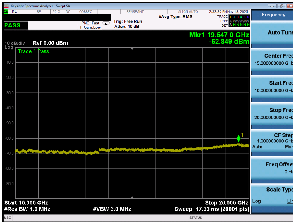
Plot 7-131. Conducted Spurious Plot (WCDMA-AWS - 5MHz QPSK - 1 RB - Low Channel - ANT2)
