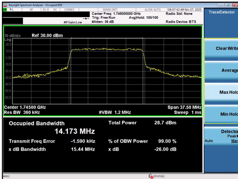
Plot 7-103. Occupied Bandwidth Plot (NR Band n66 - 15.0MHz CP-OFDM QPSK - Full RB – ANT2)
