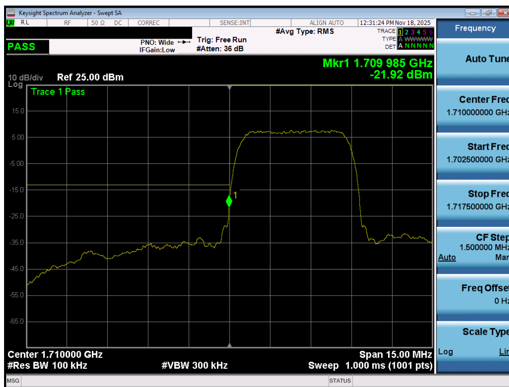
Plot 7-169. Lower Band Edge Plot (WCDMA AWS – Ch. 1312 – ANT2)
