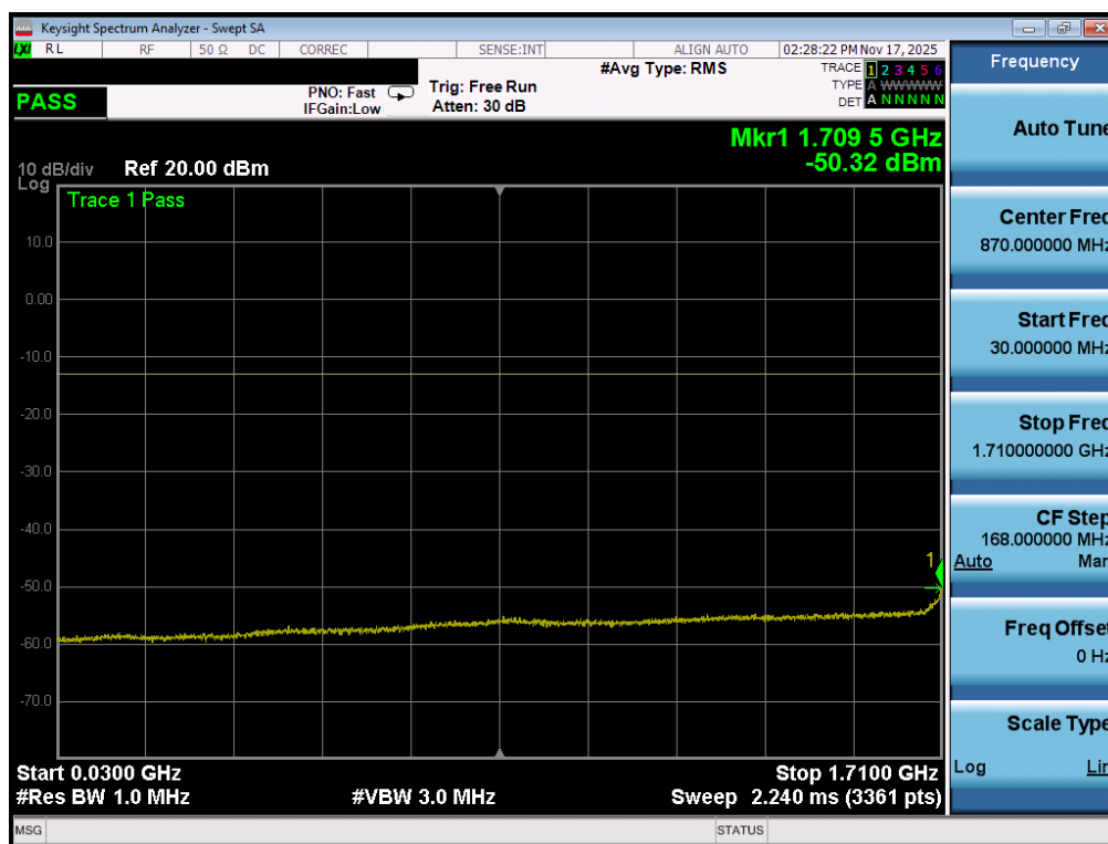
Plot 7-126. Conducted Spurious Plot (NR Band n66 - 40.0MHz - 1 RB - High Channel - ANT1)
