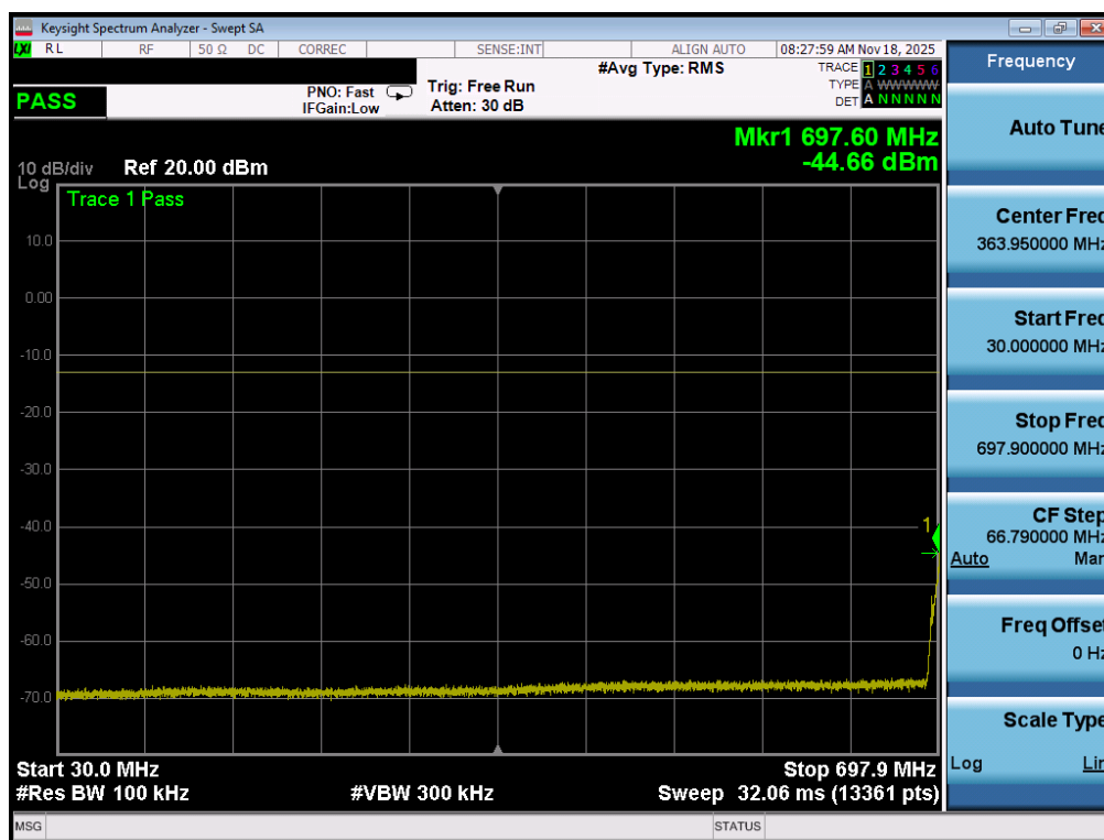
Plot 7-114. Conducted Spurious Plot (LTE Band 12/17 - 10MHz QPSK - 1 RB - Low Channel - ANT1)
