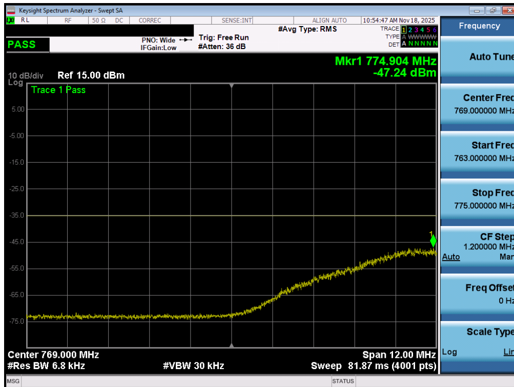
Plot 7-176. Lower Emission Mask Plot (LTE Band 13 - 5MHz QPSK – Full RB - ANT2)
