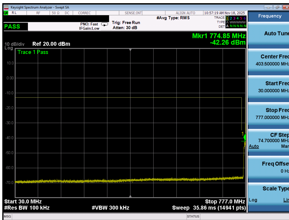
Plot 7-135. Conducted Spurious Plot (LTE Band 13 - 10MHz QPSK - 1 RB)
