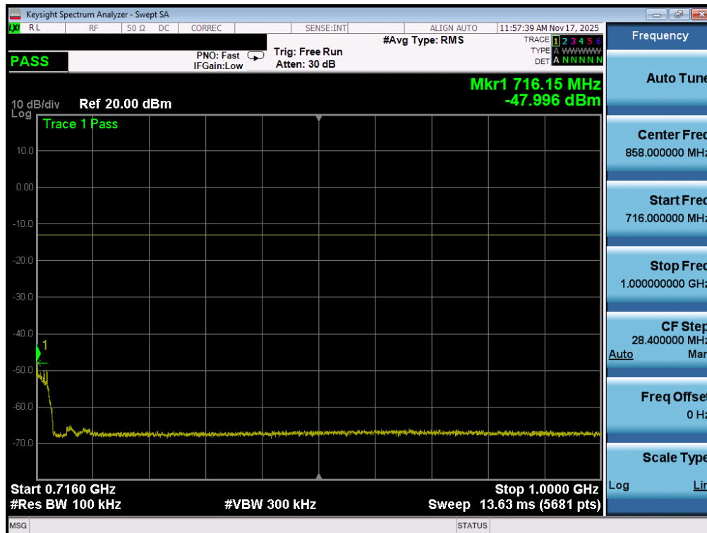
Plot 7-121. Conducted Spurious Plot (NR Band n12 - 15.0MHz - 1 RB - High Channel - ANT1)
