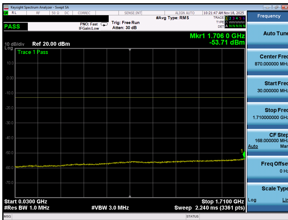
Plot 7-141. Conducted Spurious Plot (LTE Band 66/4 - 20MHz QPSK - 1 RB – High Channel)
