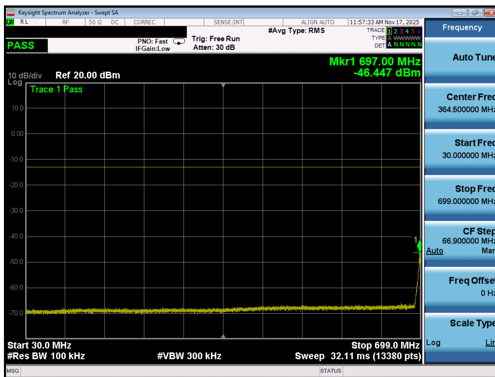
Plot 7-120. Conducted Spurious Plot (NR Band n12 - 15.0MHz - 1 RB - High Channel - ANT1)
