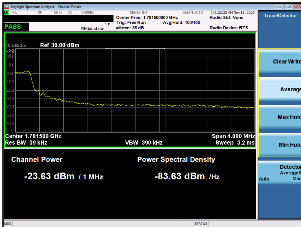
Plot 7-162. Upper Extended Band Edge Plot (LTE Band 66 – 5MHz QPSK – Full RB - ANT1)
