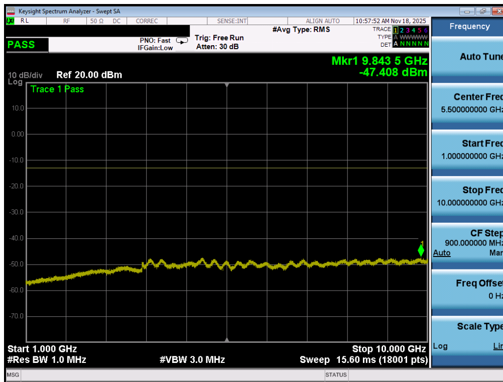
Plot 7-137. Conducted Spurious Plot (LTE Band 13 - 10MHz QPSK - 1 RB)
