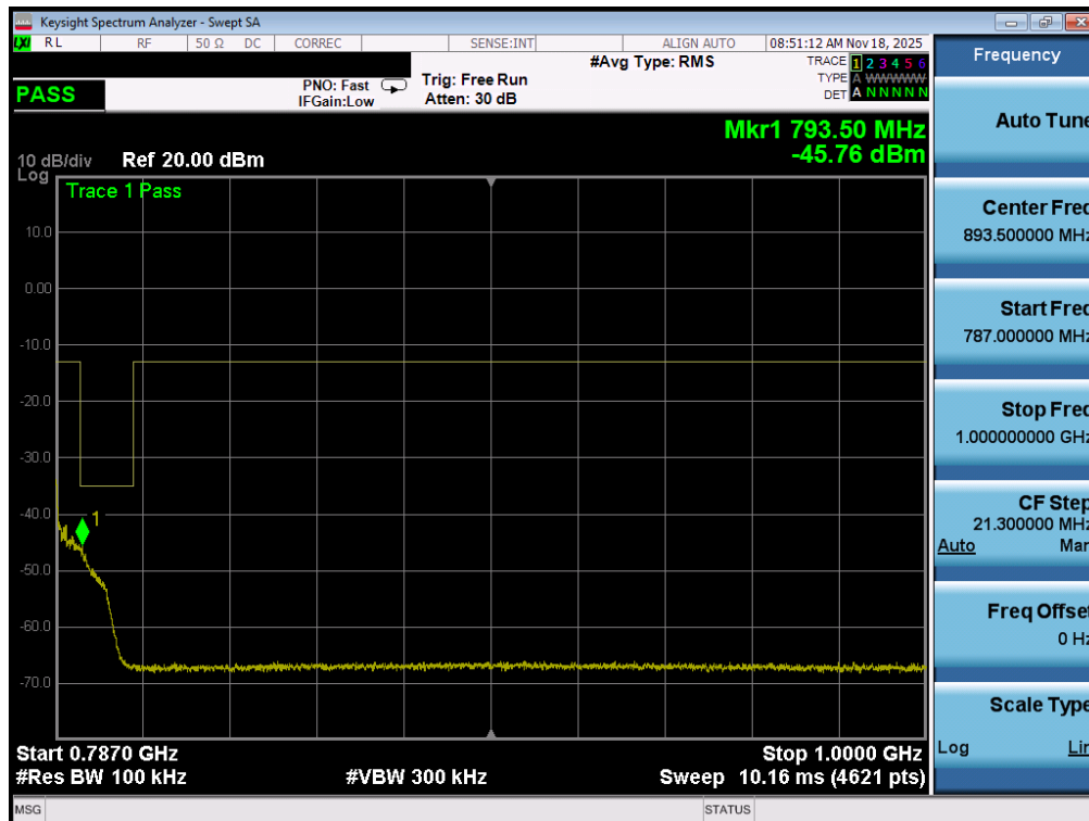
Plot 7-118. Conducted Spurious Plot (LTE Band 13 - 10MHz QPSK - 1 RB)
