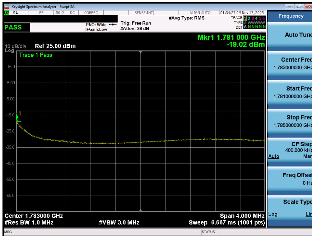
Plot 7-168. Upper Extended Band Edge Plot (NR Band n66 – 10.0MHz - Full RB - ANT1)
