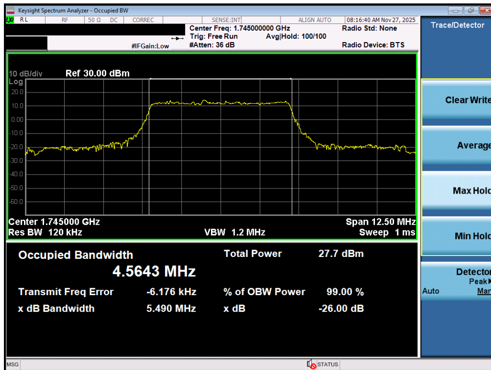
Plot 7-109. Occupied Bandwidth Plot (NR Band n66 - 5.0MHz CP-OFDM QPSK - Full RB – ANT2)
