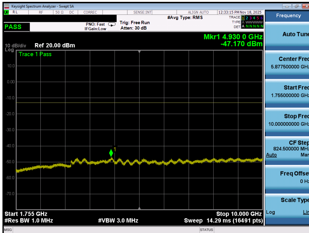
Plot 7-130. Conducted Spurious Plot (WCDMA-AWS - 5MHz QPSK - 1 RB - Low Channel - ANT2)
