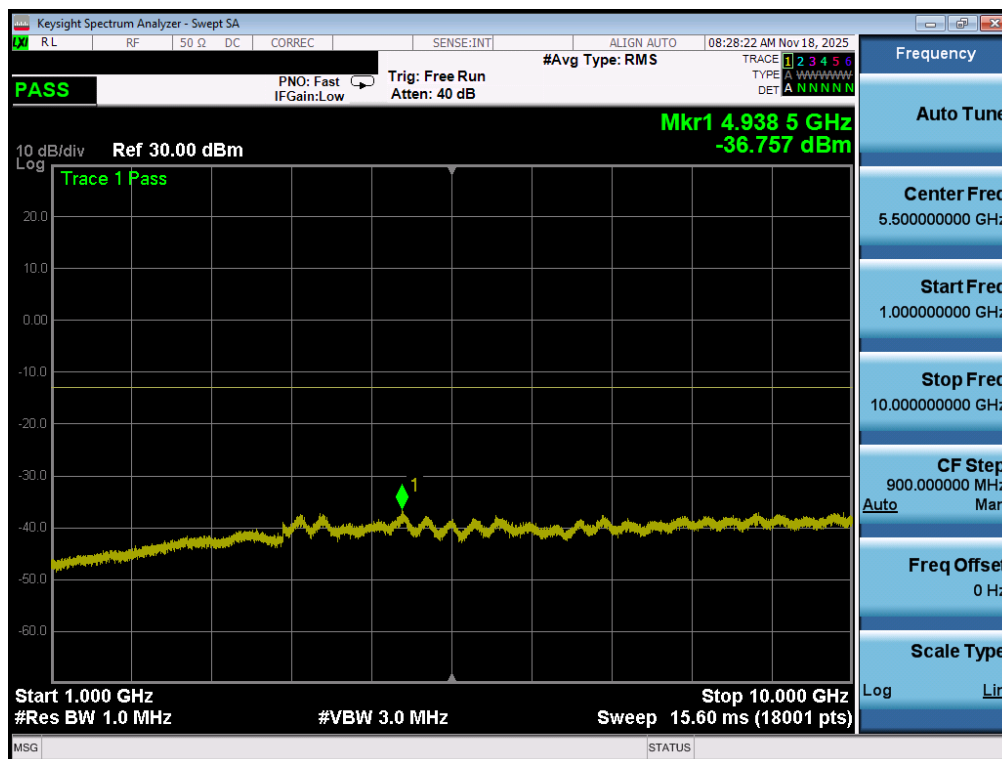
Plot 7-116. Conducted Spurious Plot (LTE Band 12/17 - 10MHz QPSK - 1 RB - Low Channel - ANT1)
