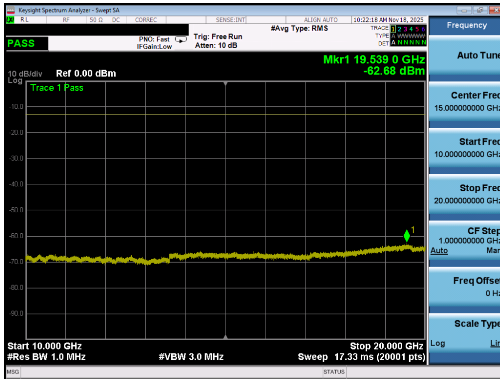
Plot 7-143. Conducted Spurious Plot (LTE Band 66/4 - 20MHz QPSK - 1 RB – High Channel)
