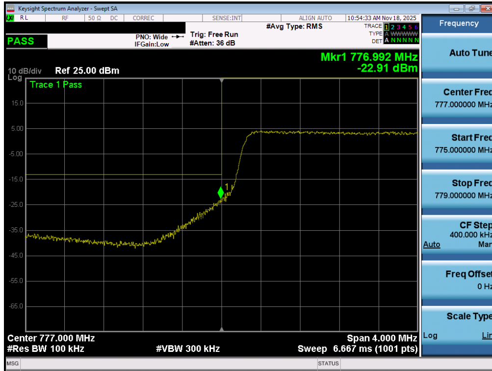
Plot 7-175. Lower Band Edge Plot (LTE Band 13 - 5MHz QPSK – Full RB - ANT2)
