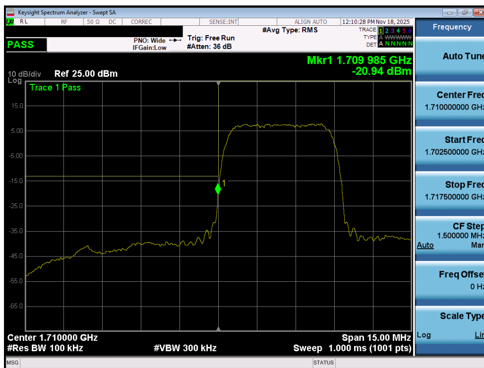
Plot 7-147. Lower Band Edge Plot (WCDMA AWS – Ch. 1312 – ANT1)
