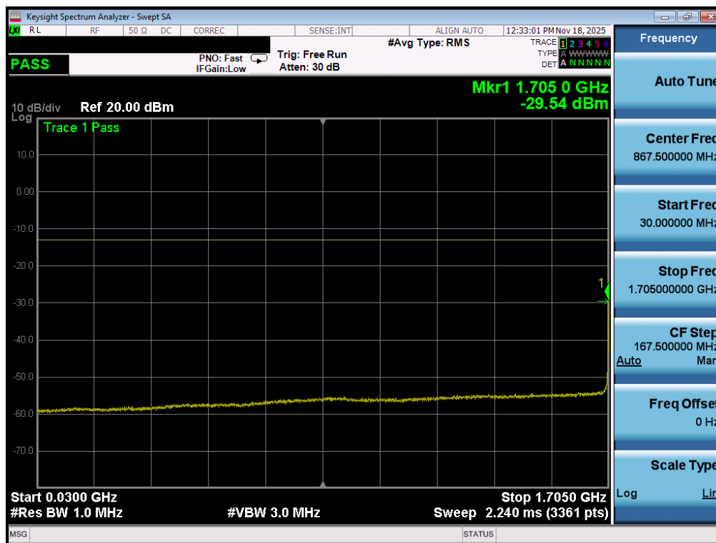
Plot 7-129. Conducted Spurious Plot (WCDMA-AWS - 5MHz QPSK - 1 RB – Low Channel - ANT2)
