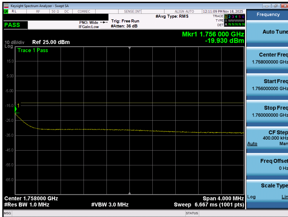
Plot 7-150. Upper Extended Band Edge Plot (WCDMA AWS – Ch. 1513– ANT1)
