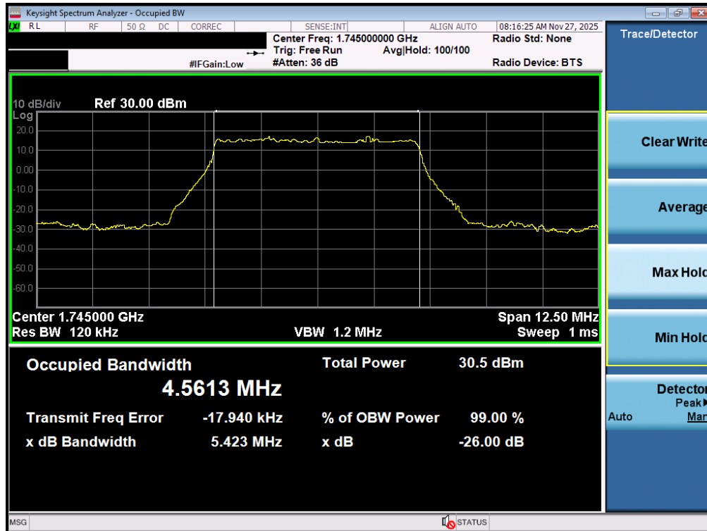
Plot 7-108. Occupied Bandwidth Plot (NR Band n66 - 5.0MHz DFT-s-OFDM BPSK - Full RB – ANT2)
