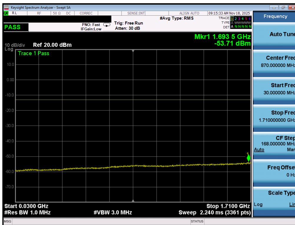
Plot 7-123. Conducted Spurious Plot (LTE Band 66/4 - 20MHz QPSK - 1 RB – High Channel)
