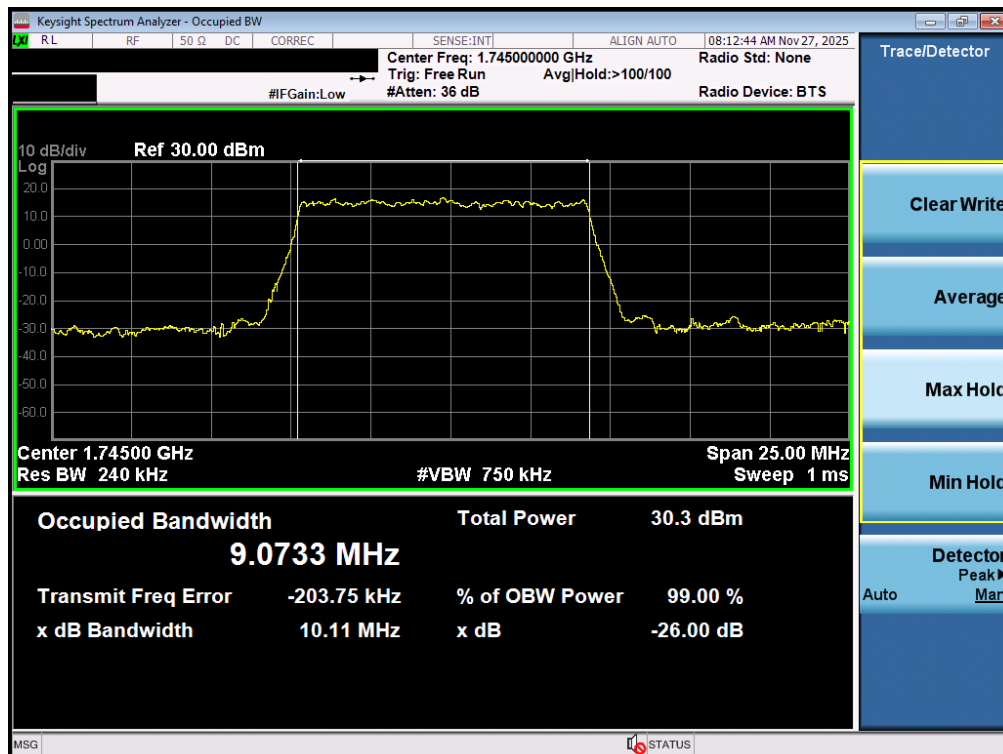
Plot 7-105. Occupied Bandwidth Plot (NR Band n66 - 10.0MHz DFT-s-OFDM BPSK - Full RB – ANT2)
