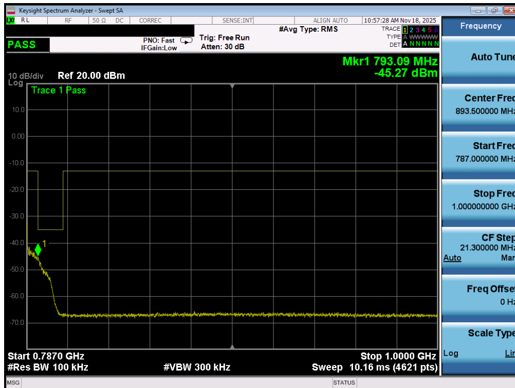
Plot 7-136. Conducted Spurious Plot (LTE Band 13 - 10MHz QPSK - 1 RB)
