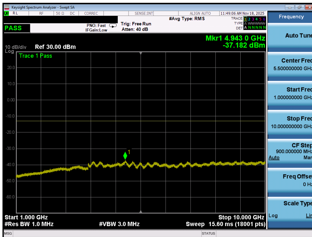
Plot 7-134. Conducted Spurious Plot (LTE Band 12/17 - 10MHz QPSK - 1 RB - Mid Channel - ANT2)
