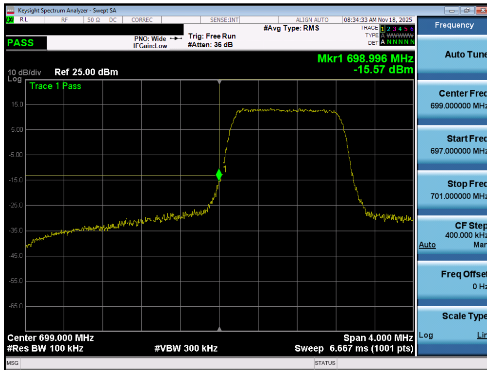
Plot 7-151. Lower Band Edge Plot (LTE Band 12 – 1.4MHz QPSK – Full RB - ANT1)
