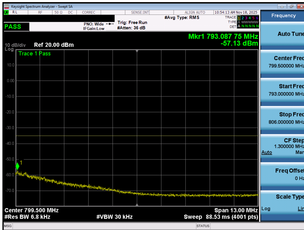
Plot 7-178. Upper Emission Mask Plot (LTE Band 13 - 5MHz QPSK – Full RB - ANT2)
