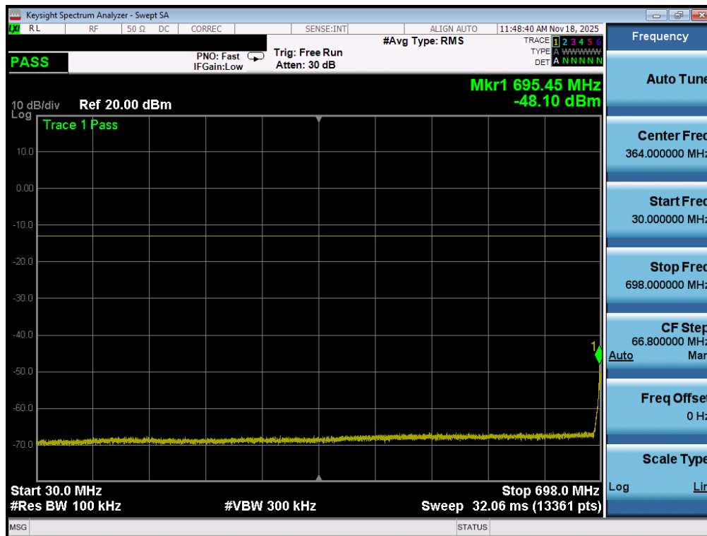
Plot 7-132. Conducted Spurious Plot (LTE Band 12/17 - 10MHz QPSK - 1 RB - Mid Channel - ANT2)
