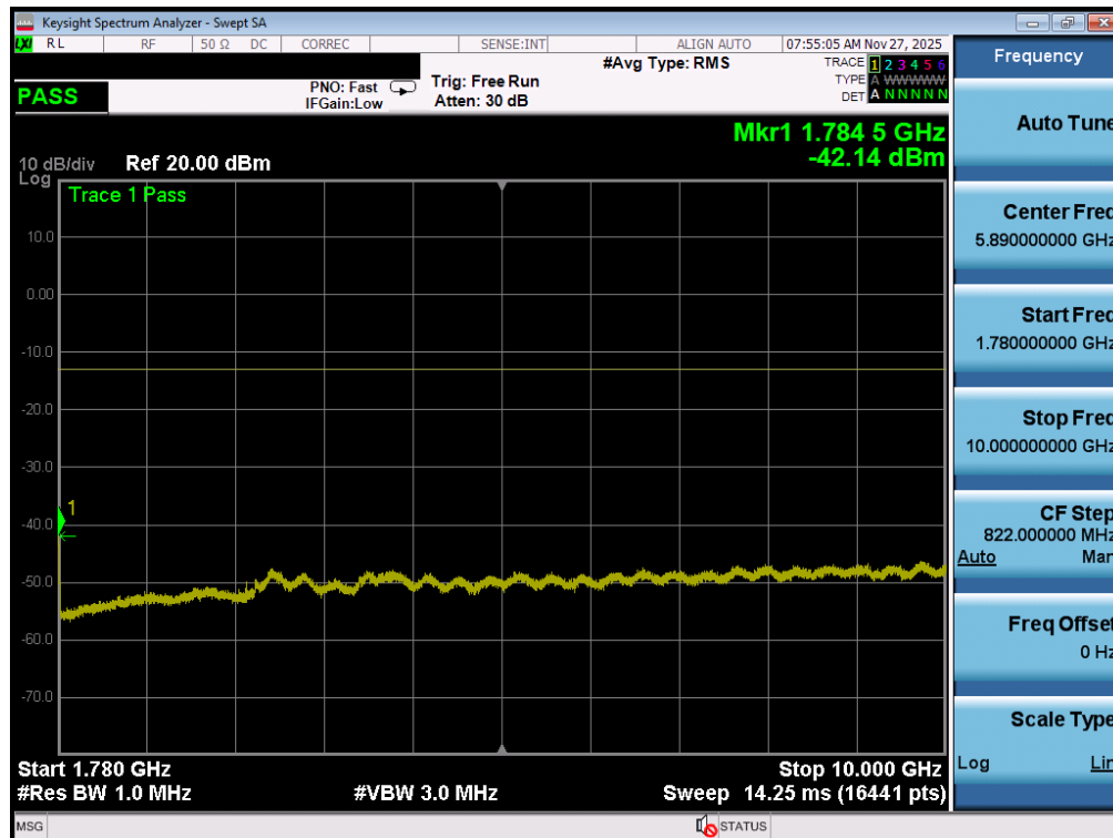
Plot 7-145. Conducted Spurious Plot (NR Band n66 - 40.0MHz - 1 RB - High Channel - ANT2)
