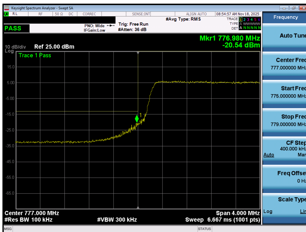
Plot 7-153. Lower Band Edge Plot (LTE Band 13 - 5MHz QPSK – Full RB - ANT1)
