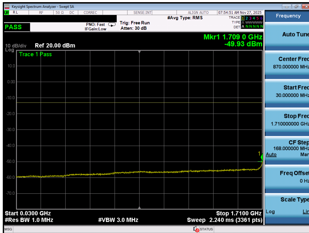
Plot 7-144. Conducted Spurious Plot (NR Band n66 - 40.0MHz - 1 RB - High Channel - ANT2)
