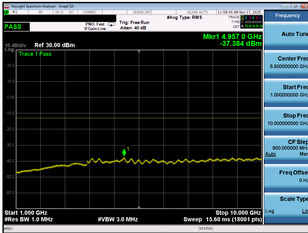
Plot 7-122. Conducted Spurious Plot (NR Band n12 - 15.0MHz - 1 RB - High Channel - ANT1)
