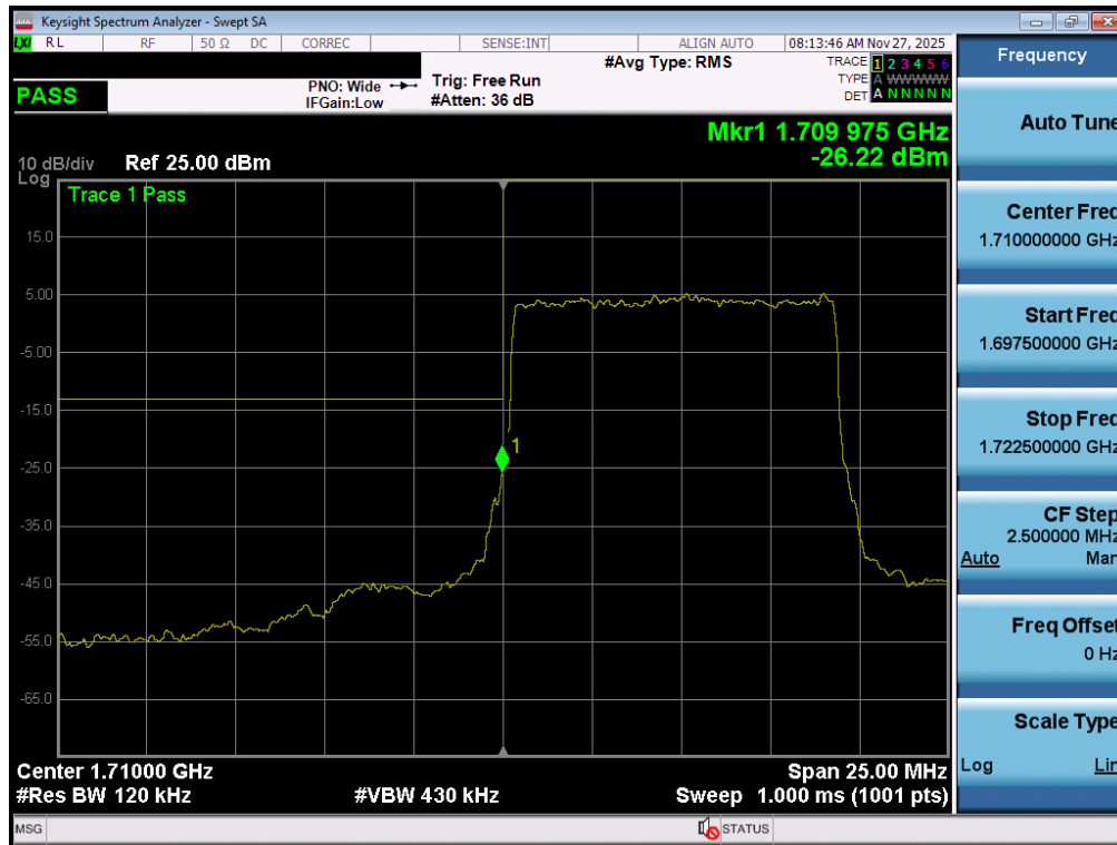
Plot 7-187. Lower Band Edge Plot (NR Band n66 – 10.0MHz - Full RB - ANT2)
