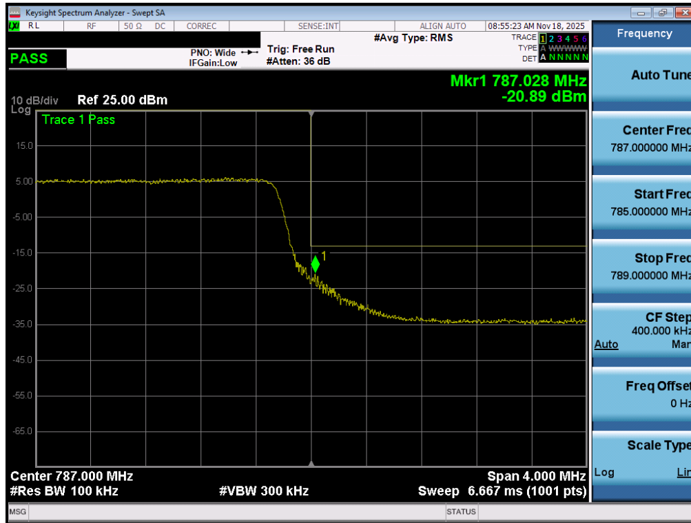
Plot 7-155. Upper Band Edge Plot (LTE Band 13 - 5MHz QPSK - Full RB - ANT1)
