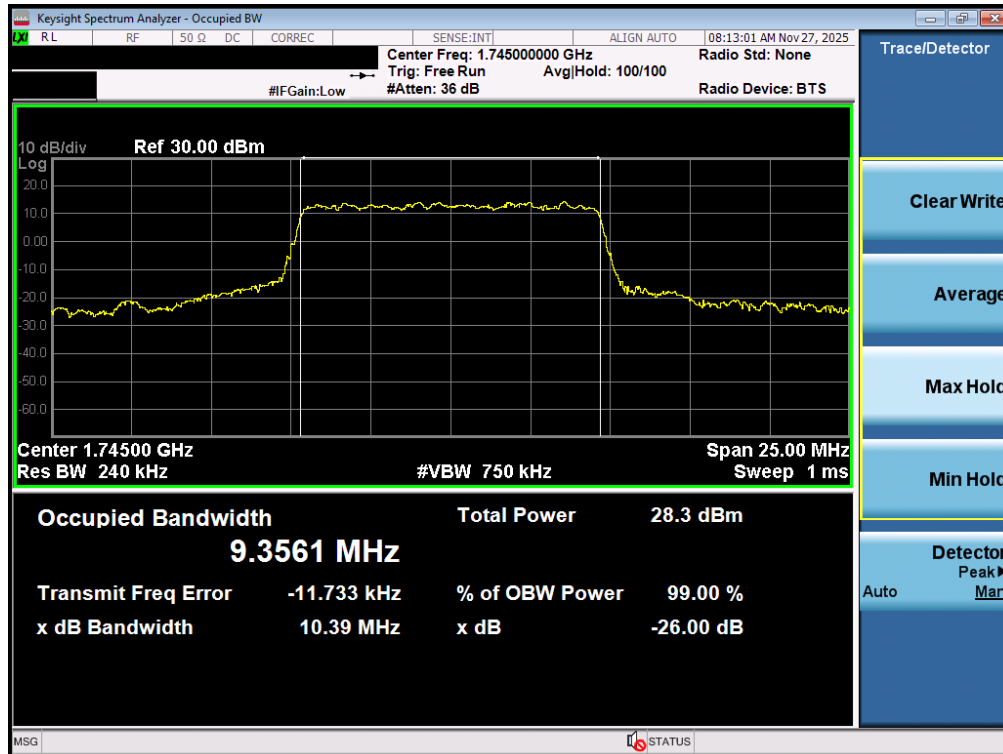
Plot 7-106. Occupied Bandwidth Plot (NR Band n66 - 10.0MHz CP-OFDM QPSK - Full RB – ANT2)
