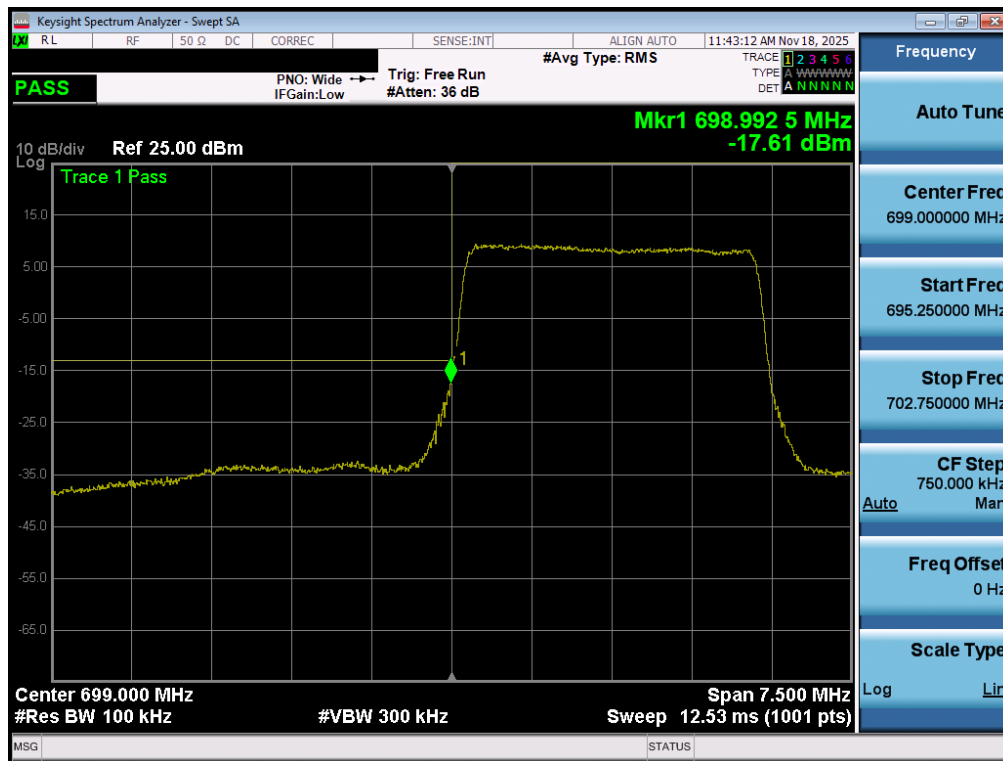
Plot 7-173. Lower Band Edge Plot (LTE Band 12 – 3MHz QPSK – Full RB - ANT2)
