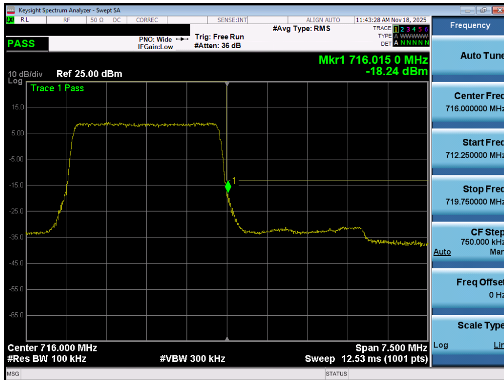
Plot 7-174. Upper Band Edge Plot (LTE Band 12 – 3MHz QPSK – Full RB - ANT2)
