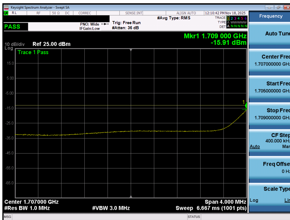
Plot 7-148. Lower Extended Band Edge Plot (WCDMA AWS – Ch. 1312 – ANT1)
