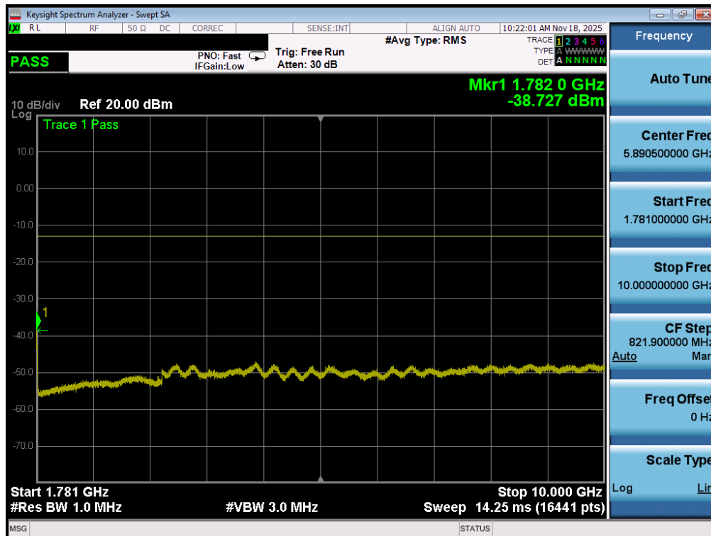
Plot 7-142. Conducted Spurious Plot (LTE Band 66/4 - 20MHz QPSK - 1 RB – High Channel)
