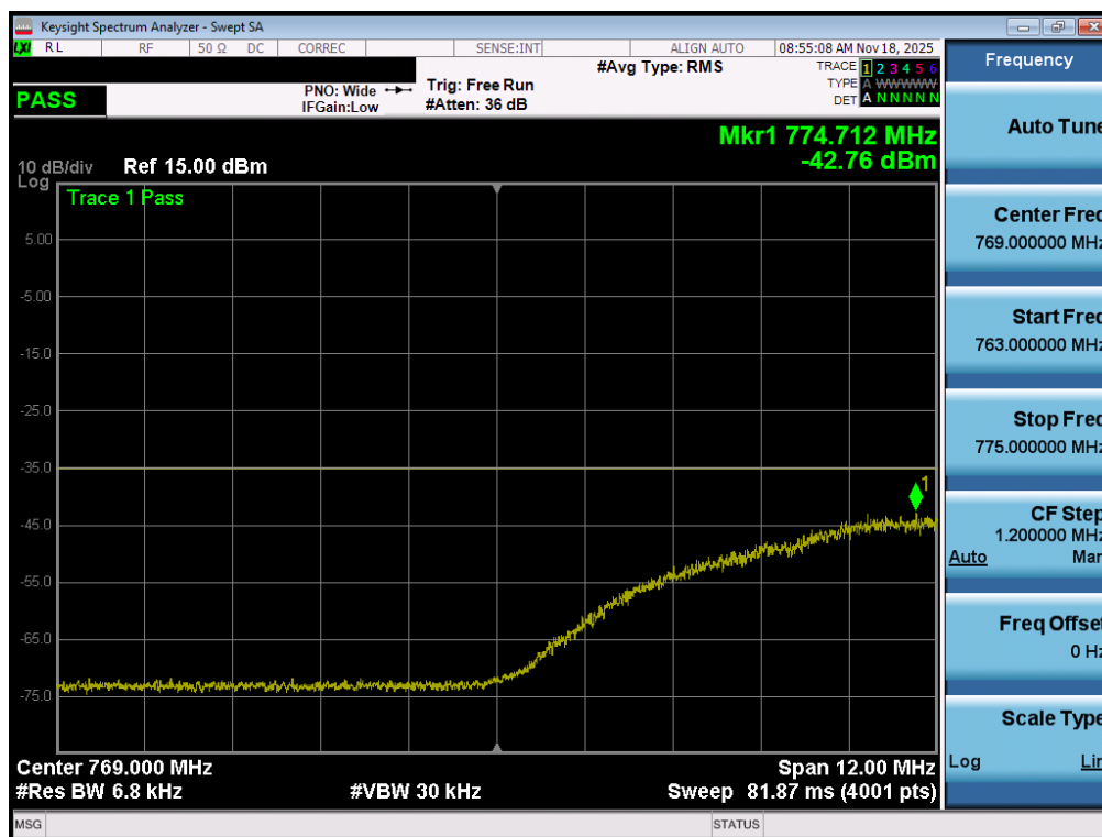
Plot 7-154. Lower Emission Mask Plot (LTE Band 13 - 5MHz QPSK – Full RB - ANT1)
