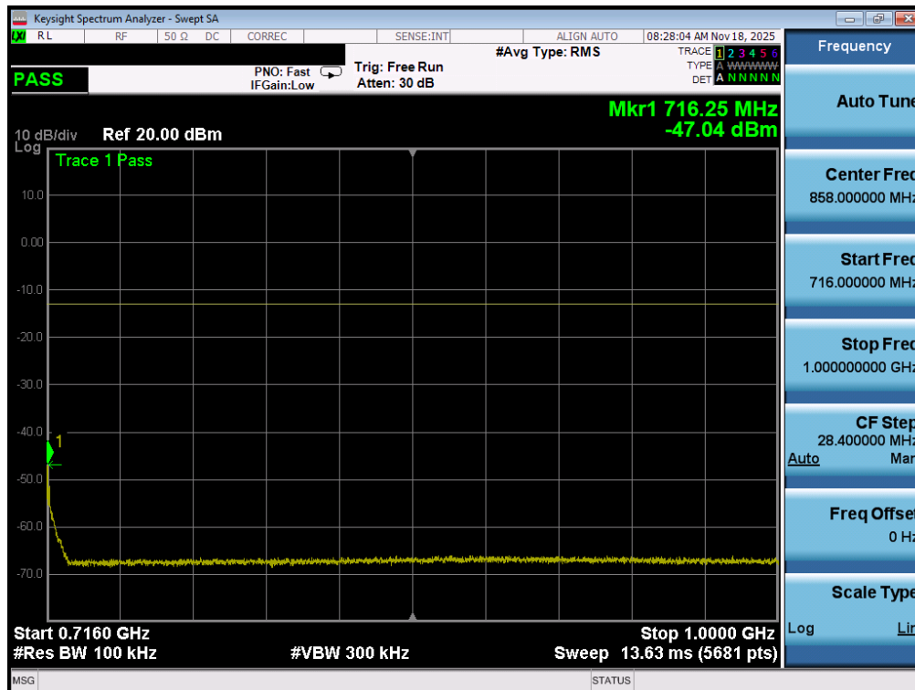
Plot 7-115. Conducted Spurious Plot (LTE Band 12/17 - 10MHz QPSK - 1 RB - Low Channel - ANT1)
