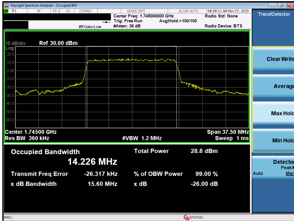
Plot 7-104. Occupied Bandwidth Plot (NR Band n66 - 15.0MHz CP-OFDM 16QAM - Full RB – ANT2)
