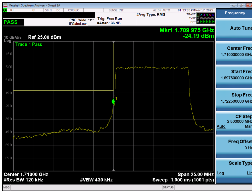
Plot 7-165. Lower Band Edge Plot (NR Band n66 – 10.0MHz - Full RB - ANT1)
