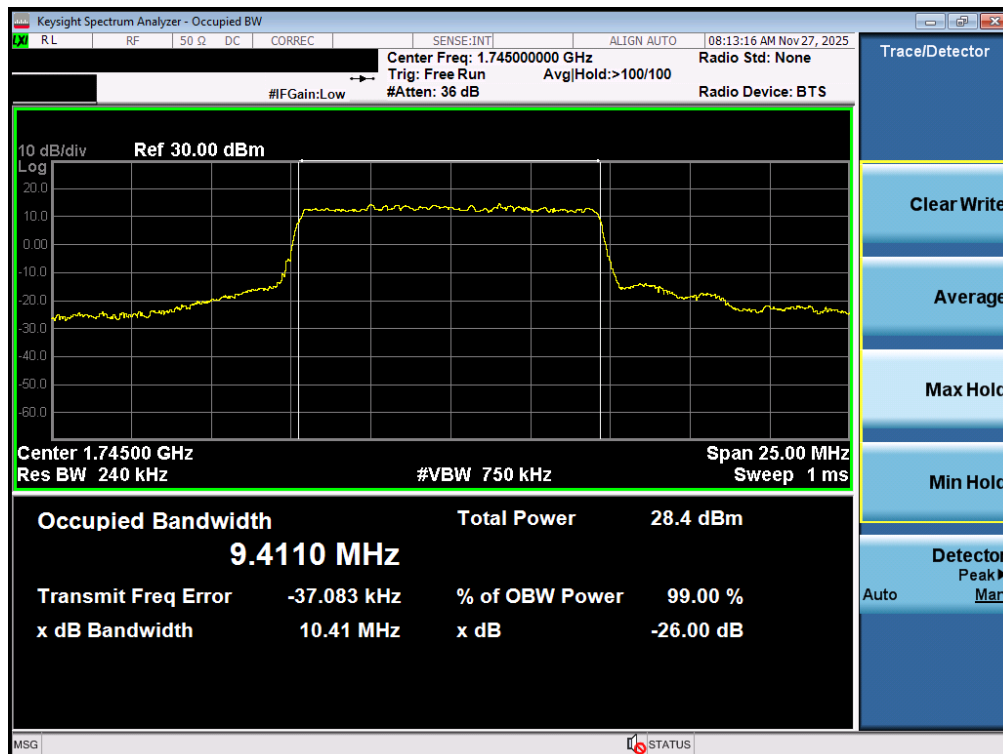
Plot 7-107. Occupied Bandwidth Plot (NR Band n66 - 10.0MHz CP-OFDM 16QAM - Full RB – ANT2)
