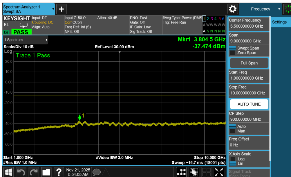
Plot 7-140. Conducted Spurious Plot (NR Band n12 - 15.0MHz - 1 RB – Low Channel - ANT2)
