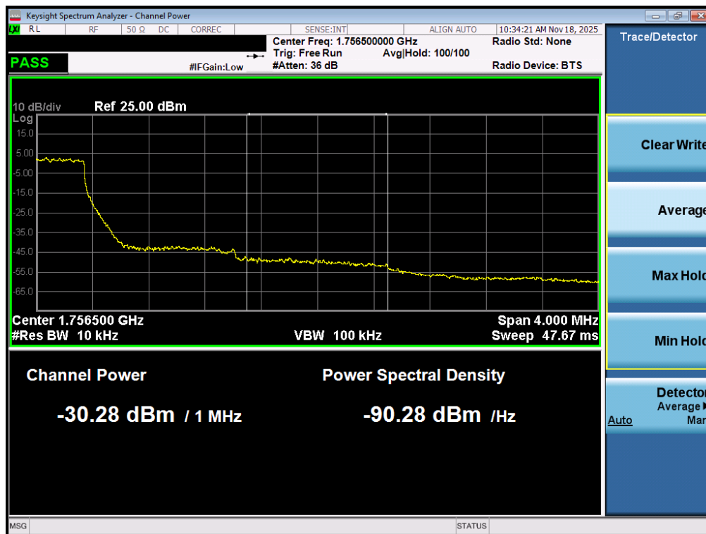
Plot 7-182. Upper Extended Band Edge Plot (LTE Band 4 – 1.4MHz QPSK – Full RB - ANT2)
