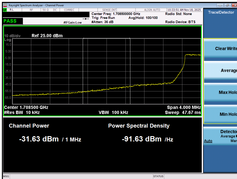
Plot 7-180. Lower Extended Band Edge Plot (LTE Band 66/4 – 1.4MHz QPSK – Full RB - ANT2)
