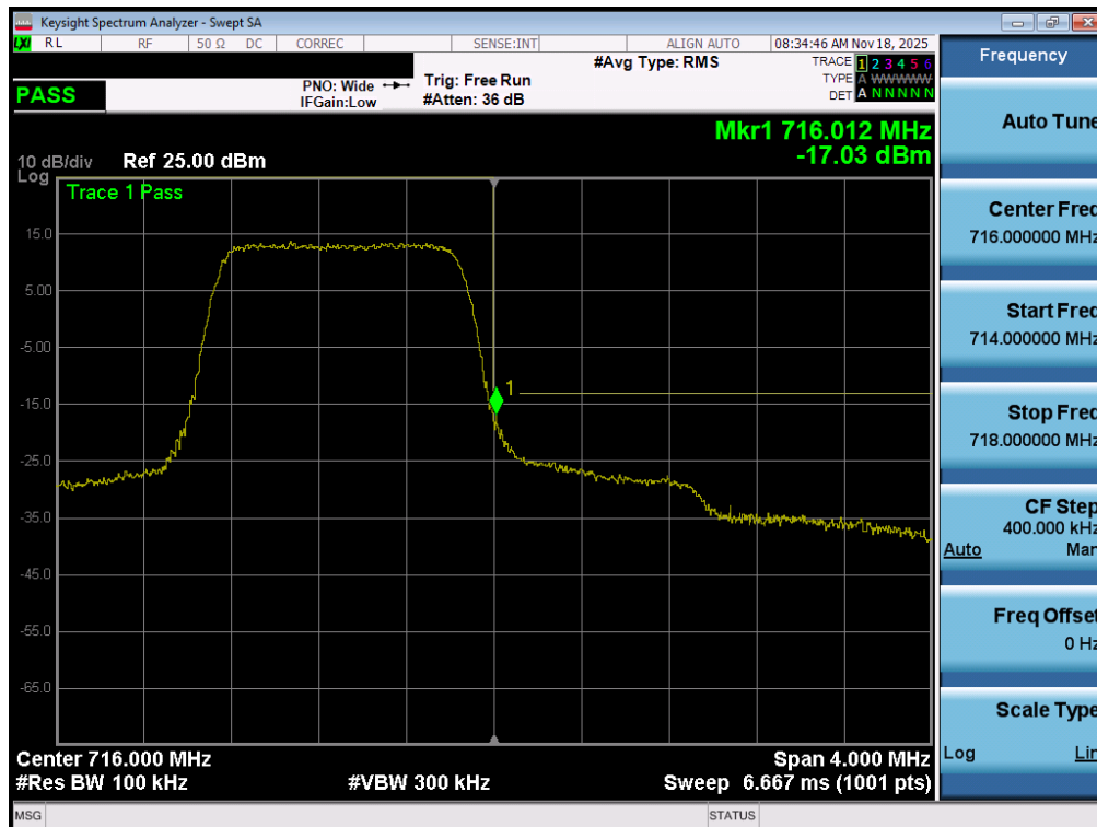
Plot 7-152. Upper Band Edge Plot (LTE Band 12 – 1.4MHz QPSK – Full RB - ANT1)
