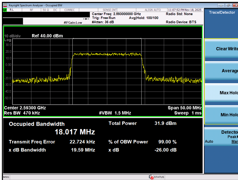
Plot 7-50. Occupied Bandwidth Plot (LTE Band 41(PC2)- 20MHz QPSK - Full RB - Ant2)
