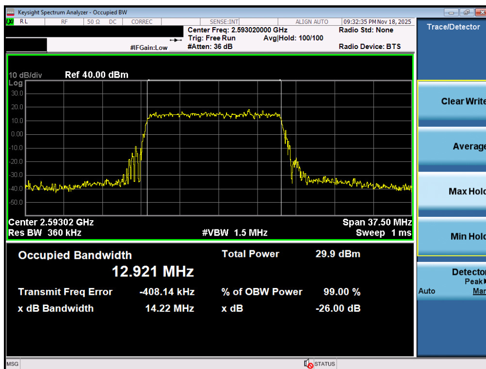
Plot 7-93. Occupied Bandwidth Plot (NR Band n41 PC3 – 15MHz \pi/2 BPSK – Full RB – Ant2)
