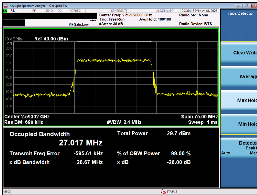
Plot 7-87. Occupied Bandwidth Plot (NR Band n41 PC3 – 30MHz \pi/2 BPSK – Full RB – Ant2)
