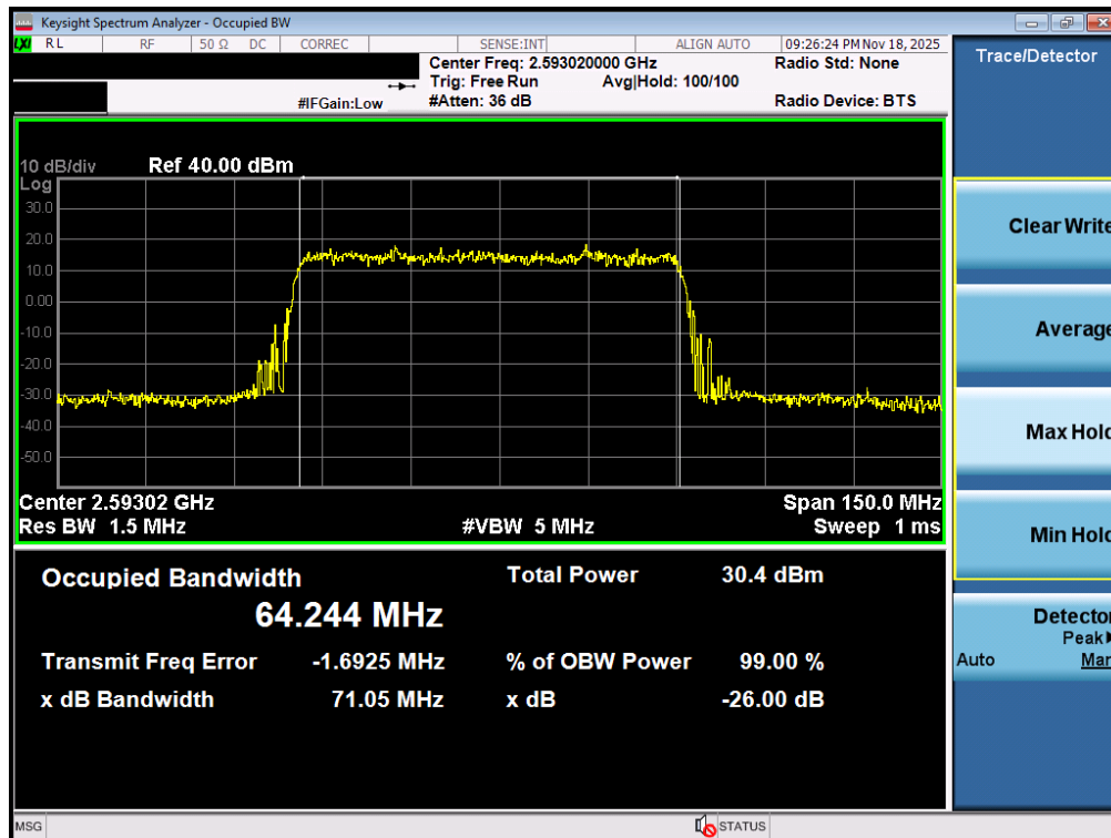
Plot 7-75. Occupied Bandwidth Plot (NR Band n41 PC3 – 70MHz \pi/2 BPSK – Full RB – Ant2)
