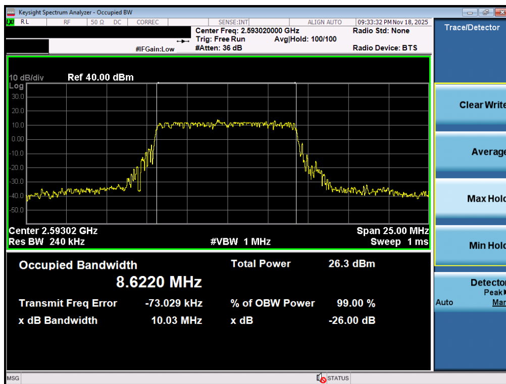
Plot 7-96. Occupied Bandwidth Plot (NR Band n41 PC3 – 10MHz \pi/2 BPSK – Full RB – Ant2)
