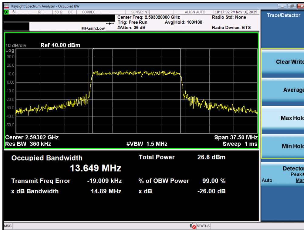
Plot 7-45. Occupied Bandwidth Plot (NR Band n41 PC3 - 15MHz QPSK - Full RB - Ant1)
