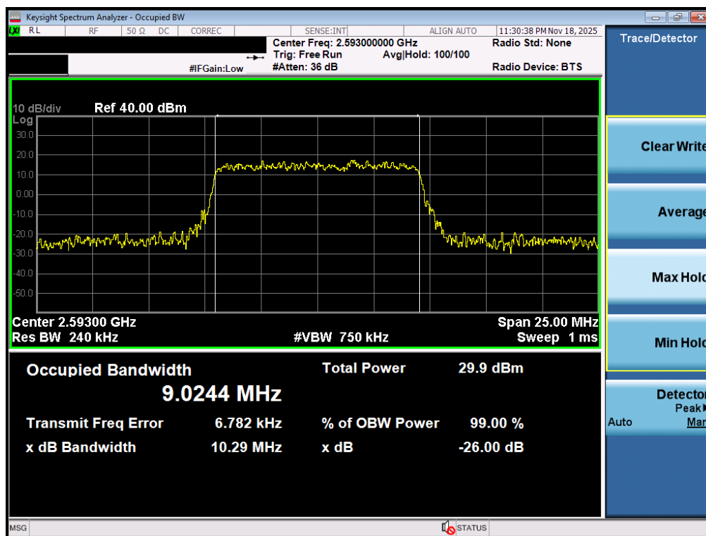
Plot 7-62. Occupied Bandwidth Plot (LTE Band 41(PC3)- 10MHz QPSK - Full RB - Ant2)
