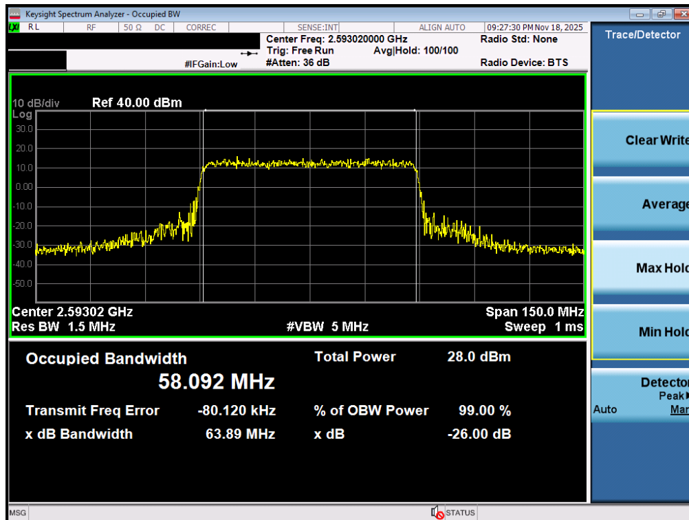
Plot 7-79. Occupied Bandwidth Plot (NR Band n41 PC3 – 60MHz QPSK – Full RB – Ant2)
