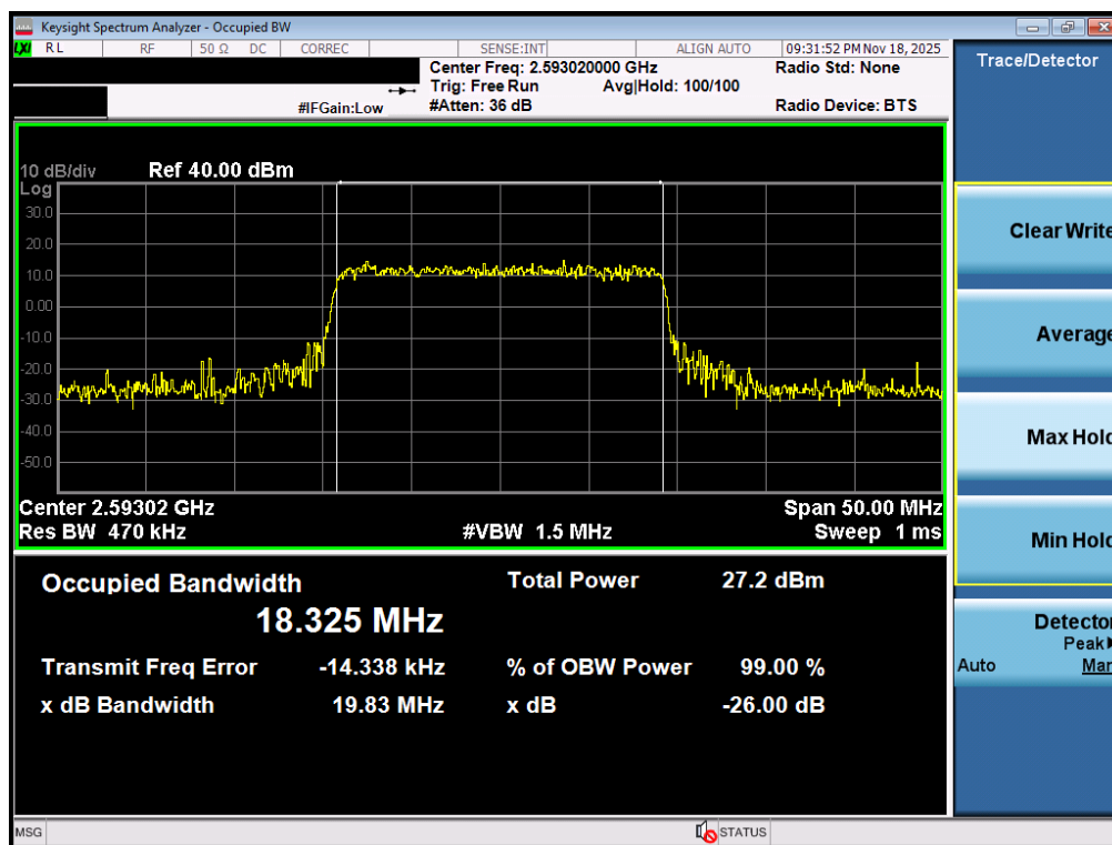
Plot 7-92. Occupied Bandwidth Plot (NR Band n41 PC3 – 20MHz 16-QAM – Full RB – Ant2)
