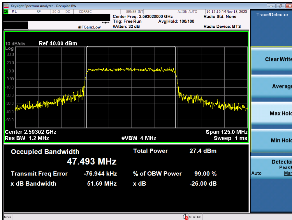
Plot 7-34. Occupied Bandwidth Plot (NR Band n41 PC3 - 50MHz 16-QAM - Full RB - Ant1)
