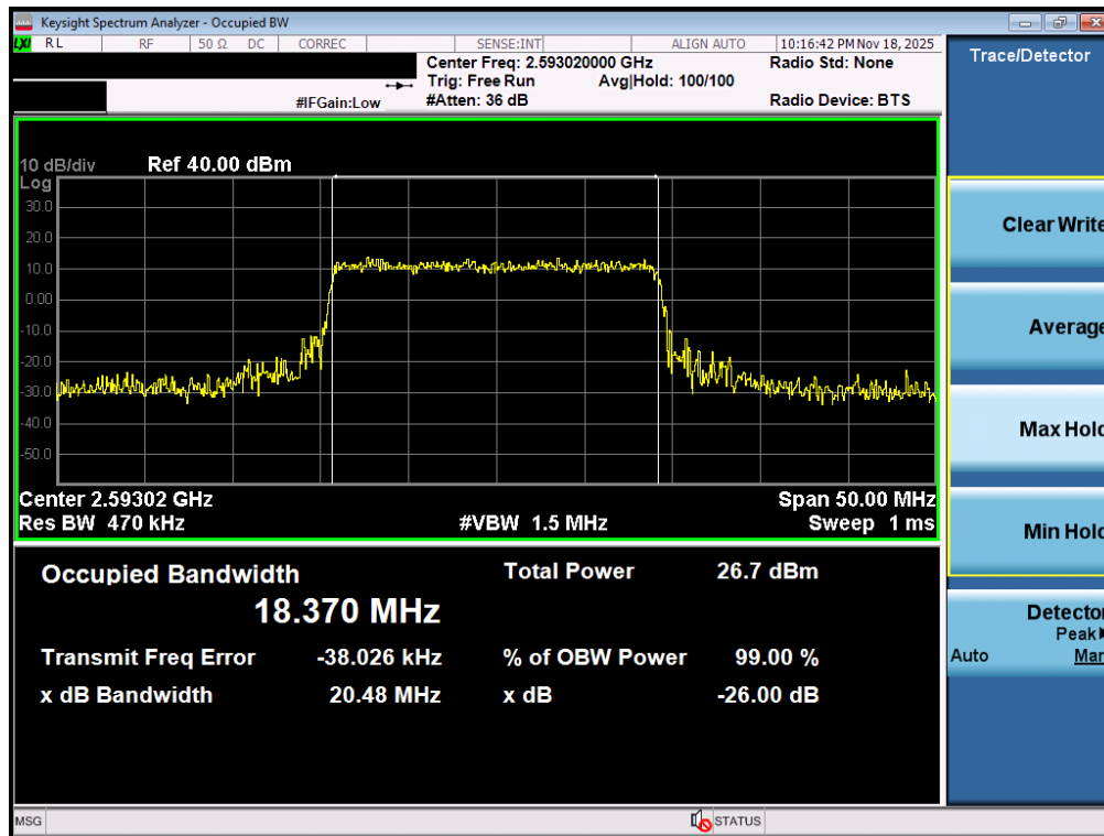
Plot 7-43. Occupied Bandwidth Plot (NR Band n41 PC3 - 20MHz 16-QAM - Full RB - Ant1)
