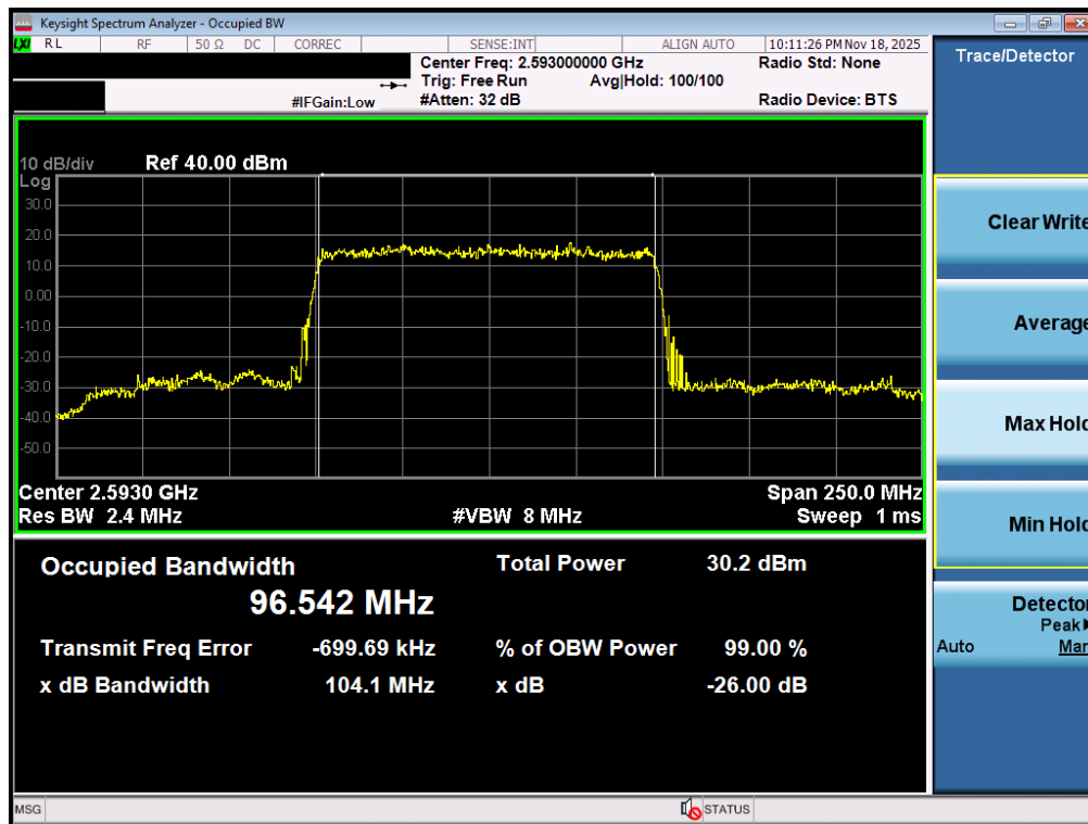
Plot 7-17. Occupied Bandwidth Plot (NR Band n41 PC3 – 100MHz \pi/2 BPSK – Full RB – Ant1)
