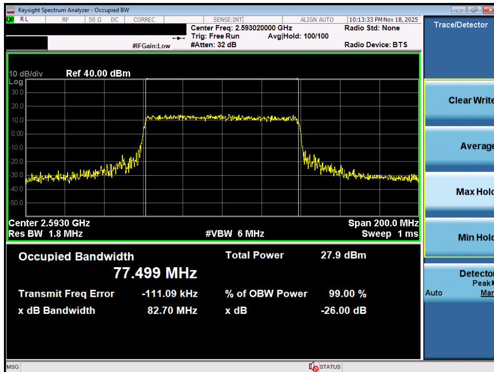
Plot 7-24. Occupied Bandwidth Plot (NR Band n41 PC3 – 80MHz QPSK – Full RB – Ant1)
