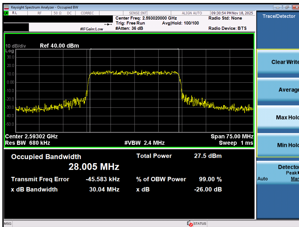
Plot 7-88. Occupied Bandwidth Plot (NR Band n41 PC3 - 30MHz QPSK - Full RB - Ant2)
