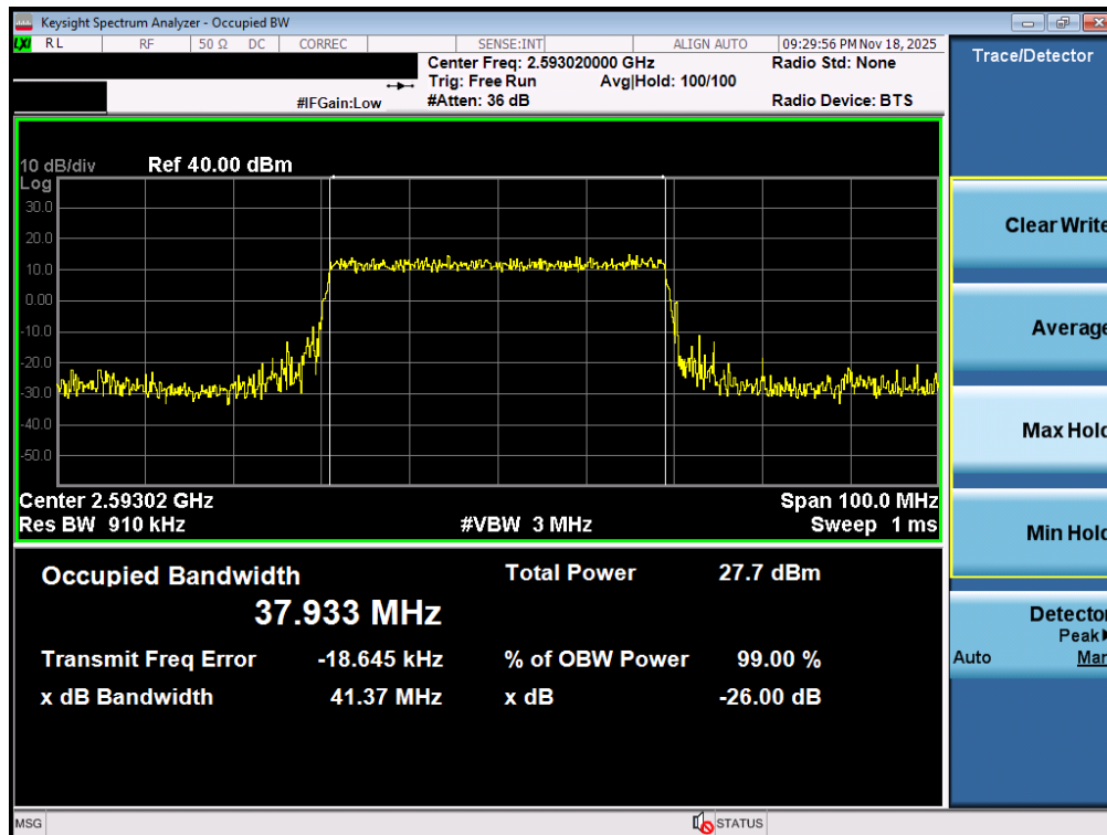
Plot 7-85. Occupied Bandwidth Plot (NR Band n41 PC3 – 40MHz QPSK – Full RB – Ant2)
