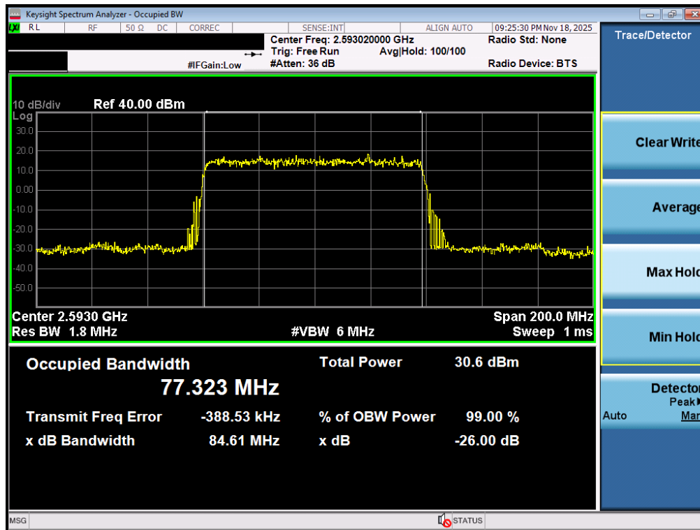
Plot 7-72. Occupied Bandwidth Plot (NR Band n41 PC3 – 80MHz \pi/2 BPSK – Full RB – Ant2)
