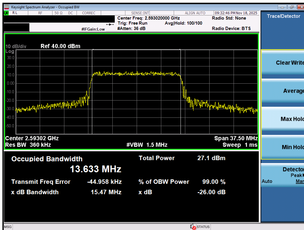
Plot 7-95. Occupied Bandwidth Plot (NR Band n41 PC3 - 15MHz 16-QAM - Full RB - Ant2)
