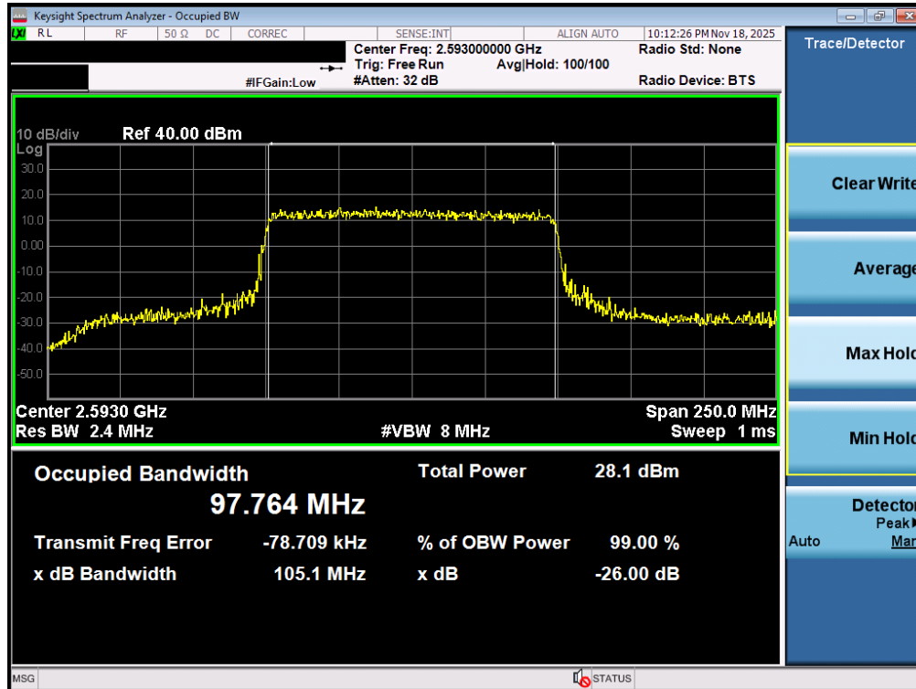
Plot 7-18. Occupied Bandwidth Plot (NR Band n41 PC3 – 100MHz QPSK – Full RB – Ant1)
