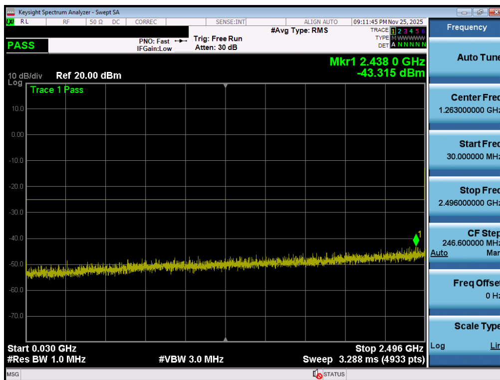
Plot 7-99. Conducted Spurious Plot (LTE Band 41(PC2)- 20MHz QPSK - RB Size 1, RB Offset 50 - Mid Channel - Ant1)
