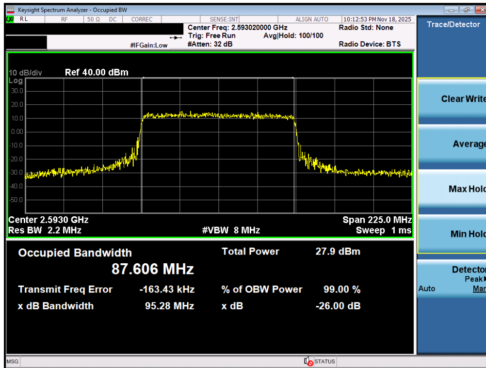
Plot 7-21. Occupied Bandwidth Plot (NR Band n41 PC3 - 90MHz QPSK - Full RB - Ant1)
