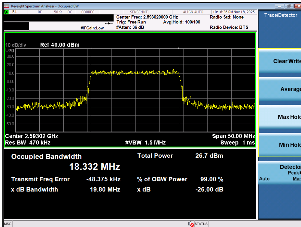
Plot 7-42. Occupied Bandwidth Plot (NR Band n41 PC3 – 20MHz QPSK – Full RB – Ant1)
