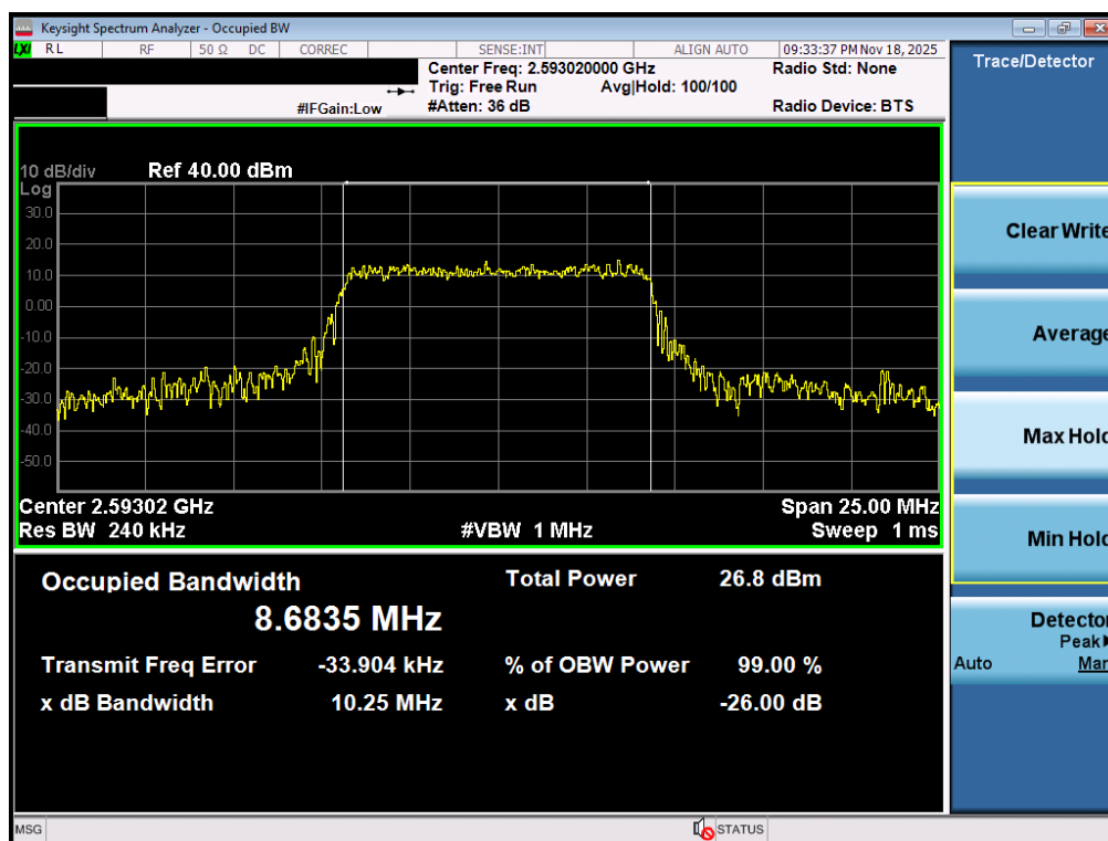
Plot 7-97. Occupied Bandwidth Plot (NR Band n41 PC3 – 10MHz QPSK – Full RB – Ant2)
