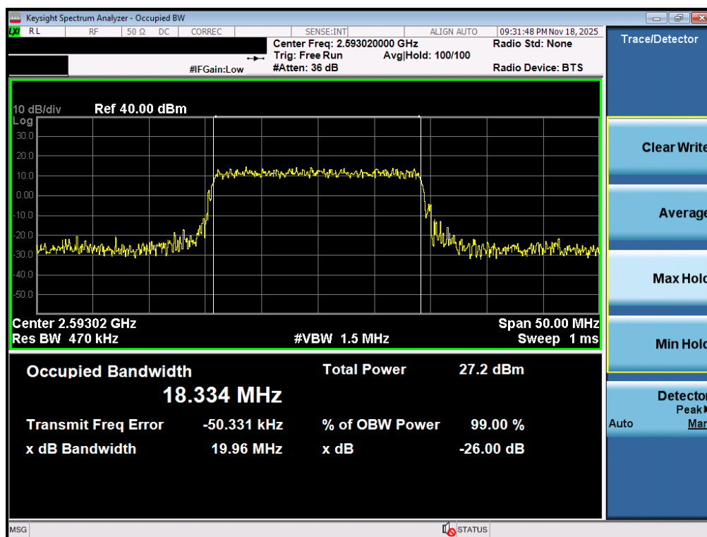
Plot 7-91. Occupied Bandwidth Plot (NR Band n41 PC3 – 20MHz QPSK – Full RB – Ant2)
