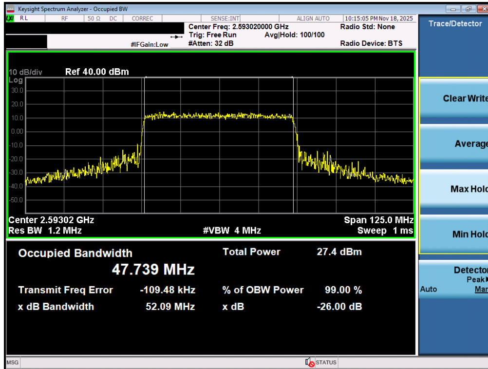
Plot 7-33. Occupied Bandwidth Plot (NR Band n41 PC3 - 50MHz QPSK - Full RB - Ant1)
