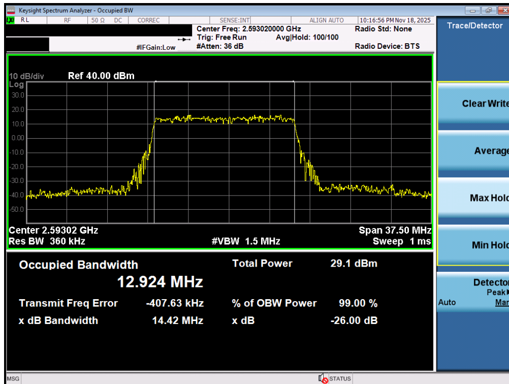
Plot 7-44. Occupied Bandwidth Plot (NR Band n41 PC3 - 15MHz \pi/2 BPSK - Full RB - Ant1)
