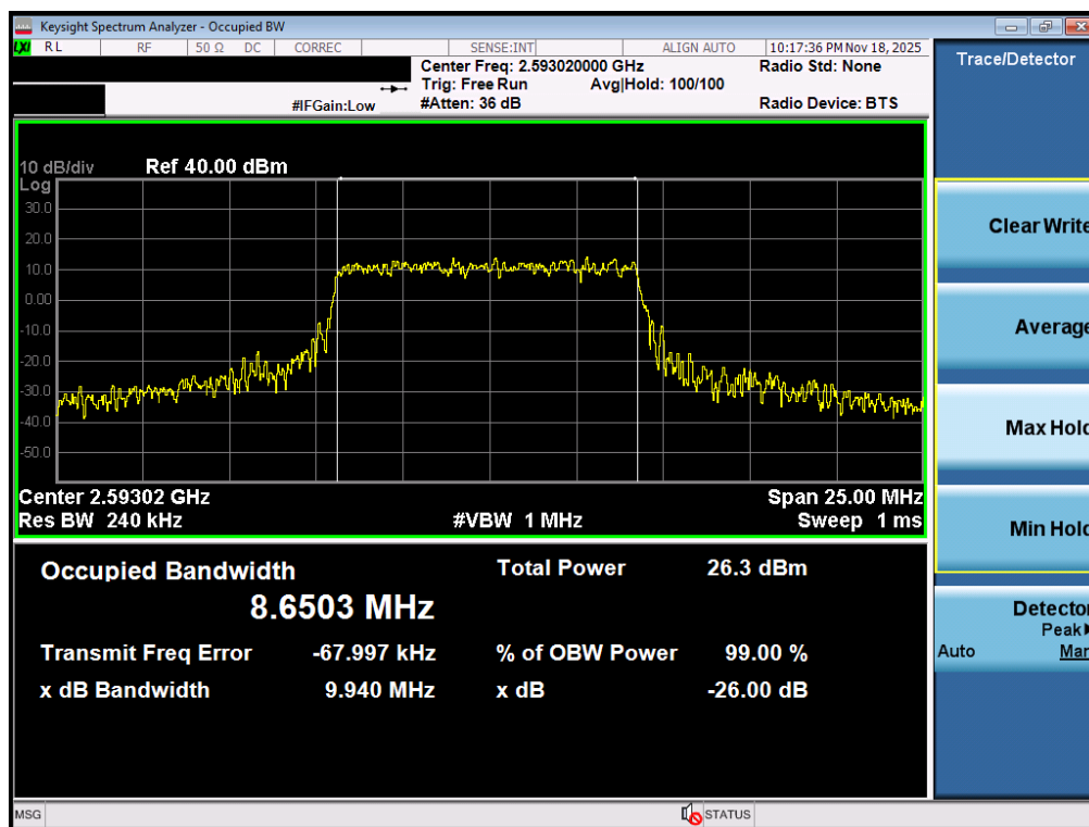
Plot 7-49. Occupied Bandwidth Plot (NR Band n41 PC3 – 10MHz 16-QAM – Full RB – Ant1)
