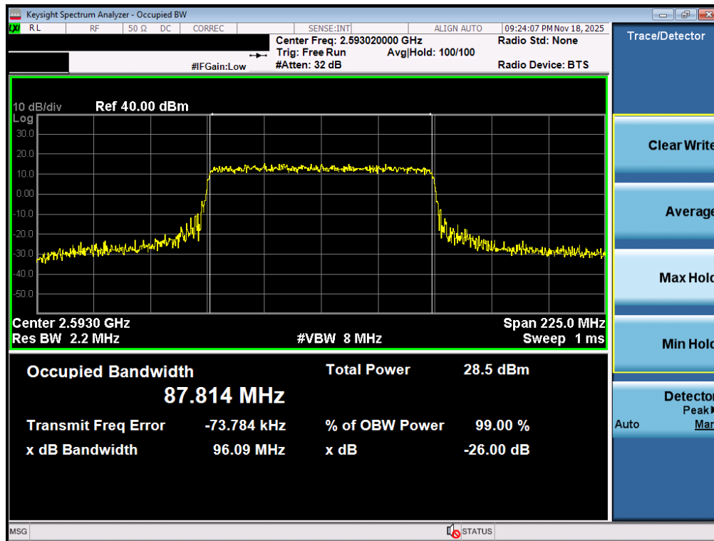
Plot 7-70. Occupied Bandwidth Plot (NR Band n41 PC3 - 90MHz QPSK - Full RB - Ant2)
