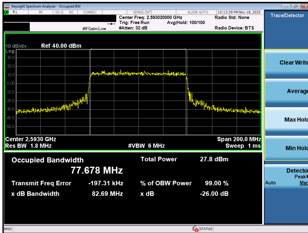
Plot 7-25. Occupied Bandwidth Plot (NR Band n41 PC3 – 80MHz 16-QAM – Full RB – Ant1)
