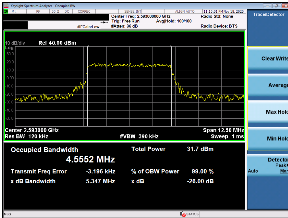
Plot 7-56. Occupied Bandwidth Plot (LTE Band 41(PC2)- 5MHz QPSK - Full RB - Ant2)
