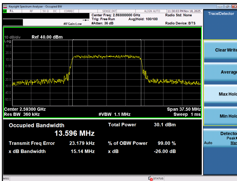
Plot 7-60. Occupied Bandwidth Plot (LTE Band 41(PC3)- 15MHz QPSK - Full RB - Ant2)
