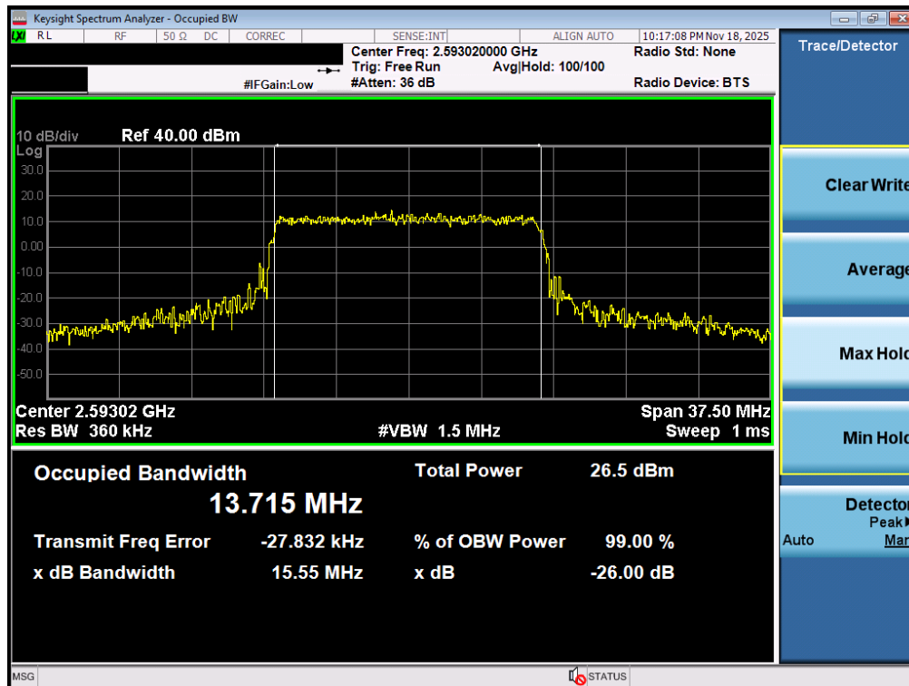
Plot 7-46. Occupied Bandwidth Plot (NR Band n41 PC3 - 15MHz 16-QAM - Full RB - Ant1)
