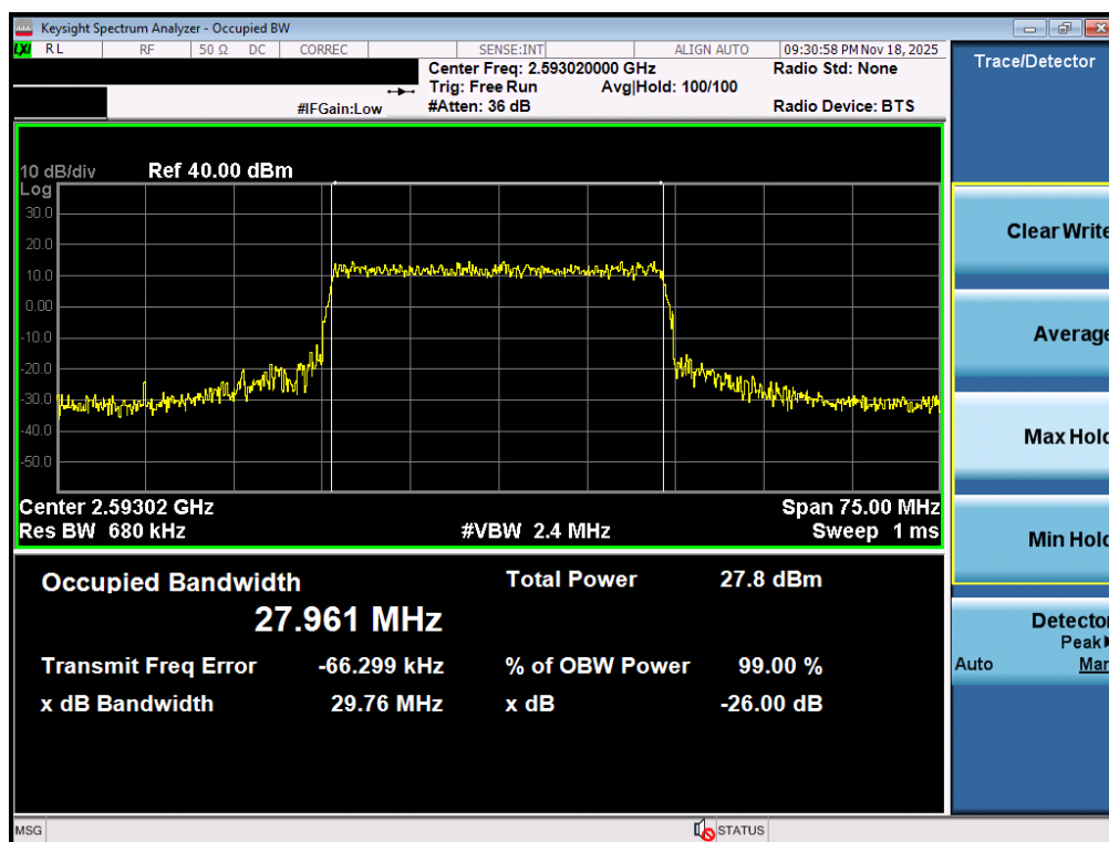
Plot 7-89. Occupied Bandwidth Plot (NR Band n41 PC3 - 30MHz 16-QAM - Full RB - Ant2)
