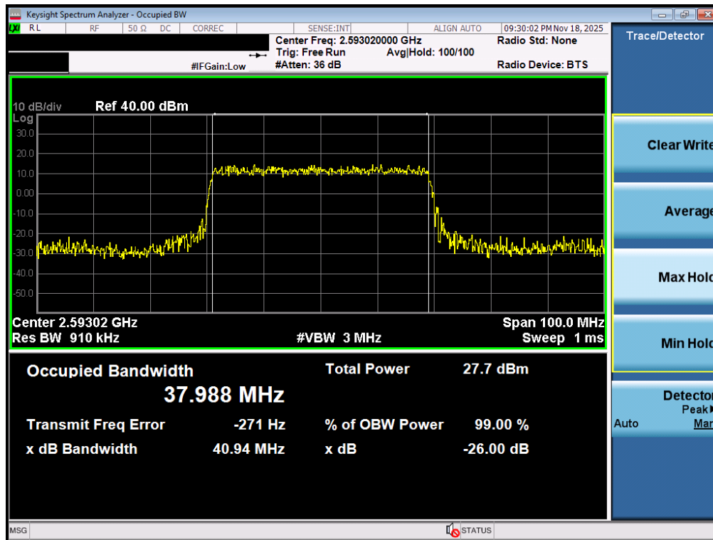
Plot 7-86. Occupied Bandwidth Plot (NR Band n41 PC3 – 40MHz 16-QAM – Full RB – Ant2)
