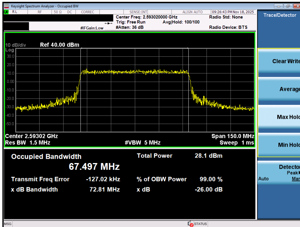
Plot 7-77. Occupied Bandwidth Plot (NR Band n41 PC3 - 70MHz 16-QAM - Full RB - Ant2)
