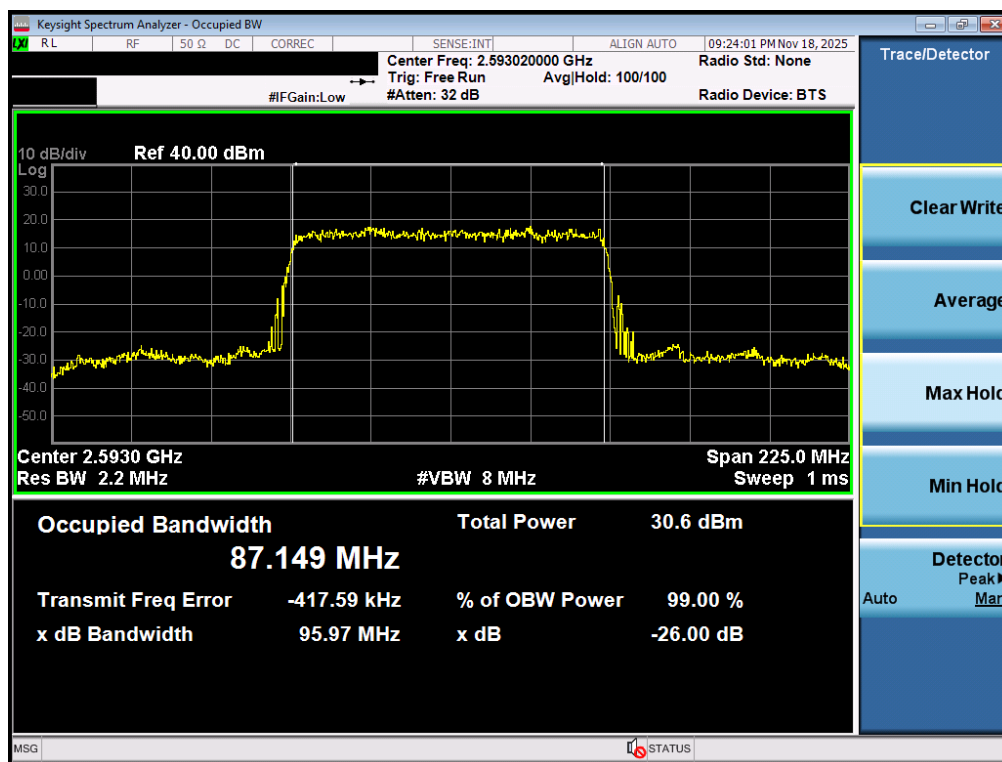
Plot 7-69. Occupied Bandwidth Plot (NR Band n41 PC3 – 90MHz \pi/2 BPSK – Full RB – Ant2)
