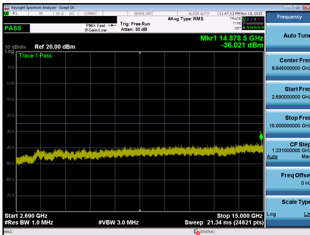
Plot 7-100. Conducted Spurious Plot (LTE Band 41(PC2)- 20MHz QPSK - RB Size 1, RB Offset 50 - Mid Channel - Ant1)
