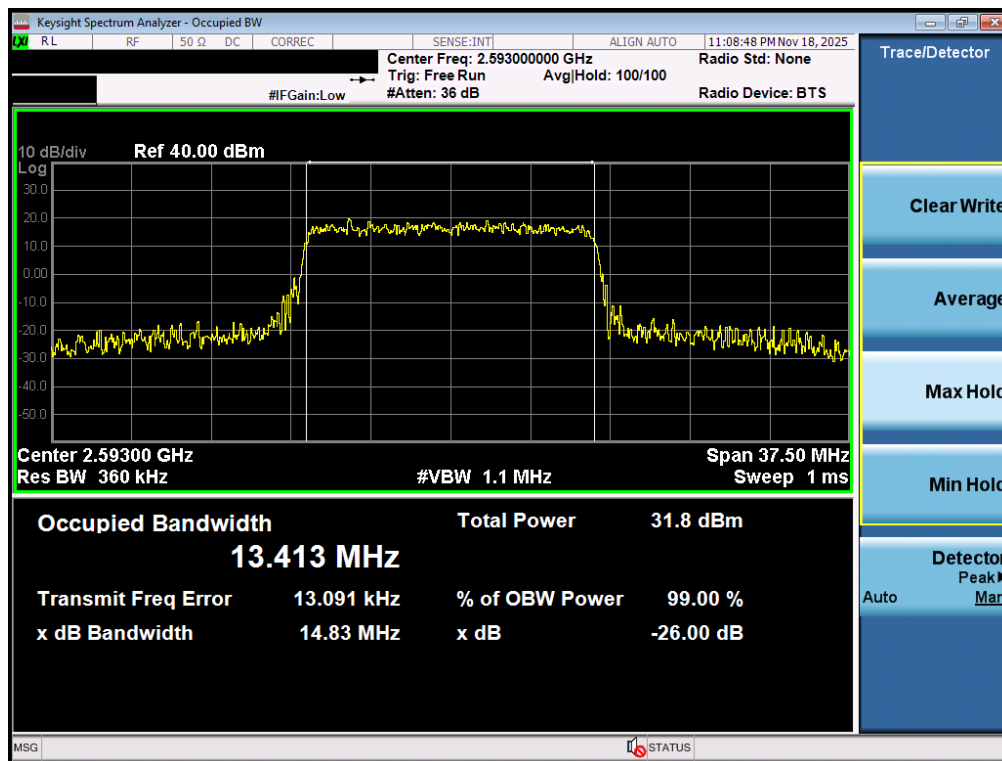
Plot 7-52. Occupied Bandwidth Plot (LTE Band 41(PC2)- 15MHz QPSK - Full RB - Ant2)
