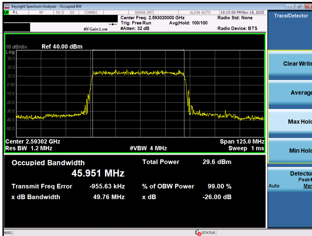
Plot 7-32. Occupied Bandwidth Plot (NR Band n41 PC3 – 50MHz \pi/2 BPSK – Full RB – Ant1)
