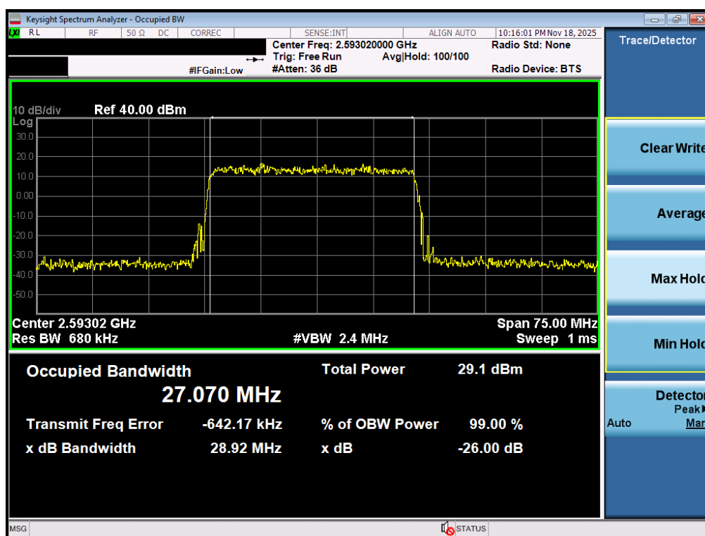
Plot 7-38. Occupied Bandwidth Plot (NR Band n41 PC3 – 30MHz \pi/2 BPSK – Full RB – Ant1)
