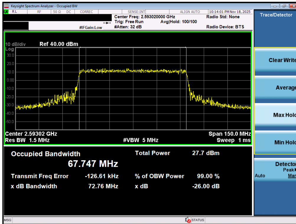
Plot 7-27. Occupied Bandwidth Plot (NR Band n41 PC3 - 70MHz QPSK - Full RB - Ant1)
