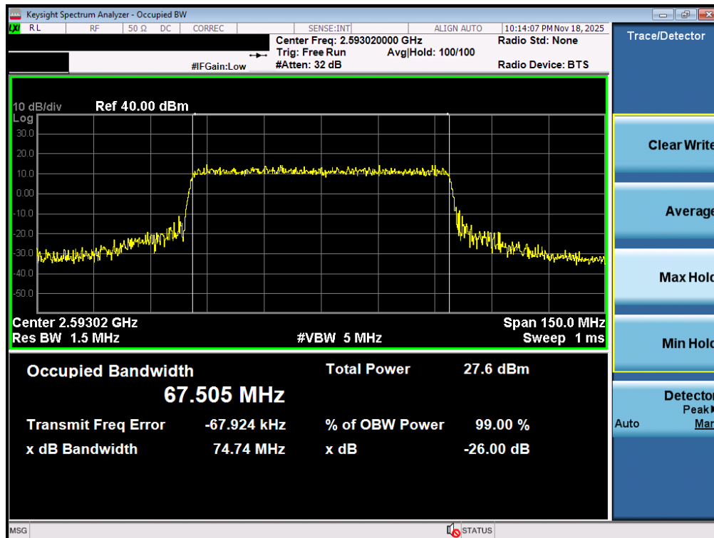
Plot 7-28. Occupied Bandwidth Plot (NR Band n41 PC3 - 70MHz 16-QAM - Full RB - Ant1)
