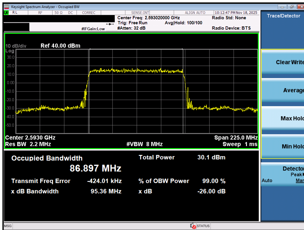
Plot 7-20. Occupied Bandwidth Plot (NR Band n41 PC3 – 90MHz \pi/2 BPSK – Full RB – Ant1)
