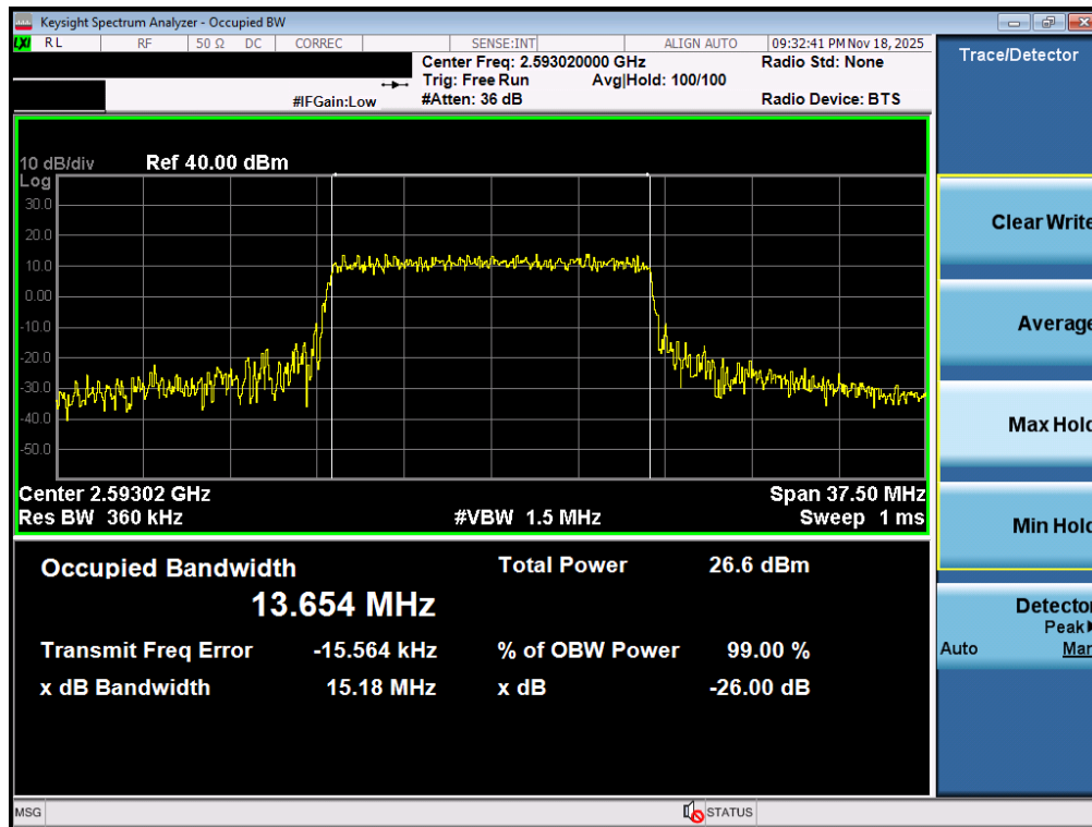
Plot 7-94. Occupied Bandwidth Plot (NR Band n41 PC3 - 15MHz QPSK - Full RB - Ant2)
