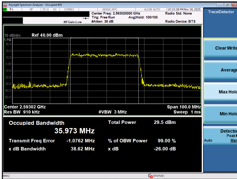
Plot 7-35. Occupied Bandwidth Plot (NR Band n41 PC3 – 40MHz \pi/2 BPSK – Full RB – Ant1)
