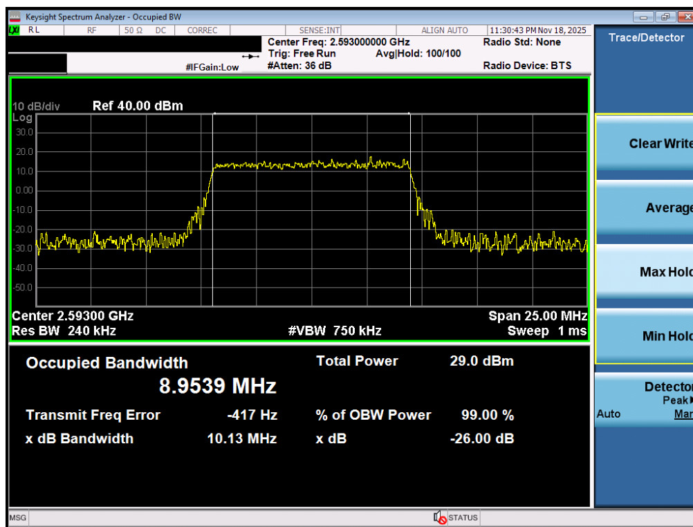
Plot 7-63. Occupied Bandwidth Plot (LTE Band 41(PC3)- 10MHz 16-QAM - Full RB - Ant2)
