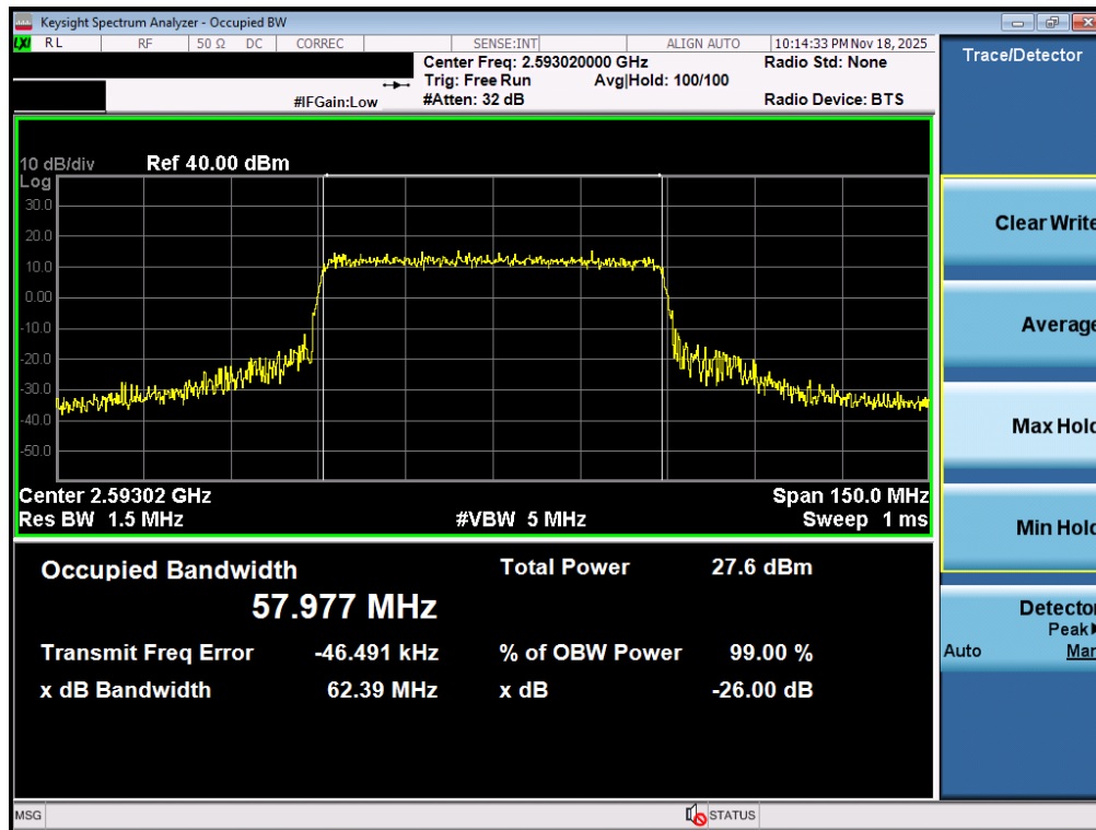
Plot 7-31. Occupied Bandwidth Plot (NR Band n41 PC3 – 60MHz 16-QAM – Full RB – Ant1)
