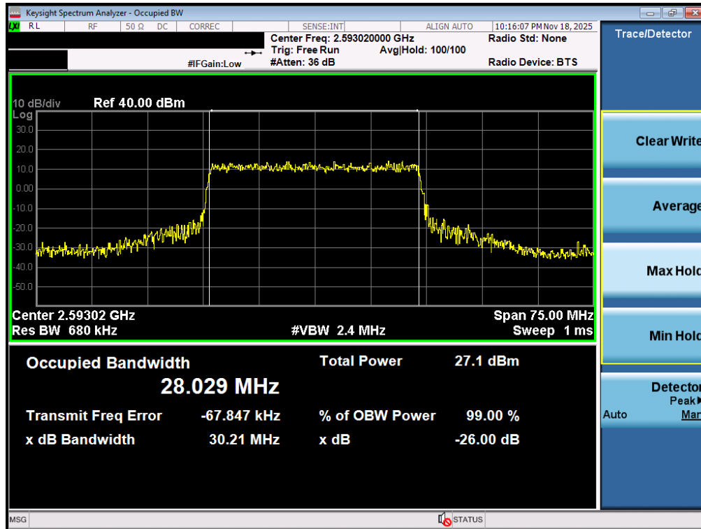
Plot 7-39. Occupied Bandwidth Plot (NR Band n41 PC3 - 30MHz QPSK - Full RB - Ant1)
