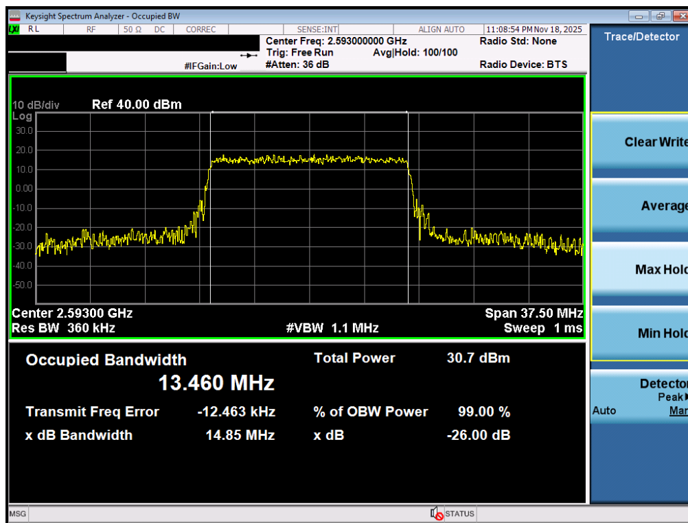
Plot 7-53. Occupied Bandwidth Plot (LTE Band 41(PC2)- 15MHz 16-QAM - Full RB - Ant2)
