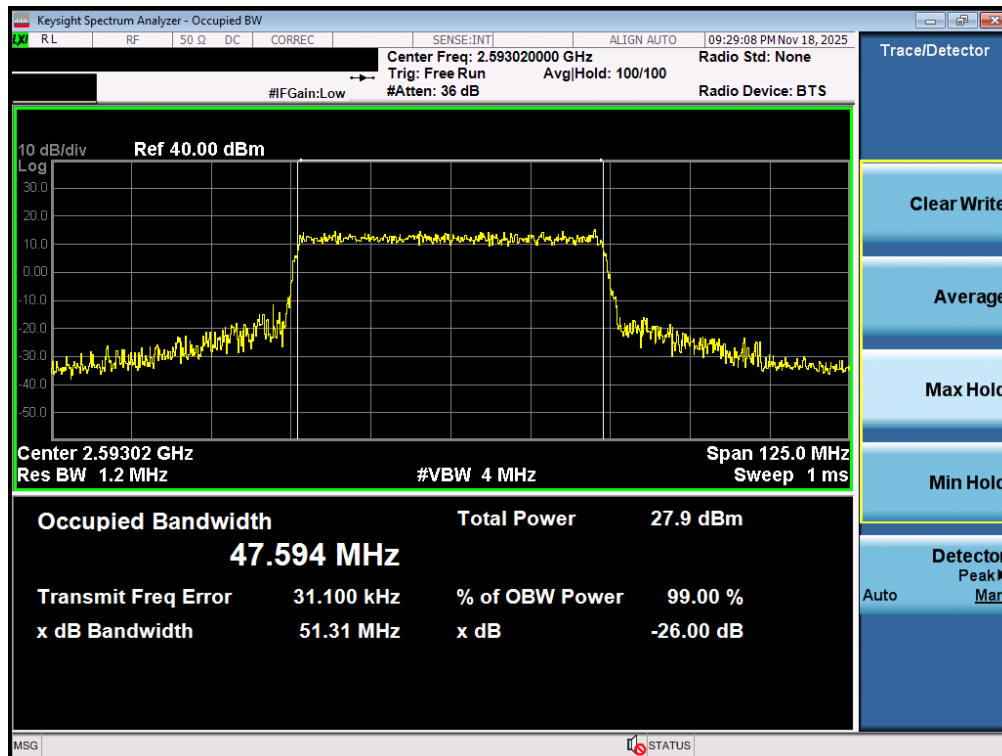
Plot 7-83. Occupied Bandwidth Plot (NR Band n41 PC3 – 50MHz 16-QAM – Full RB – Ant2)
