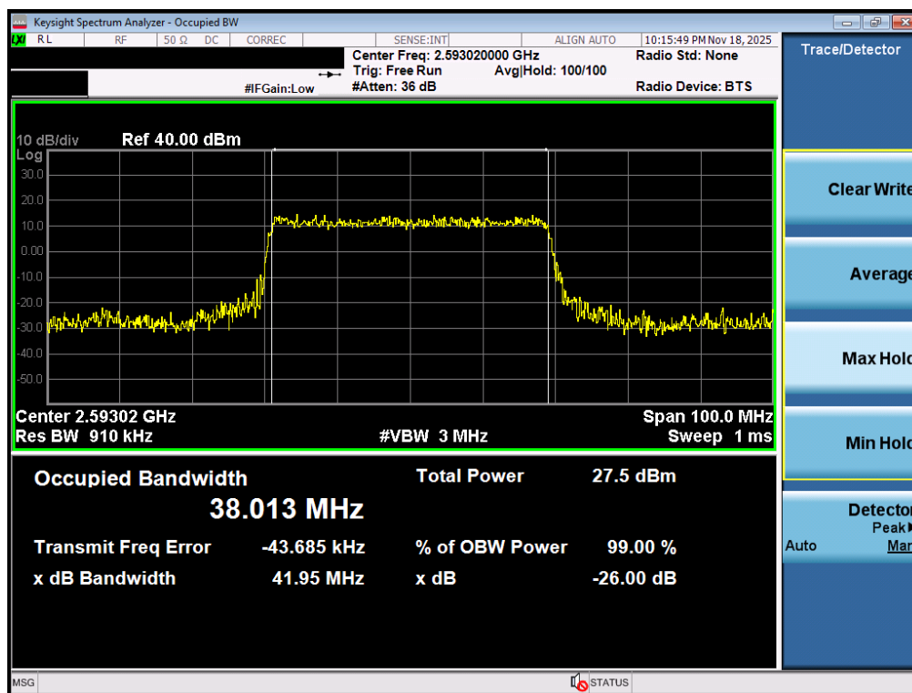
Plot 7-37. Occupied Bandwidth Plot (NR Band n41 PC3 – 40MHz 16-QAM – Full RB – Ant1)
