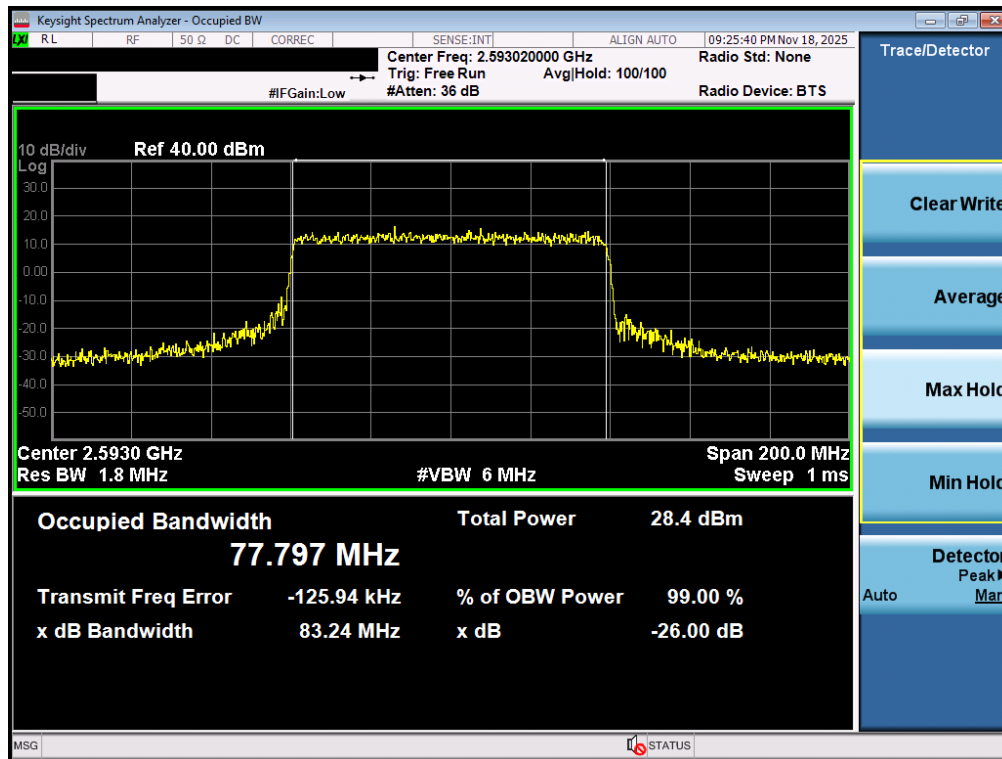
Plot 7-74. Occupied Bandwidth Plot (NR Band n41 PC3 – 80MHz 16-QAM – Full RB – Ant2)
