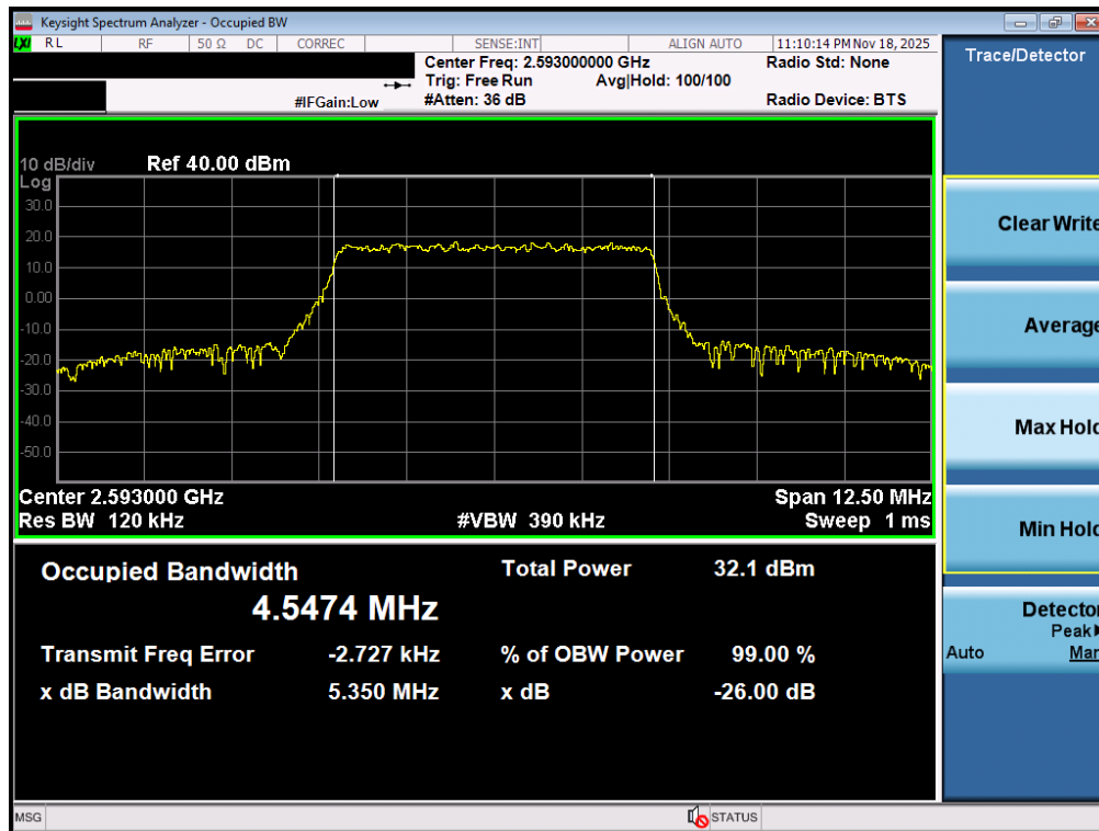
Plot 7-57. Occupied Bandwidth Plot (LTE Band 41(PC2)- 5MHz 16-QAM - Full RB - Ant2)
