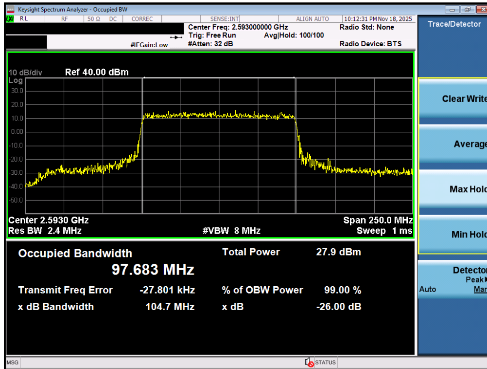
Plot 7-19. Occupied Bandwidth Plot (NR Band n41 PC3 – 100MHz 16-QAM – Full RB – Ant1)
