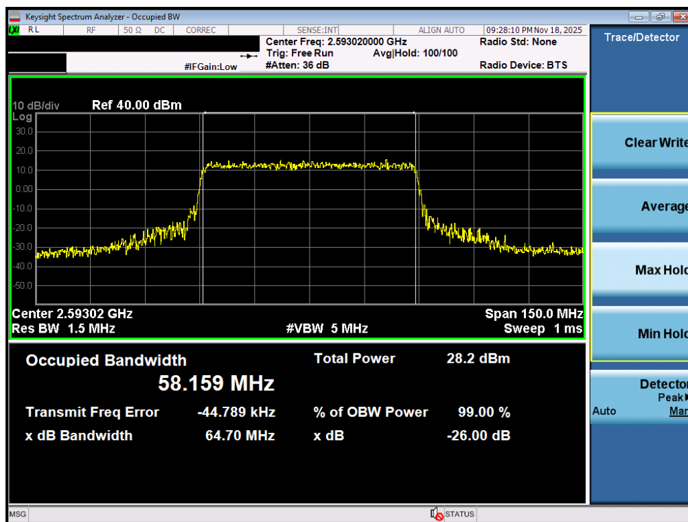
Plot 7-80. Occupied Bandwidth Plot (NR Band n41 PC3 – 60MHz 16-QAM – Full RB – Ant2)
