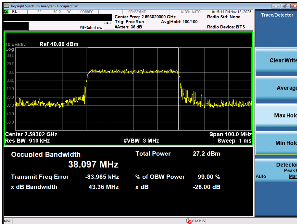
Plot 7-36. Occupied Bandwidth Plot (NR Band n41 PC3 – 40MHz QPSK – Full RB – Ant1)
