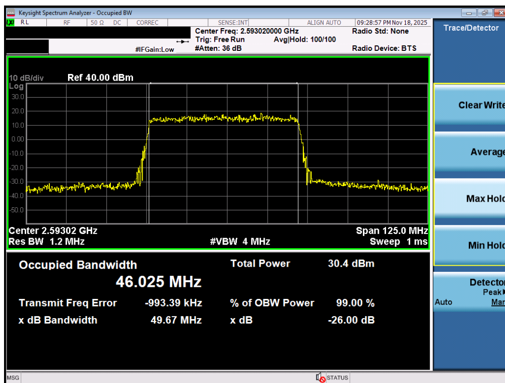
Plot 7-81. Occupied Bandwidth Plot (NR Band n41 PC3 – 50MHz \pi/2 BPSK – Full RB – Ant2)
