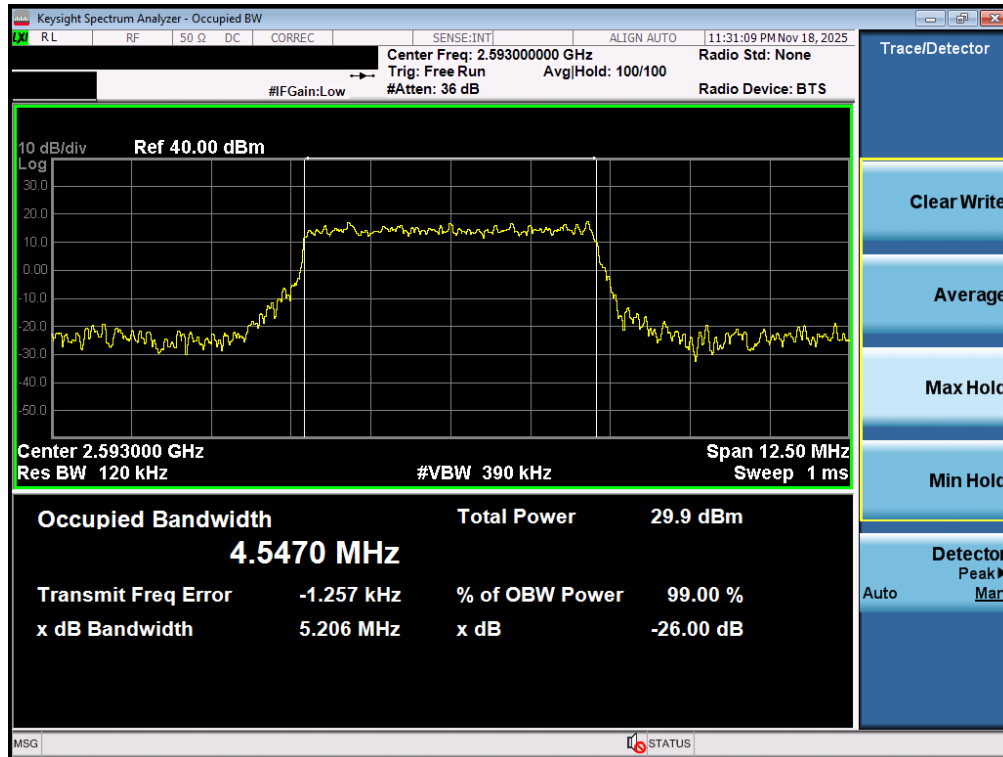
Plot 7-64. Occupied Bandwidth Plot (LTE Band 41(PC3)- 5MHz QPSK - Full RB - Ant2)
