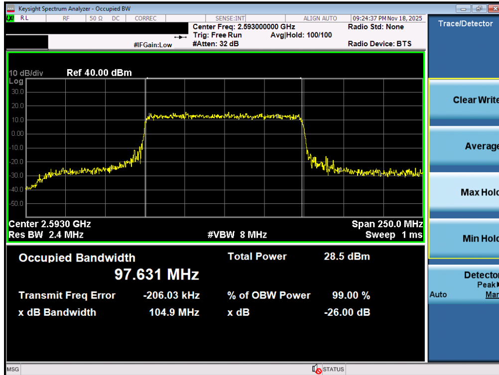
Plot 7-67. Occupied Bandwidth Plot (NR Band n41 PC3 – 100MHz QPSK – Full RB – Ant2)
