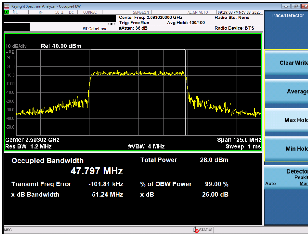
Plot 7-82. Occupied Bandwidth Plot (NR Band n41 PC3 – 50MHz QPSK – Full RB – Ant2)
