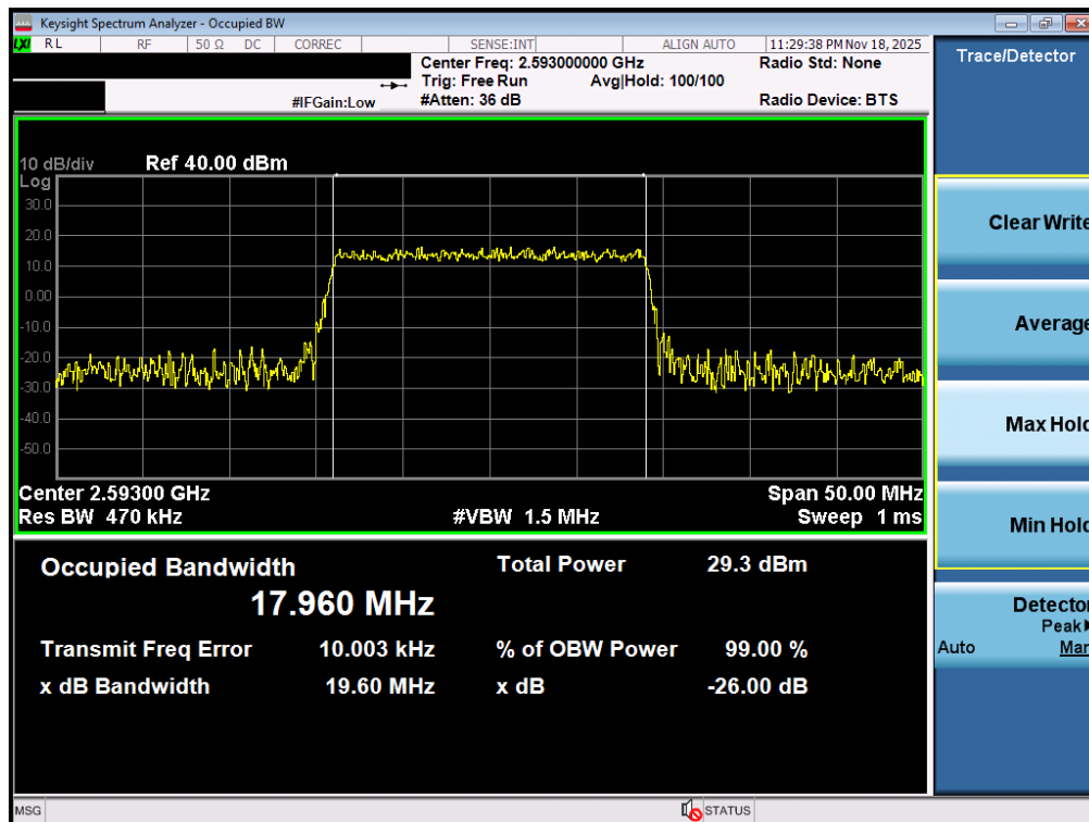
Plot 7-59. Occupied Bandwidth Plot (LTE Band 41(PC3)- 20MHz 16-QAM - Full RB - Ant2)
