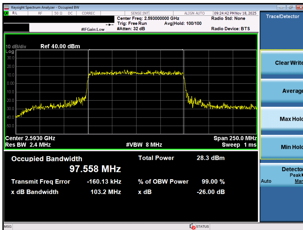
Plot 7-68. Occupied Bandwidth Plot (NR Band n41 PC3 – 100MHz 16-QAM – Full RB – Ant2)
