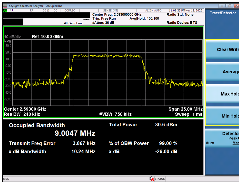
Plot 7-55. Occupied Bandwidth Plot (LTE Band 41(PC2)- 10MHz 16-QAM - Full RB - Ant2)
