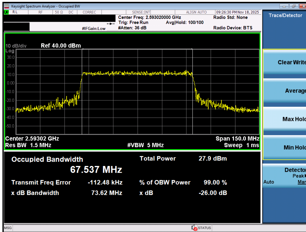
Plot 7-76. Occupied Bandwidth Plot (NR Band n41 PC3 - 70MHz QPSK - Full RB - Ant2)
