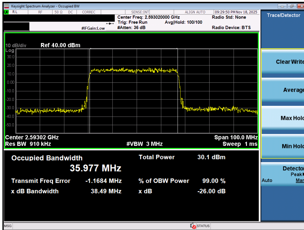
Plot 7-84. Occupied Bandwidth Plot (NR Band n41 PC3 – 40MHz \pi/2 BPSK – Full RB – Ant2)
