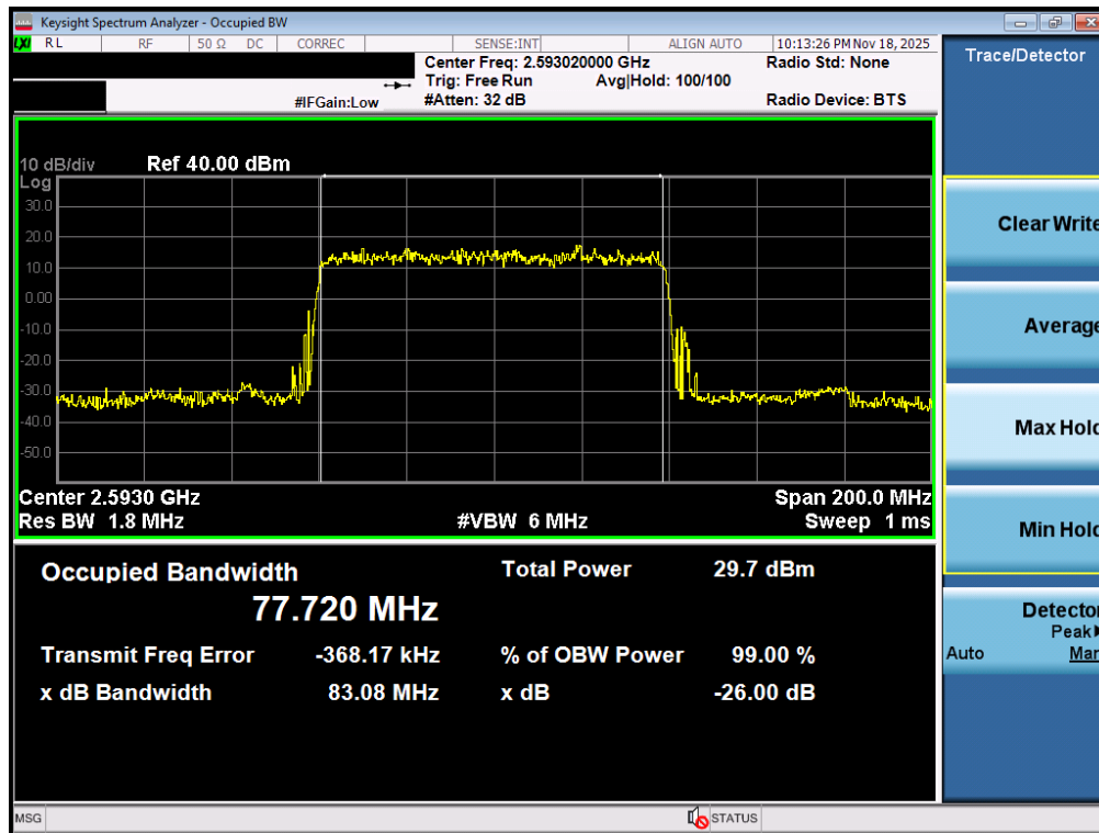
Plot 7-23. Occupied Bandwidth Plot (NR Band n41 PC3 – 80MHz \pi/2 BPSK – Full RB – Ant1)
