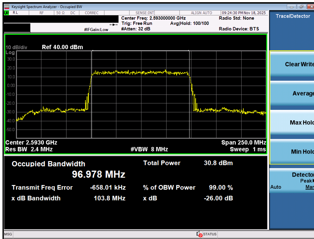
Plot 7-66. Occupied Bandwidth Plot (NR Band n41 PC3 – 100MHz \pi/2 BPSK – Full RB – Ant2)
