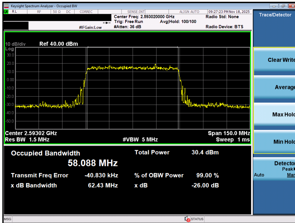
Plot 7-78. Occupied Bandwidth Plot (NR Band n41 PC3 – 60MHz \pi/2 BPSK – Full RB – Ant2)
