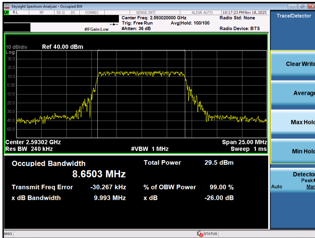
Plot 7-47. Occupied Bandwidth Plot (NR Band n41 PC3 – 10MHz \pi/2 BPSK – Full RB – Ant1)
