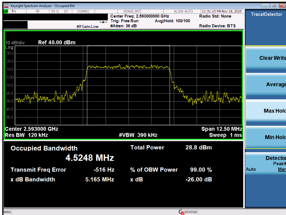
Plot 7-65. Occupied Bandwidth Plot (LTE Band 41(PC3)- 5MHz 16-QAM - Full RB - Ant2)
