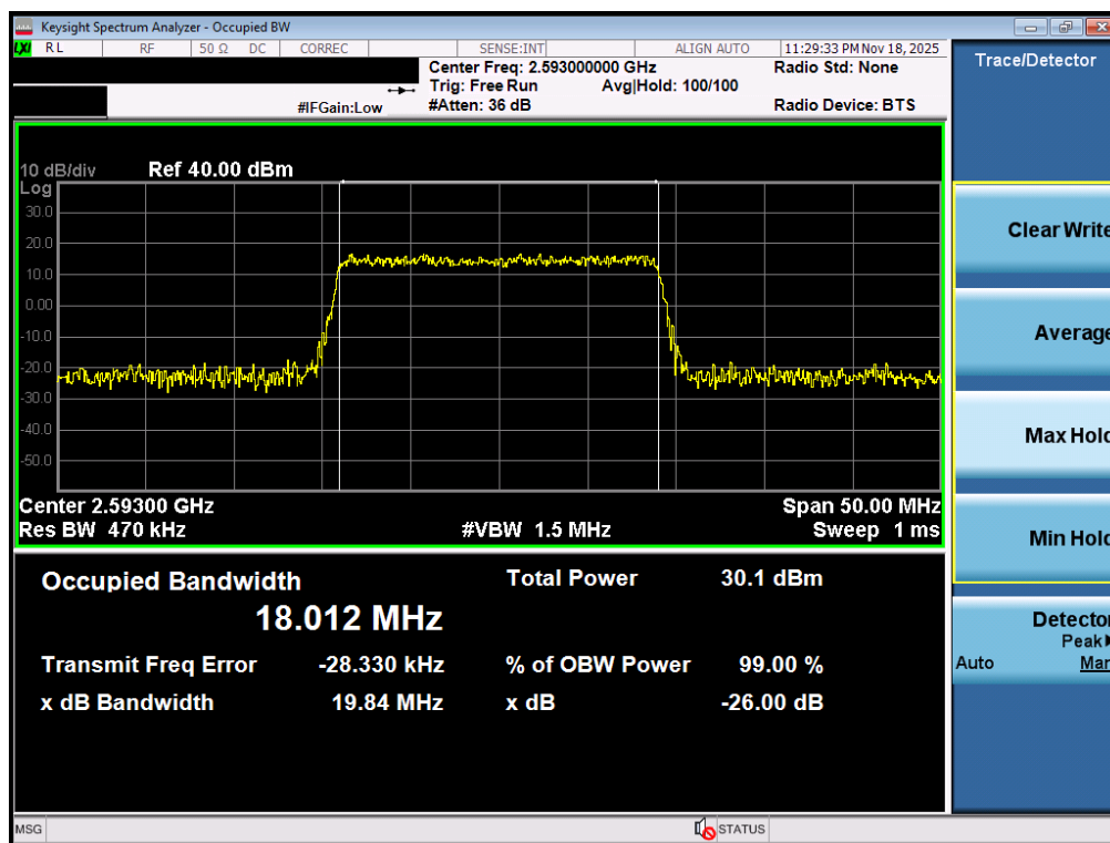
Plot 7-58. Occupied Bandwidth Plot (LTE Band 41(PC3)- 20MHz QPSK - Full RB - Ant2)
