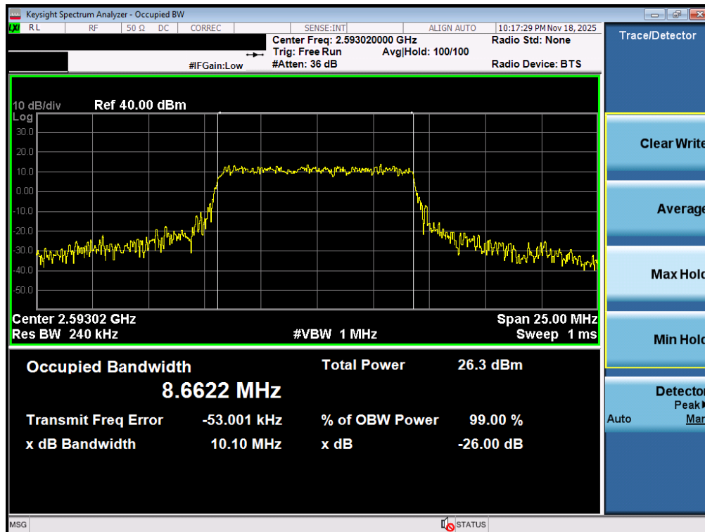
Plot 7-48. Occupied Bandwidth Plot (NR Band n41 PC3 – 10MHz QPSK – Full RB – Ant1)
