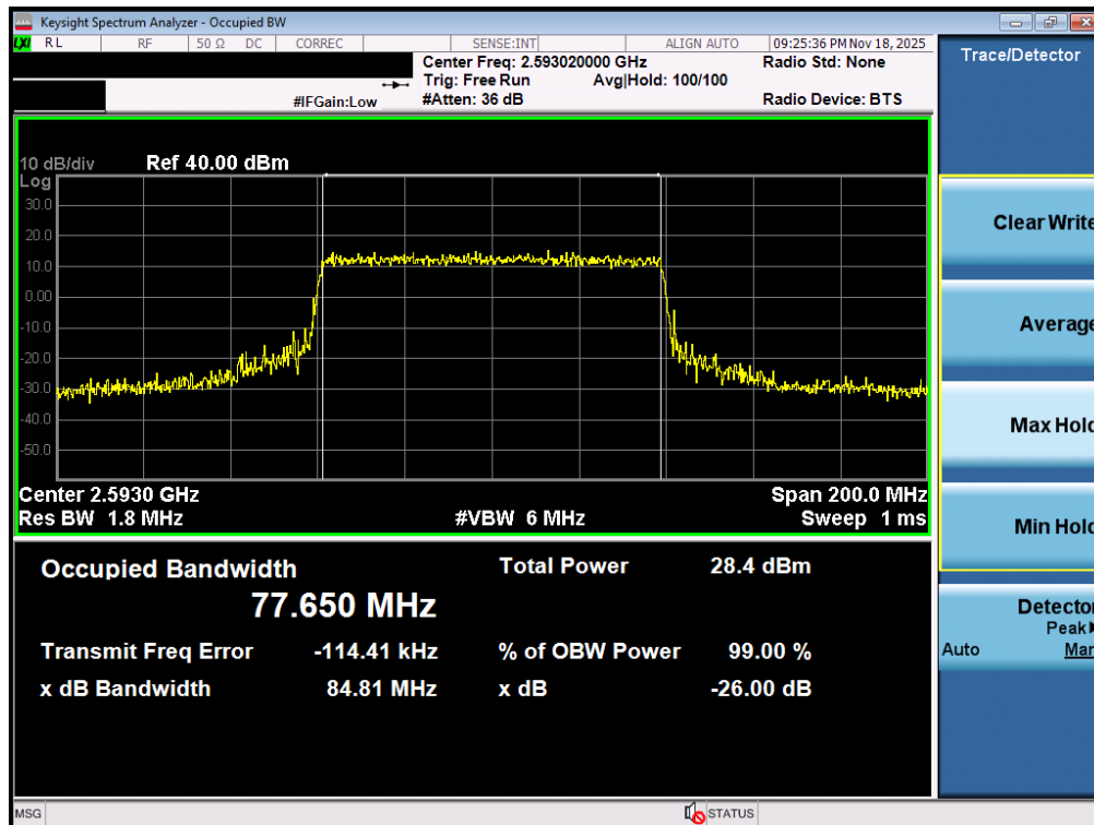
Plot 7-73. Occupied Bandwidth Plot (NR Band n41 PC3 – 80MHz QPSK – Full RB – Ant2)
