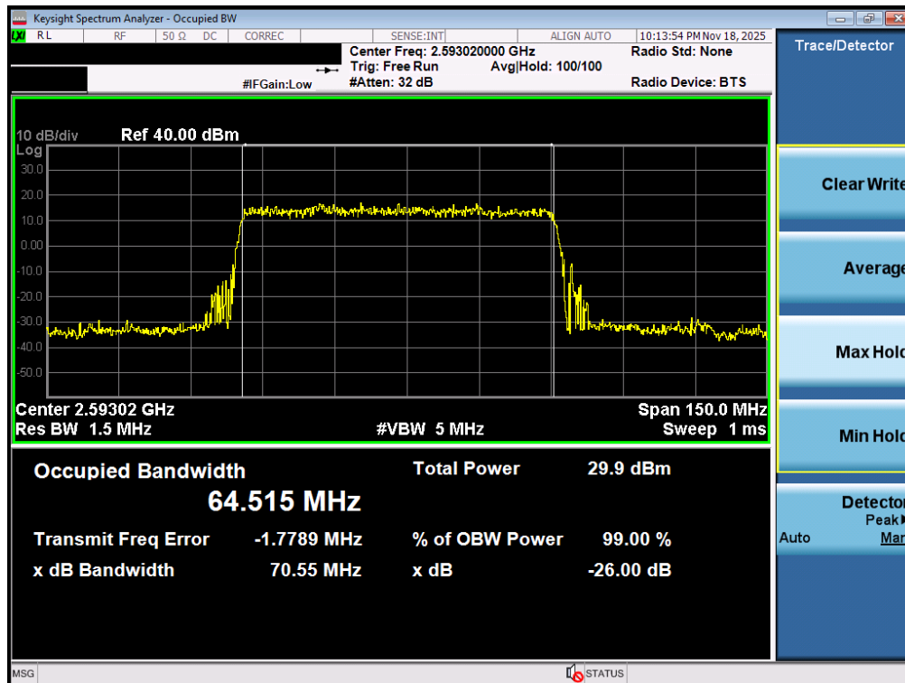
Plot 7-26. Occupied Bandwidth Plot (NR Band n41 PC3 – 70MHz \pi/2 BPSK – Full RB – Ant1)
