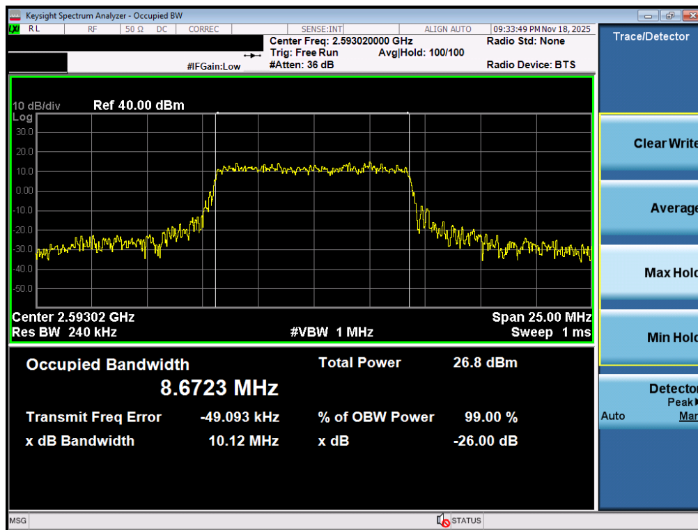
Plot 7-98. Occupied Bandwidth Plot (NR Band n41 PC3 – 10MHz 16-QAM – Full RB – Ant2)
