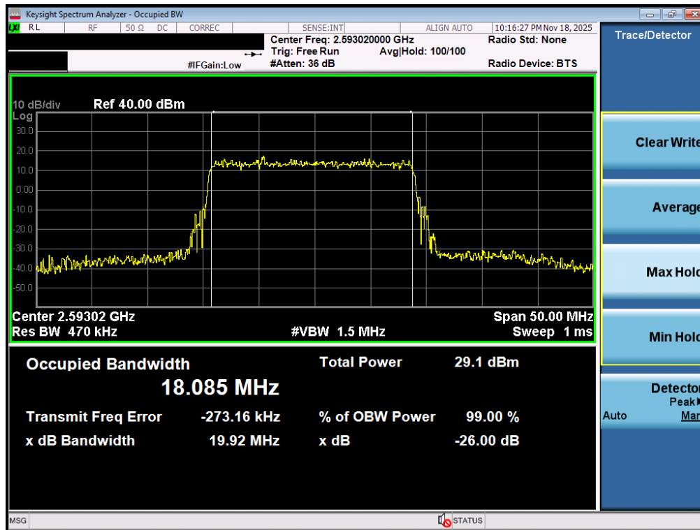
Plot 7-41. Occupied Bandwidth Plot (NR Band n41 PC3 – 20MHz \pi/2 BPSK – Full RB – Ant1)
