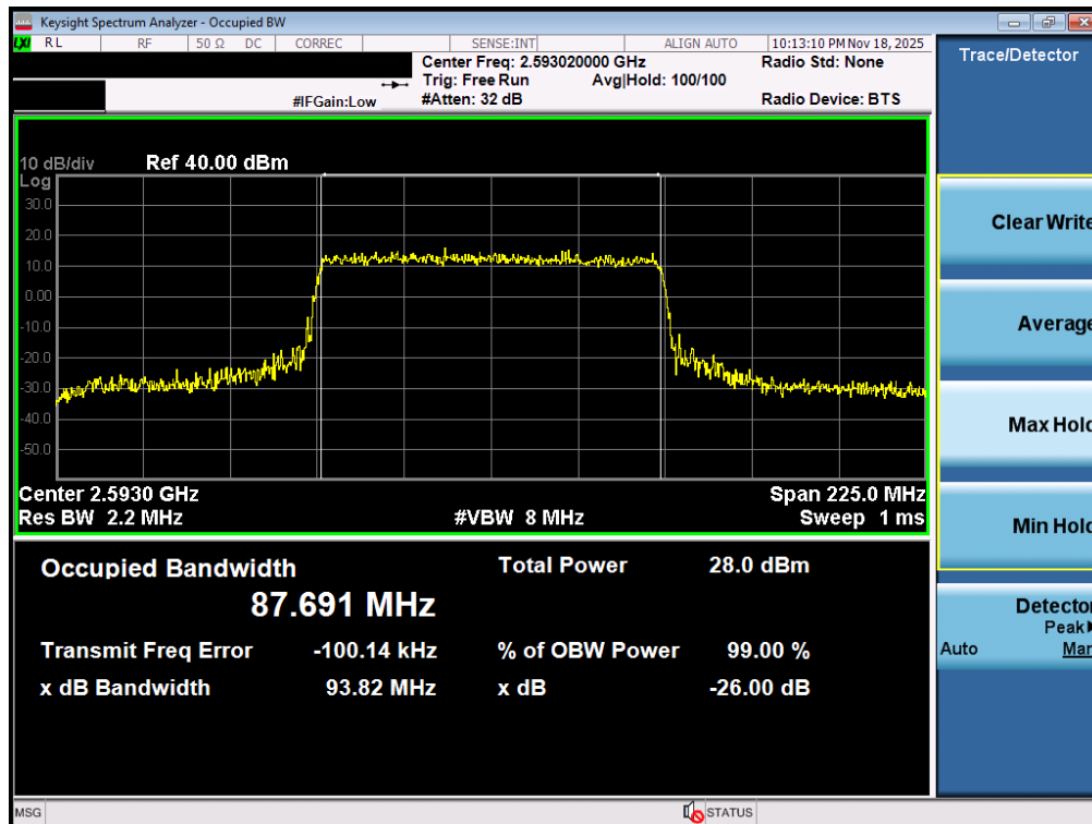
Plot 7-22. Occupied Bandwidth Plot (NR Band n41 PC3 - 90MHz 16-QAM - Full RB - Ant1)
