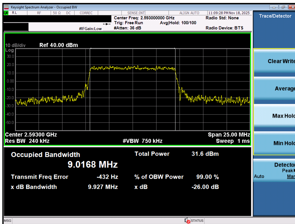
Plot 7-54. Occupied Bandwidth Plot (LTE Band 41(PC2)- 10MHz QPSK - Full RB - Ant2)
