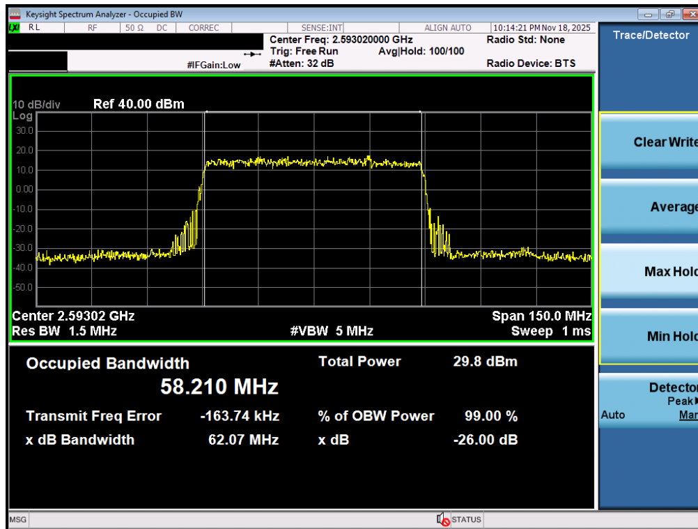
Plot 7-29. Occupied Bandwidth Plot (NR Band n41 PC3 – 60MHz \pi/2 BPSK – Full RB – Ant1)
