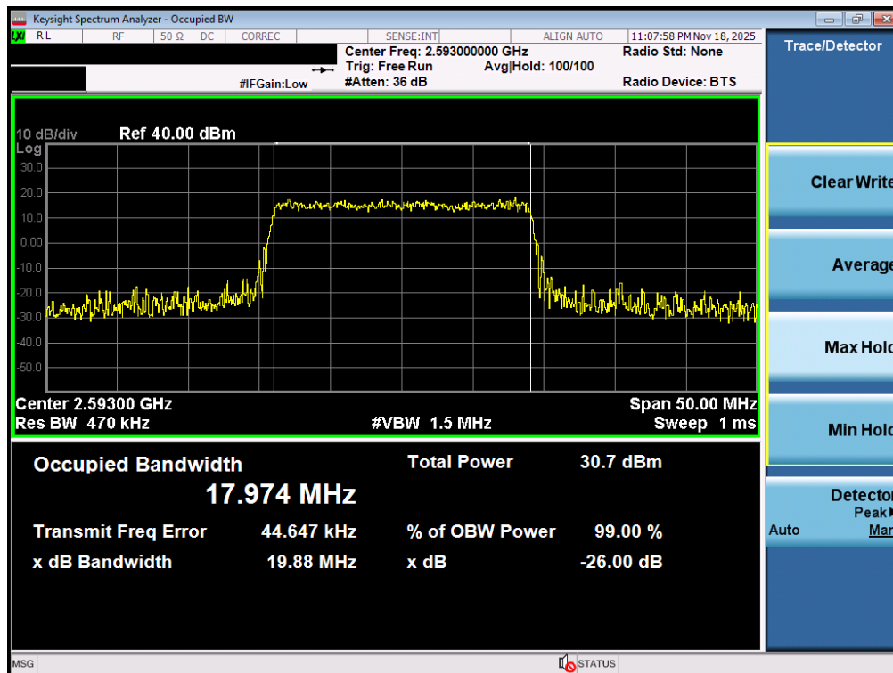
Plot 7-51. Occupied Bandwidth Plot (LTE Band 41(PC2)- 20MHz 16-QAM - Full RB - Ant2)
