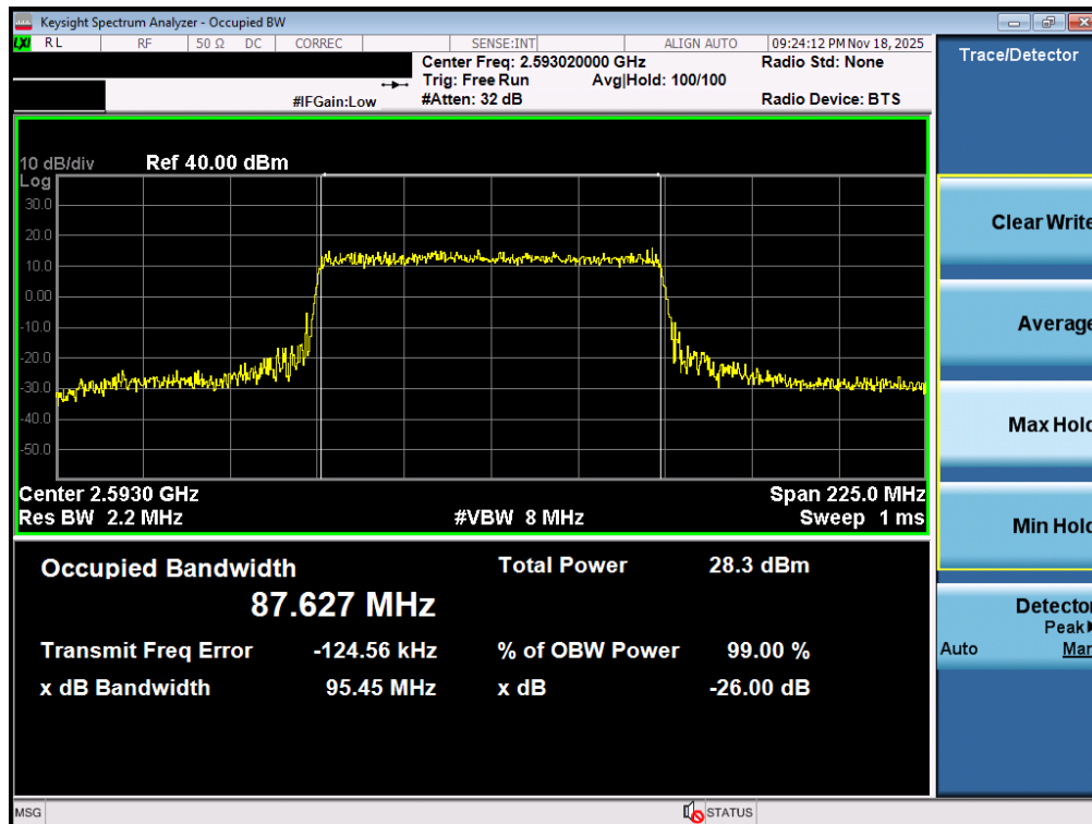
Plot 7-71. Occupied Bandwidth Plot (NR Band n41 PC3 - 90MHz 16-QAM - Full RB - Ant2)
