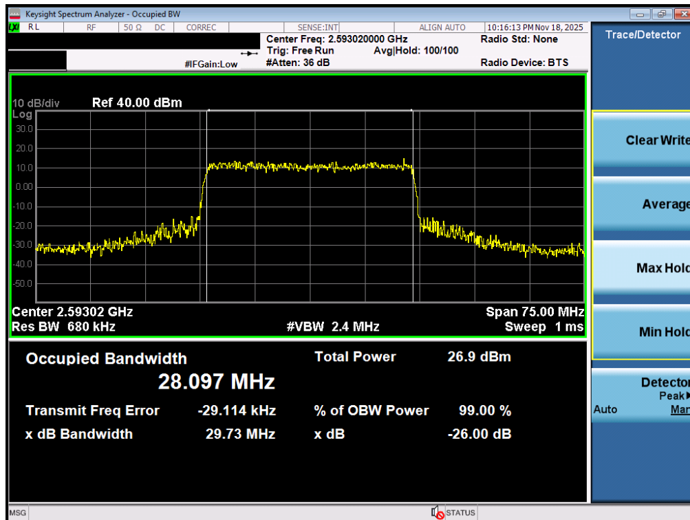
Plot 7-40. Occupied Bandwidth Plot (NR Band n41 PC3 - 30MHz 16-QAM - Full RB - Ant1)
