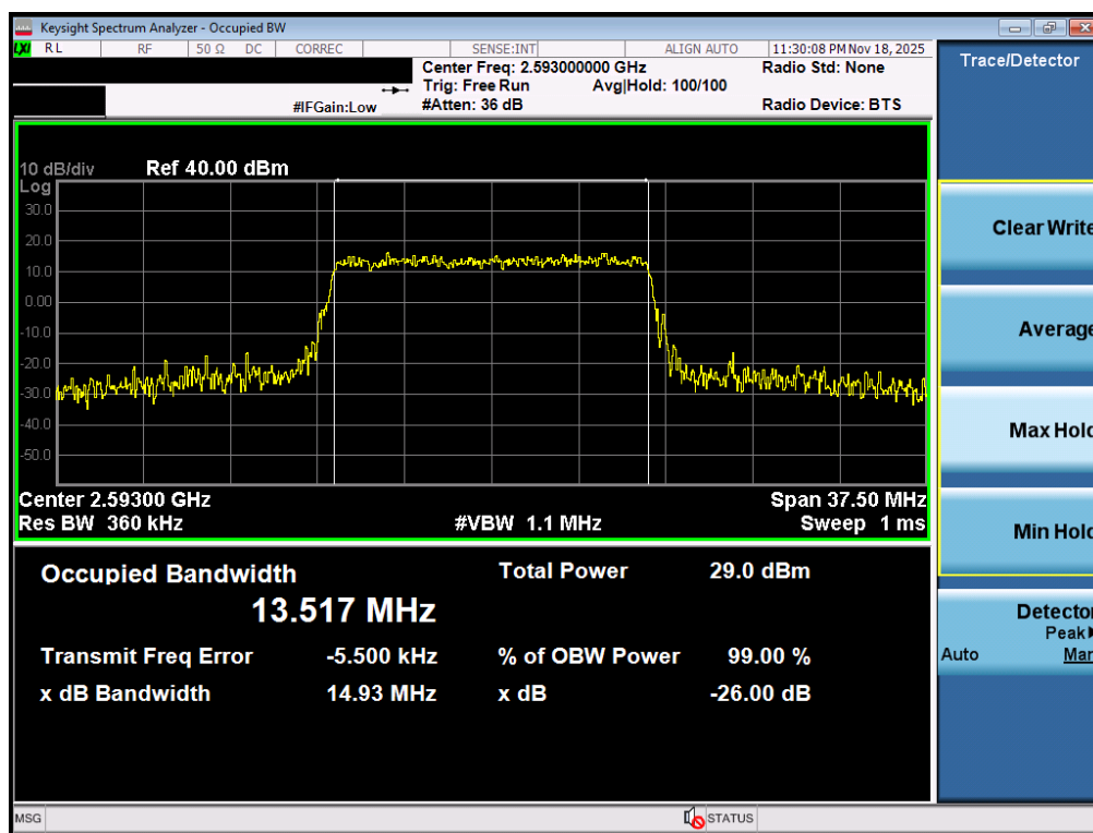
Plot 7-61. Occupied Bandwidth Plot (LTE Band 41(PC3)- 15MHz 16-QAM - Full RB - Ant2)
