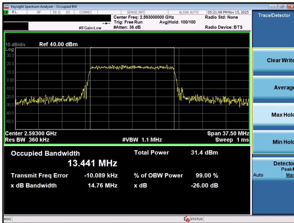
Plot 7-3. Occupied Bandwidth Plot (LTE Band 41(PC2)- 15MHz QPSK - Full RB - Ant1)
