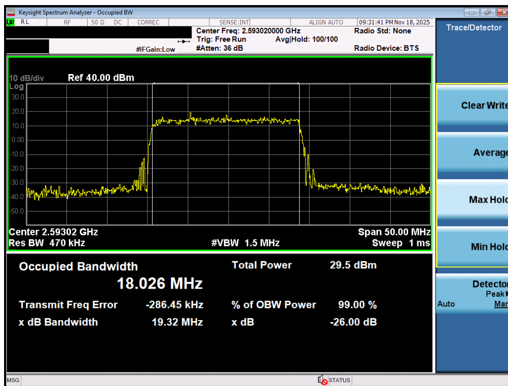
Plot 7-90. Occupied Bandwidth Plot (NR Band n41 PC3 – 20MHz \pi/2 BPSK – Full RB – Ant2)
