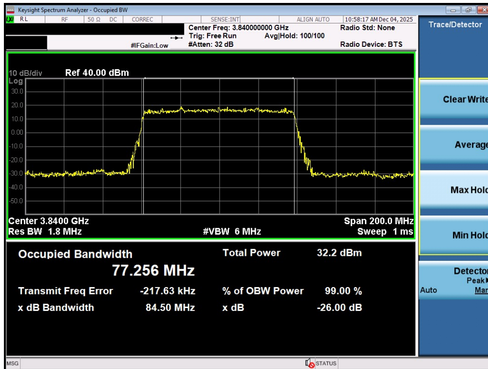
Plot 7-40. Occupied Bandwidth Plot (NR Band n77 - 80MHz \pi/2 BPSK - Full RB - Ant1 - C-Band - Main)
