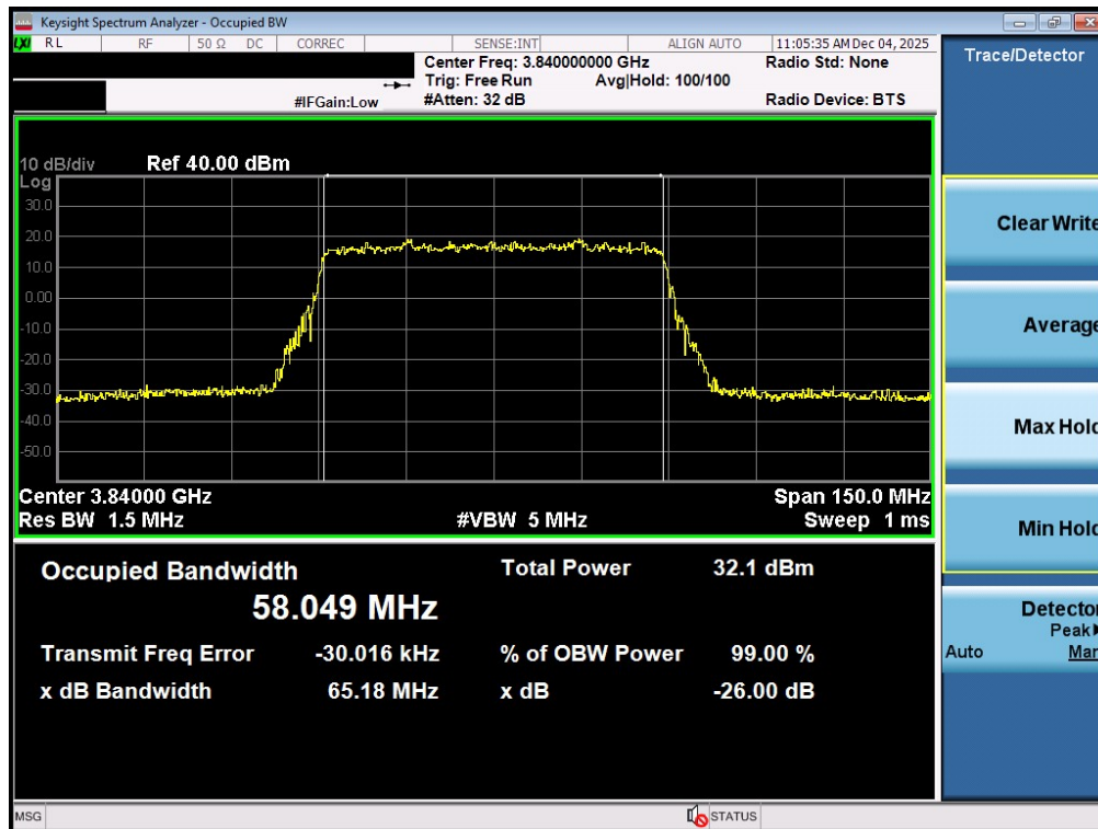
Plot 7-46. Occupied Bandwidth Plot (NR Band n77 - 60MHz \pi/2 BPSK - Full RB - Ant1 - C-Band - Main)
