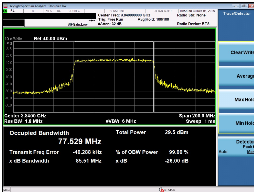
Plot 7-41. Occupied Bandwidth Plot (NR Band n77 - 80MHz QPSK - Full RB - Ant1 - C-Band - Main)
