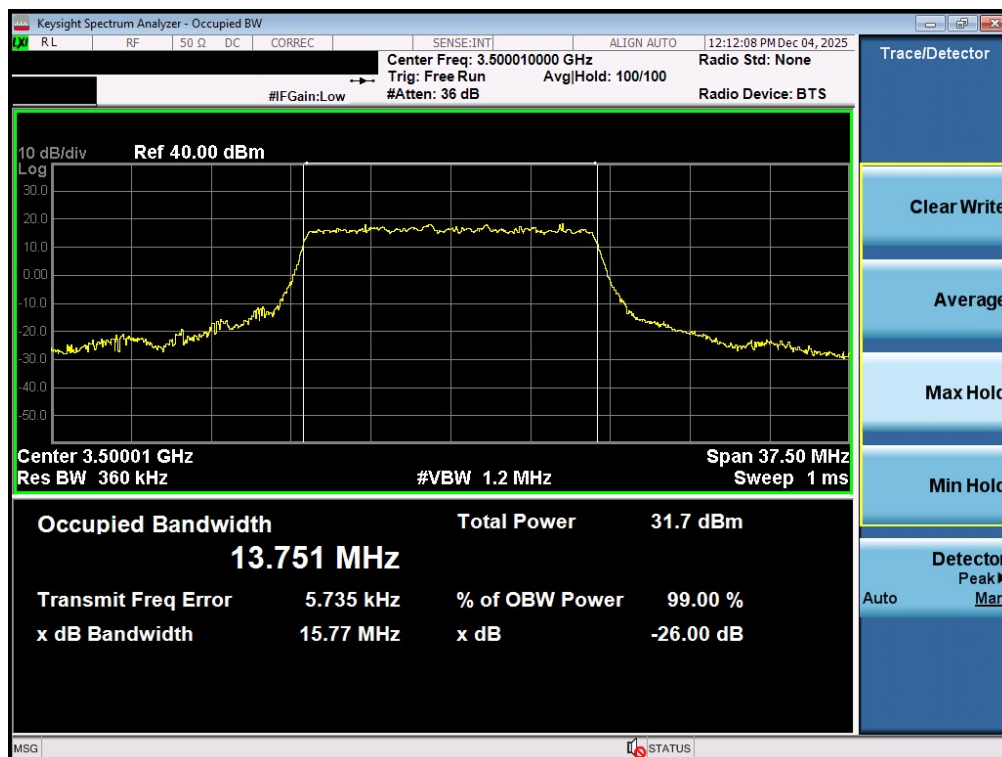
Plot 7-30. Occupied Bandwidth Plot (NR Band n77 - 15MHz 16-QAM - Full RB - Ant1 - DoD Band - Main)
