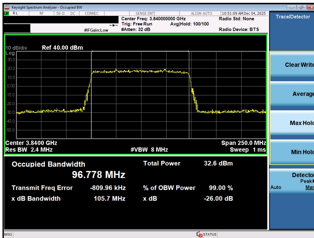
Plot 7-34. Occupied Bandwidth Plot (NR Band n77PC2 - 100MHz \pi/2 BPSK - Full RB - Ant1 - C-Band - Main)
