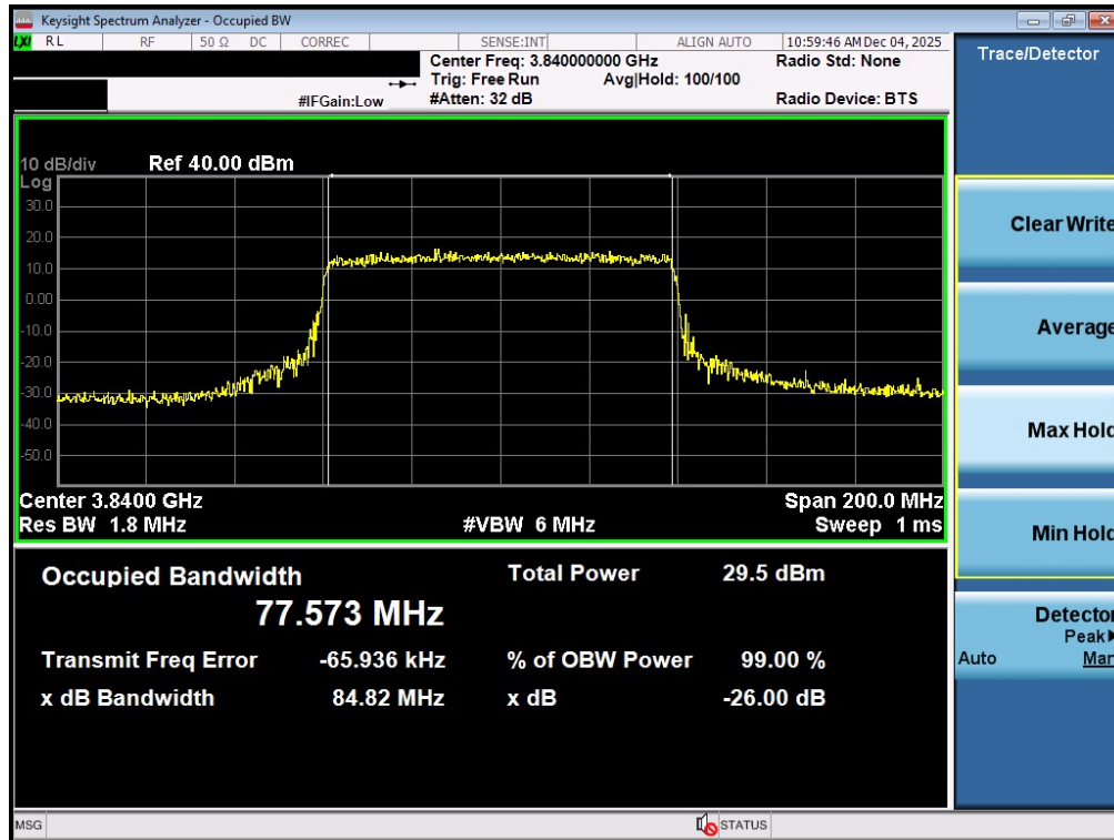
Plot 7-42. Occupied Bandwidth Plot (NR Band n77 - 80MHz 16-QAM - Full RB - Ant1 - C-Band - Main)
