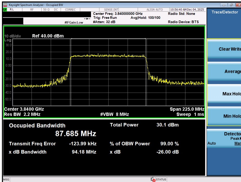
Plot 7-39. Occupied Bandwidth Plot (NR Band n77 - 90MHz 16-QAM - Full RB - Ant1 - C-Band - Main)
