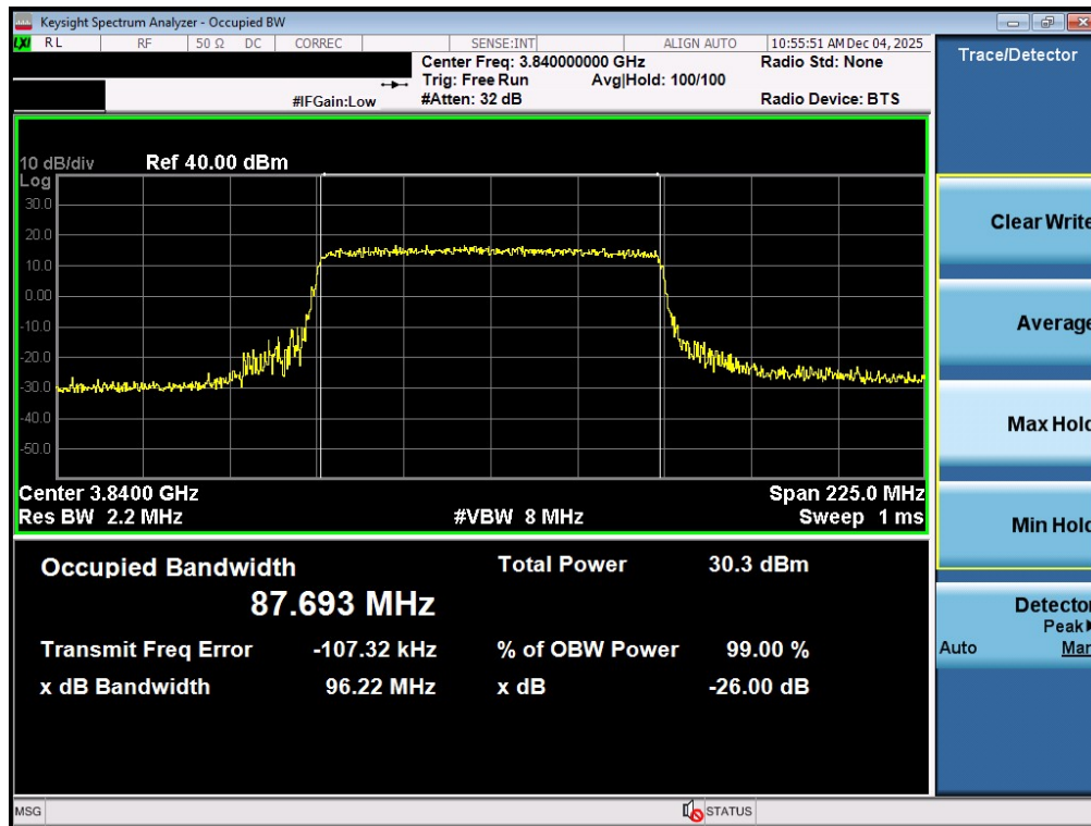
Plot 7-38. Occupied Bandwidth Plot (NR Band n77 - 90MHz QPSK - Full RB - Ant1 - C-Band - Main)
