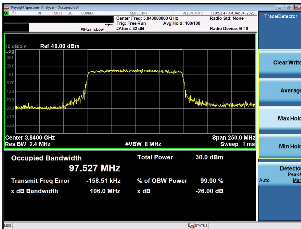
Plot 7-36. Occupied Bandwidth Plot (NR Band n77PC2 - 100MHz 16-QAM - Full RB - Ant1 - C-Band - Main)
