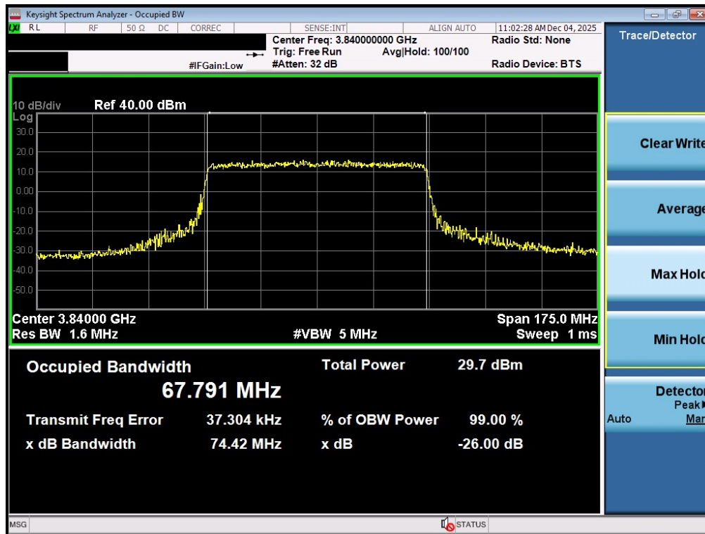
Plot 7-44. Occupied Bandwidth Plot (NR Band n77 - 70MHz QPSK - Full RB - Ant1 - C-Band - Main)
