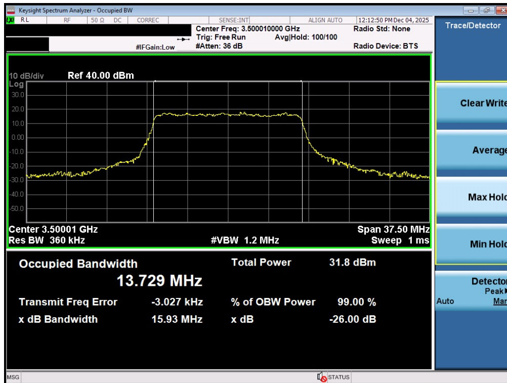
Plot 7-29. Occupied Bandwidth Plot (NR Band n77 - 15MHz QPSK - Full RB - Ant1 - DoD Band - Main)
