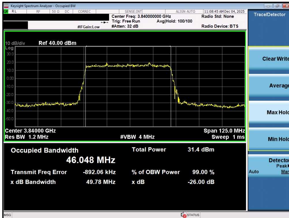
Plot 7-49. Occupied Bandwidth Plot (NR Band n77 - 50MHz \pi/2 BPSK - Full RB - Ant1 - C-Band - Main)
