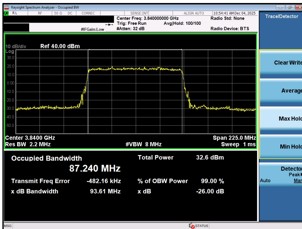
Plot 7-37. Occupied Bandwidth Plot (NR Band n77 - 90MHz \pi/2 BPSK - Full RB - Ant1 - C-Band - Main)
