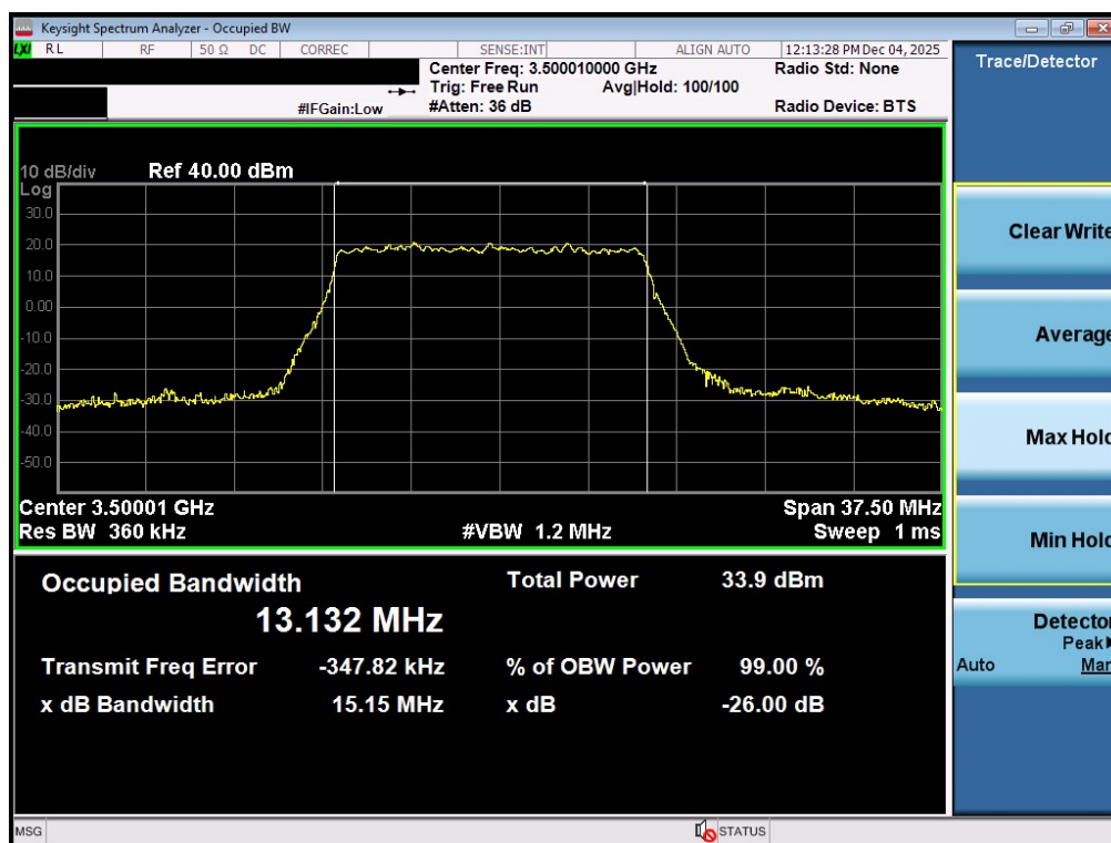
Plot 7-28. Occupied Bandwidth Plot (NR Band n77 - 15MHz \pi/2 BPSK - Full RB - Ant1 - DoD Band - Main)
