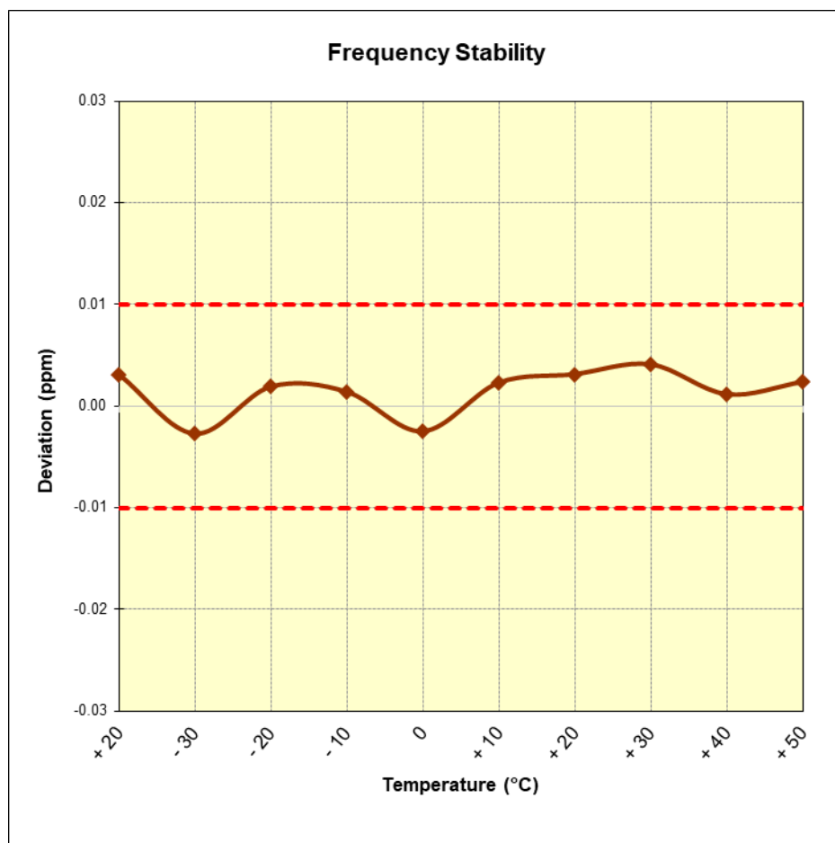
Figure 7-3. Frequency Stability Plot
